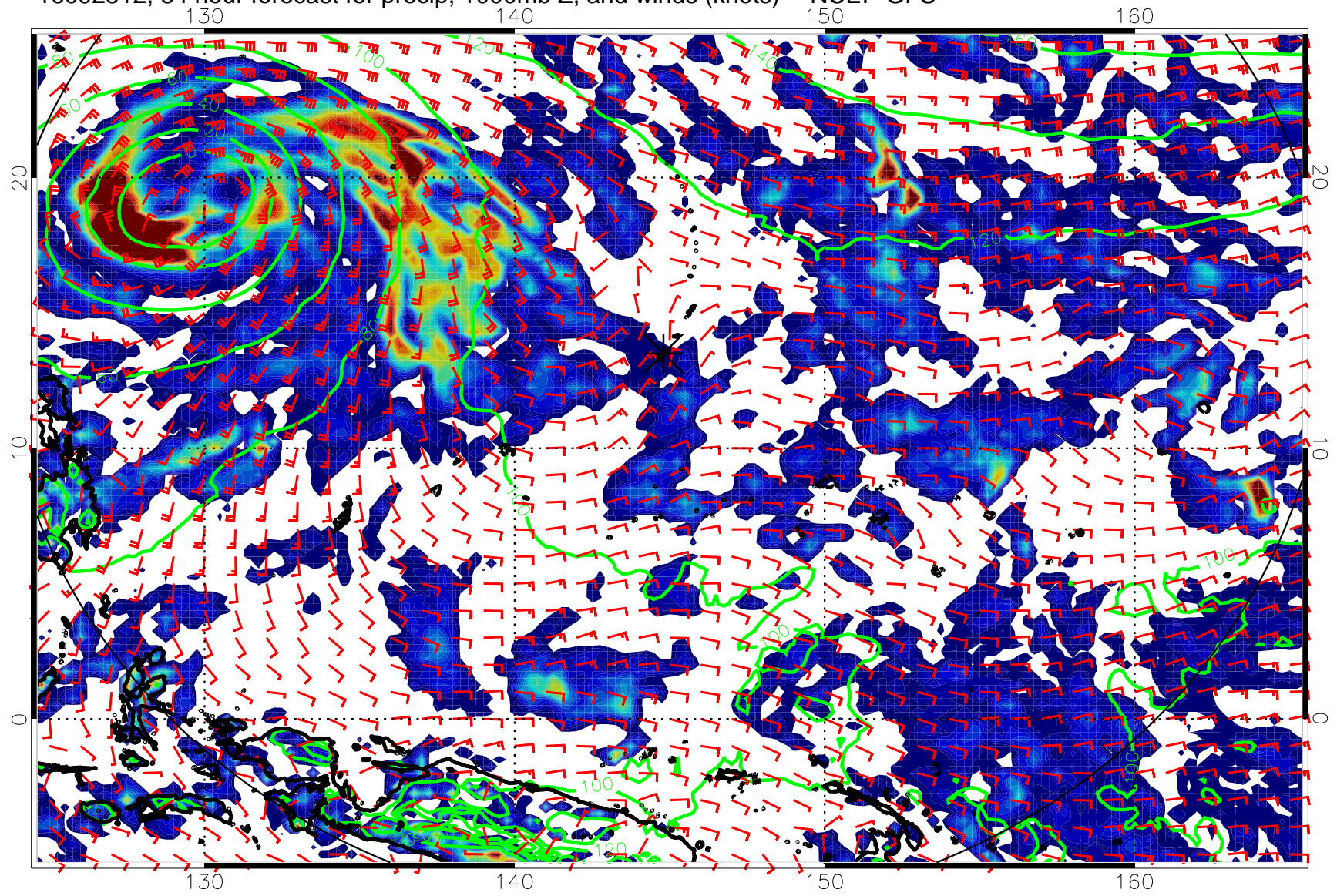
16092512, 84 hour forecast for precip, 1000mb Z, and winds (knots) -- NCEP GFS
