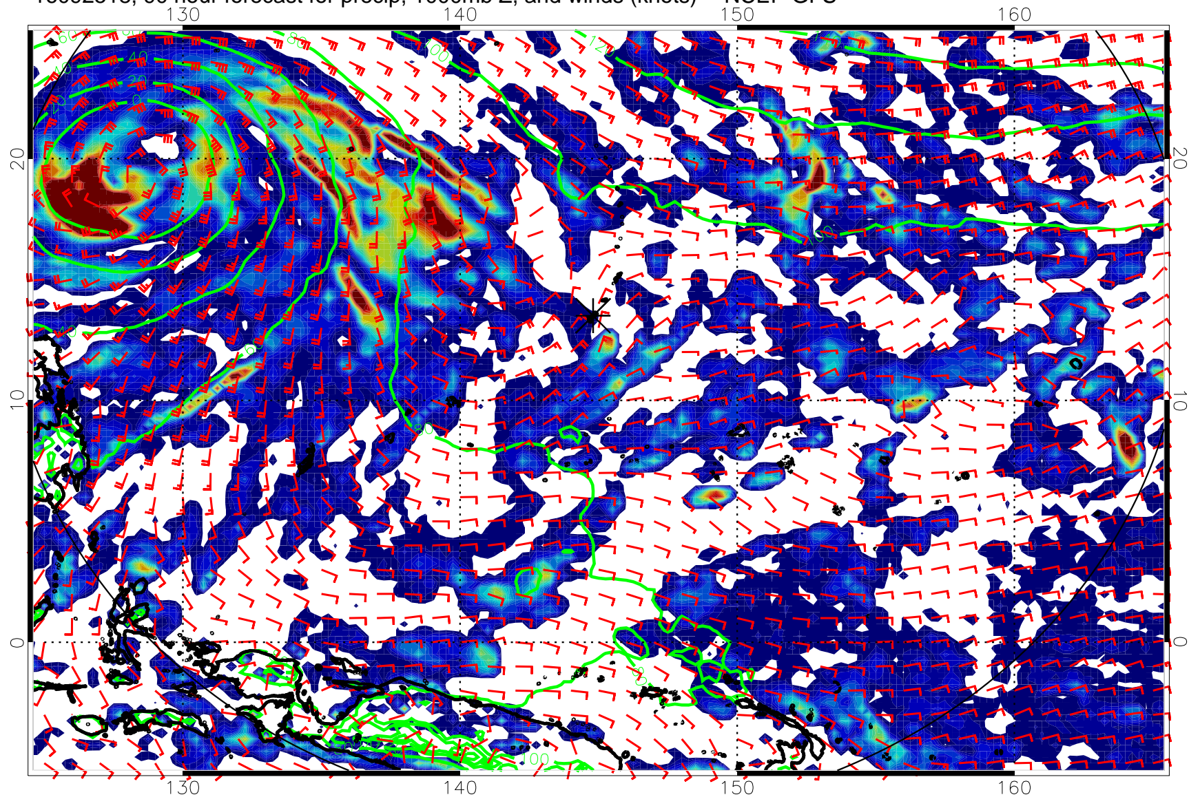
16092518, 90 hour forecast for precip, 1000mb Z, and winds (knots) -- NCEP GFS
