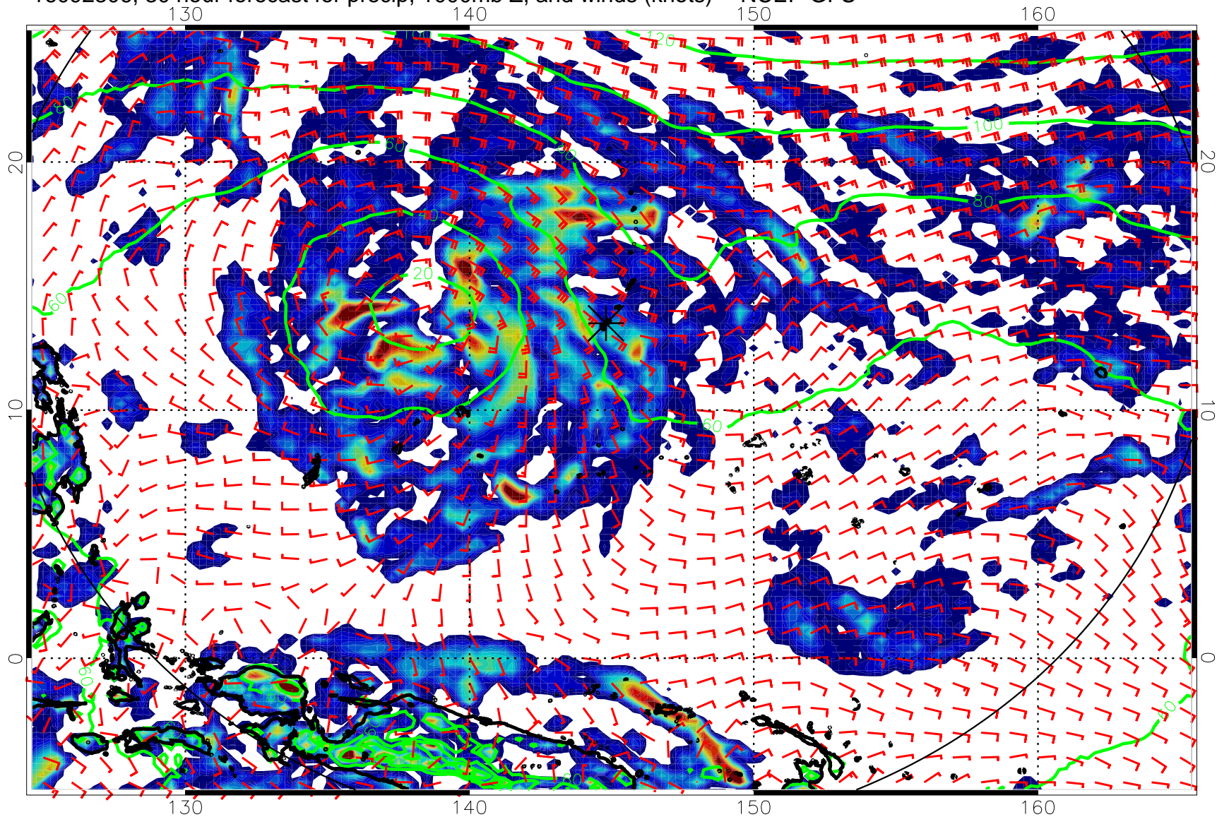
16092306, 30 hour forecast for precip, 1000mb Z, and winds (knots) -- NCEP GFS
