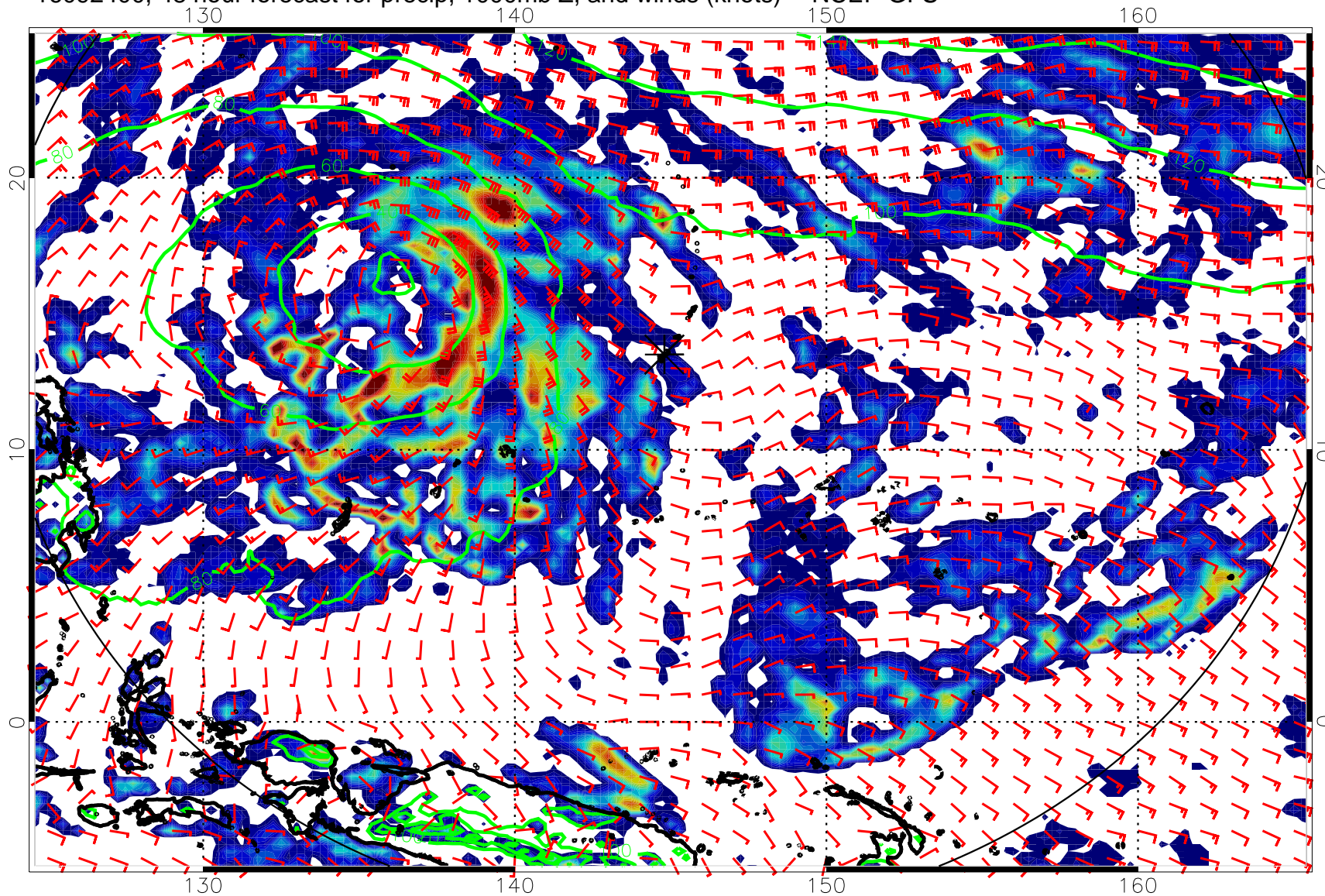
16092400, 48 hour forecast for precip, 1000mb Z, and winds (knots) -- NCEP GFS
