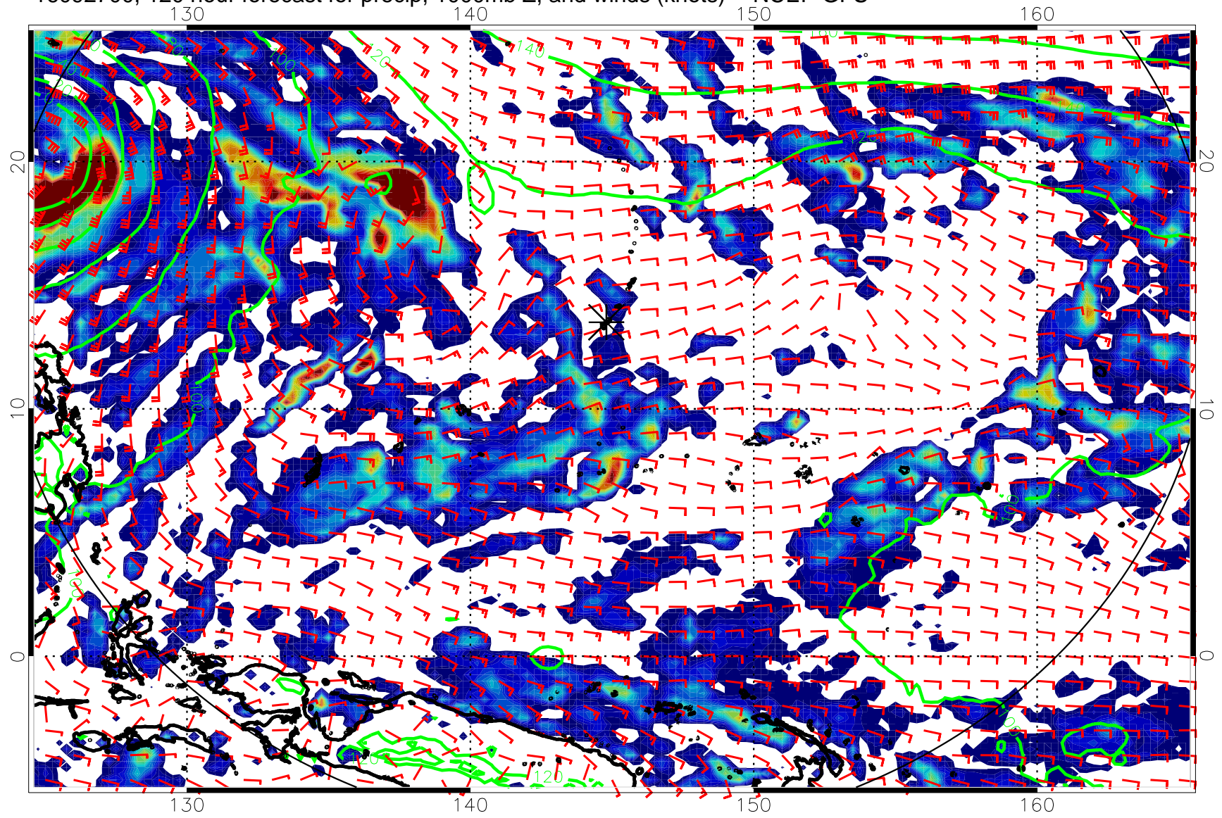
16092700, 120 hour forecast for precip, 1000mb Z, and winds (knots) -- NCEP GFS
