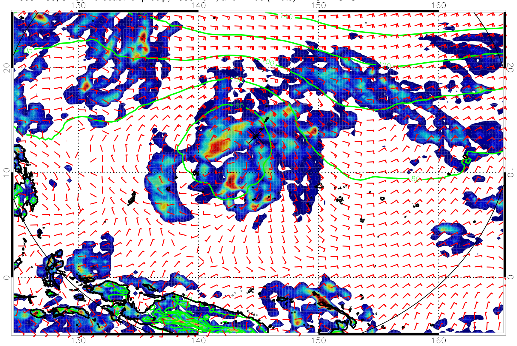
16092206, 6 hour forecast for precip, 1000mb Z, and winds (knots) -- NCEP GFS
