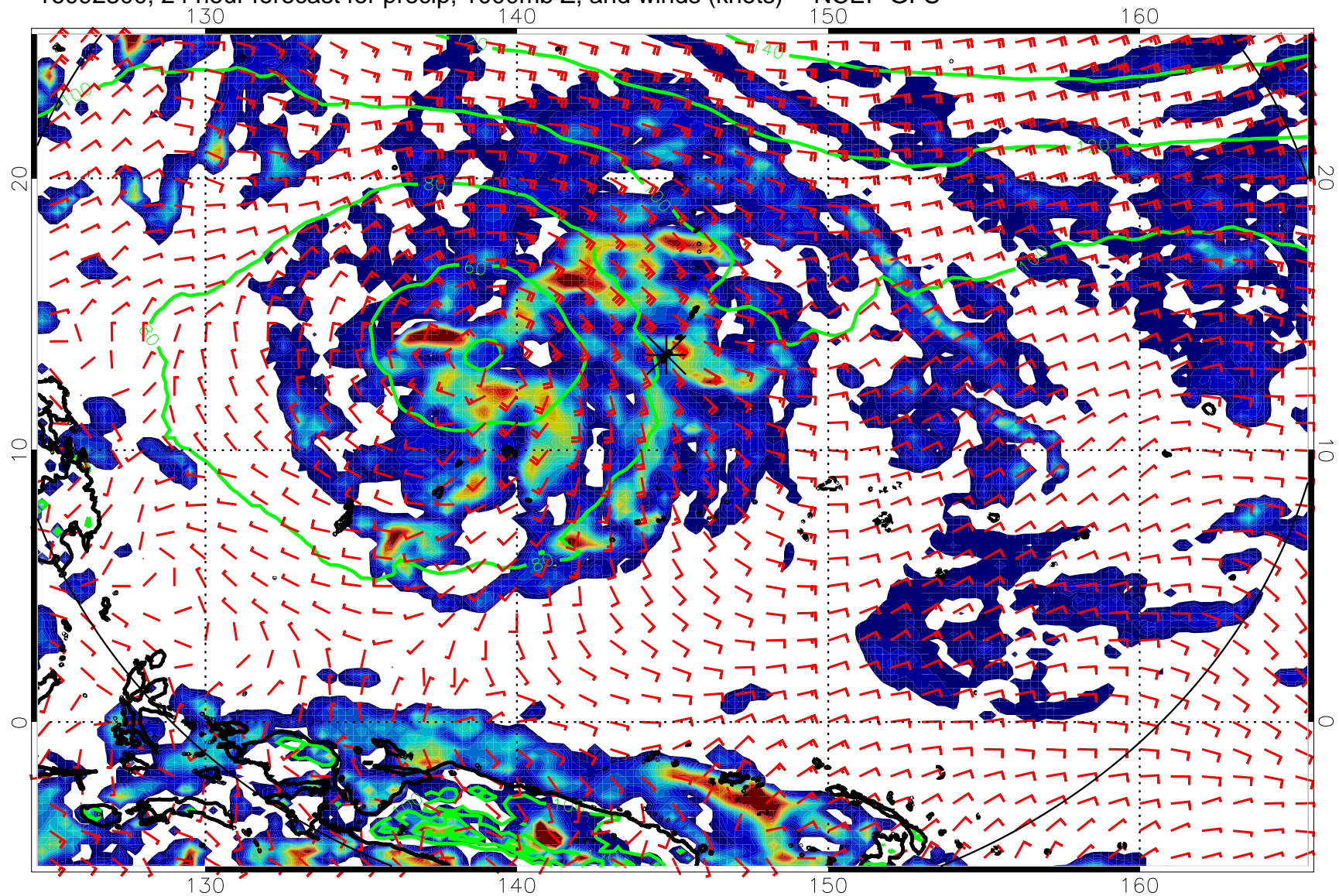
16092300, 24 hour forecast for precip, 1000mb Z, and winds (knots) -- NCEP GFS
