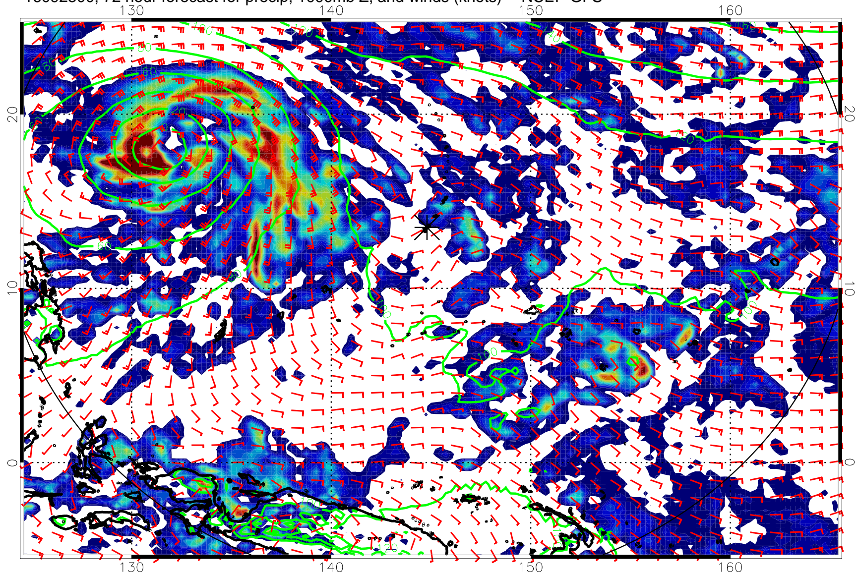
16092500, 72 hour forecast for precip, 1000mb Z, and winds (knots) -- NCEP GFS
