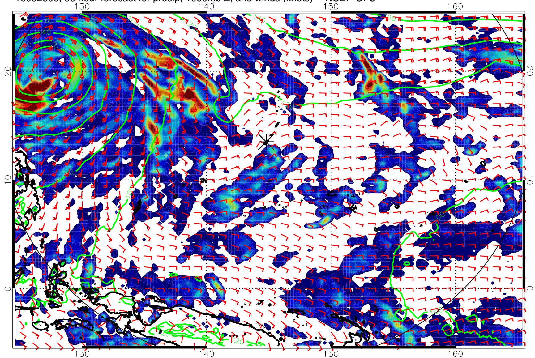
16092600, 96 hour forecast for precip, 1000mb Z, and winds (knots) -- NCEP GFS
