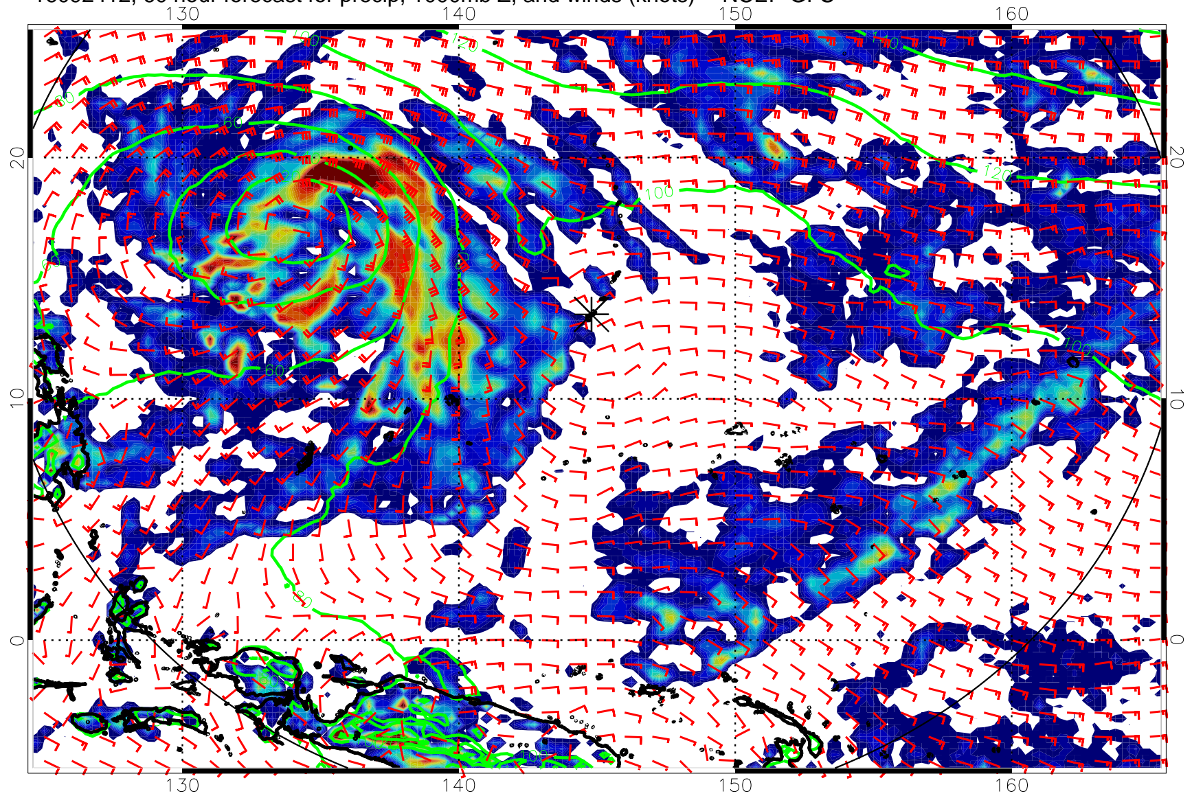
16092412, 60 hour forecast for precip, 1000mb Z, and winds (knots) -- NCEP GFS
