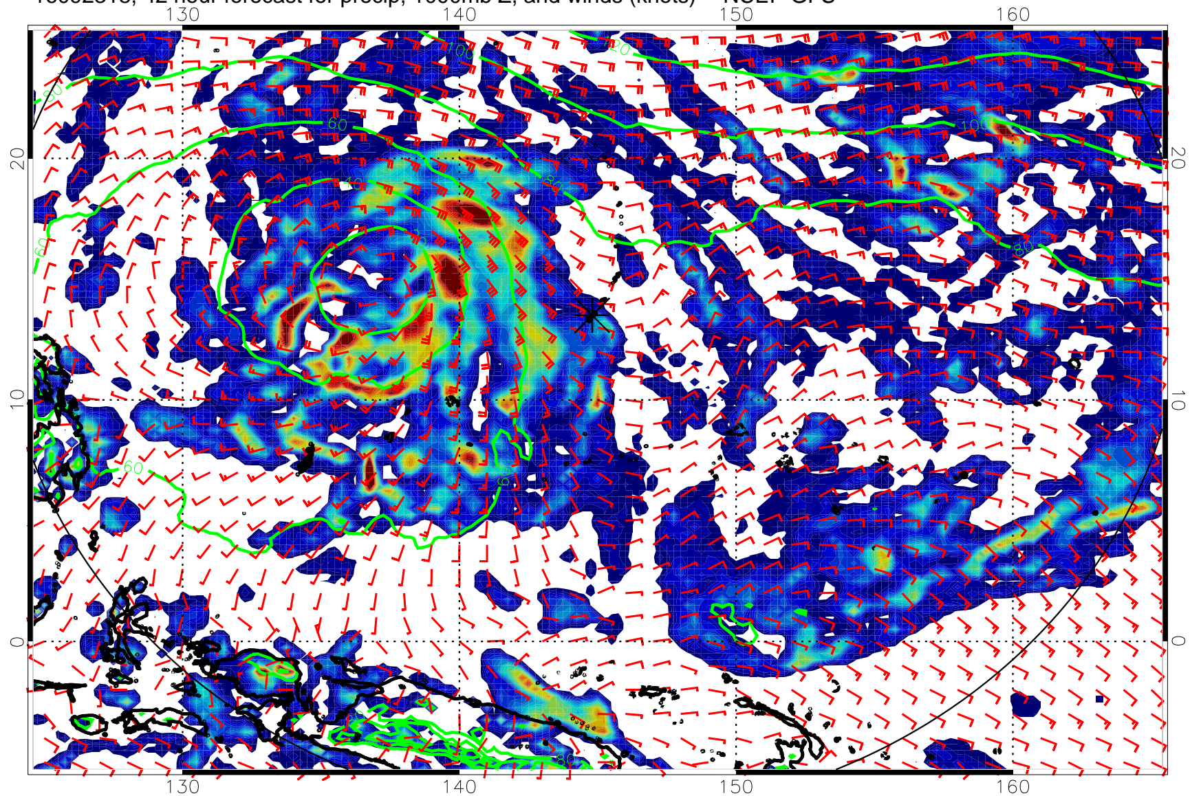
16092318, 42 hour forecast for precip, 1000mb Z, and winds (knots) -- NCEP GFS
