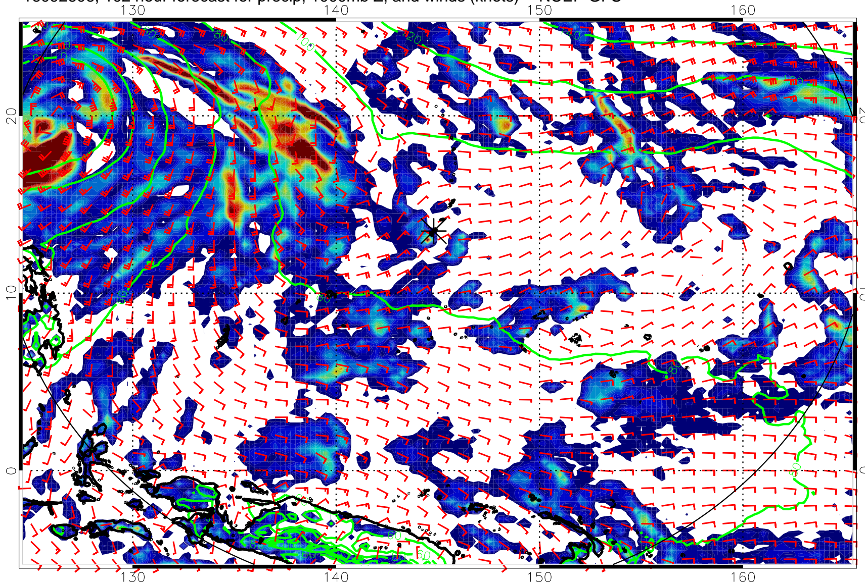
16092606, 102 hour forecast for precip, 1000mb Z, and winds (knots) -- NCEP GFS
