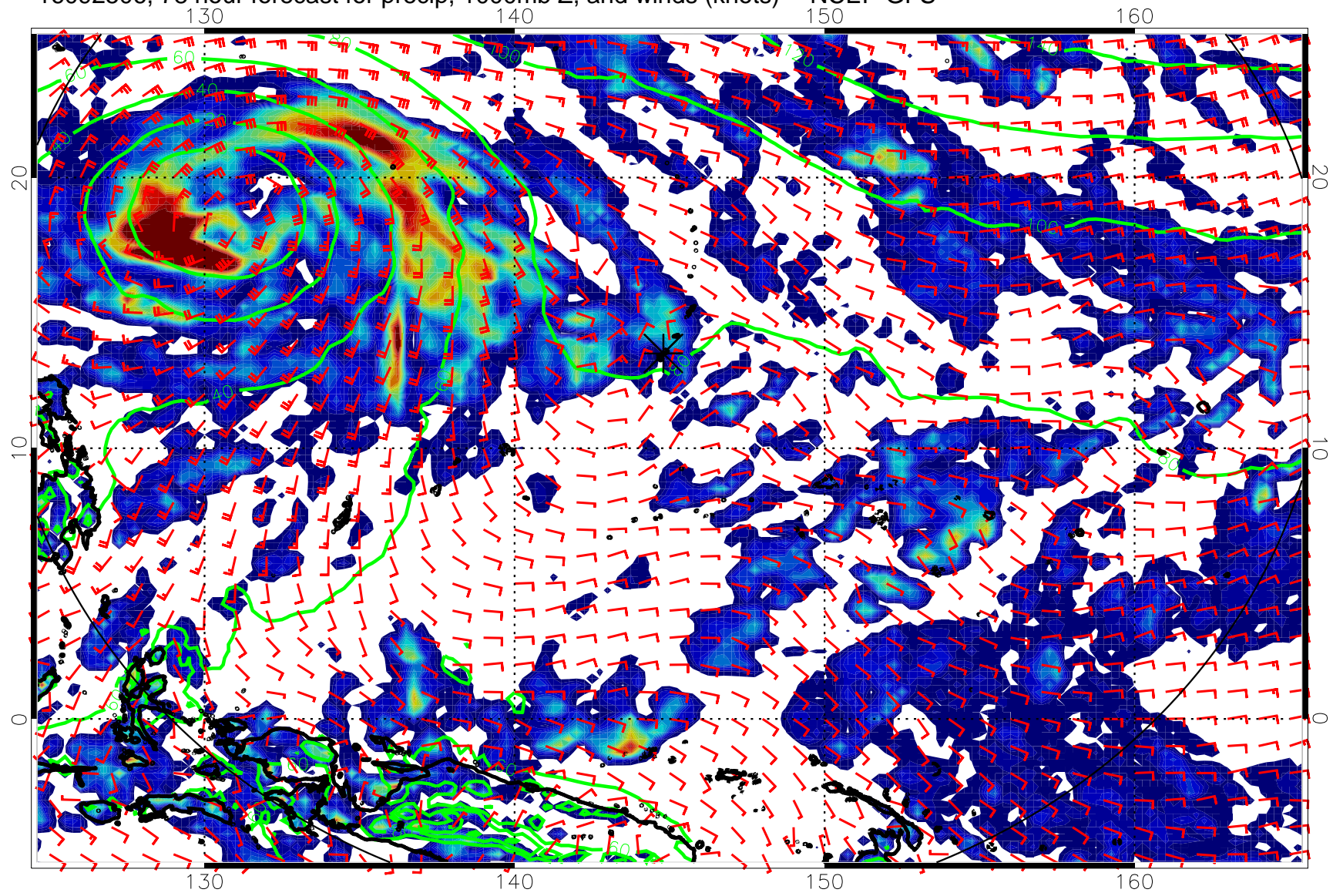
16092506, 78 hour forecast for precip, 1000mb Z, and winds (knots) -- NCEP GFS
