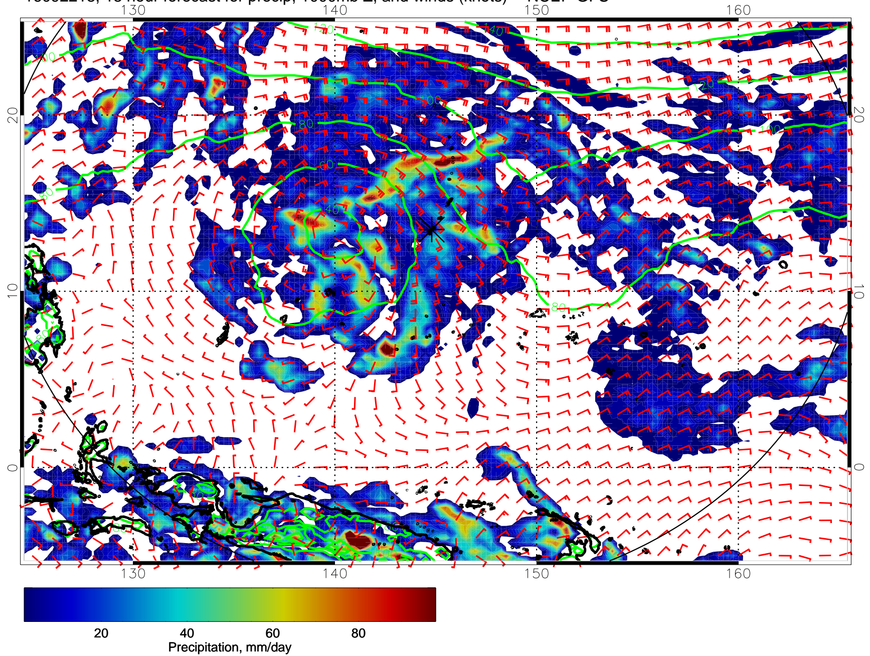
16092218, 18 hour forecast for precip, 1000mb Z, and winds (knots) -- NCEP GFS
