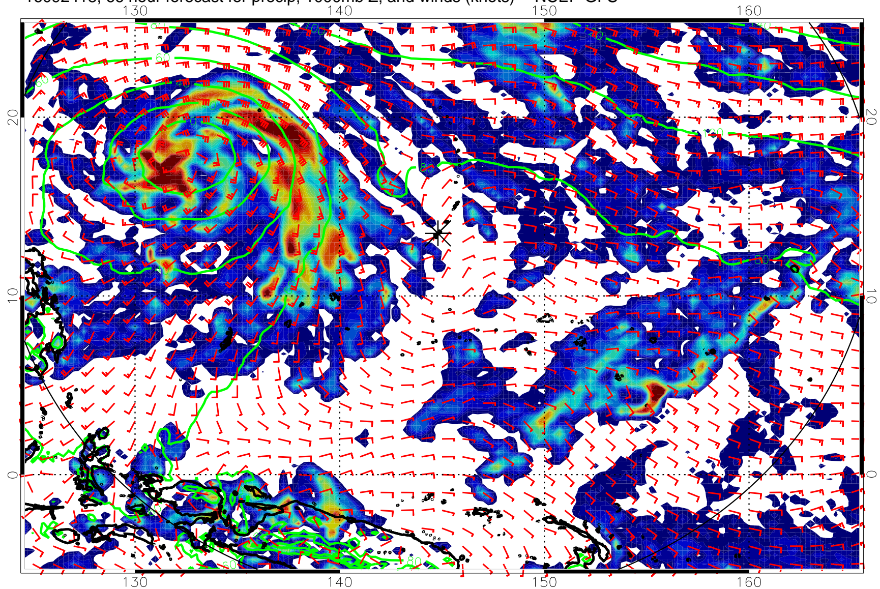
16092418, 66 hour forecast for precip, 1000mb Z, and winds (knots) -- NCEP GFS
