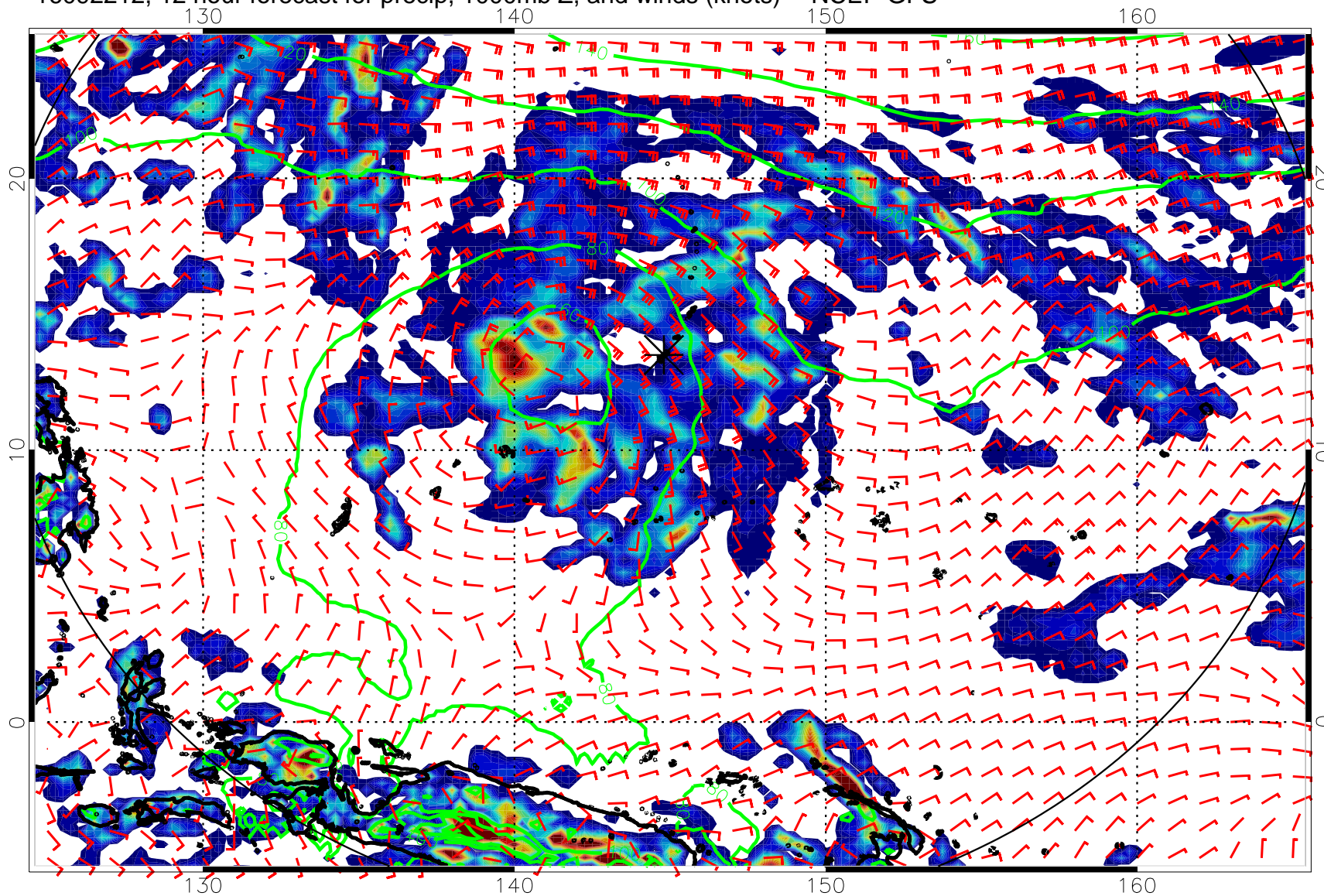
16092212, 12 hour forecast for precip, 1000mb Z, and winds (knots) -- NCEP GFS
