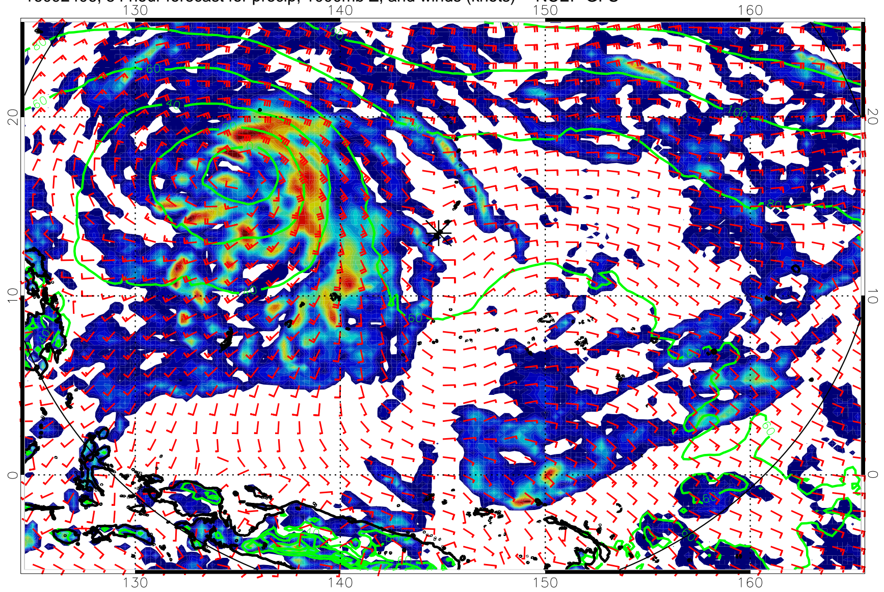
16092406, 54 hour forecast for precip, 1000mb Z, and winds (knots) -- NCEP GFS
