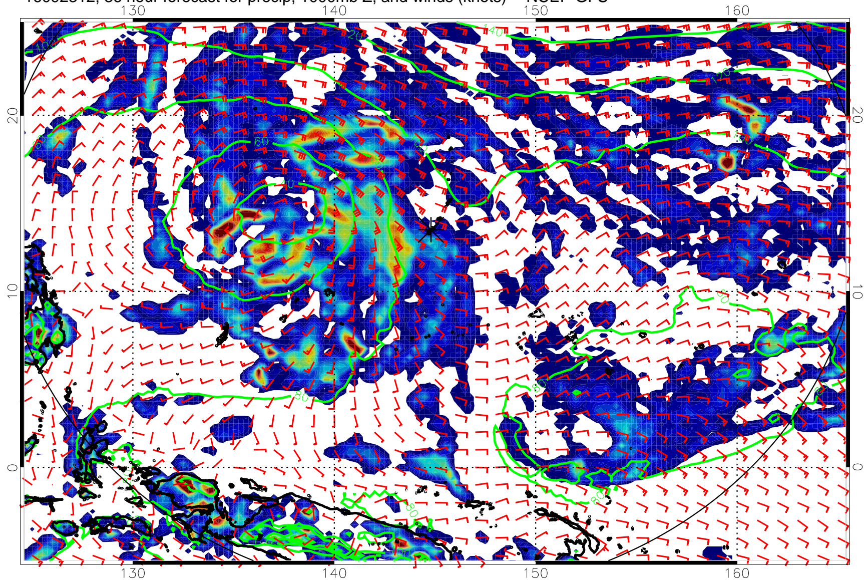
16092312, 36 hour forecast for precip, 1000mb Z, and winds (knots) -- NCEP GFS
