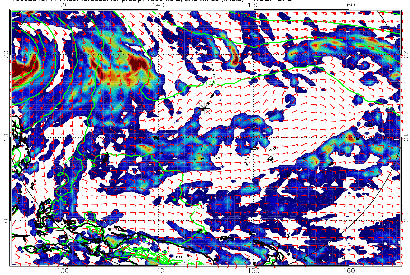
16092618, 114 hour forecast for precip, 1000mb Z, and winds (knots) -- NCEP GFS
