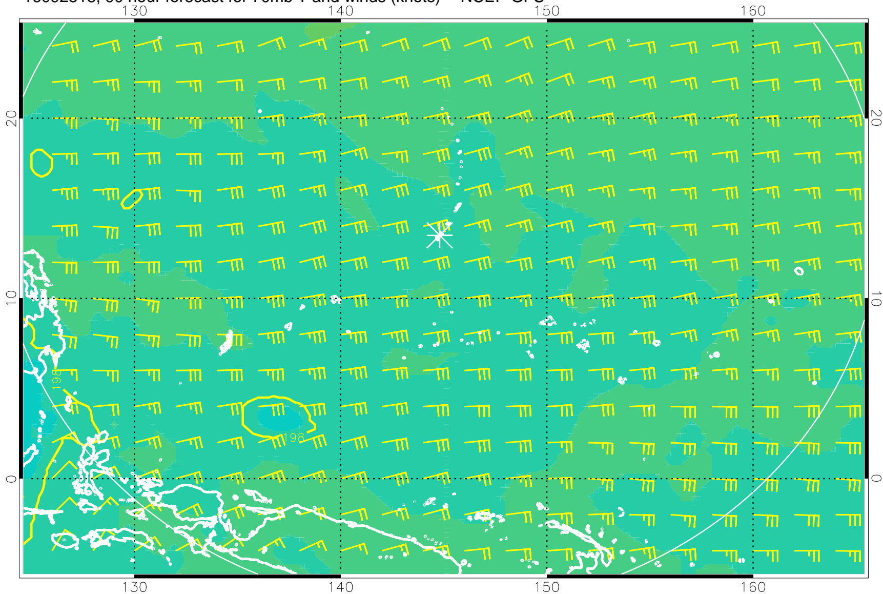
16092518, 90 hour forecast for 70mb T and winds (knots) -- NCEP GFS
