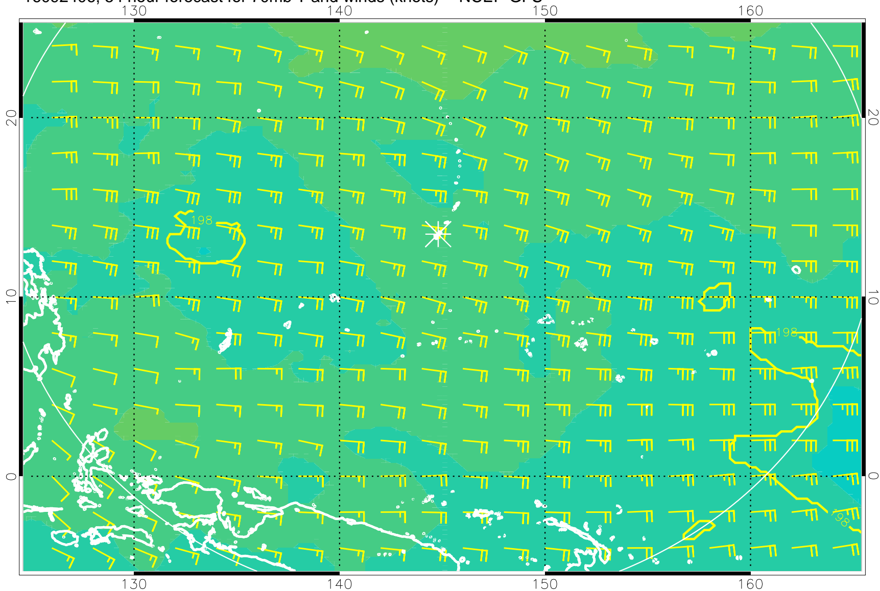
16092406, 54 hour forecast for 70mb T and winds (knots) -- NCEP GFS
