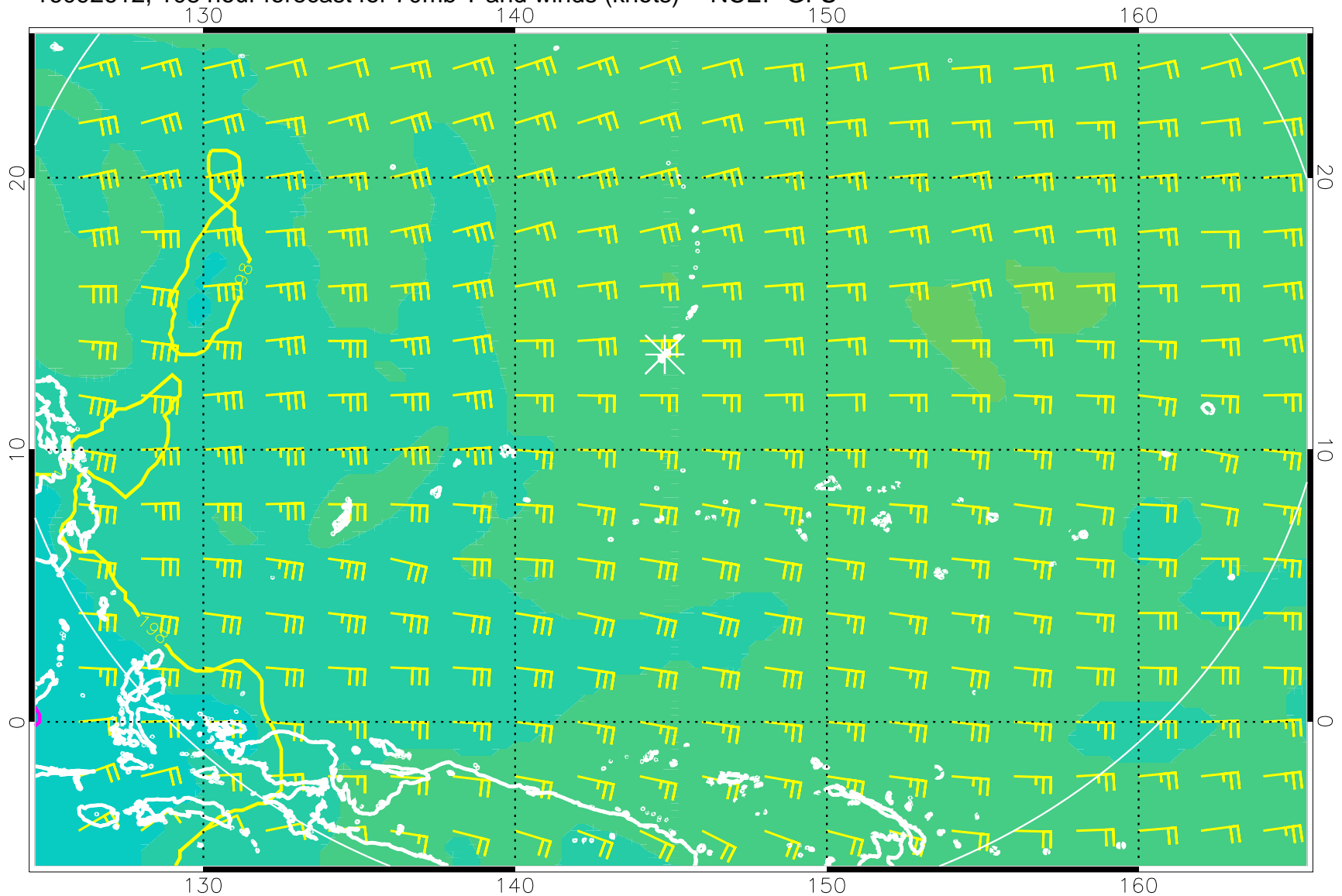
16092612, 108 hour forecast for 70mb T and winds (knots) -- NCEP GFS
