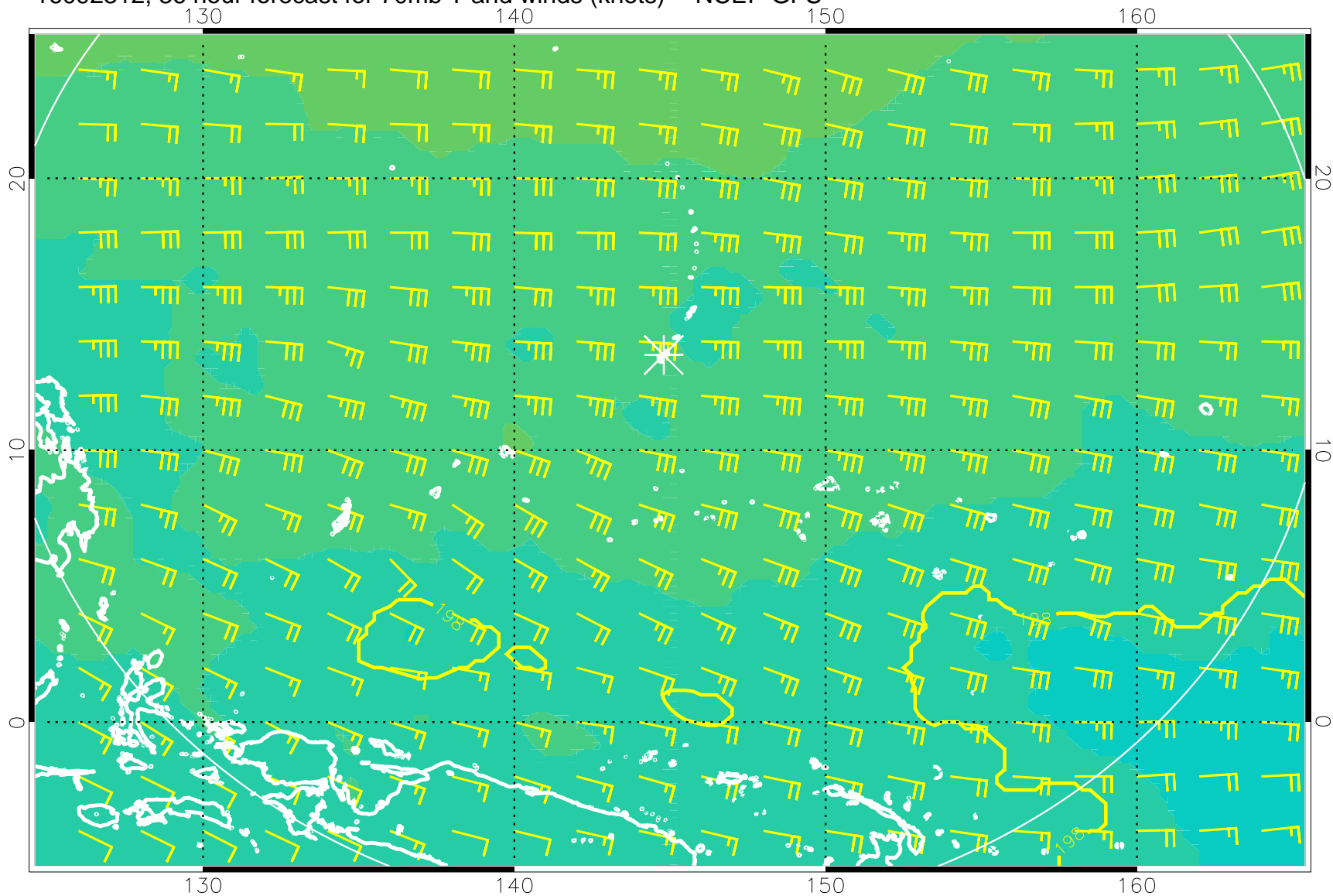
16092312, 36 hour forecast for 70mb T and winds (knots) -- NCEP GFS
