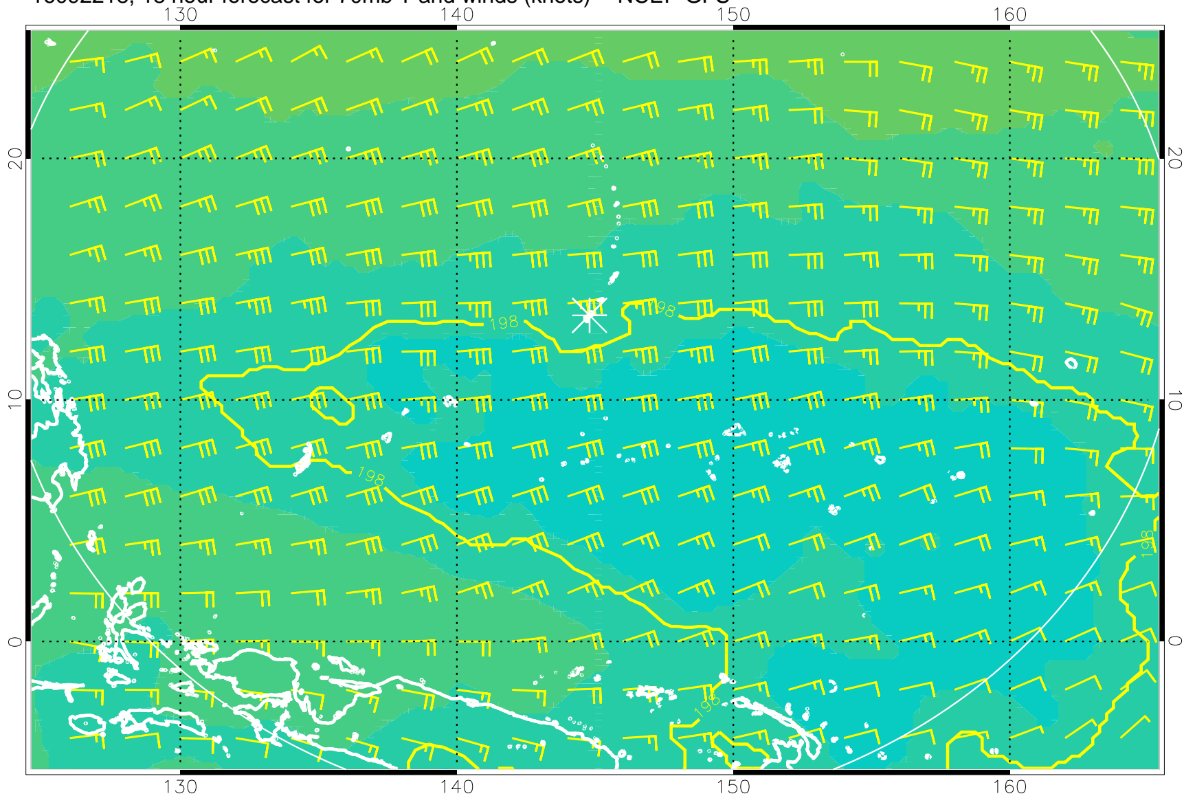
16092218, 18 hour forecast for 70mb T and winds (knots) -- NCEP GFS
