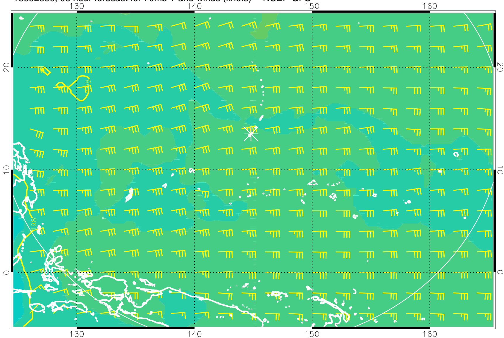
16092600, 96 hour forecast for 70mb T and winds (knots) -- NCEP GFS
