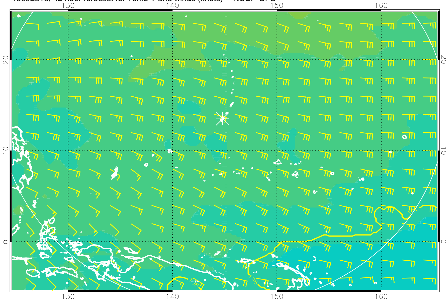
16092318, 42 hour forecast for 70mb T and winds (knots) -- NCEP GFS
