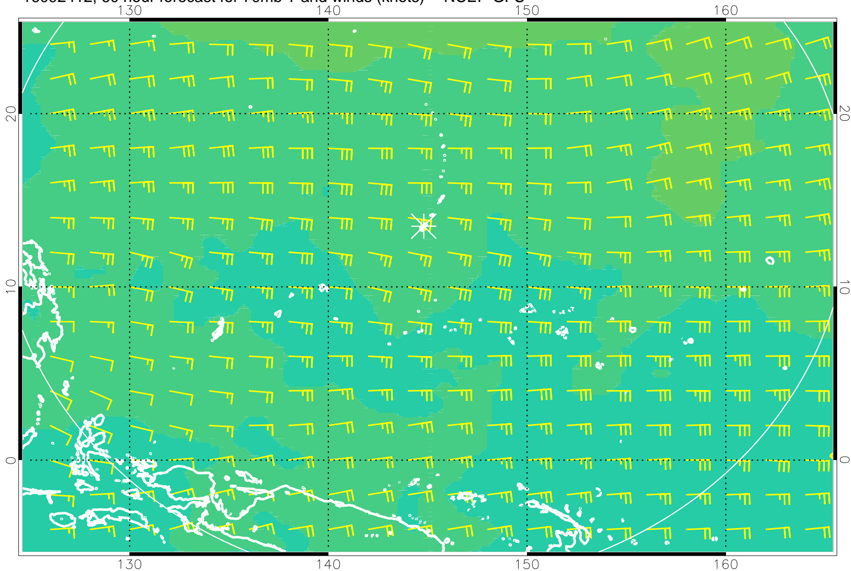
16092412, 60 hour forecast for 70mb T and winds (knots) -- NCEP GFS
