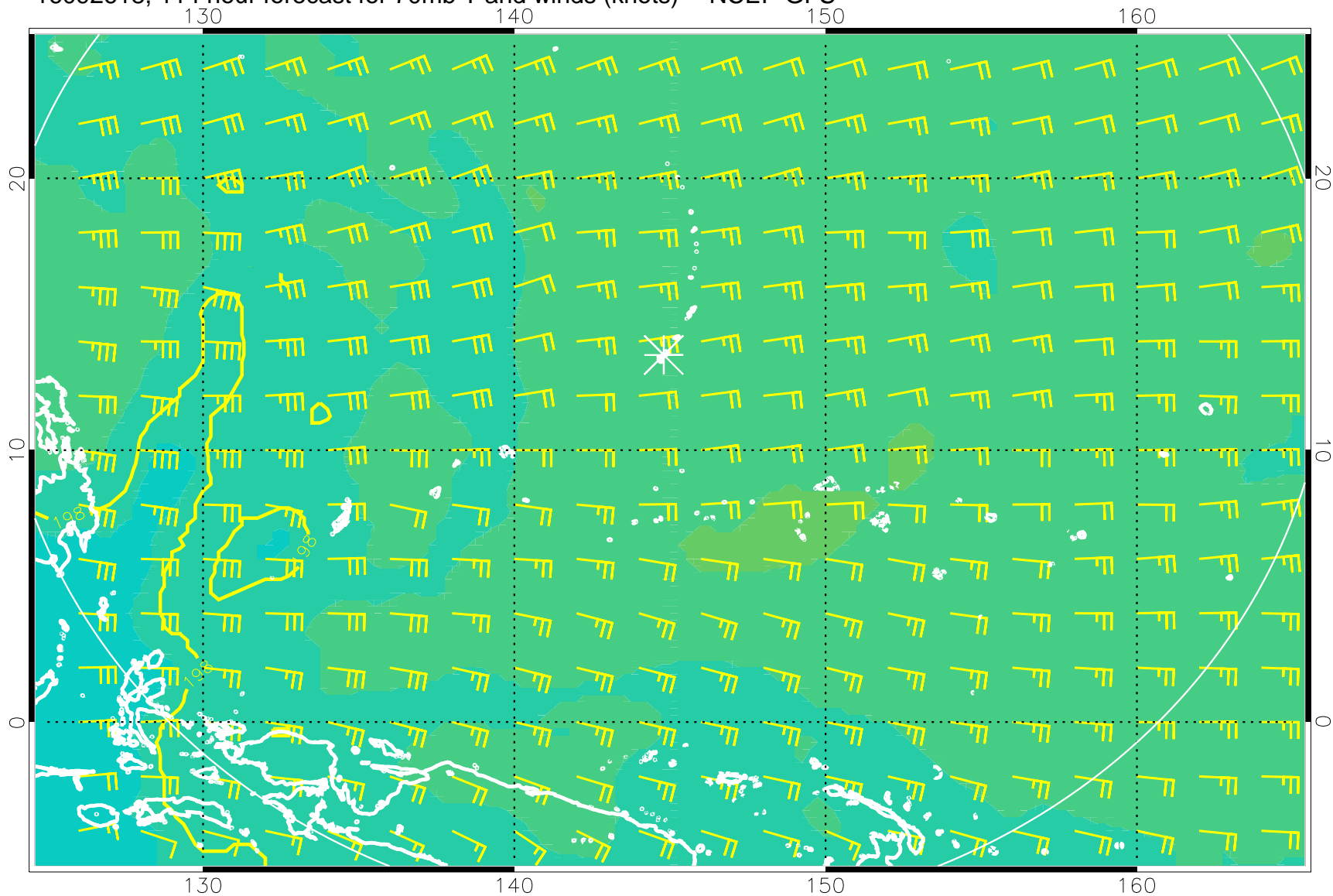
16092618, 114 hour forecast for 70mb T and winds (knots) -- NCEP GFS
