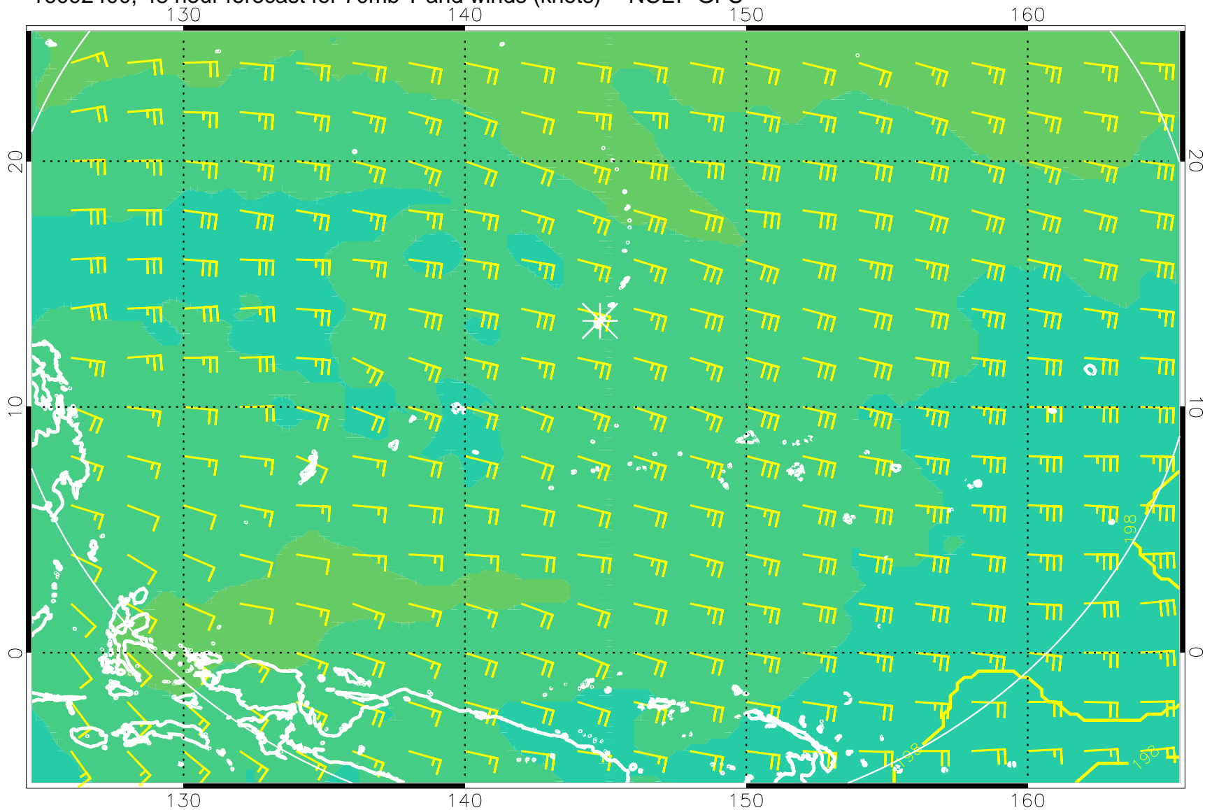
16092400, 48 hour forecast for 70mb T and winds (knots) -- NCEP GFS
