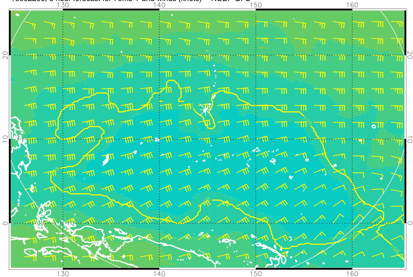
16092206, 6 hour forecast for 70mb T and winds (knots) -- NCEP GFS
