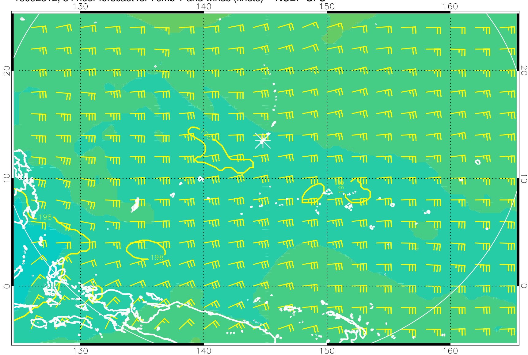
16092512, 84 hour forecast for 70mb T and winds (knots) -- NCEP GFS
