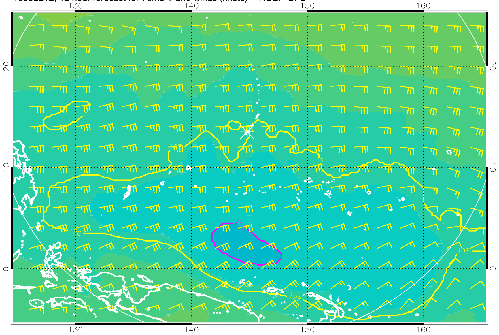
16092212, 12 hour forecast for 70mb T and winds (knots) -- NCEP GFS
