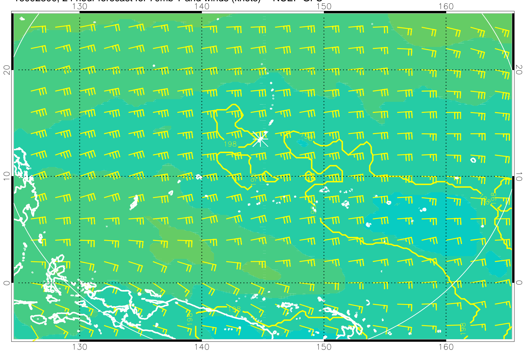
16092300, 24 hour forecast for 70mb T and winds (knots) -- NCEP GFS
