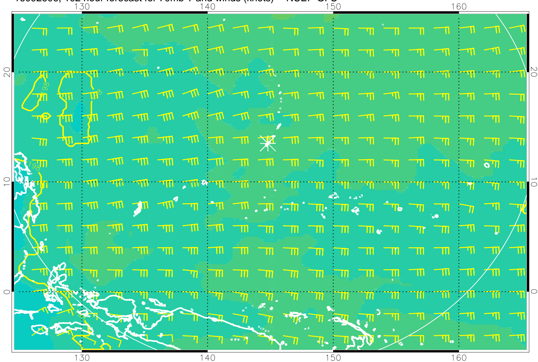
16092606, 102 hour forecast for 70mb T and winds (knots) -- NCEP GFS
