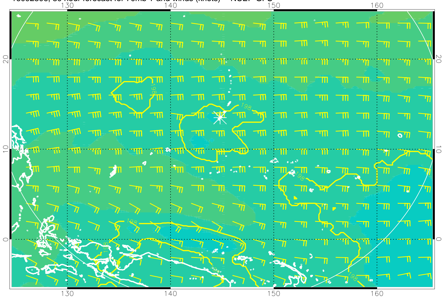
16092306, 30 hour forecast for 70mb T and winds (knots) -- NCEP GFS
