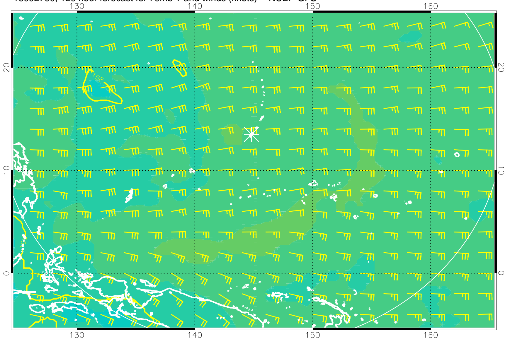
16092700, 120 hour forecast for 70mb T and winds (knots) -- NCEP GFS
