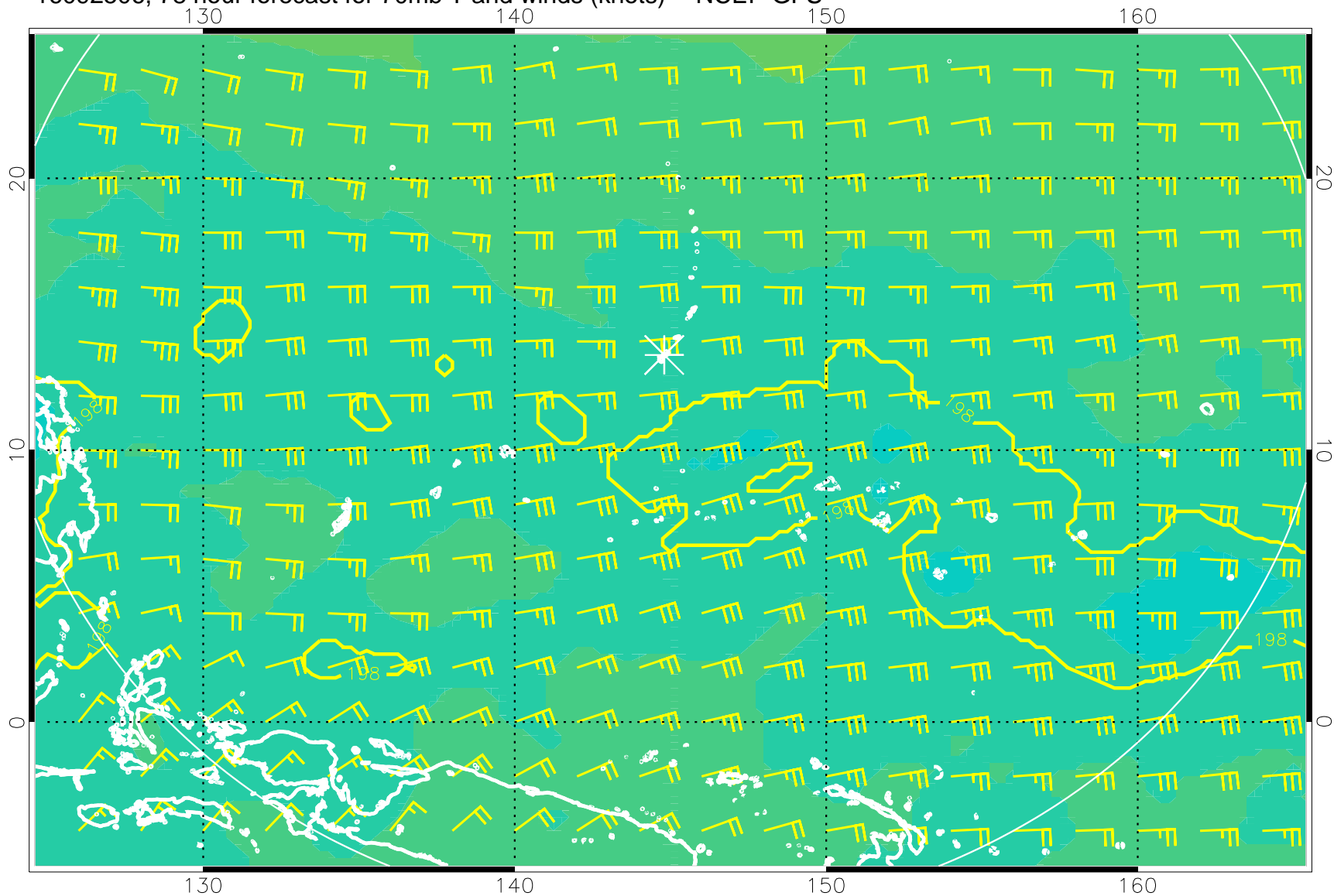
16092506, 78 hour forecast for 70mb T and winds (knots) -- NCEP GFS
