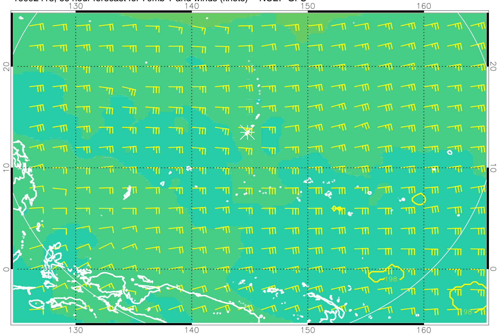
16092418, 66 hour forecast for 70mb T and winds (knots) -- NCEP GFS
