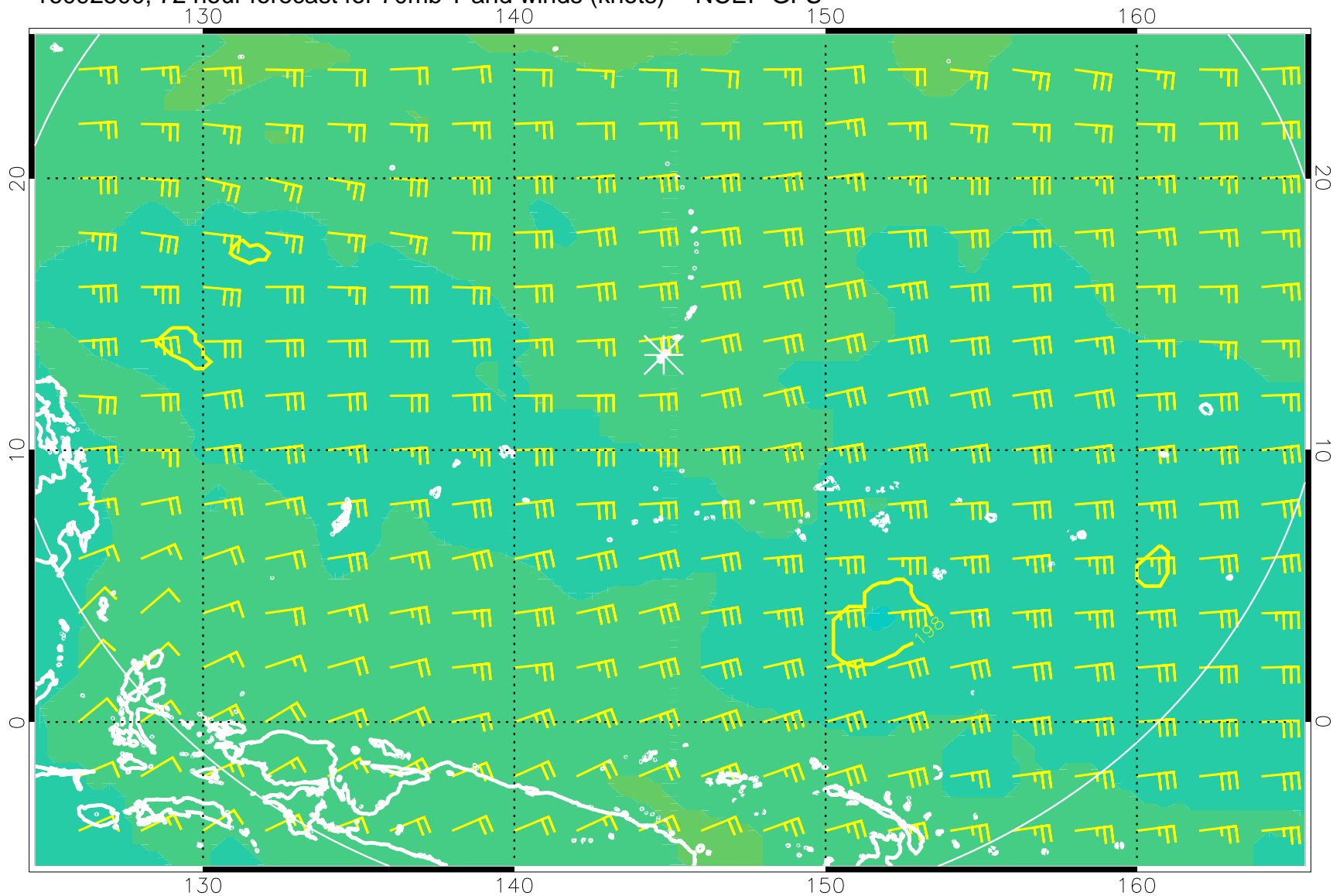
16092500, 72 hour forecast for 70mb T and winds (knots) -- NCEP GFS
