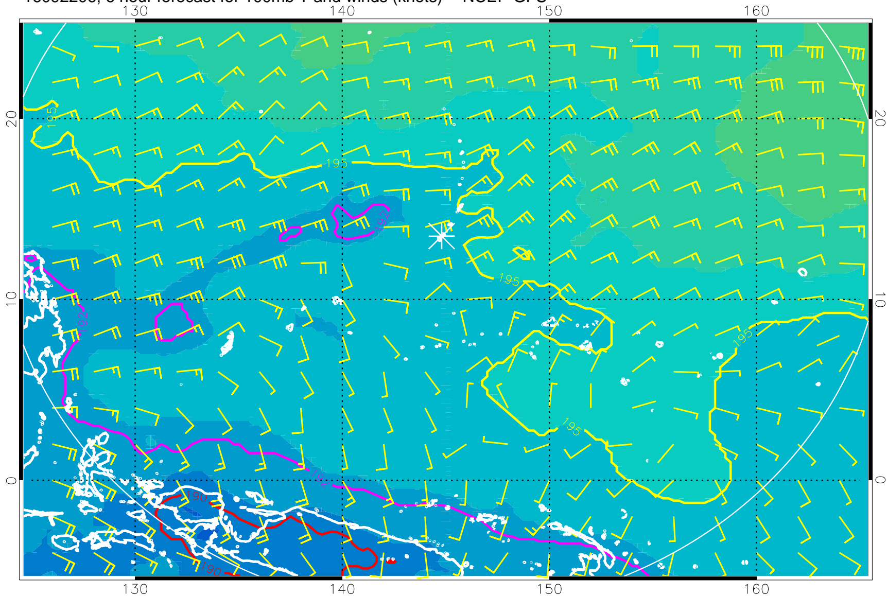
16092206, 6 hour forecast for 100mb T and winds (knots) -- NCEP GFS
