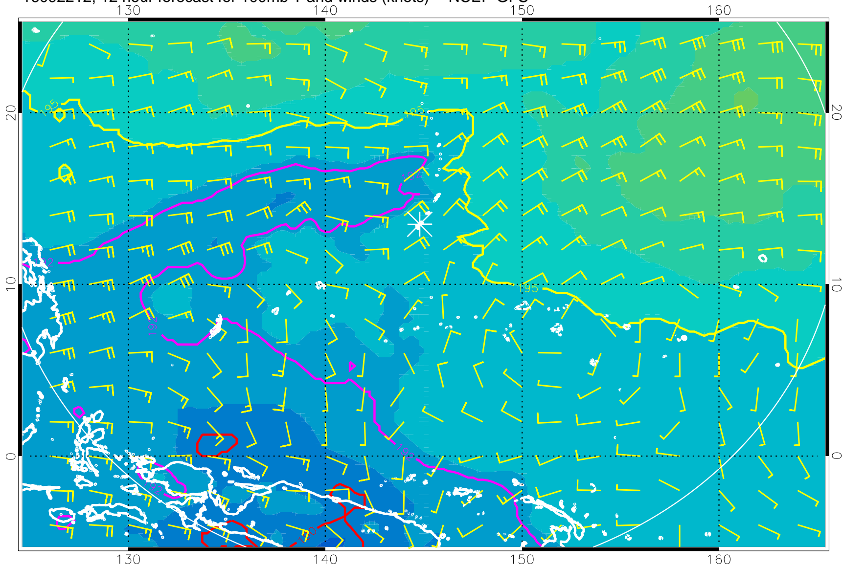
16092212, 12 hour forecast for 100mb T and winds (knots) -- NCEP GFS
