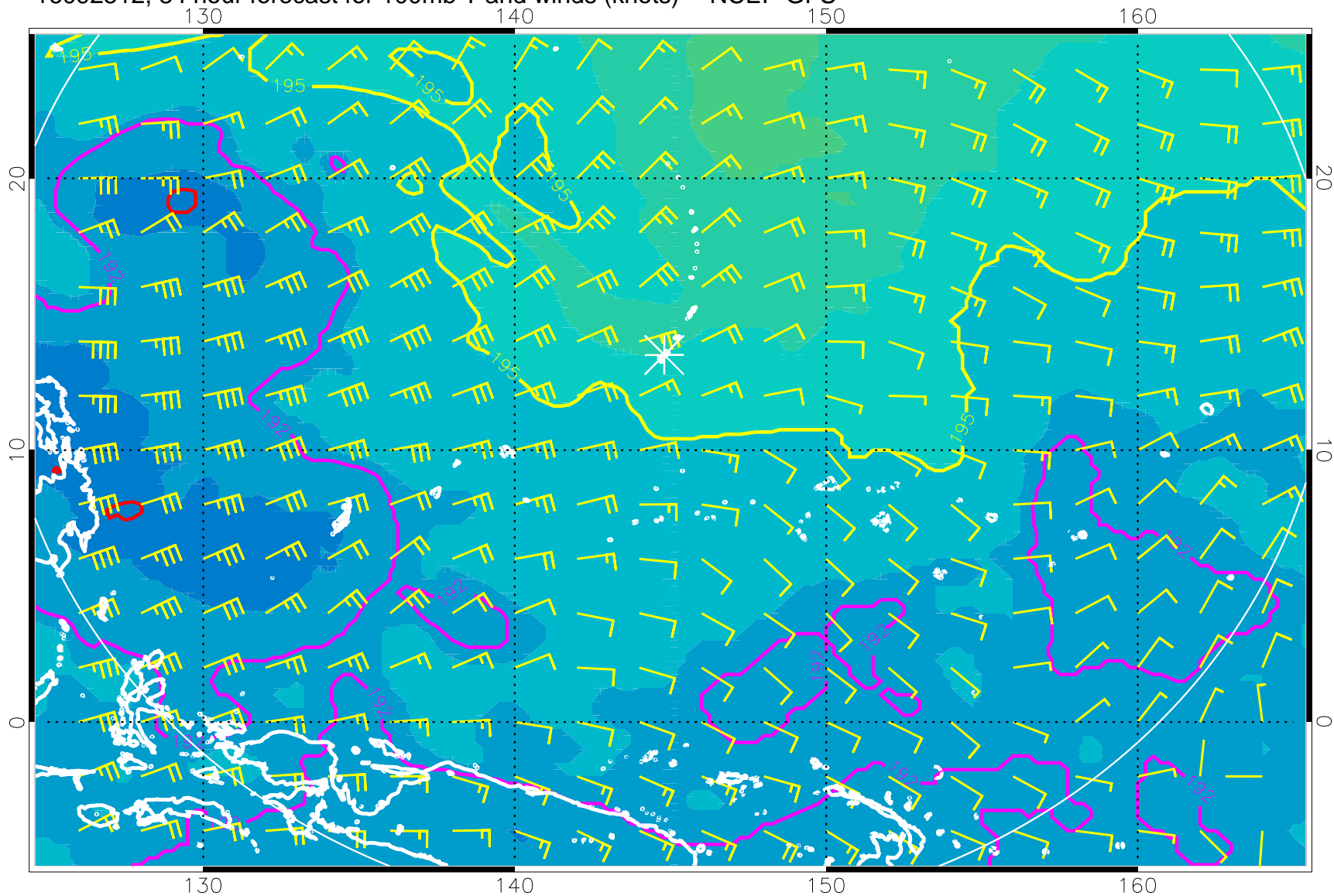
16092512, 84 hour forecast for 100mb T and winds (knots) -- NCEP GFS
