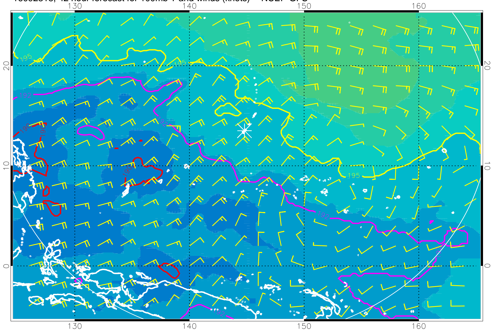
16092318, 42 hour forecast for 100mb T and winds (knots) -- NCEP GFS
