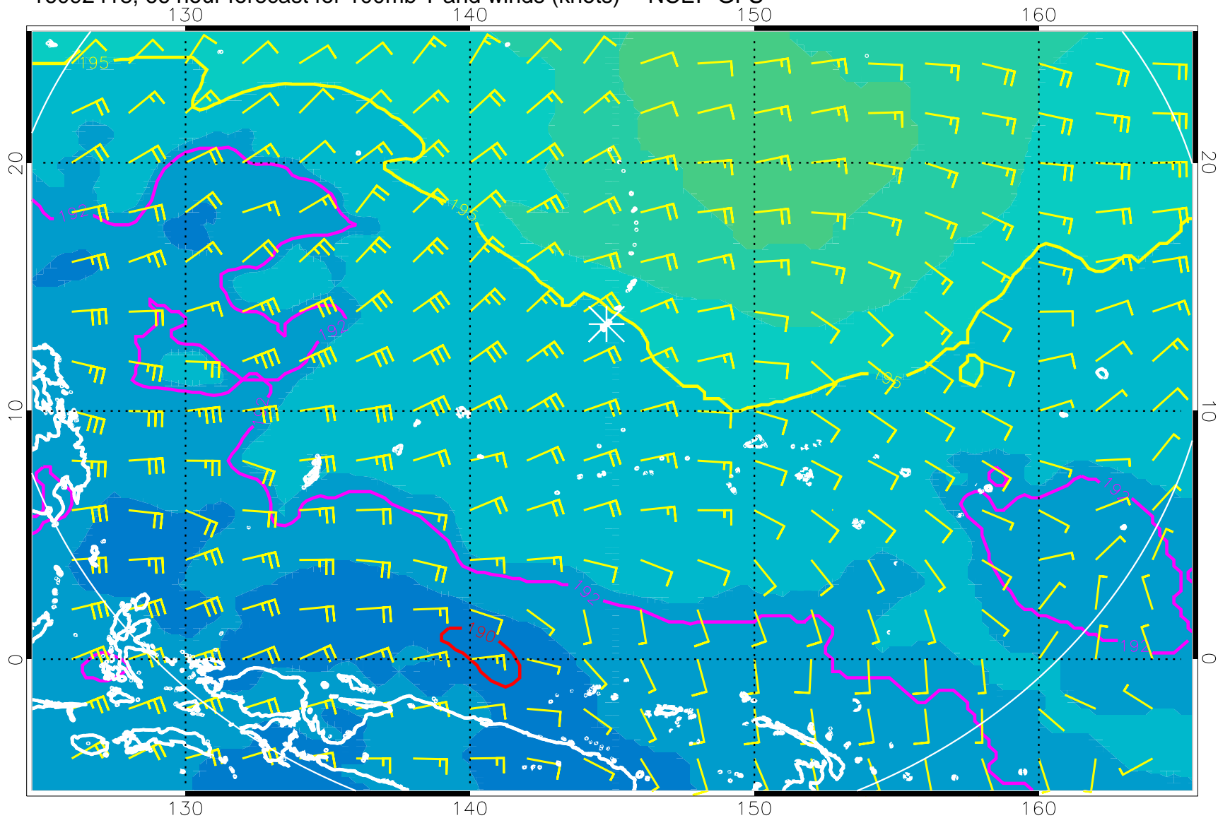
16092418, 66 hour forecast for 100mb T and winds (knots) -- NCEP GFS
