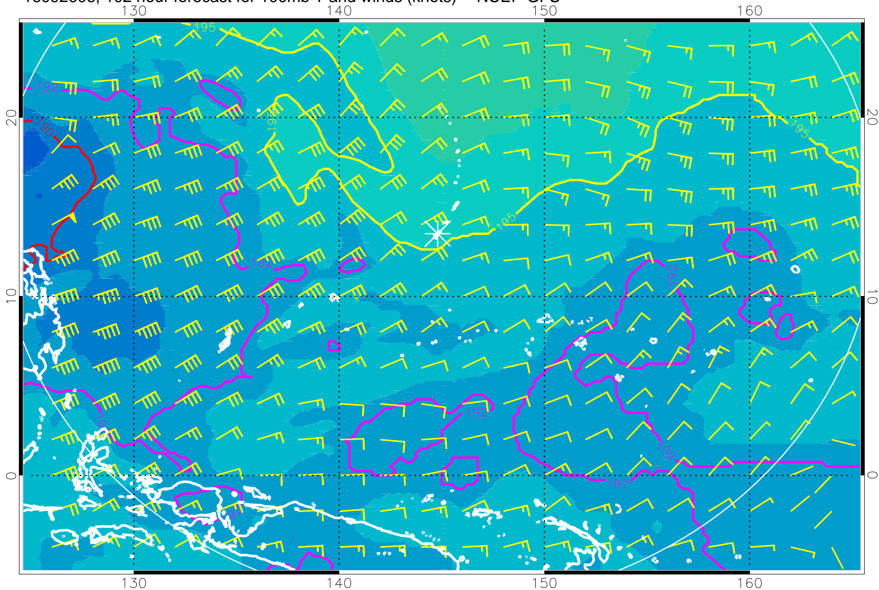
16092606, 102 hour forecast for 100mb T and winds (knots) -- NCEP GFS
