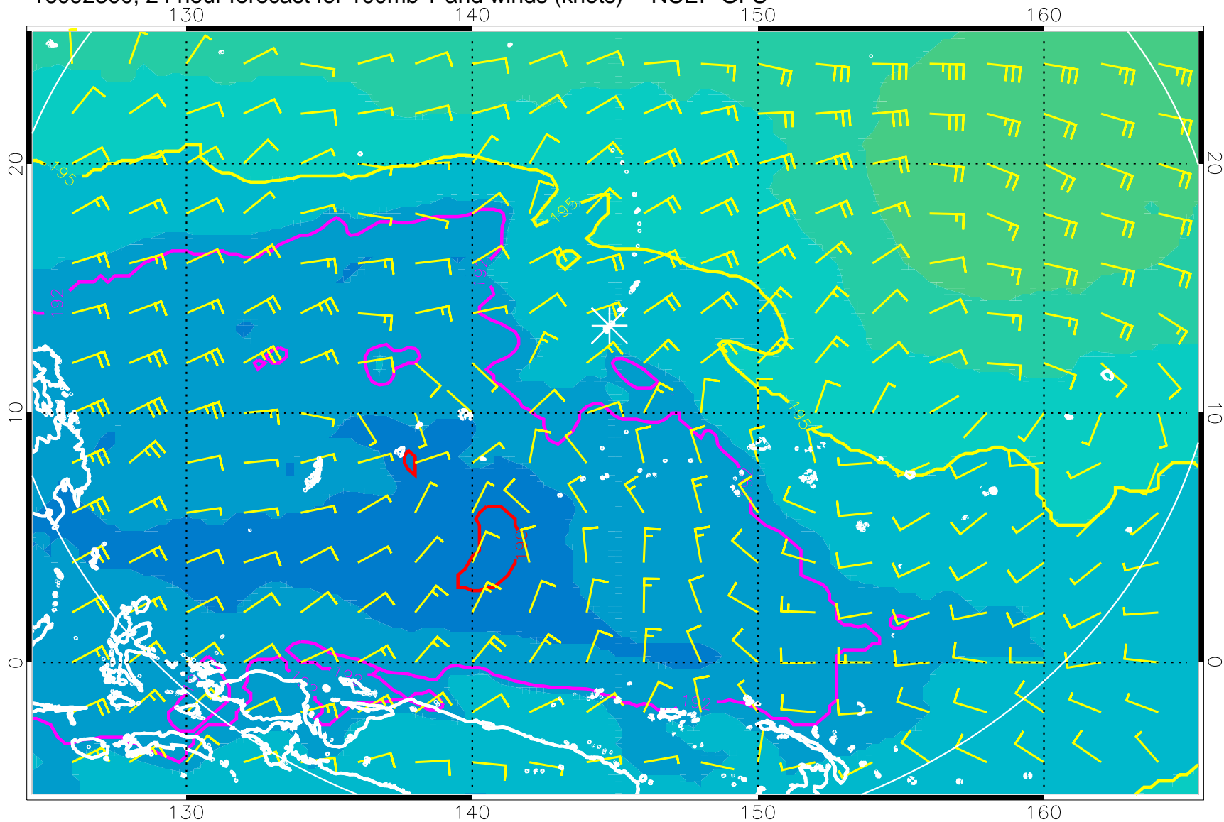
16092300, 24 hour forecast for 100mb T and winds (knots) -- NCEP GFS
