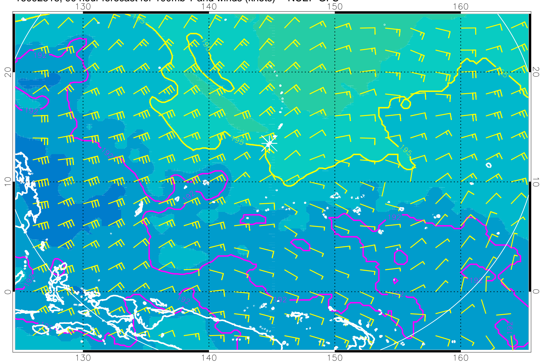
16092518, 90 hour forecast for 100mb T and winds (knots) -- NCEP GFS
