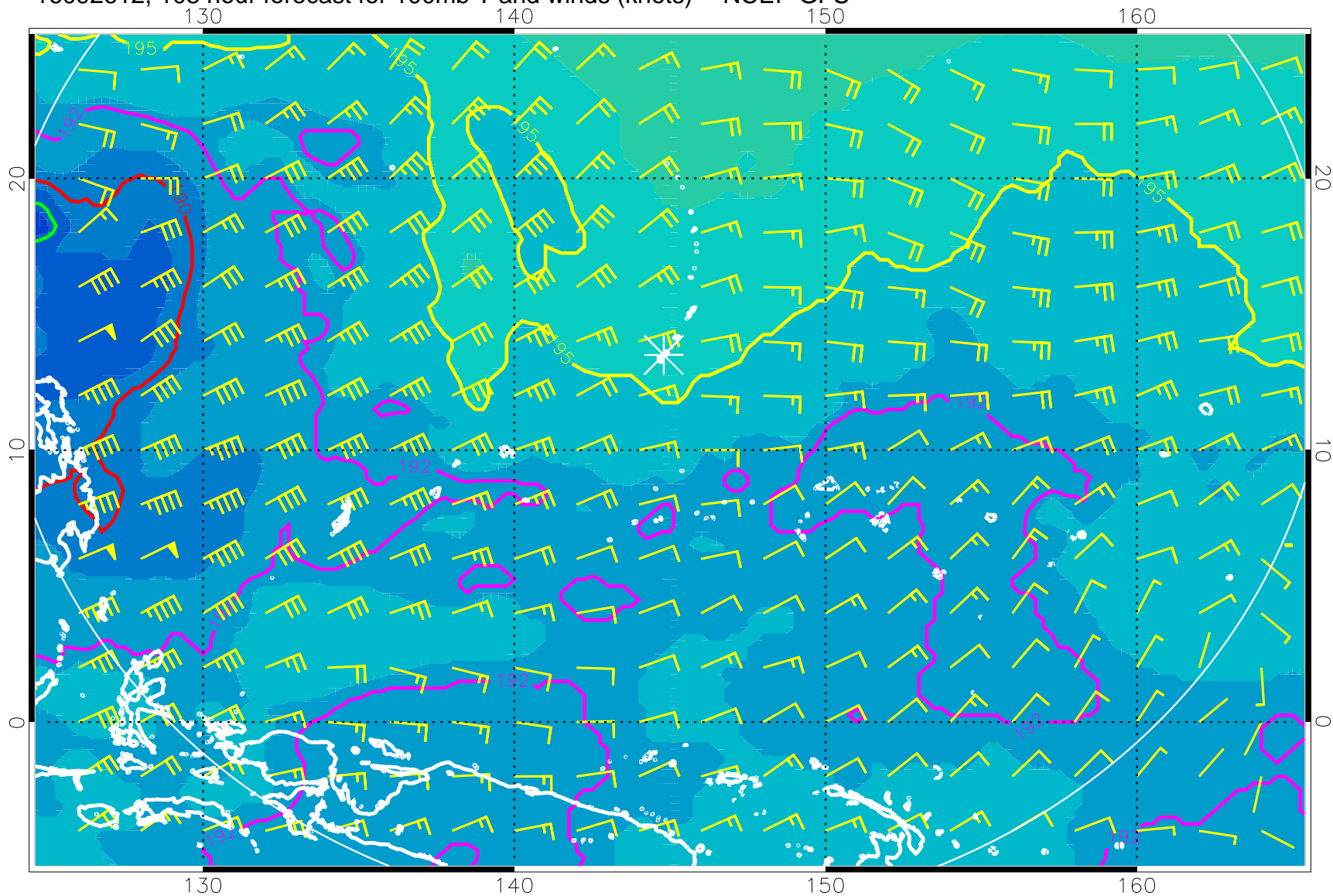
16092612, 108 hour forecast for 100mb T and winds (knots) -- NCEP GFS
