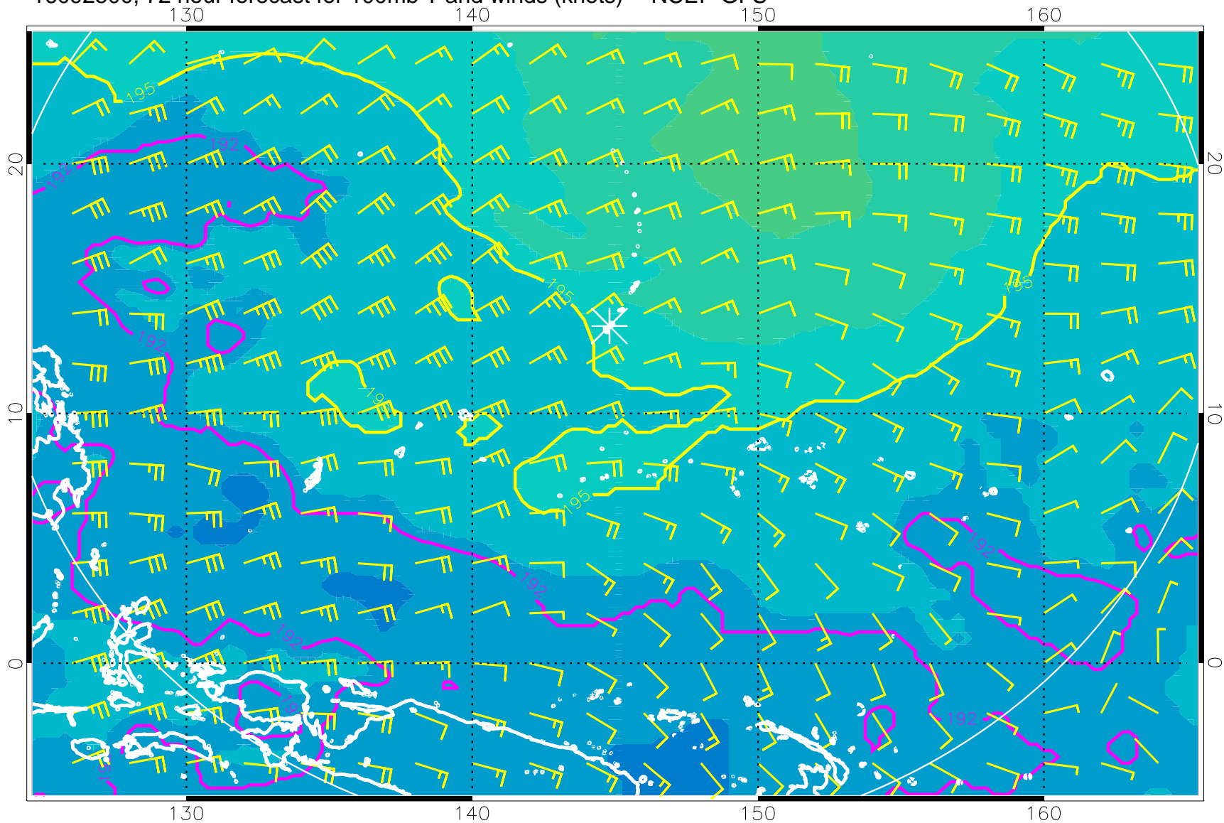
16092500, 72 hour forecast for 100mb T and winds (knots) -- NCEP GFS
