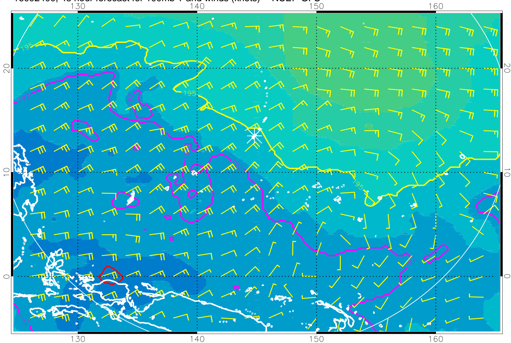
16092400, 48 hour forecast for 100mb T and winds (knots) -- NCEP GFS
