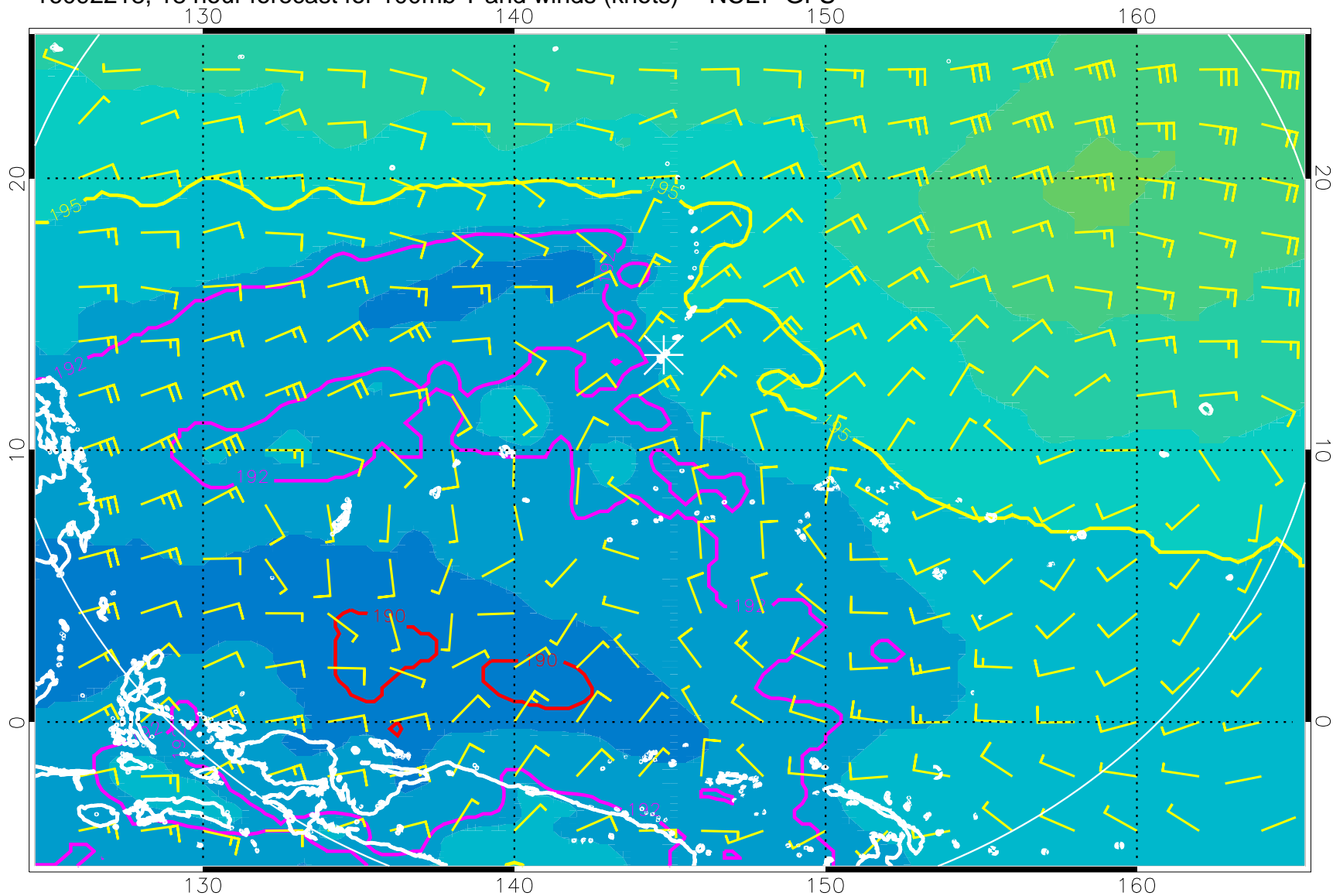
16092218, 18 hour forecast for 100mb T and winds (knots) -- NCEP GFS
