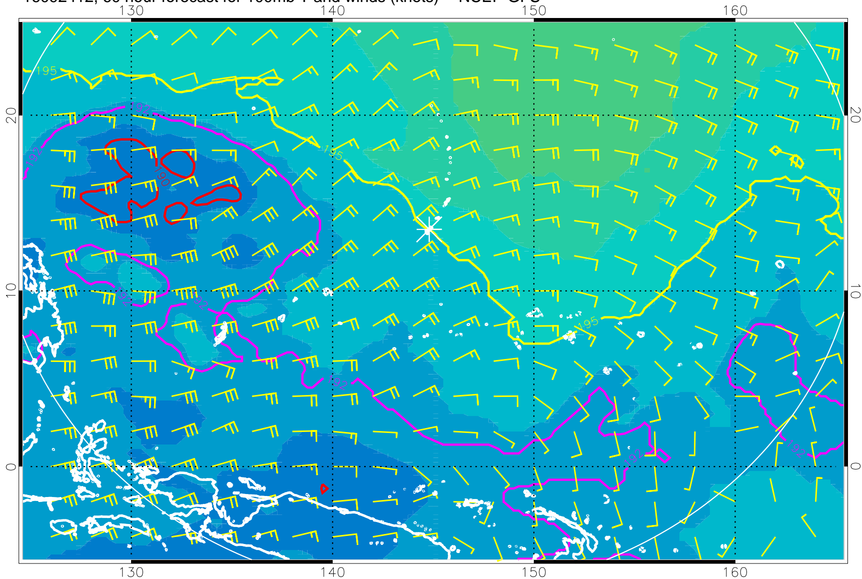
16092412, 60 hour forecast for 100mb T and winds (knots) -- NCEP GFS
