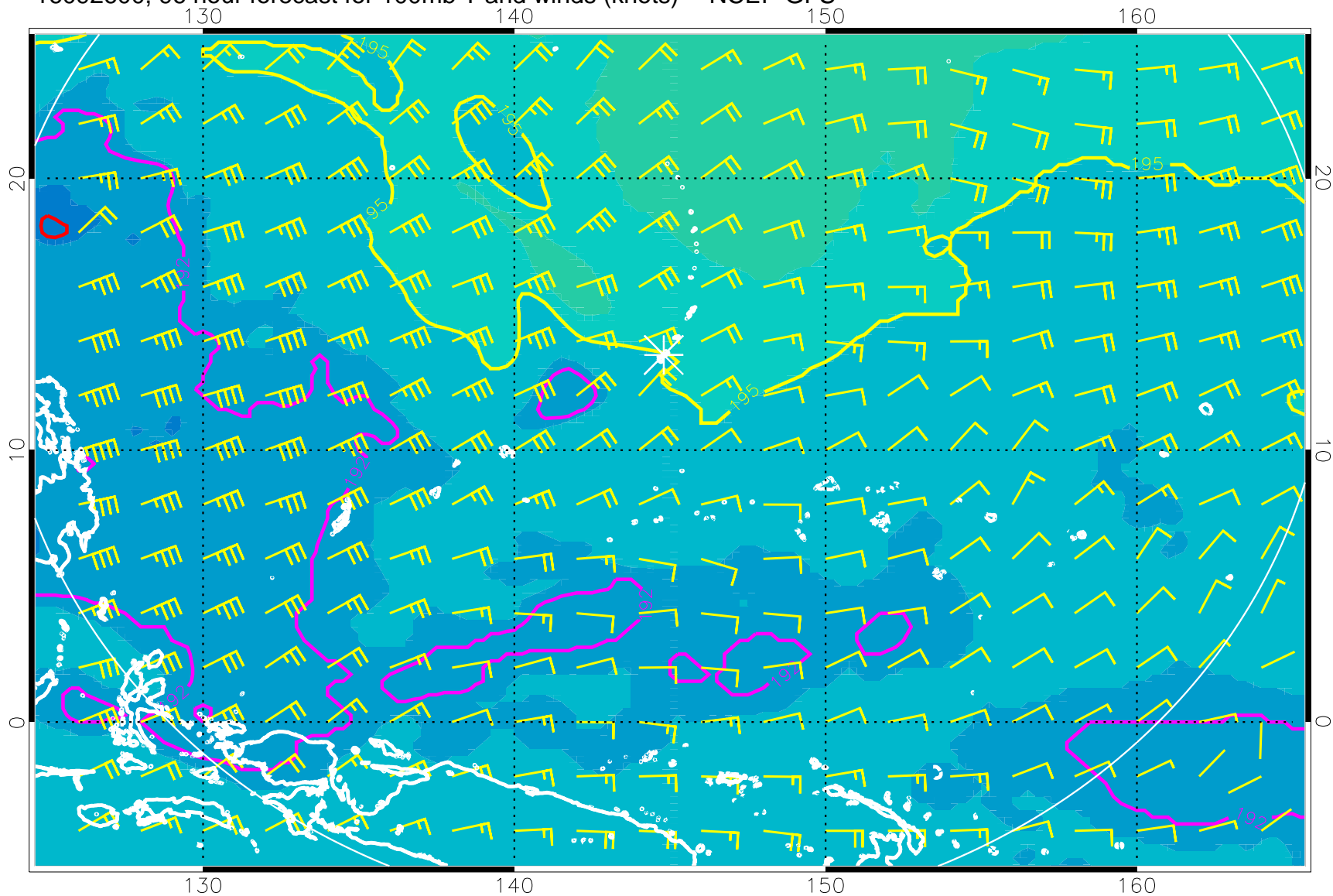
16092600, 96 hour forecast for 100mb T and winds (knots) -- NCEP GFS
