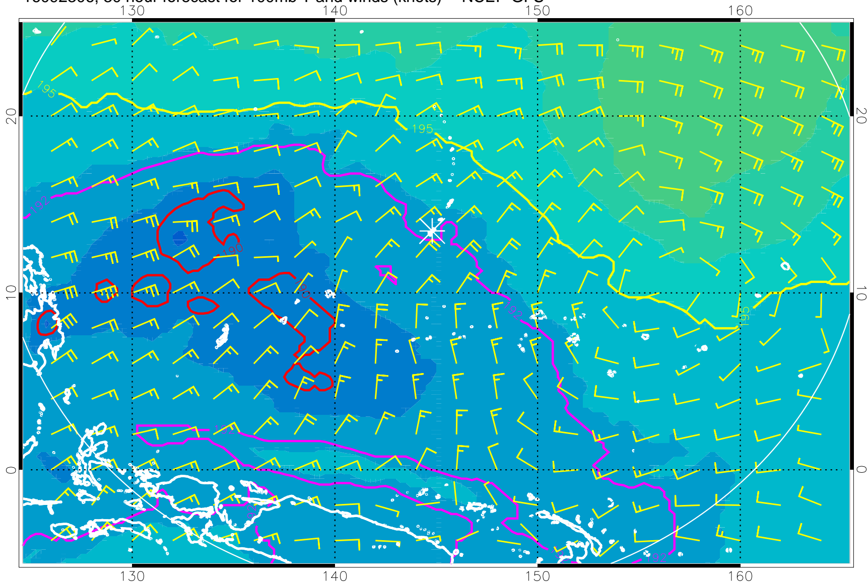
16092306, 30 hour forecast for 100mb T and winds (knots) -- NCEP GFS
