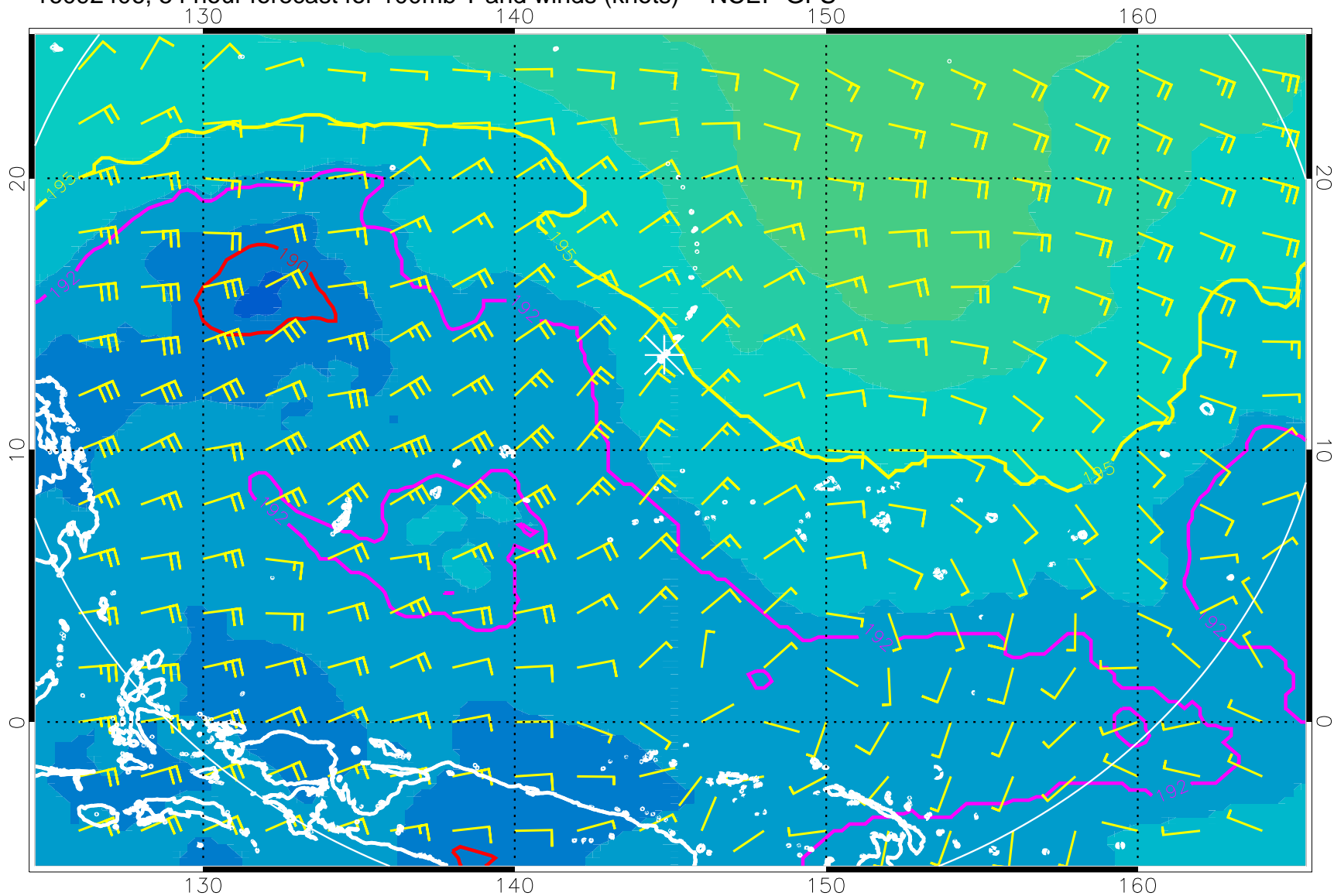
16092406, 54 hour forecast for 100mb T and winds (knots) -- NCEP GFS
