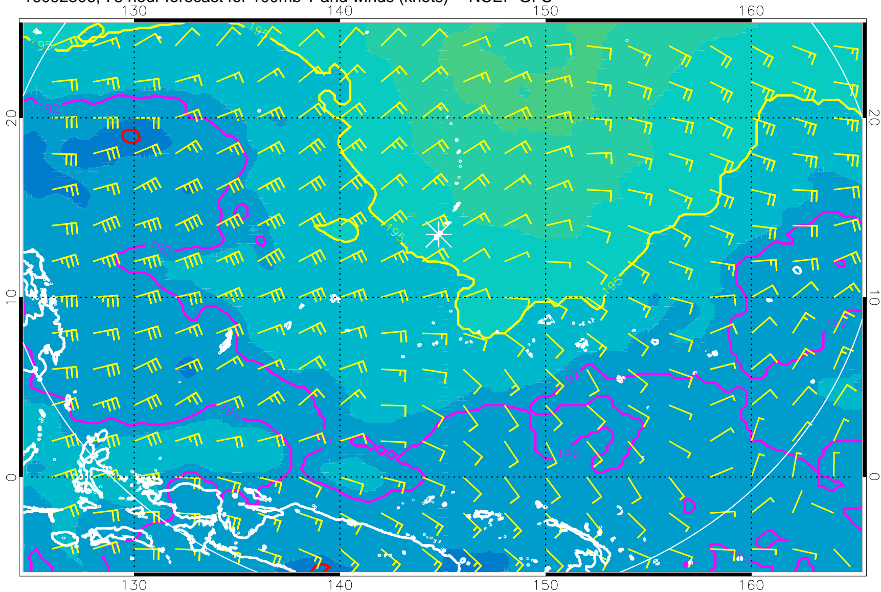
16092506, 78 hour forecast for 100mb T and winds (knots) -- NCEP GFS
