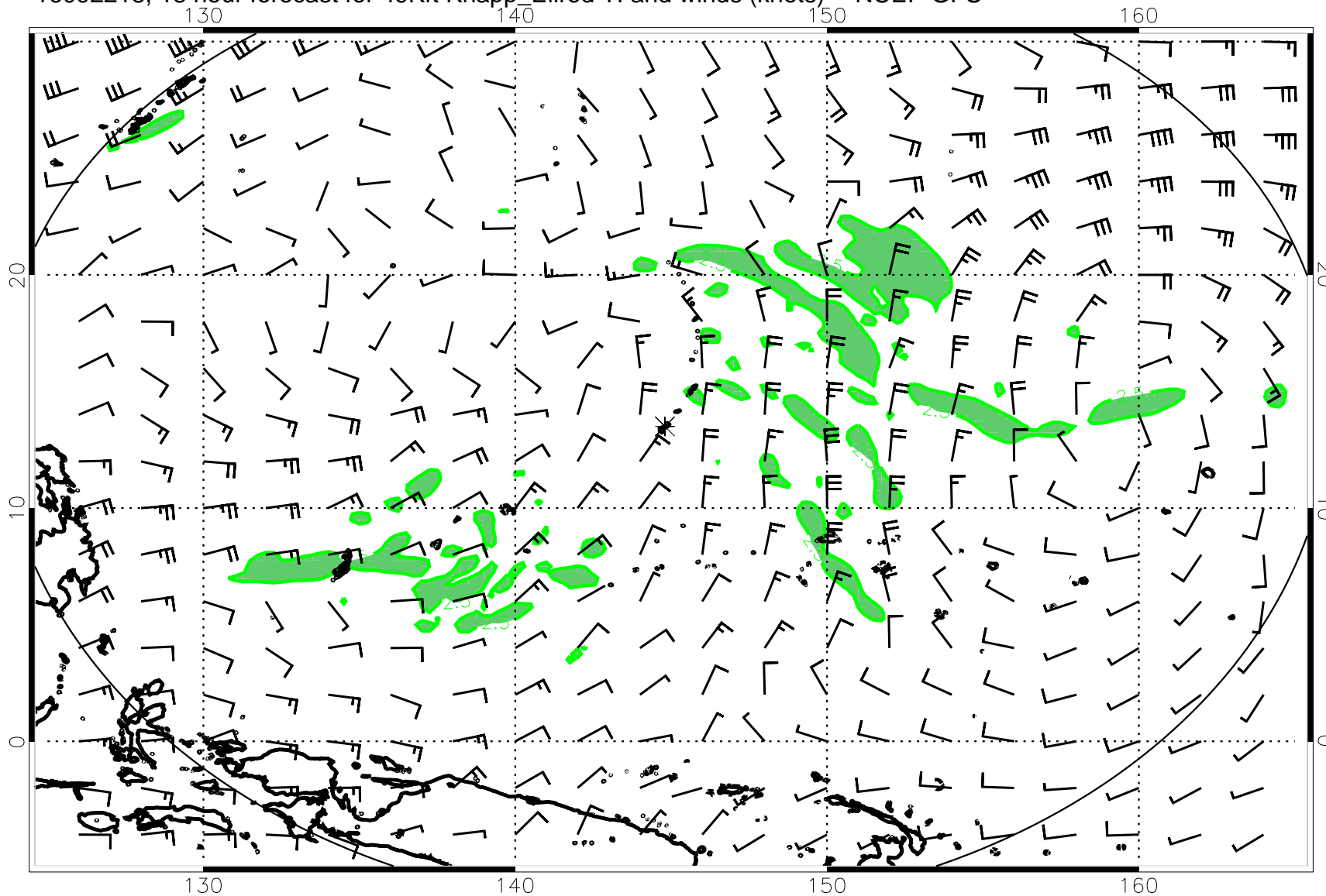
16092218, 18 hour forecast for 49Kft Knapp_Ellrod TI and winds (knots) -- NCEP GFS
