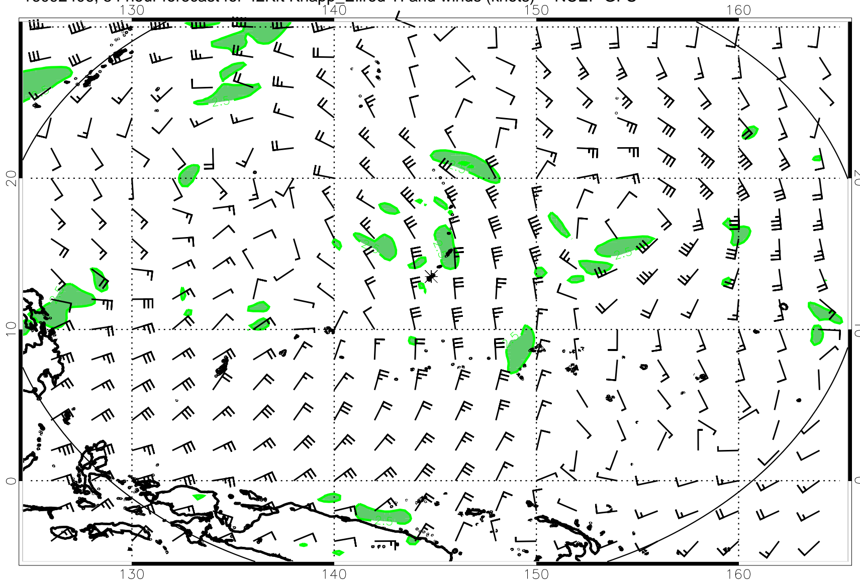
16092406, 54 hour forecast for 42Kft Knapp_Ellrod TI and winds (knots) -- NCEP GFS
