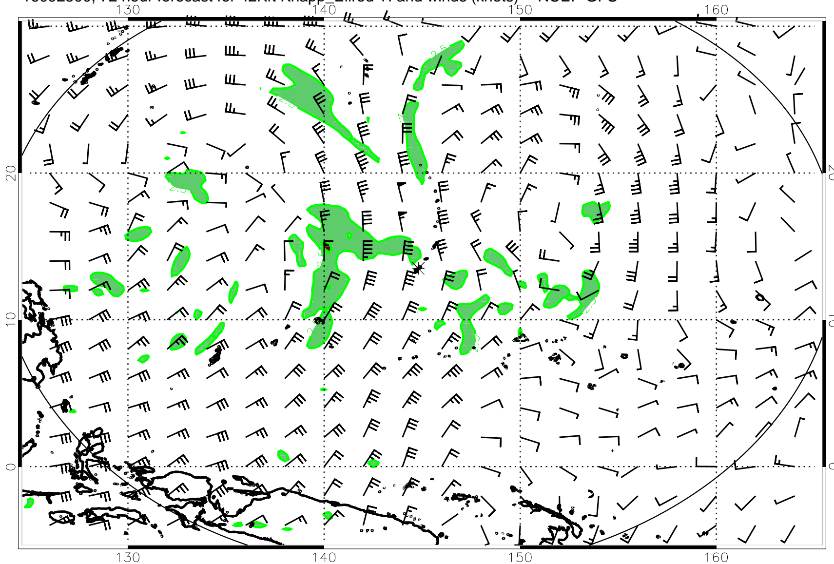
16092500, 72 hour forecast for 42Kft Knapp_Ellrod TI and winds (knots) -- NCEP GFS
