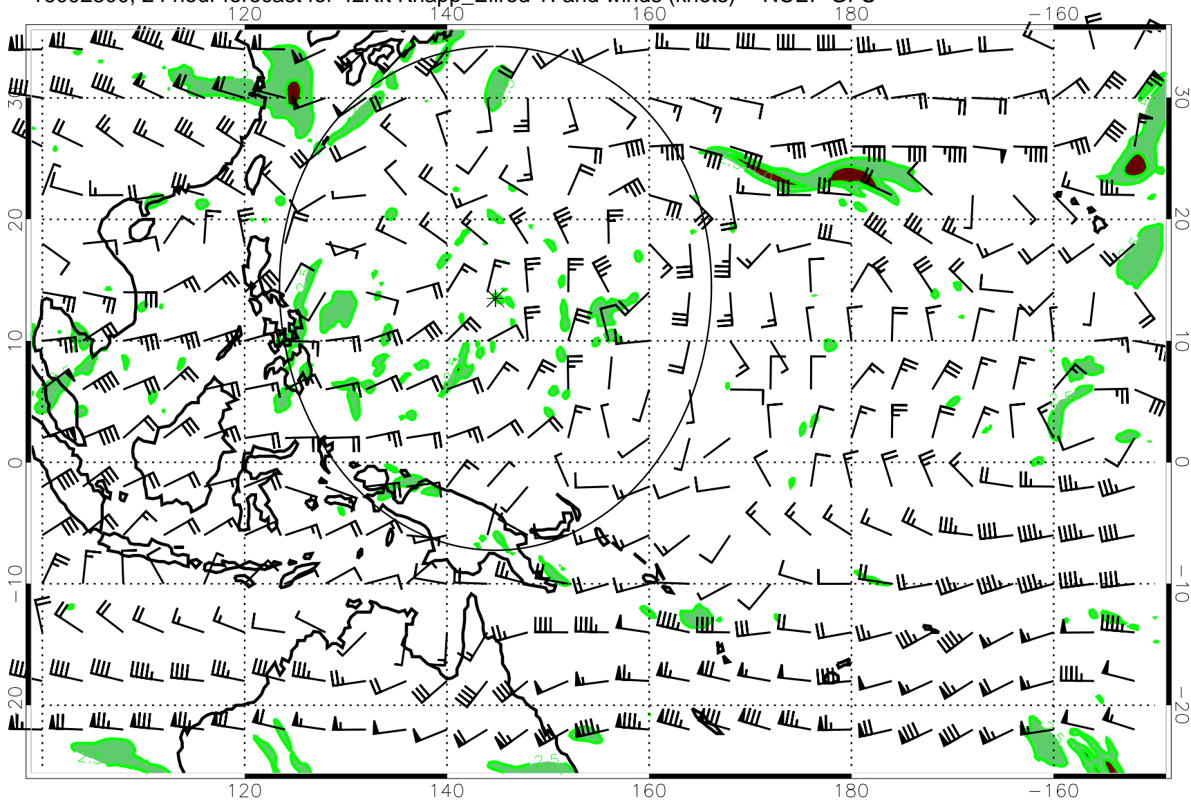
16092300, 24 hour forecast for 42Kft Knapp_Ellrod TI and winds (knots) -- NCEP GFS
