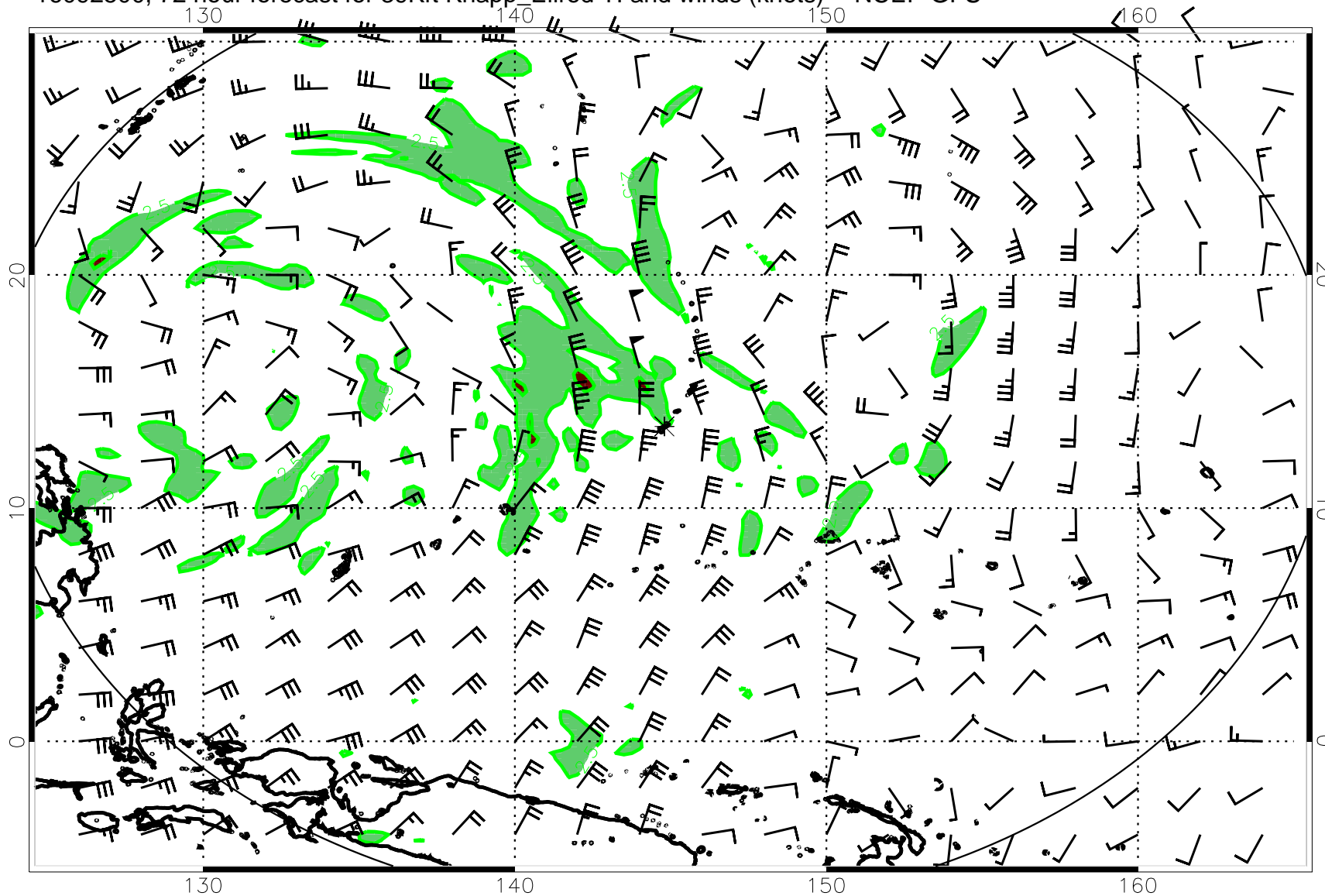
16092500, 72 hour forecast for 39Kft Knapp_Ellrod TI and winds (knots) -- NCEP GFS
