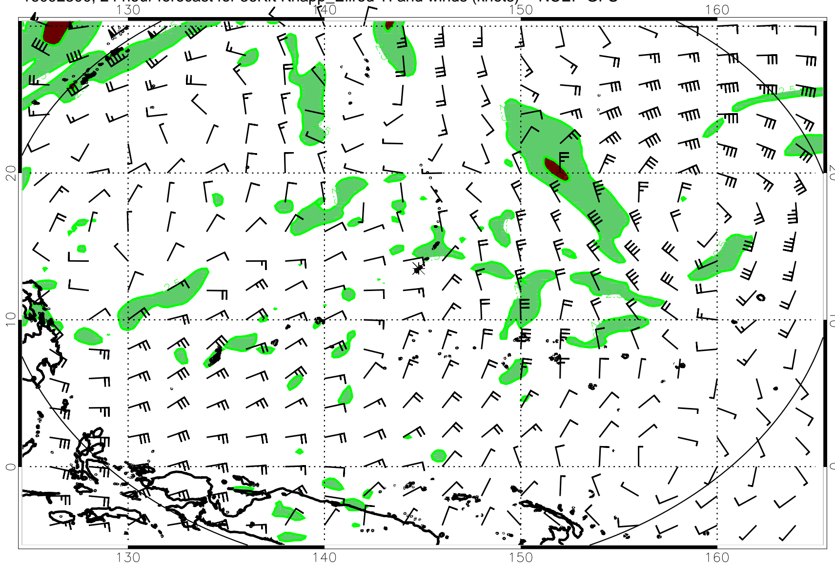
16092300, 24 hour forecast for 36Kft Knapp_Ellrod TI and winds (knots) -- NCEP GFS
