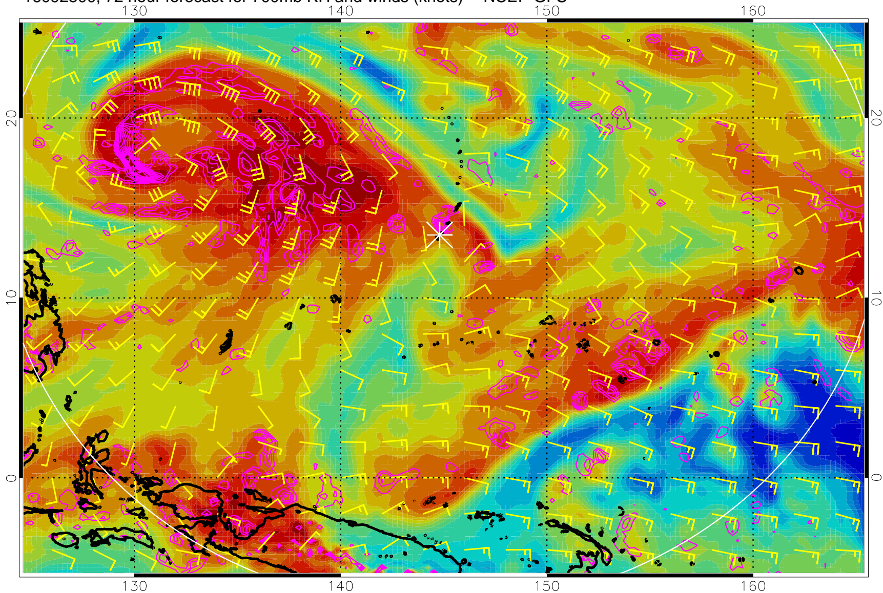
16092500, 72 hour forecast for 700mb RH and winds (knots) -- NCEP GFS
