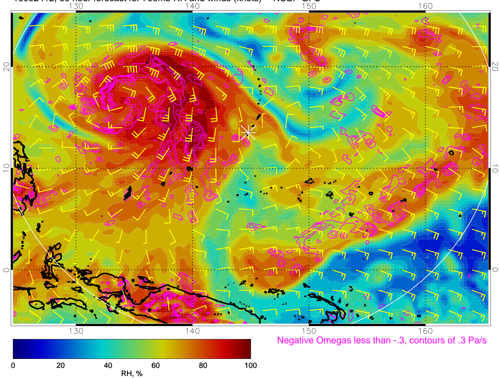
16092412, 60 hour forecast for 700mb RH and winds (knots) -- NCEP GFS
