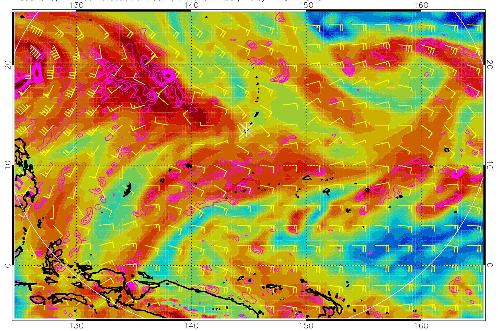
16092618, 114 hour forecast for 700mb RH and winds (knots) -- NCEP GFS
