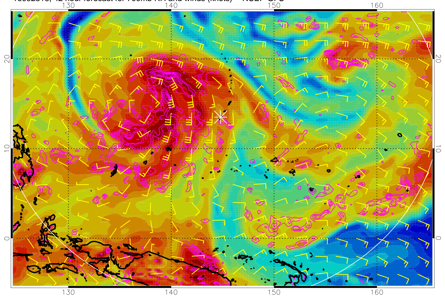
16092318, 42 hour forecast for 700mb RH and winds (knots) -- NCEP GFS
