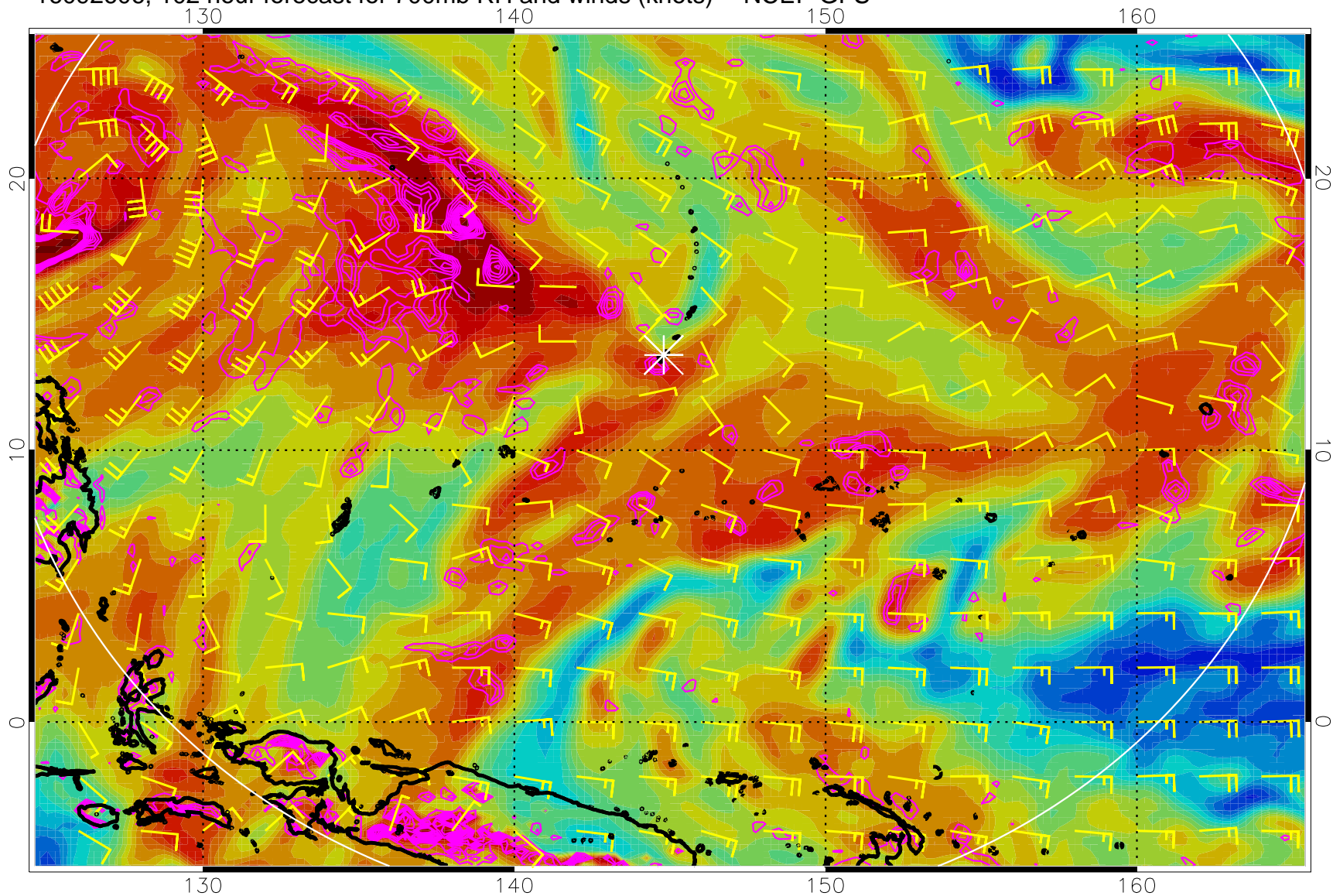
16092606, 102 hour forecast for 700mb RH and winds (knots) -- NCEP GFS
