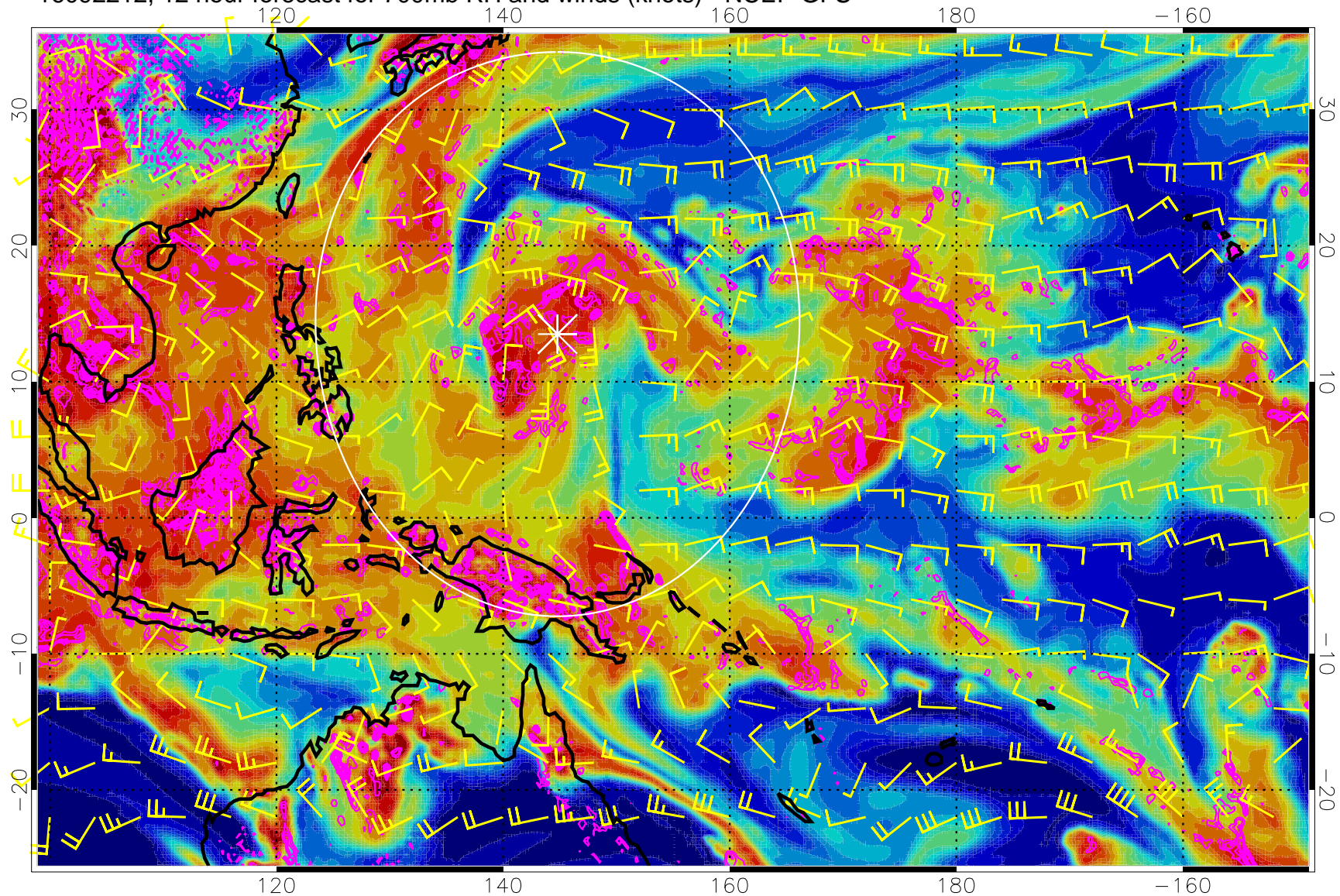
16092212, 12 hour forecast for 700mb RH and winds (knots) - NCEP GFS
