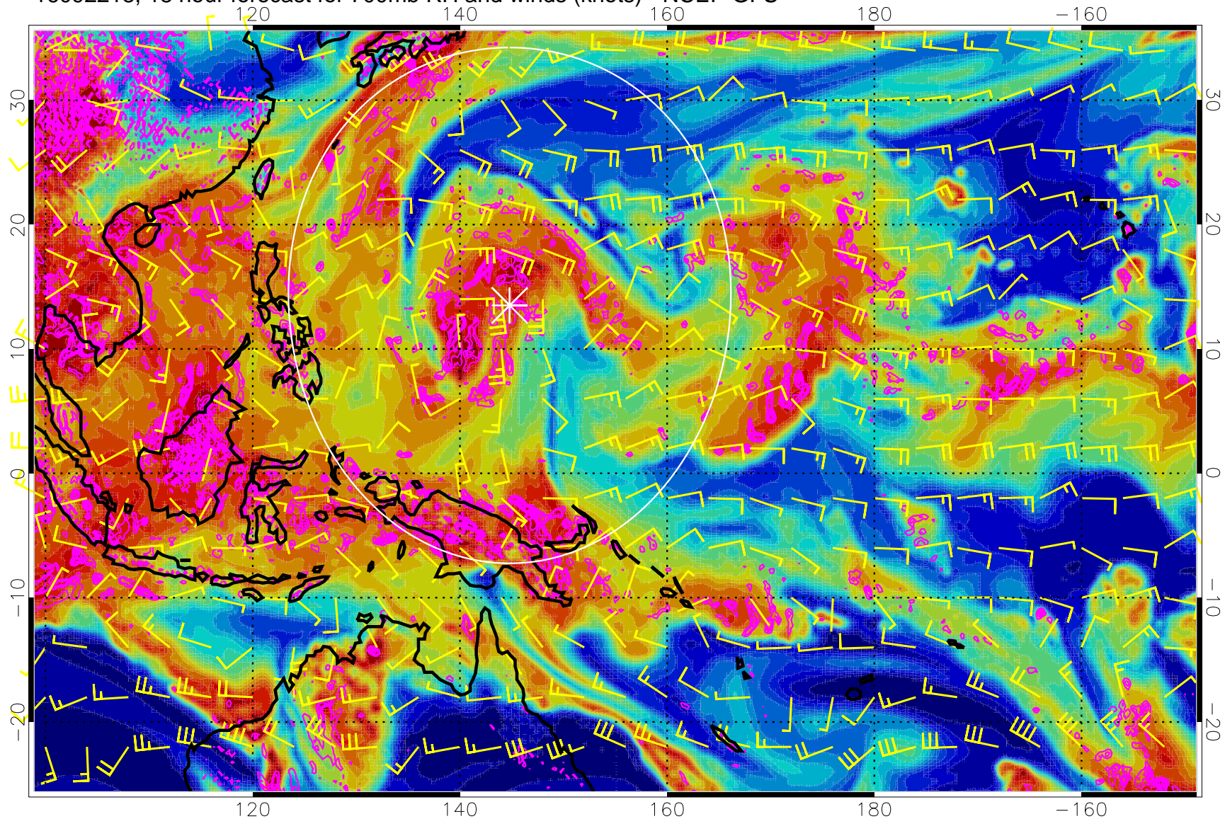
16092218, 18 hour forecast for 700mb RH and winds (knots) - NCEP GFS
