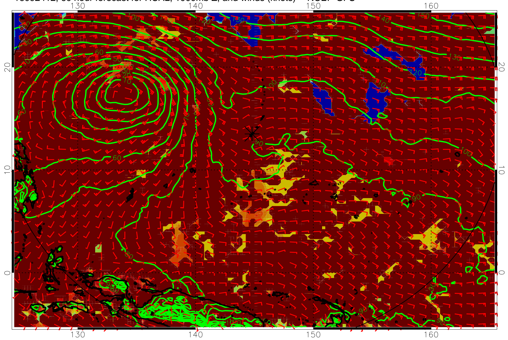
16092412, 60 hour forecast for HCAL, 1000mb Z, and winds (knots) -- NCEP GFS
