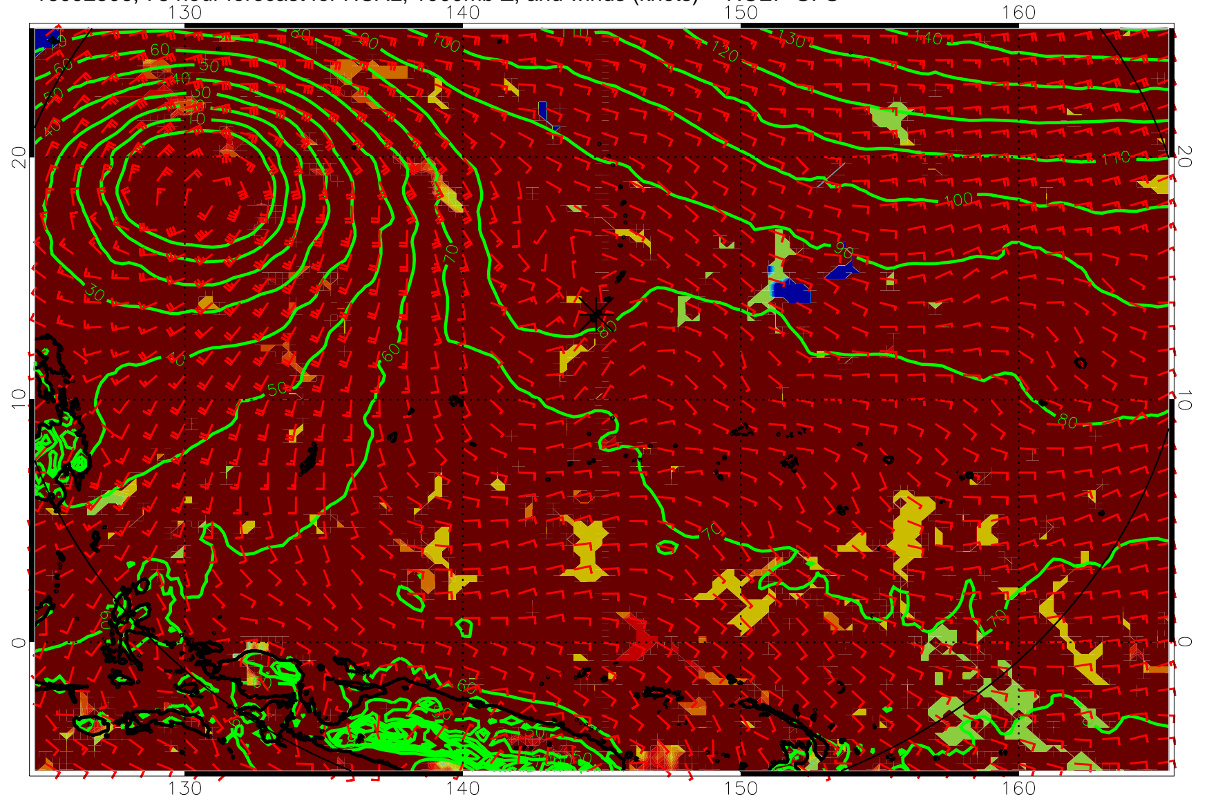
16092506, 78 hour forecast for HCAL, 1000mb Z, and winds (knots) -- NCEP GFS
