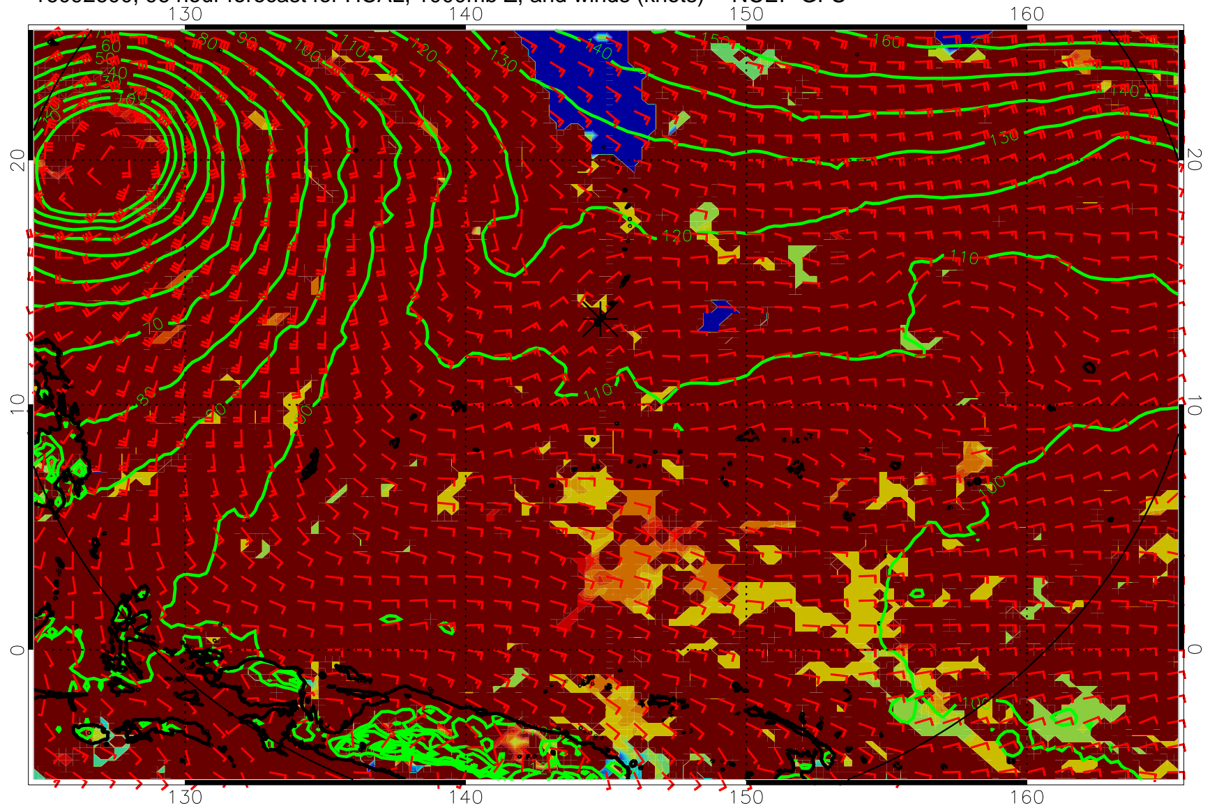
16092600, 96 hour forecast for HCAL, 1000mb Z, and winds (knots) -- NCEP GFS
