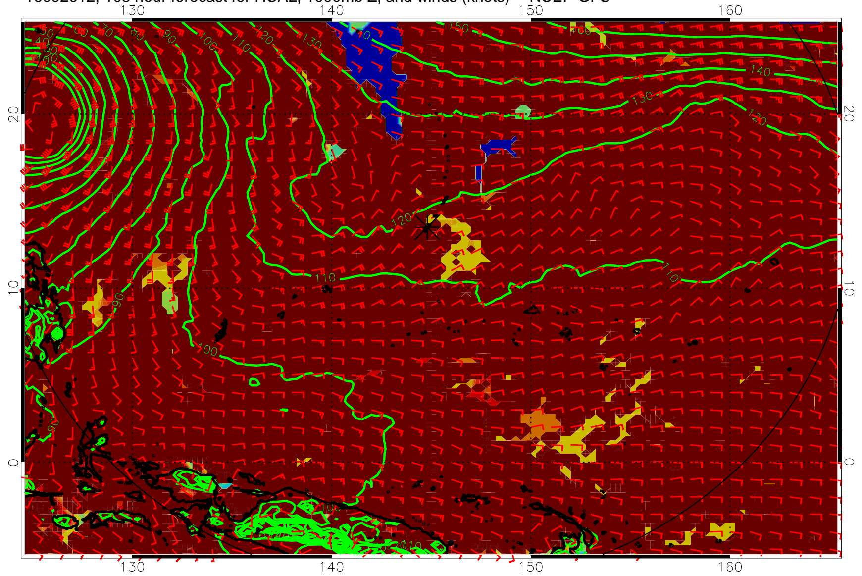
16092612, 108 hour forecast for HCAL, 1000mb Z, and winds (knots) -- NCEP GFS
