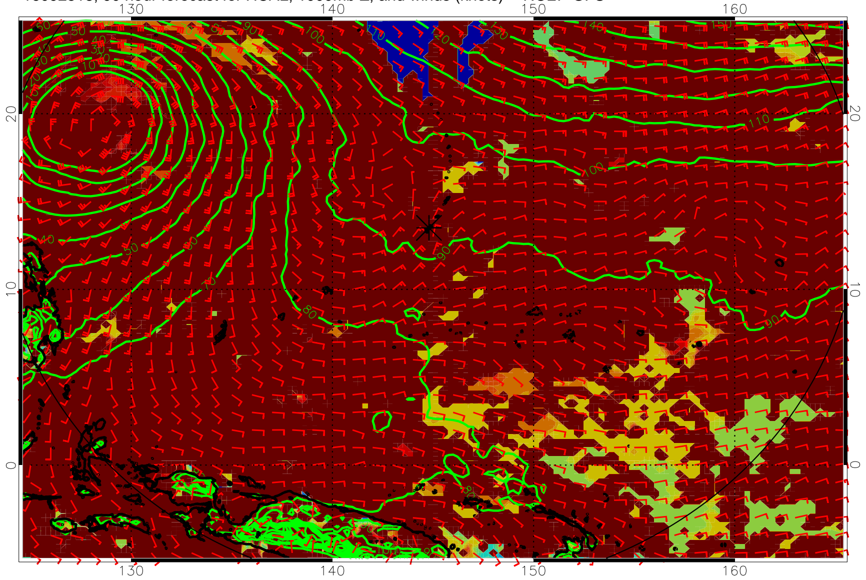
16092518, 90 hour forecast for HCAL, 1000mb Z, and winds (knots) -- NCEP GFS
