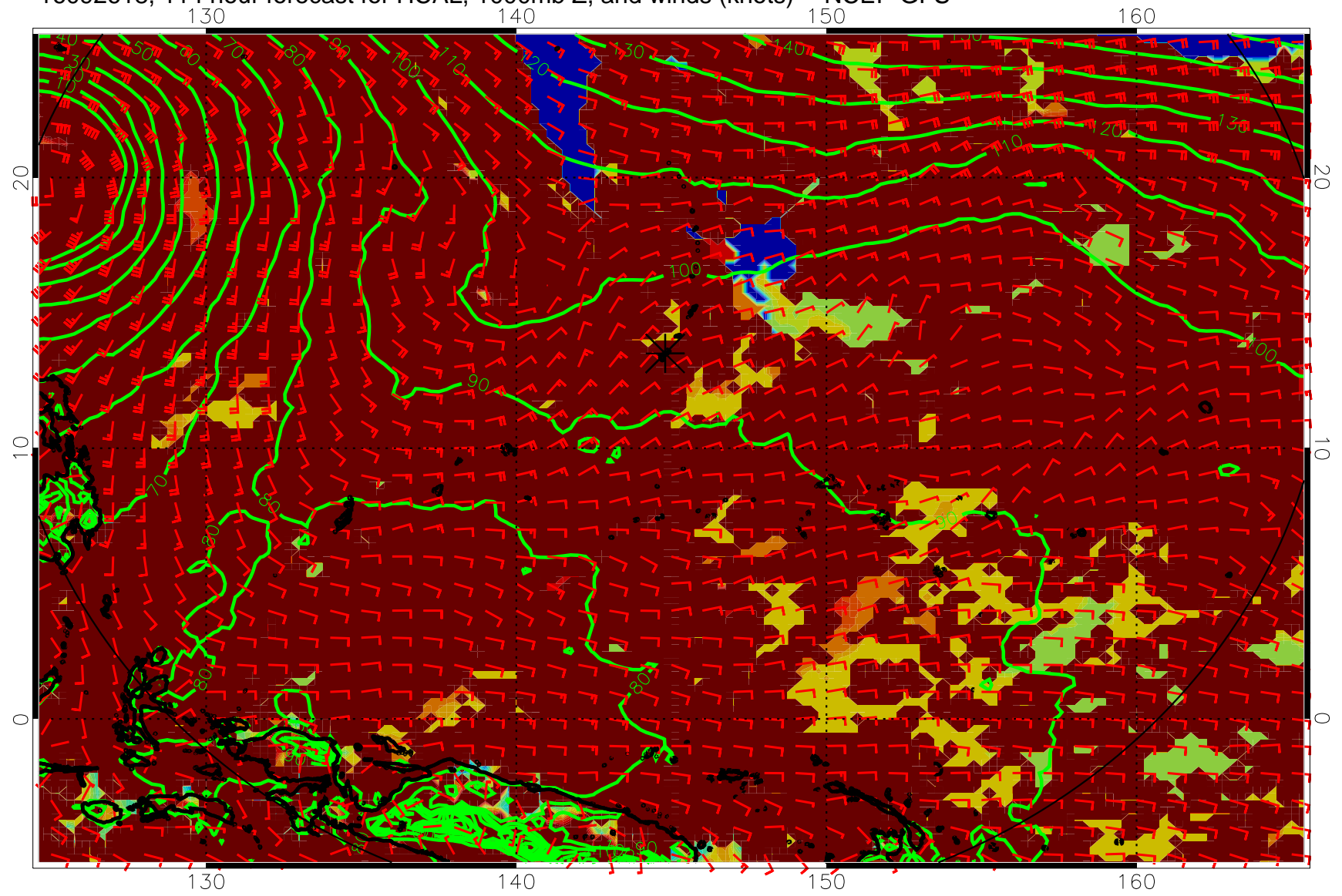
16092618, 114 hour forecast for HCAL, 1000mb Z, and winds (knots) -- NCEP GFS
