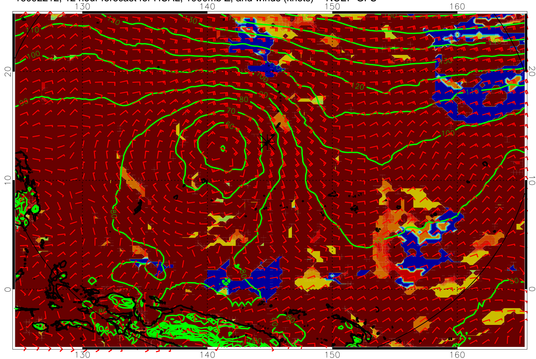
16092212, 12 hour forecast for HCAL, 1000mb Z, and winds (knots) -- NCEP GFS
