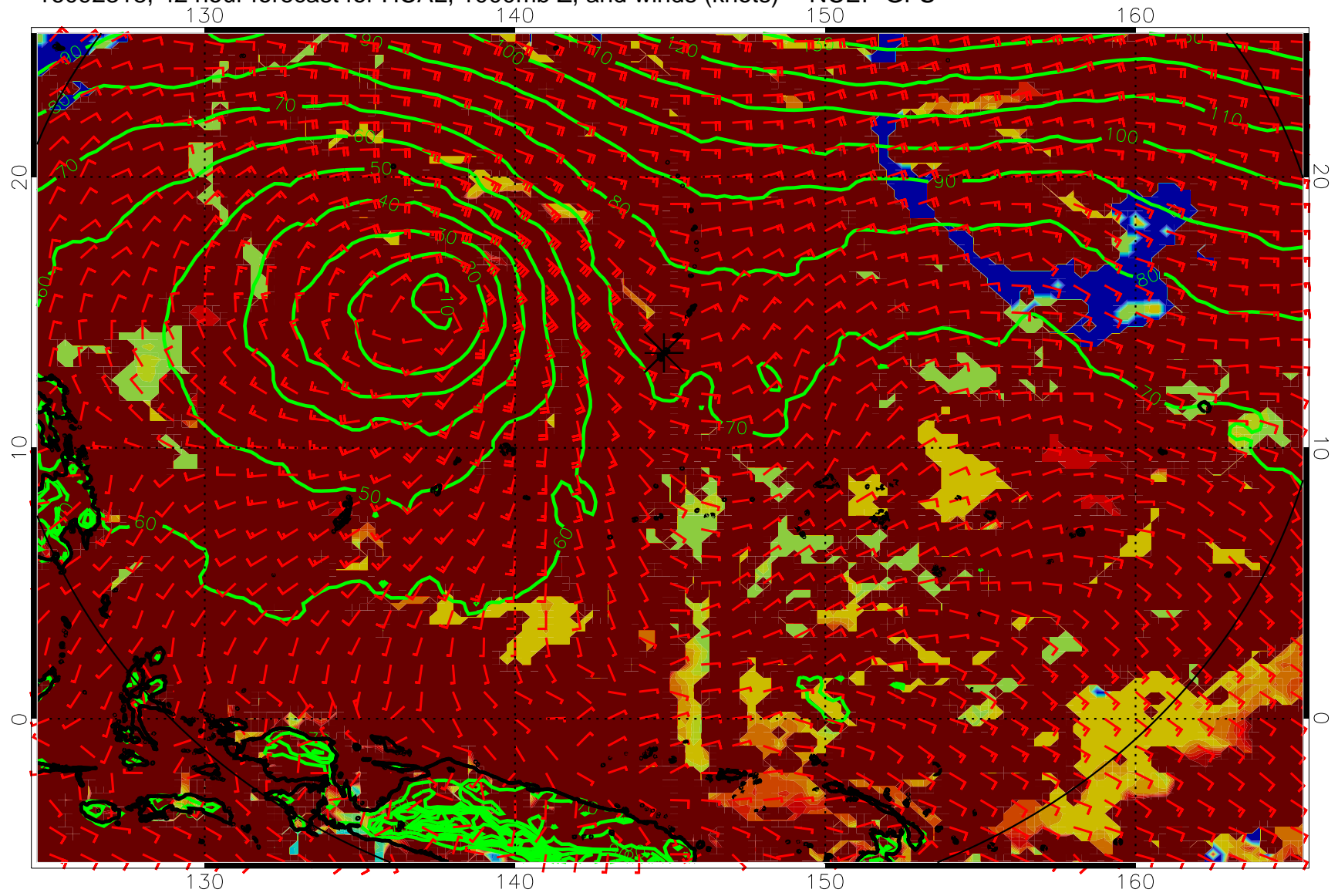
16092318, 42 hour forecast for HCAL, 1000mb Z, and winds (knots) -- NCEP GFS
