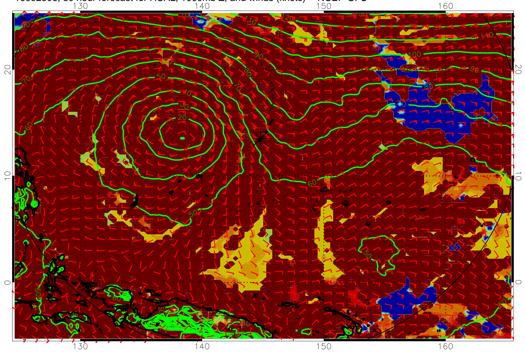
16092306, 30 hour forecast for HCAL, 1000mb Z, and winds (knots) -- NCEP GFS
