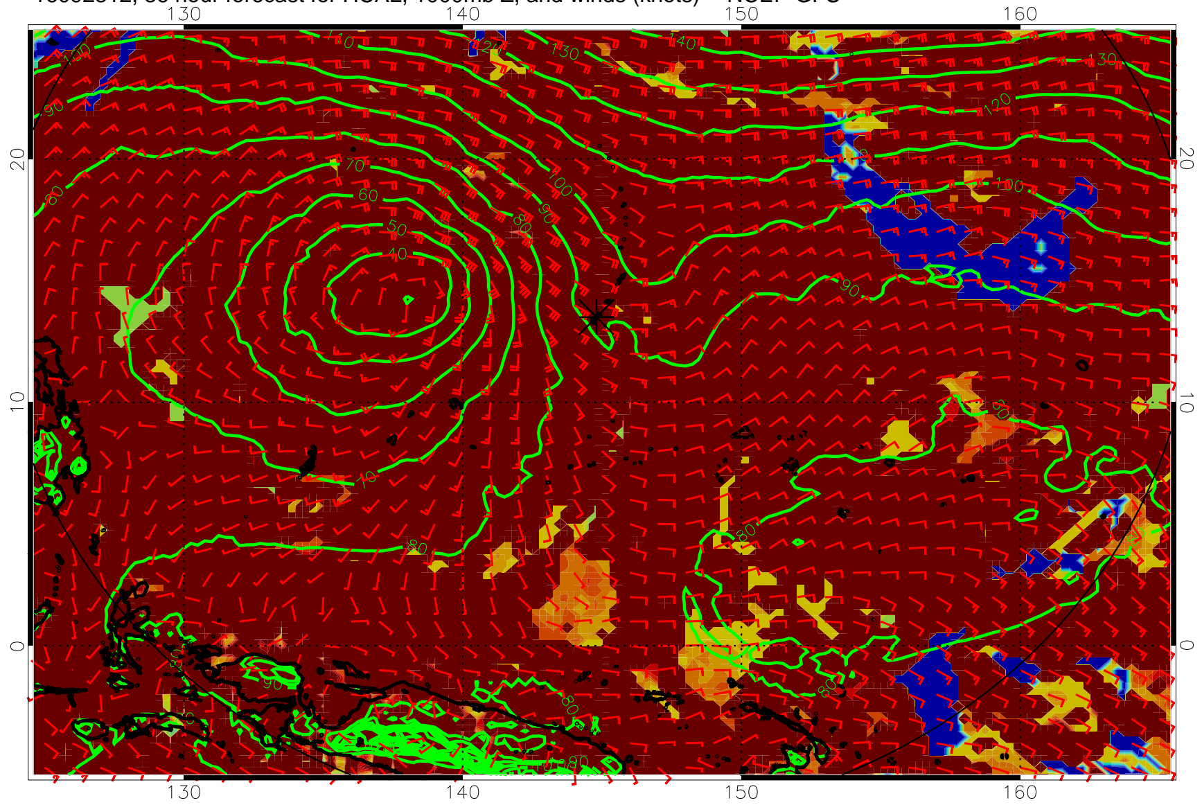
16092312, 36 hour forecast for HCAL, 1000mb Z, and winds (knots) -- NCEP GFS
