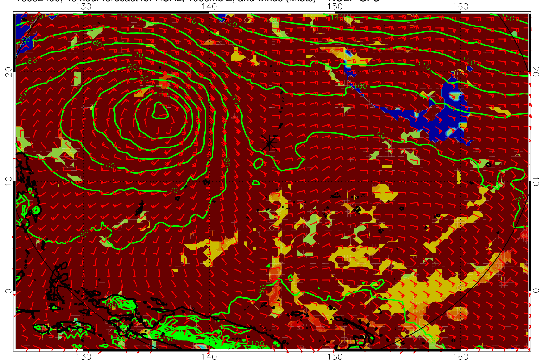
16092400, 48 hour forecast for HCAL, 1000mb Z, and winds (knots) -- NCEP GFS
