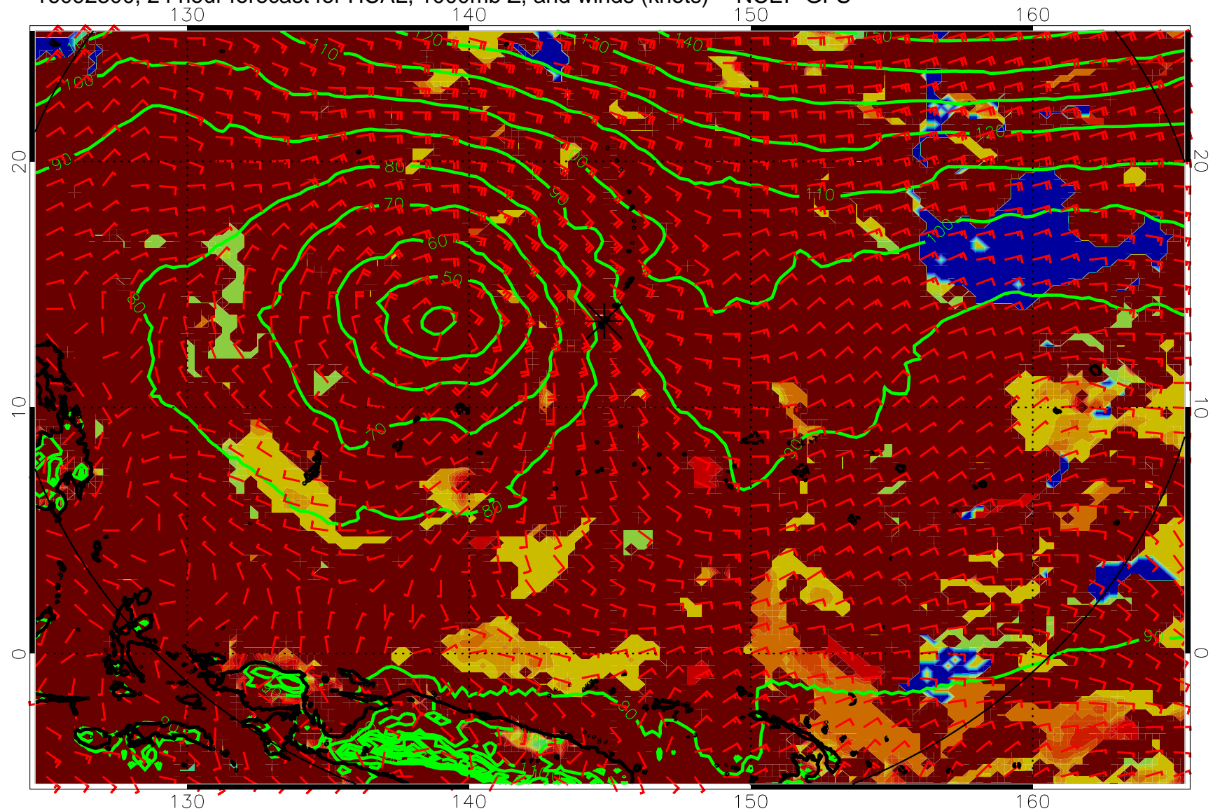
16092300, 24 hour forecast for HCAL, 1000mb Z, and winds (knots) -- NCEP GFS
