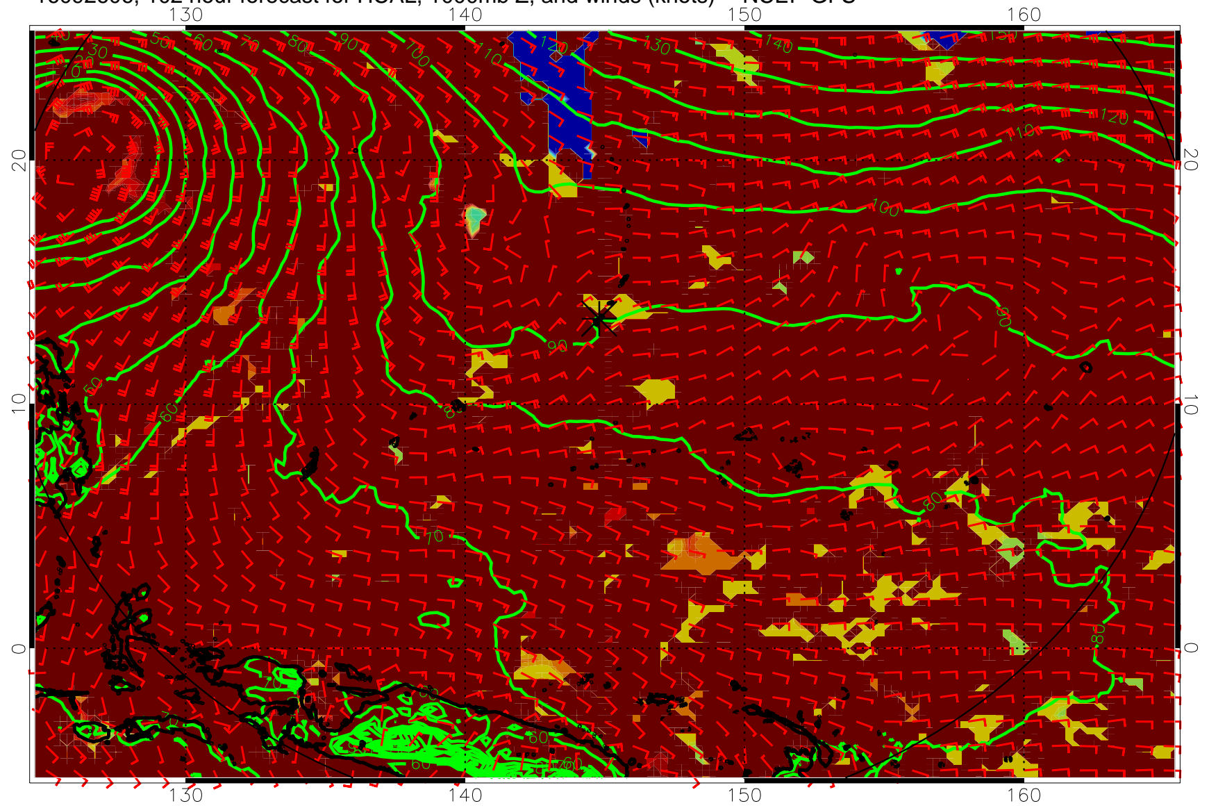
16092606, 102 hour forecast for HCAL, 1000mb Z, and winds (knots) -- NCEP GFS
