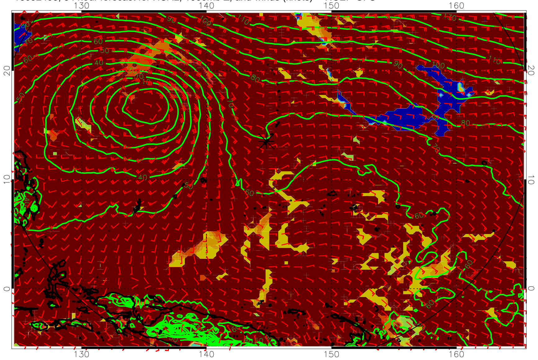
16092406, 54 hour forecast for HCAL, 1000mb Z, and winds (knots) -- NCEP GFS
