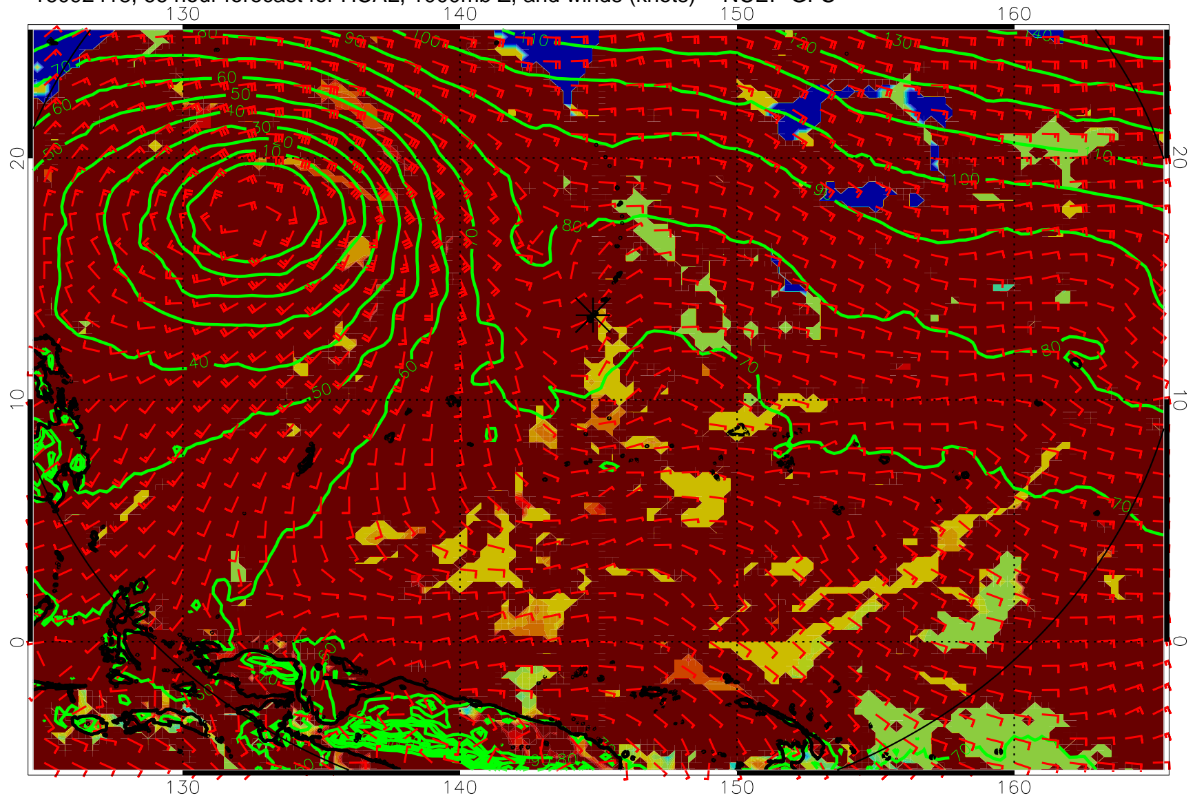
16092418, 66 hour forecast for HCAL, 1000mb Z, and winds (knots) -- NCEP GFS
