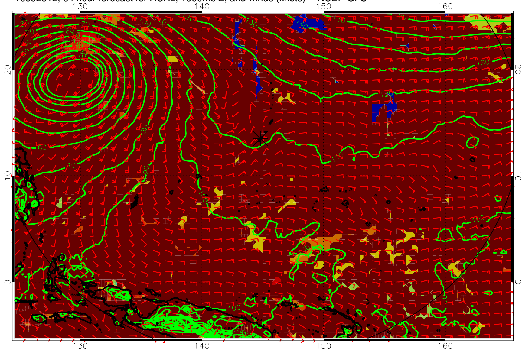
16092512, 84 hour forecast for HCAL, 1000mb Z, and winds (knots) -- NCEP GFS
