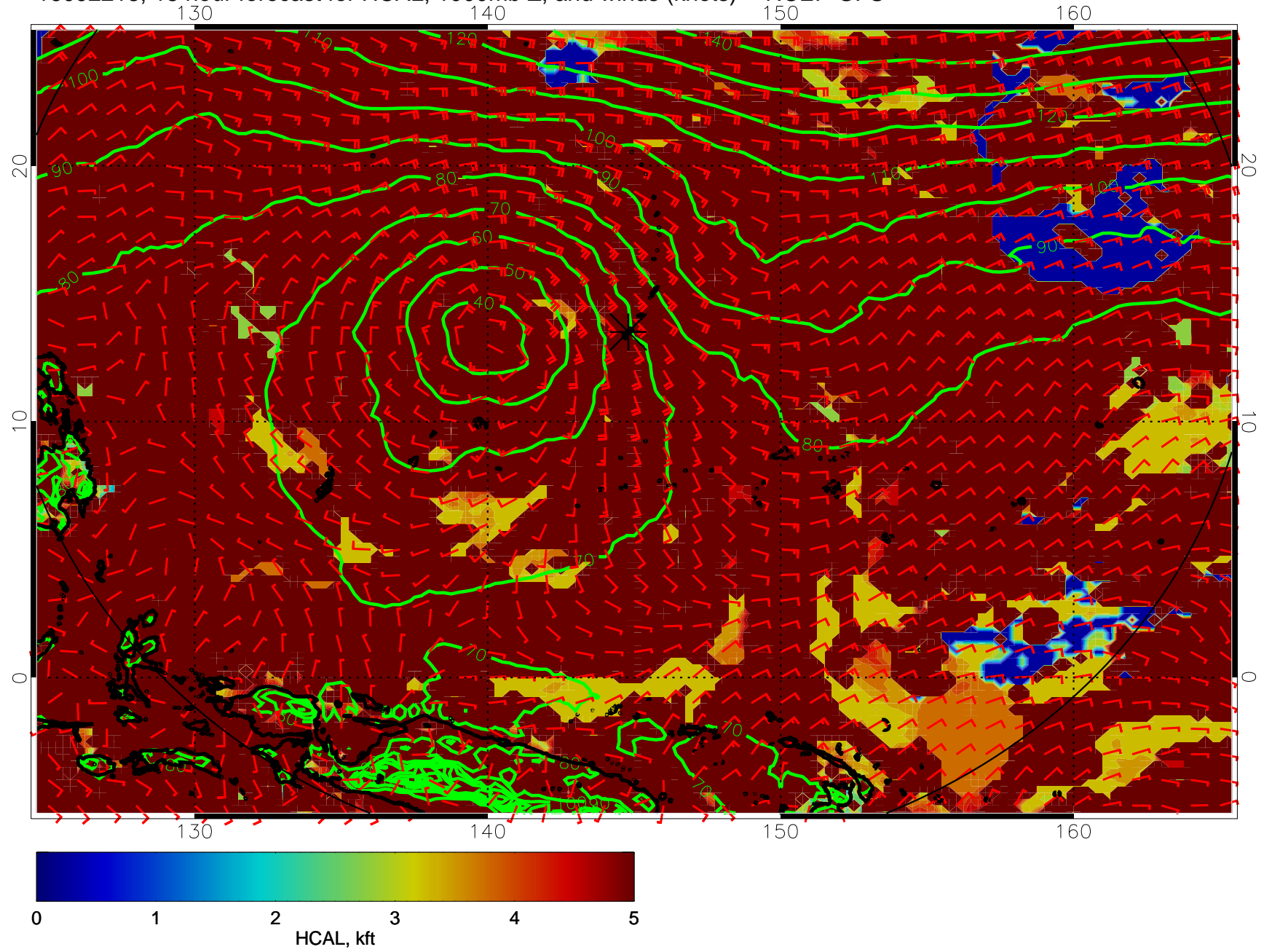
16092218, 18 hour forecast for HCAL, 1000mb Z, and winds (knots) -- NCEP GFS
