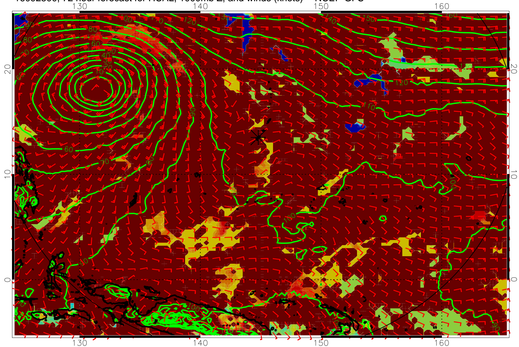
16092500, 72 hour forecast for HCAL, 1000mb Z, and winds (knots) -- NCEP GFS
