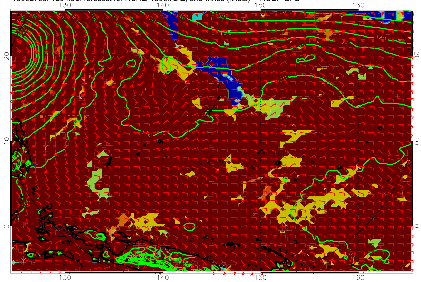
16092700, 120 hour forecast for HCAL, 1000mb Z, and winds (knots) -- NCEP GFS
