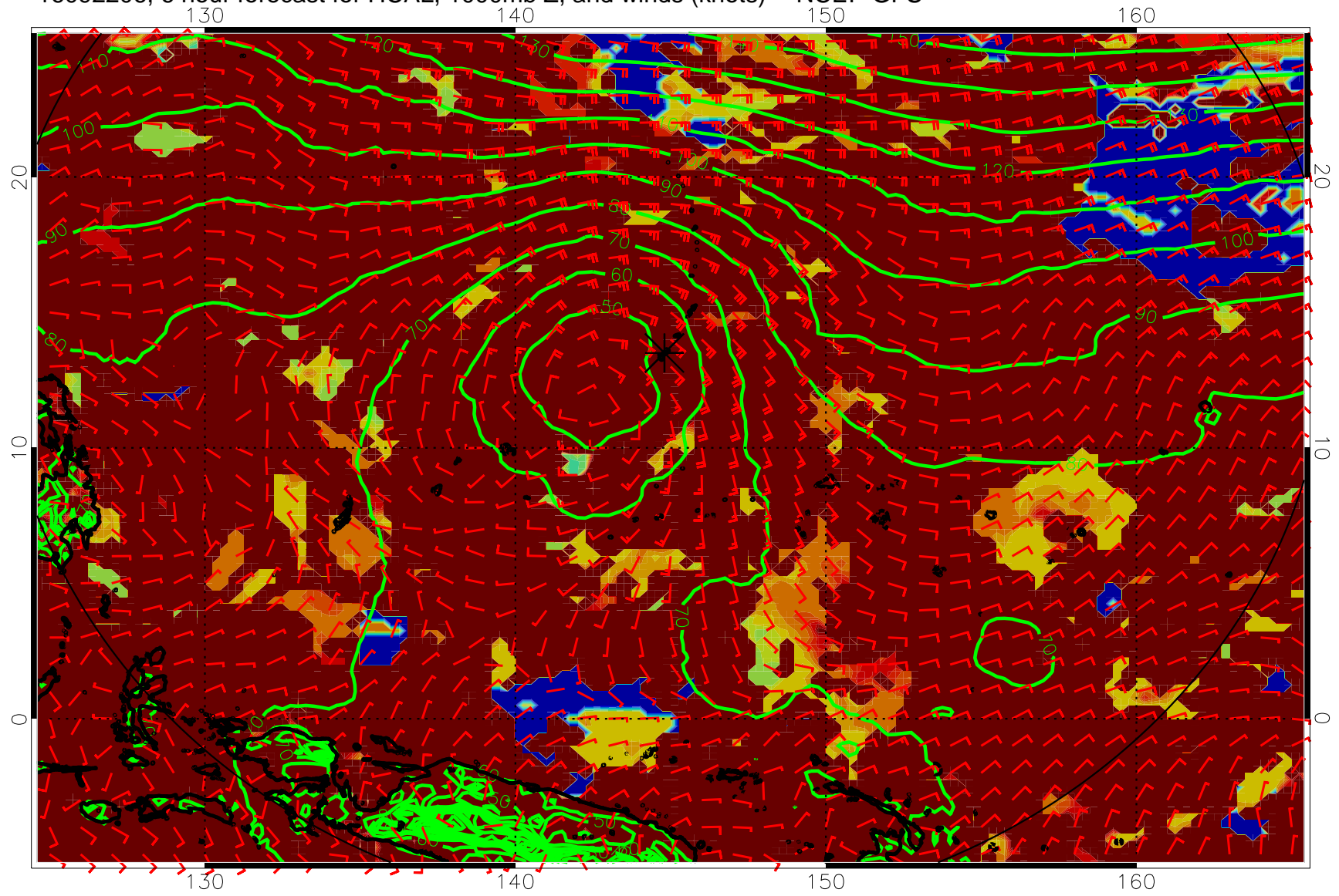
16092206, 6 hour forecast for HCAL, 1000mb Z, and winds (knots) -- NCEP GFS
