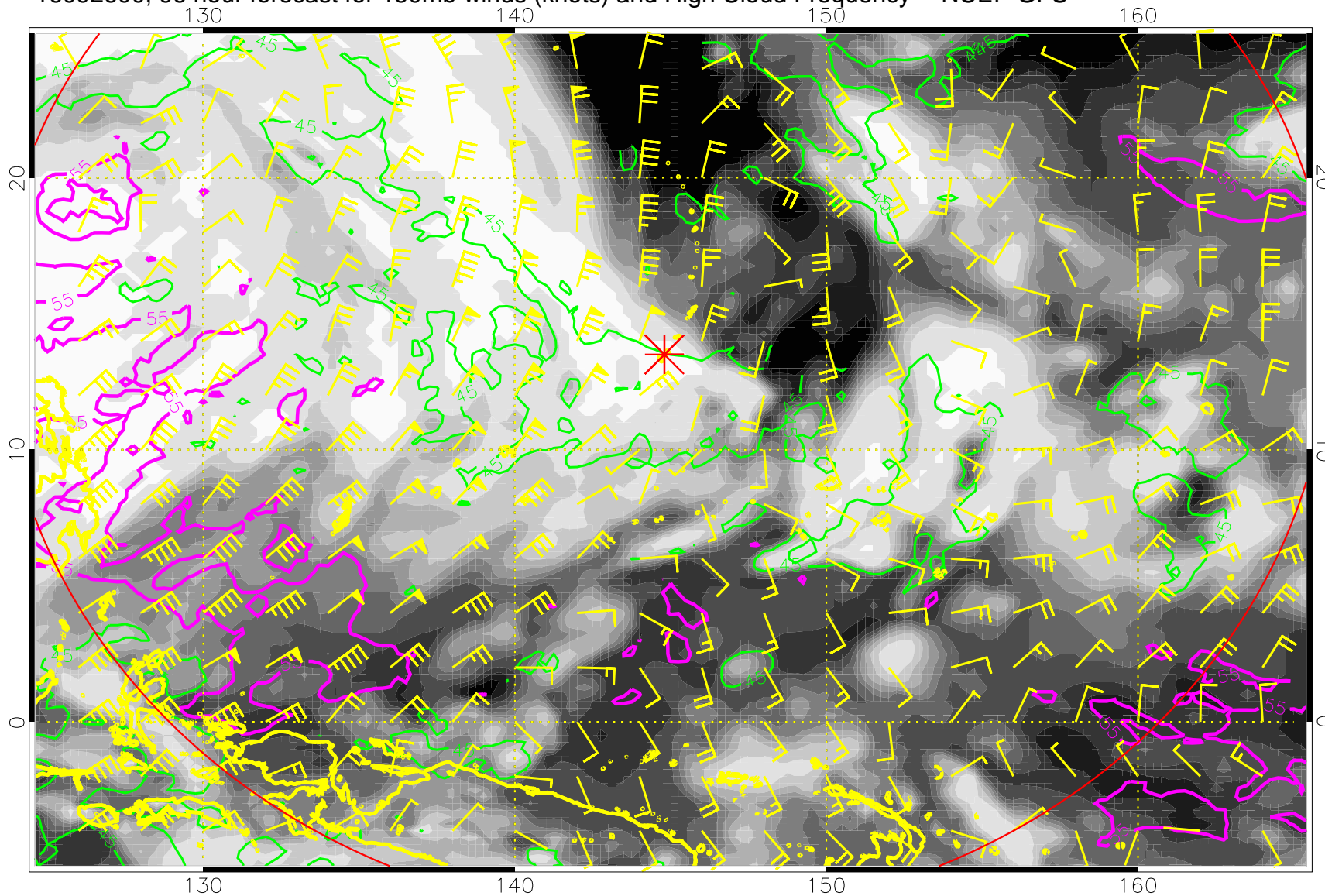
16092600, 96 hour forecast for 150mb winds (knots) and High Cloud Frequency -- NCEP GFS
