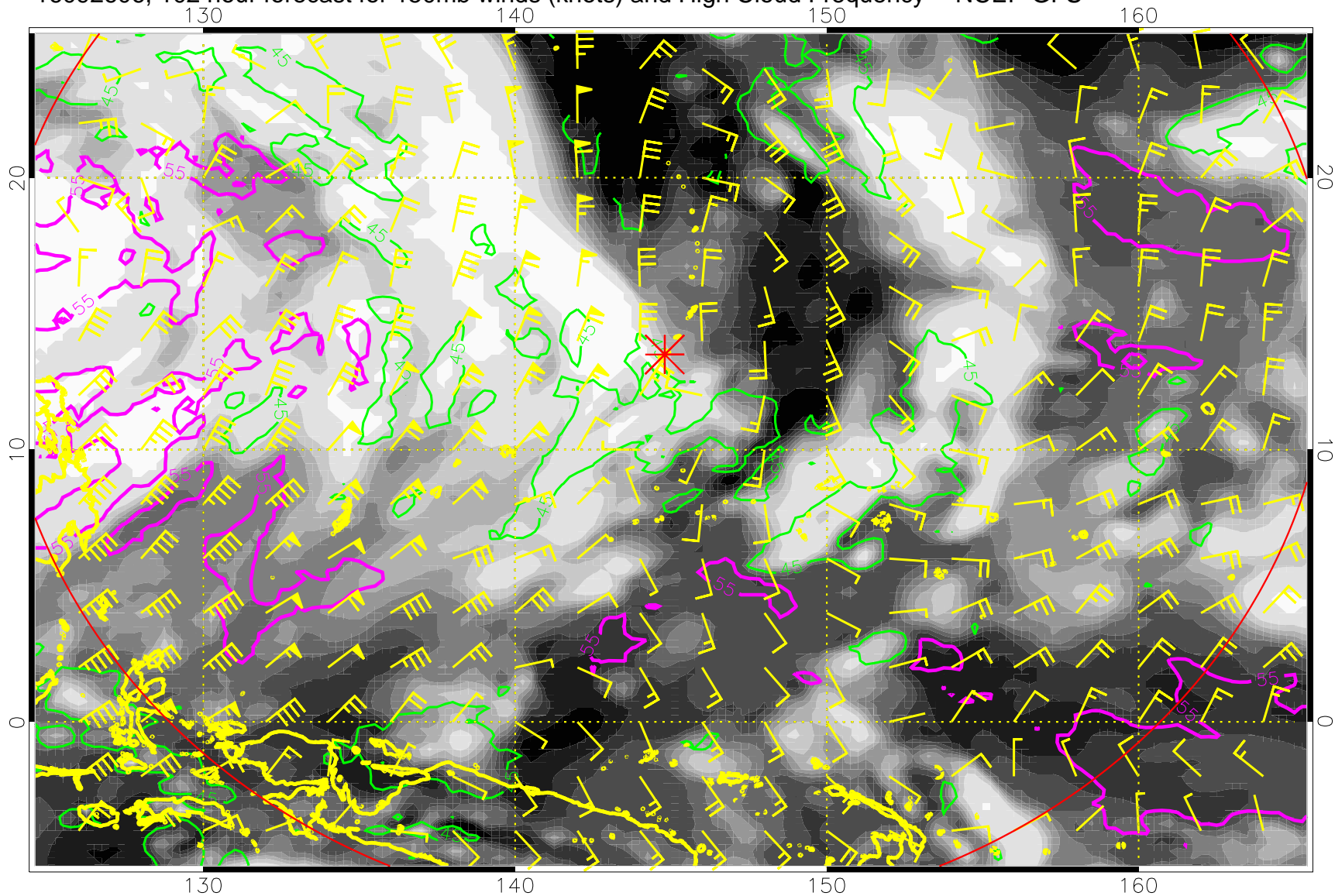
16092606, 102 hour forecast for 150mb winds (knots) and High Cloud Frequency -- NCEP GFS
