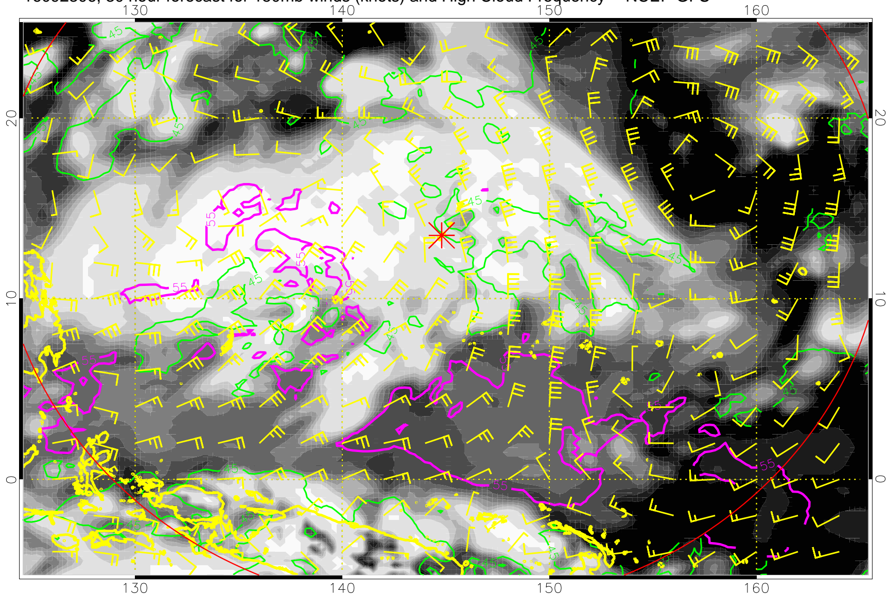
16092306, 30 hour forecast for 150mb winds (knots) and High Cloud Frequency -- NCEP GFS
