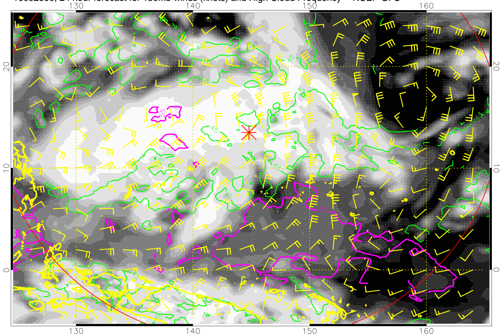
16092300, 24 hour forecast for 150mb winds (knots) and High Cloud Frequency -- NCEP GFS
