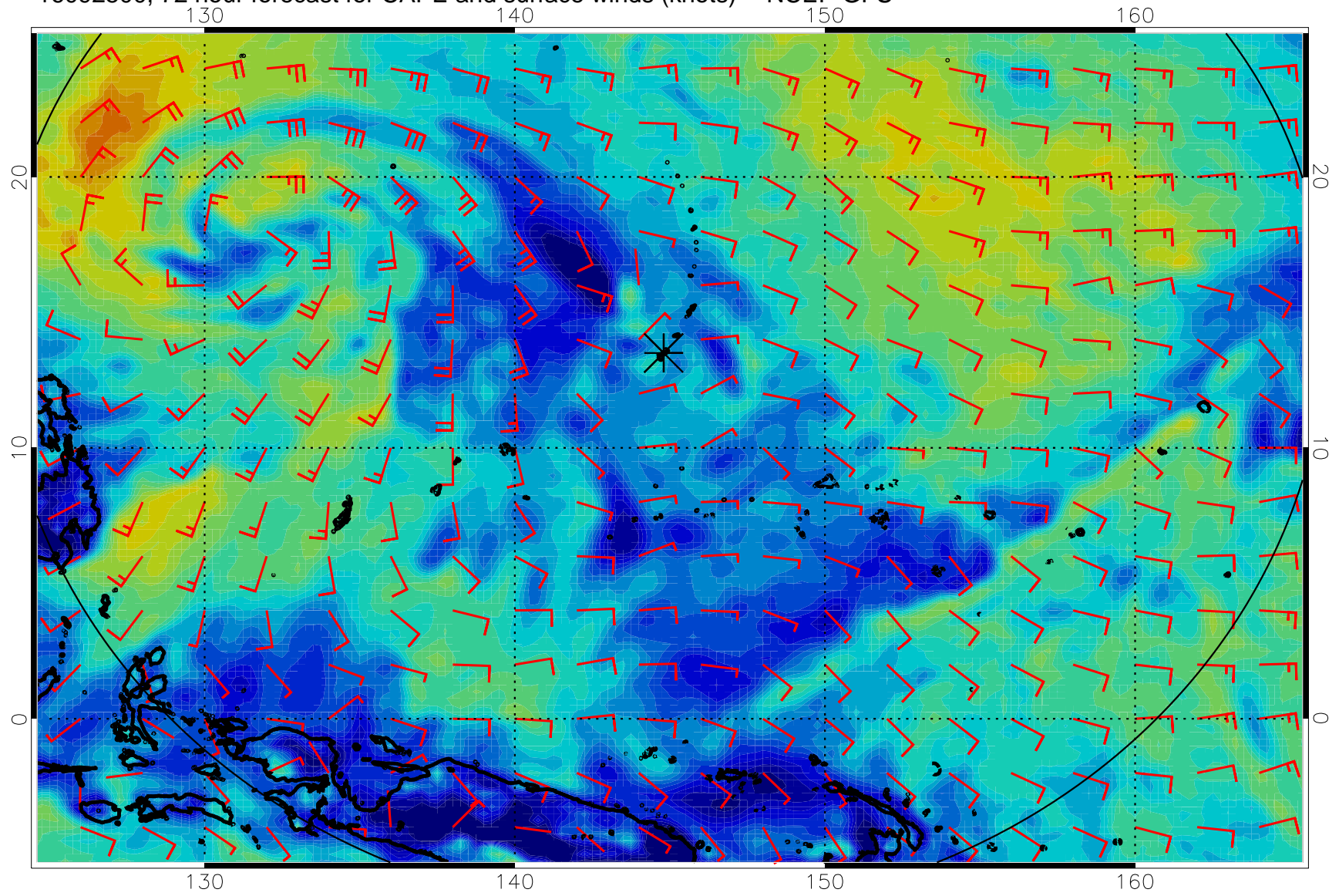
16092500, 72 hour forecast for CAPE and surface winds (knots) -- NCEP GFS
