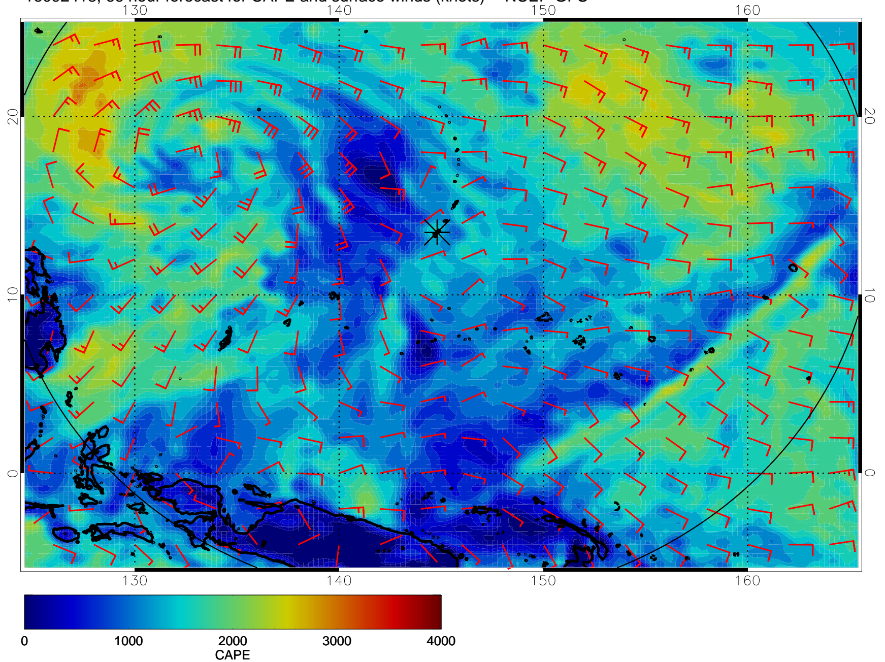
16092418, 66 hour forecast for CAPE and surface winds (knots) -- NCEP GFS
