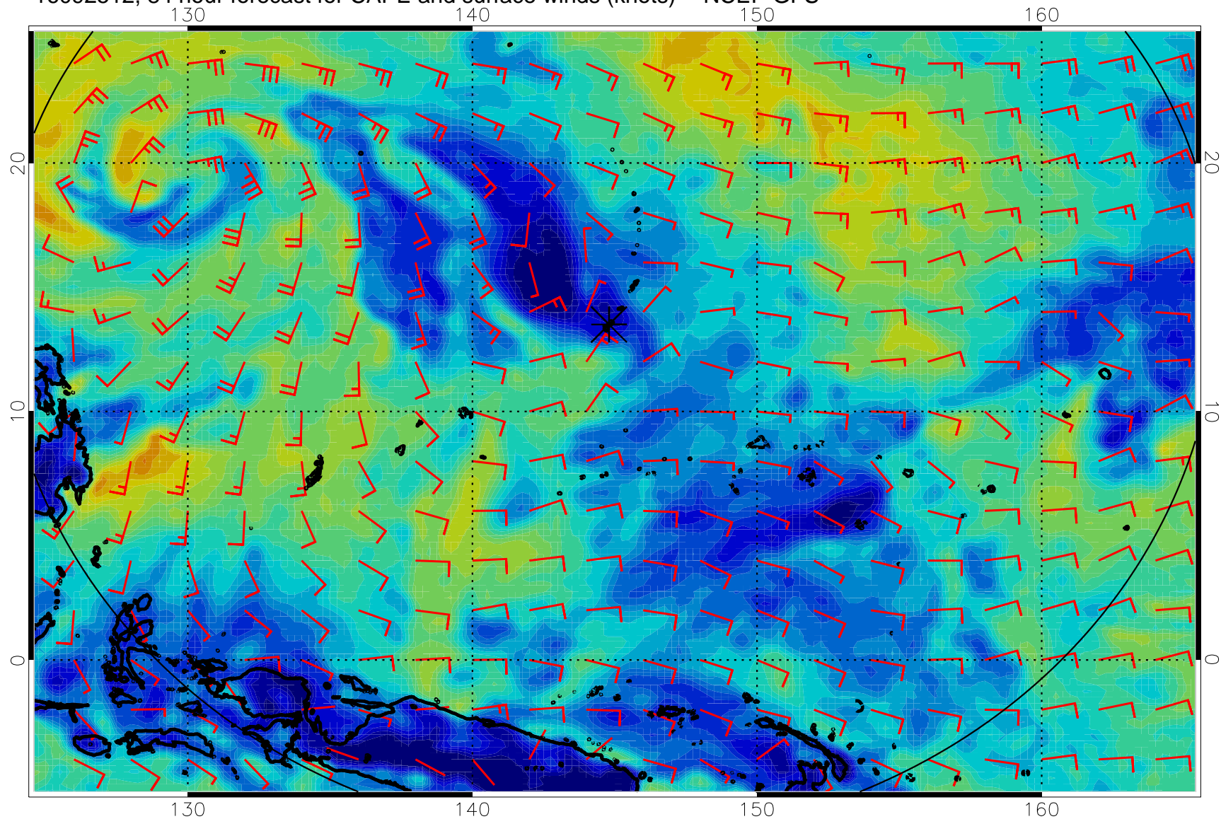
16092512, 84 hour forecast for CAPE and surface winds (knots) -- NCEP GFS
