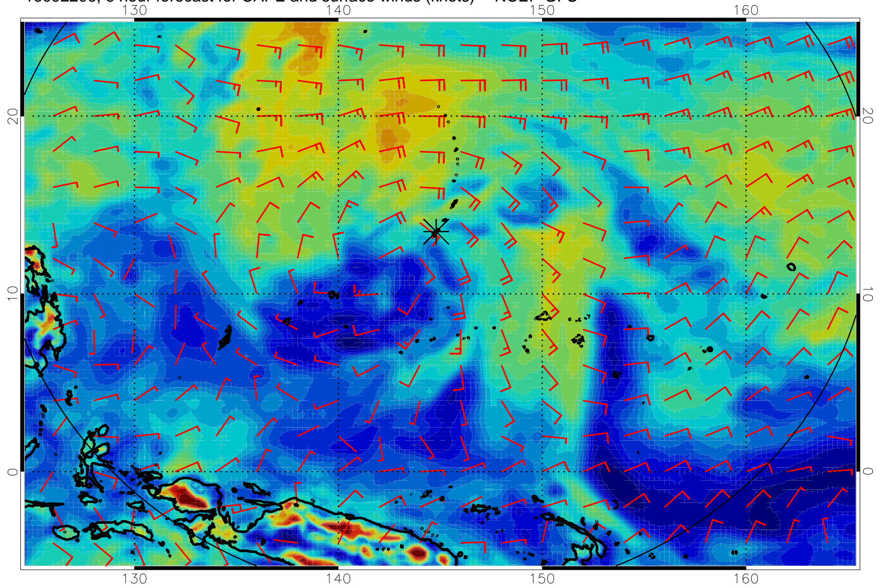
16092206, 6 hour forecast for CAPE and surface winds (knots) -- NCEP GFS
