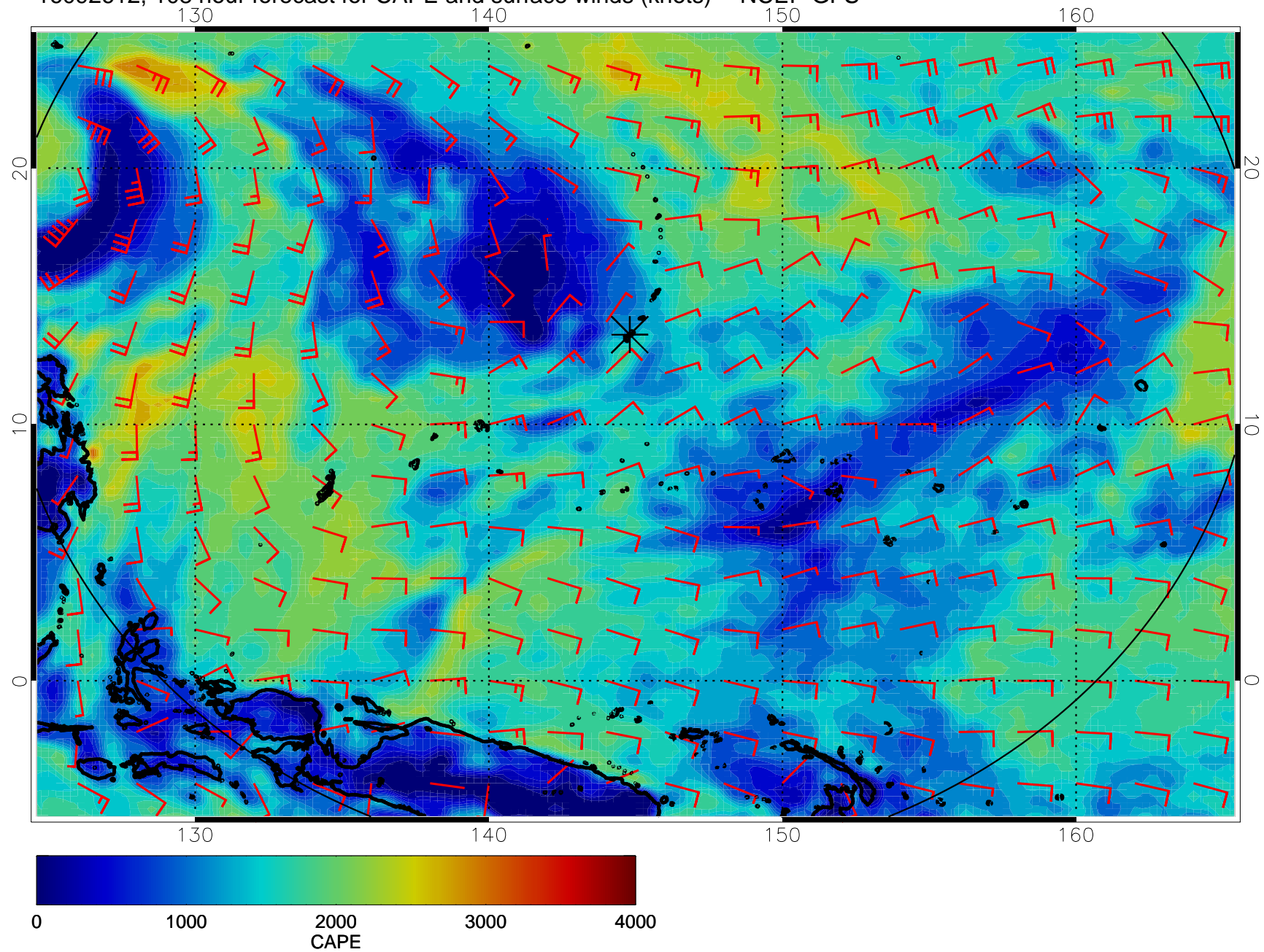
16092612, 108 hour forecast for CAPE and surface winds (knots) -- NCEP GFS
