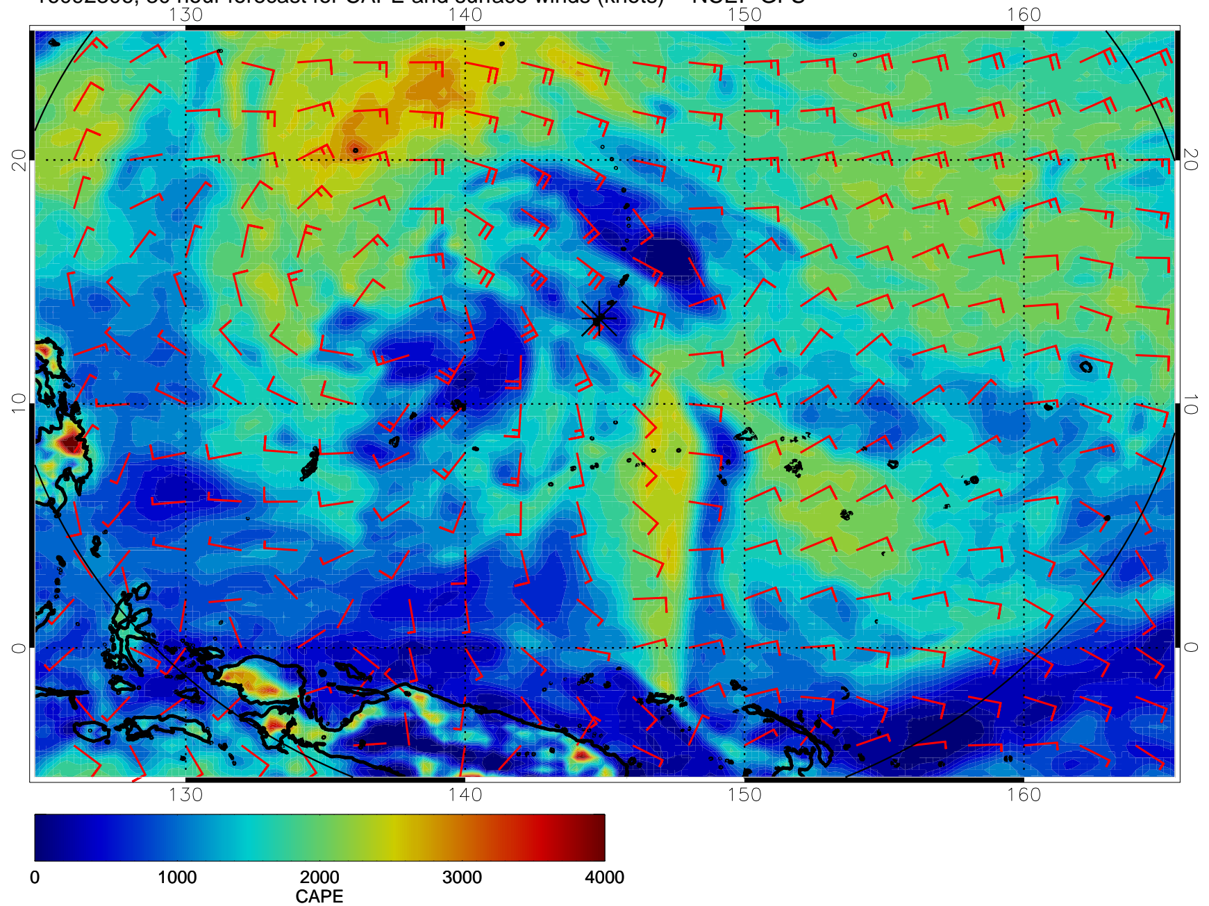
16092306, 30 hour forecast for CAPE and surface winds (knots) -- NCEP GFS
