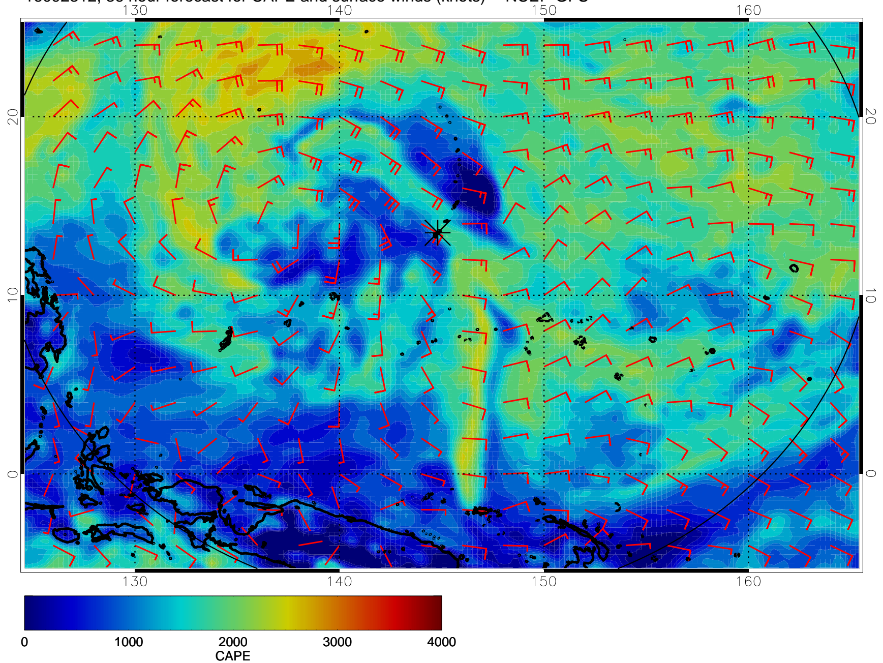
16092312, 36 hour forecast for CAPE and surface winds (knots) -- NCEP GFS
