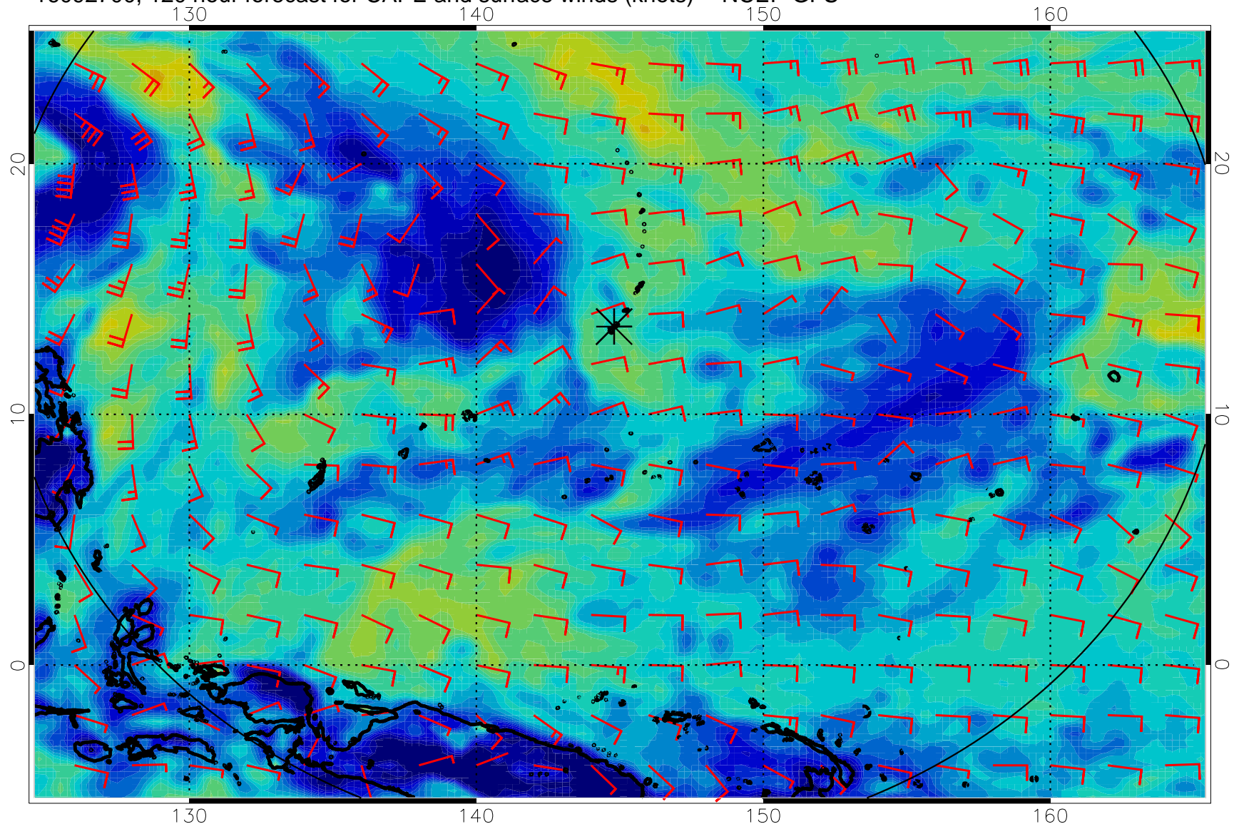
16092700, 120 hour forecast for CAPE and surface winds (knots) -- NCEP GFS
