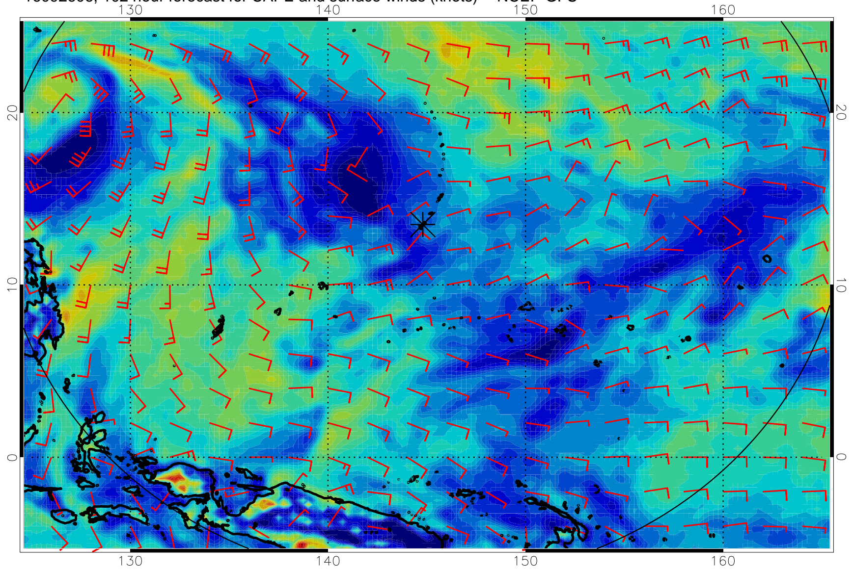
16092606, 102 hour forecast for CAPE and surface winds (knots) -- NCEP GFS
