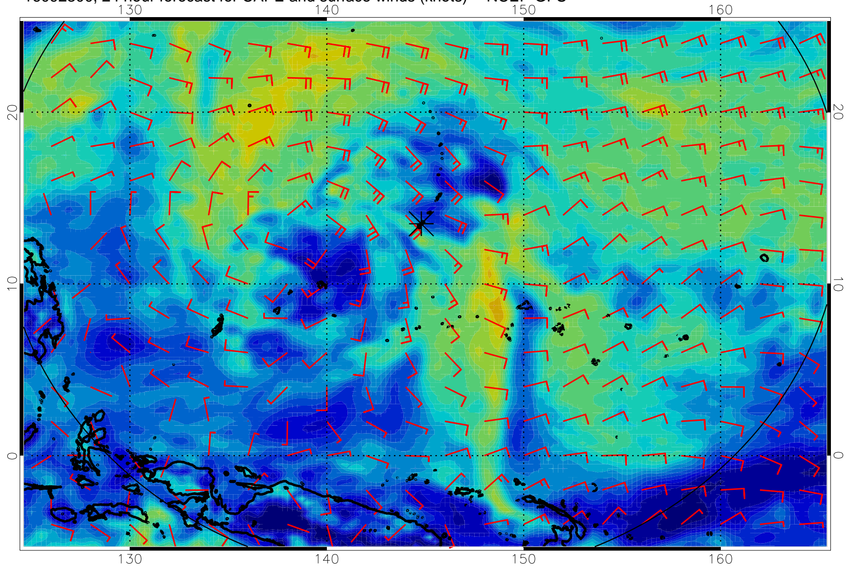
16092300, 24 hour forecast for CAPE and surface winds (knots) -- NCEP GFS
