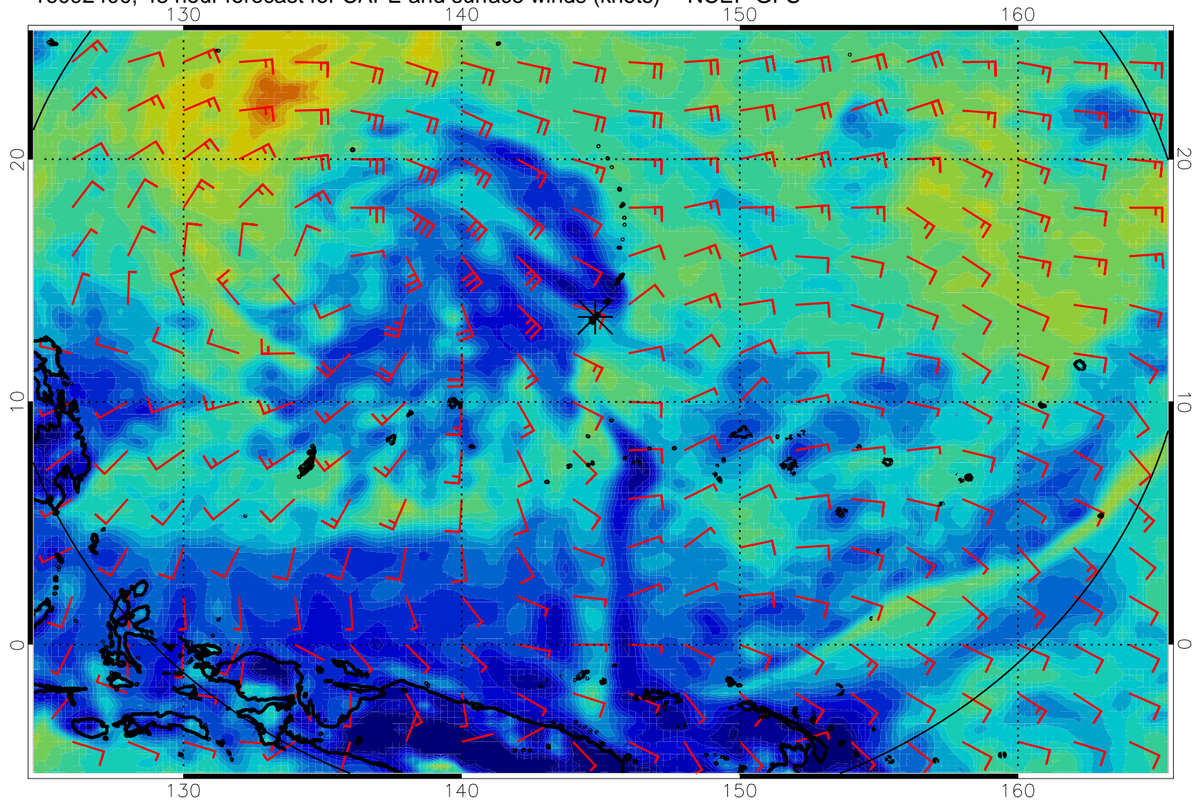
16092400, 48 hour forecast for CAPE and surface winds (knots) -- NCEP GFS
