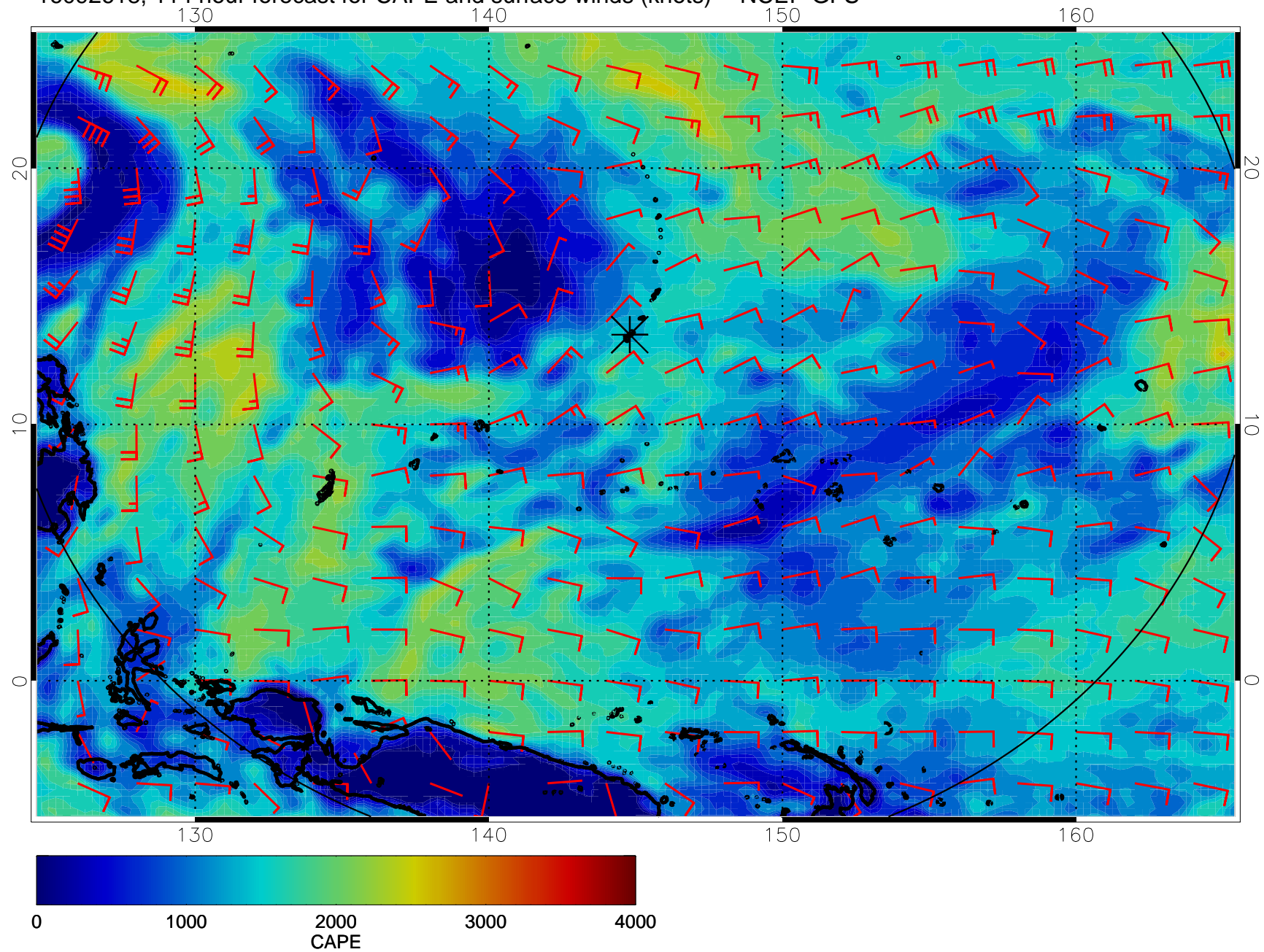
16092618, 114 hour forecast for CAPE and surface winds (knots) -- NCEP GFS
