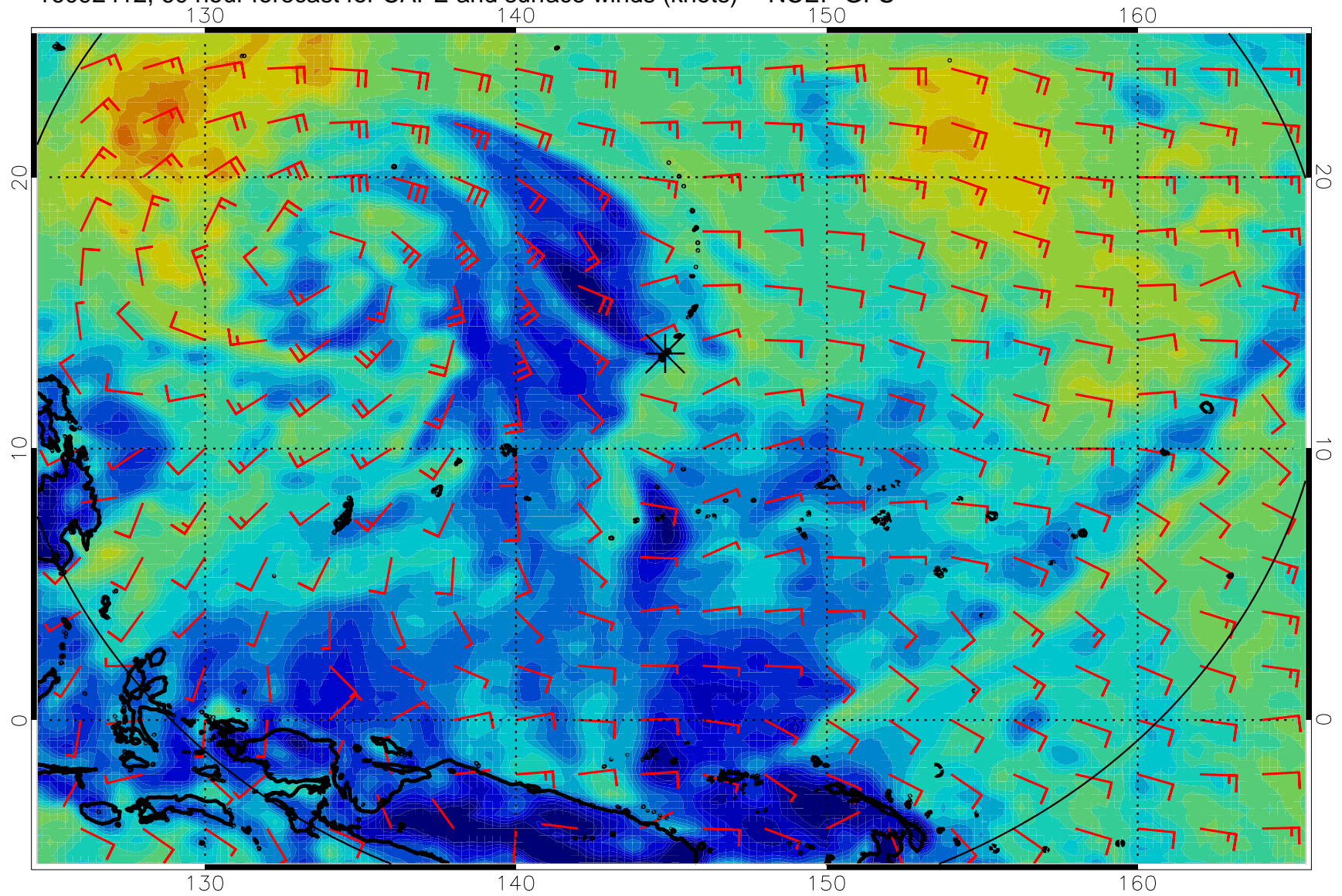
16092412, 60 hour forecast for CAPE and surface winds (knots) -- NCEP GFS
