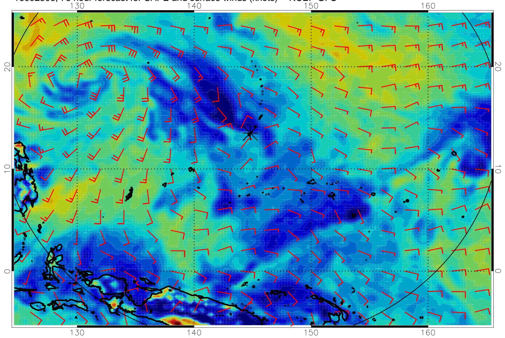
16092506, 78 hour forecast for CAPE and surface winds (knots) -- NCEP GFS
