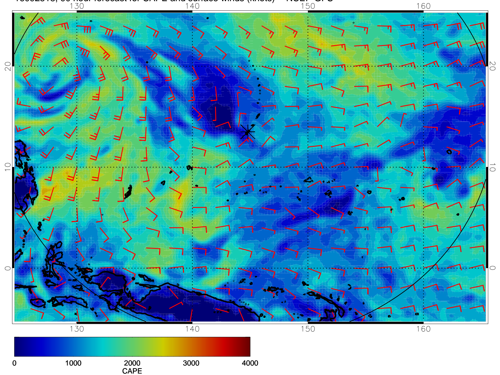
16092518, 90 hour forecast for CAPE and surface winds (knots) -- NCEP GFS
