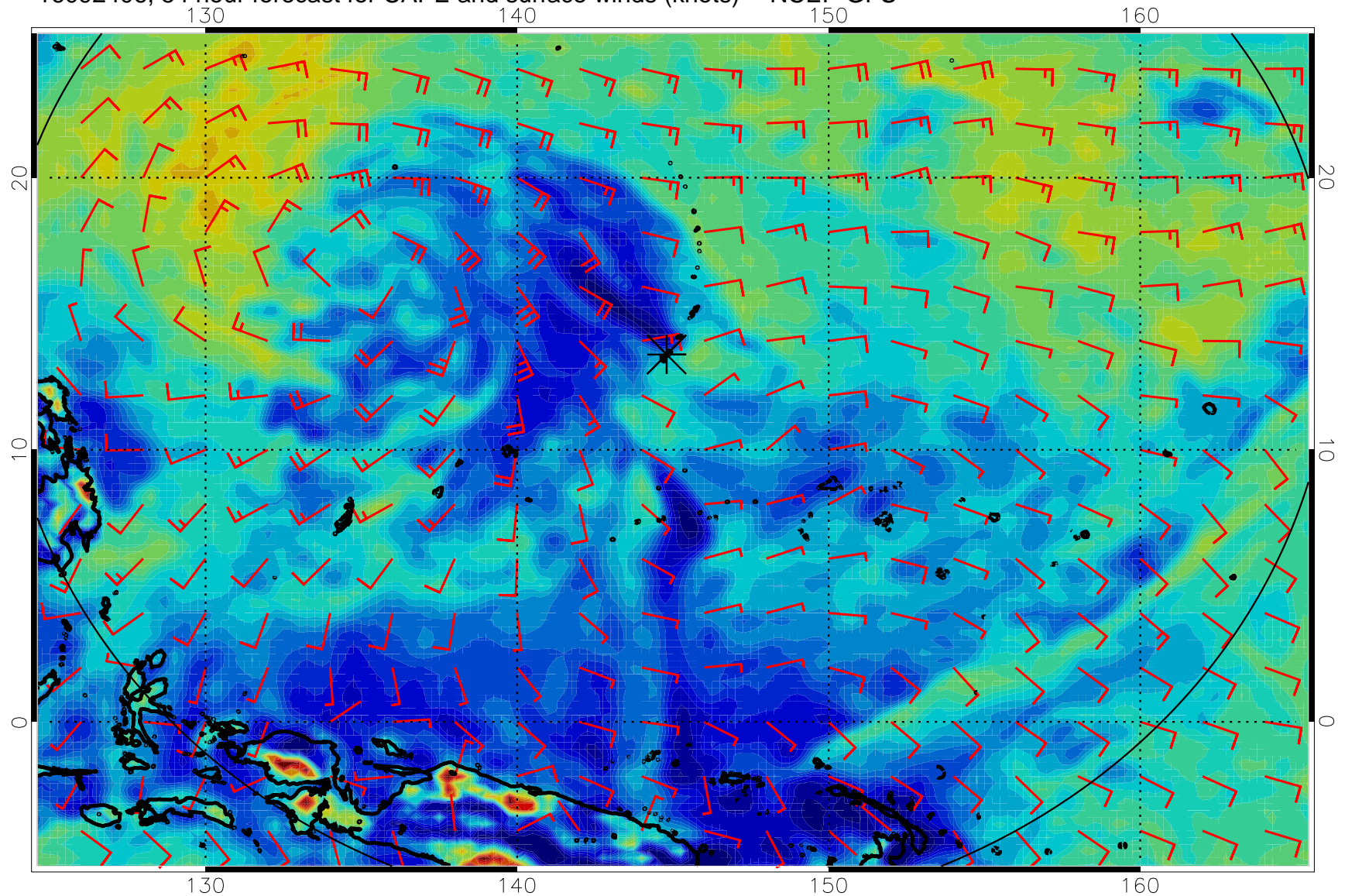
16092406, 54 hour forecast for CAPE and surface winds (knots) -- NCEP GFS
