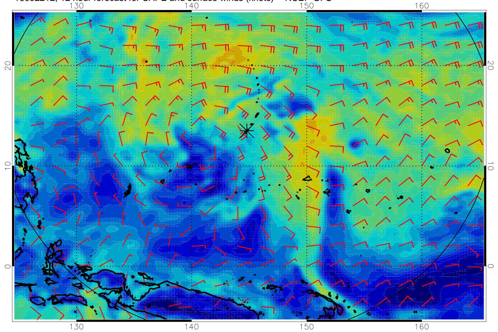
16092212, 12 hour forecast for CAPE and surface winds (knots) -- NCEP GFS
