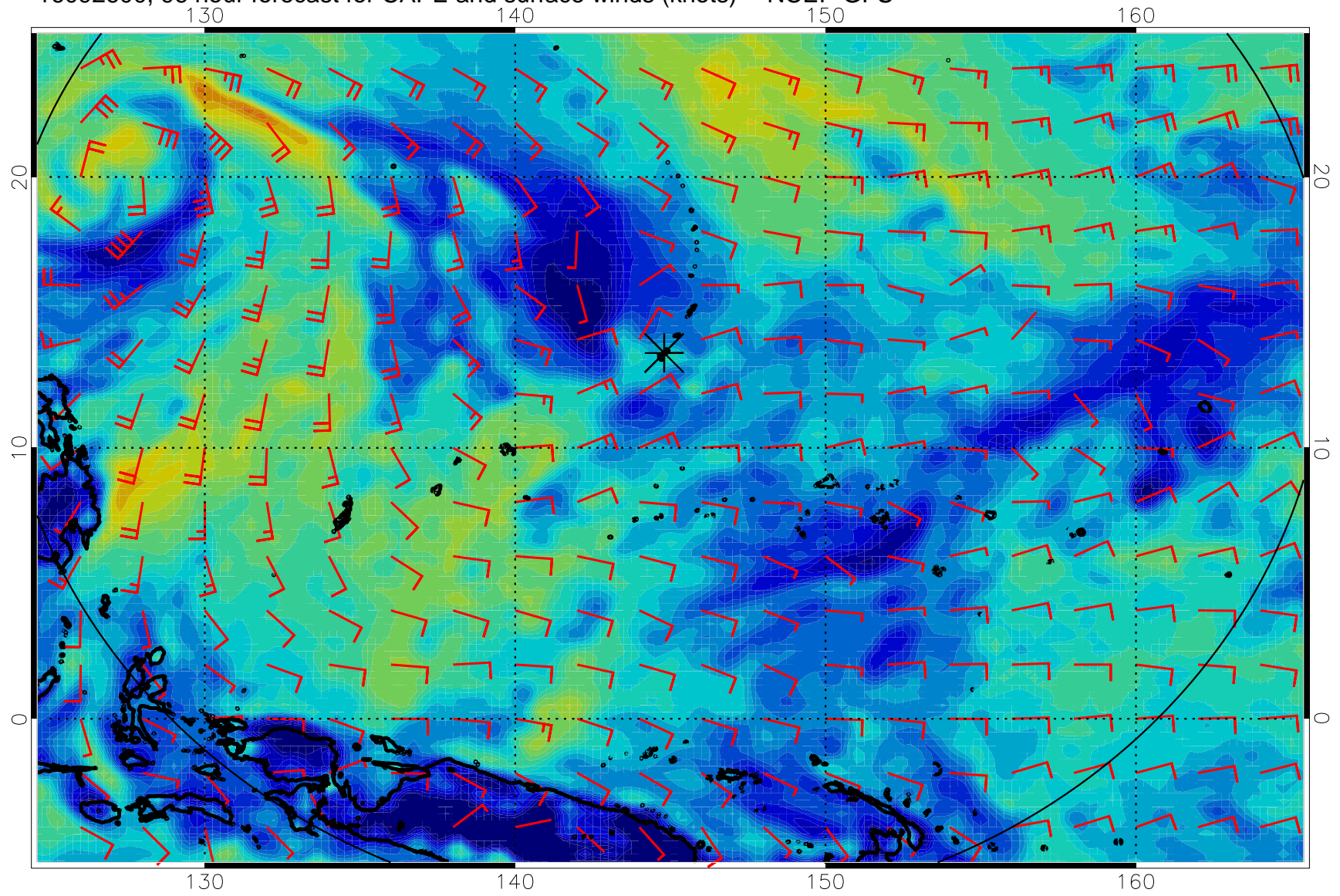
16092600, 96 hour forecast for CAPE and surface winds (knots) -- NCEP GFS
