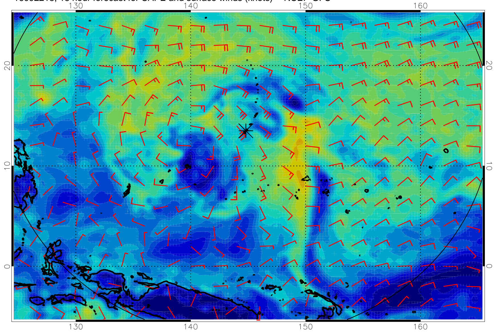
16092218, 18 hour forecast for CAPE and surface winds (knots) -- NCEP GFS
