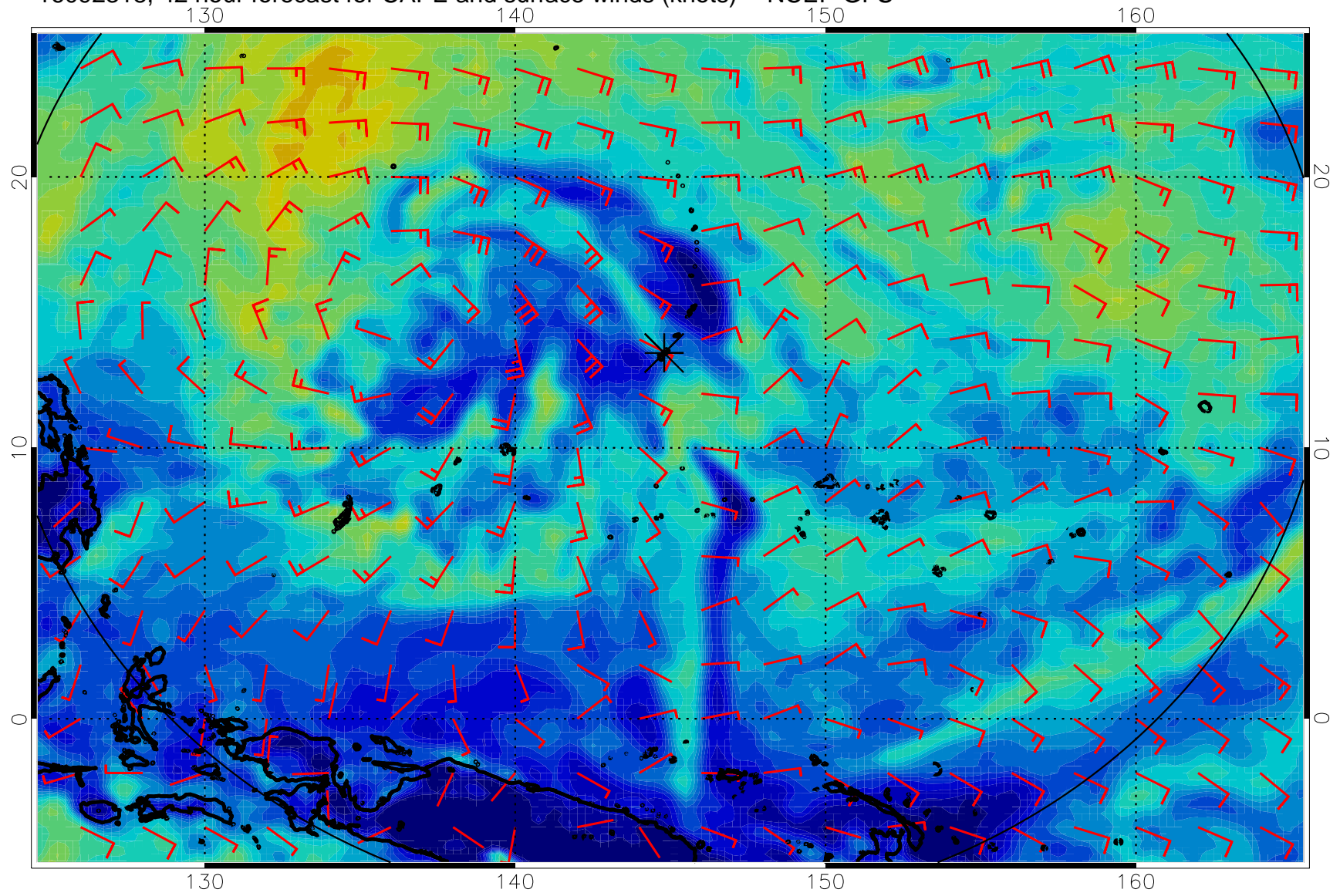
16092318, 42 hour forecast for CAPE and surface winds (knots) -- NCEP GFS
