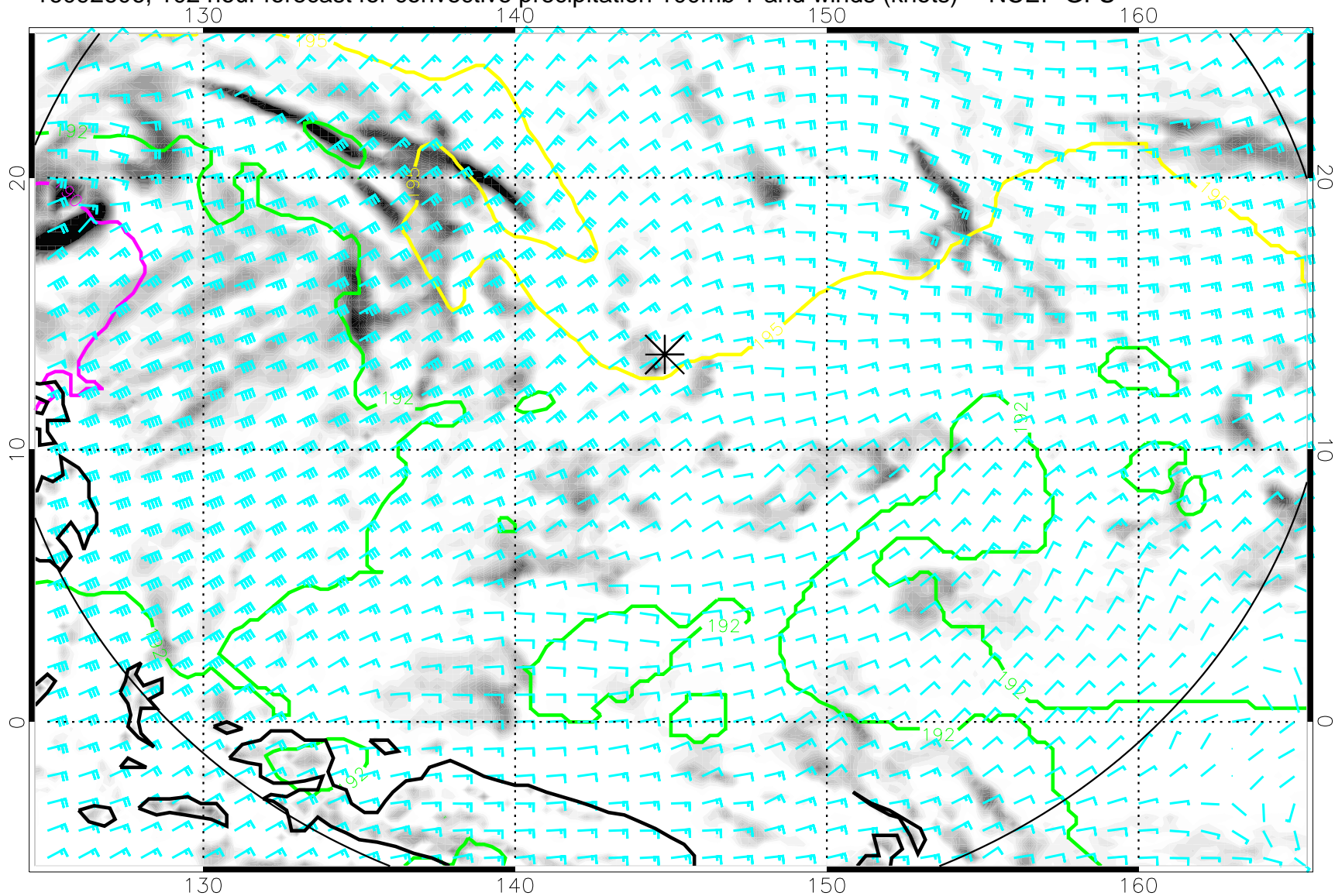
16092606, 102 hour forecast for convective precipitation 100mb T and winds (knots) -- NCEP GFS
