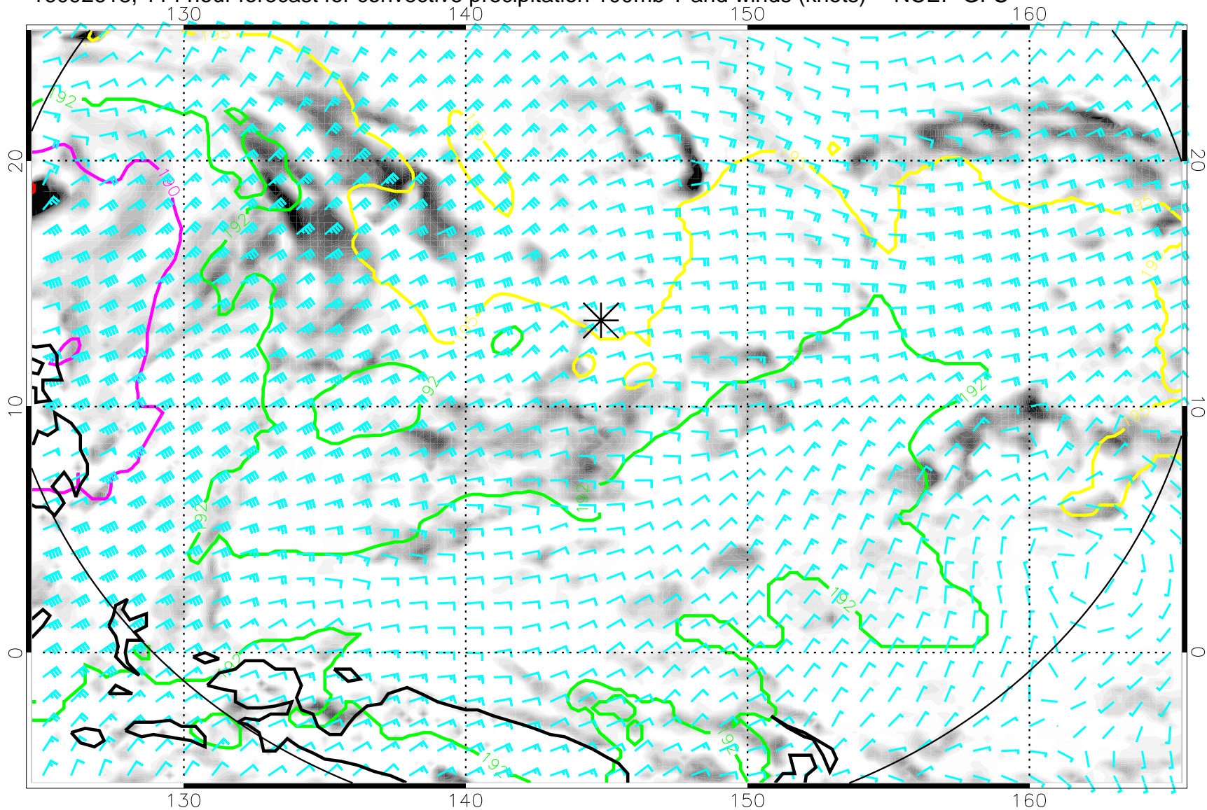
16092618, 114 hour forecast for convective precipitation 100mb T and winds (knots) -- NCEP GFS
