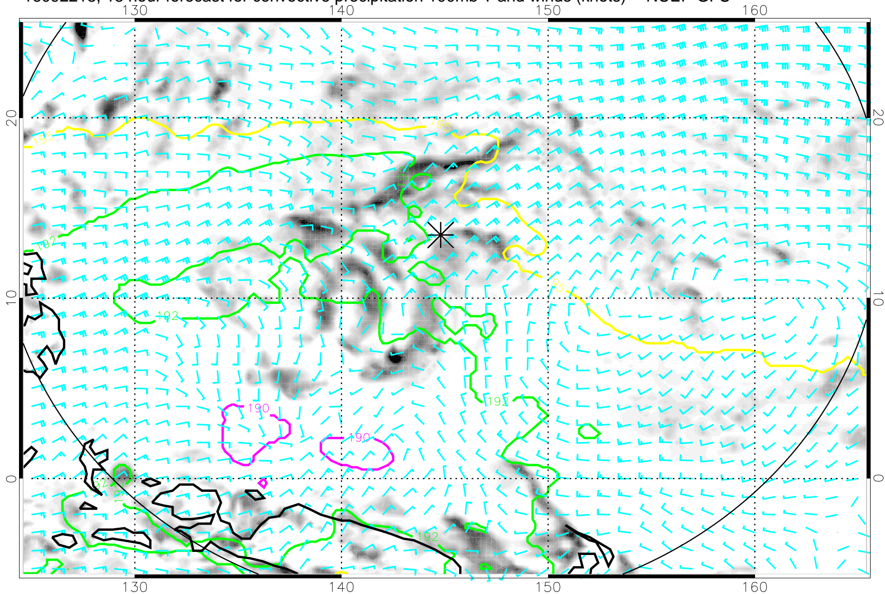
16092218, 18 hour forecast for convective precipitation 100mb T and winds (knots) -- NCEP GFS
