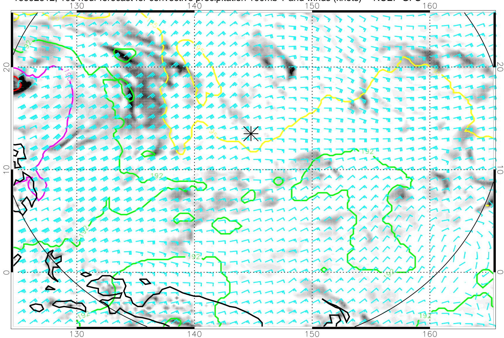
16092612, 108 hour forecast for convective precipitation 100mb T and winds (knots) -- NCEP GFS
