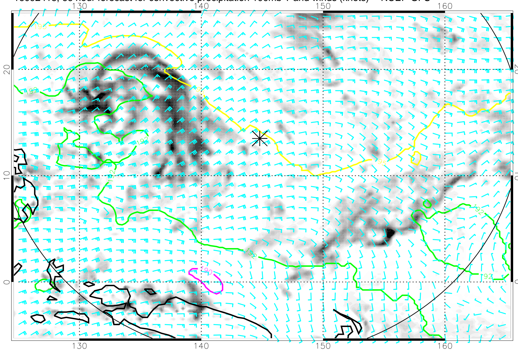
16092418, 66 hour forecast for convective precipitation 100mb T and winds (knots) -- NCEP GFS
