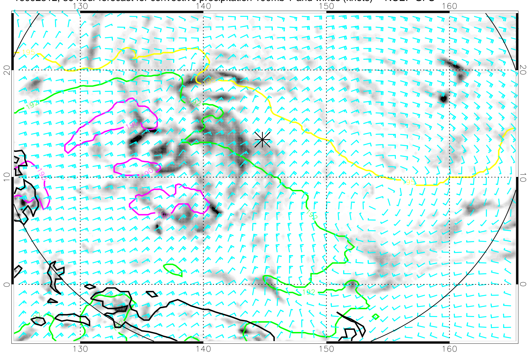
16092312, 36 hour forecast for convective precipitation 100mb T and winds (knots) -- NCEP GFS
