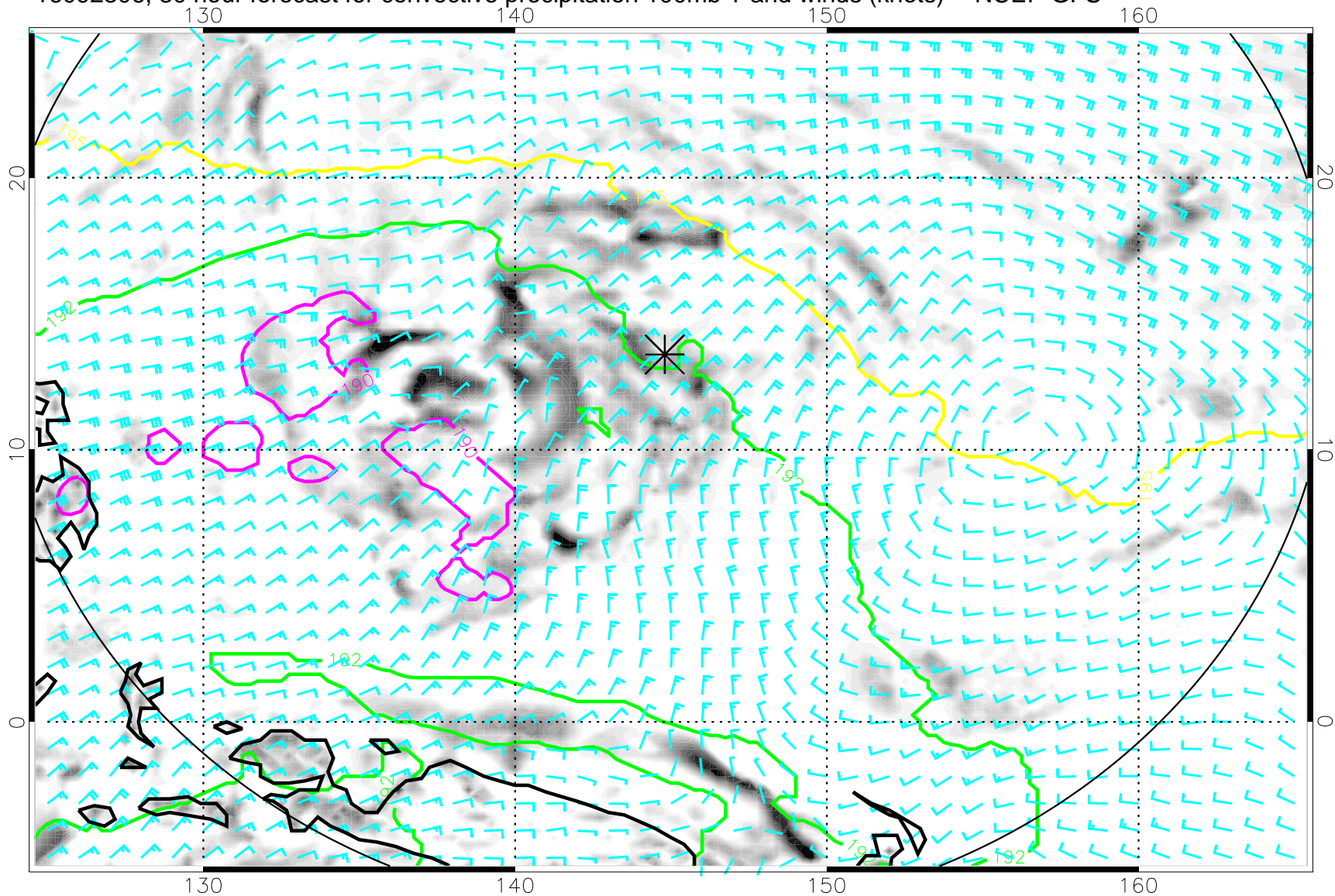
16092306, 30 hour forecast for convective precipitation 100mb T and winds (knots) -- NCEP GFS
