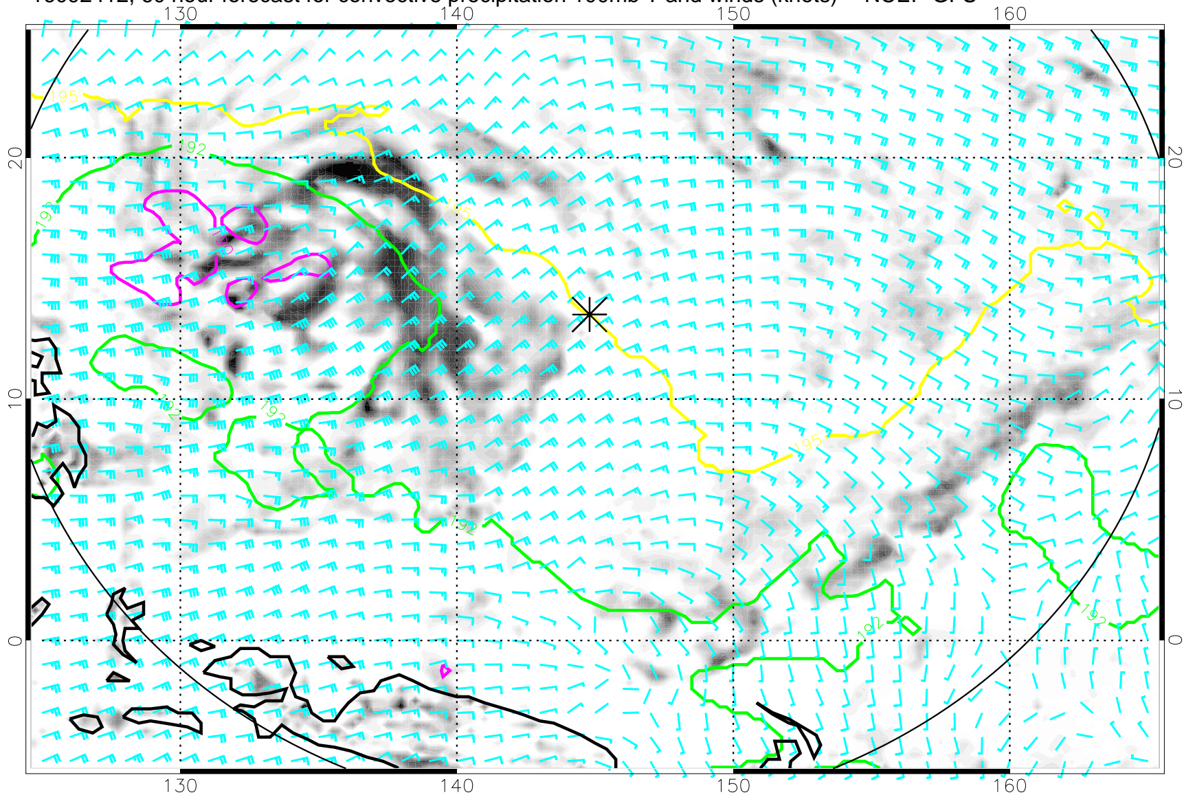
16092412, 60 hour forecast for convective precipitation 100mb T and winds (knots) -- NCEP GFS
