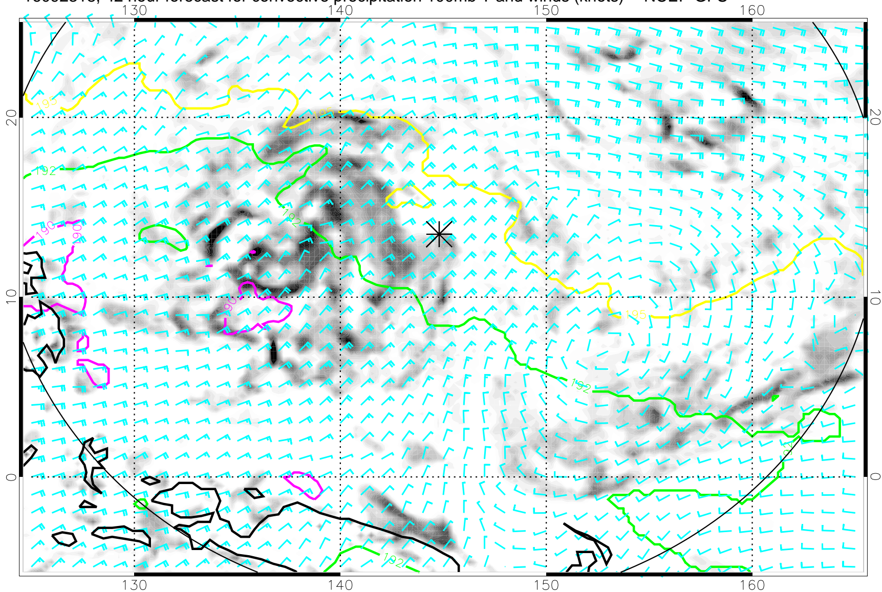
16092318, 42 hour forecast for convective precipitation 100mb T and winds (knots) -- NCEP GFS
