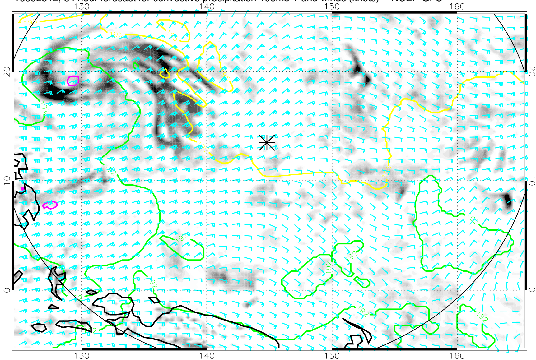
16092512, 84 hour forecast for convective precipitation 100mb T and winds (knots) -- NCEP GFS
