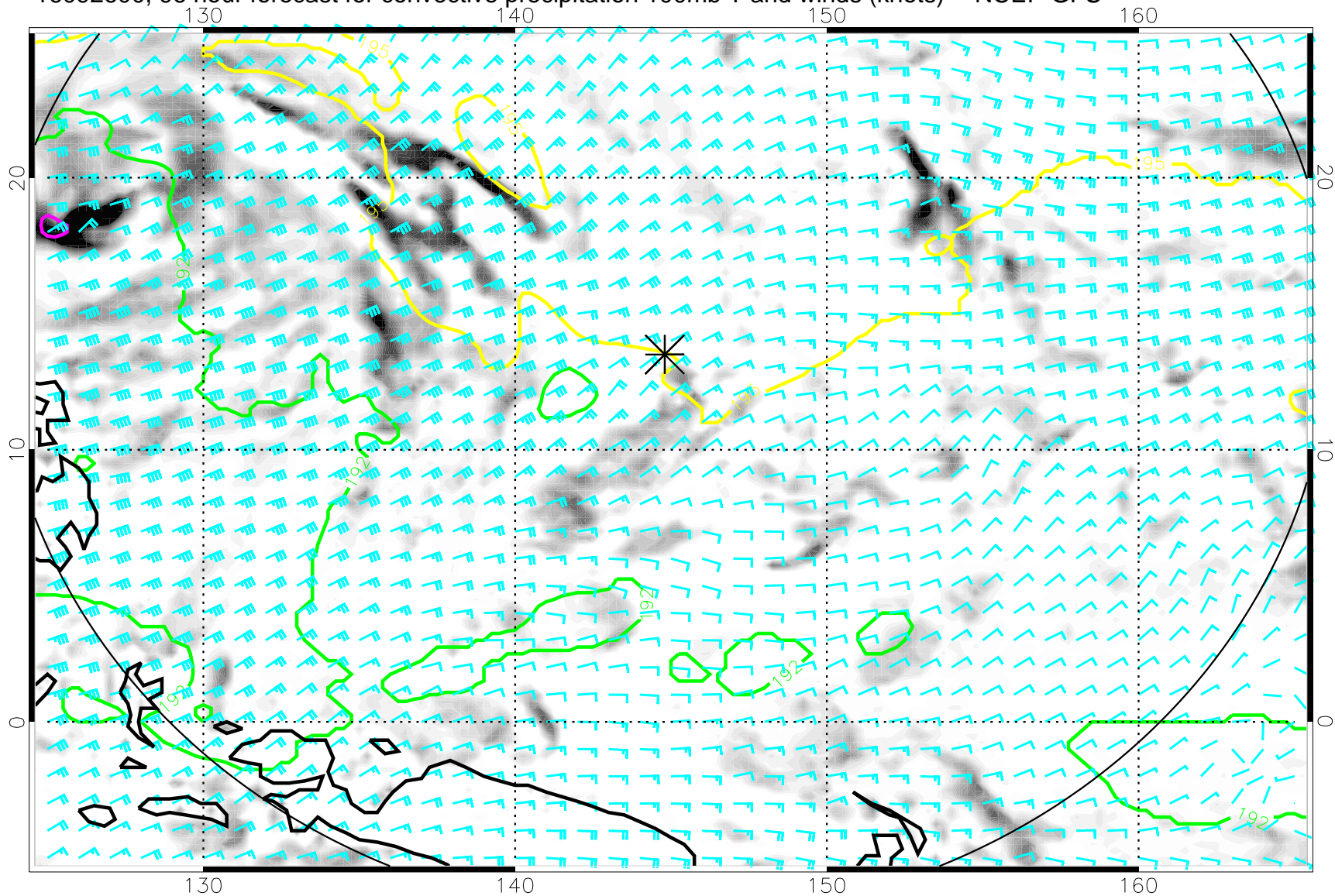
16092600, 96 hour forecast for convective precipitation 100mb T and winds (knots) -- NCEP GFS
