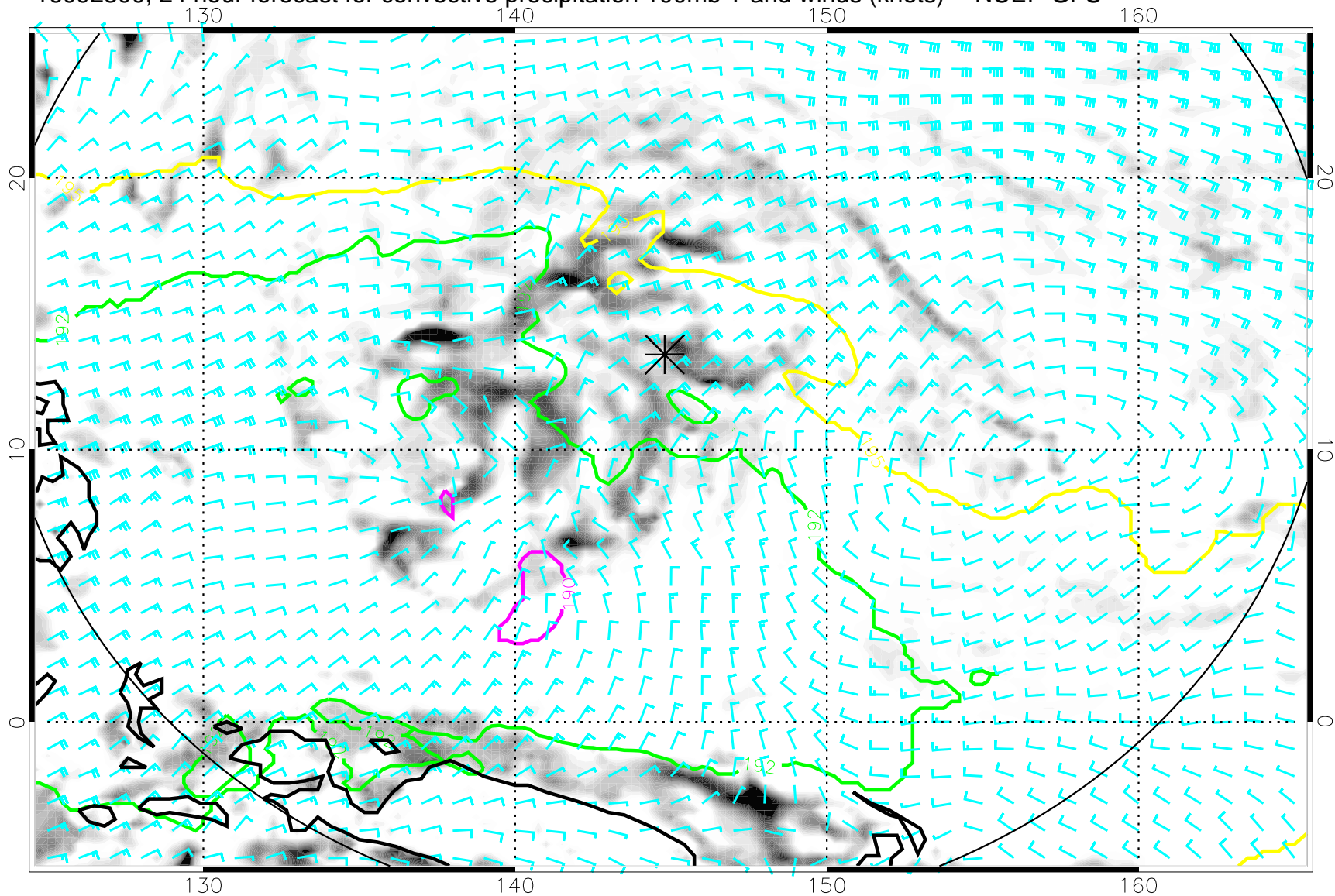
16092300, 24 hour forecast for convective precipitation 100mb T and winds (knots) -- NCEP GFS
