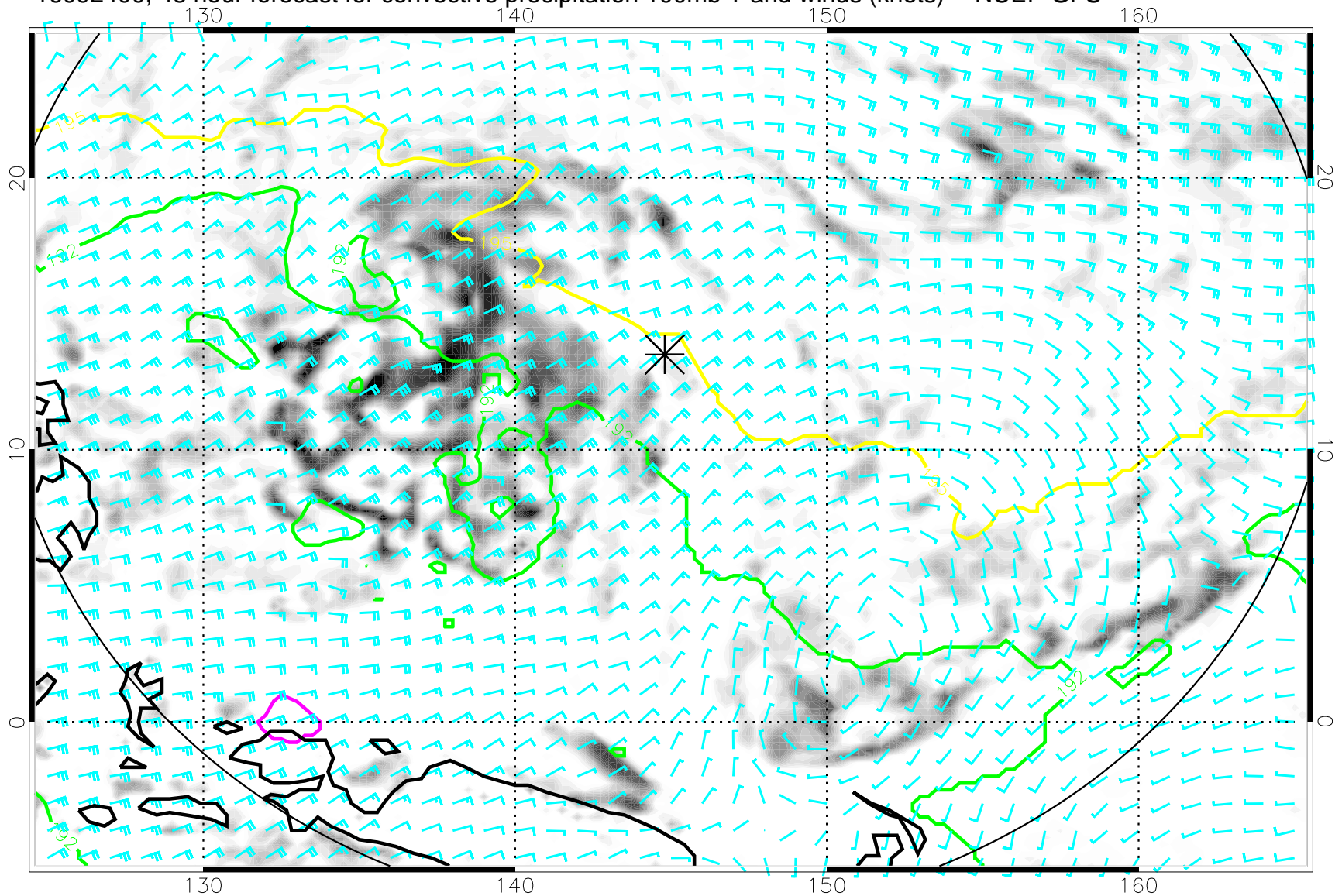
16092400, 48 hour forecast for convective precipitation 100mb T and winds (knots) -- NCEP GFS
