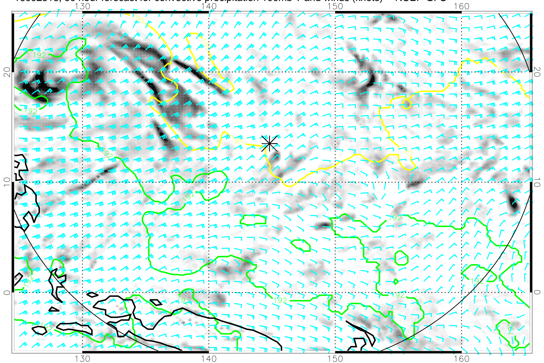
16092518, 90 hour forecast for convective precipitation 100mb T and winds (knots) -- NCEP GFS
