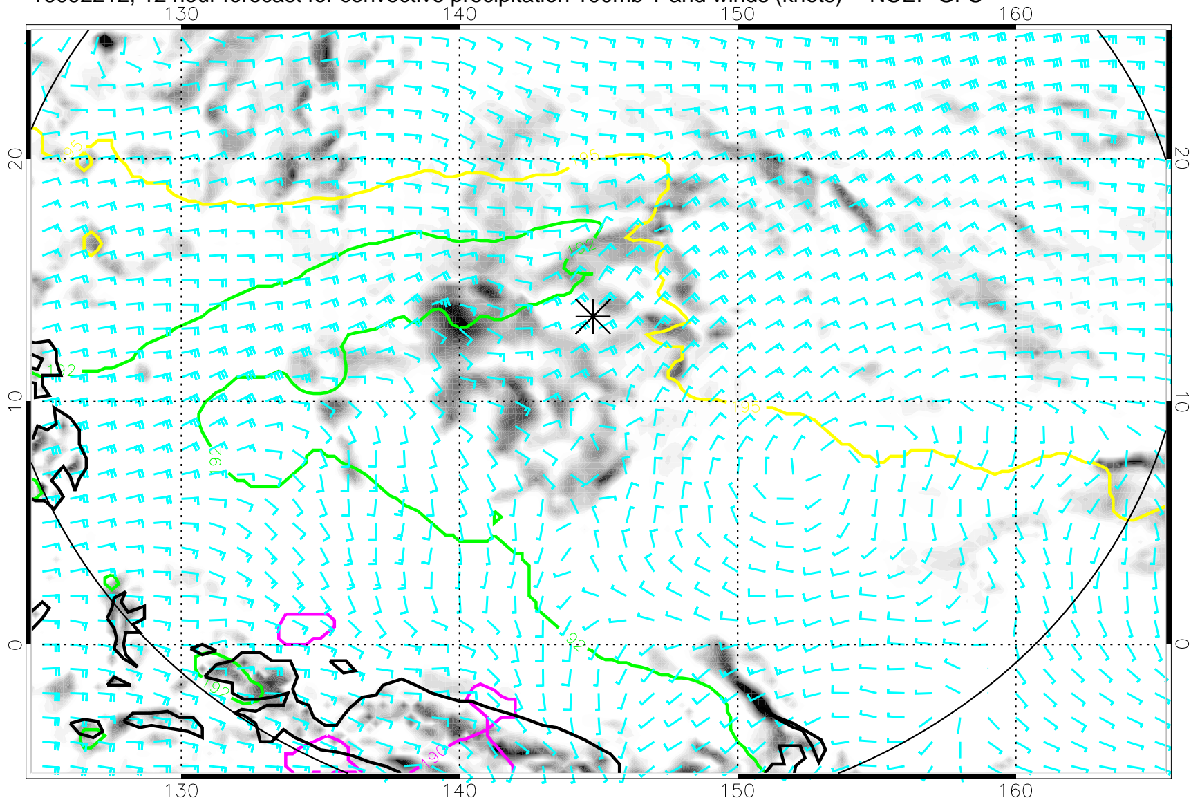
16092212, 12 hour forecast for convective precipitation 100mb T and winds (knots) -- NCEP GFS
