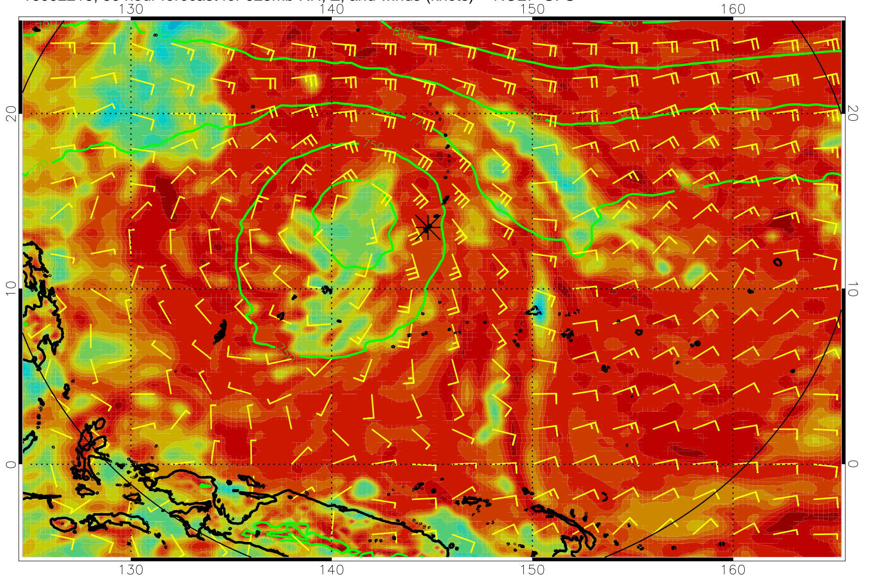
16092218, 30 hour forecast for 925mb RH, Z, and winds (knots) -- NCEP GFS
