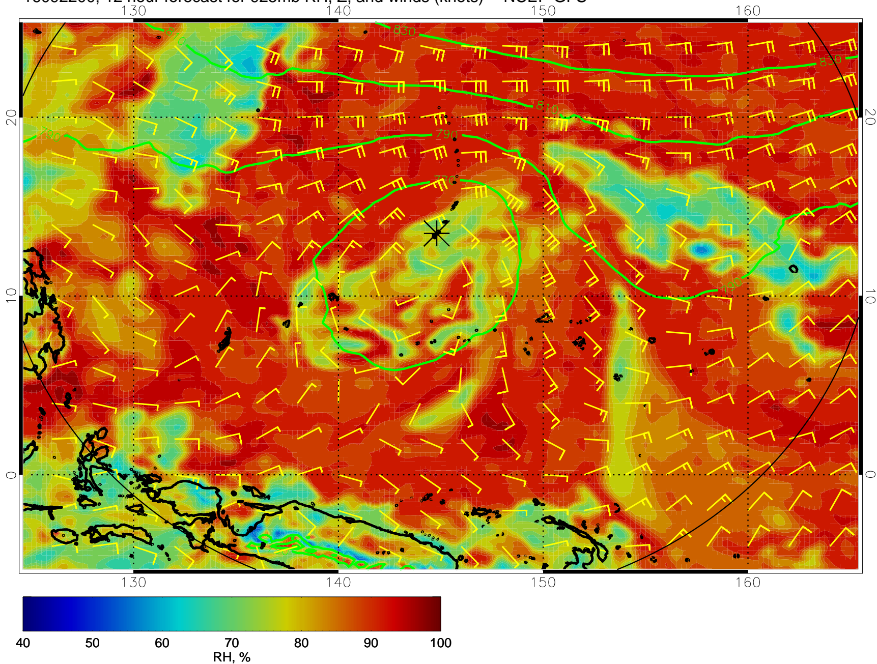
16092200, 12 hour forecast for 925mb RH, Z, and winds (knots) -- NCEP GFS
