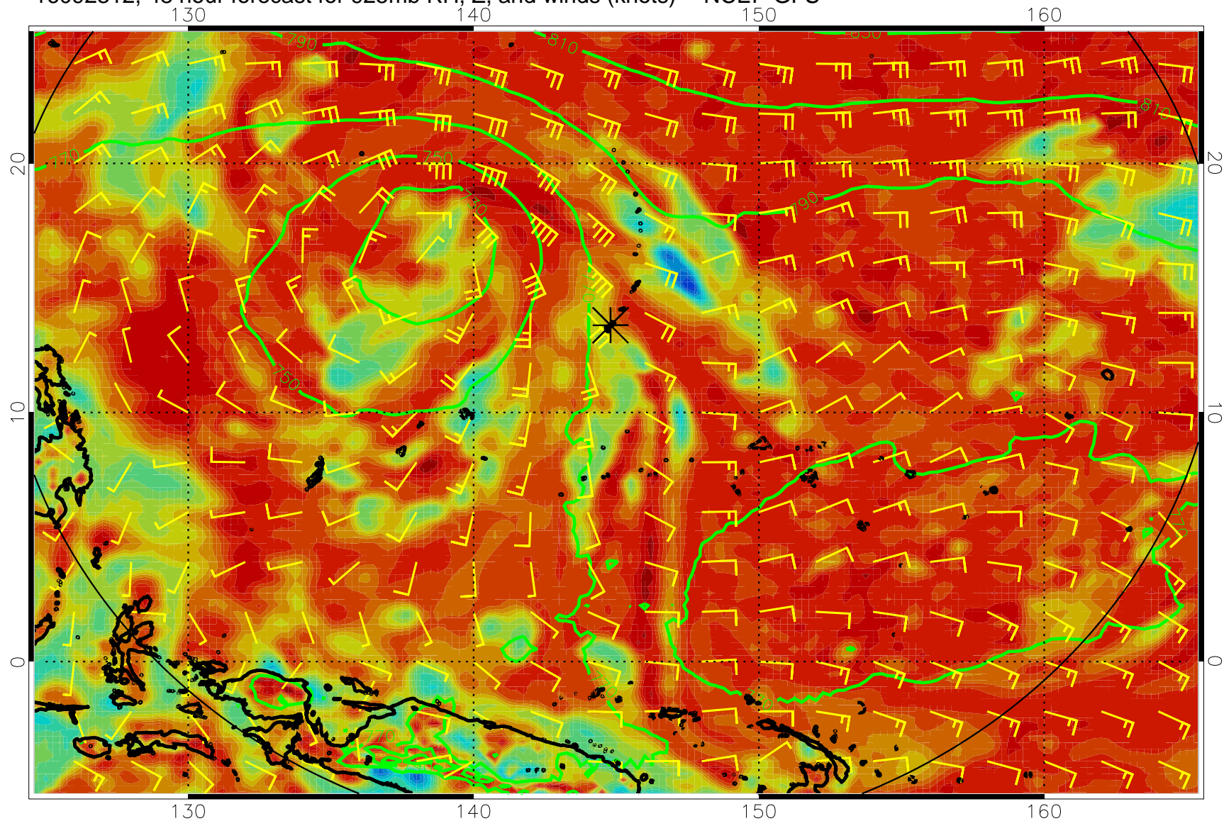
16092312, 48 hour forecast for 925mb RH, Z, and winds (knots) -- NCEP GFS
