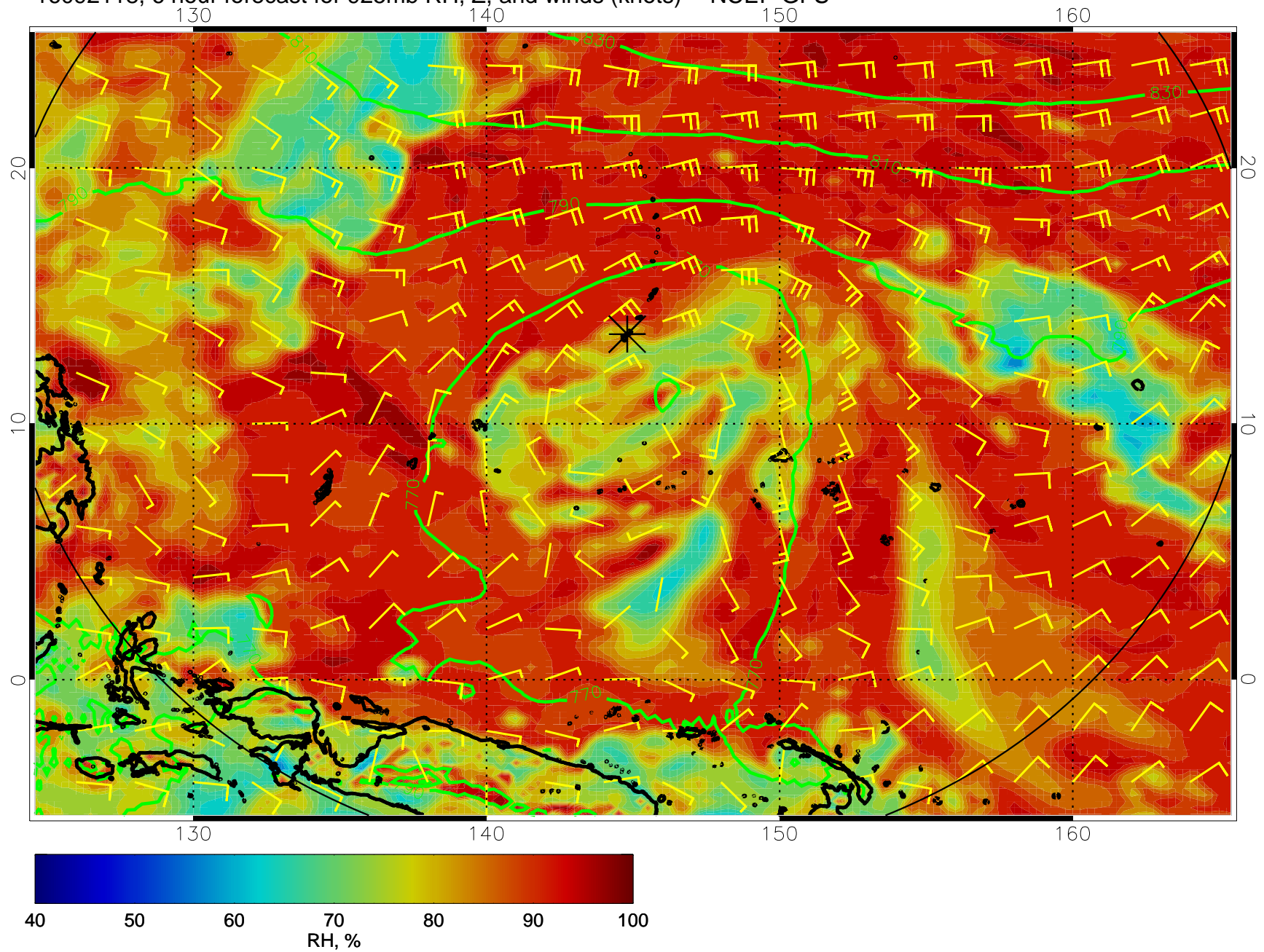
16092118, 6 hour forecast for 925mb RH, Z, and winds (knots) -- NCEP GFS
