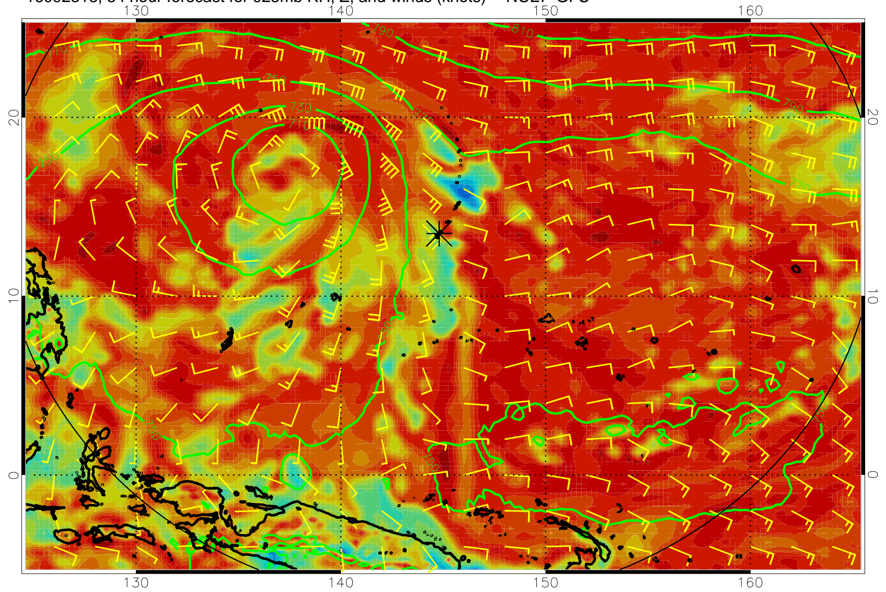
16092318, 54 hour forecast for 925mb RH, Z, and winds (knots) -- NCEP GFS
