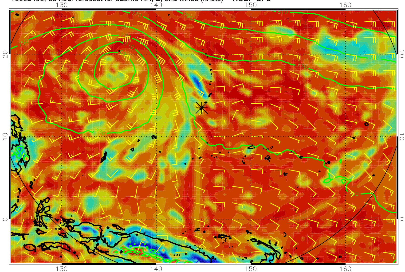
16092406, 66 hour forecast for 925mb RH, Z, and winds (knots) -- NCEP GFS
