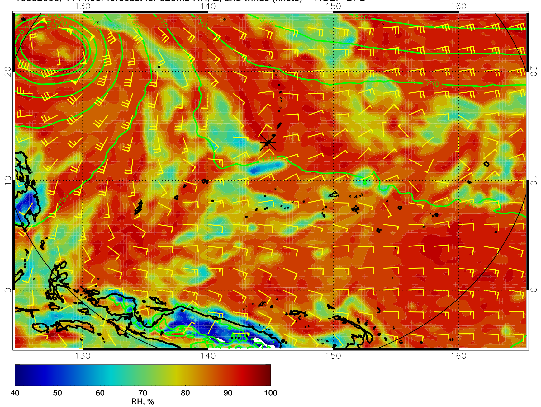
16092606, 114 hour forecast for 925mb RH, Z, and winds (knots) -- NCEP GFS
