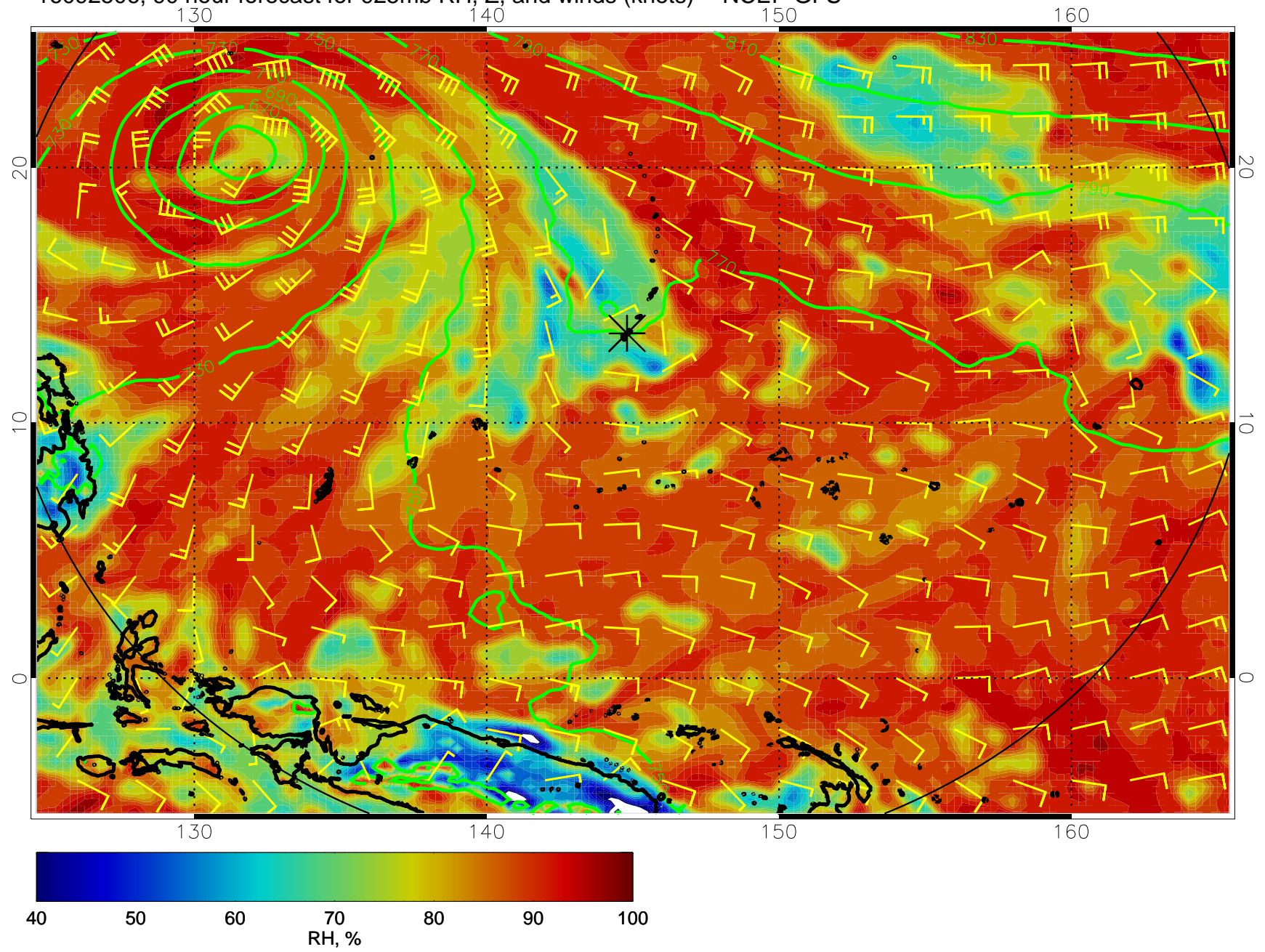
16092506, 90 hour forecast for 925mb RH, Z, and winds (knots) -- NCEP GFS
