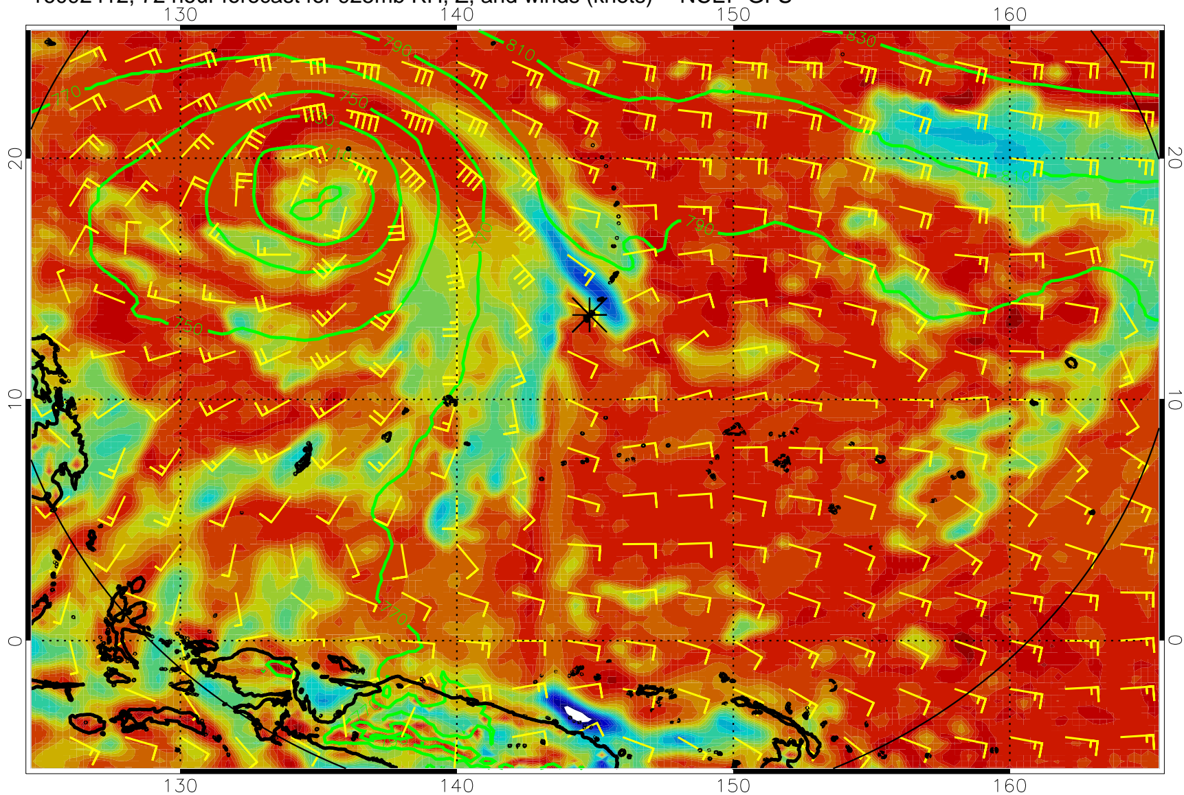
16092412, 72 hour forecast for 925mb RH, Z, and winds (knots) -- NCEP GFS
