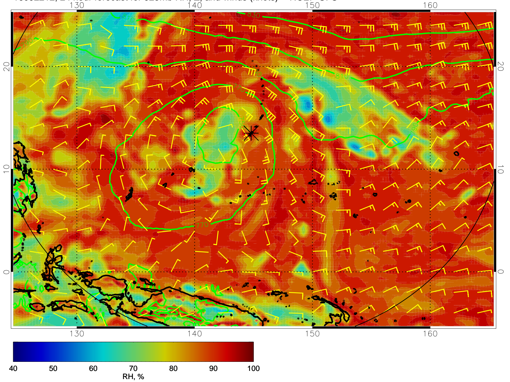
16092212, 24 hour forecast for 925mb RH, Z, and winds (knots) -- NCEP GFS
