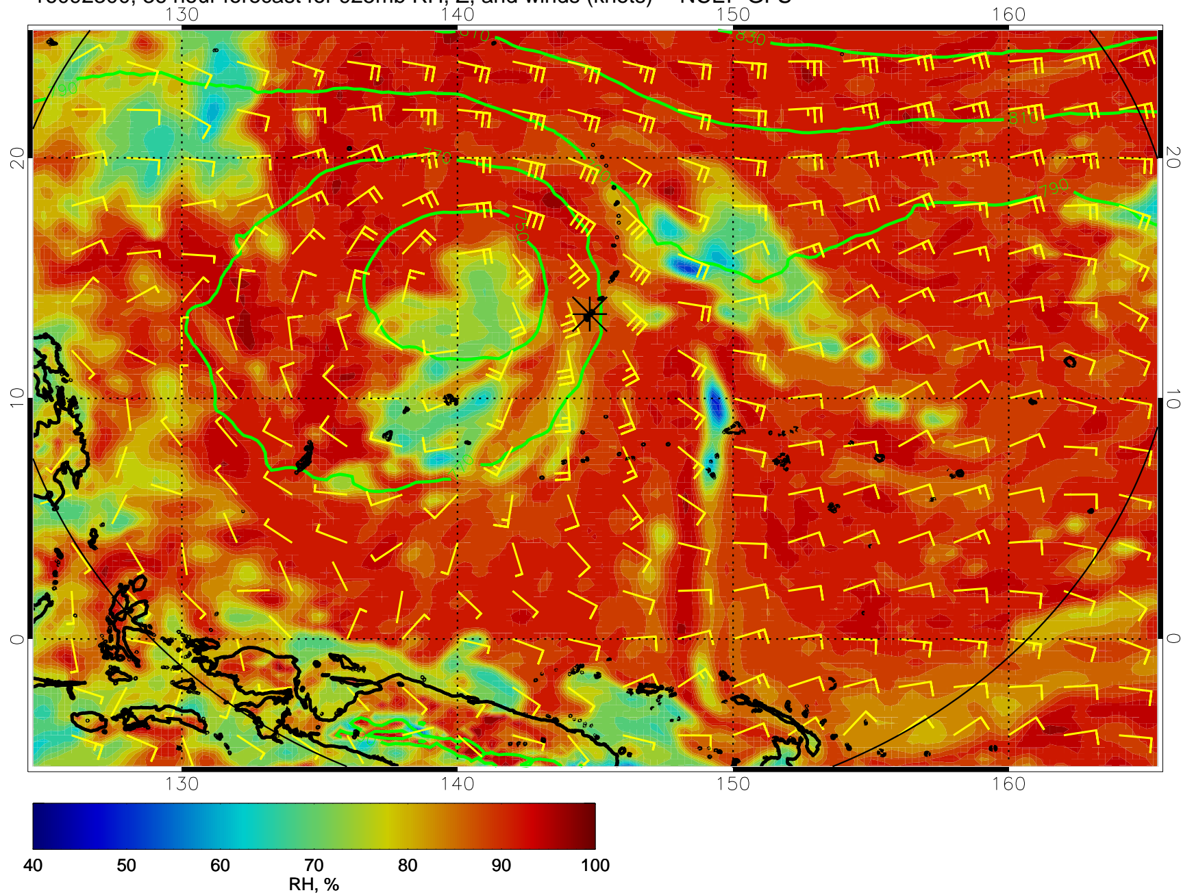
16092300, 36 hour forecast for 925mb RH, Z, and winds (knots) -- NCEP GFS
