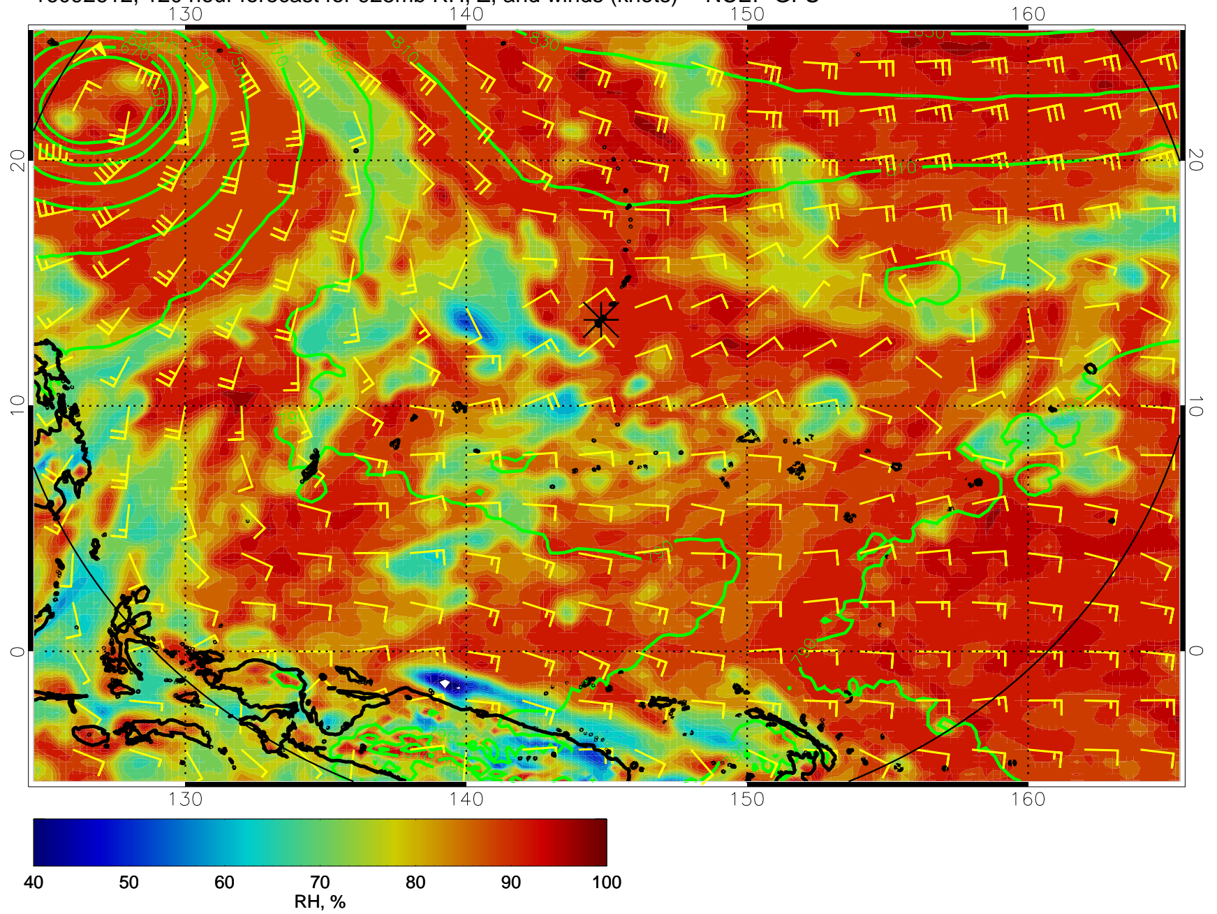
16092612, 120 hour forecast for 925mb RH, Z, and winds (knots) -- NCEP GFS
