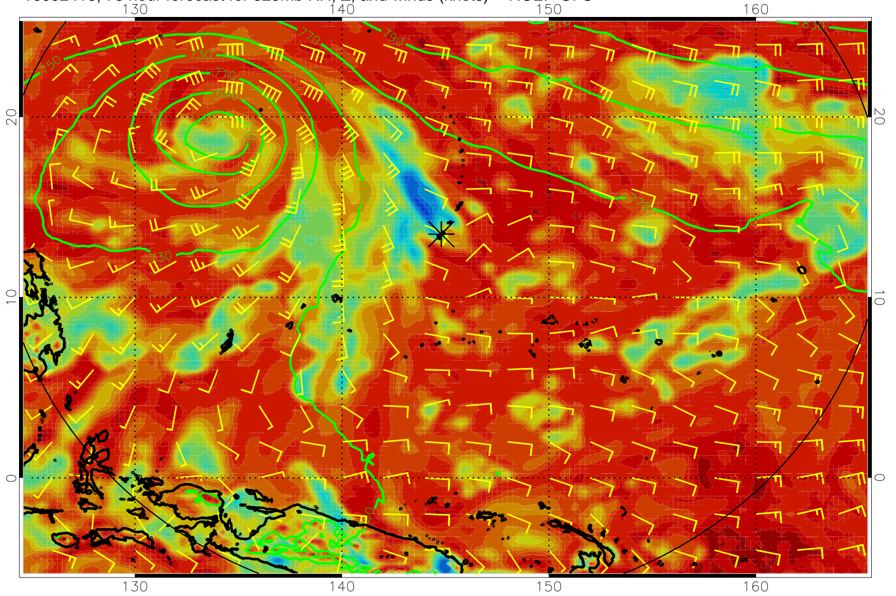
16092418, 78 hour forecast for 925mb RH, Z, and winds (knots) -- NCEP GFS
