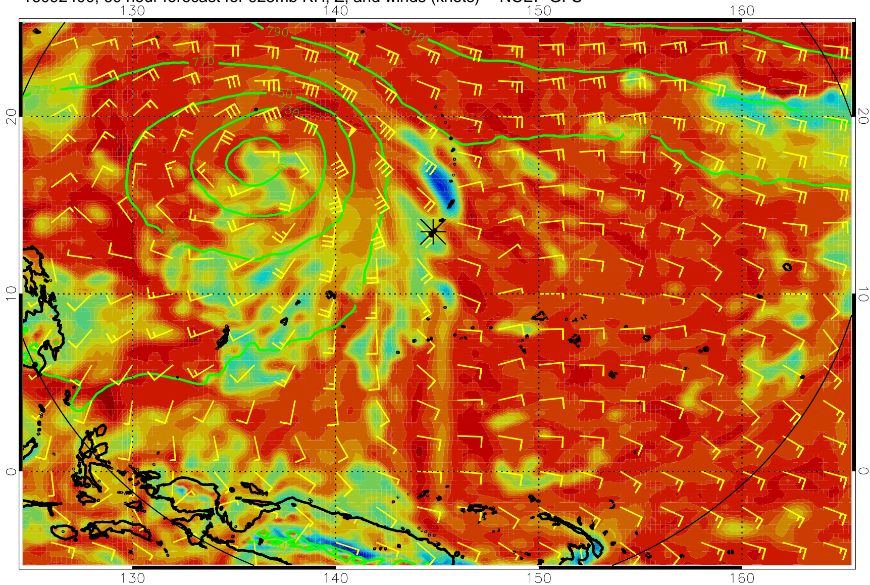
16092400, 60 hour forecast for 925mb RH, Z, and winds (knots) -- NCEP GFS
