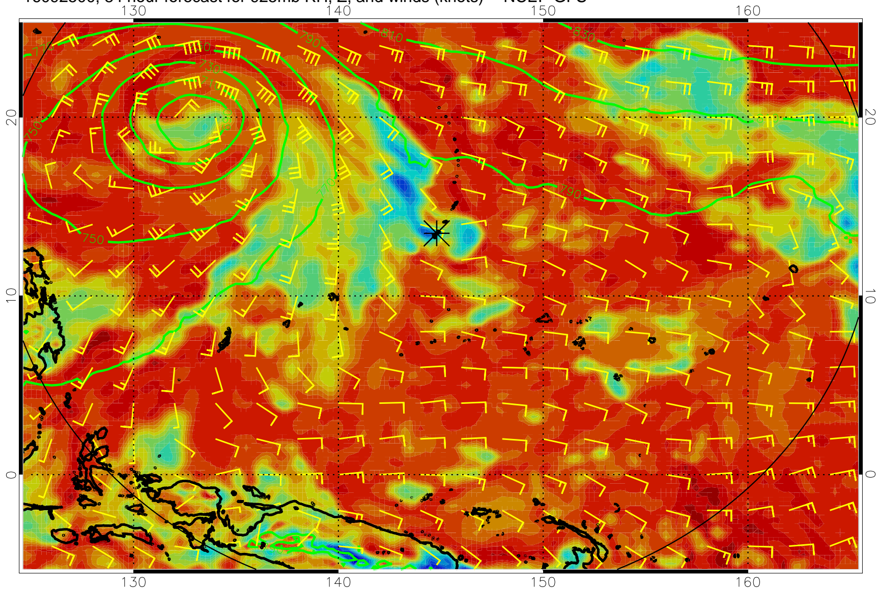
16092500, 84 hour forecast for 925mb RH, Z, and winds (knots) -- NCEP GFS
