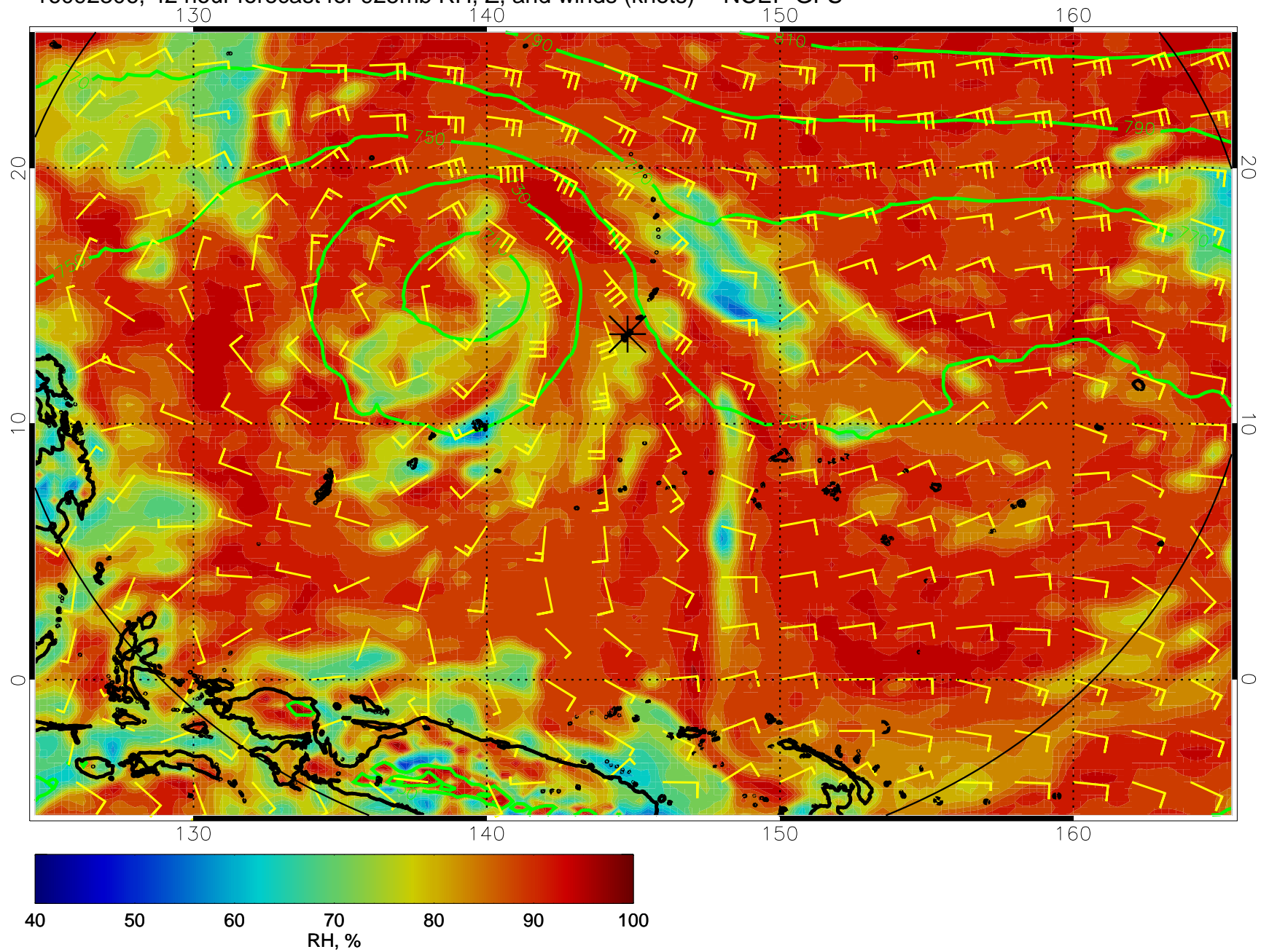
16092306, 42 hour forecast for 925mb RH, Z, and winds (knots) -- NCEP GFS
