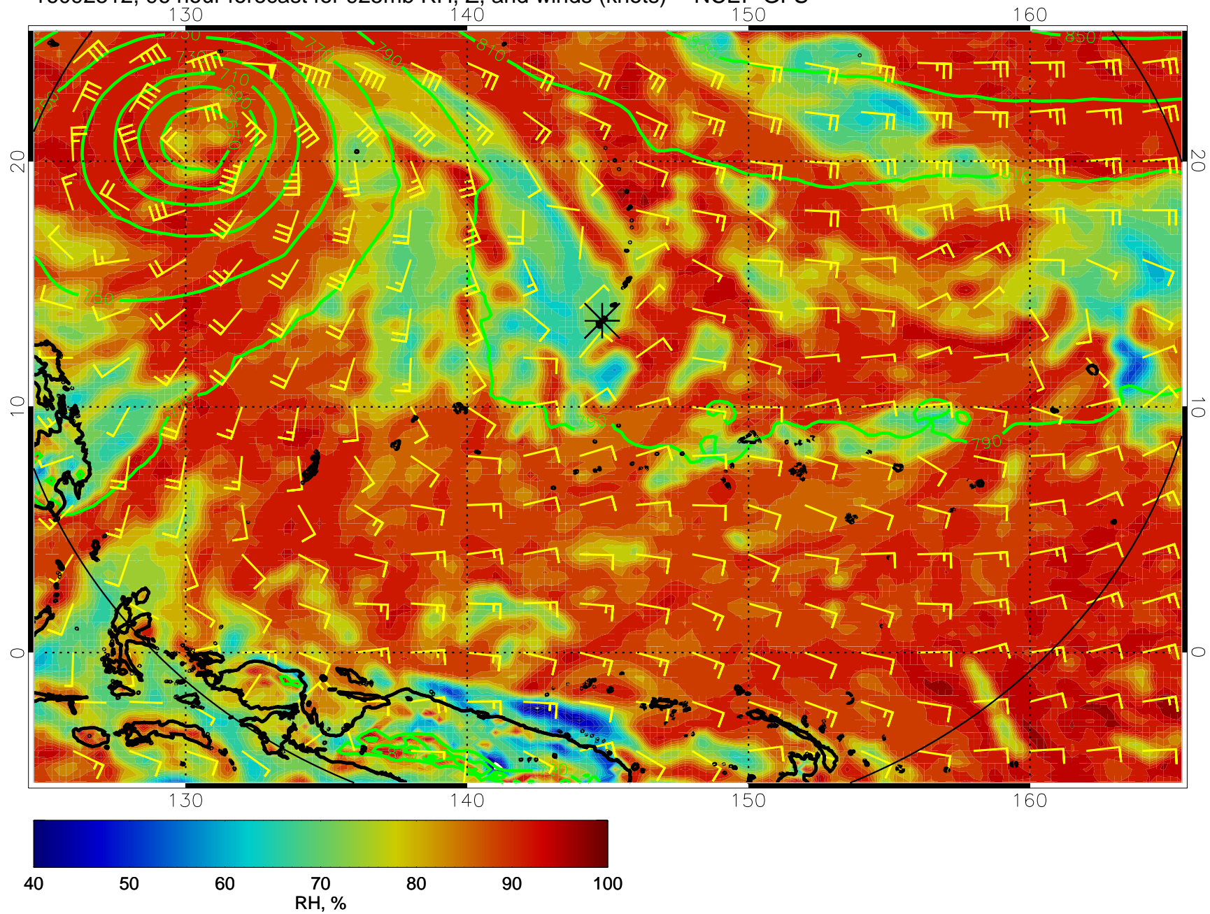
16092512, 96 hour forecast for 925mb RH, Z, and winds (knots) -- NCEP GFS
