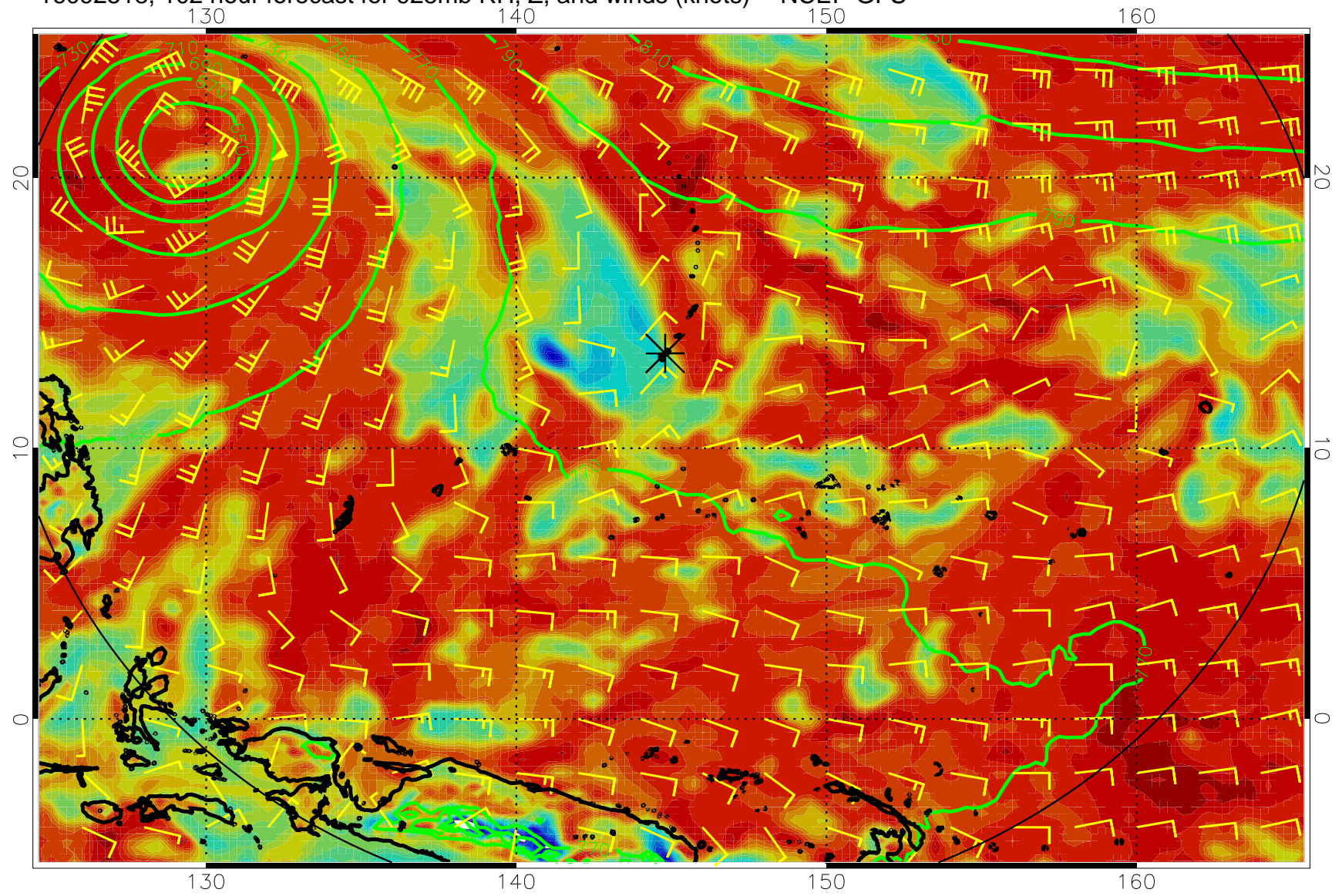
16092518, 102 hour forecast for 925mb RH, Z, and winds (knots) -- NCEP GFS
