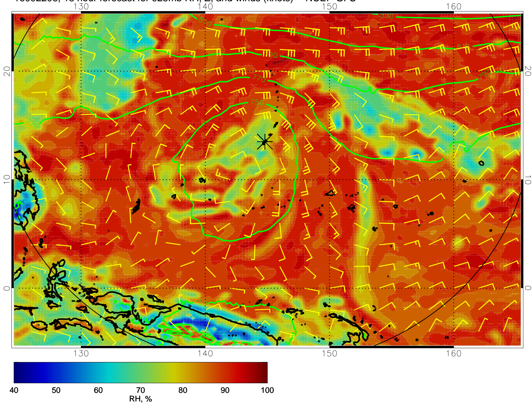
16092206, 18 hour forecast for 925mb RH, Z, and winds (knots) -- NCEP GFS
