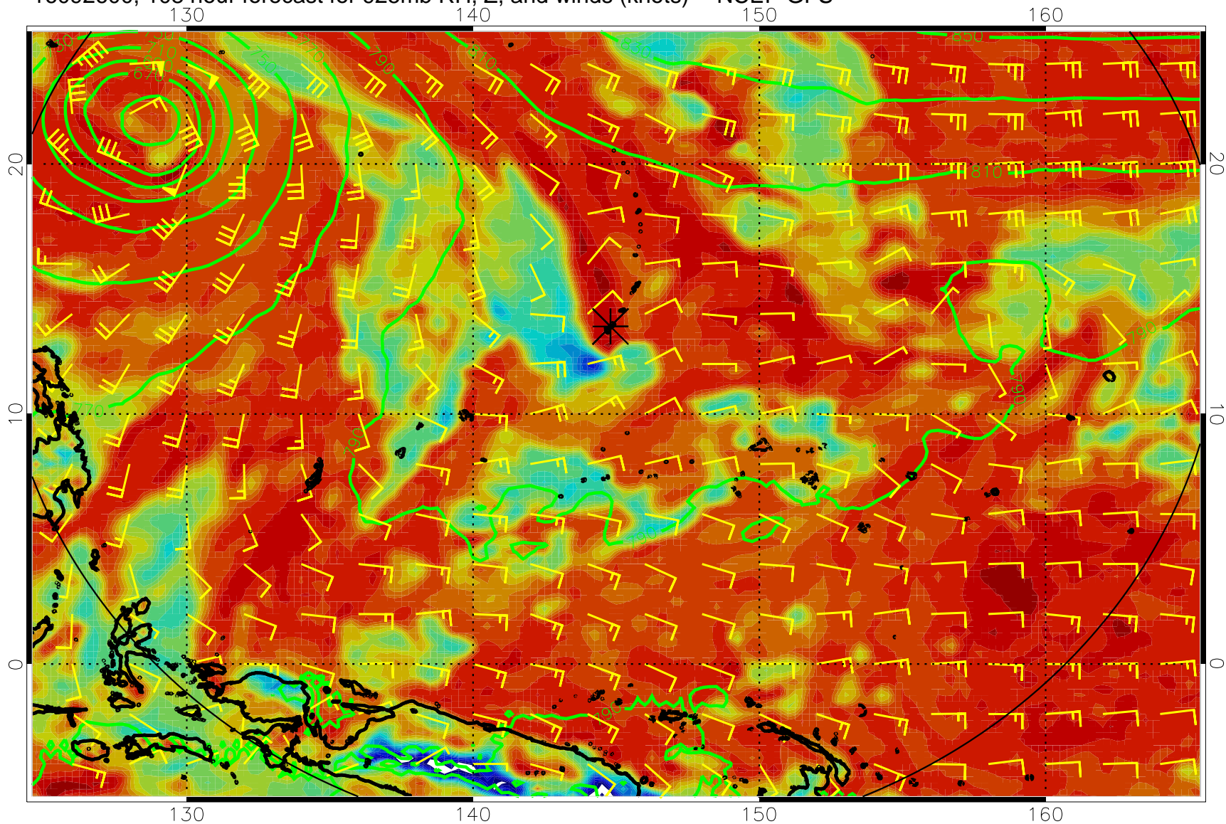
16092600, 108 hour forecast for 925mb RH, Z, and winds (knots) -- NCEP GFS
