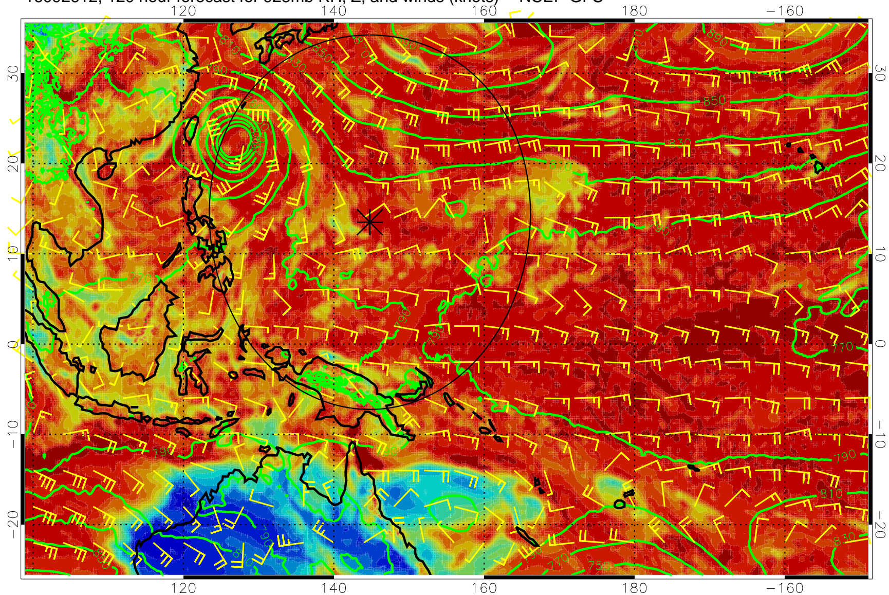
16092612, 120 hour forecast for 925mb RH, Z, and winds (knots) -- NCEP GFS
