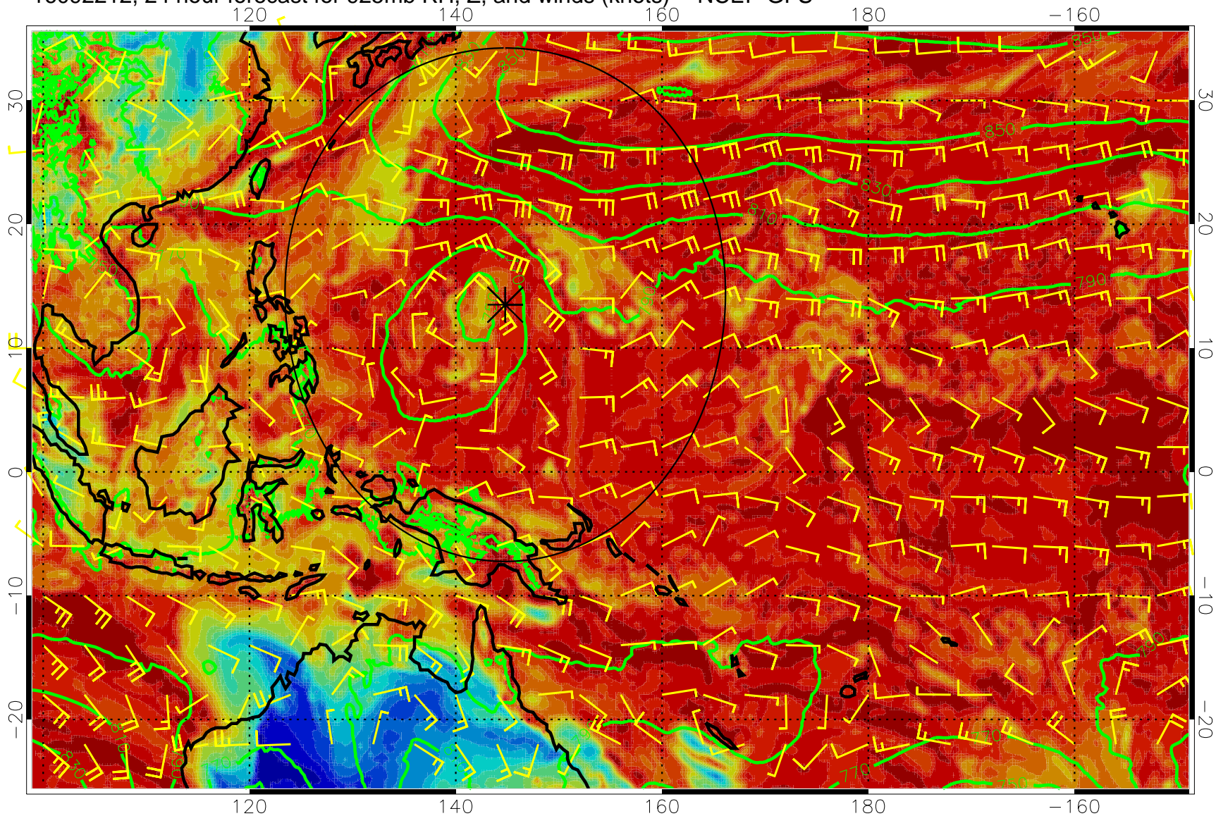
16092212, 24 hour forecast for 925mb RH, Z, and winds (knots) -- NCEP GFS
