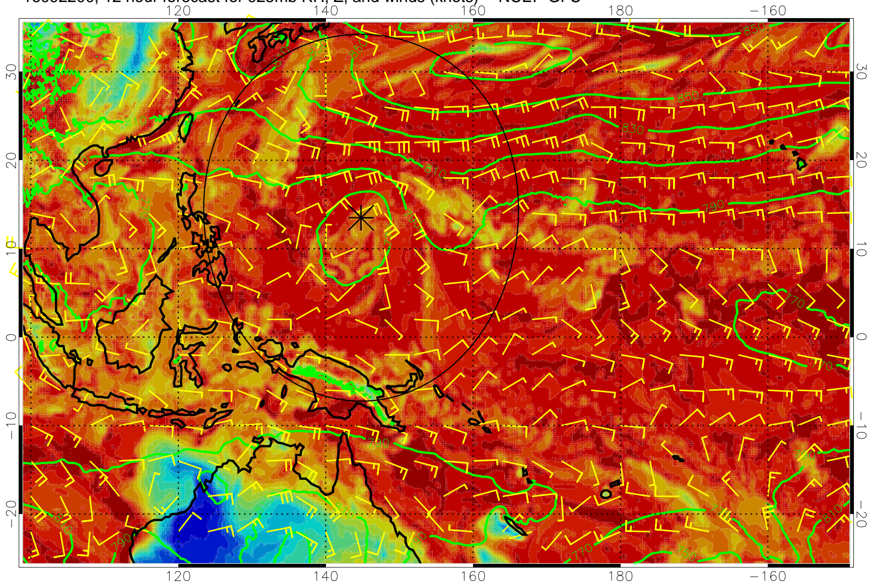
16092200, 12 hour forecast for 925mb RH, Z, and winds (knots) -- NCEP GFS
