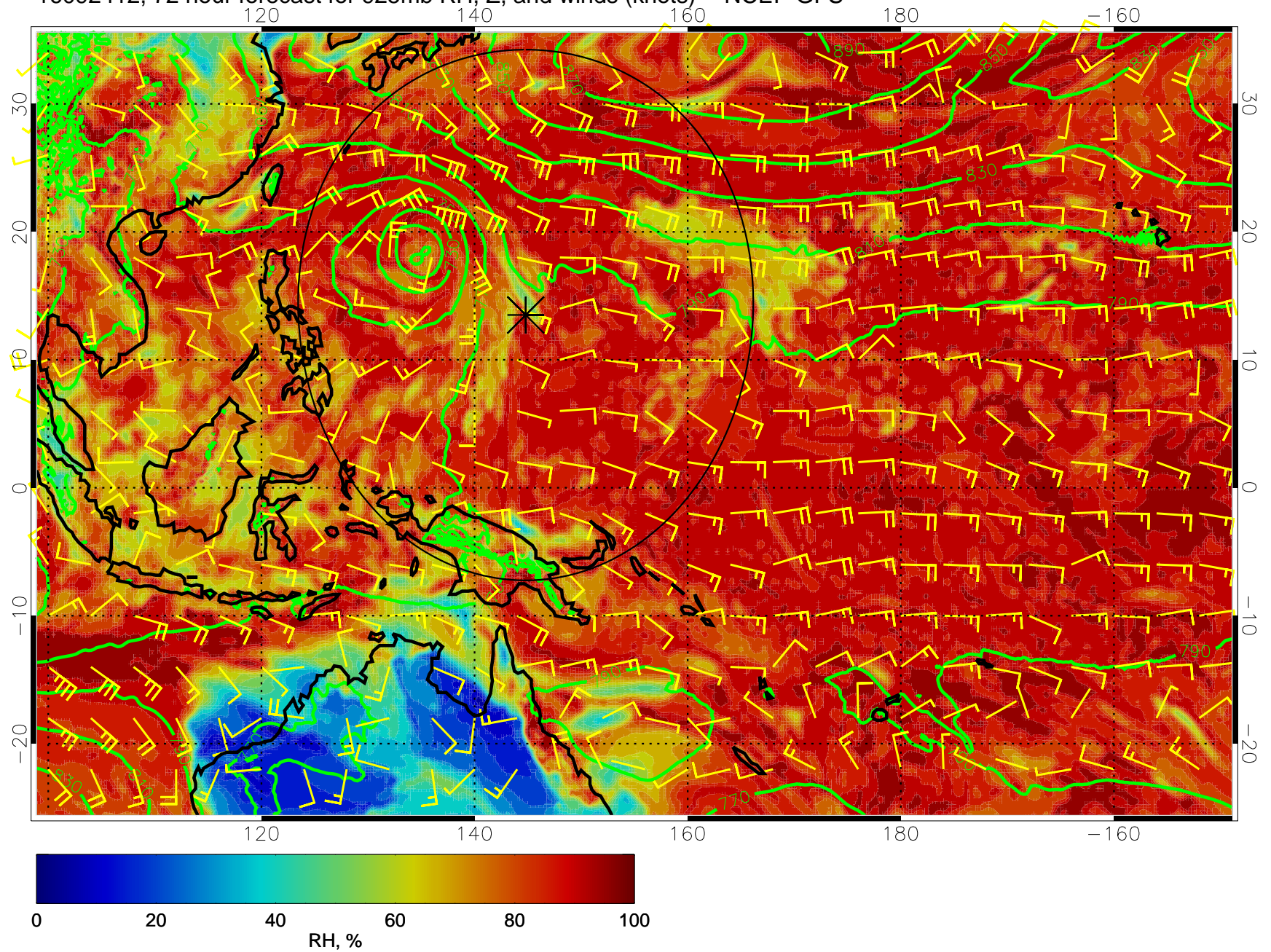
16092412, 72 hour forecast for 925mb RH, Z, and winds (knots) -- NCEP GFS
