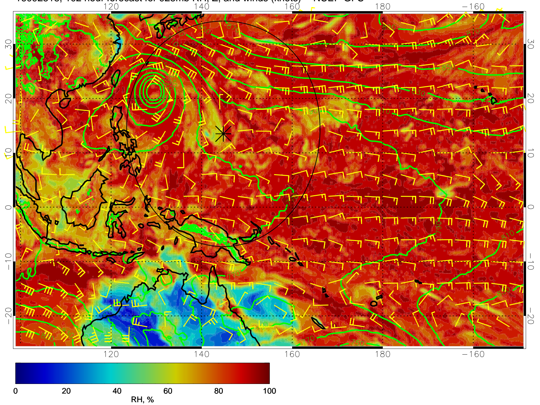
16092518, 102 hour forecast for 925mb RH, Z, and winds (knots) -- NCEP GFS
