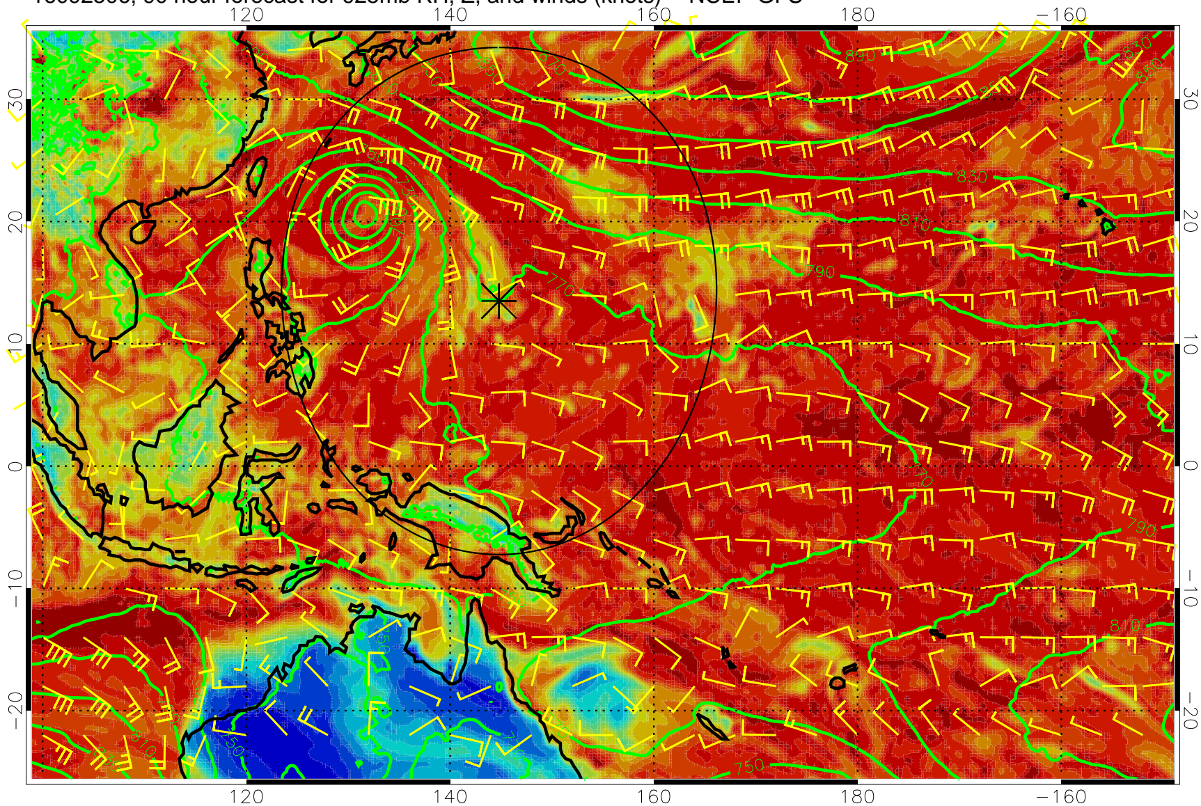
16092506, 90 hour forecast for 925mb RH, Z, and winds (knots) -- NCEP GFS
