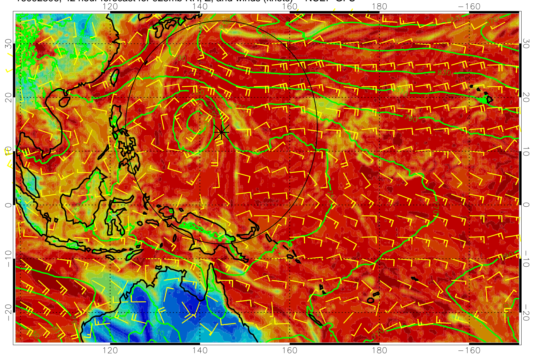
16092306, 42 hour forecast for 925mb RH, Z, and winds (knots) -- NCEP GFS
