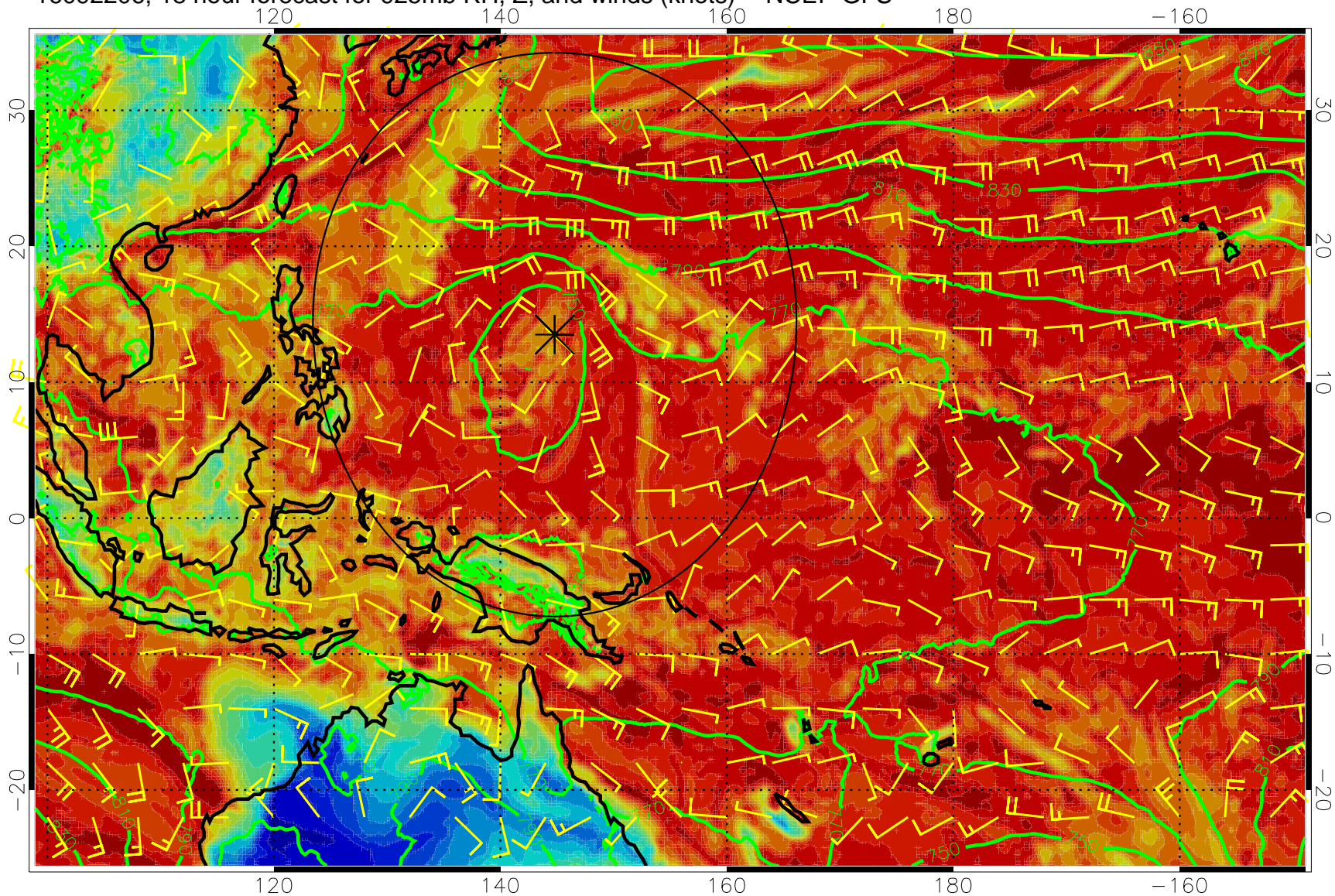
16092206, 18 hour forecast for 925mb RH, Z, and winds (knots) -- NCEP GFS
