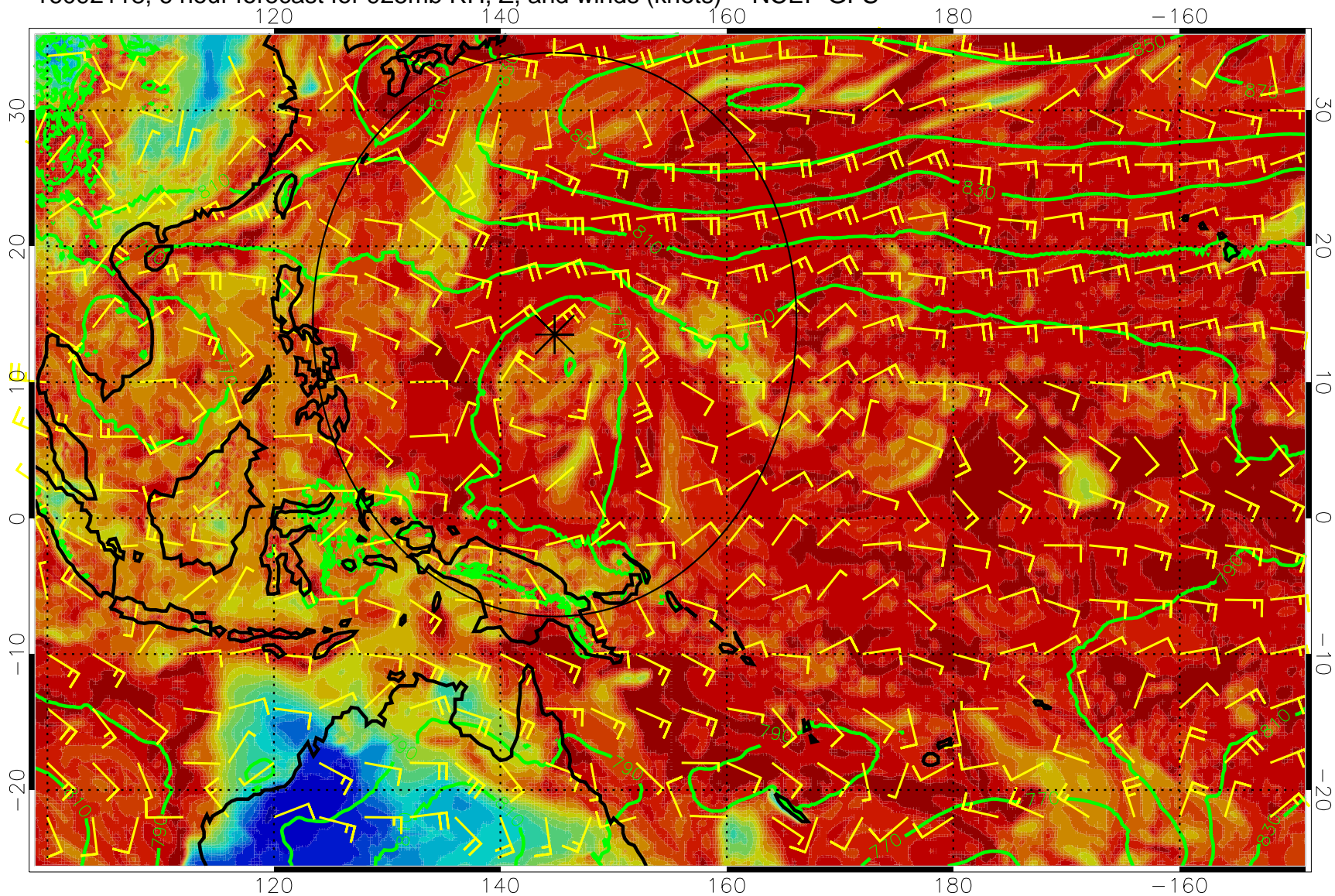
16092118, 6 hour forecast for 925mb RH, Z, and winds (knots) -- NCEP GFS
