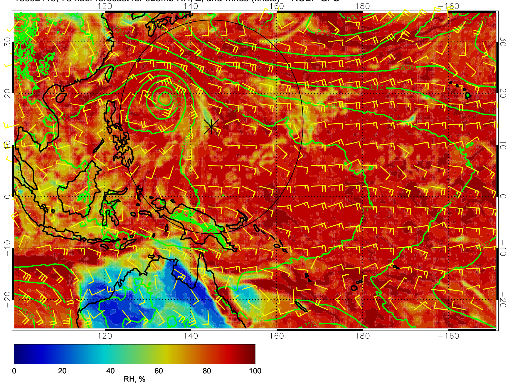
16092418, 78 hour forecast for 925mb RH, Z, and winds (knots) -- NCEP GFS
