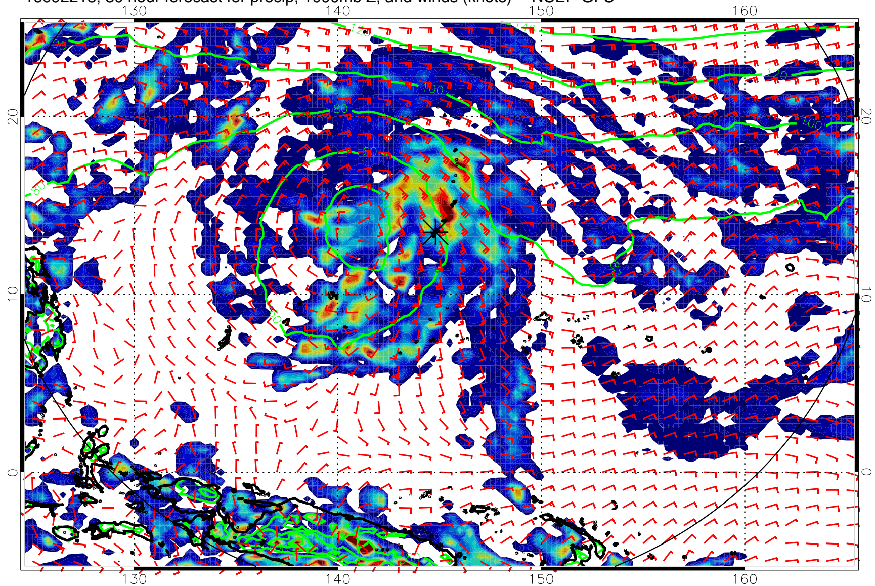
16092218, 30 hour forecast for precip, 1000mb Z, and winds (knots) -- NCEP GFS
