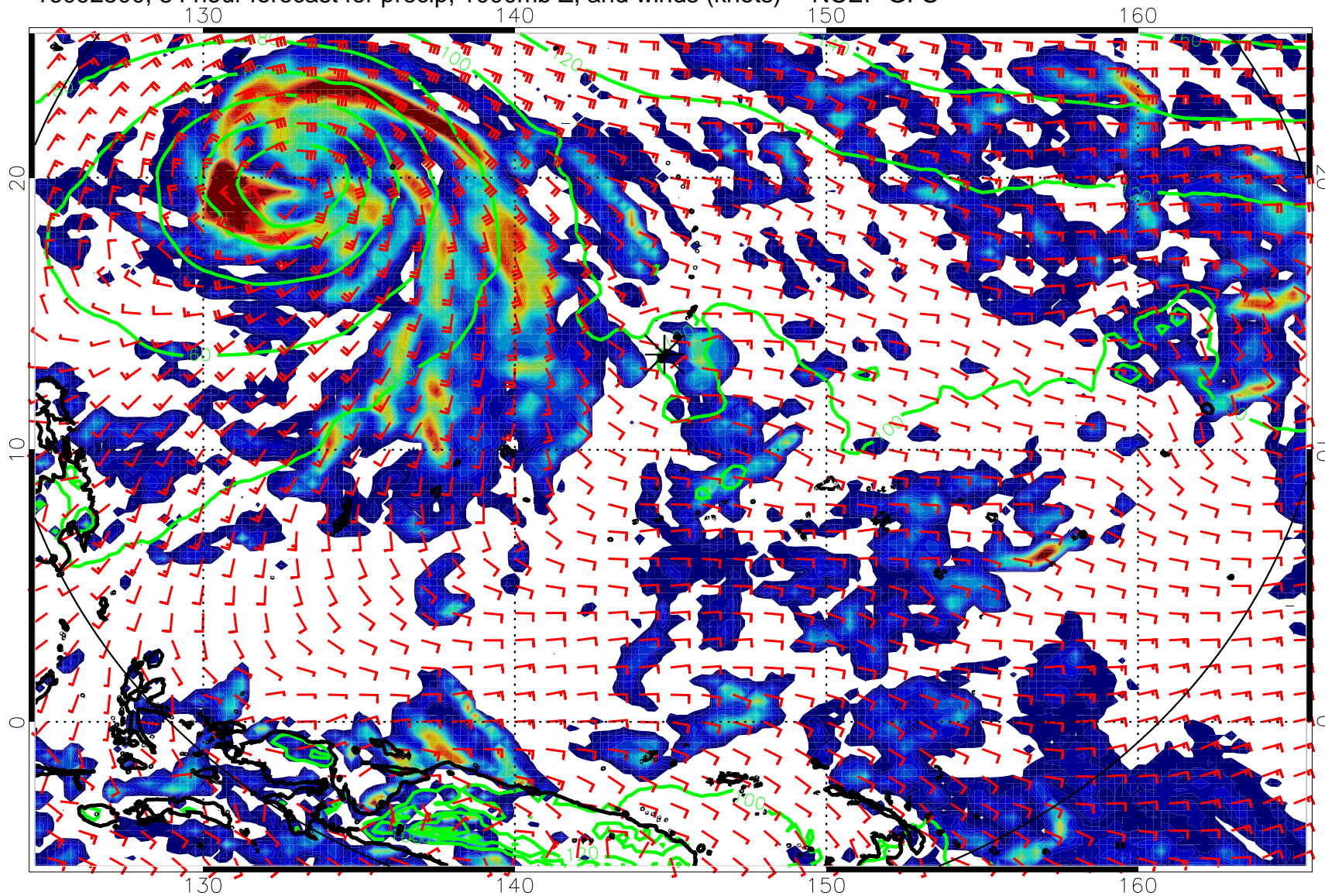
16092500, 84 hour forecast for precip, 1000mb Z, and winds (knots) -- NCEP GFS
