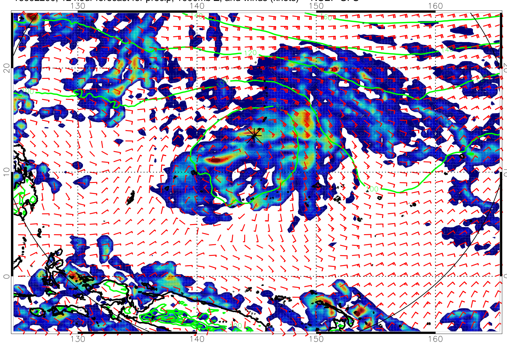
16092200, 12 hour forecast for precip, 1000mb Z, and winds (knots) -- NCEP GFS
