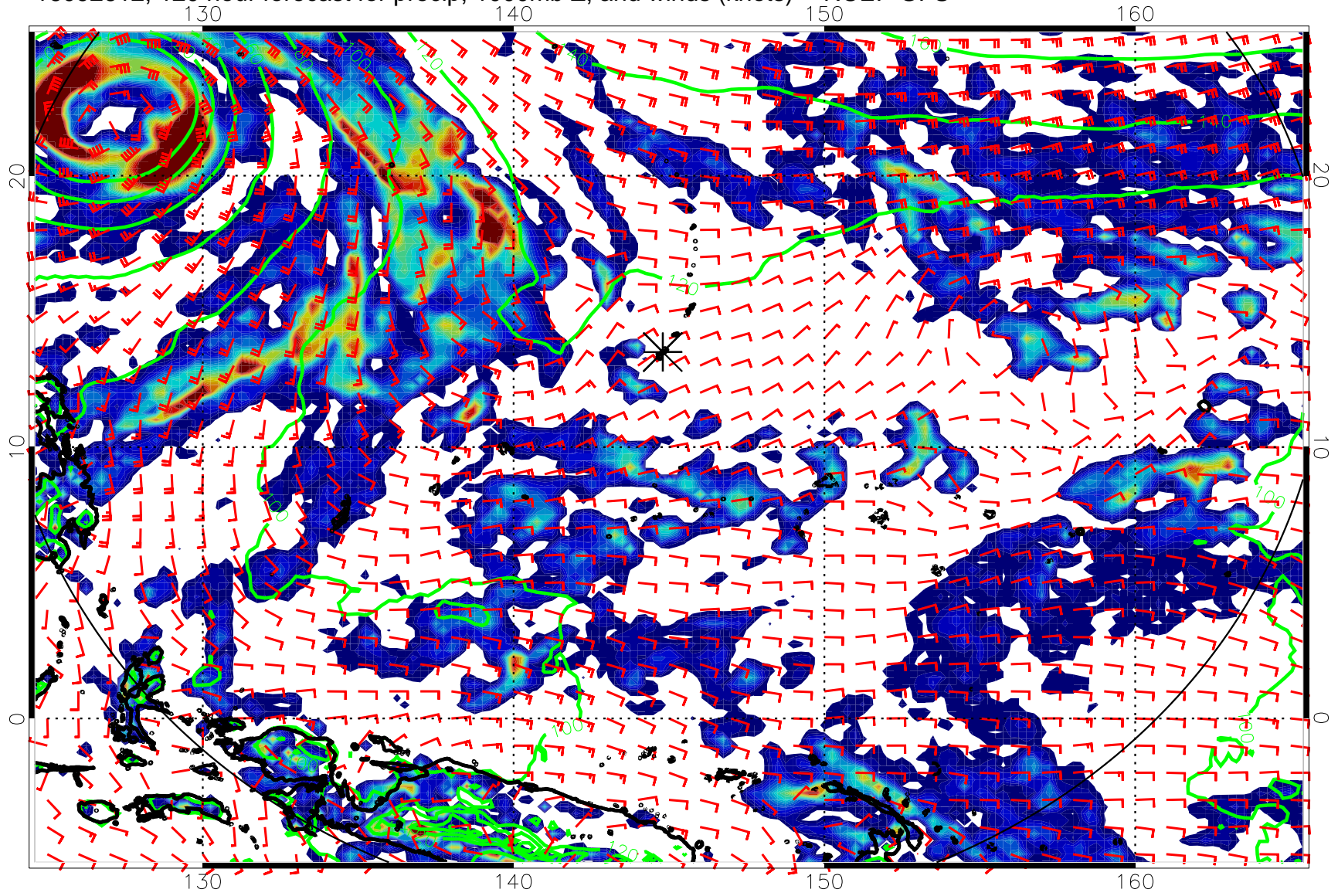
16092612, 120 hour forecast for precip, 1000mb Z, and winds (knots) -- NCEP GFS
