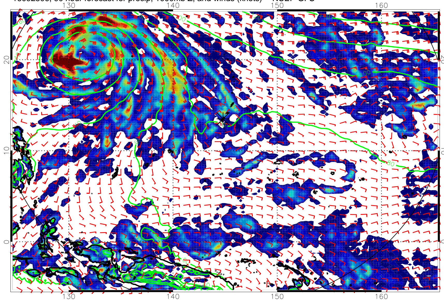
16092506, 90 hour forecast for precip, 1000mb Z, and winds (knots) -- NCEP GFS
