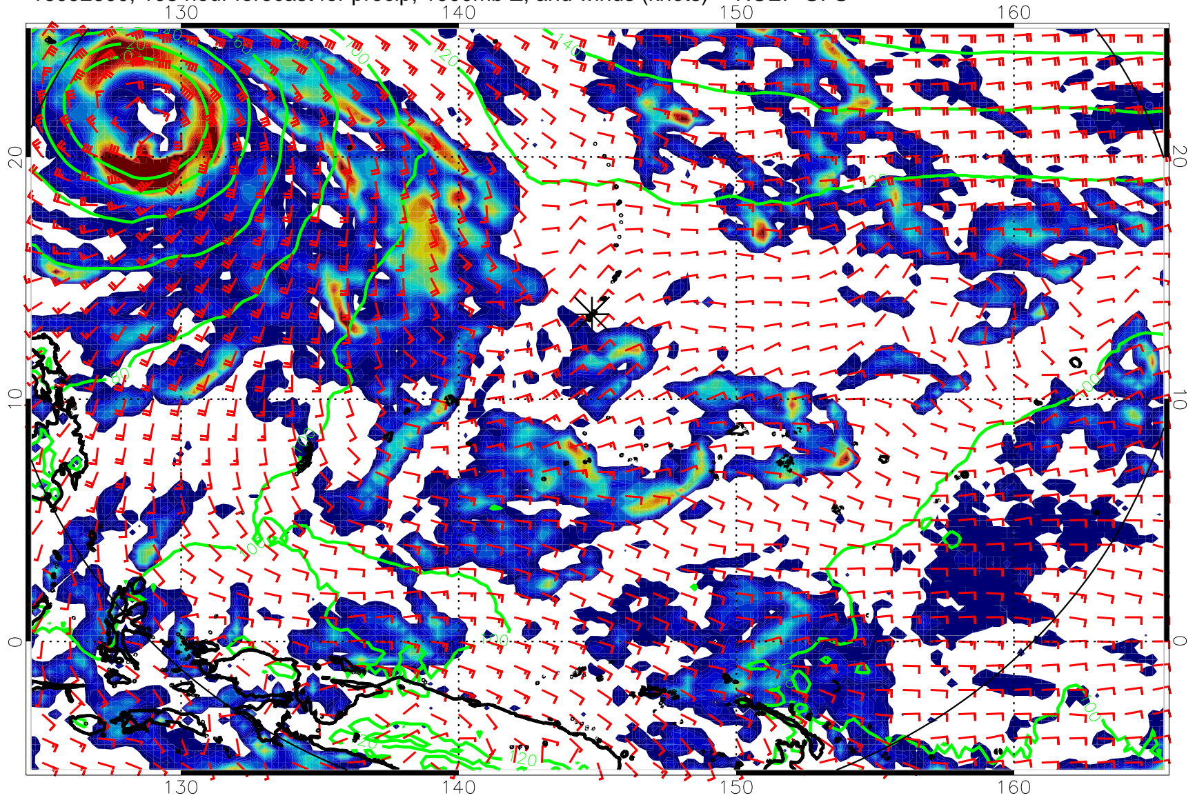
16092600, 108 hour forecast for precip, 1000mb Z, and winds (knots) -- NCEP GFS
