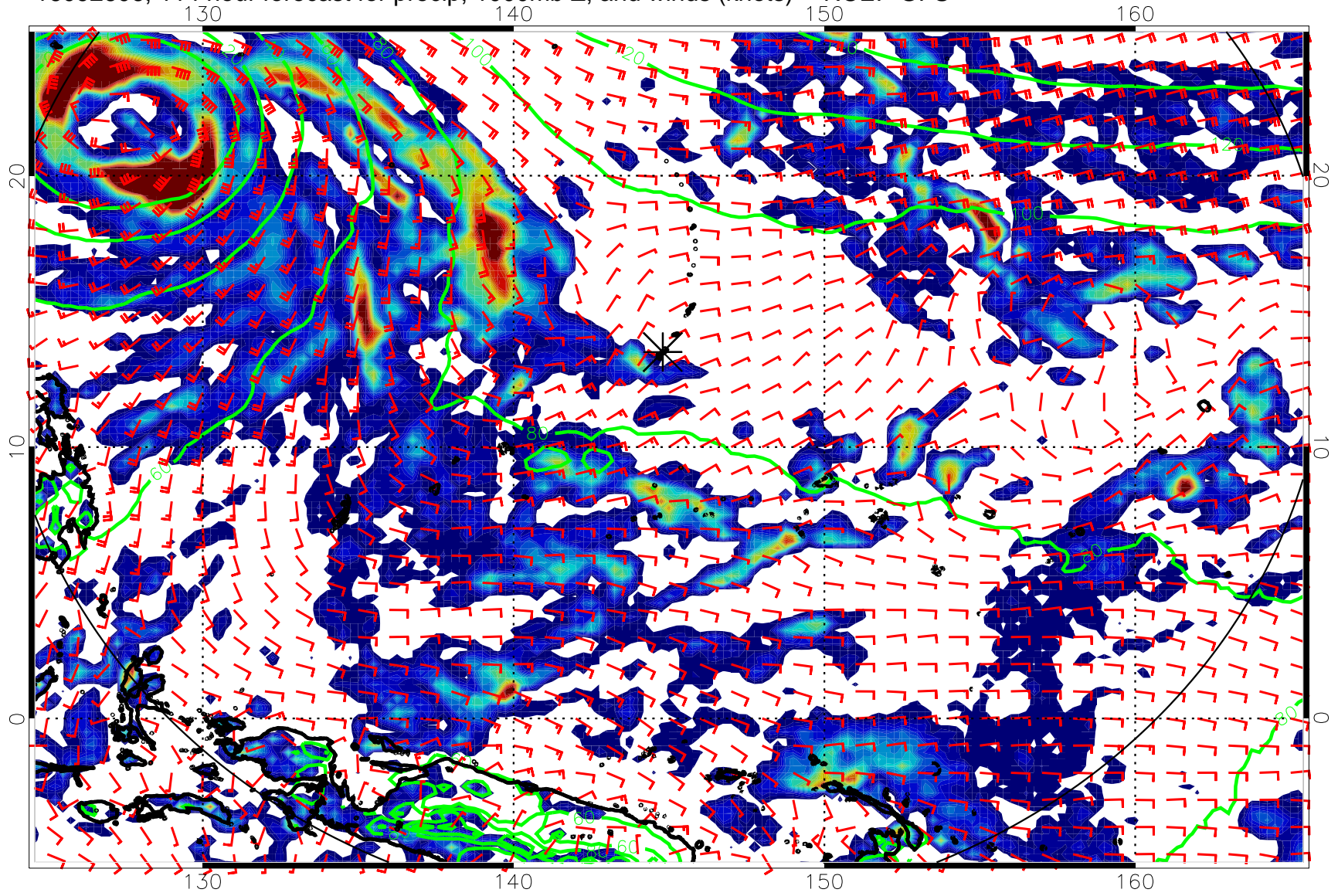
16092606, 114 hour forecast for precip, 1000mb Z, and winds (knots) -- NCEP GFS
