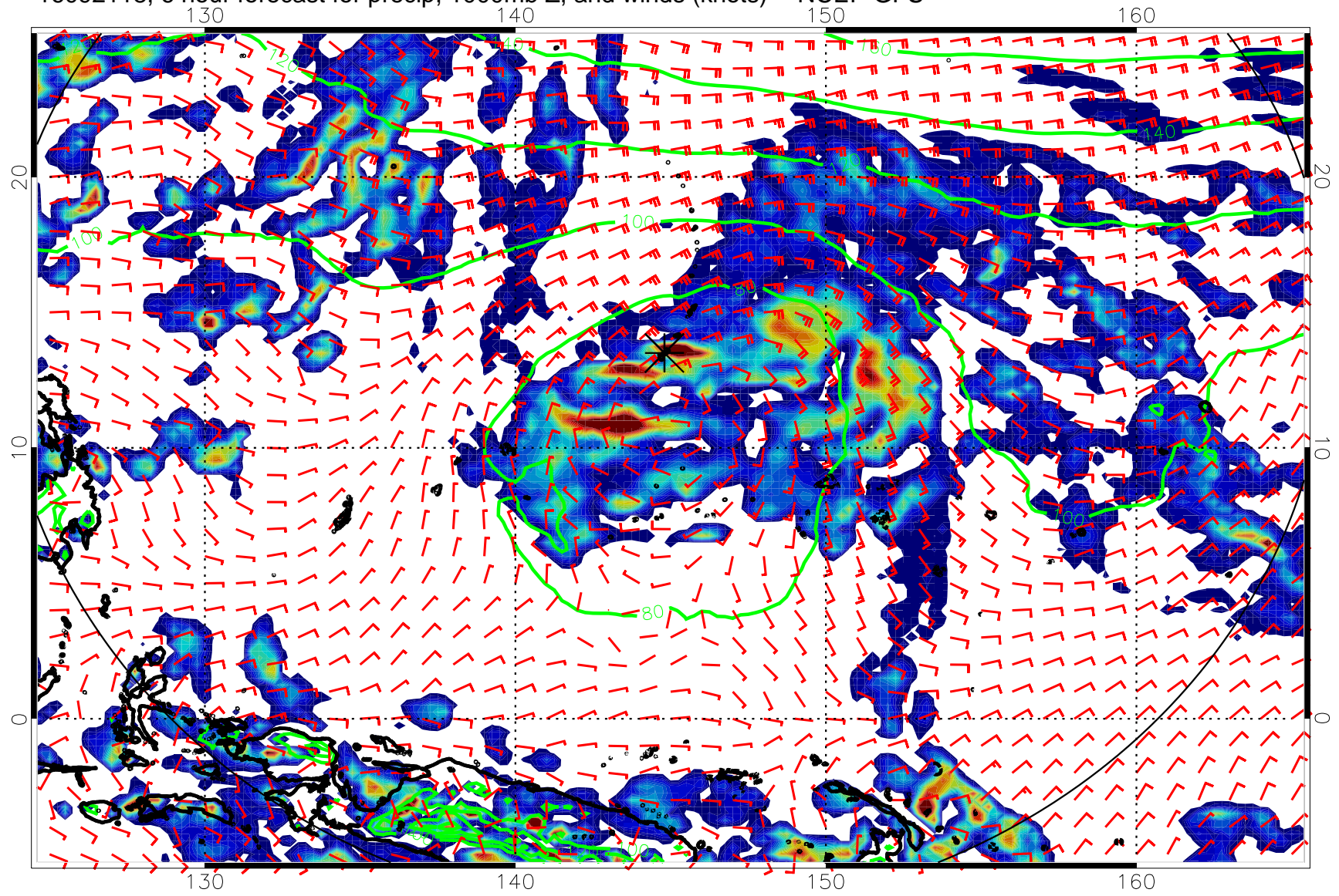
16092118, 6 hour forecast for precip, 1000mb Z, and winds (knots) -- NCEP GFS
