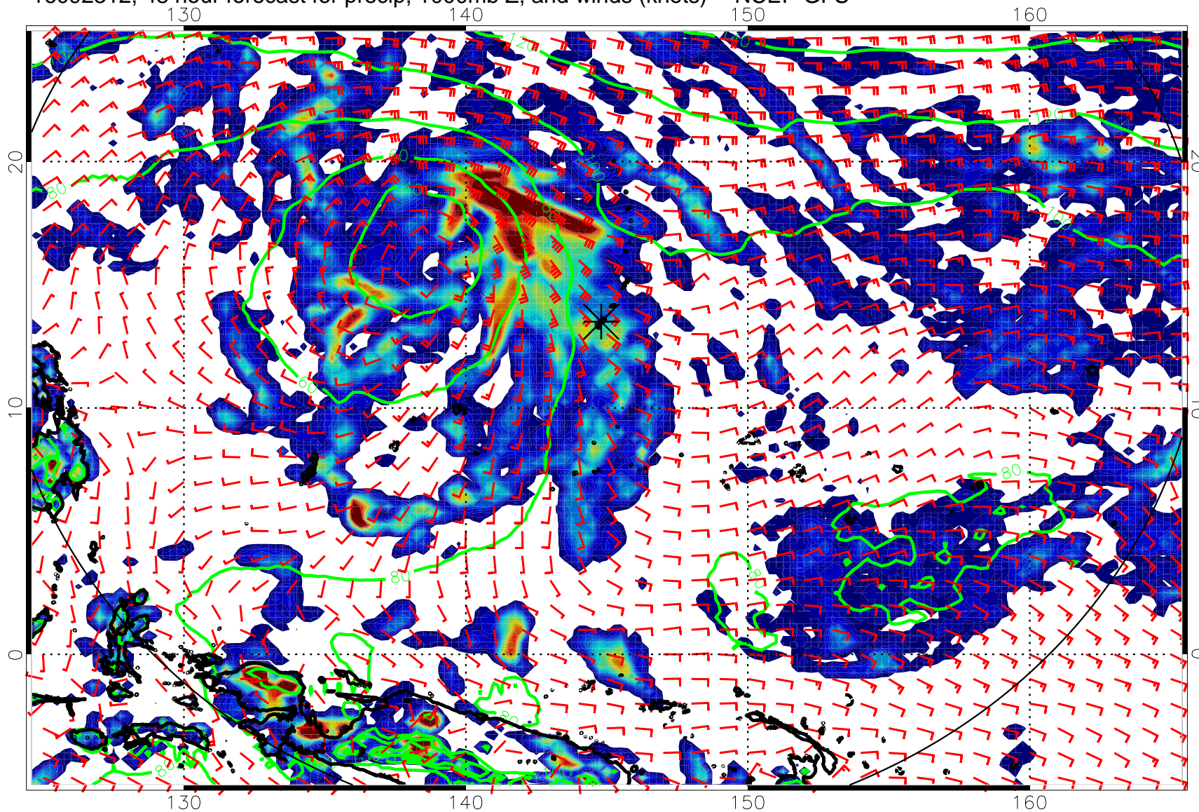
16092312, 48 hour forecast for precip, 1000mb Z, and winds (knots) -- NCEP GFS
