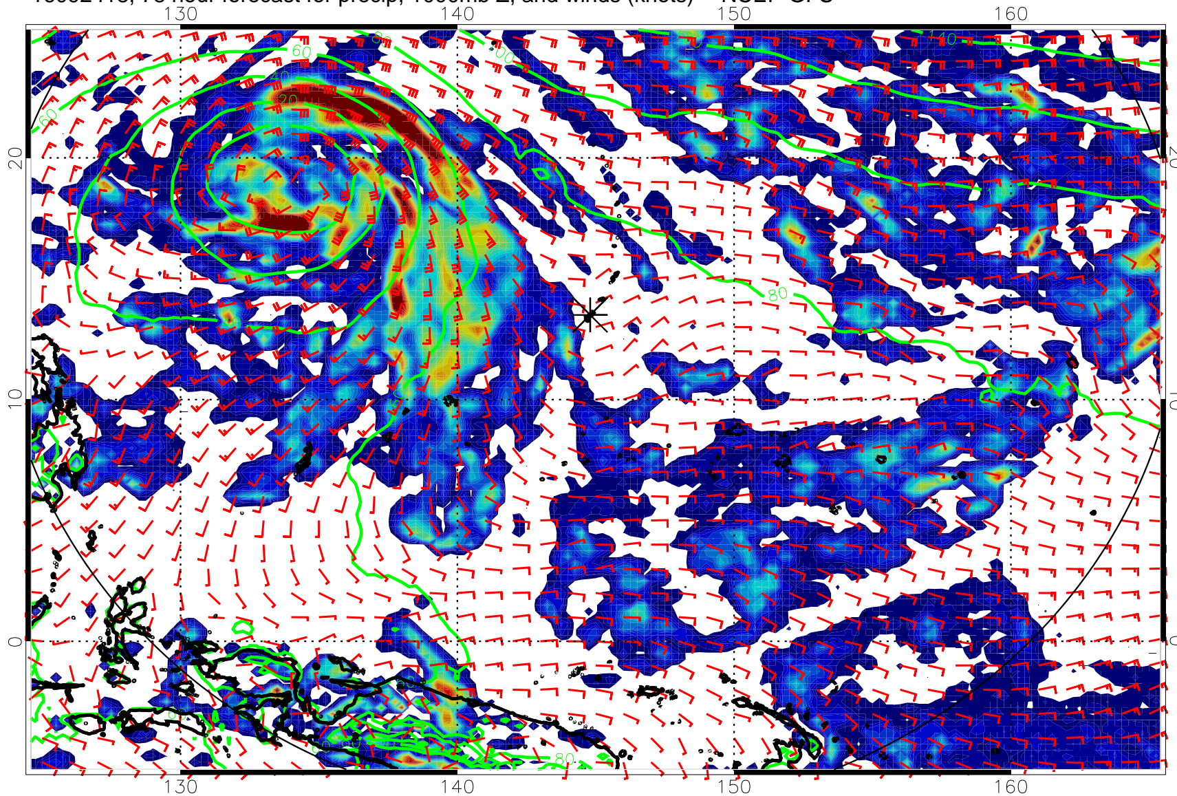
16092418, 78 hour forecast for precip, 1000mb Z, and winds (knots) -- NCEP GFS
