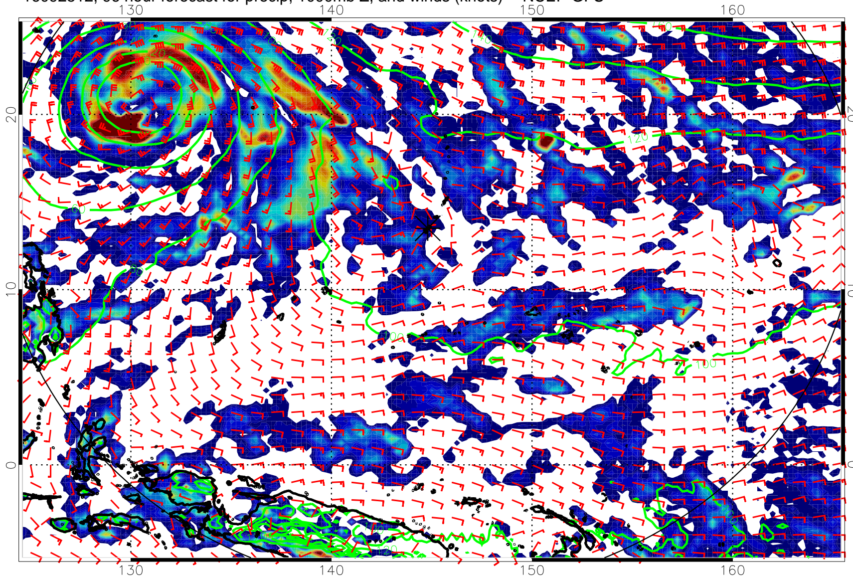
16092512, 96 hour forecast for precip, 1000mb Z, and winds (knots) -- NCEP GFS
