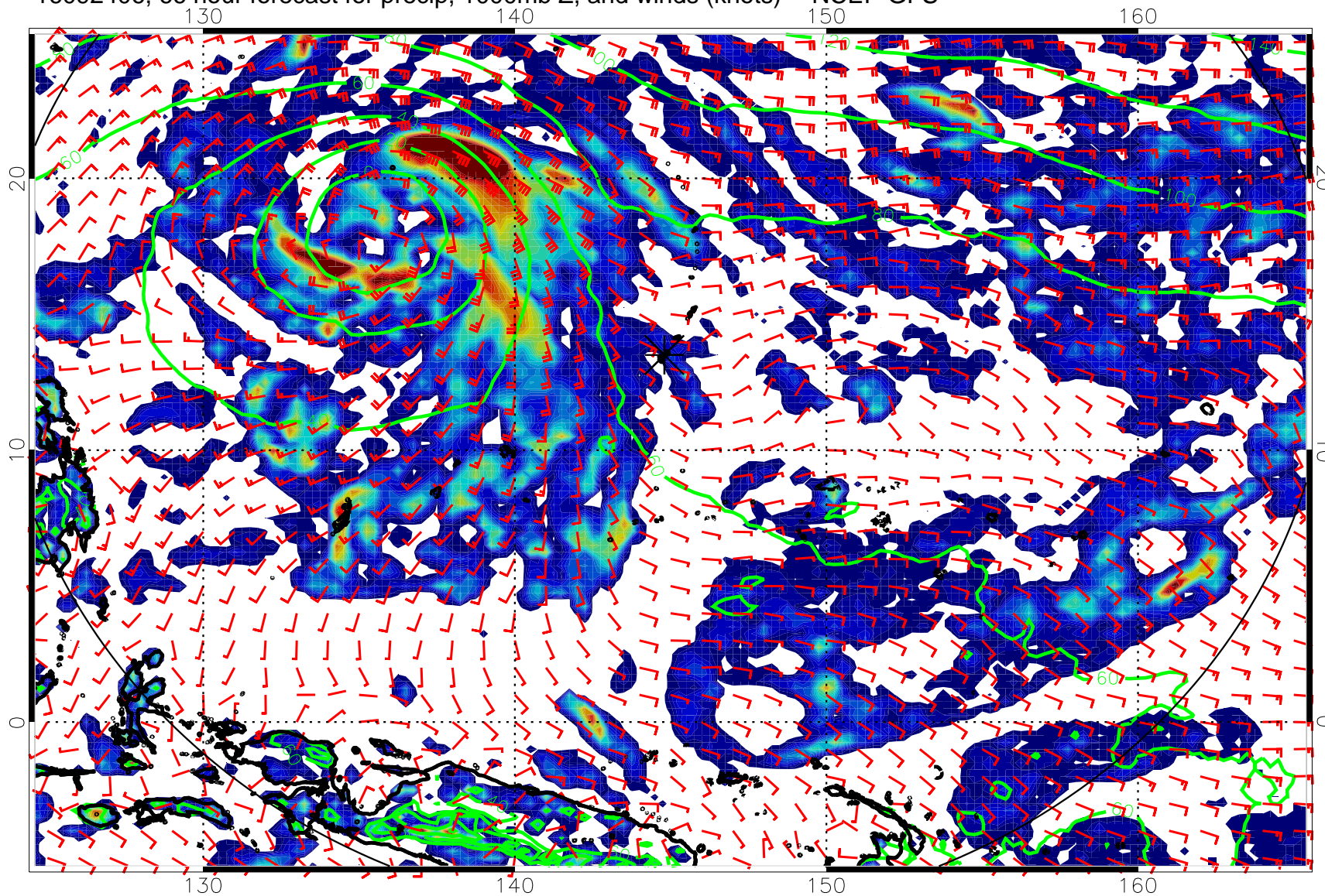
16092406, 66 hour forecast for precip, 1000mb Z, and winds (knots) -- NCEP GFS
