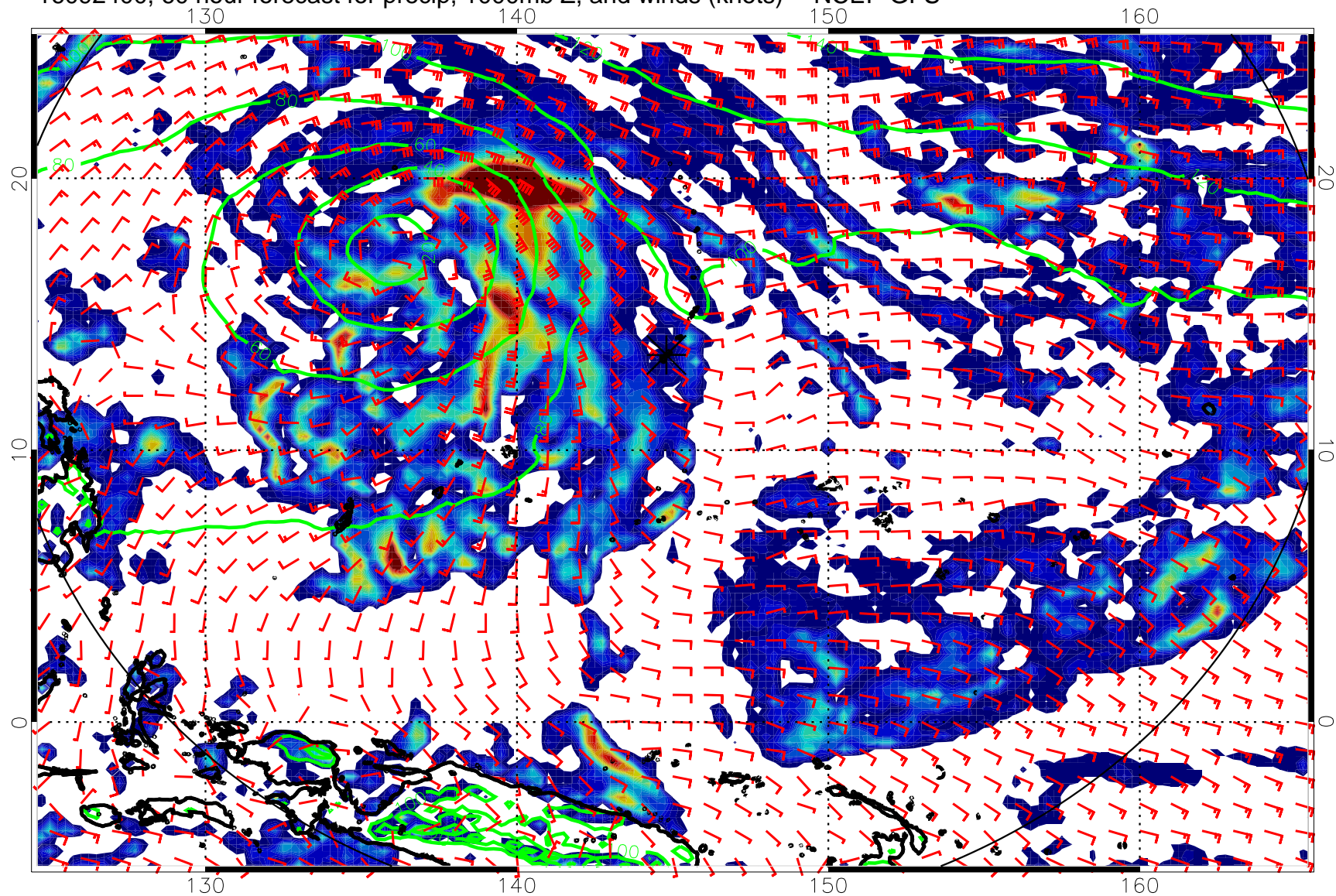
16092400, 60 hour forecast for precip, 1000mb Z, and winds (knots) -- NCEP GFS
