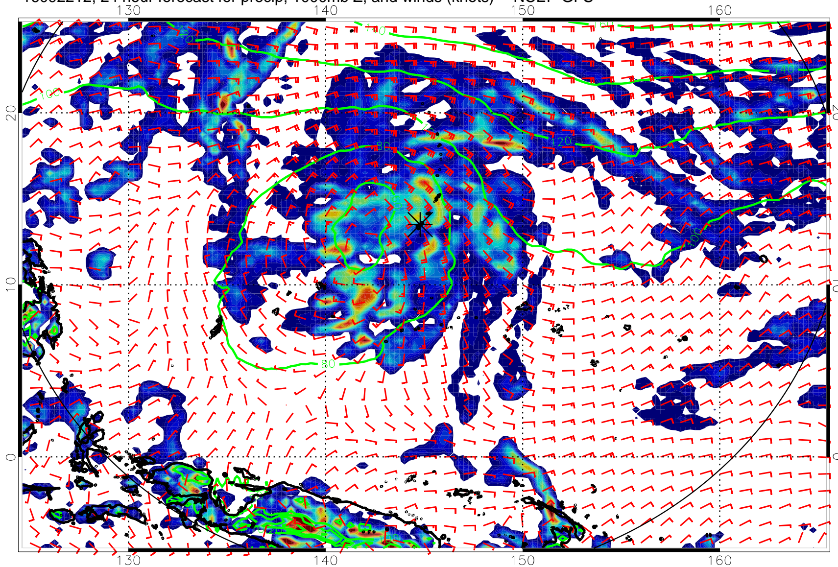
16092212, 24 hour forecast for precip, 1000mb Z, and winds (knots) -- NCEP GFS
