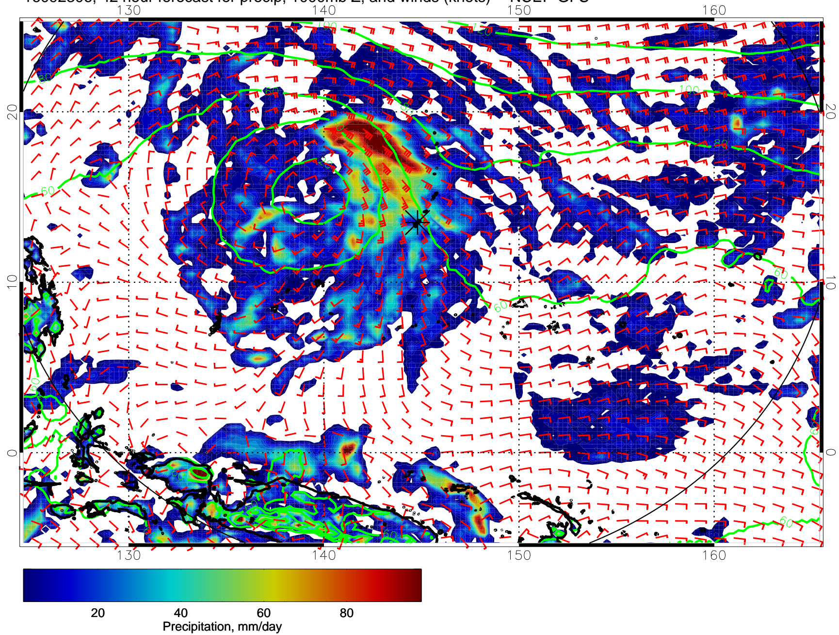
16092306, 42 hour forecast for precip, 1000mb Z, and winds (knots) -- NCEP GFS
