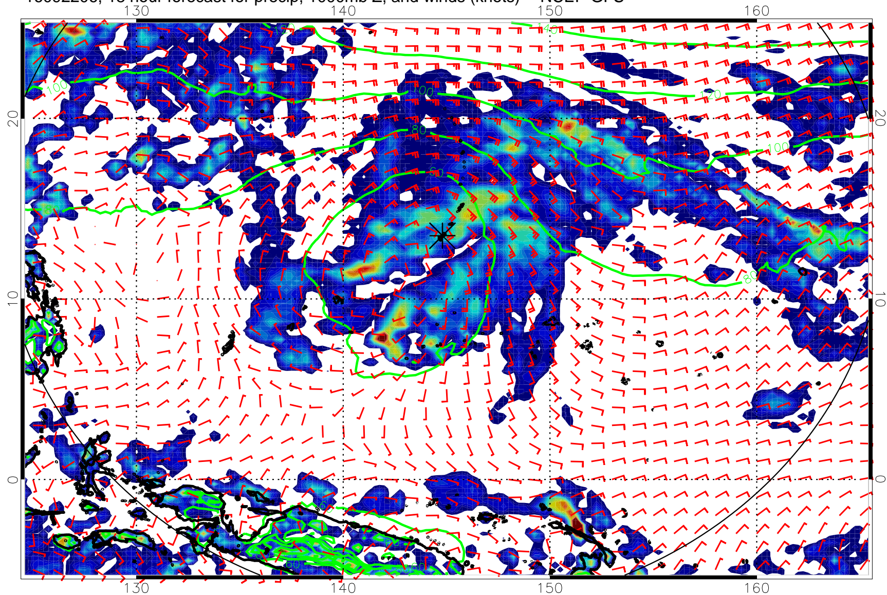
16092206, 18 hour forecast for precip, 1000mb Z, and winds (knots) -- NCEP GFS
