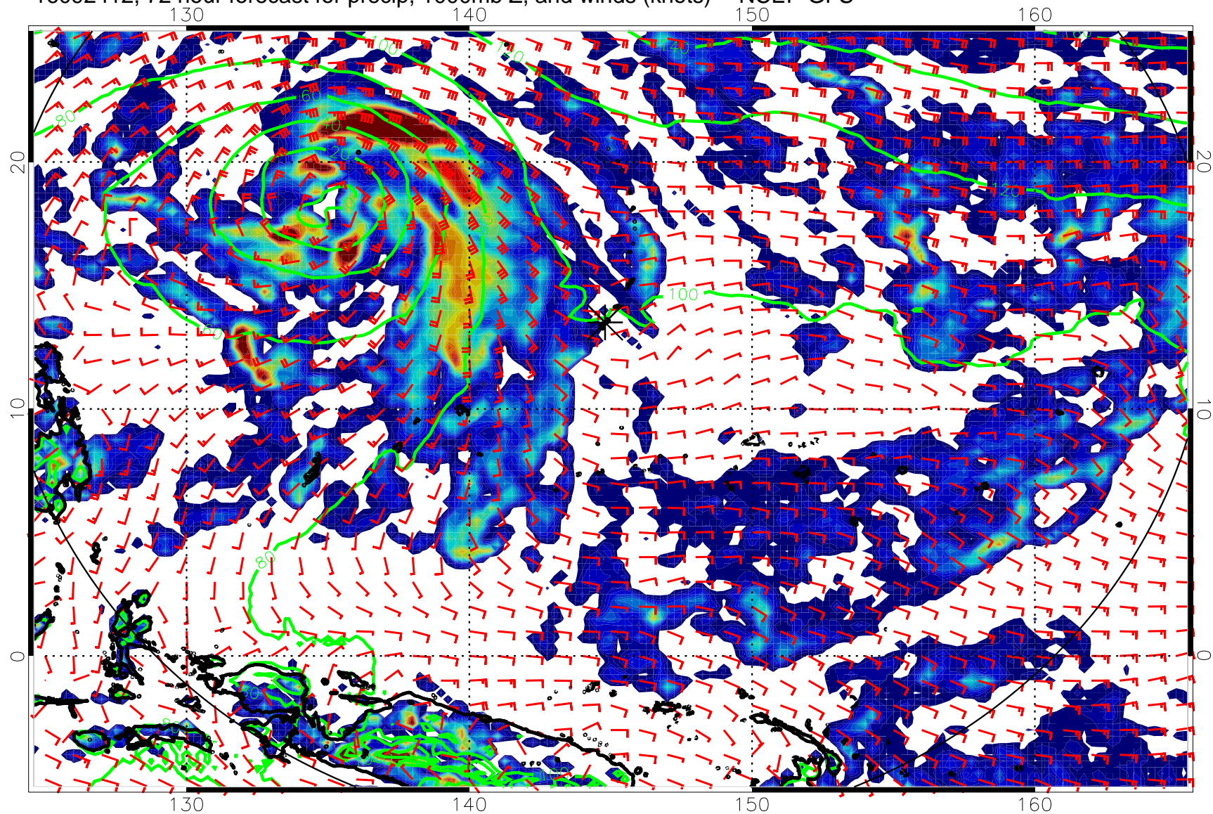
16092412, 72 hour forecast for precip, 1000mb Z, and winds (knots) -- NCEP GFS
