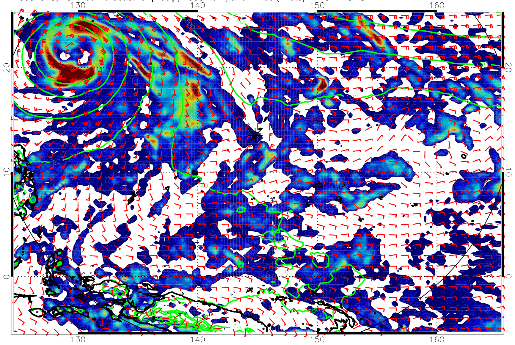
16092518, 102 hour forecast for precip, 1000mb Z, and winds (knots) -- NCEP GFS
