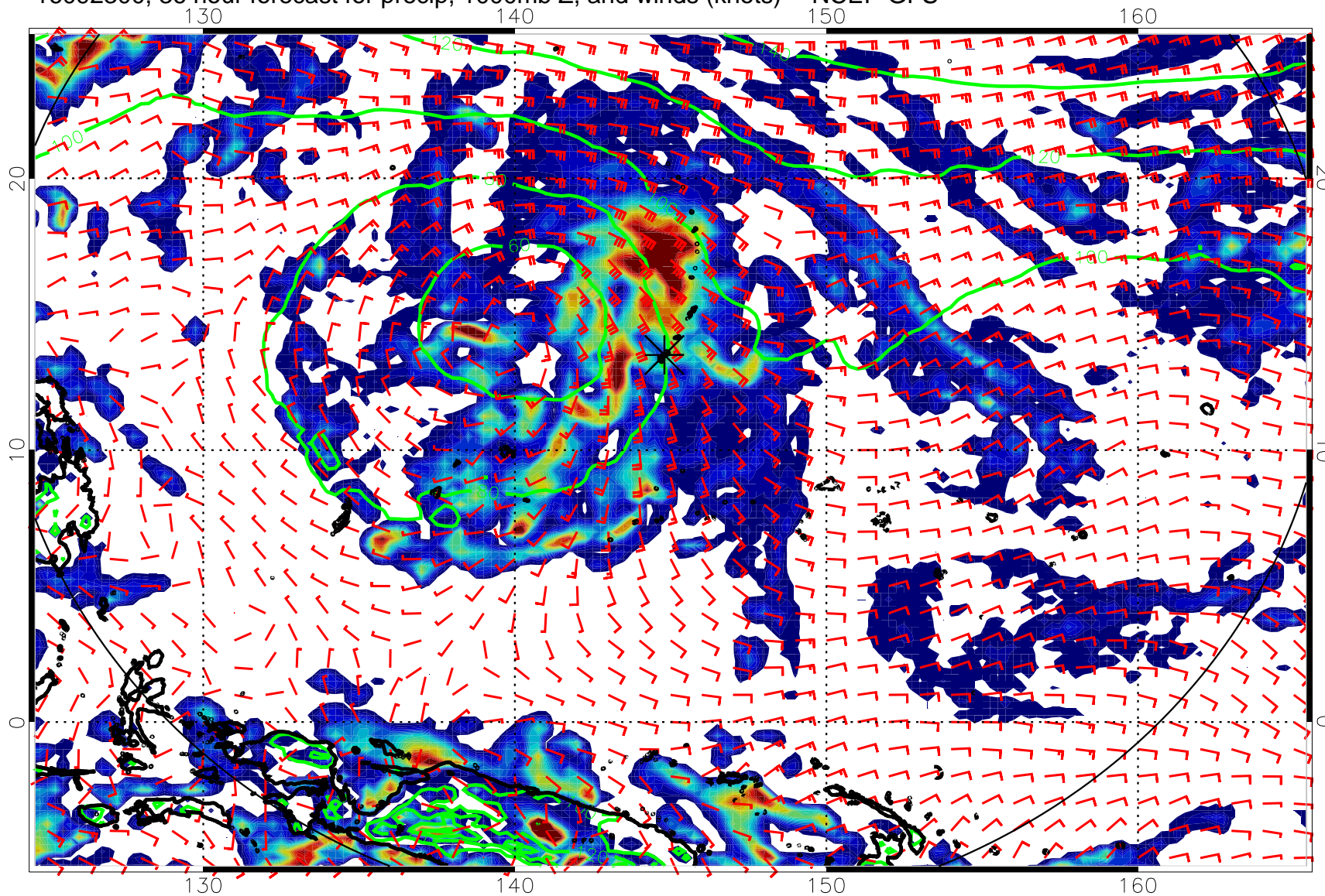
16092300, 36 hour forecast for precip, 1000mb Z, and winds (knots) -- NCEP GFS
