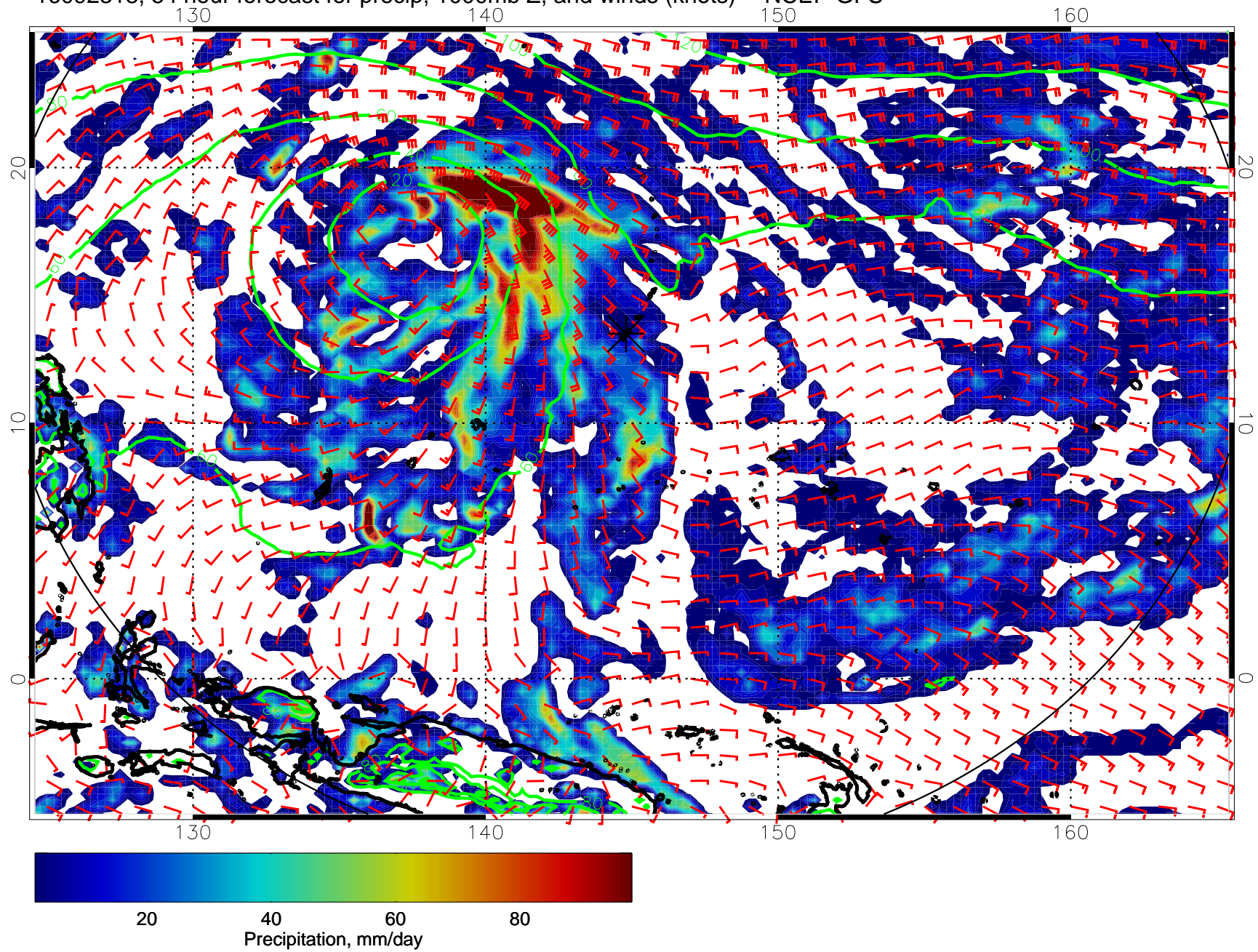
16092318, 54 hour forecast for precip, 1000mb Z, and winds (knots) -- NCEP GFS
