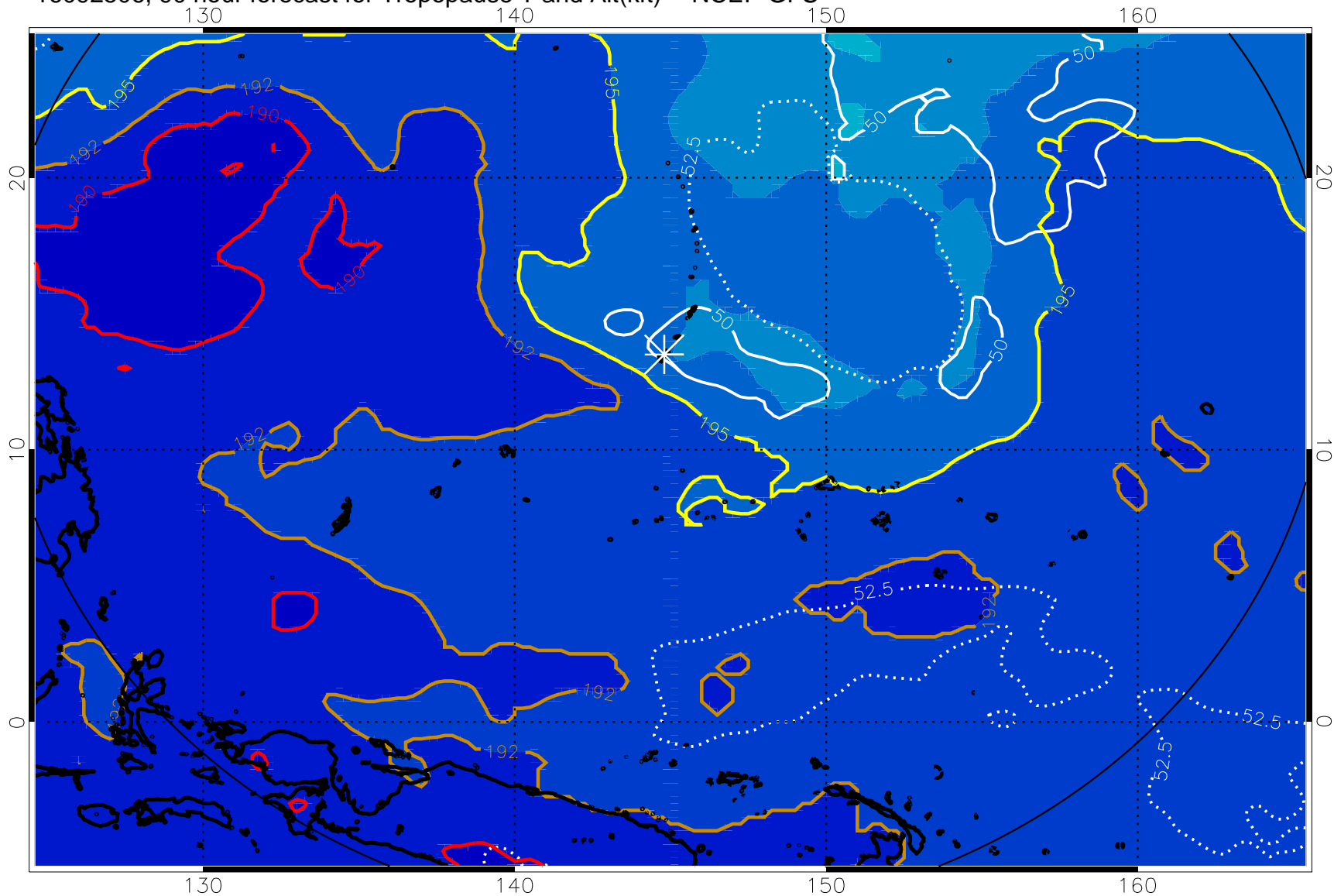
16092506, 90 hour forecast for Tropopause T and Alt(kft) -- NCEP GFS
