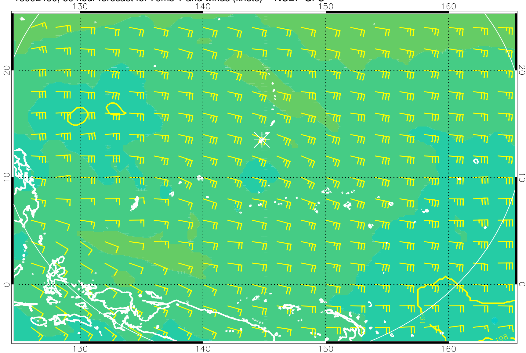
16092400, 60 hour forecast for 70mb T and winds (knots) -- NCEP GFS
