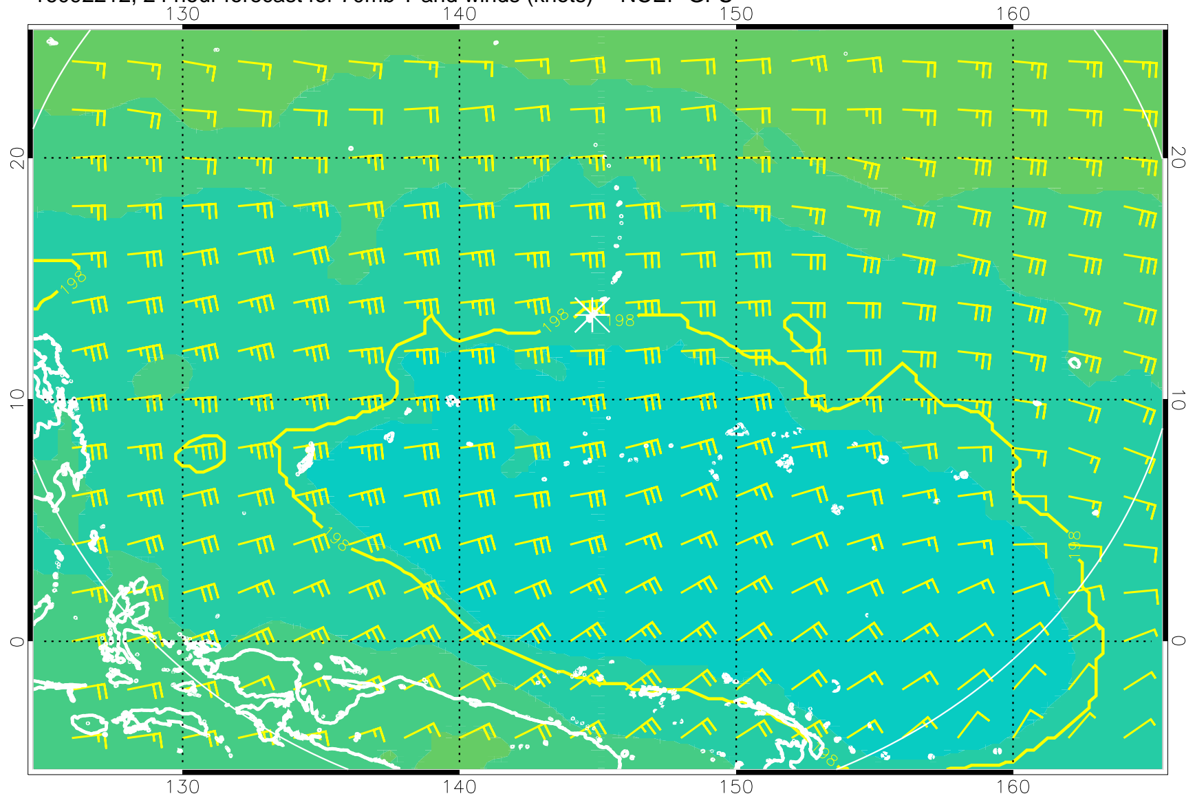
16092212, 24 hour forecast for 70mb T and winds (knots) -- NCEP GFS
