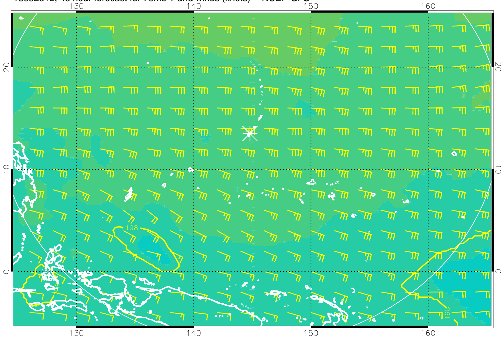
16092312, 48 hour forecast for 70mb T and winds (knots) -- NCEP GFS
