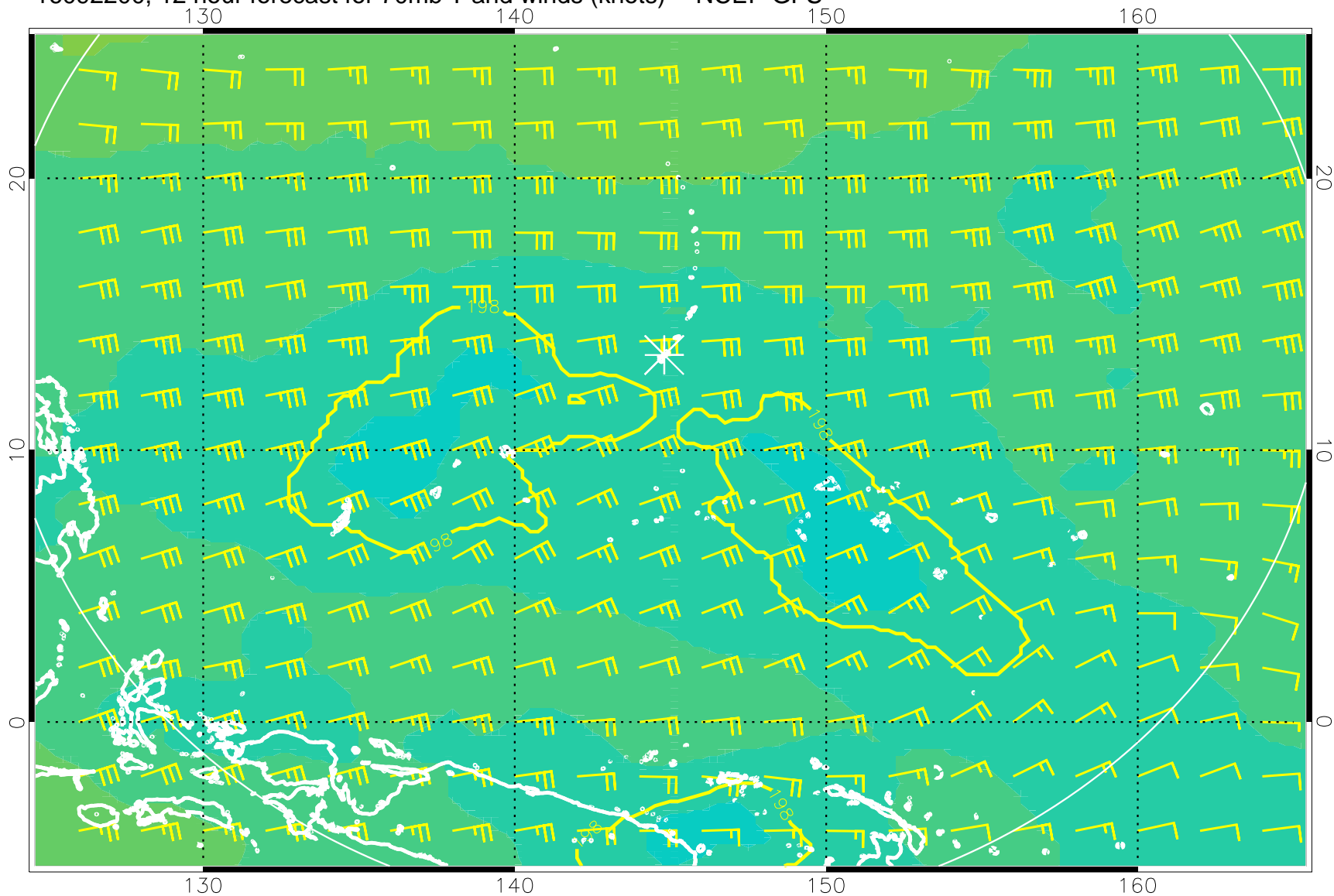
16092200, 12 hour forecast for 70mb T and winds (knots) -- NCEP GFS
