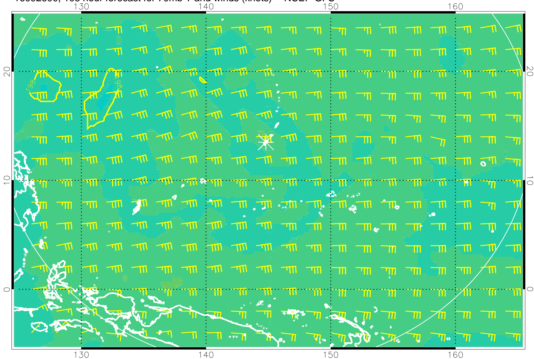
16092600, 108 hour forecast for 70mb T and winds (knots) -- NCEP GFS
