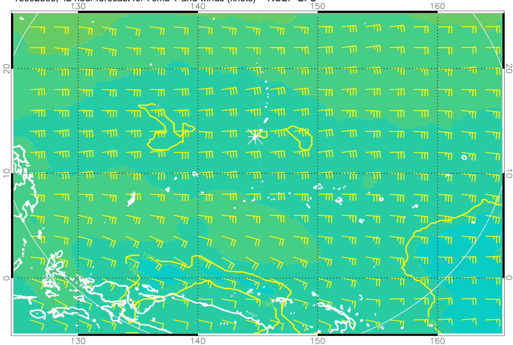
16092306, 42 hour forecast for 70mb T and winds (knots) -- NCEP GFS
