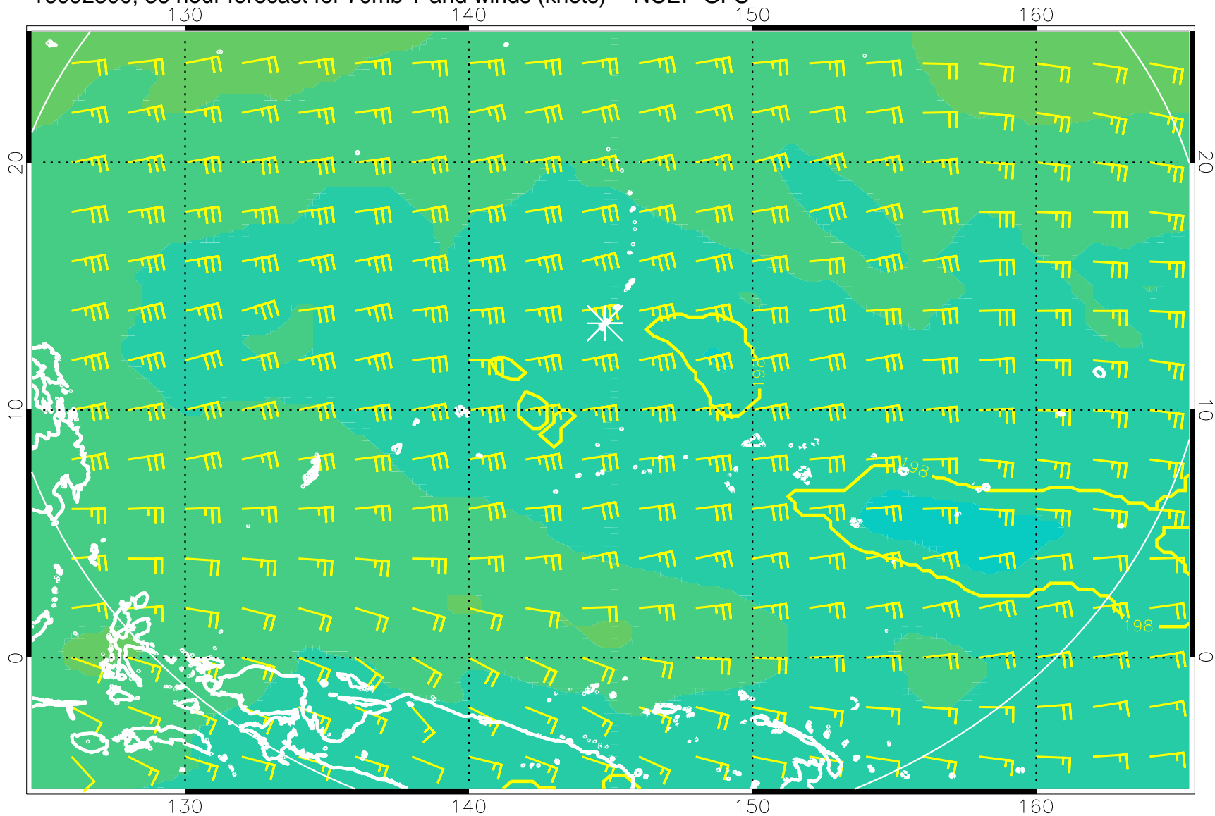
16092300, 36 hour forecast for 70mb T and winds (knots) -- NCEP GFS
