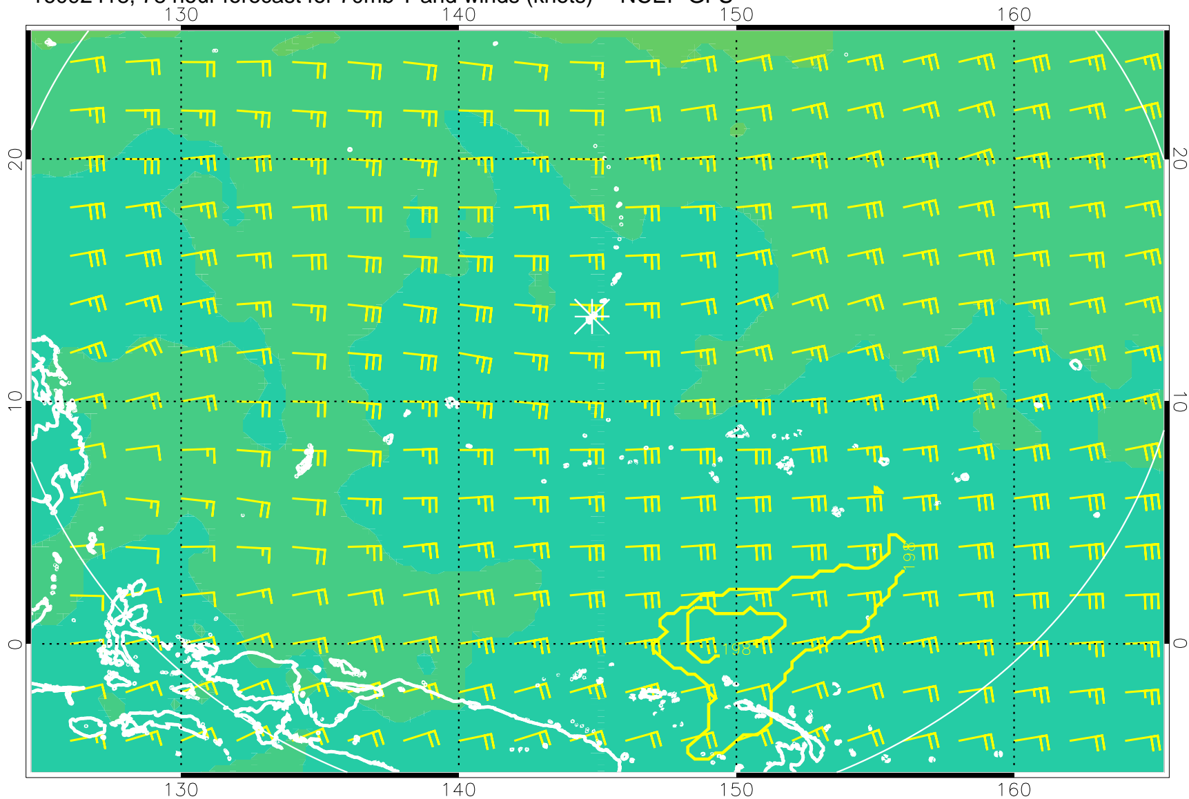
16092418, 78 hour forecast for 70mb T and winds (knots) -- NCEP GFS
