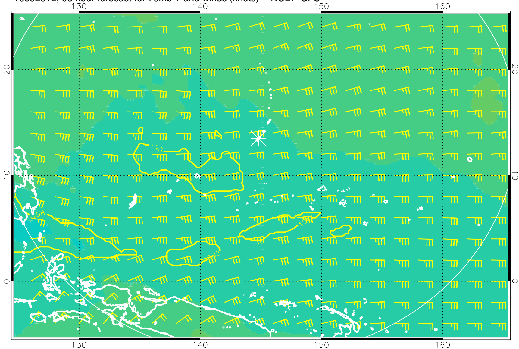
16092512, 96 hour forecast for 70mb T and winds (knots) -- NCEP GFS
