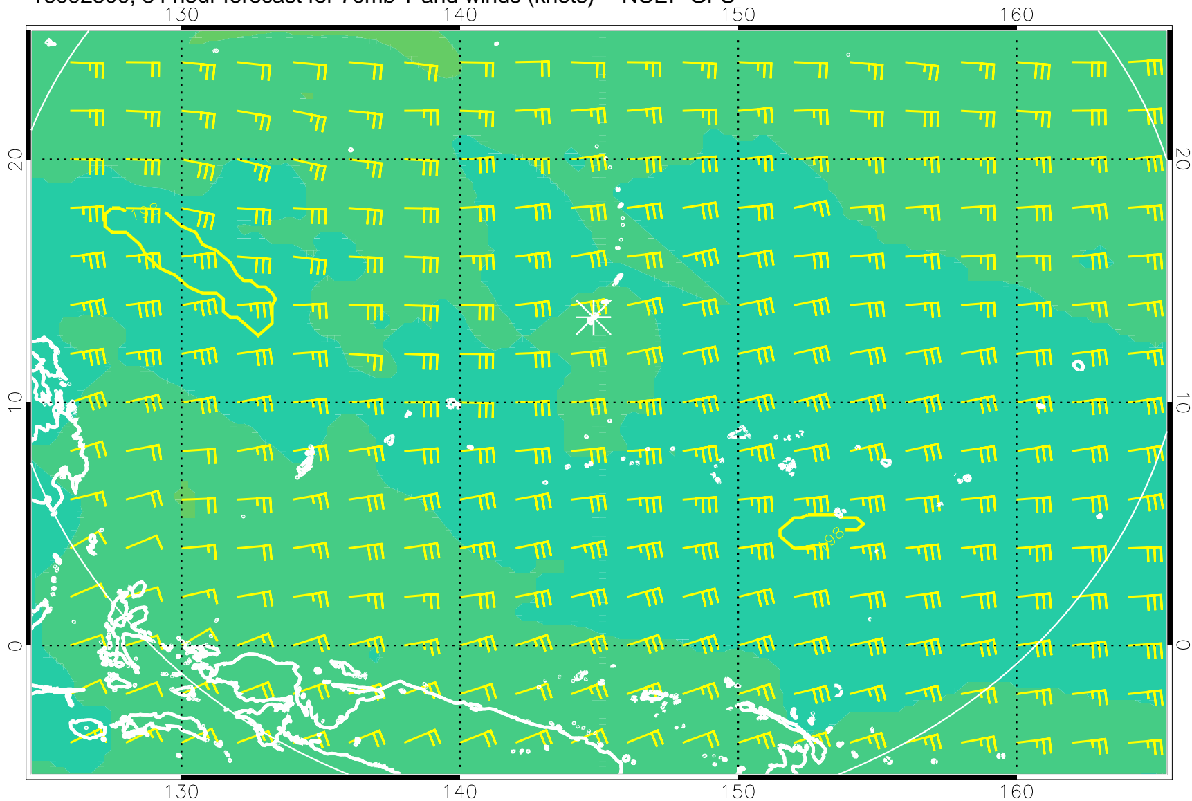
16092500, 84 hour forecast for 70mb T and winds (knots) -- NCEP GFS
