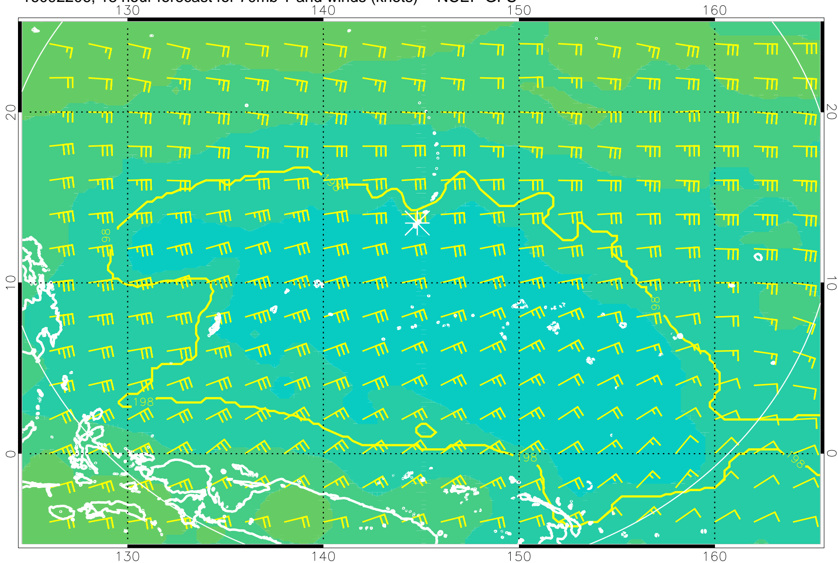
16092206, 18 hour forecast for 70mb T and winds (knots) -- NCEP GFS
