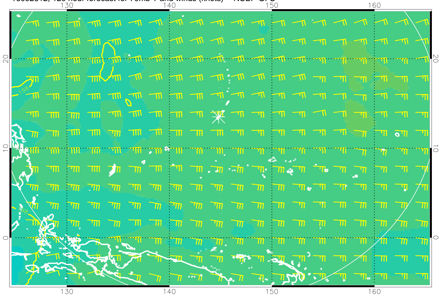
16092612, 120 hour forecast for 70mb T and winds (knots) -- NCEP GFS
