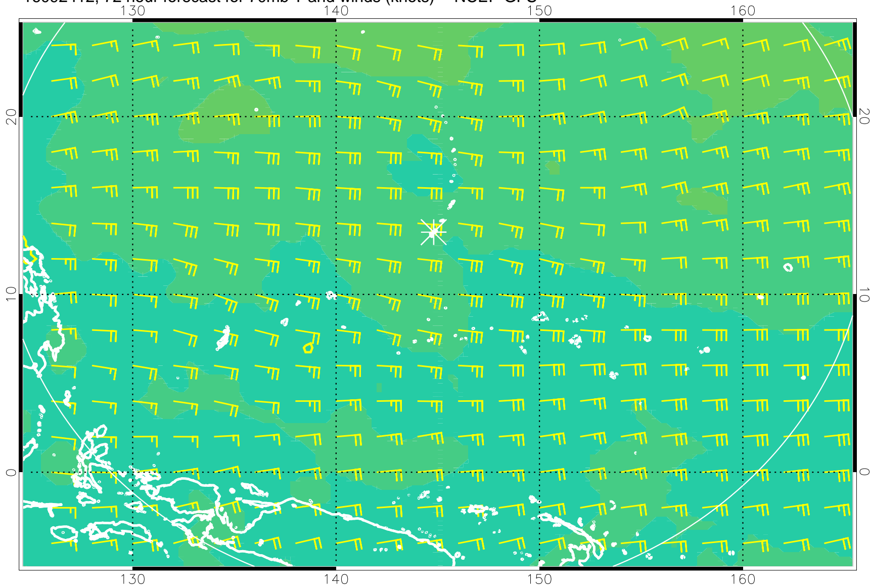
16092412, 72 hour forecast for 70mb T and winds (knots) -- NCEP GFS
