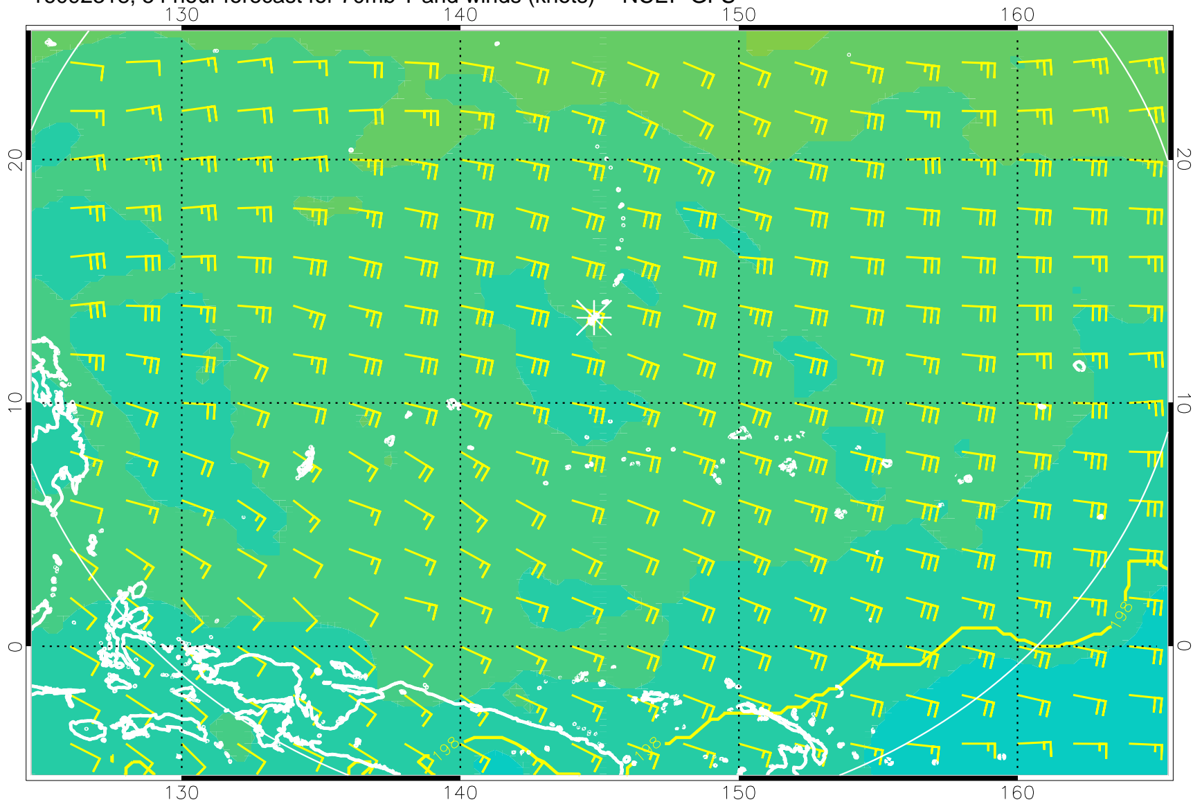
16092318, 54 hour forecast for 70mb T and winds (knots) -- NCEP GFS
