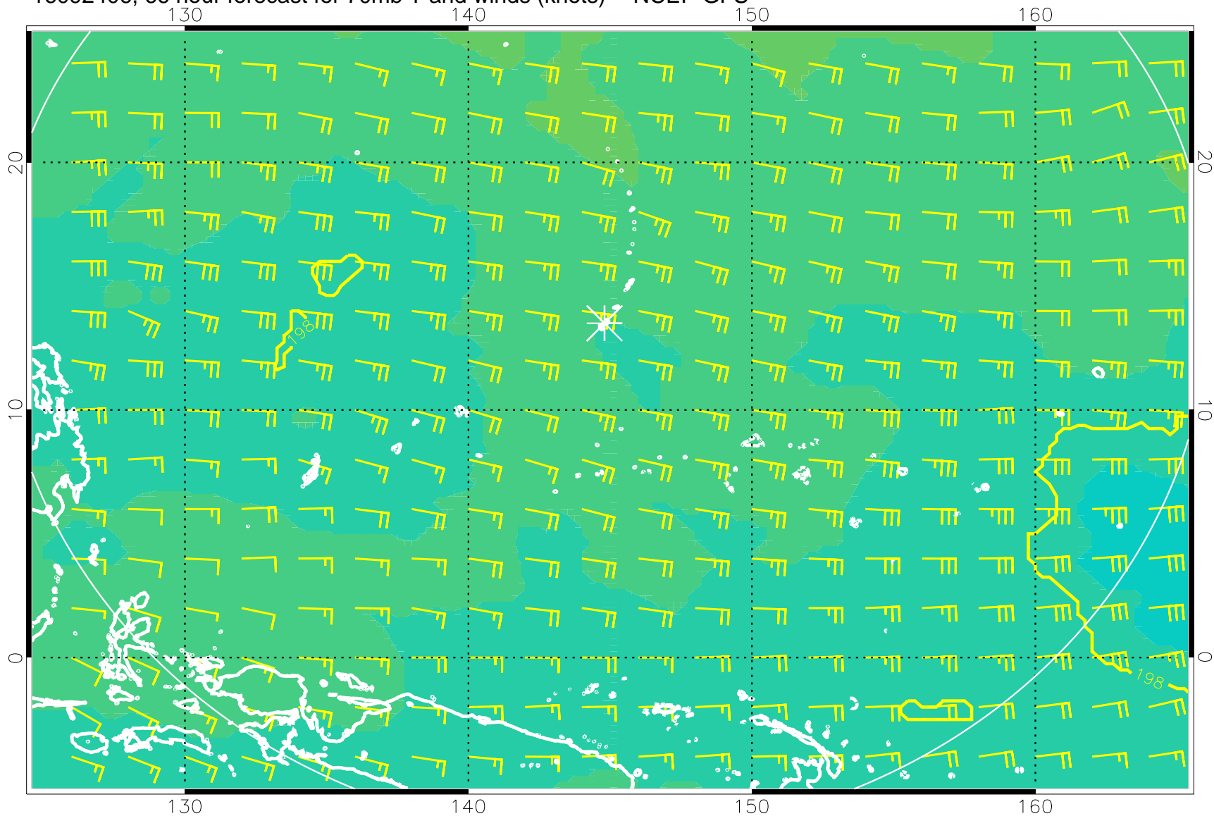
16092406, 66 hour forecast for 70mb T and winds (knots) -- NCEP GFS
