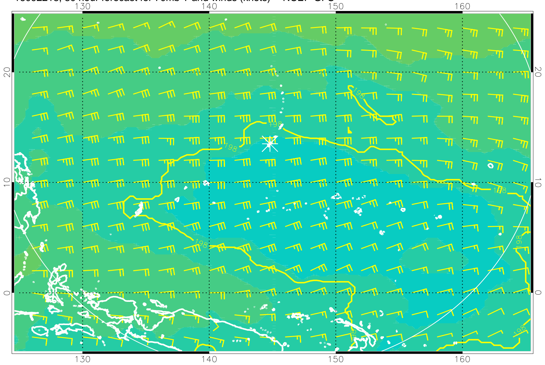
16092218, 30 hour forecast for 70mb T and winds (knots) -- NCEP GFS
