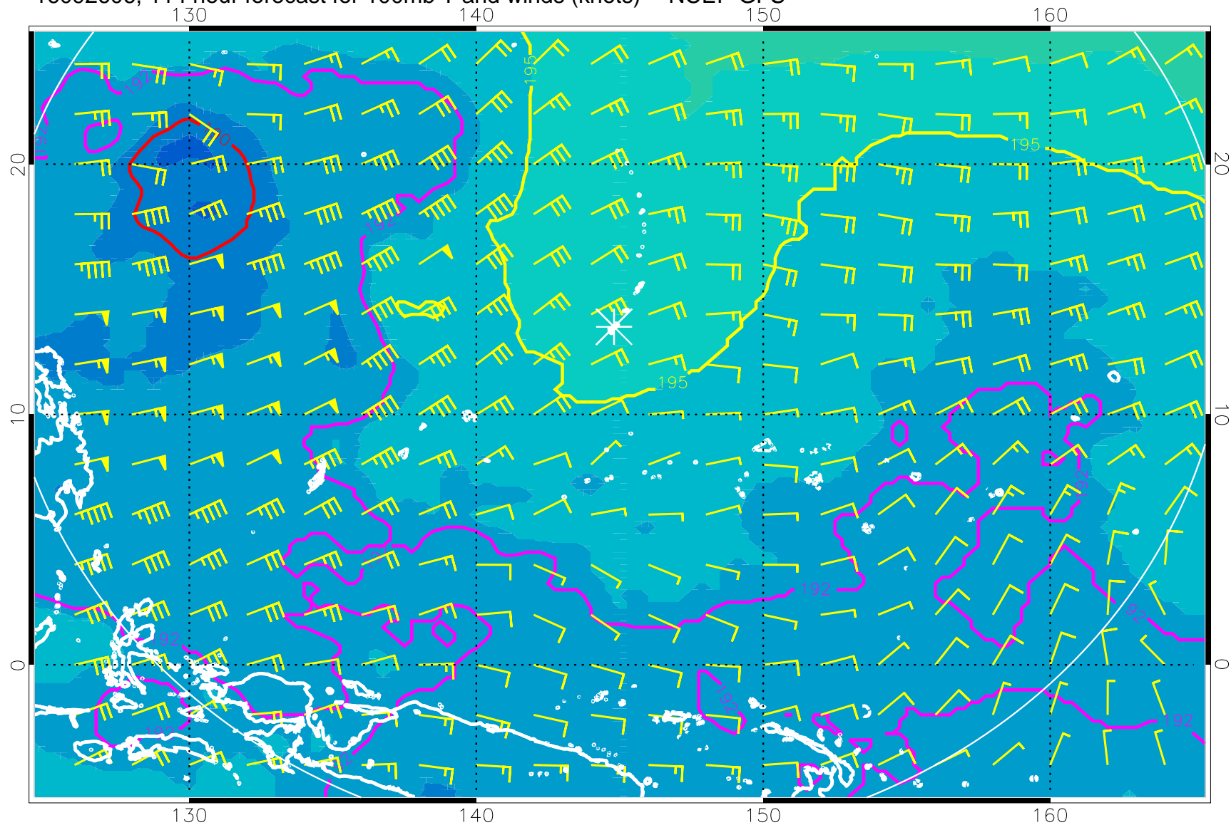
16092606, 114 hour forecast for 100mb T and winds (knots) -- NCEP GFS
