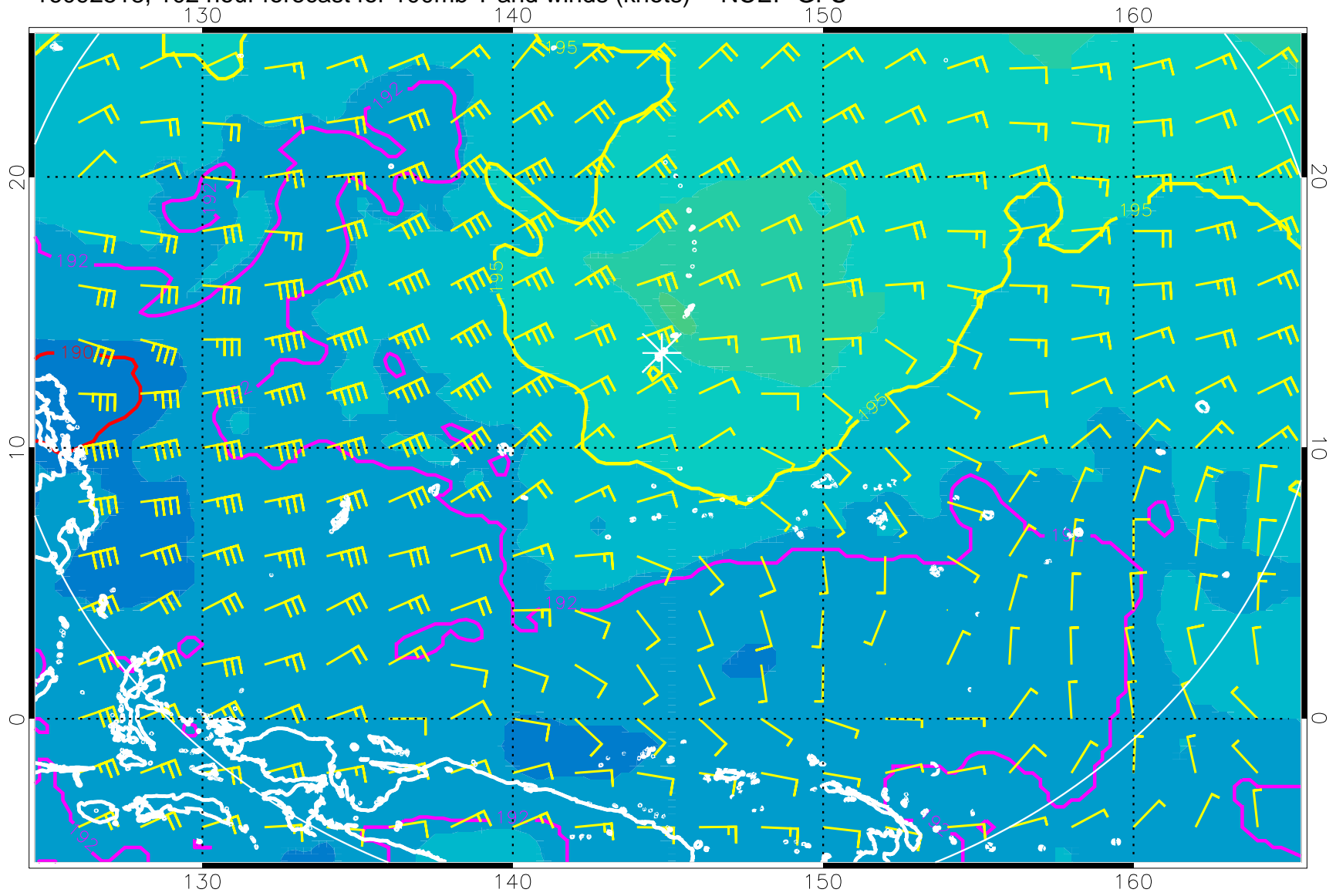
16092518, 102 hour forecast for 100mb T and winds (knots) -- NCEP GFS
