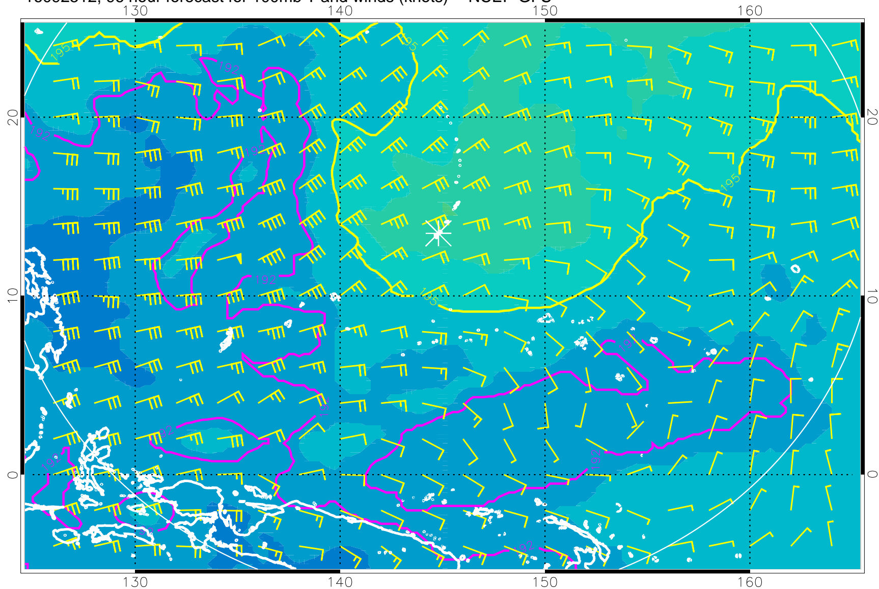
16092512, 96 hour forecast for 100mb T and winds (knots) -- NCEP GFS
