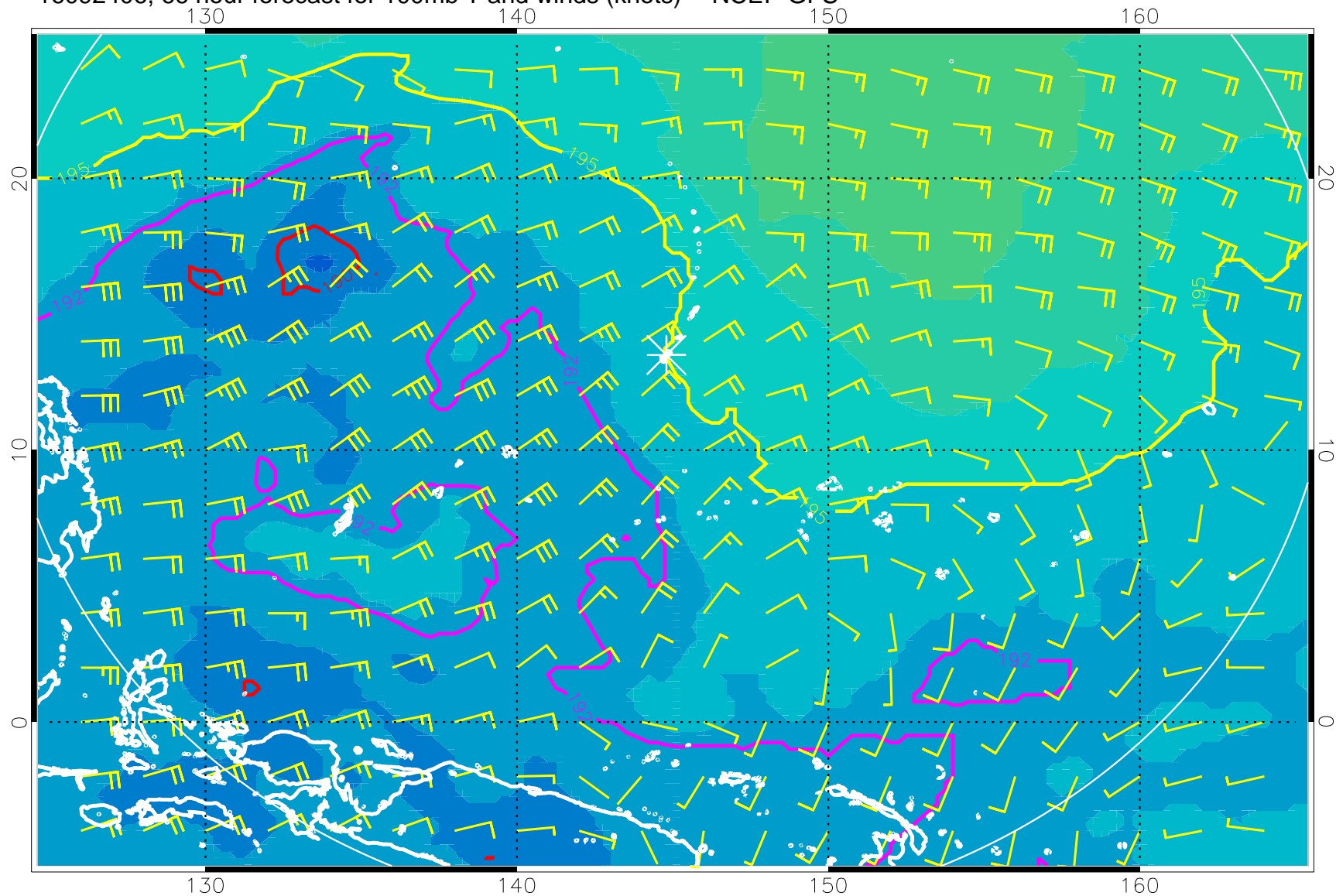
16092406, 66 hour forecast for 100mb T and winds (knots) -- NCEP GFS
