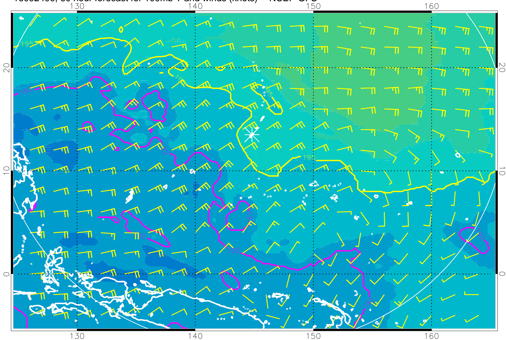
16092400, 60 hour forecast for 100mb T and winds (knots) -- NCEP GFS
