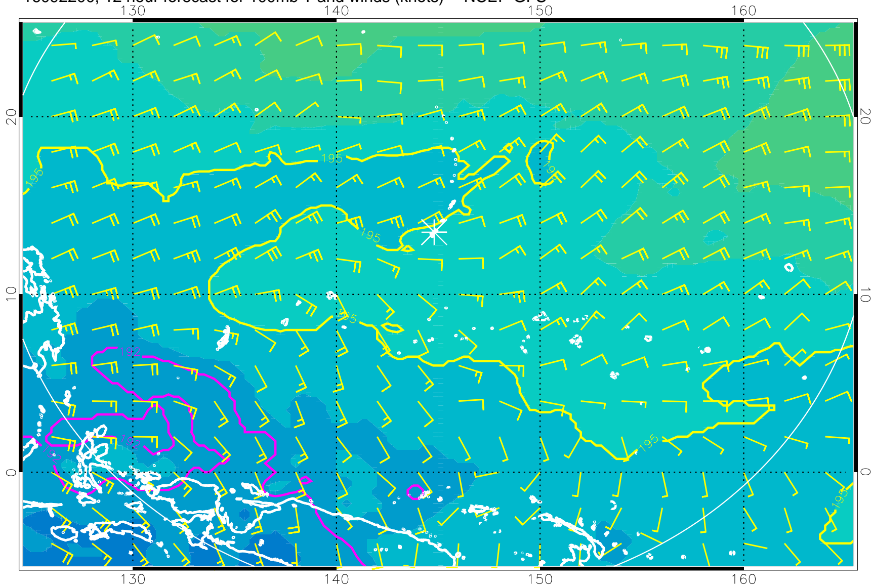
16092200, 12 hour forecast for 100mb T and winds (knots) -- NCEP GFS
