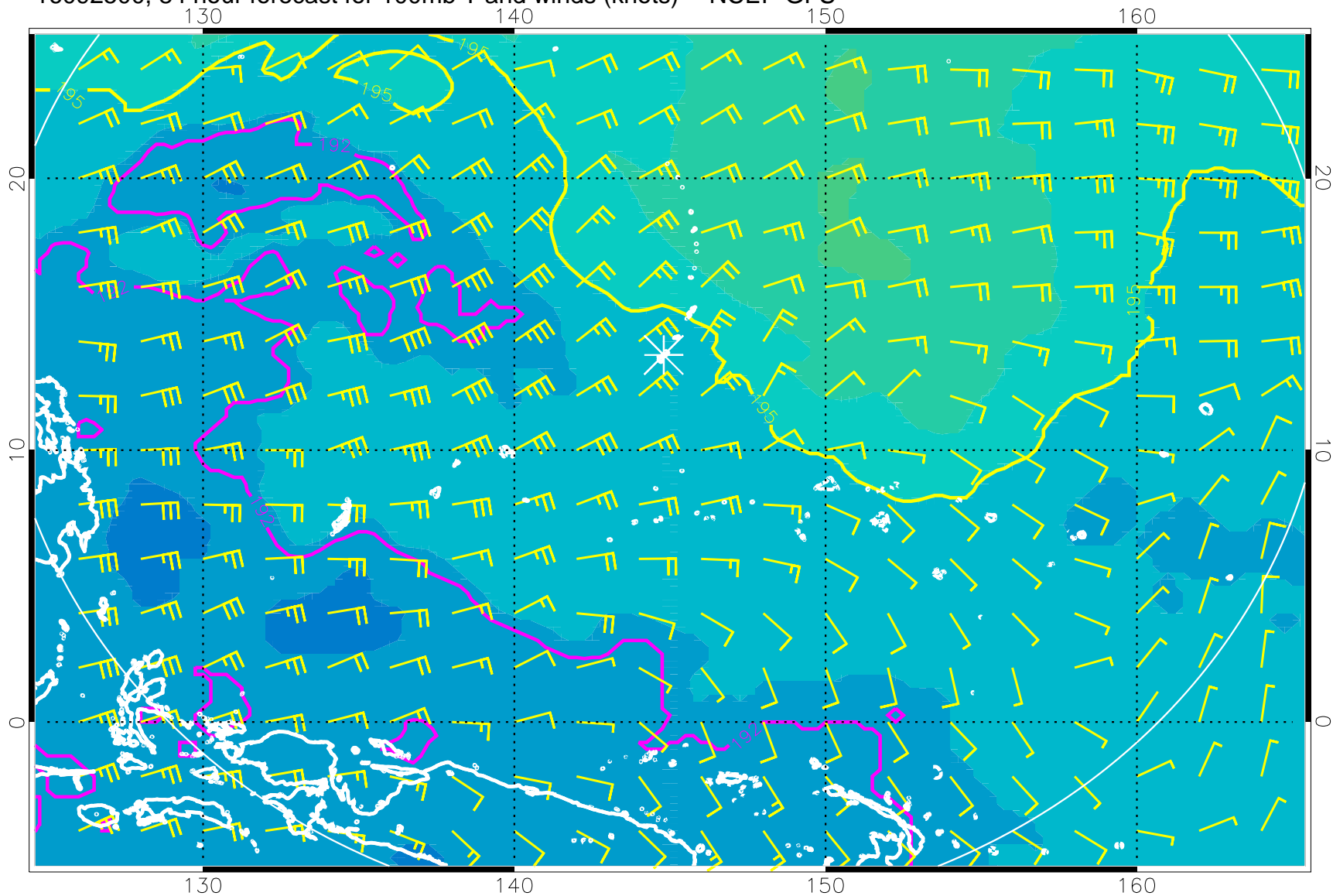
16092500, 84 hour forecast for 100mb T and winds (knots) -- NCEP GFS
