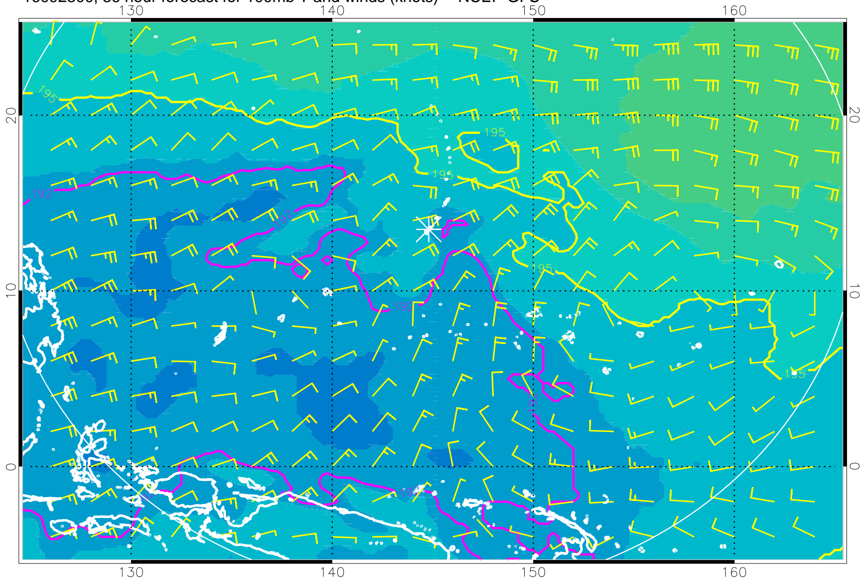
16092300, 36 hour forecast for 100mb T and winds (knots) -- NCEP GFS
