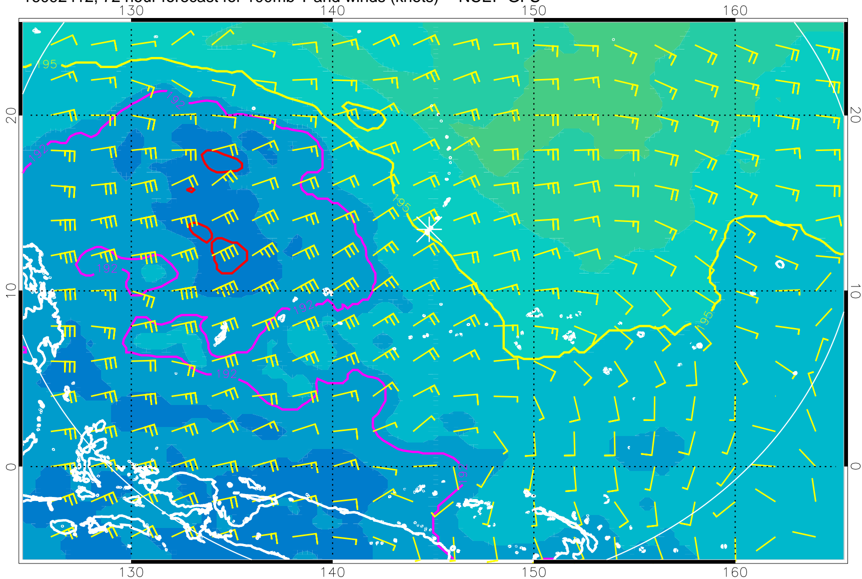
16092412, 72 hour forecast for 100mb T and winds (knots) -- NCEP GFS
