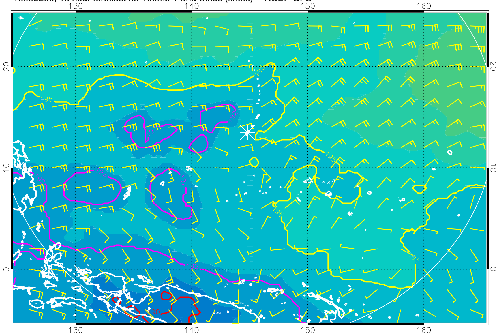
16092206, 18 hour forecast for 100mb T and winds (knots) -- NCEP GFS
