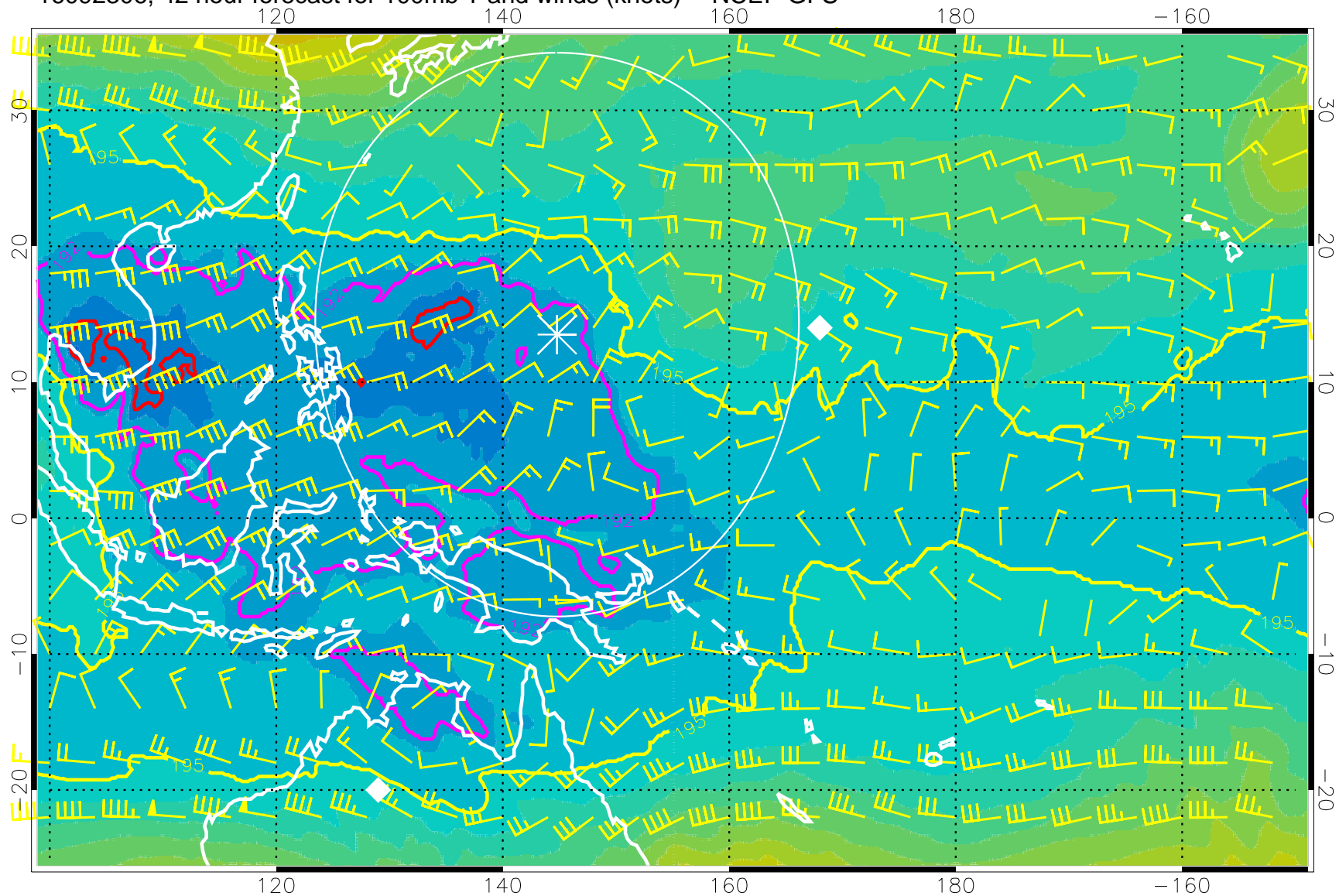
16092306, 42 hour forecast for 100mb T and winds (knots) -- NCEP GFS
