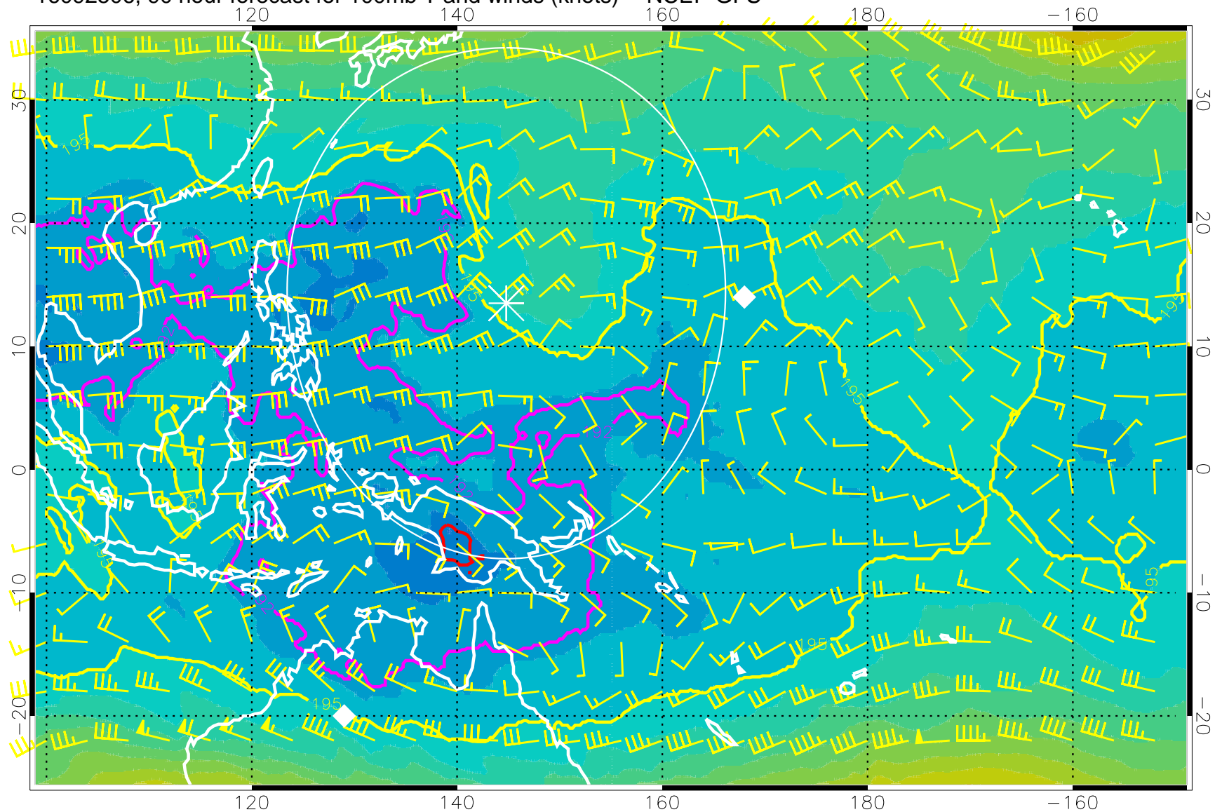
16092506, 90 hour forecast for 100mb T and winds (knots) -- NCEP GFS
