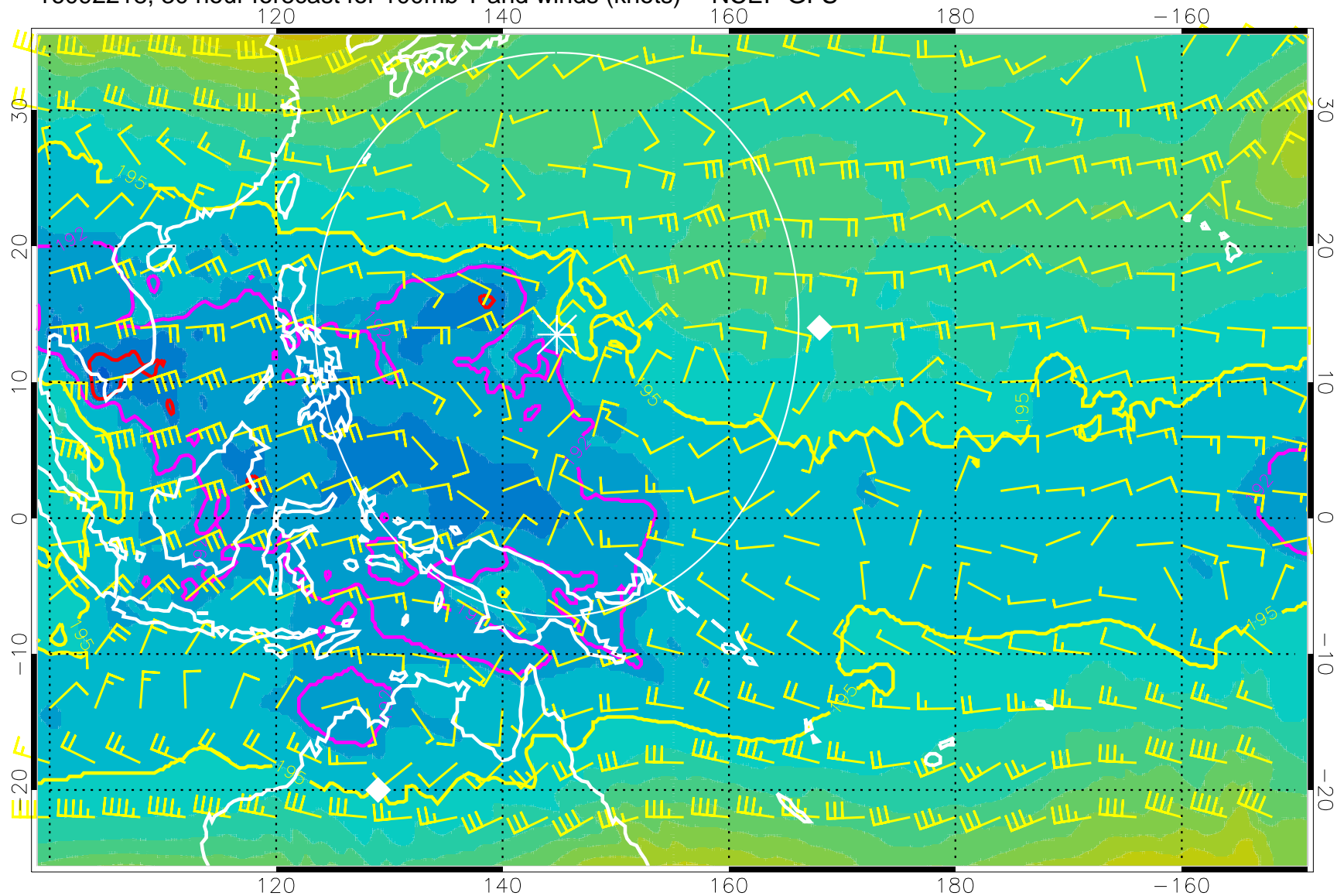
16092218, 30 hour forecast for 100mb T and winds (knots) -- NCEP GFS
