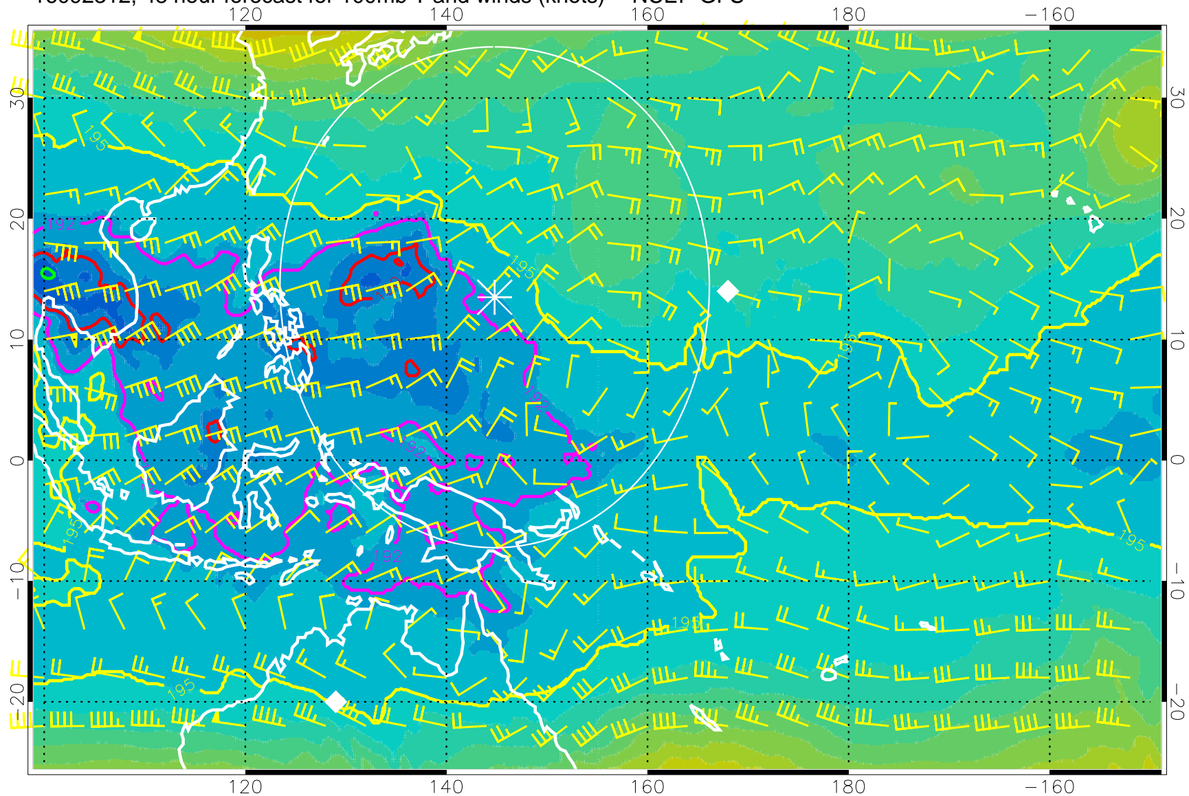
16092312, 48 hour forecast for 100mb T and winds (knots) -- NCEP GFS
