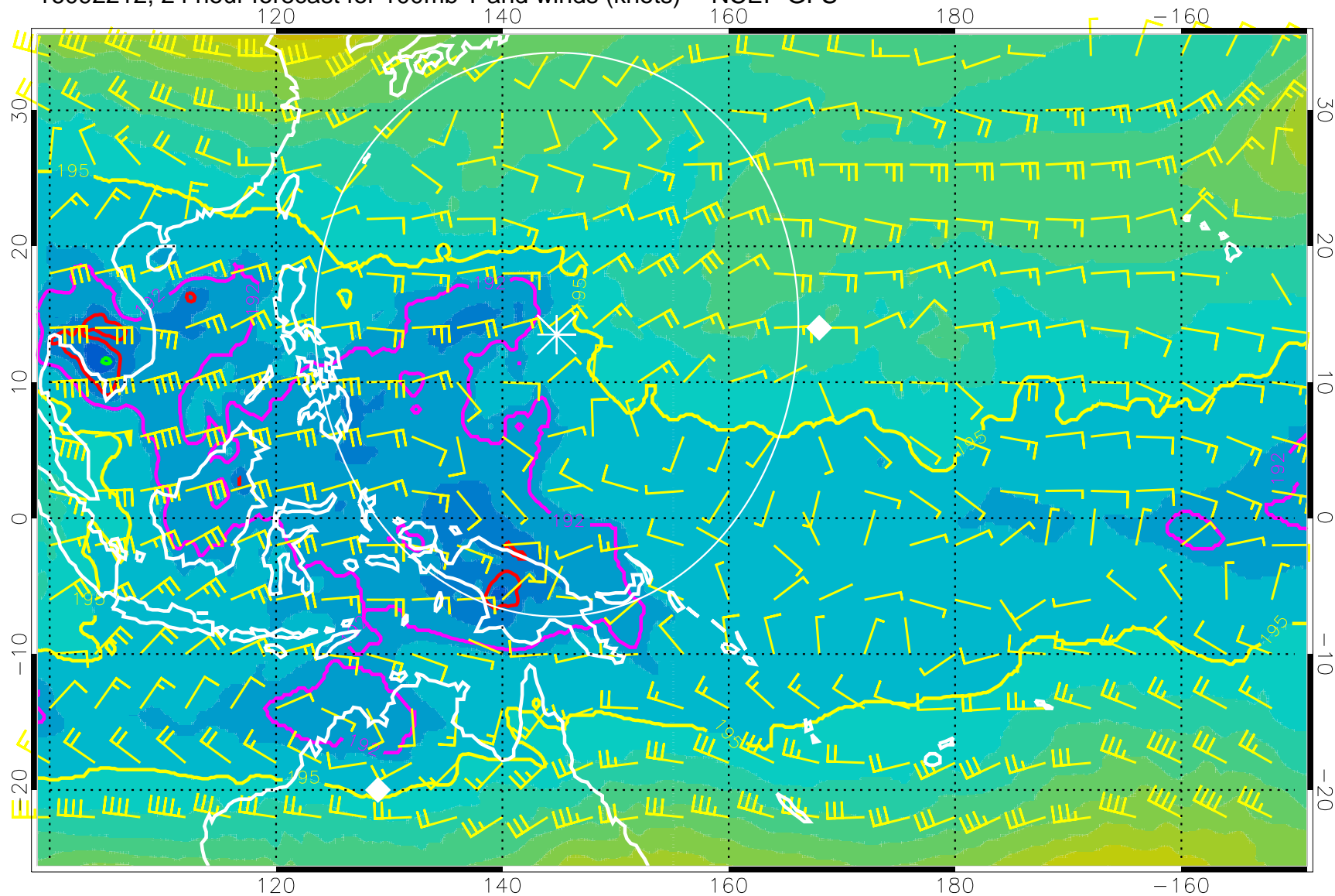
16092212, 24 hour forecast for 100mb T and winds (knots) -- NCEP GFS
