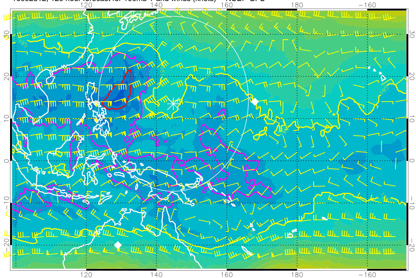
16092612, 120 hour forecast for 100mb T and winds (knots) -- NCEP GFS
