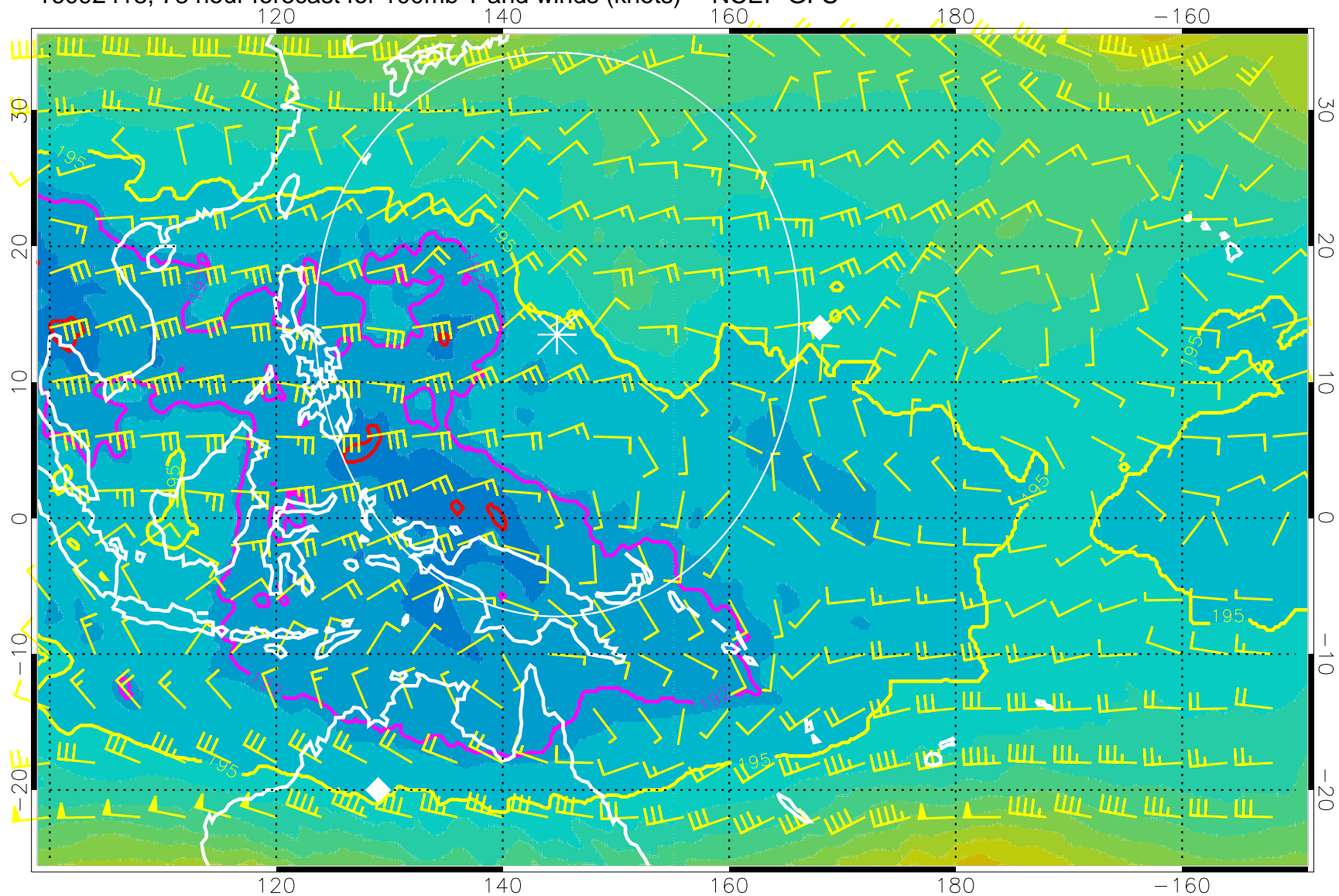
16092418, 78 hour forecast for 100mb T and winds (knots) -- NCEP GFS
