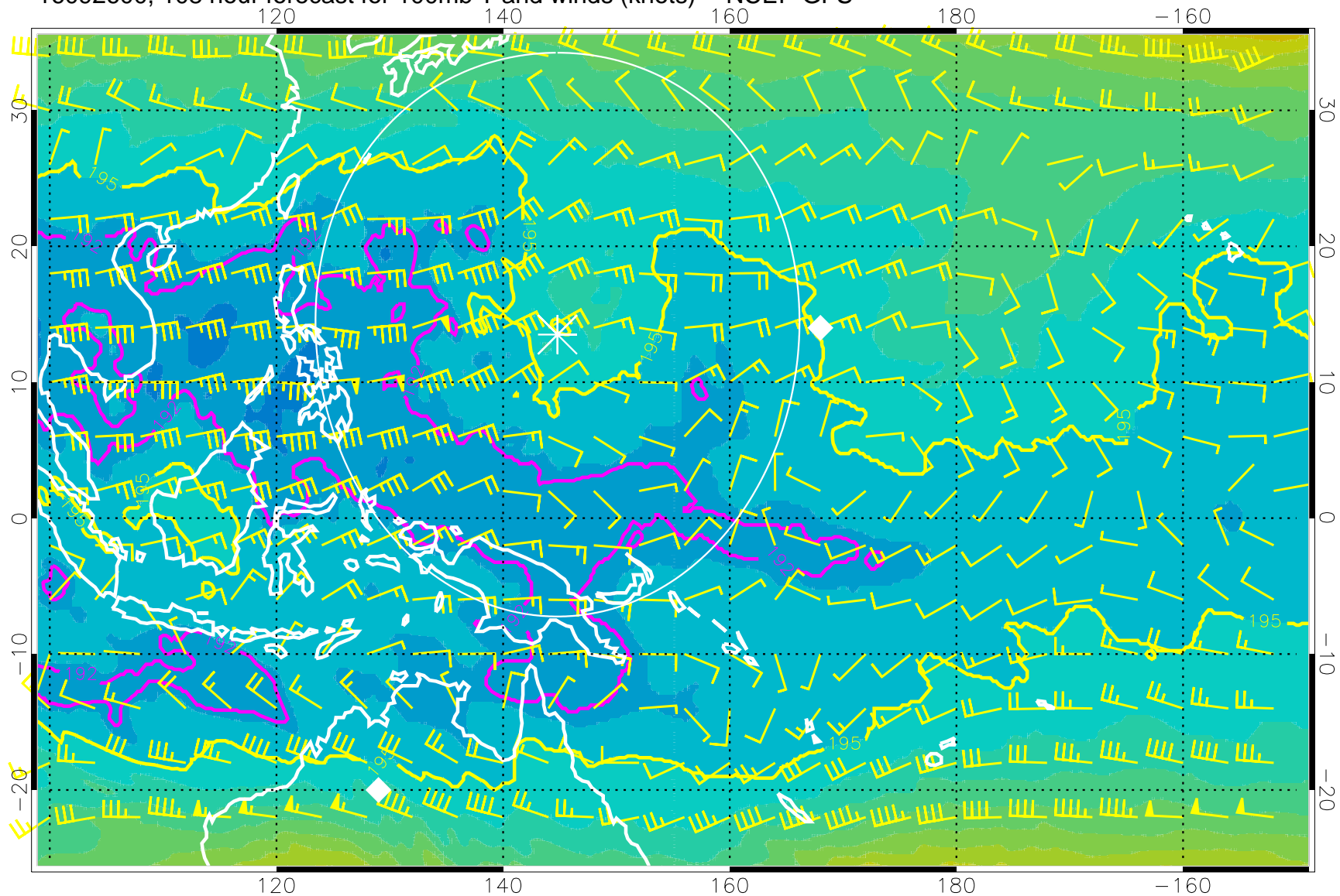
16092600, 108 hour forecast for 100mb T and winds (knots) -- NCEP GFS
