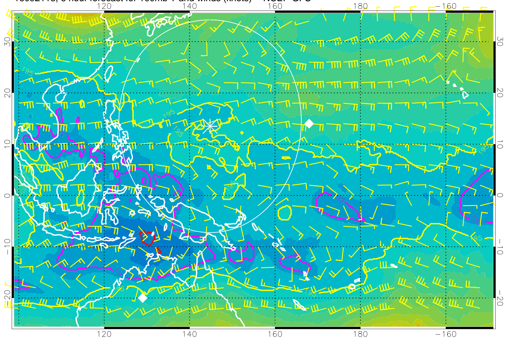
16092118, 6 hour forecast for 100mb T and winds (knots) -- NCEP GFS
