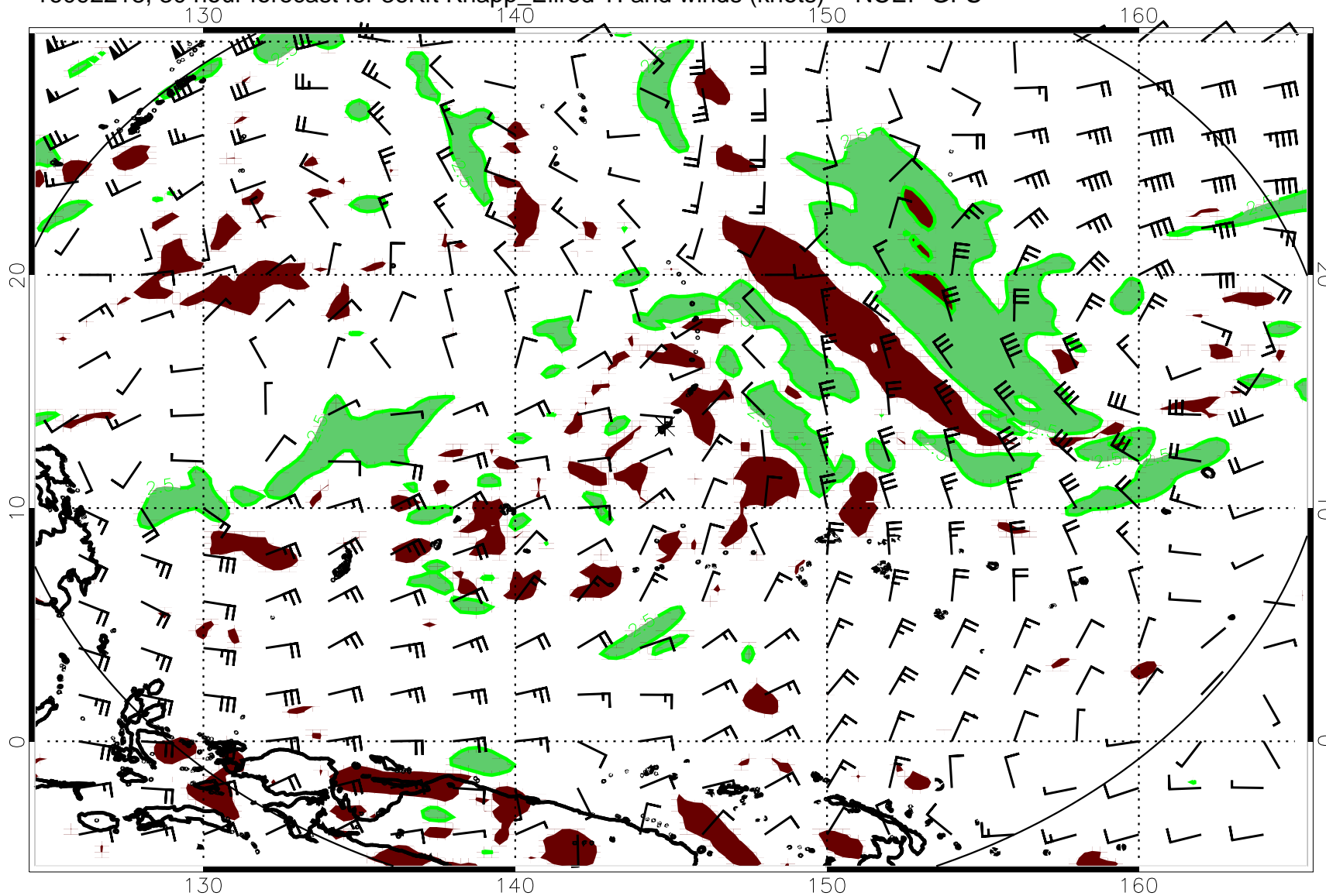
16092218, 30 hour forecast for 36Kft Knapp_Ellrod TI and winds (knots) -- NCEP GFS
