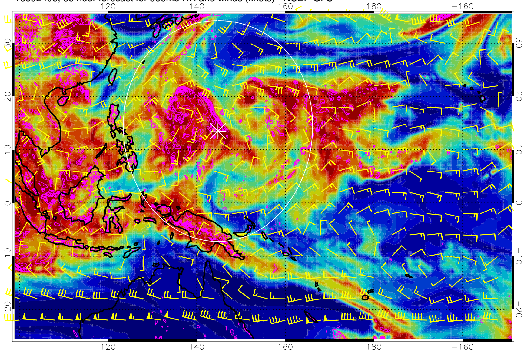
16092406, 66 hour forecast for 500mb RH and winds (knots) - NCEP GFS
