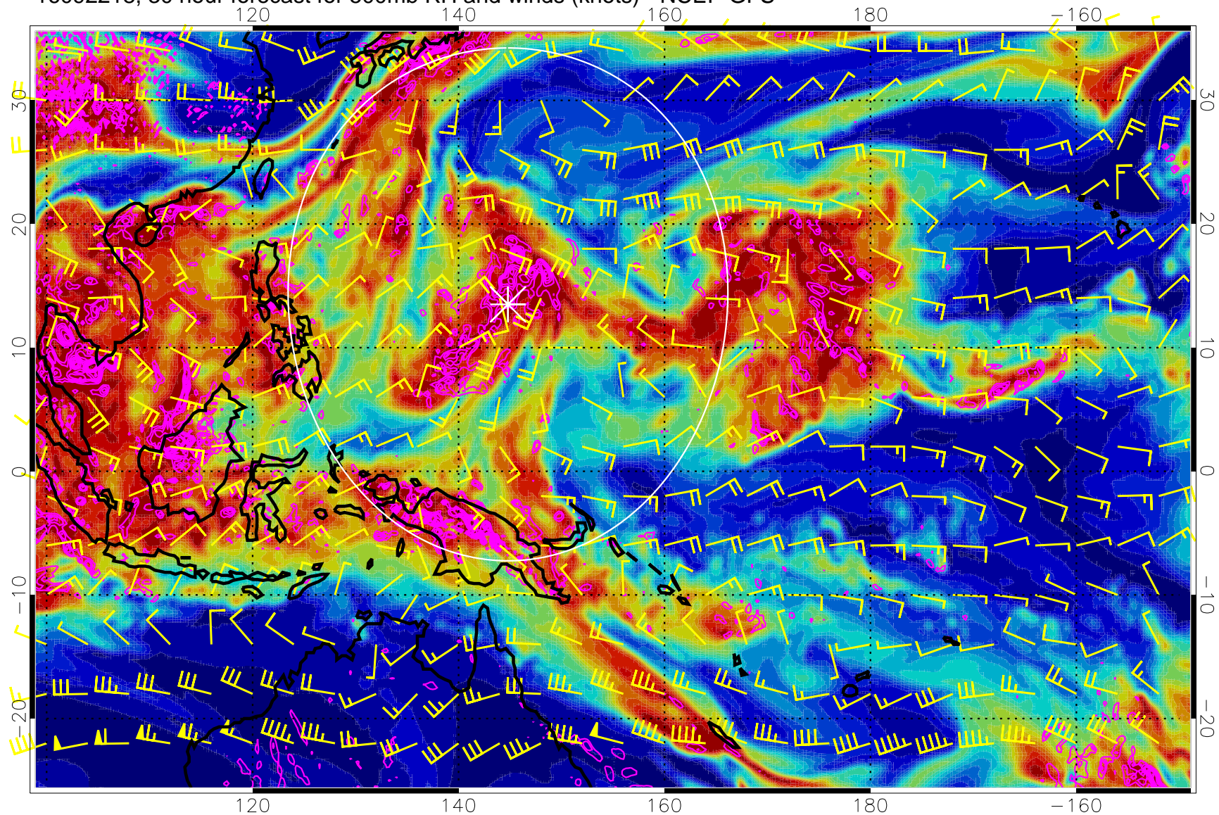
16092218, 30 hour forecast for 500mb RH and winds (knots) - NCEP GFS
