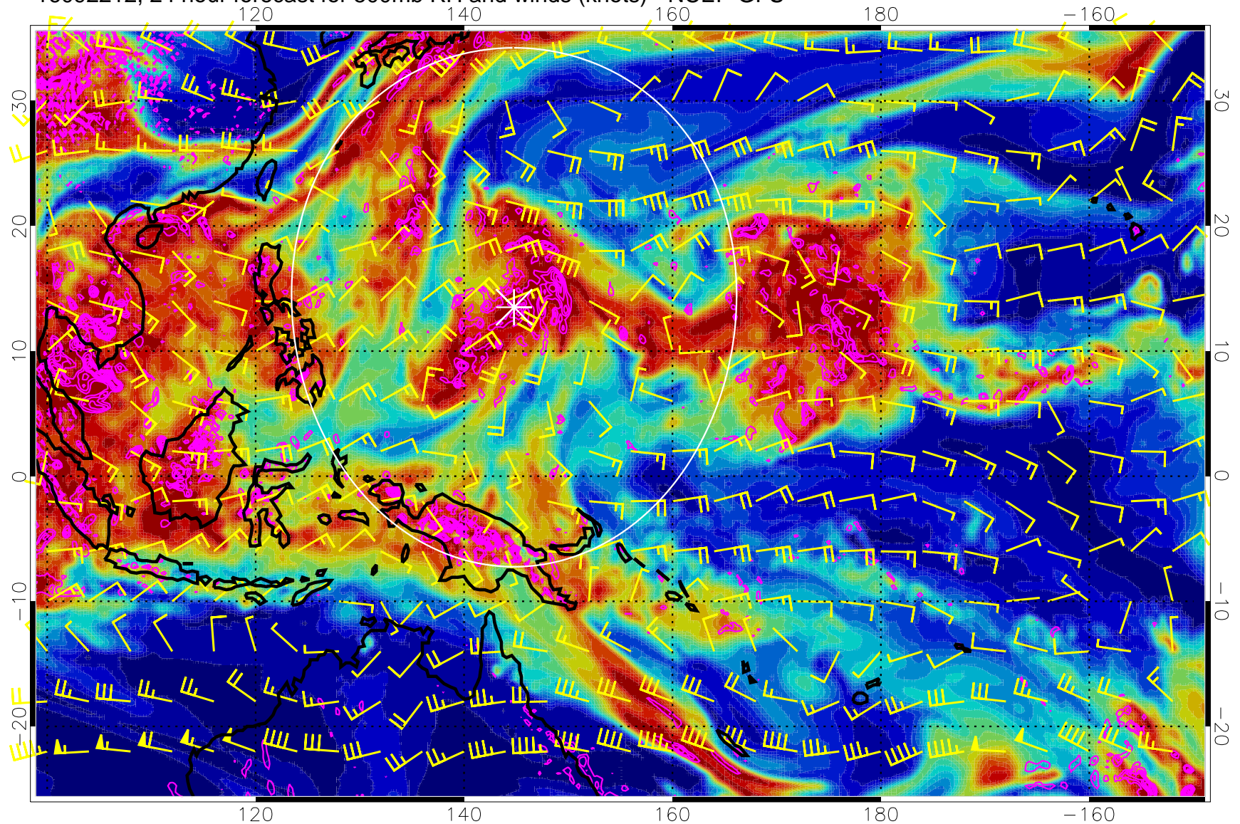
16092212, 24 hour forecast for 500mb RH and winds (knots) - NCEP GFS
