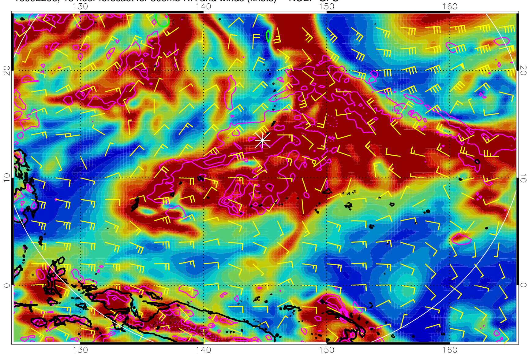
16092206, 18 hour forecast for 300mb RH and winds (knots) -- NCEP GFS
