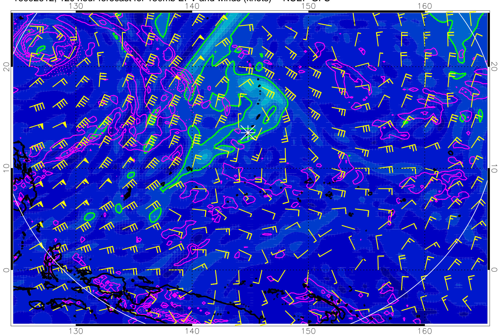
16092612, 120 hour forecast for 150mb EPV and winds (knots) -- NCEP GFS
