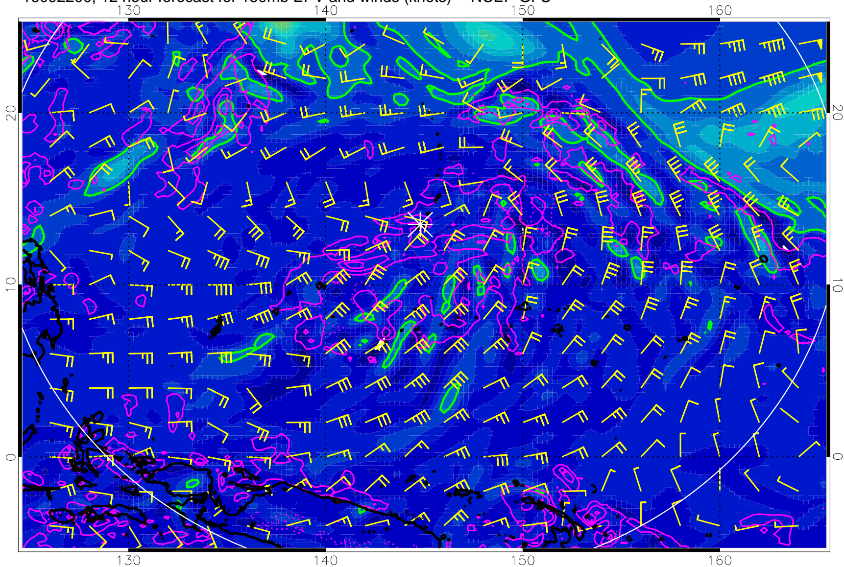
16092200, 12 hour forecast for 150mb EPV and winds (knots) -- NCEP GFS
