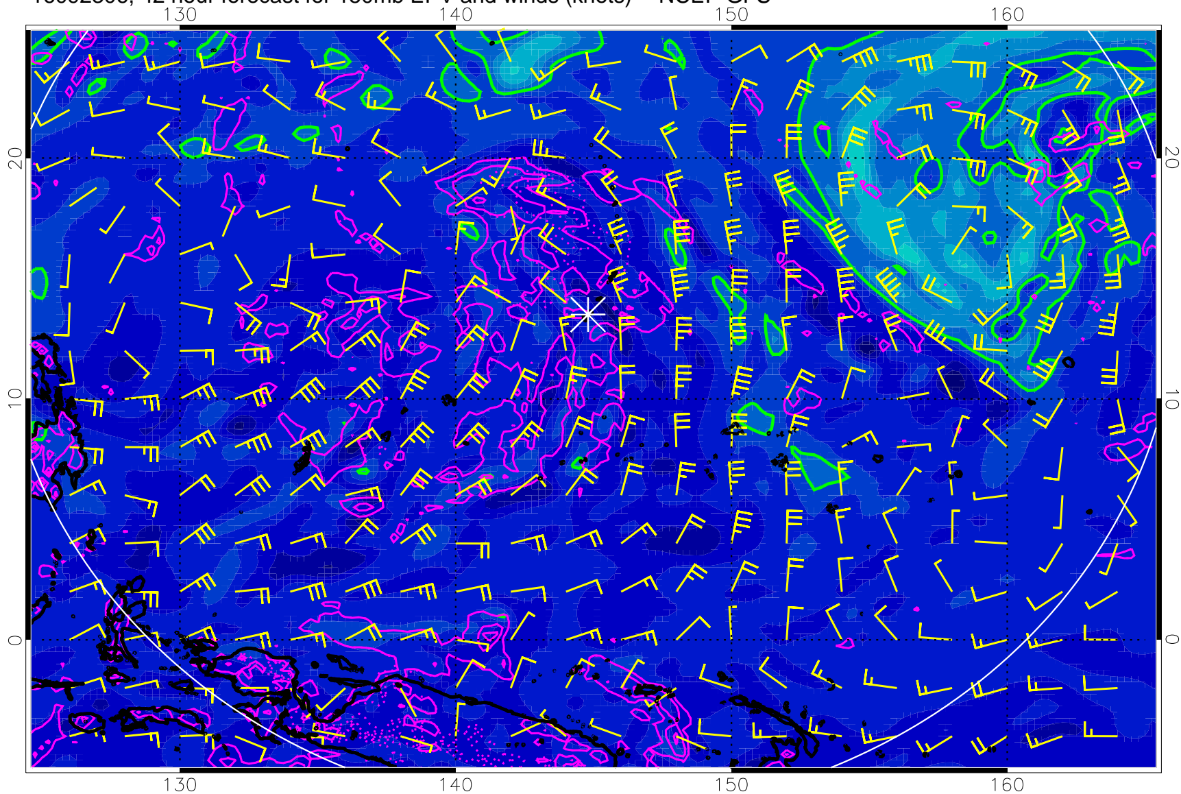
16092306, 42 hour forecast for 150mb EPV and winds (knots) -- NCEP GFS
