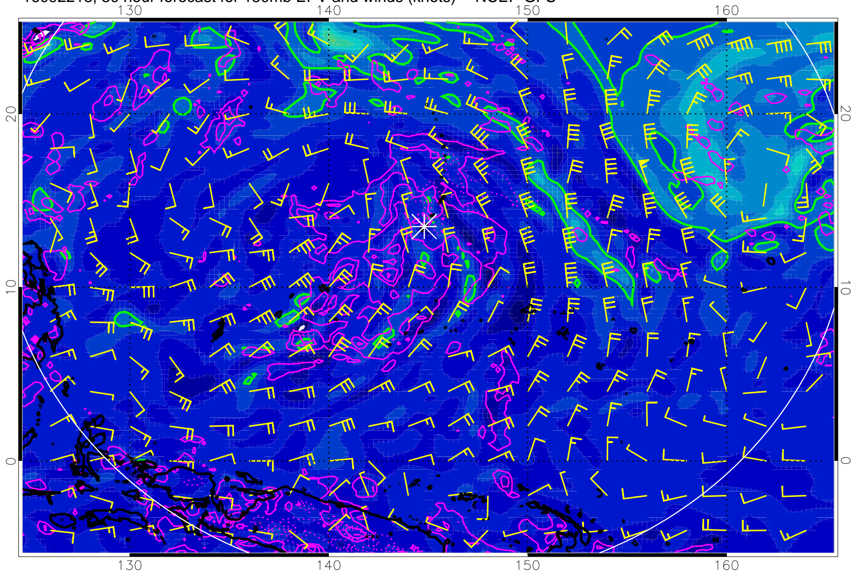
16092218, 30 hour forecast for 150mb EPV and winds (knots) -- NCEP GFS
