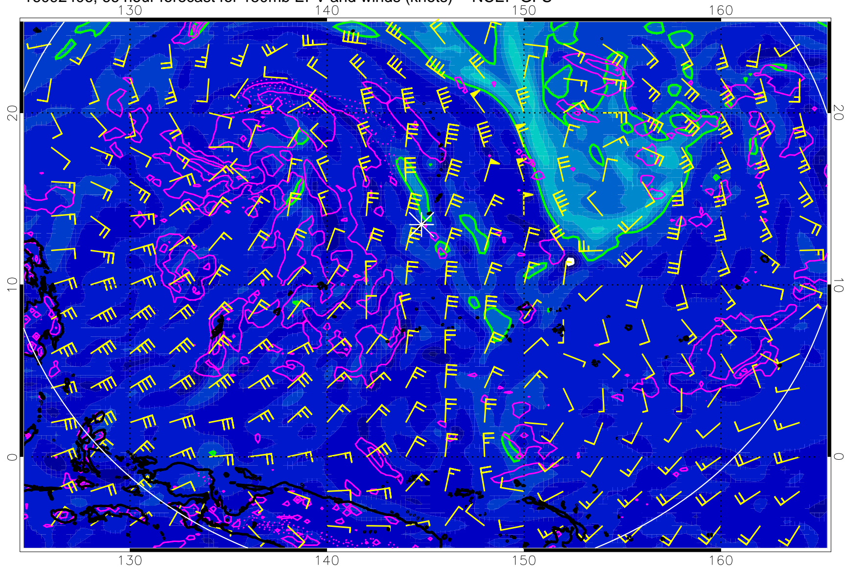
16092406, 66 hour forecast for 150mb EPV and winds (knots) -- NCEP GFS
