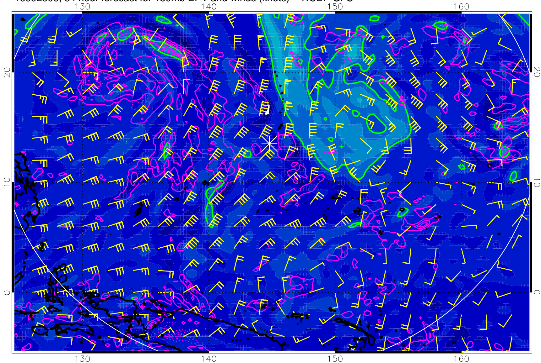
16092500, 84 hour forecast for 150mb EPV and winds (knots) -- NCEP GFS
