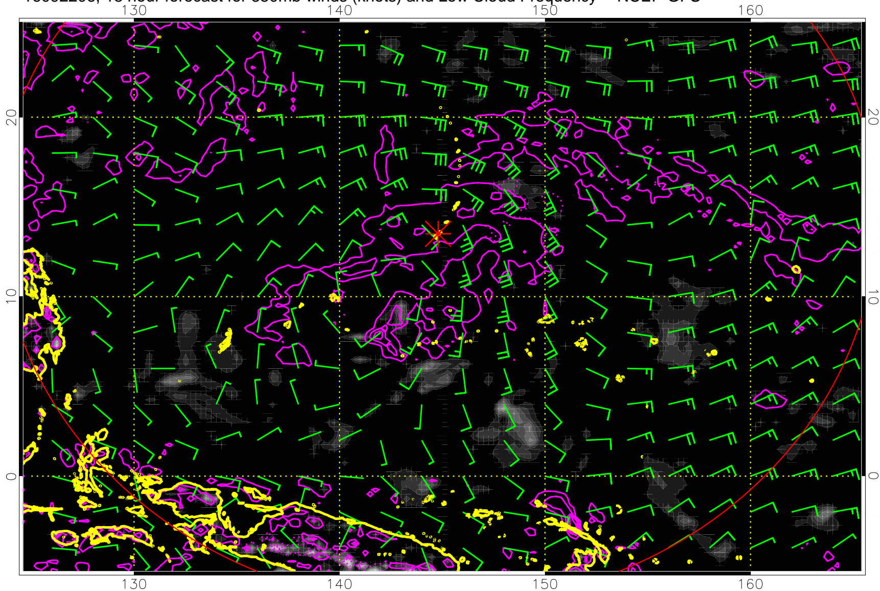
16092206, 18 hour forecast for 850mb winds (knots) and Low Cloud Frequency -- NCEP GFS
