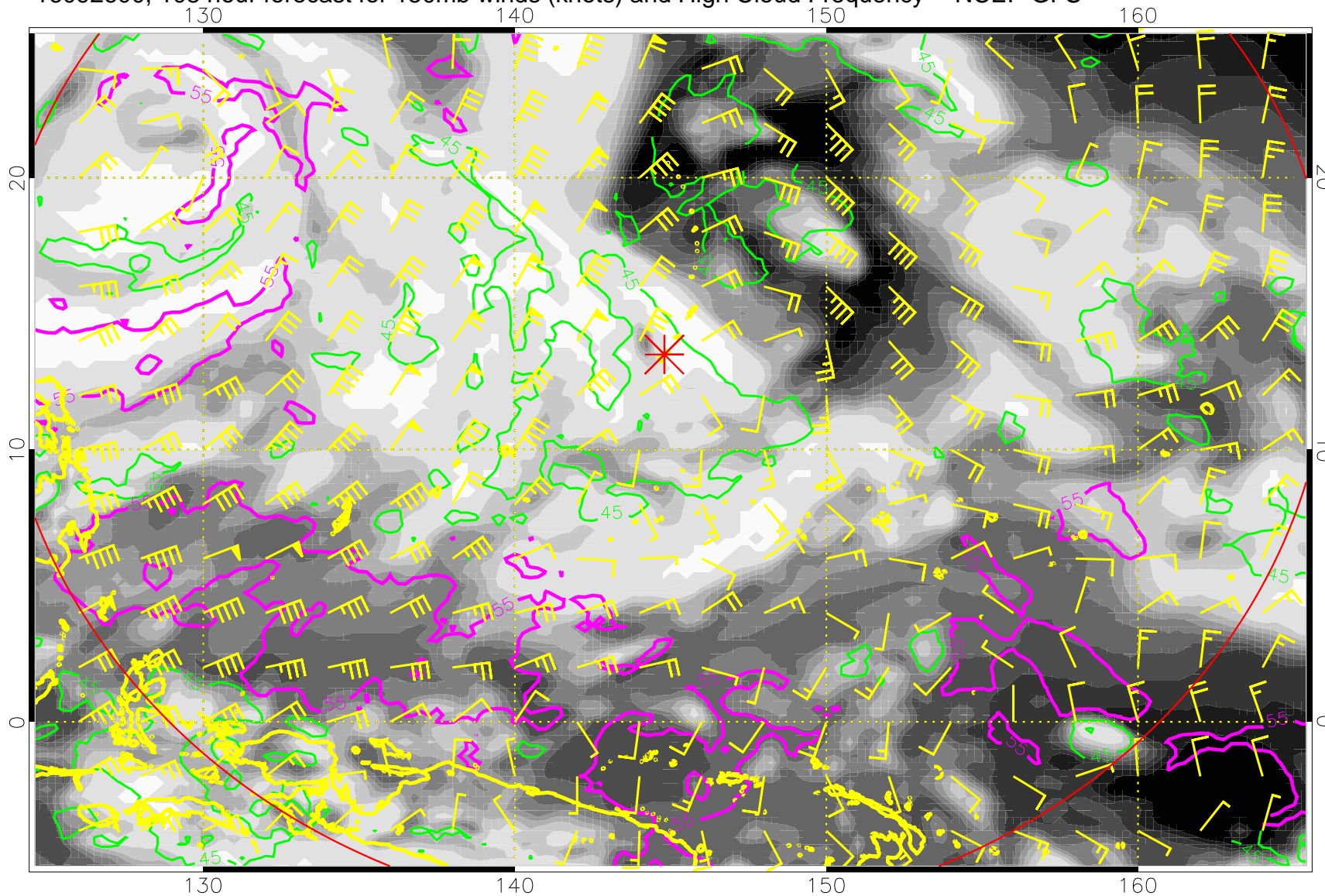
16092600, 108 hour forecast for 150mb winds (knots) and High Cloud Frequency -- NCEP GFS
