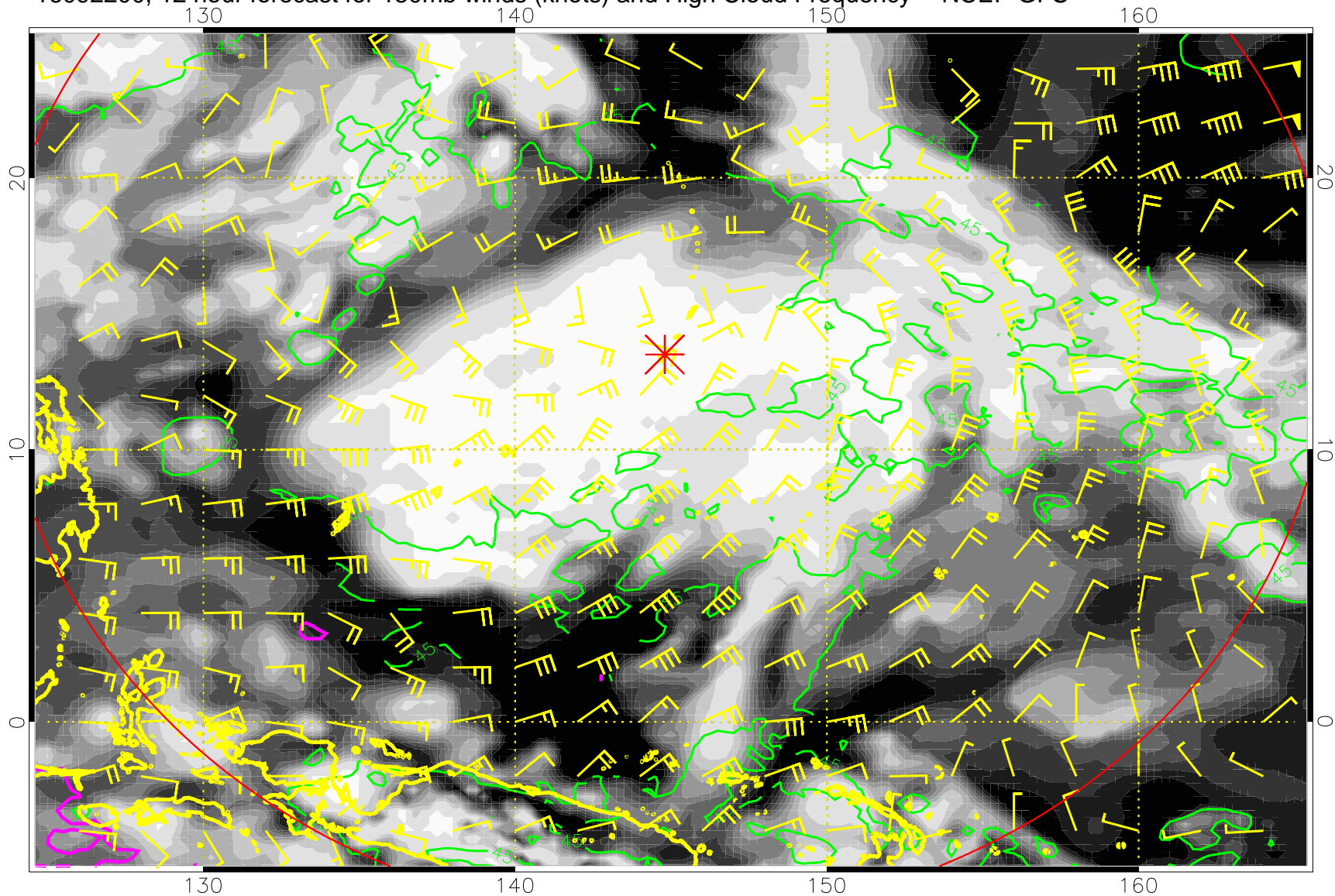
16092200, 12 hour forecast for 150mb winds (knots) and High Cloud Frequency -- NCEP GFS
