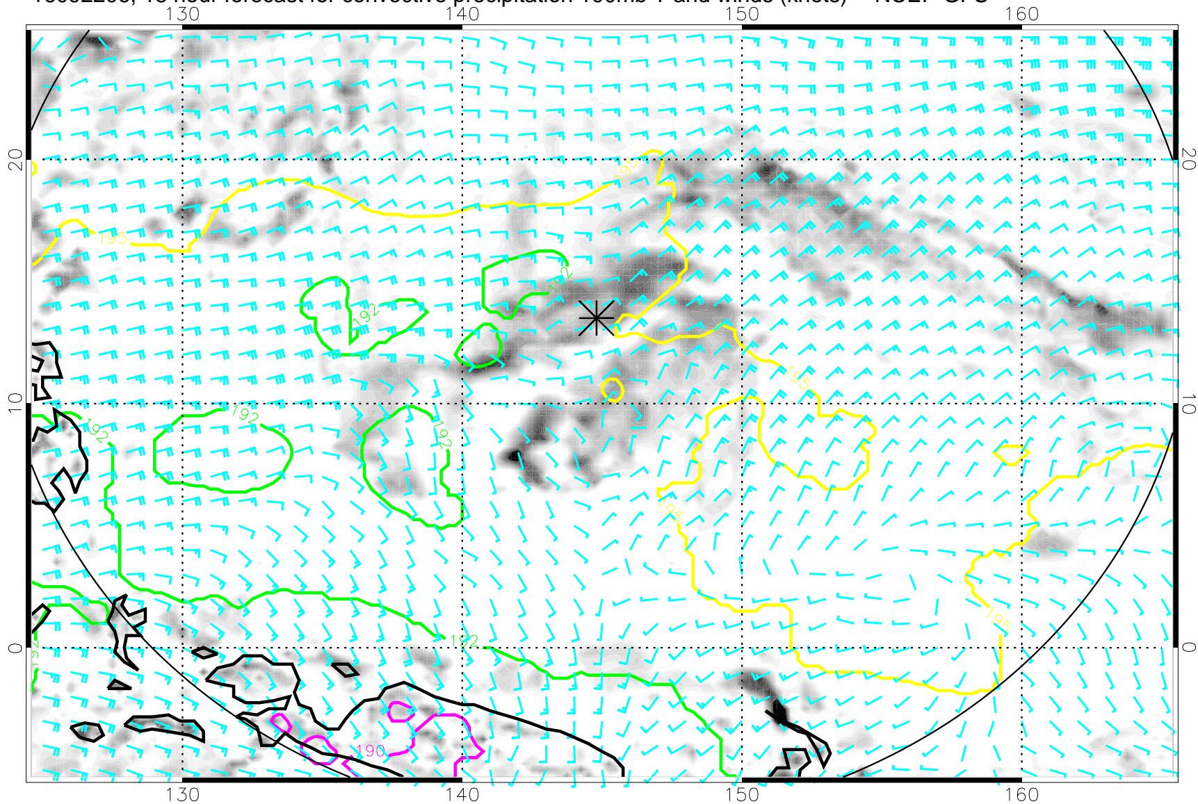
16092206, 18 hour forecast for convective precipitation 100mb T and winds (knots) -- NCEP GFS
