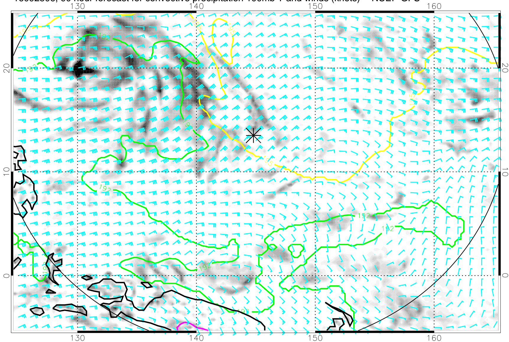
16092506, 90 hour forecast for convective precipitation 100mb T and winds (knots) -- NCEP GFS
