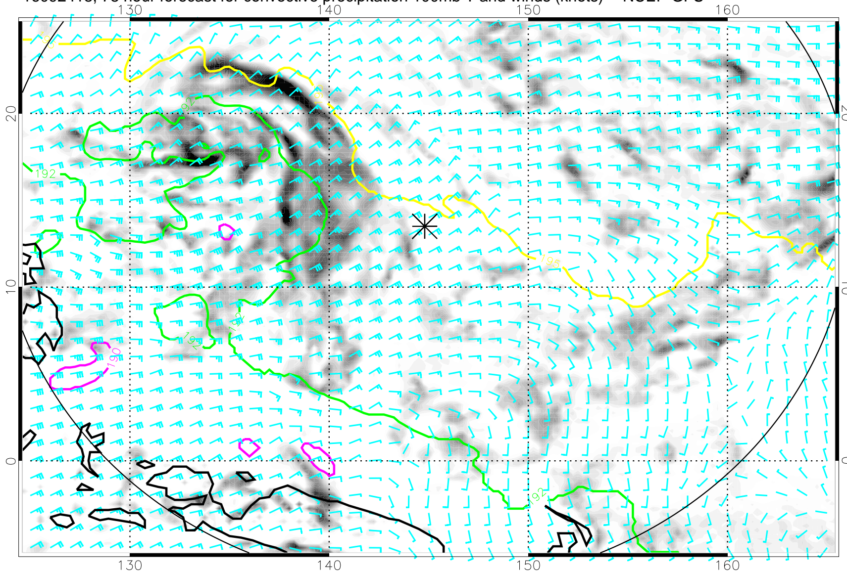
16092418, 78 hour forecast for convective precipitation 100mb T and winds (knots) -- NCEP GFS
