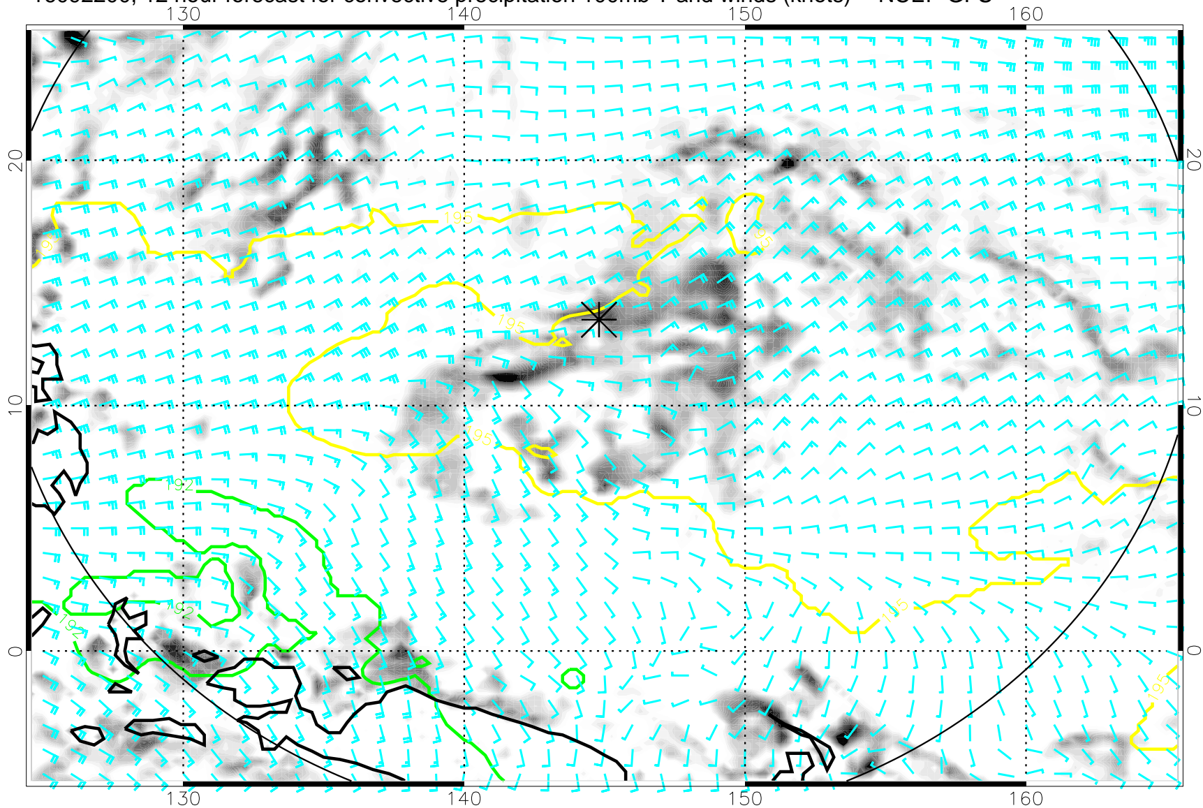
16092200, 12 hour forecast for convective precipitation 100mb T and winds (knots) -- NCEP GFS
