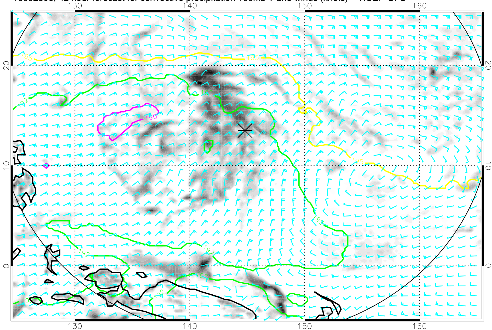
16092306, 42 hour forecast for convective precipitation 100mb T and winds (knots) -- NCEP GFS
