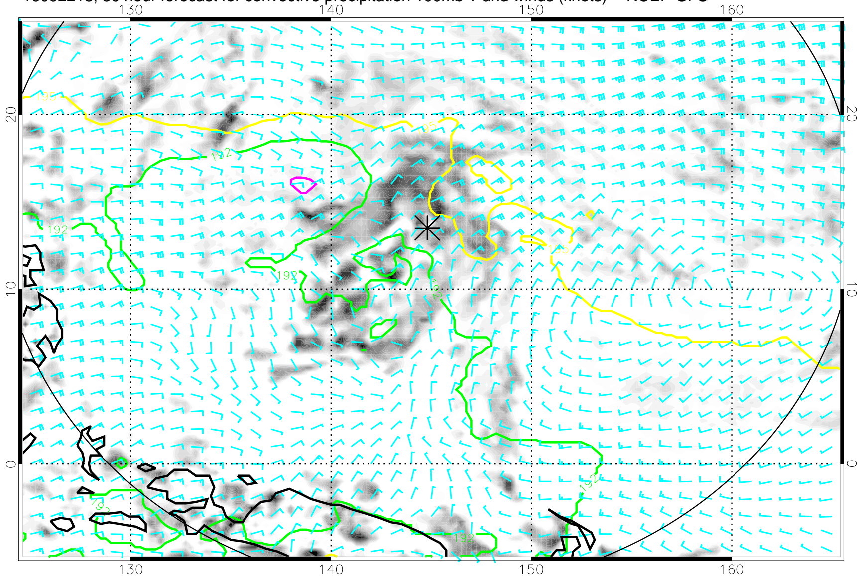
16092218, 30 hour forecast for convective precipitation 100mb T and winds (knots) -- NCEP GFS
