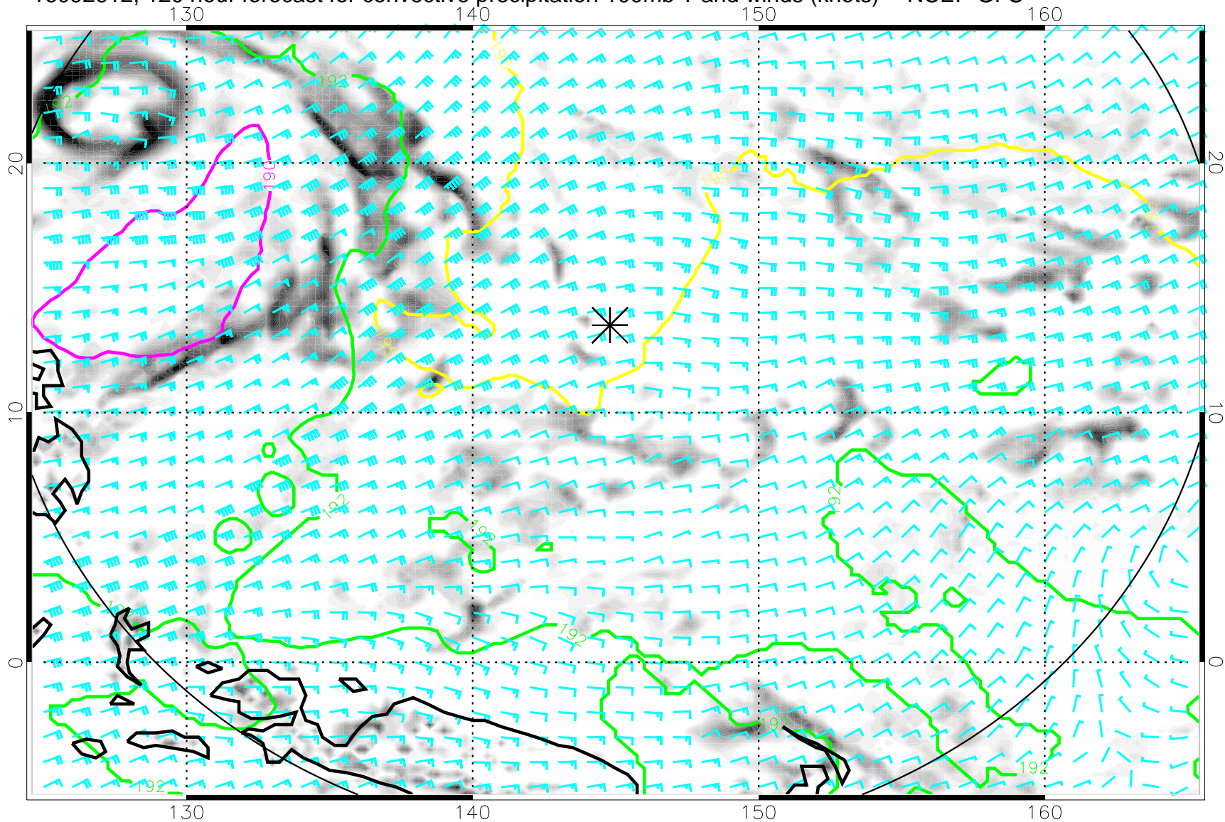
16092612, 120 hour forecast for convective precipitation 100mb T and winds (knots) -- NCEP GFS
