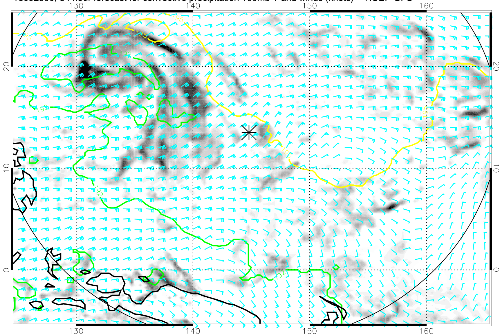
16092500, 84 hour forecast for convective precipitation 100mb T and winds (knots) -- NCEP GFS
