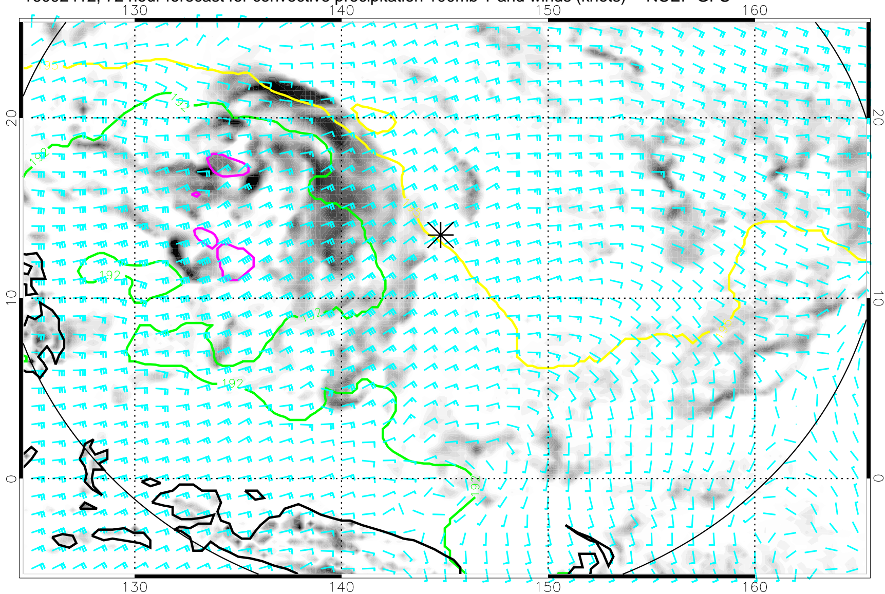
16092412, 72 hour forecast for convective precipitation 100mb T and winds (knots) -- NCEP GFS
