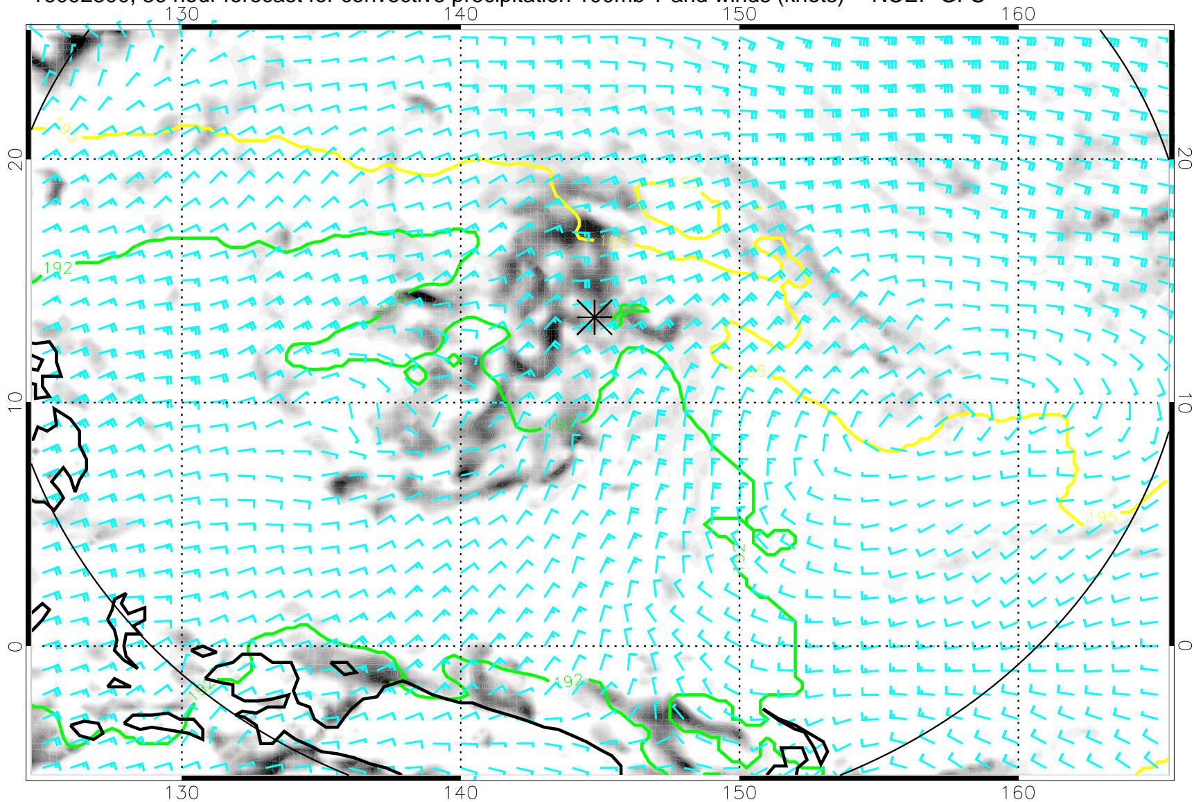
16092300, 36 hour forecast for convective precipitation 100mb T and winds (knots) -- NCEP GFS
