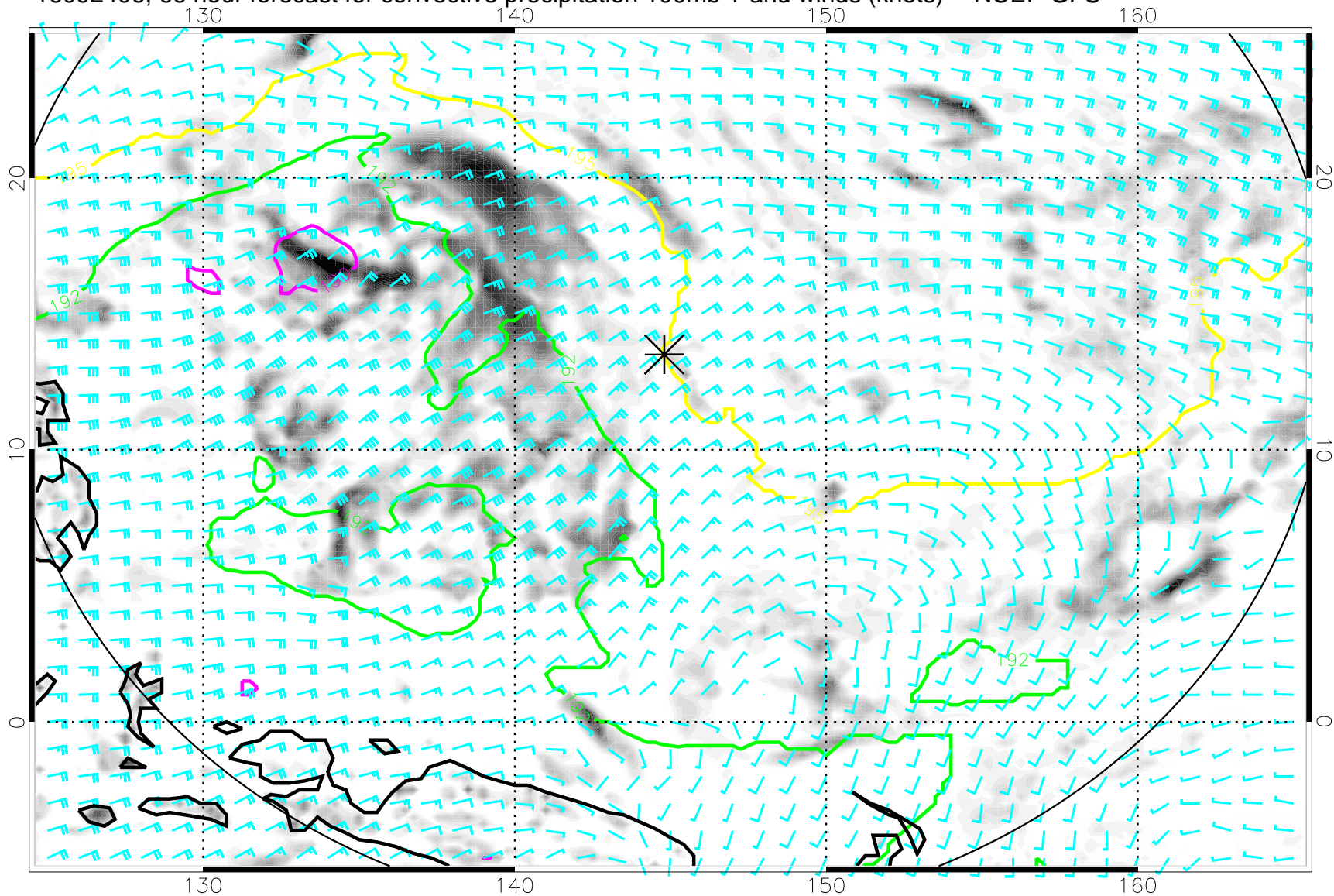
16092406, 66 hour forecast for convective precipitation 100mb T and winds (knots) -- NCEP GFS
