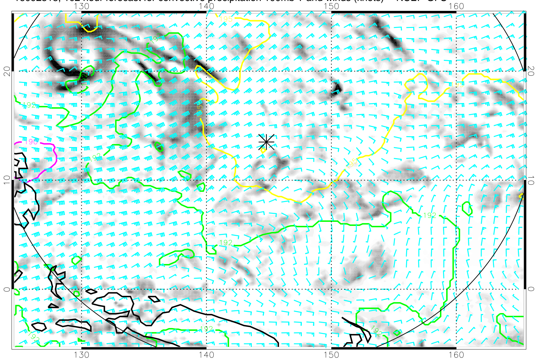
16092518, 102 hour forecast for convective precipitation 100mb T and winds (knots) -- NCEP GFS
