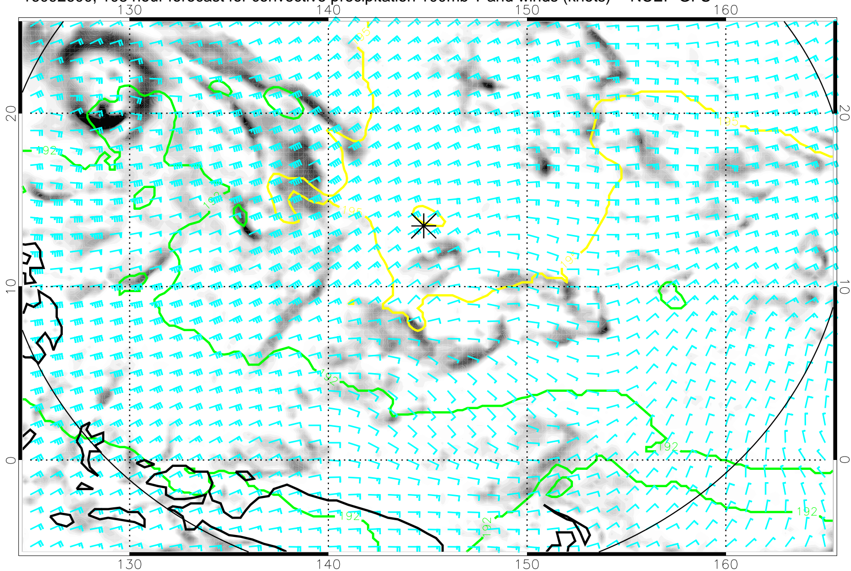
16092600, 108 hour forecast for convective precipitation 100mb T and winds (knots) -- NCEP GFS
