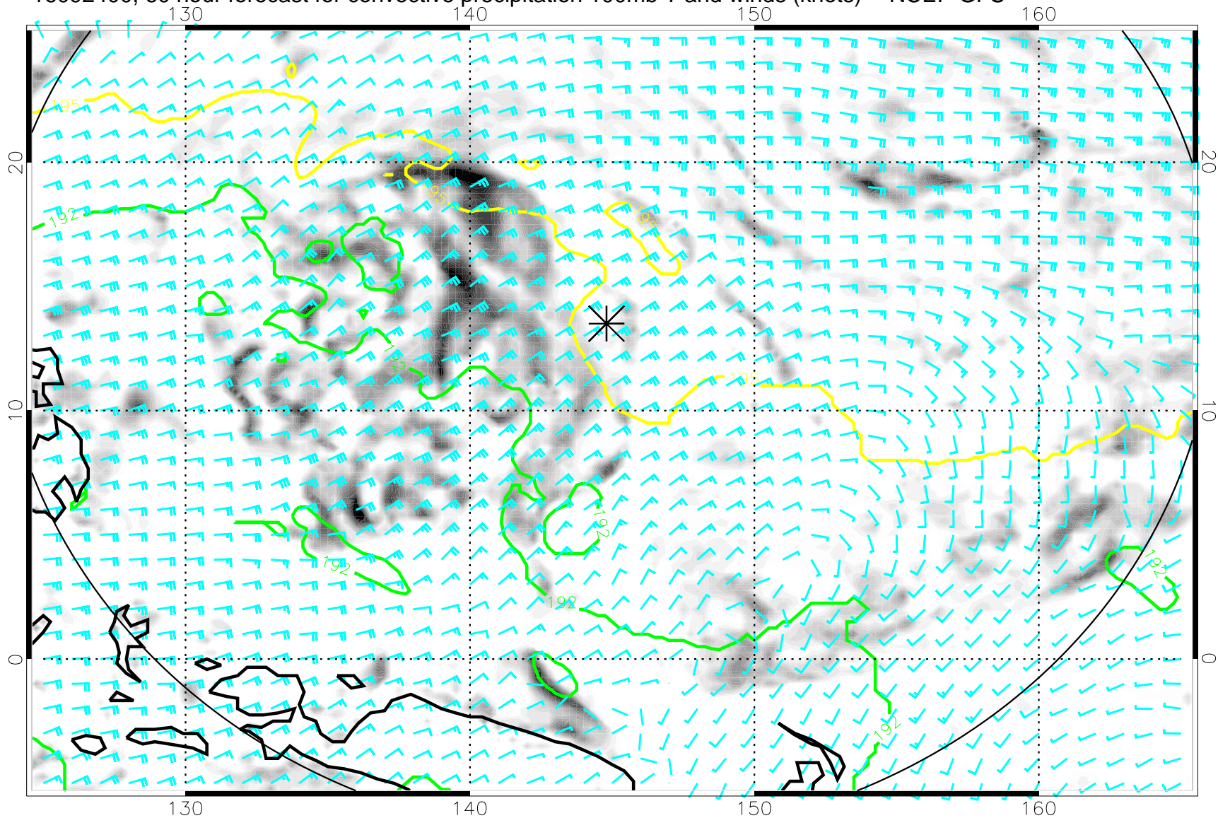
16092400, 60 hour forecast for convective precipitation 100mb T and winds (knots) -- NCEP GFS
