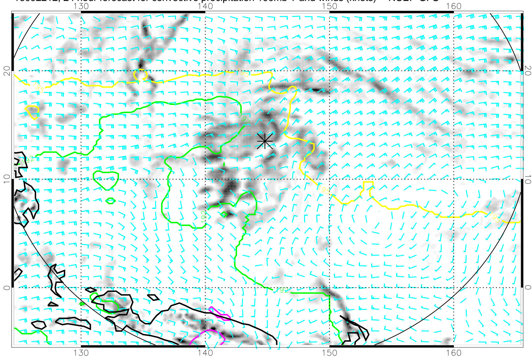
16092212, 24 hour forecast for convective precipitation 100mb T and winds (knots) -- NCEP GFS
