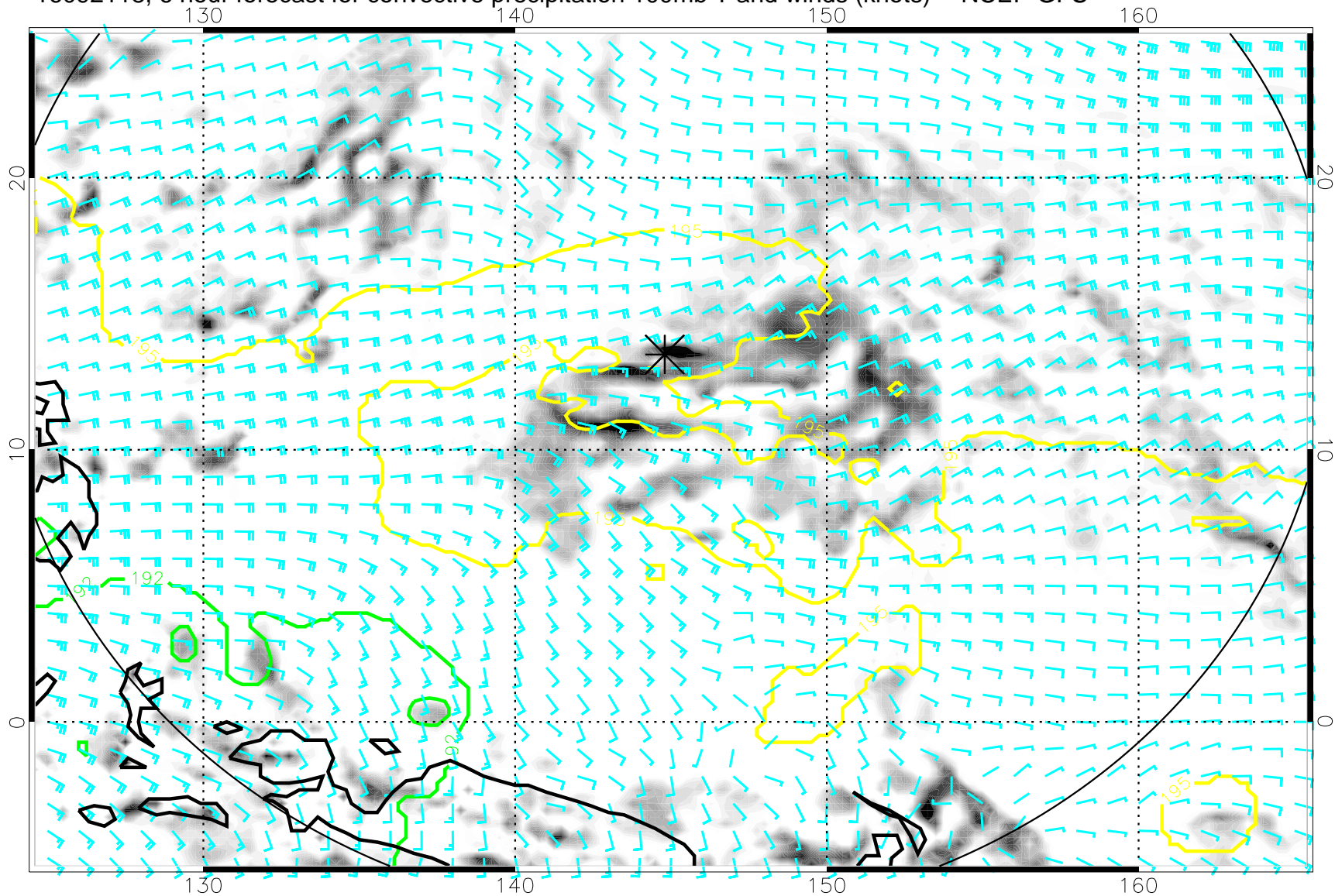
16092118, 6 hour forecast for convective precipitation 100mb T and winds (knots) -- NCEP GFS
