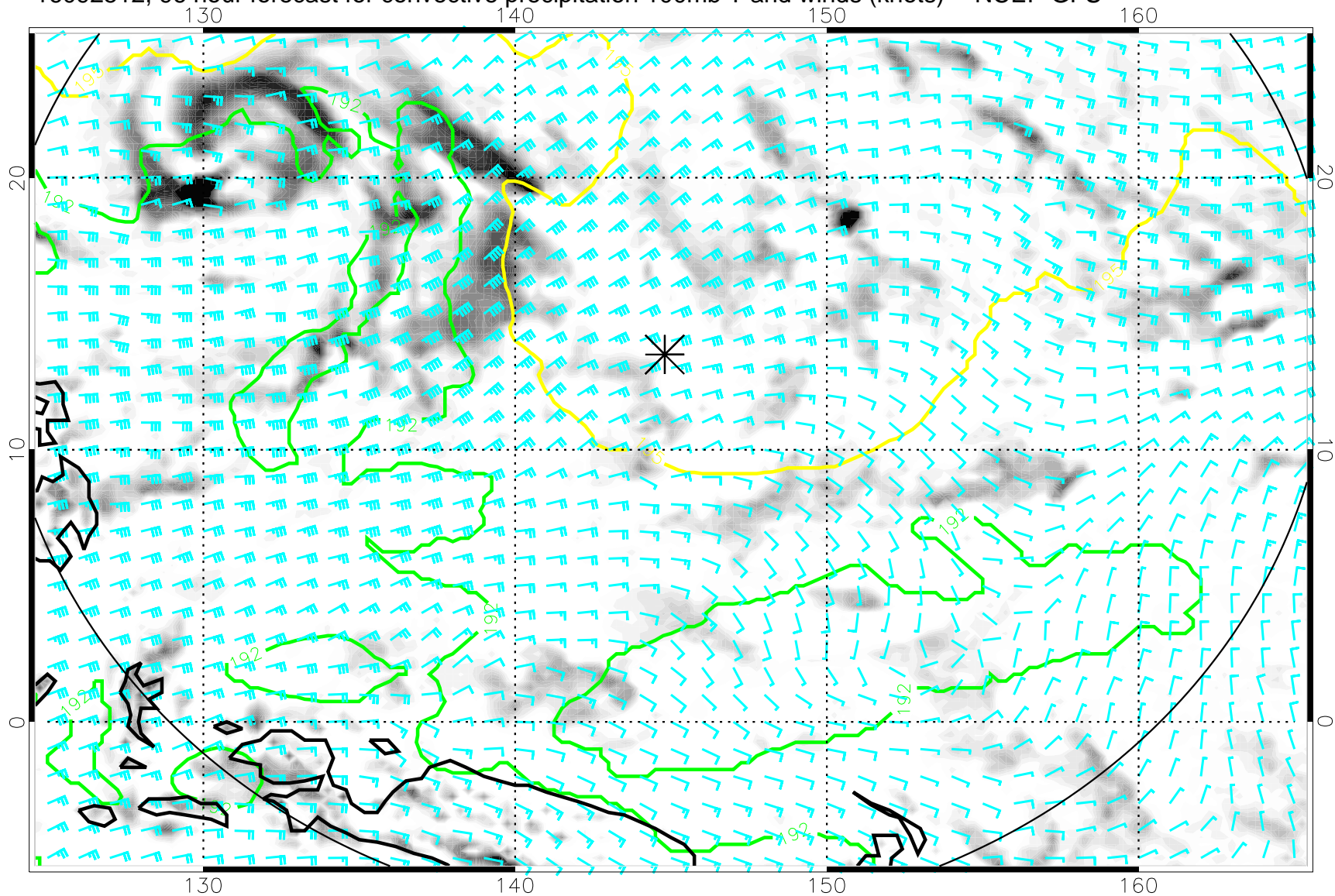
16092512, 96 hour forecast for convective precipitation 100mb T and winds (knots) -- NCEP GFS
