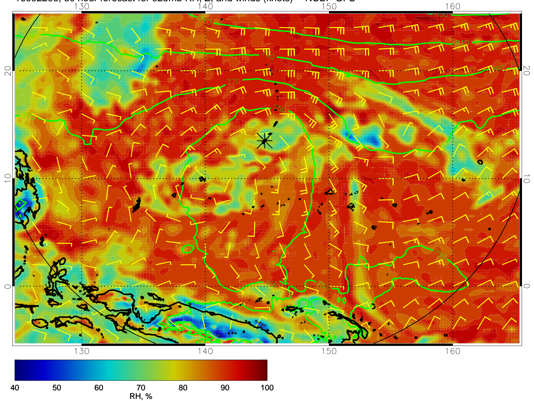
16092206, 30 hour forecast for 925mb RH, Z, and winds (knots) -- NCEP GFS
