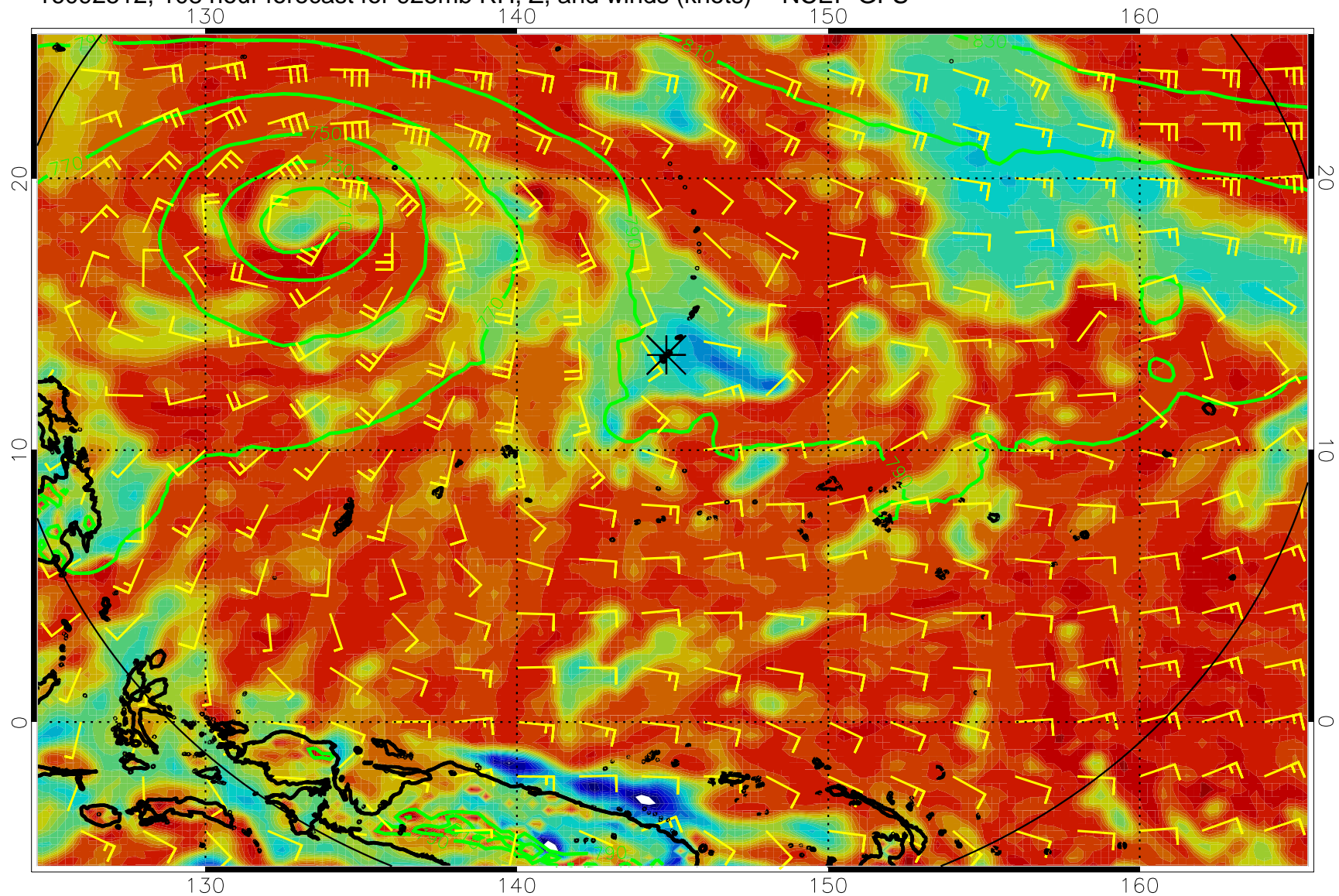
16092512, 108 hour forecast for 925mb RH, Z, and winds (knots) -- NCEP GFS
