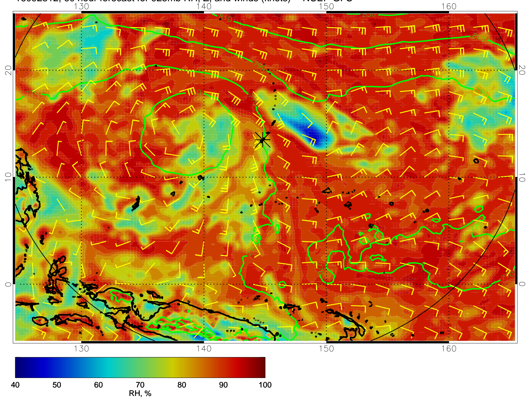
16092312, 60 hour forecast for 925mb RH, Z, and winds (knots) -- NCEP GFS
