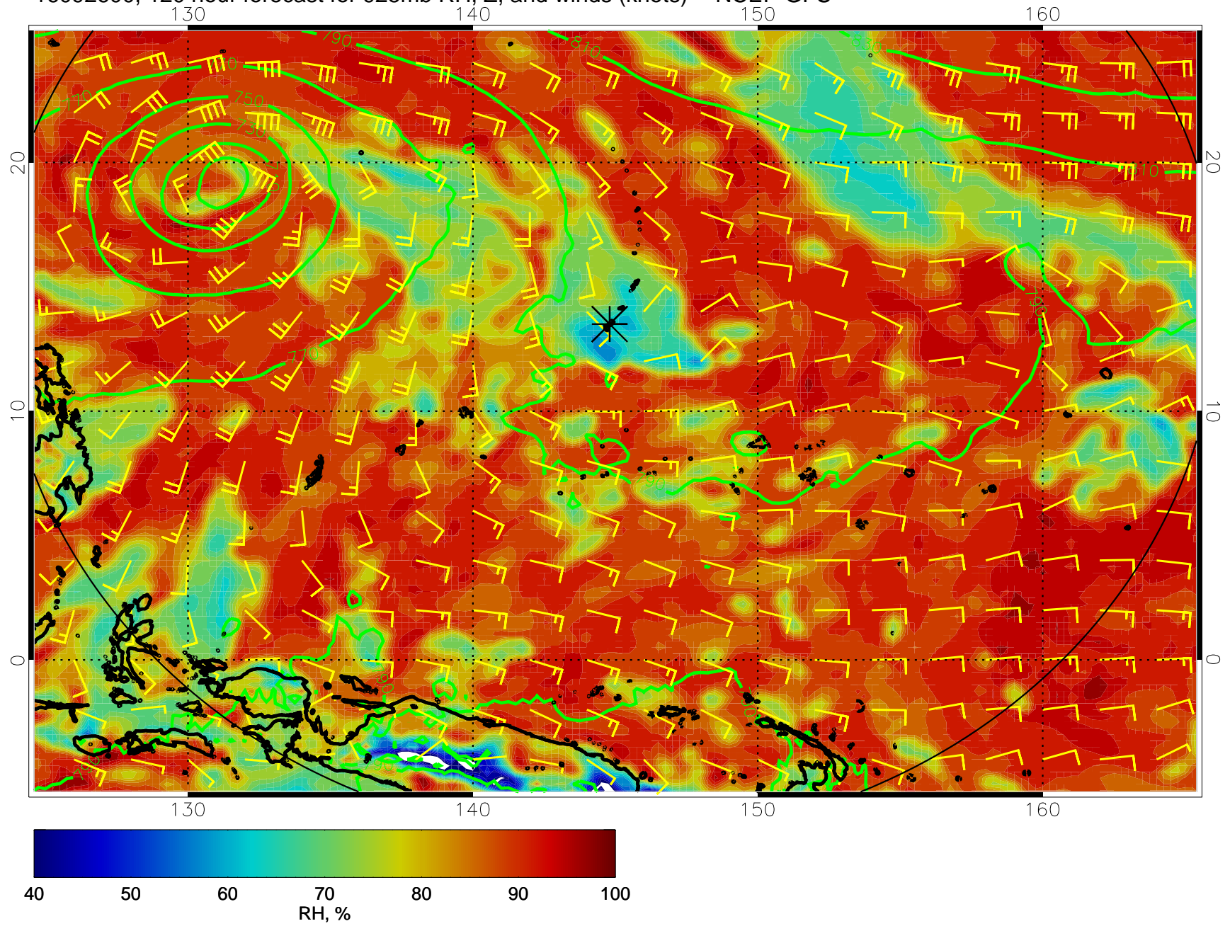
16092600, 120 hour forecast for 925mb RH, Z, and winds (knots) -- NCEP GFS
