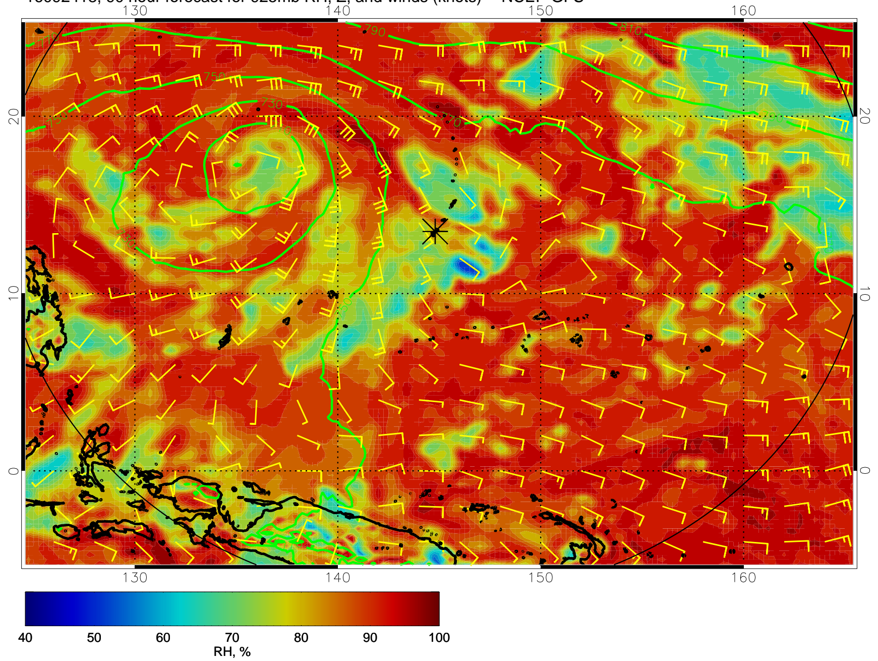
16092418, 90 hour forecast for 925mb RH, Z, and winds (knots) -- NCEP GFS
