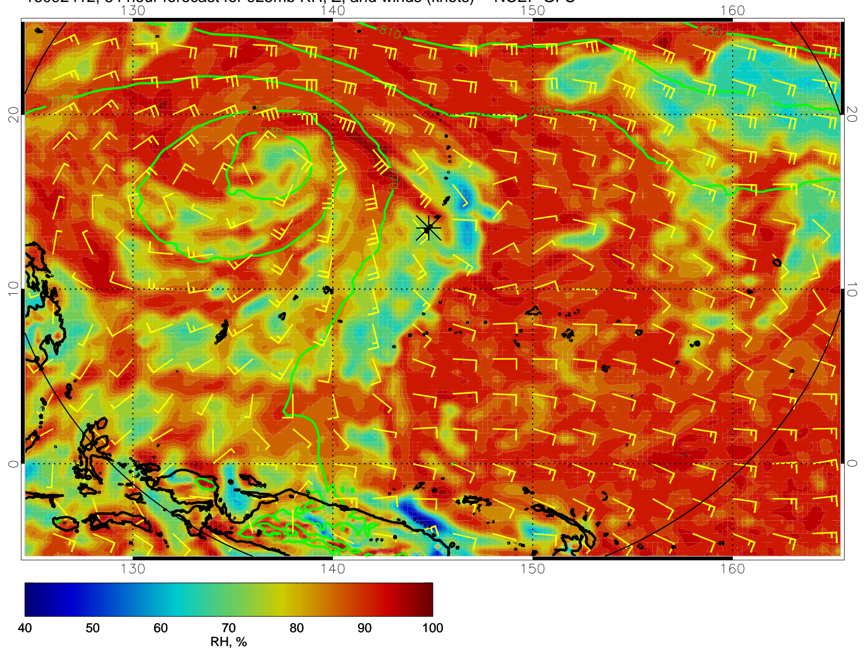
16092412, 84 hour forecast for 925mb RH, Z, and winds (knots) -- NCEP GFS
