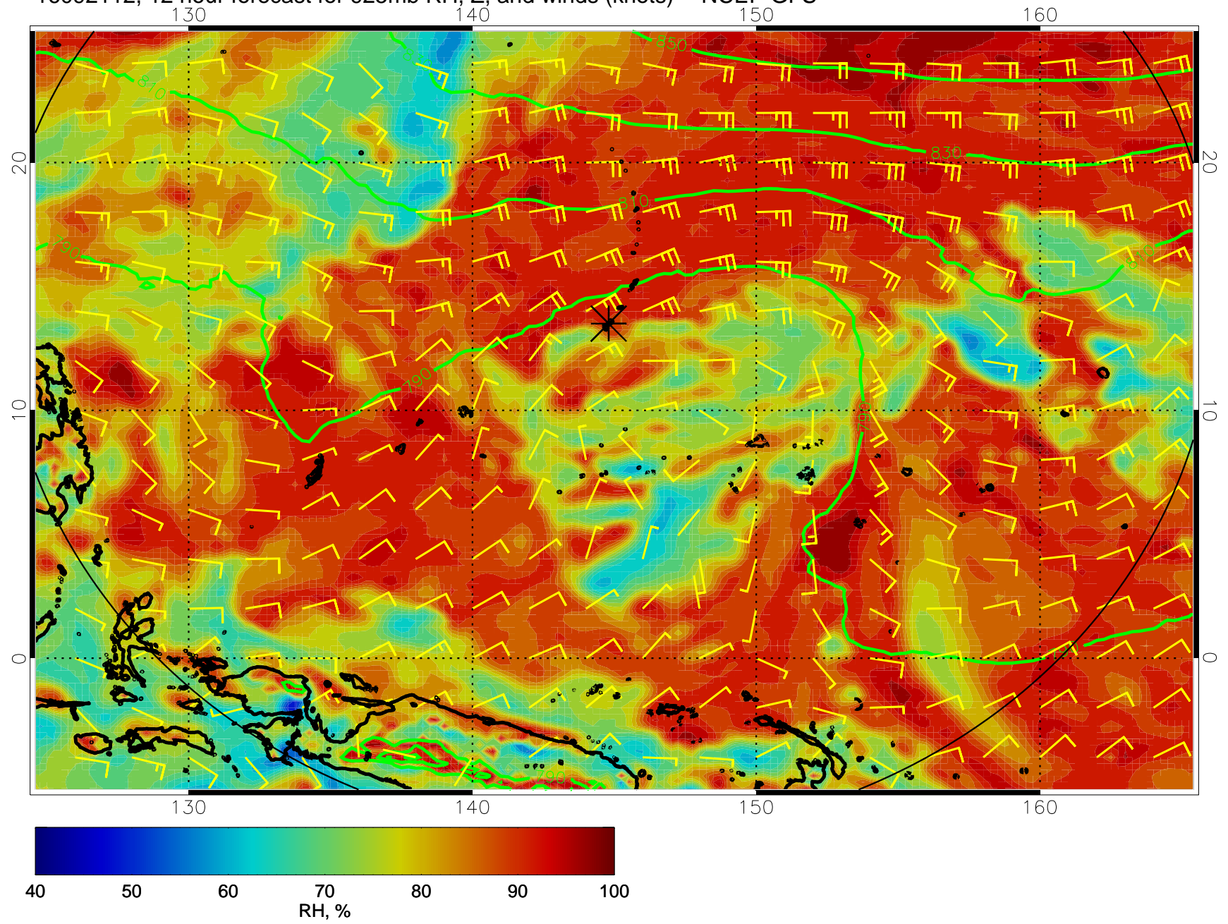
16092112, 12 hour forecast for 925mb RH, Z, and winds (knots) -- NCEP GFS
