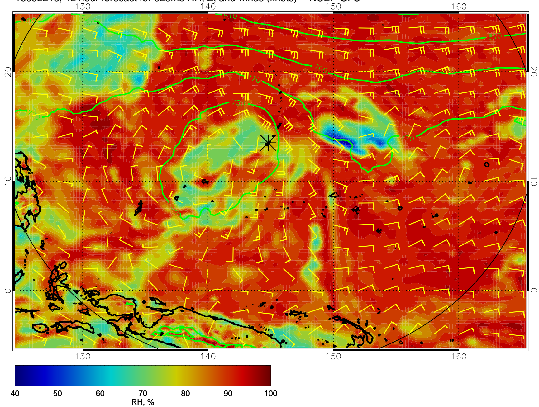
16092218, 42 hour forecast for 925mb RH, Z, and winds (knots) -- NCEP GFS
