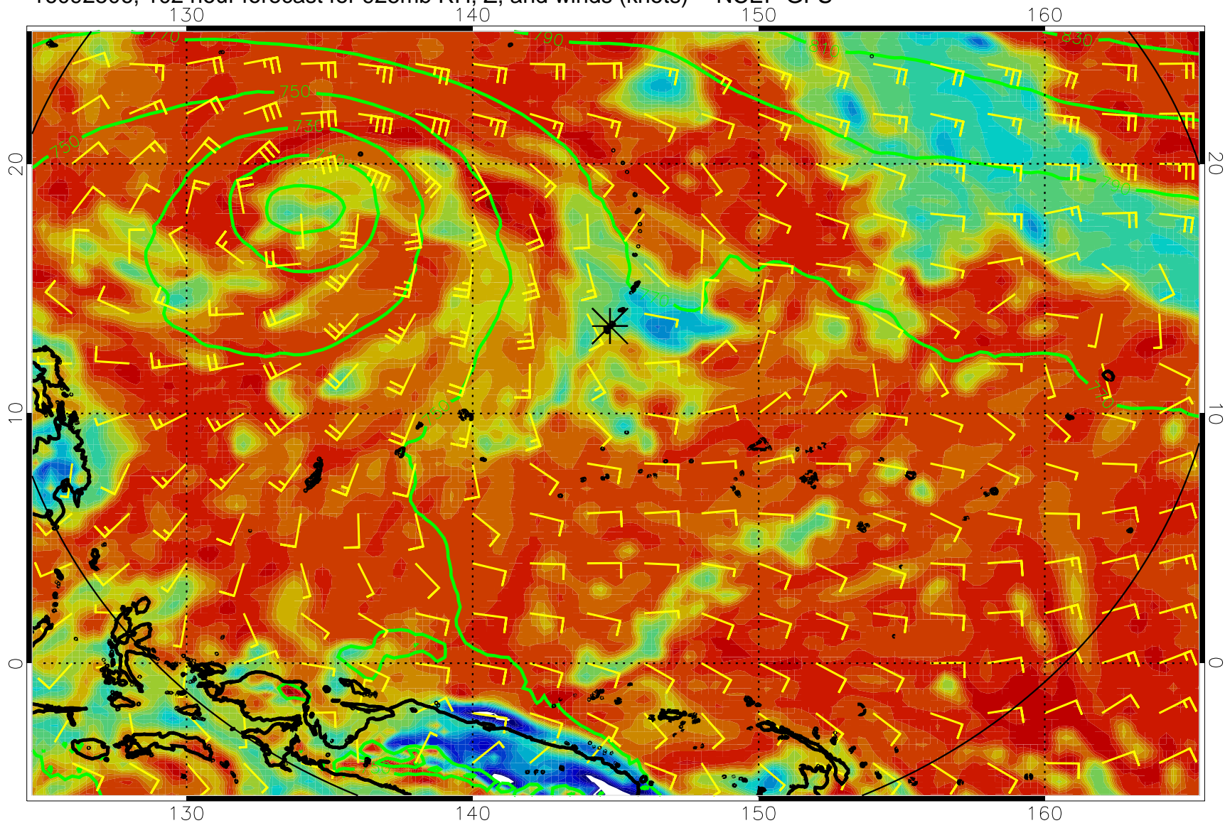
16092506, 102 hour forecast for 925mb RH, Z, and winds (knots) -- NCEP GFS
