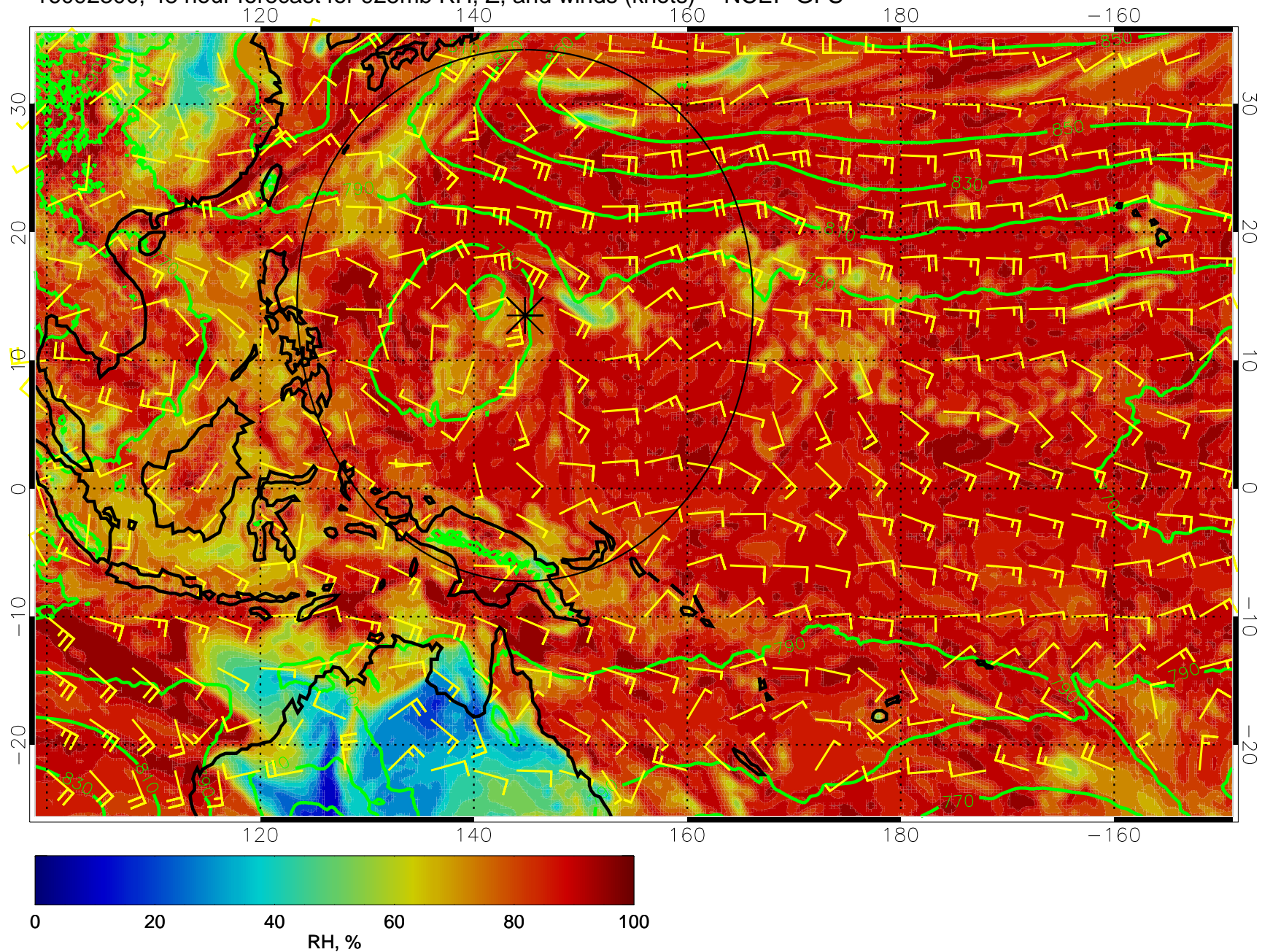
16092300, 48 hour forecast for 925mb RH, Z, and winds (knots) -- NCEP GFS
