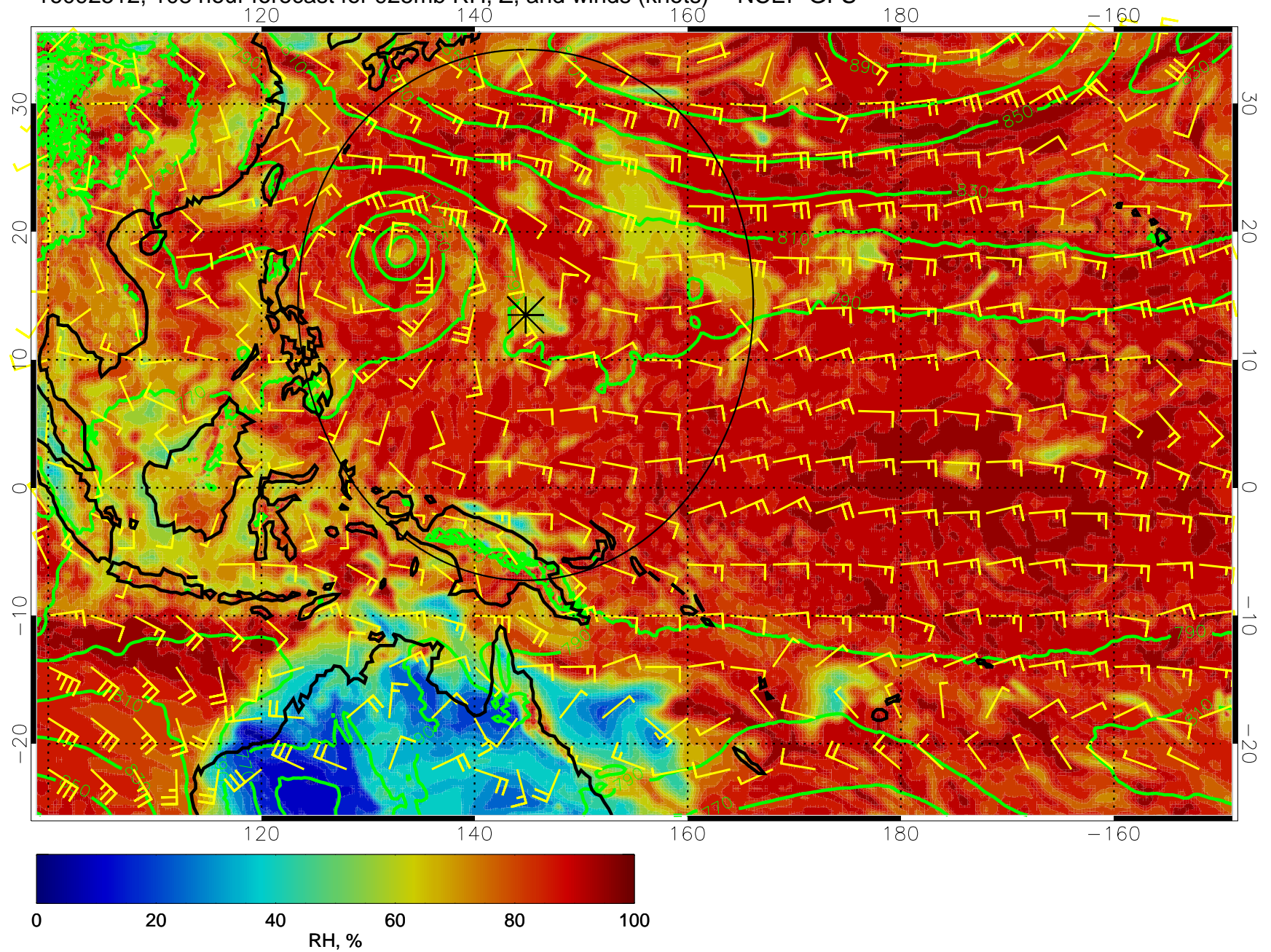
16092512, 108 hour forecast for 925mb RH, Z, and winds (knots) -- NCEP GFS
