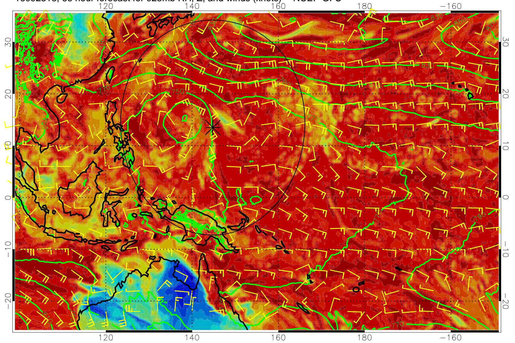
16092318, 66 hour forecast for 925mb RH, Z, and winds (knots) -- NCEP GFS
