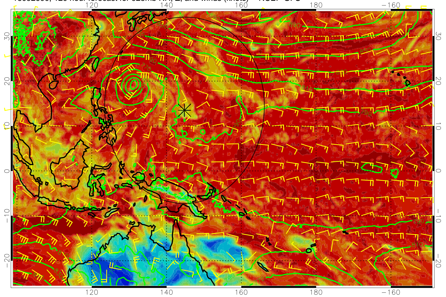
16092600, 120 hour forecast for 925mb RH, Z, and winds (knots) -- NCEP GFS
