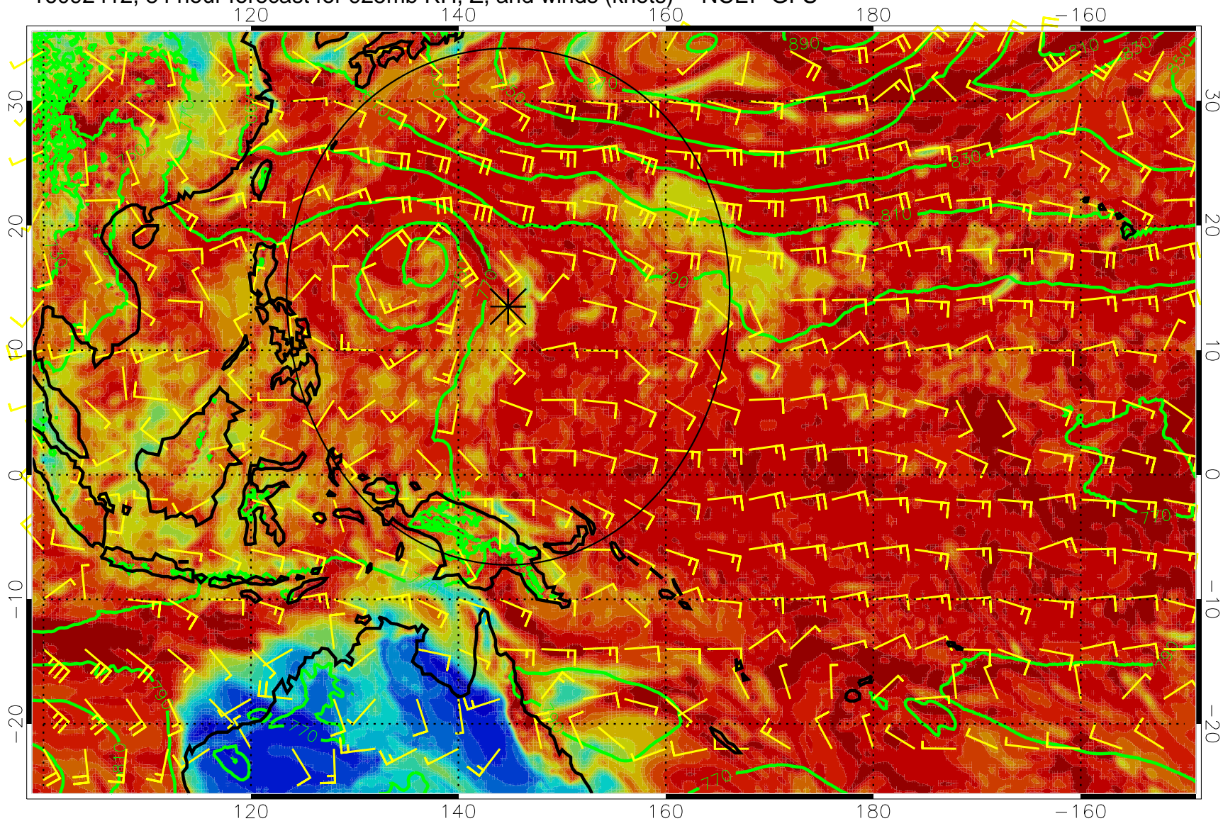
16092412, 84 hour forecast for 925mb RH, Z, and winds (knots) -- NCEP GFS
