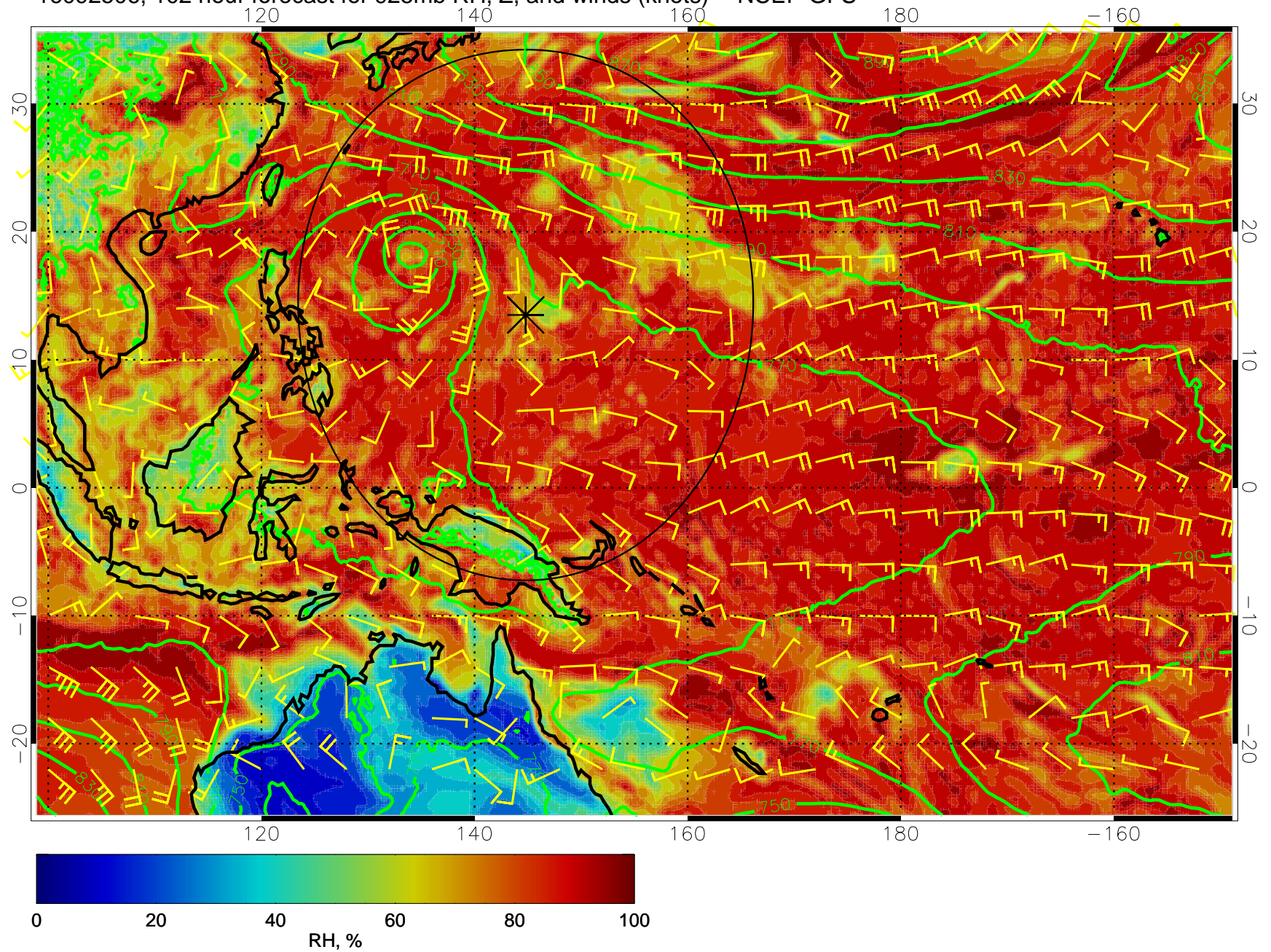
16092506, 102 hour forecast for 925mb RH, Z, and winds (knots) -- NCEP GFS
