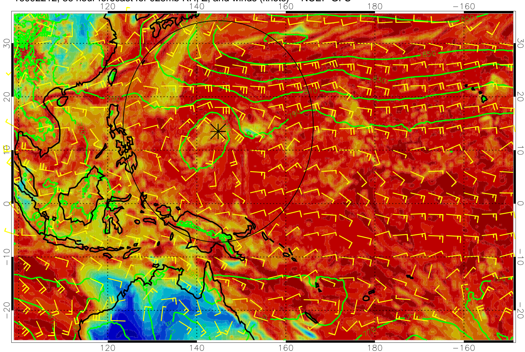
16092212, 36 hour forecast for 925mb RH, Z, and winds (knots) -- NCEP GFS
