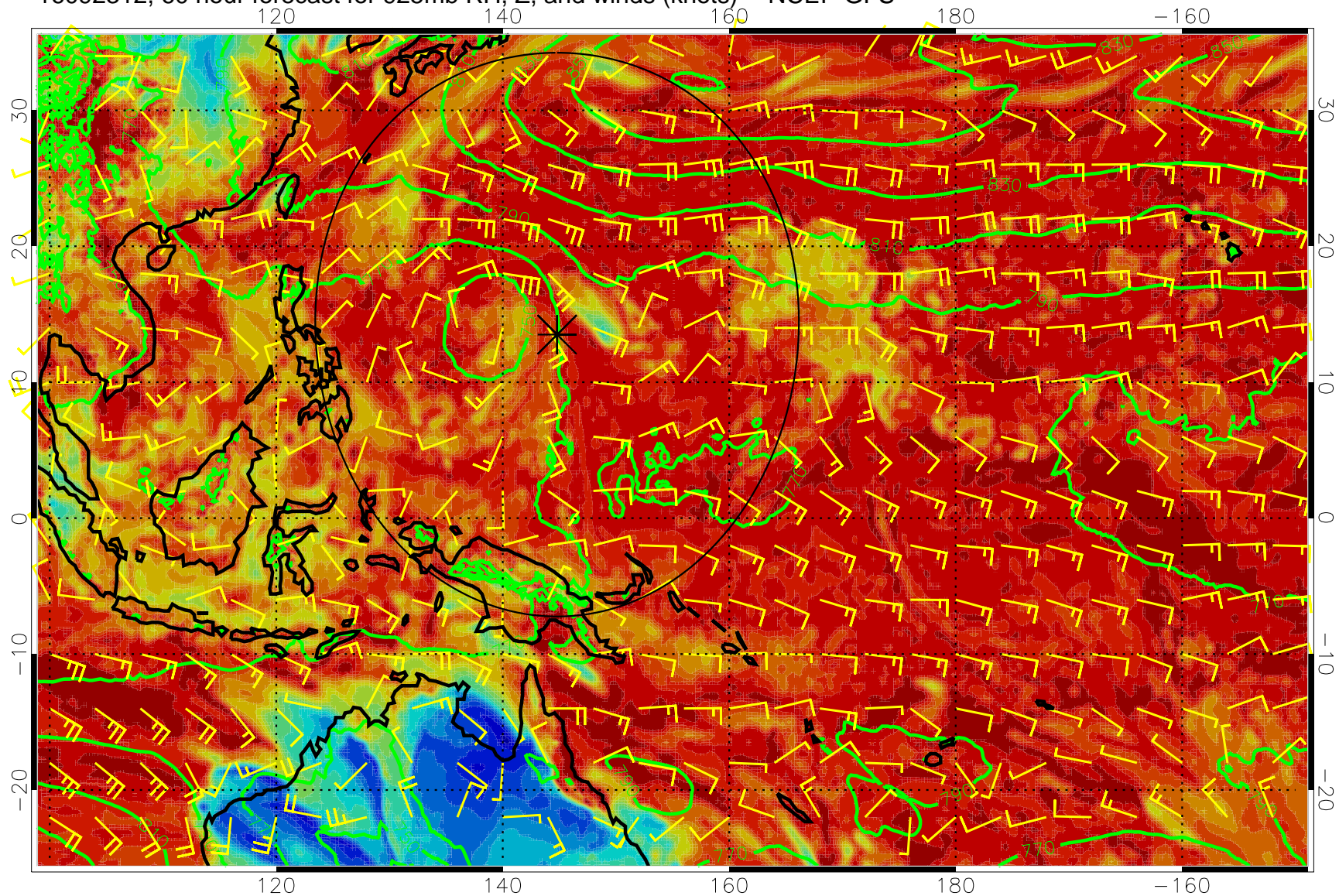
16092312, 60 hour forecast for 925mb RH, Z, and winds (knots) -- NCEP GFS
