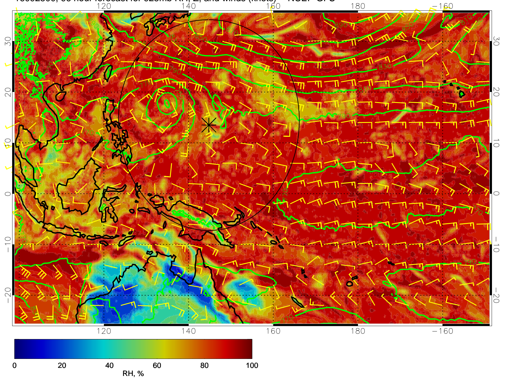
16092500, 96 hour forecast for 925mb RH, Z, and winds (knots) -- NCEP GFS
