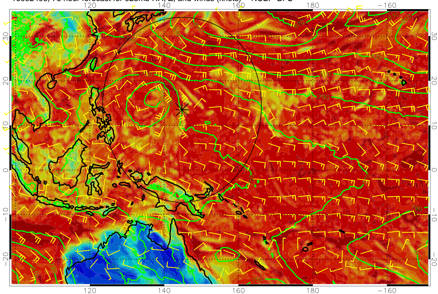
16092406, 78 hour forecast for 925mb RH, Z, and winds (knots) -- NCEP GFS
