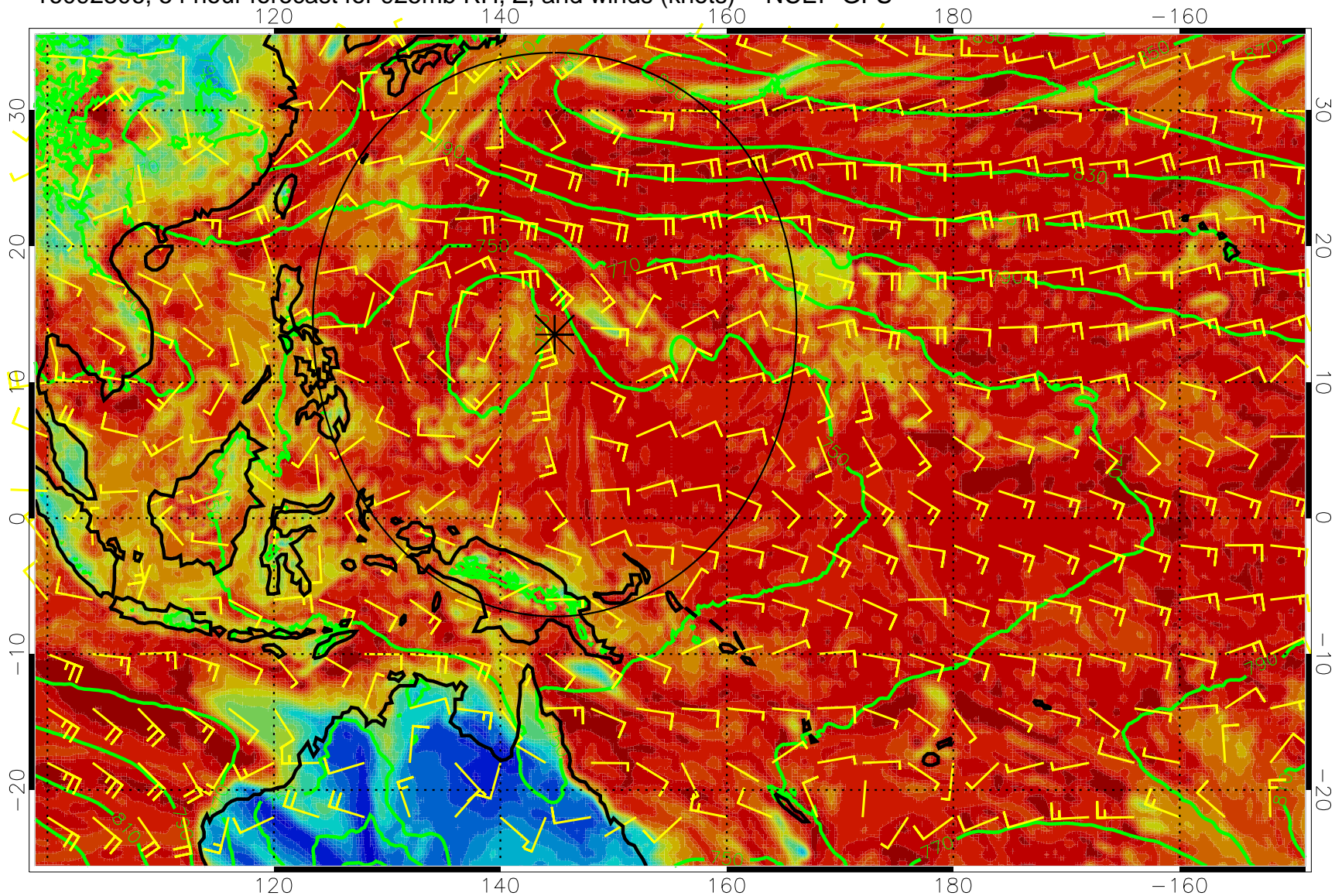
16092306, 54 hour forecast for 925mb RH, Z, and winds (knots) -- NCEP GFS
