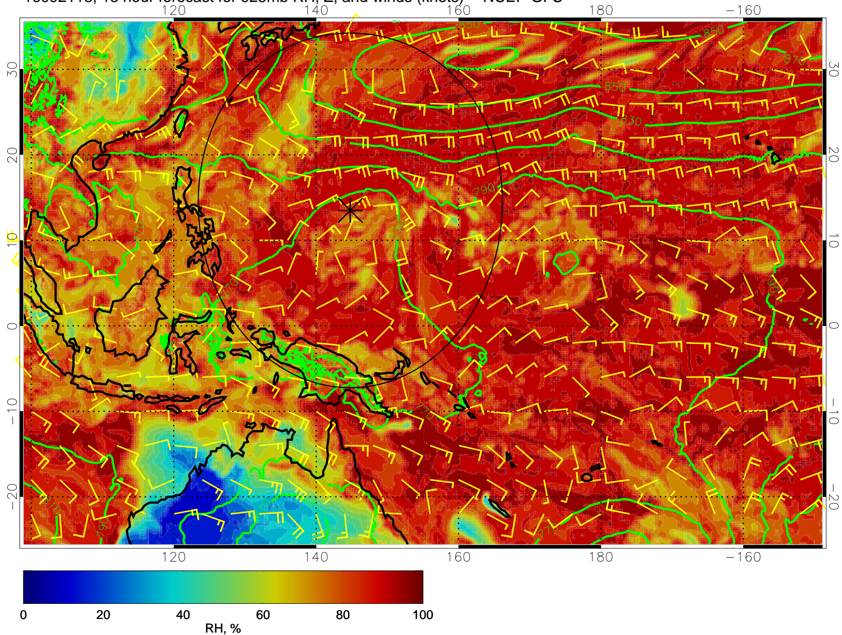
16092118, 18 hour forecast for 925mb RH, Z, and winds (knots) -- NCEP GFS
