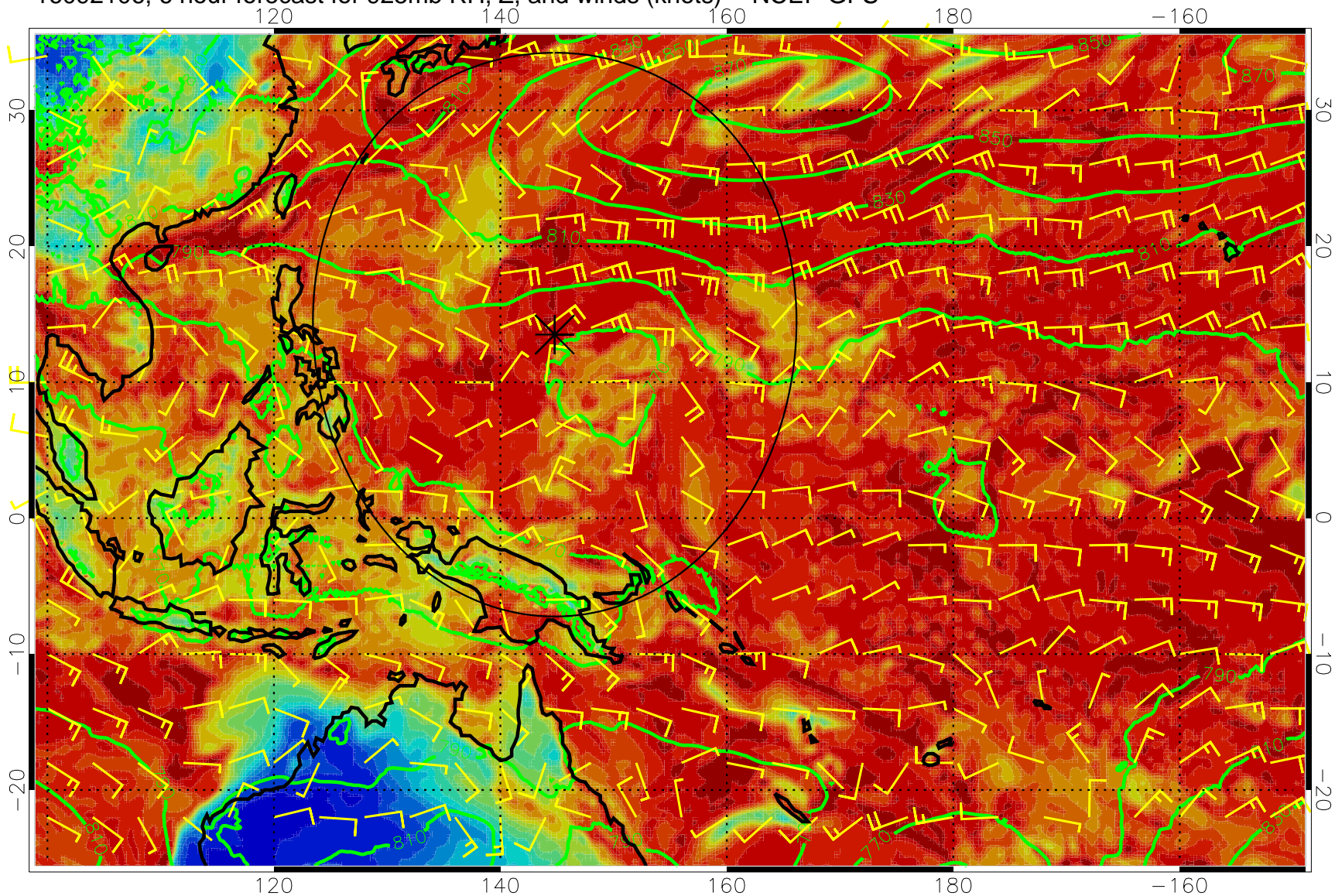
16092106, 6 hour forecast for 925mb RH, Z, and winds (knots) -- NCEP GFS
