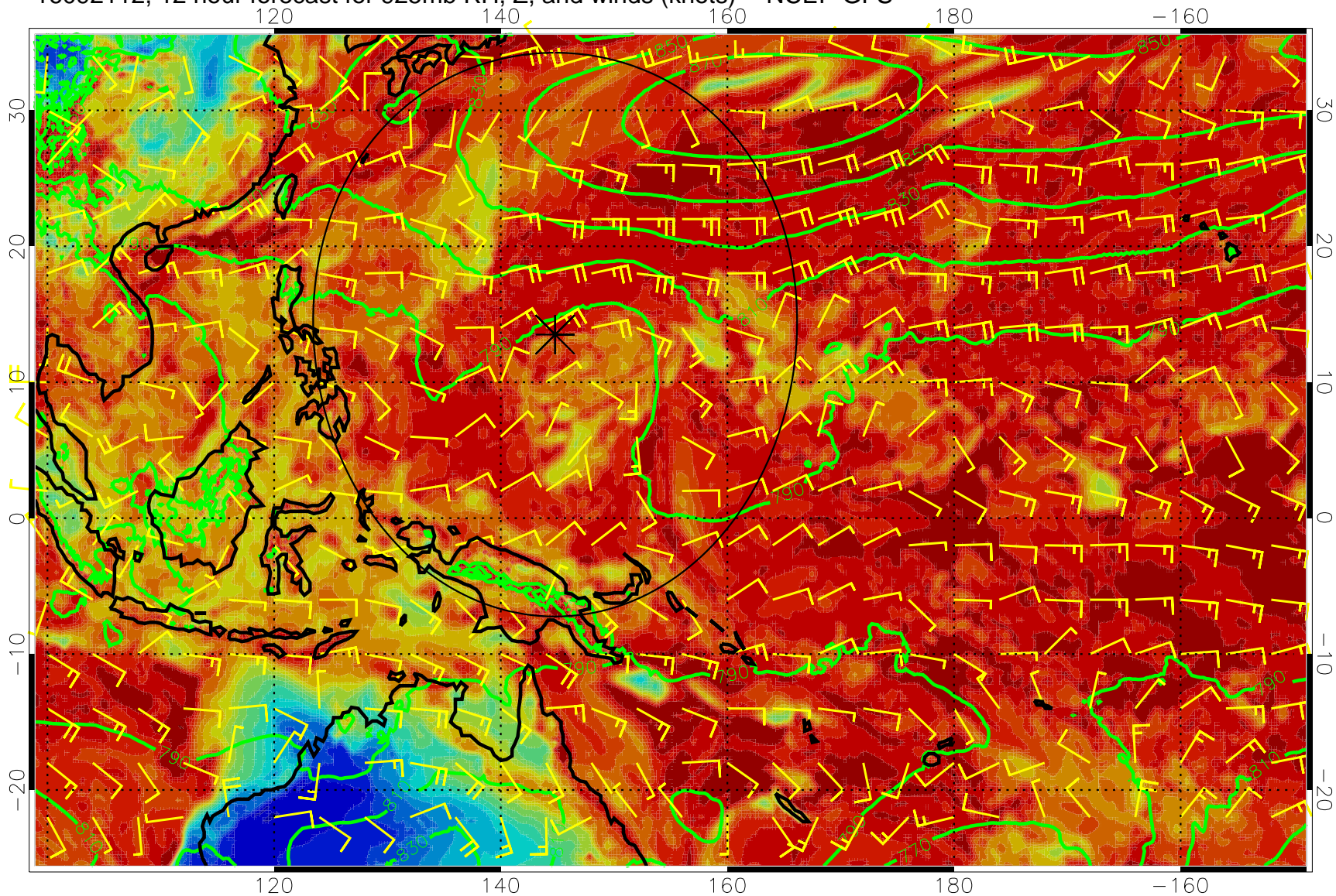
16092112, 12 hour forecast for 925mb RH, Z, and winds (knots) -- NCEP GFS
