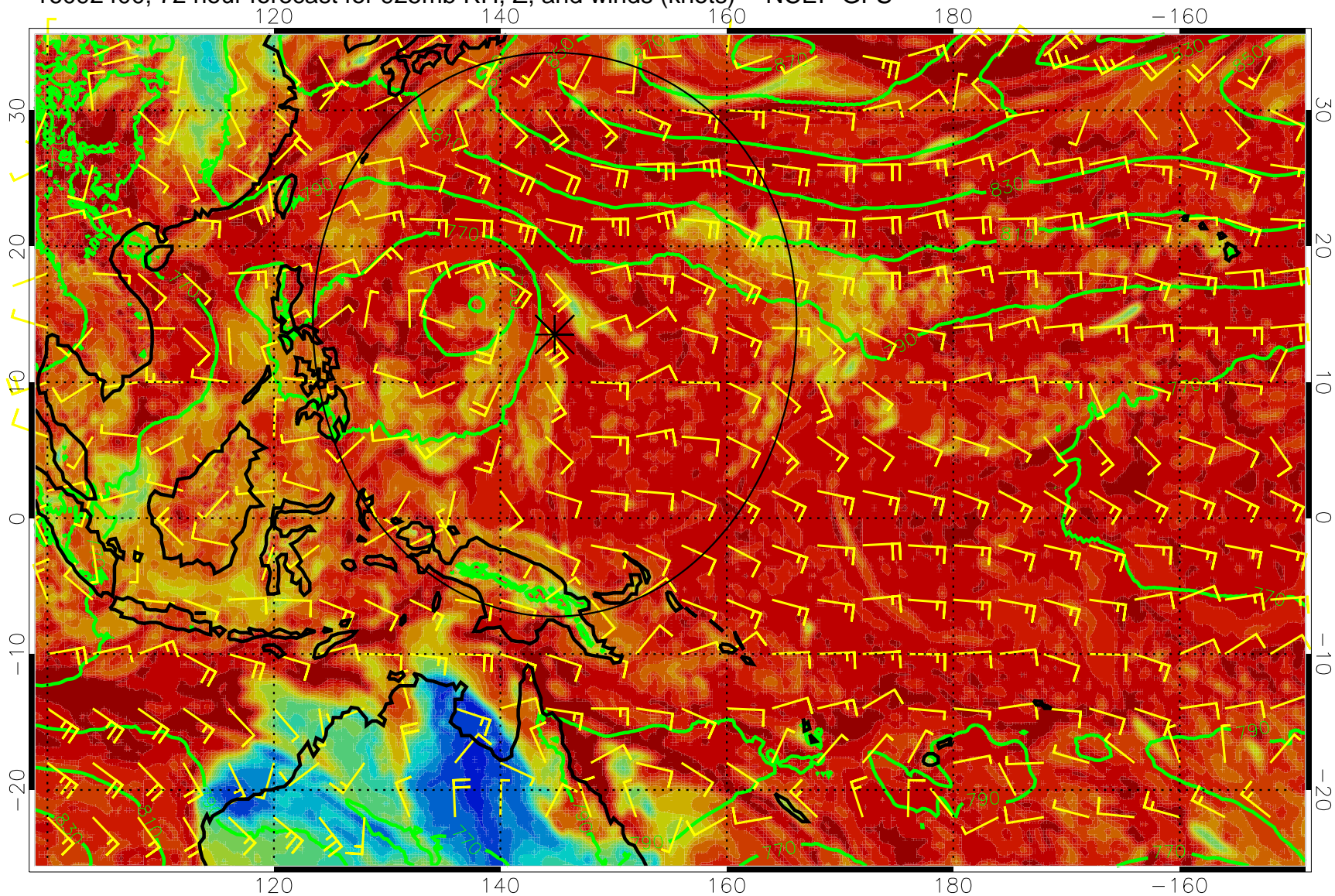
16092400, 72 hour forecast for 925mb RH, Z, and winds (knots) -- NCEP GFS
