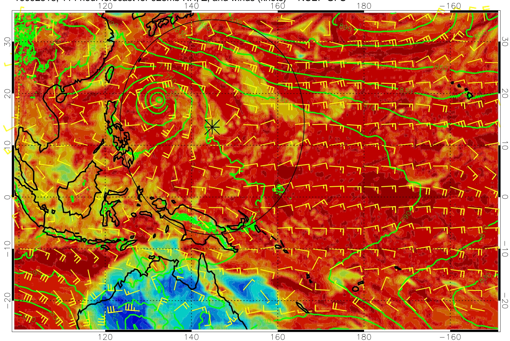
16092518, 114 hour forecast for 925mb RH, Z, and winds (knots) -- NCEP GFS
