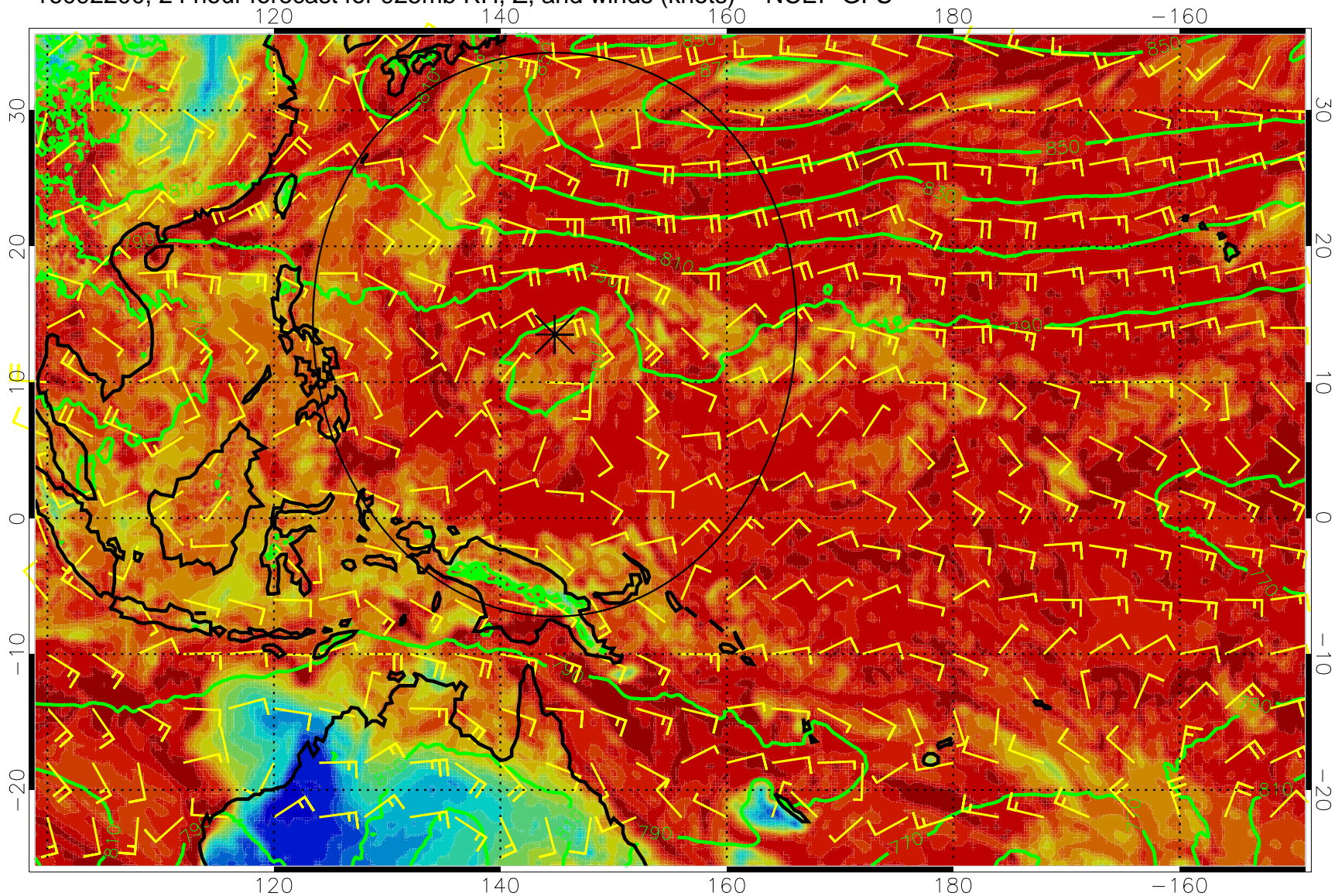
16092200, 24 hour forecast for 925mb RH, Z, and winds (knots) -- NCEP GFS
