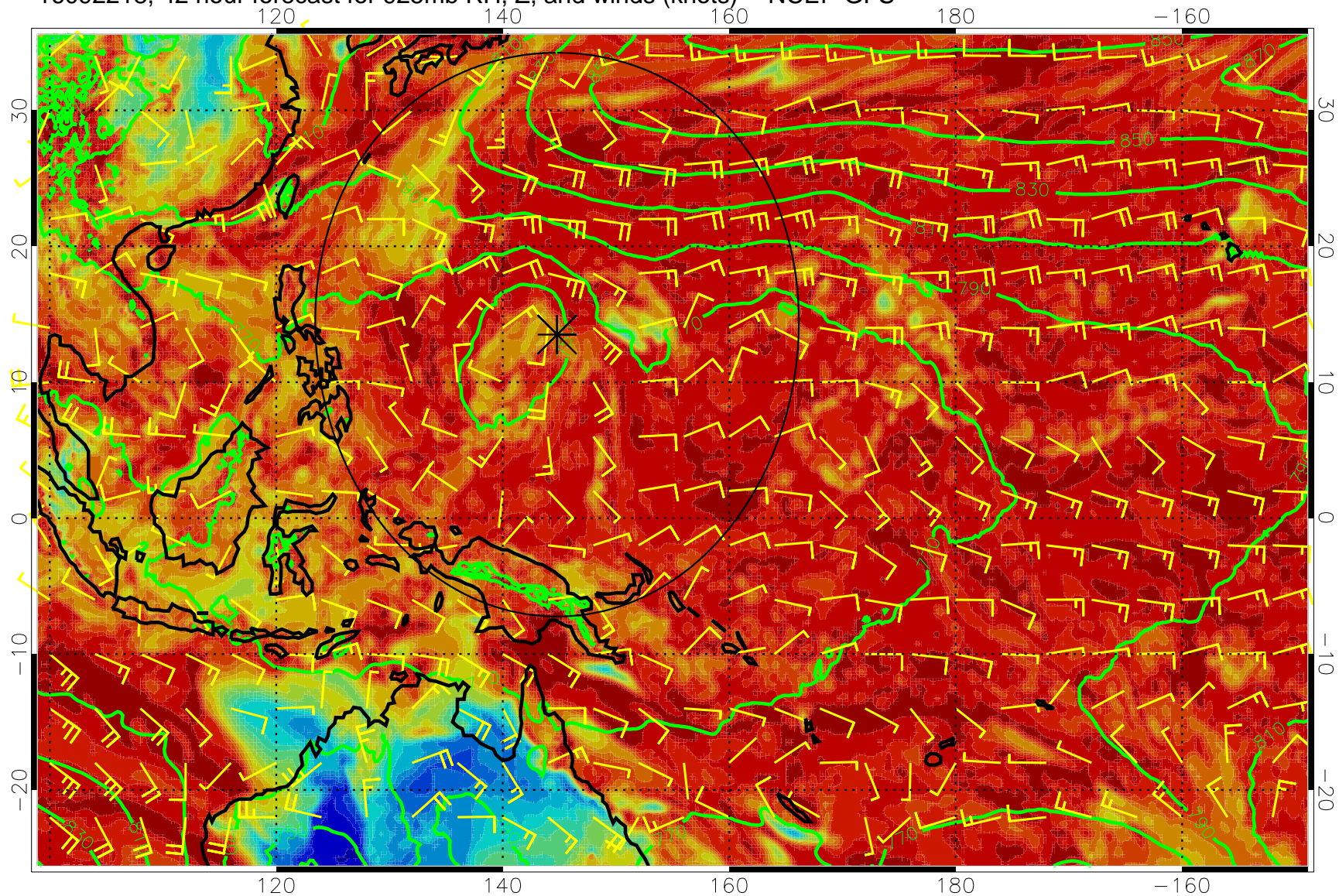
16092218, 42 hour forecast for 925mb RH, Z, and winds (knots) -- NCEP GFS
