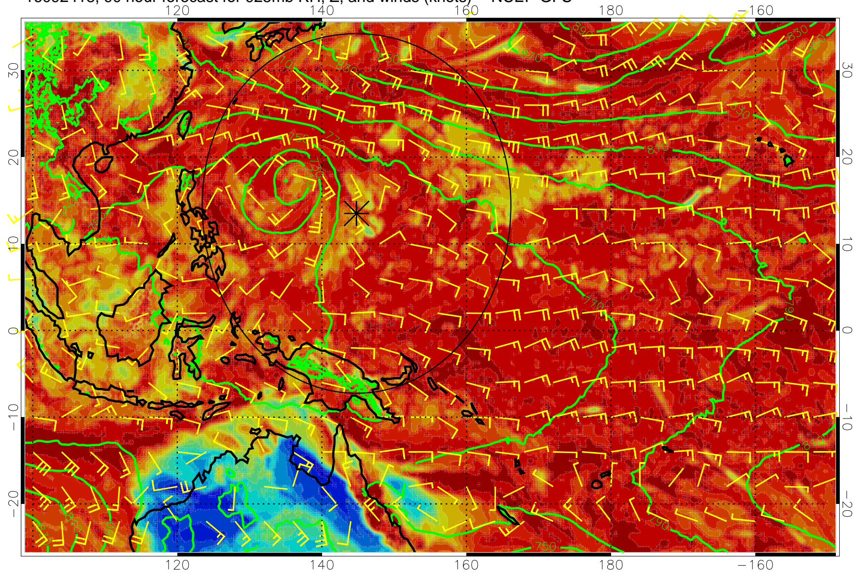
16092418, 90 hour forecast for 925mb RH, Z, and winds (knots) -- NCEP GFS
