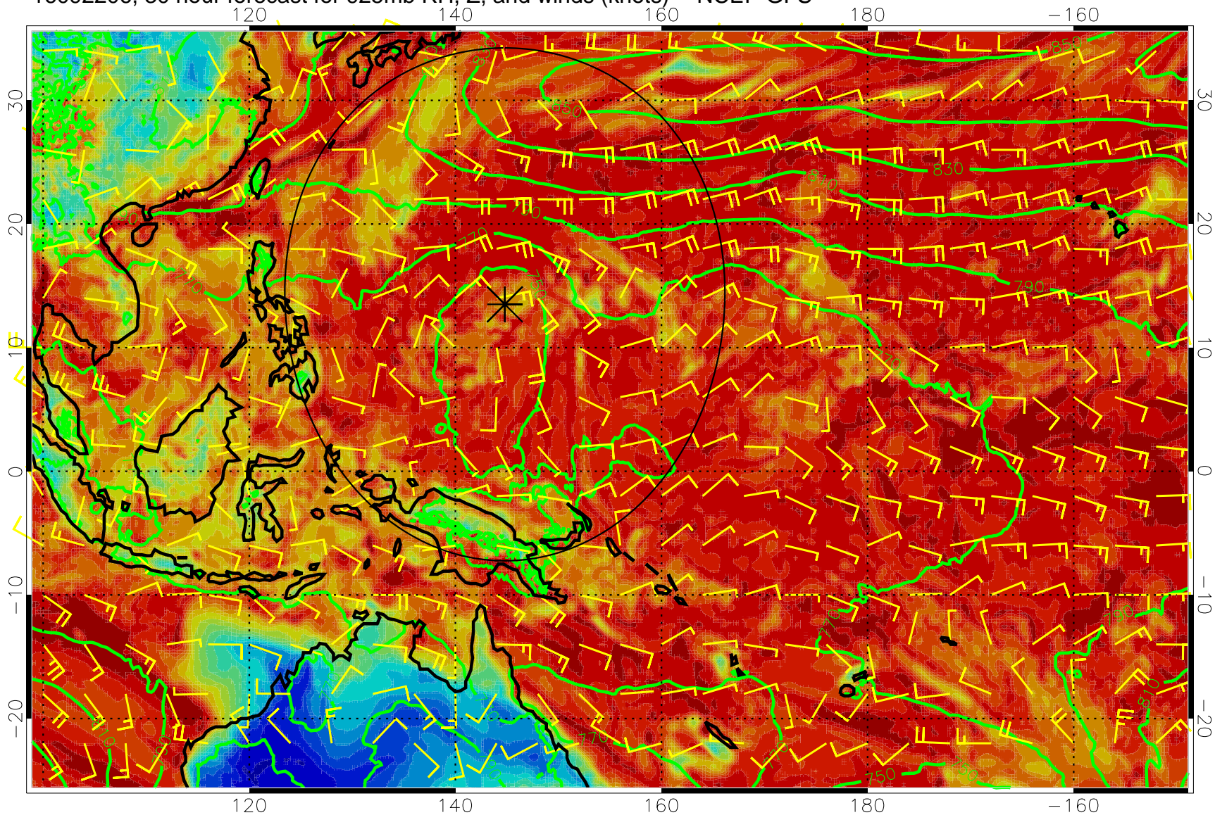
16092206, 30 hour forecast for 925mb RH, Z, and winds (knots) -- NCEP GFS
