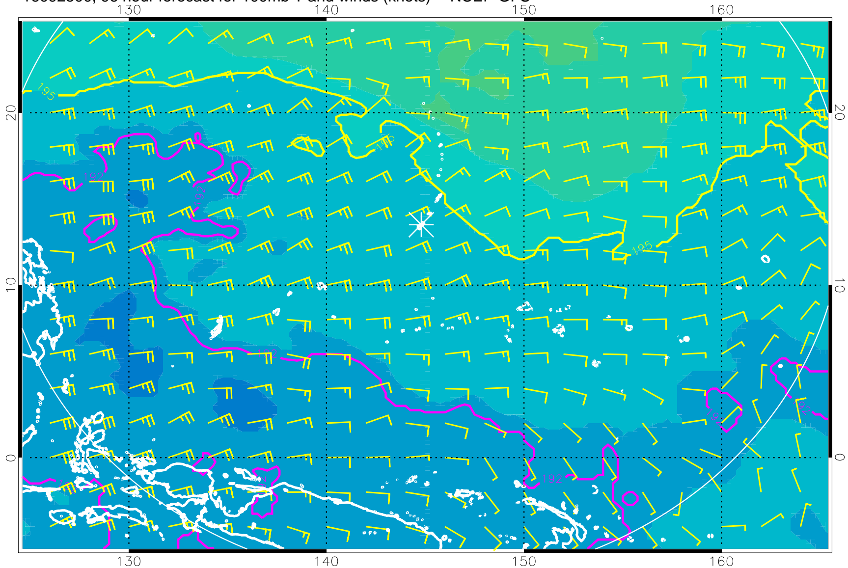
16092500, 96 hour forecast for 100mb T and winds (knots) -- NCEP GFS
