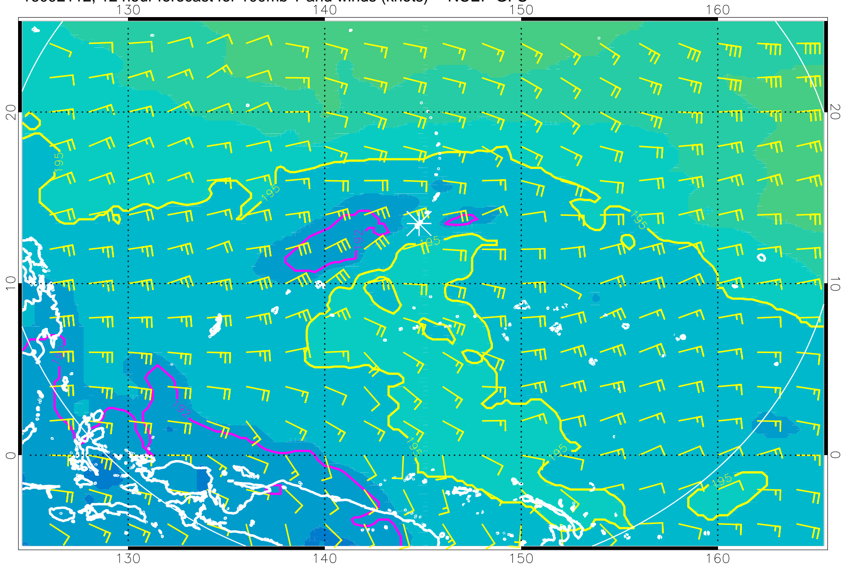
16092112, 12 hour forecast for 100mb T and winds (knots) -- NCEP GFS
