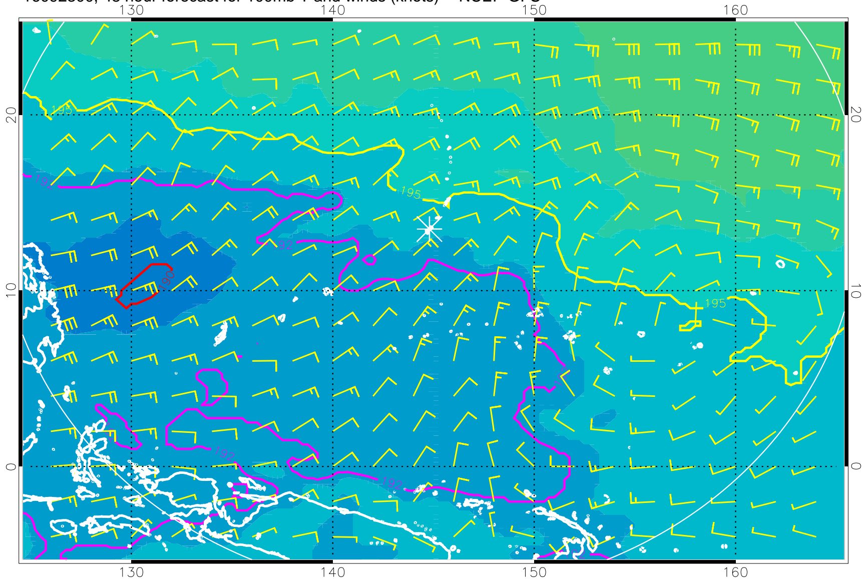
16092300, 48 hour forecast for 100mb T and winds (knots) -- NCEP GFS
