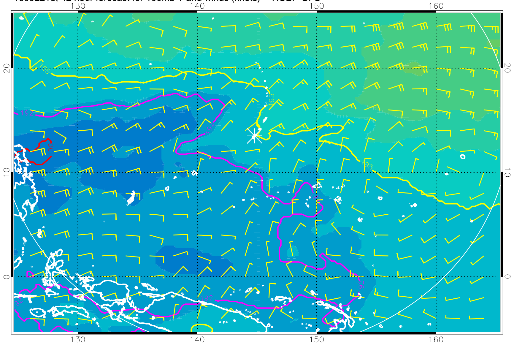
16092218, 42 hour forecast for 100mb T and winds (knots) -- NCEP GFS
