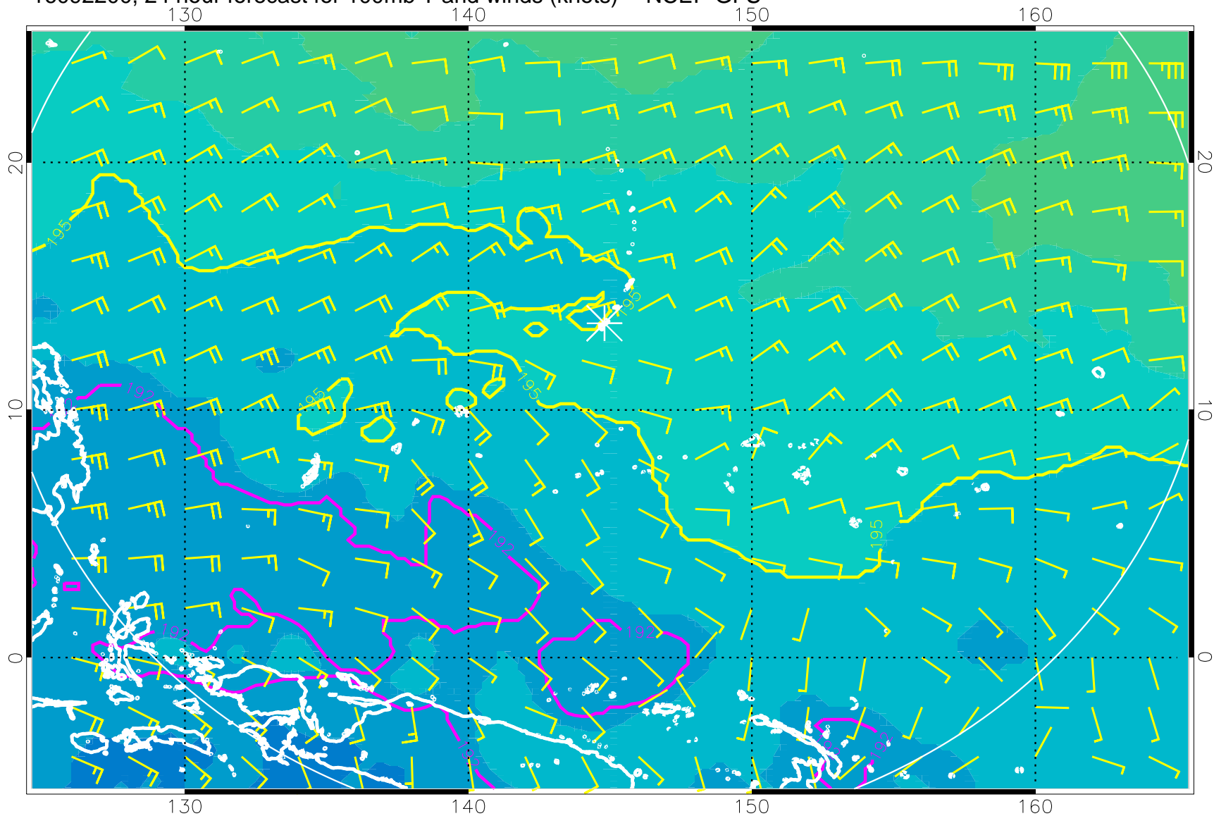
16092200, 24 hour forecast for 100mb T and winds (knots) -- NCEP GFS
