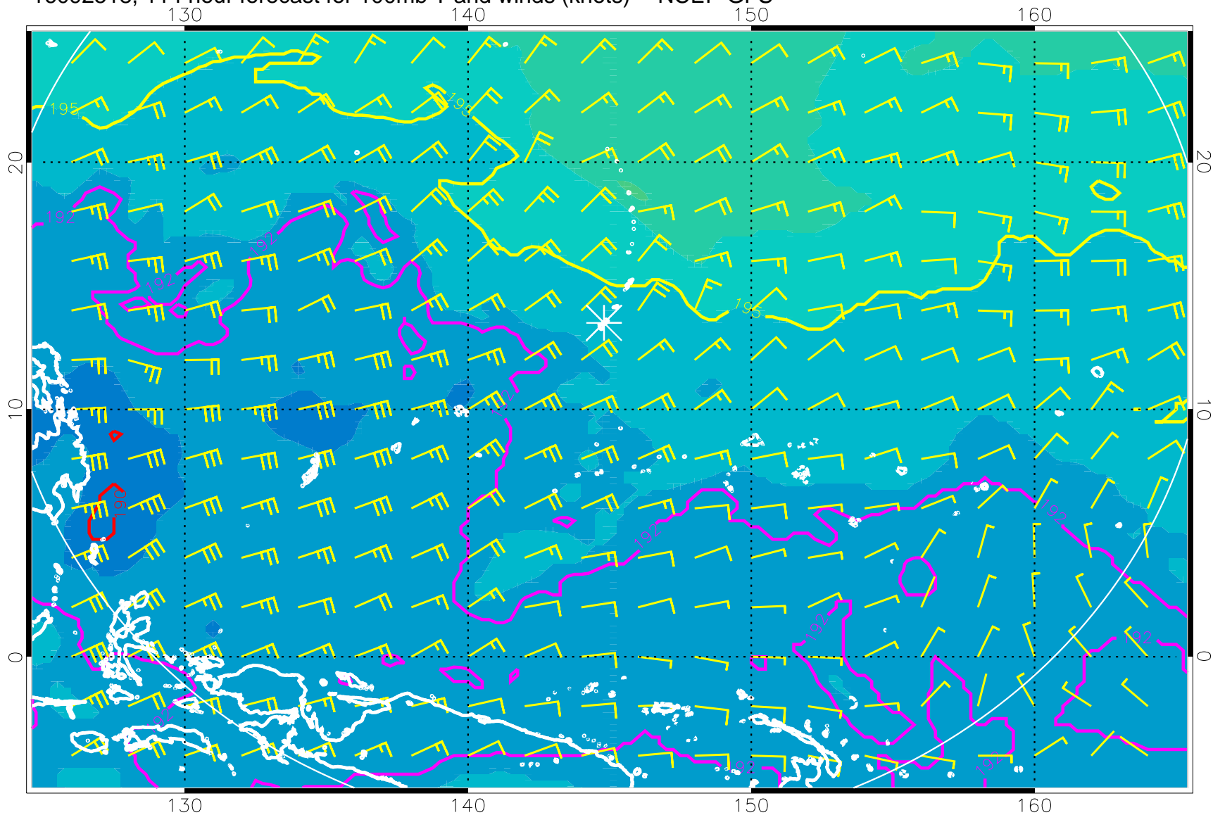
16092518, 114 hour forecast for 100mb T and winds (knots) -- NCEP GFS
