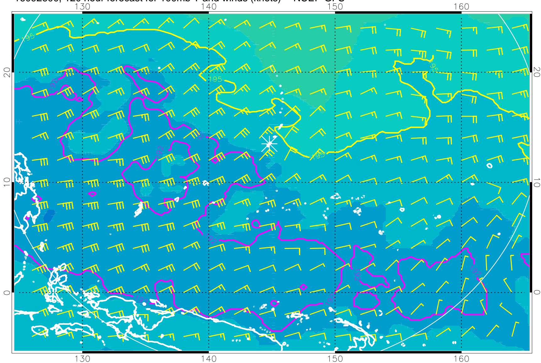
16092600, 120 hour forecast for 100mb T and winds (knots) -- NCEP GFS
