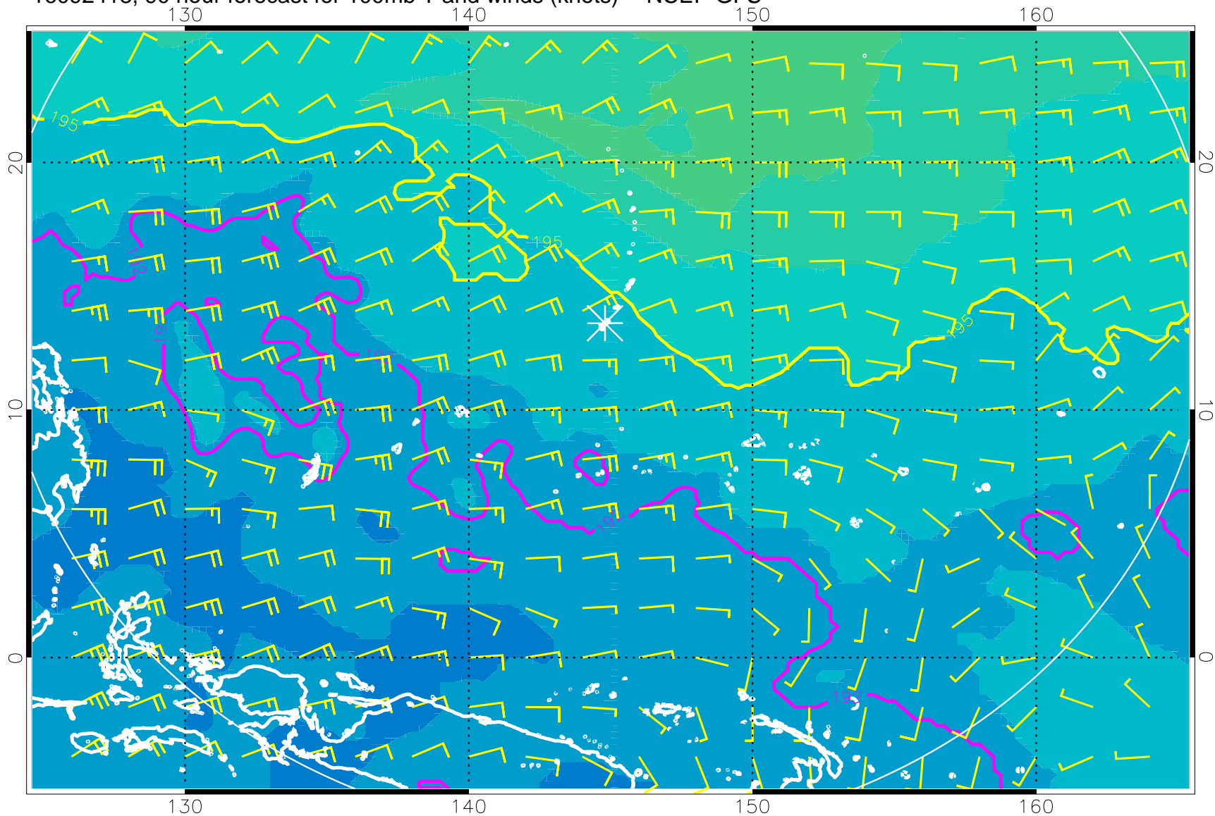
16092418, 90 hour forecast for 100mb T and winds (knots) -- NCEP GFS
