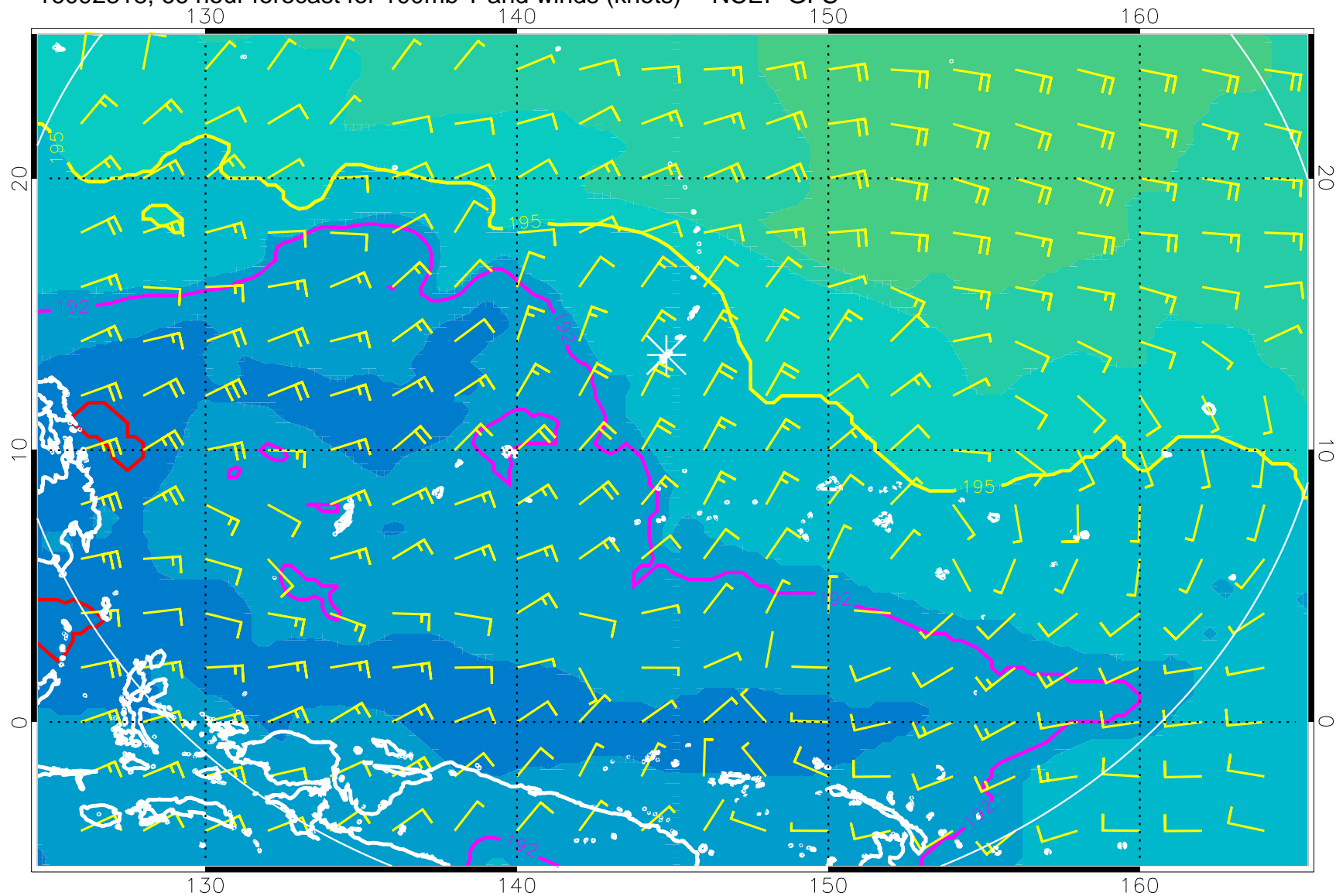
16092318, 66 hour forecast for 100mb T and winds (knots) -- NCEP GFS
