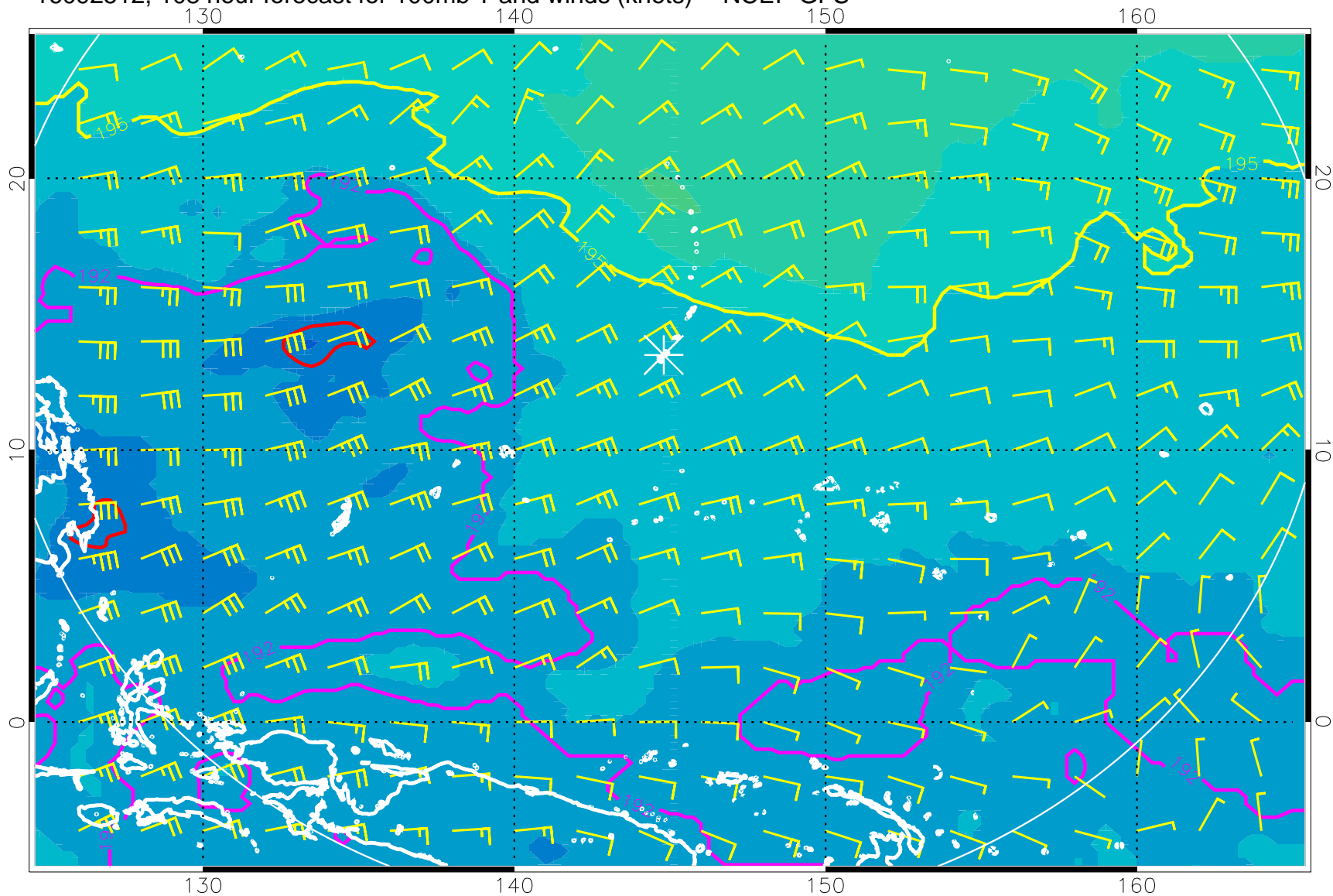
16092512, 108 hour forecast for 100mb T and winds (knots) -- NCEP GFS
