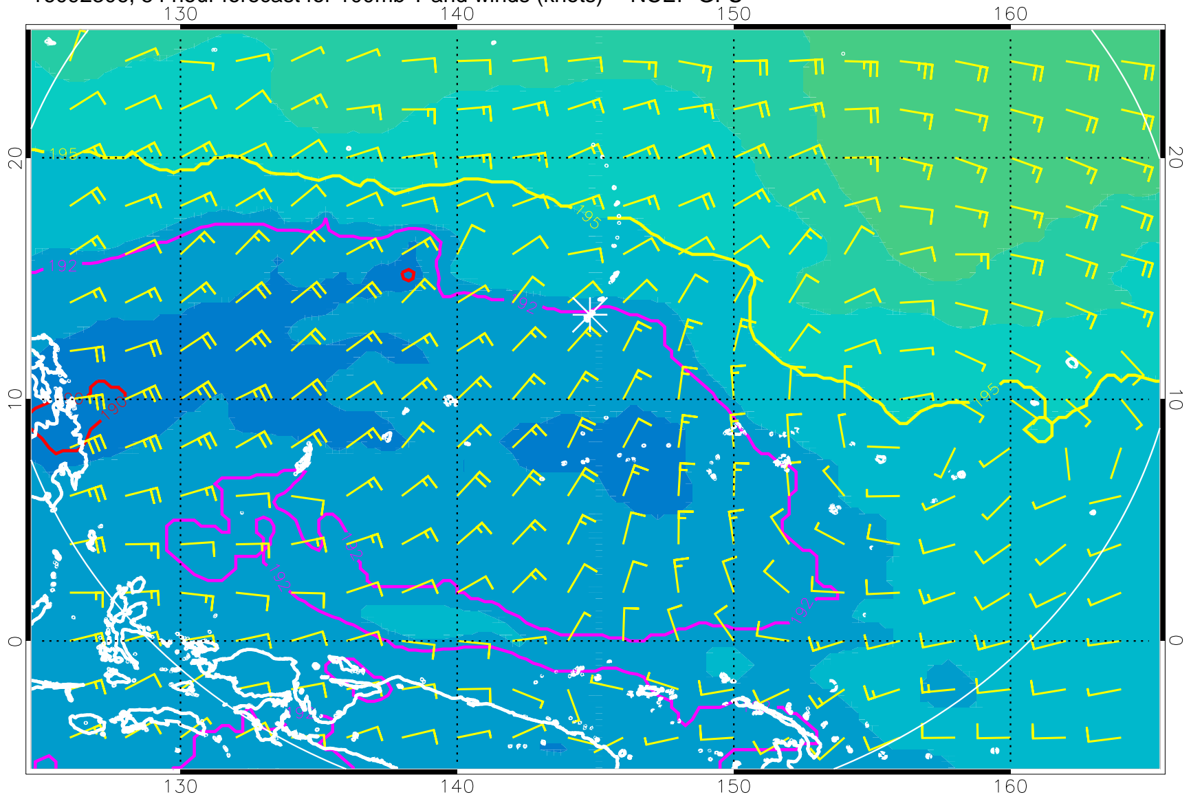
16092306, 54 hour forecast for 100mb T and winds (knots) -- NCEP GFS
