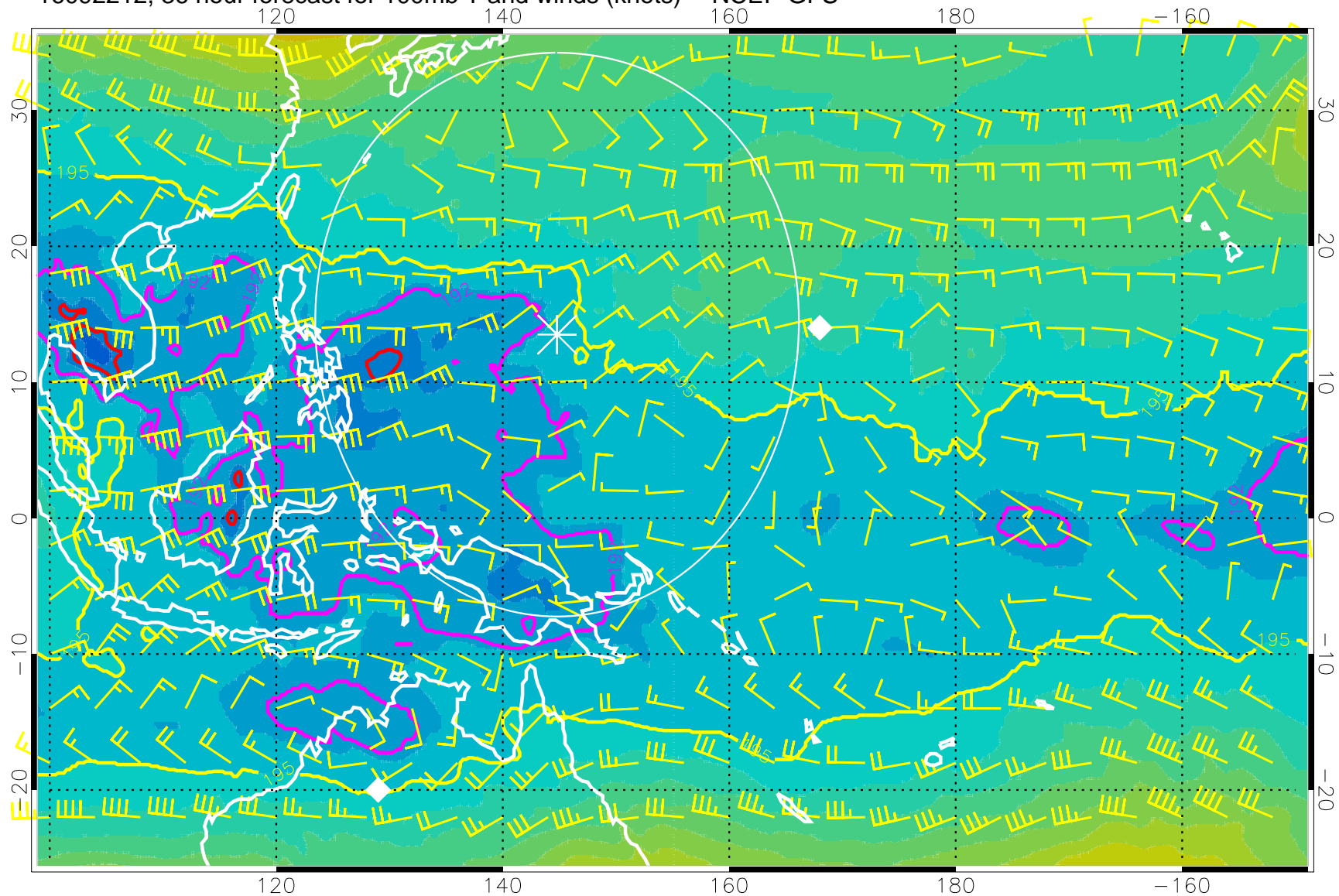
16092212, 36 hour forecast for 100mb T and winds (knots) -- NCEP GFS
