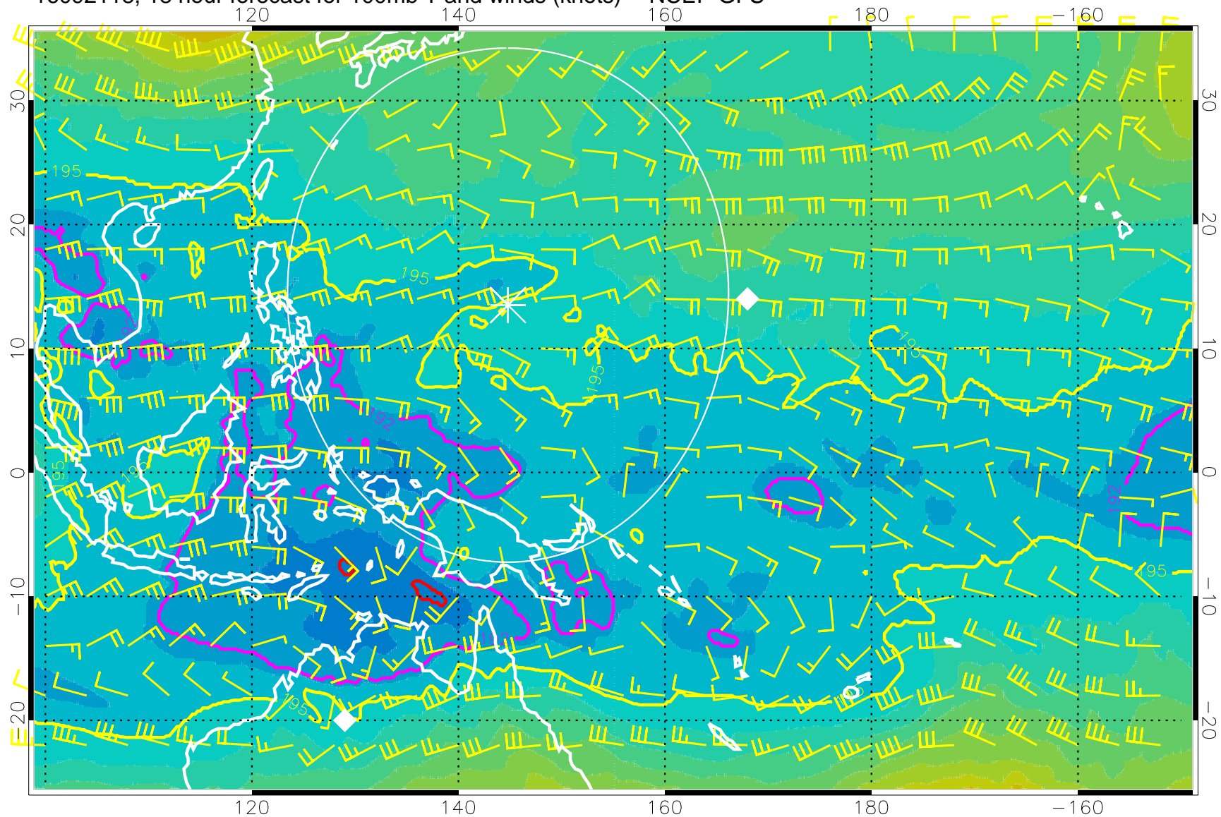
16092118, 18 hour forecast for 100mb T and winds (knots) -- NCEP GFS
