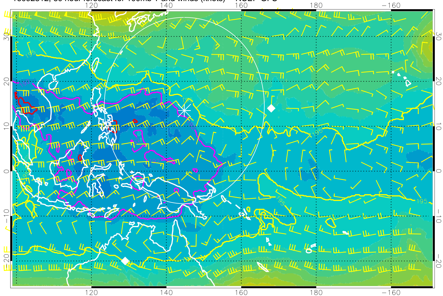
16092312, 60 hour forecast for 100mb T and winds (knots) -- NCEP GFS
