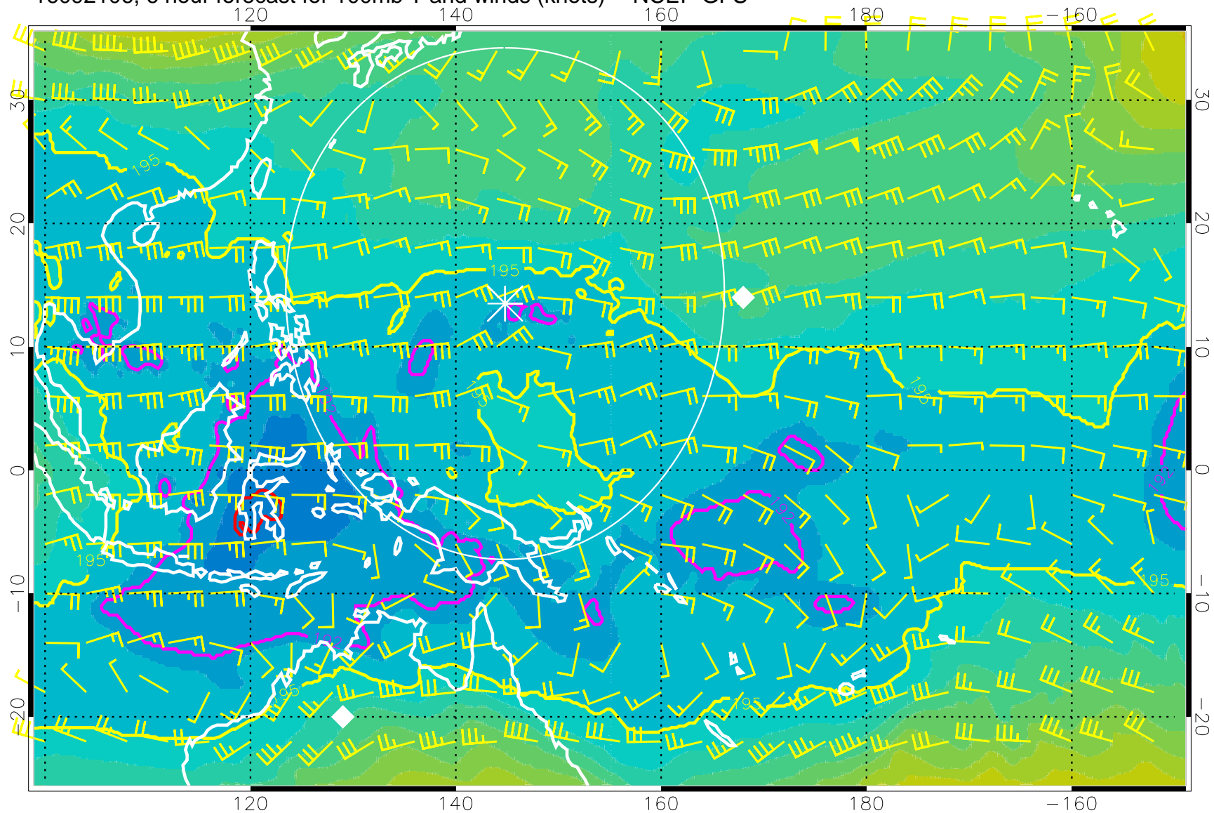
16092106, 6 hour forecast for 100mb T and winds (knots) -- NCEP GFS
