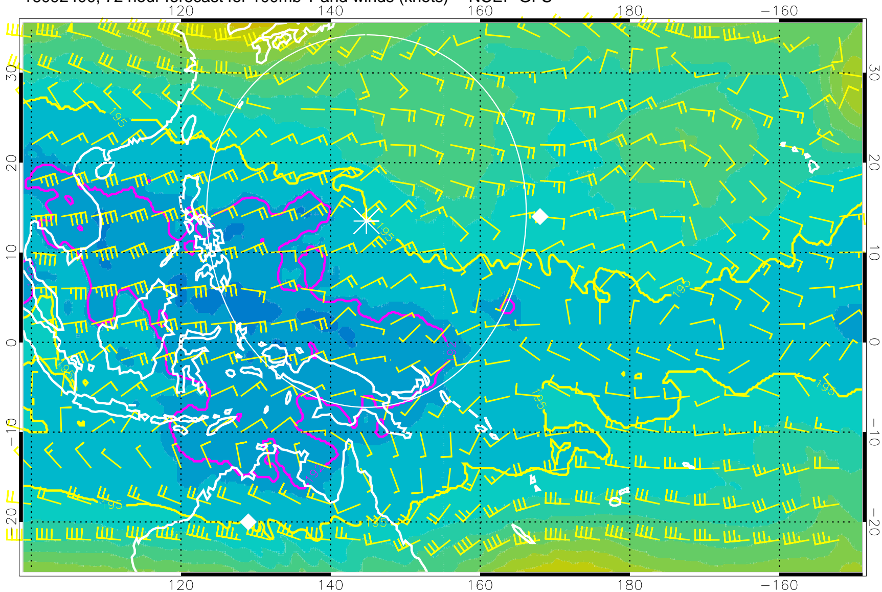
16092400, 72 hour forecast for 100mb T and winds (knots) -- NCEP GFS
