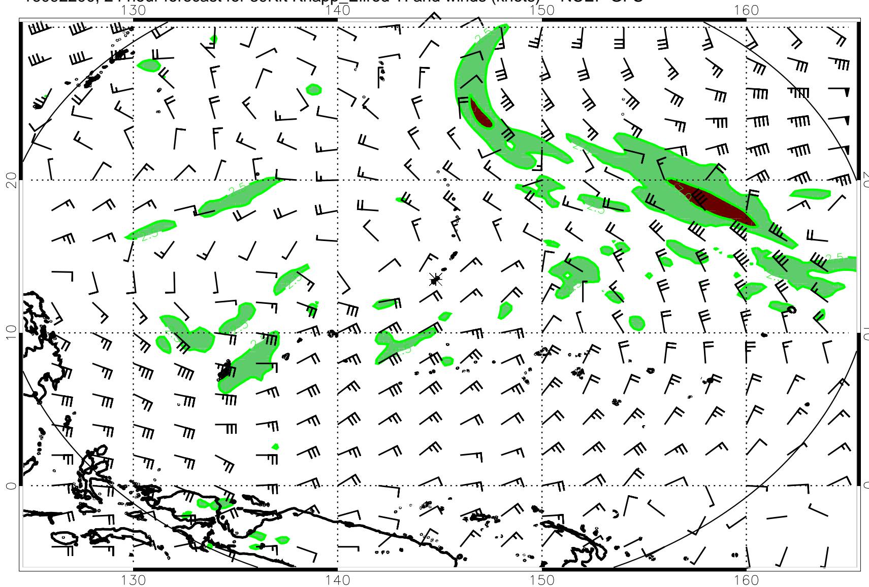
16092200, 24 hour forecast for 39Kft Knapp_Ellrod TI and winds (knots) -- NCEP GFS
