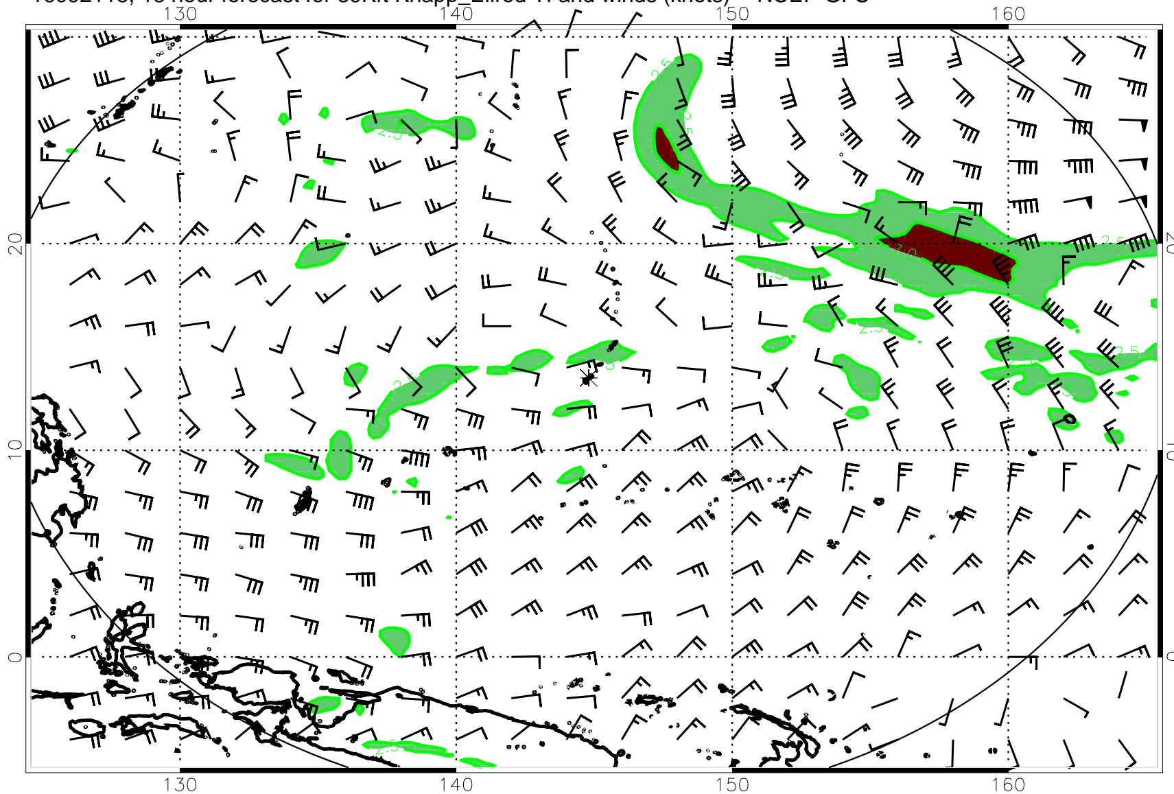
16092118, 18 hour forecast for 39Kft Knapp_Ellrod TI and winds (knots) -- NCEP GFS
