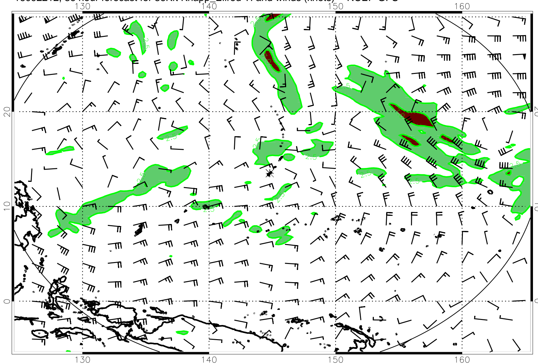
16092212, 36 hour forecast for 36Kft Knapp_Ellrod TI and winds (knots) -- NCEP GFS
