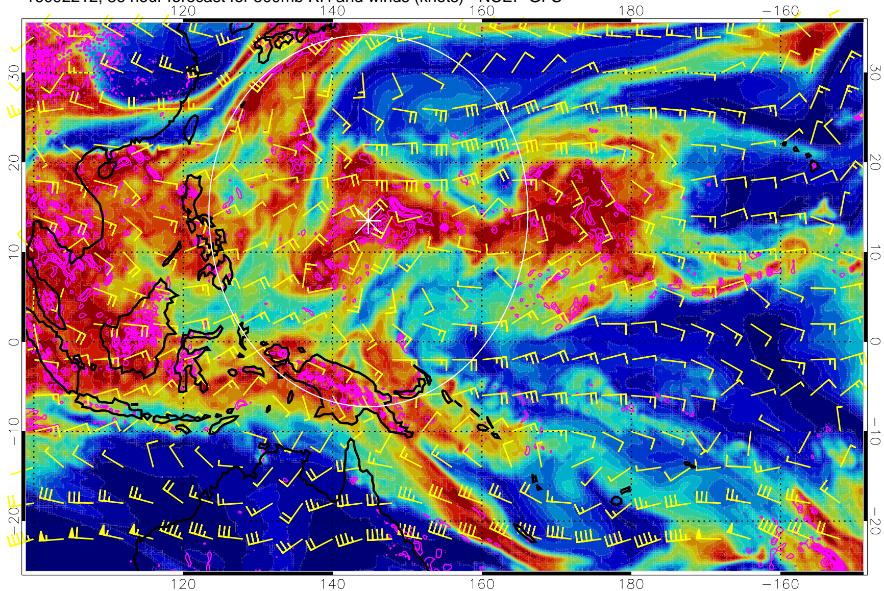
16092212, 36 hour forecast for 500mb RH and winds (knots) - NCEP GFS
