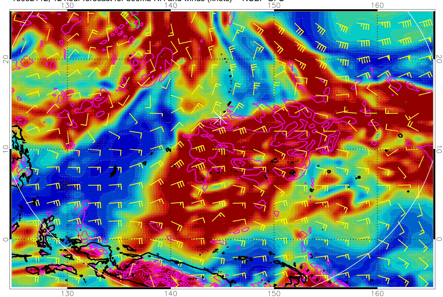
16092112, 12 hour forecast for 300mb RH and winds (knots) -- NCEP GFS
