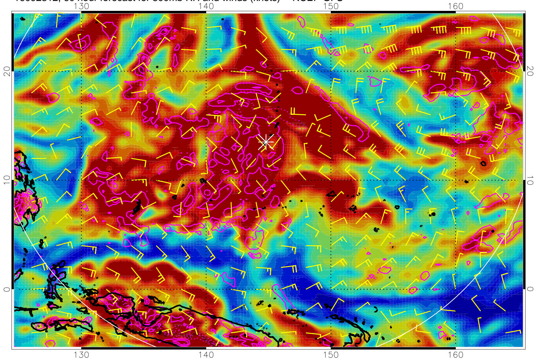
16092312, 60 hour forecast for 300mb RH and winds (knots) -- NCEP GFS
