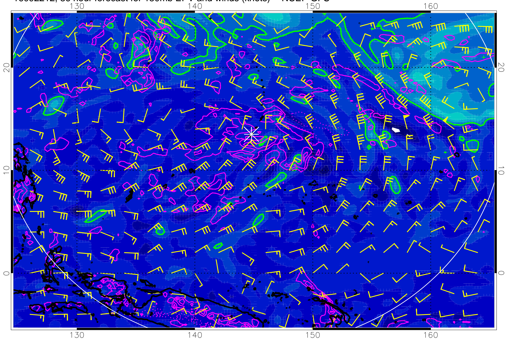
16092212, 36 hour forecast for 150mb EPV and winds (knots) -- NCEP GFS
