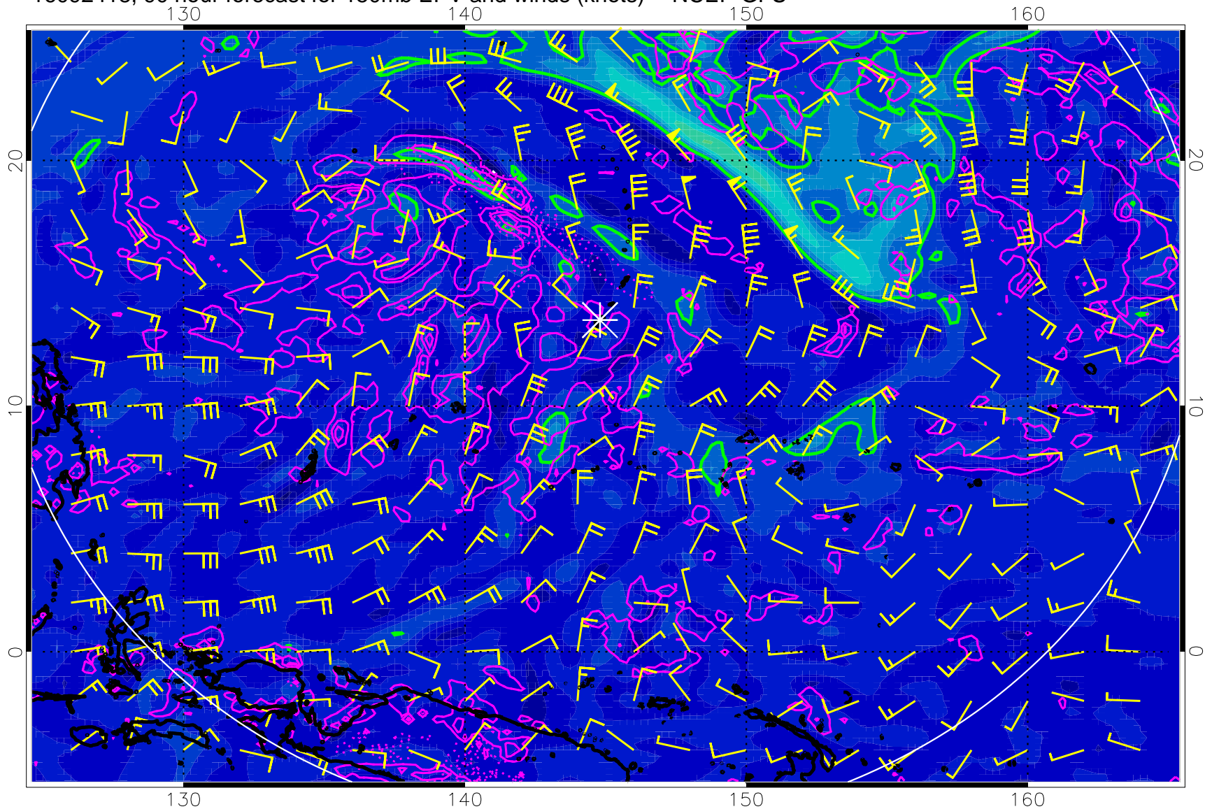
16092418, 90 hour forecast for 150mb EPV and winds (knots) -- NCEP GFS
