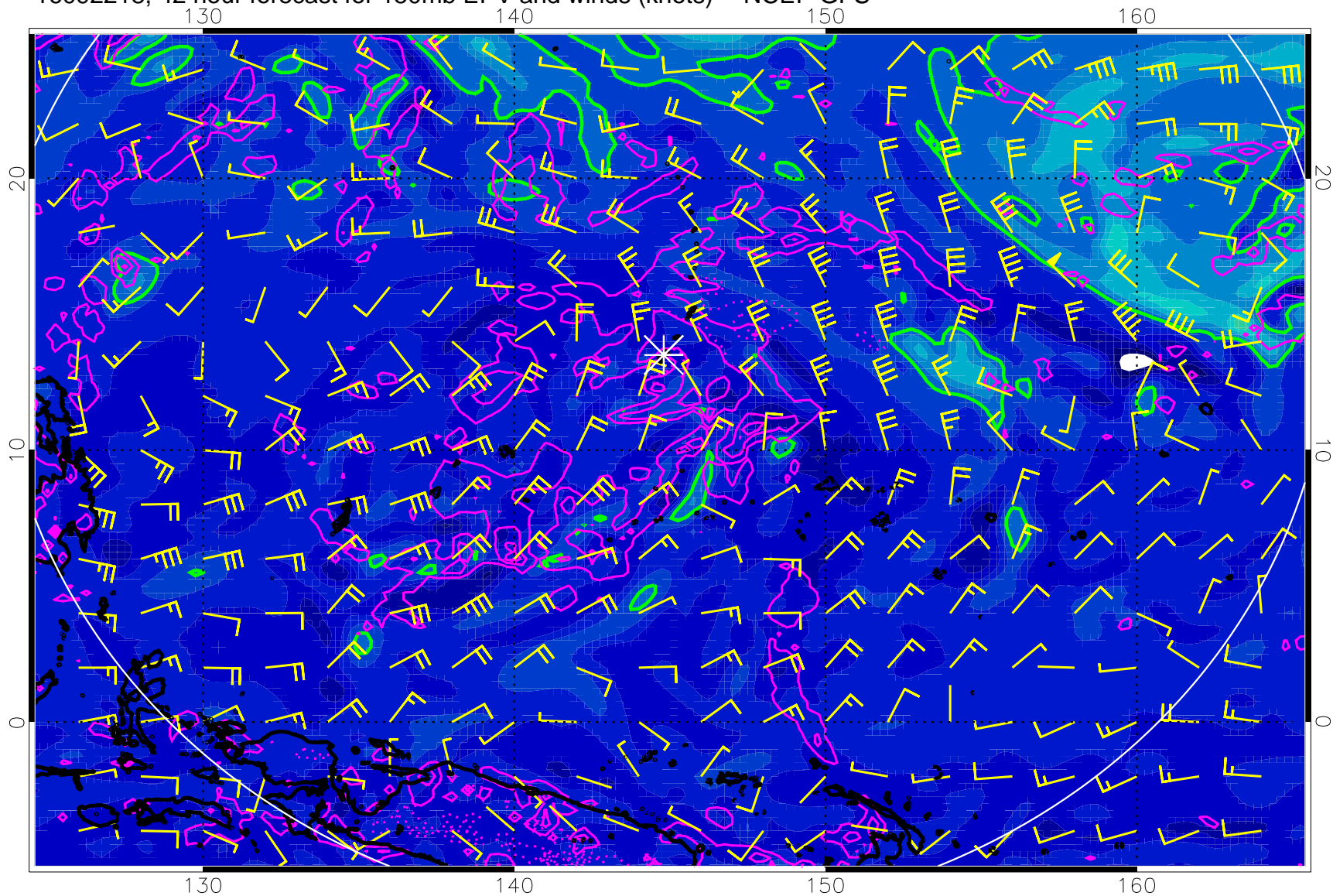
16092218, 42 hour forecast for 150mb EPV and winds (knots) -- NCEP GFS
