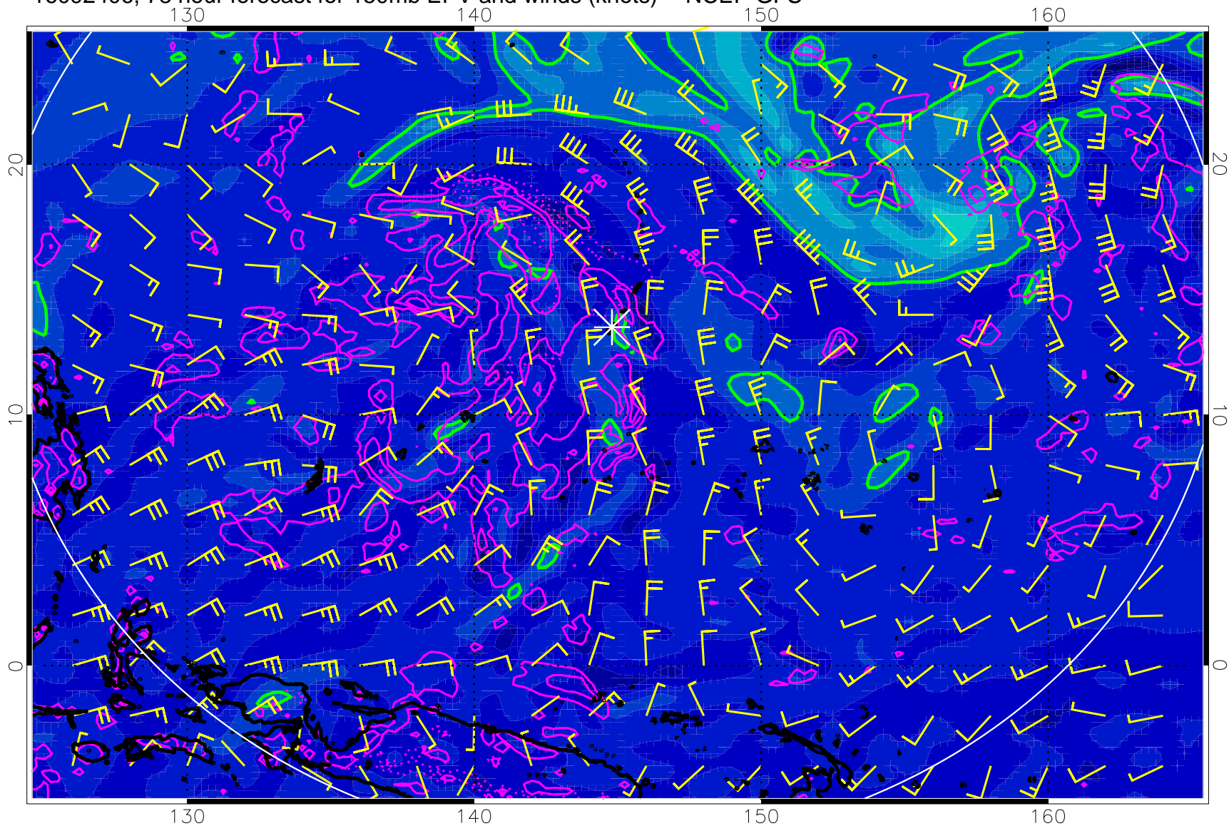
16092406, 78 hour forecast for 150mb EPV and winds (knots) -- NCEP GFS
