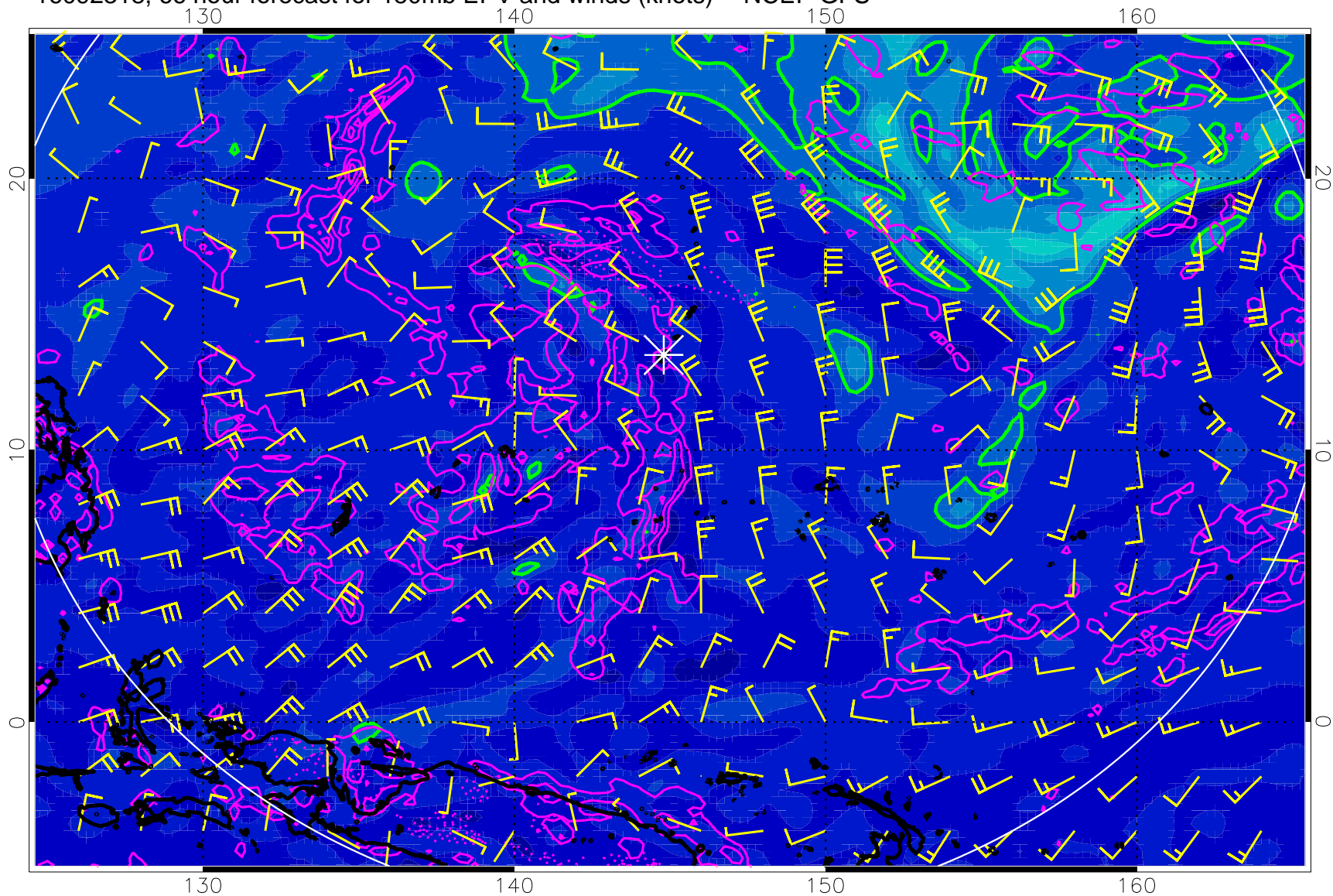
16092318, 66 hour forecast for 150mb EPV and winds (knots) -- NCEP GFS
