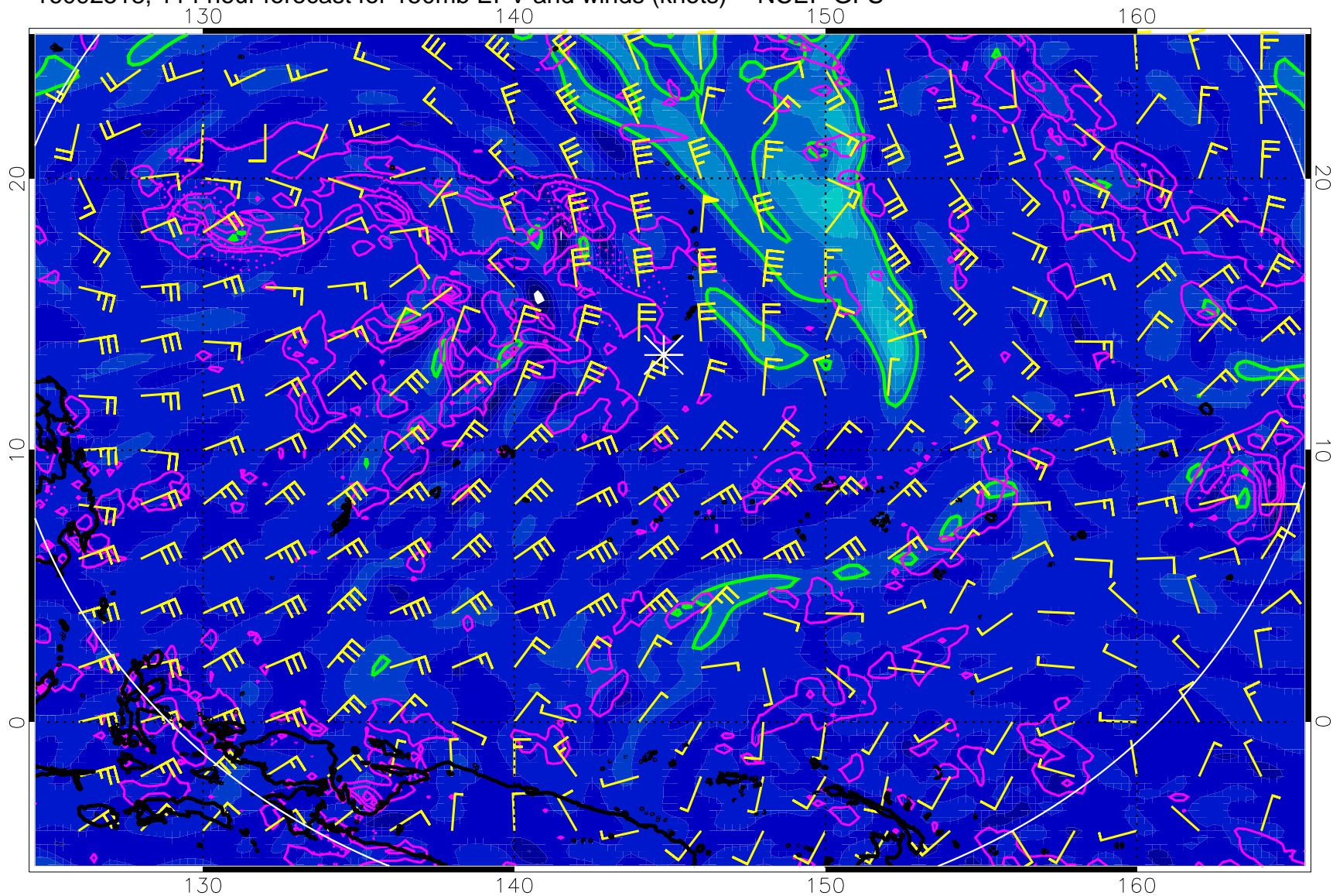
16092518, 114 hour forecast for 150mb EPV and winds (knots) -- NCEP GFS
