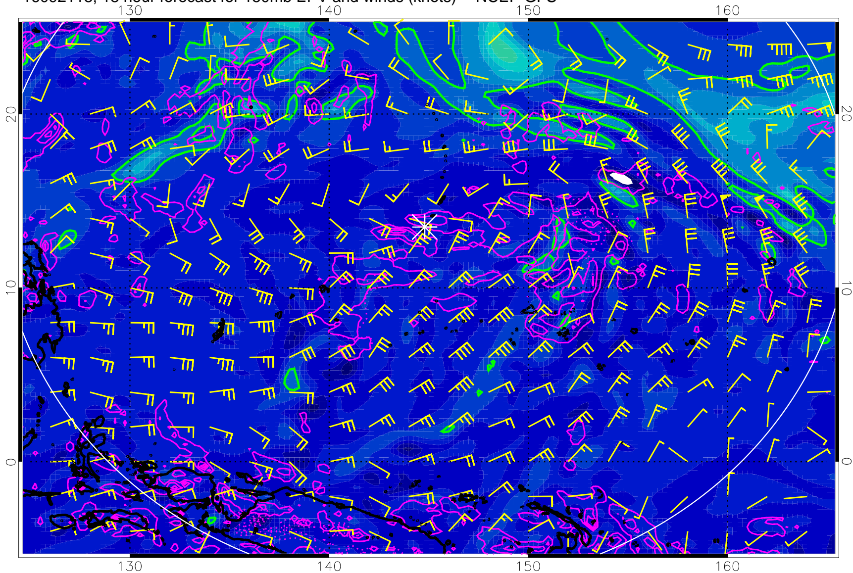
16092118, 18 hour forecast for 150mb EPV and winds (knots) -- NCEP GFS
