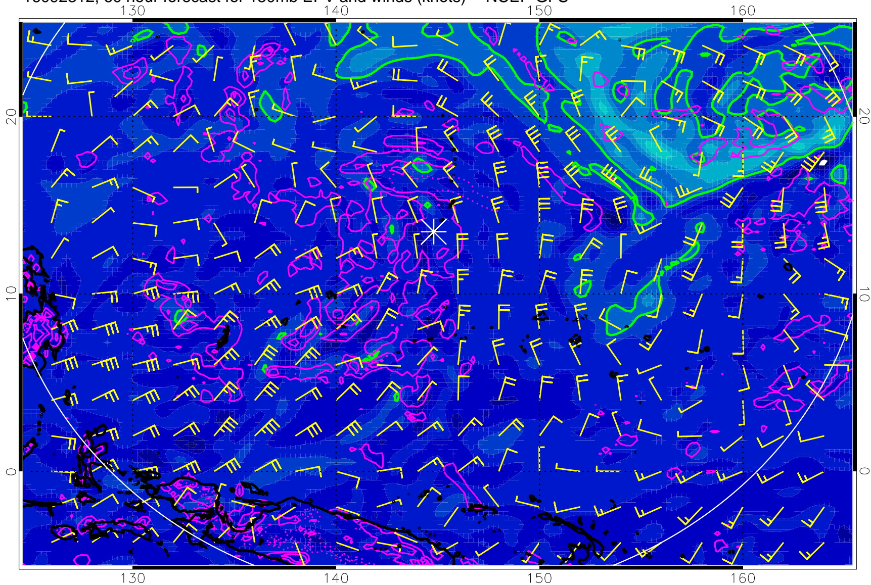
16092312, 60 hour forecast for 150mb EPV and winds (knots) -- NCEP GFS
