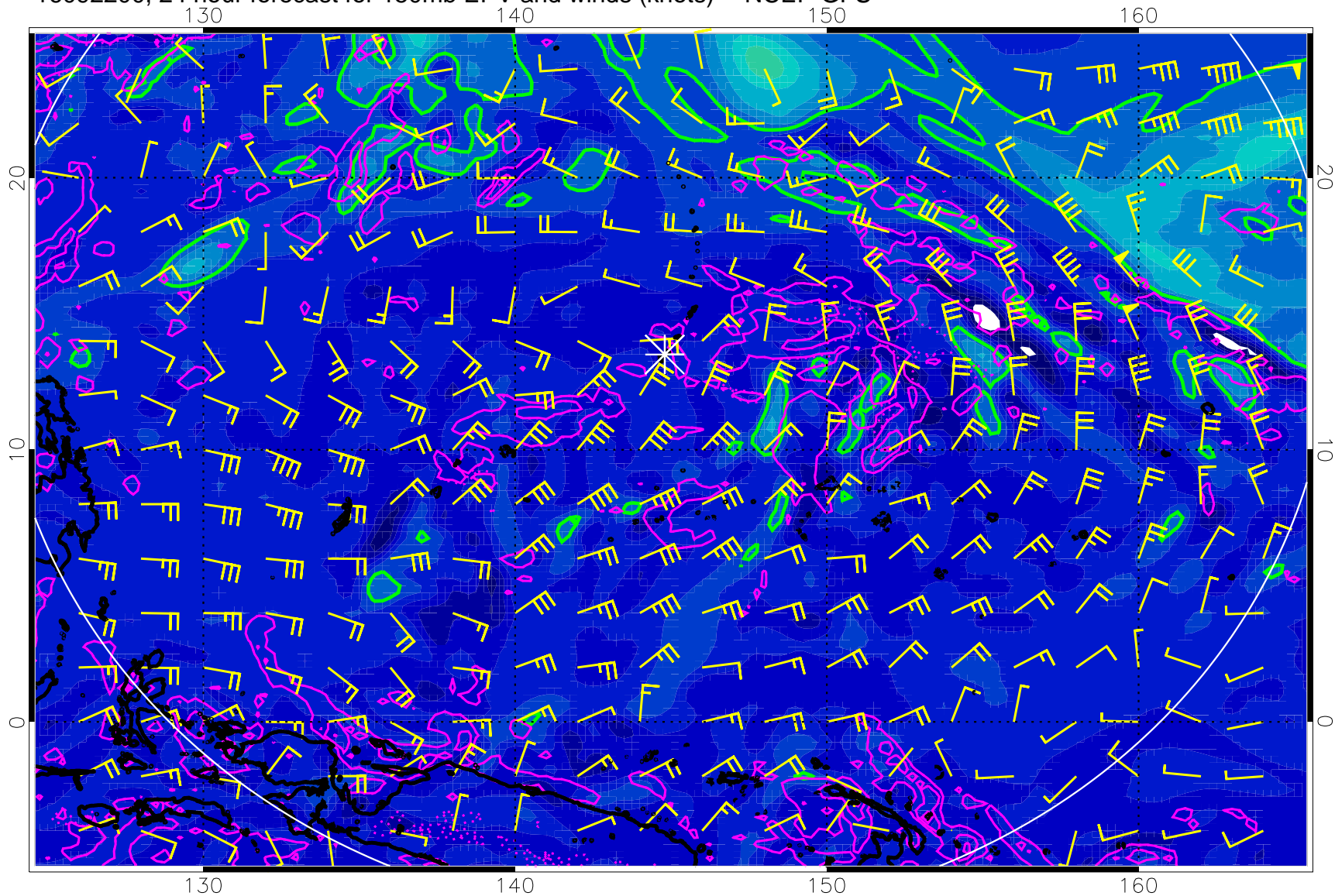
16092200, 24 hour forecast for 150mb EPV and winds (knots) -- NCEP GFS
