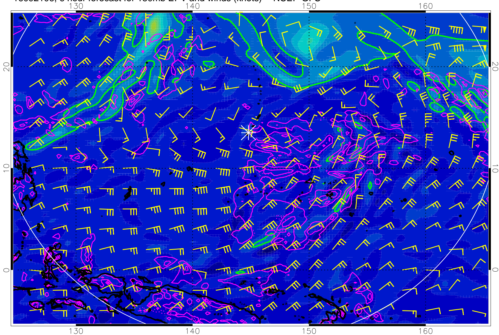
16092106, 6 hour forecast for 150mb EPV and winds (knots) -- NCEP GFS
