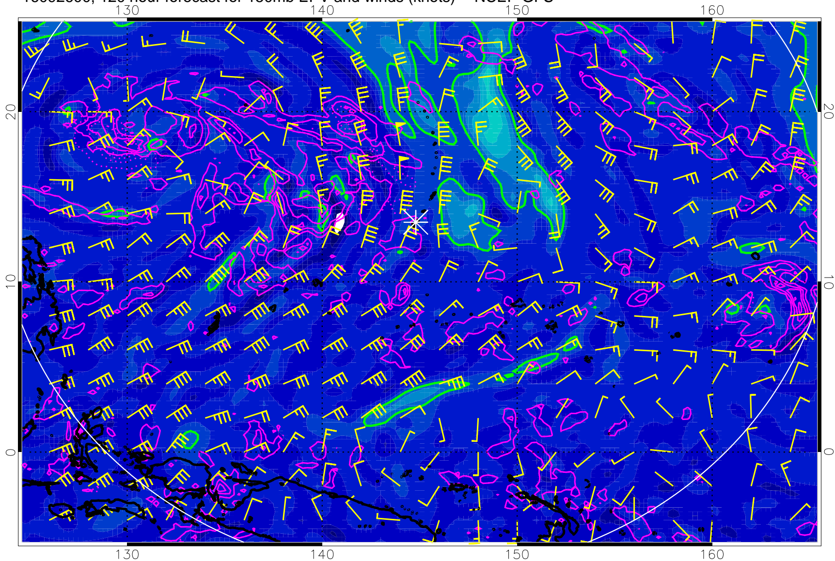
16092600, 120 hour forecast for 150mb EPV and winds (knots) -- NCEP GFS
