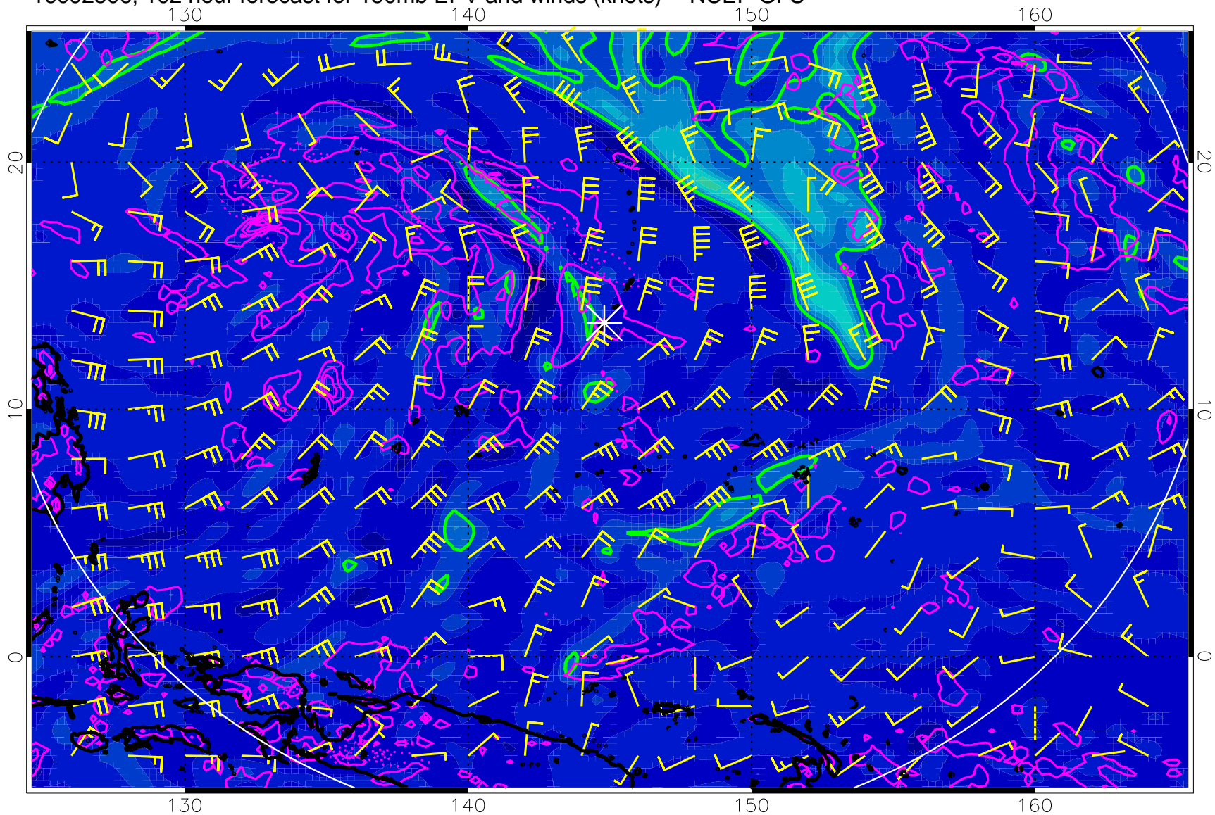
16092506, 102 hour forecast for 150mb EPV and winds (knots) -- NCEP GFS
