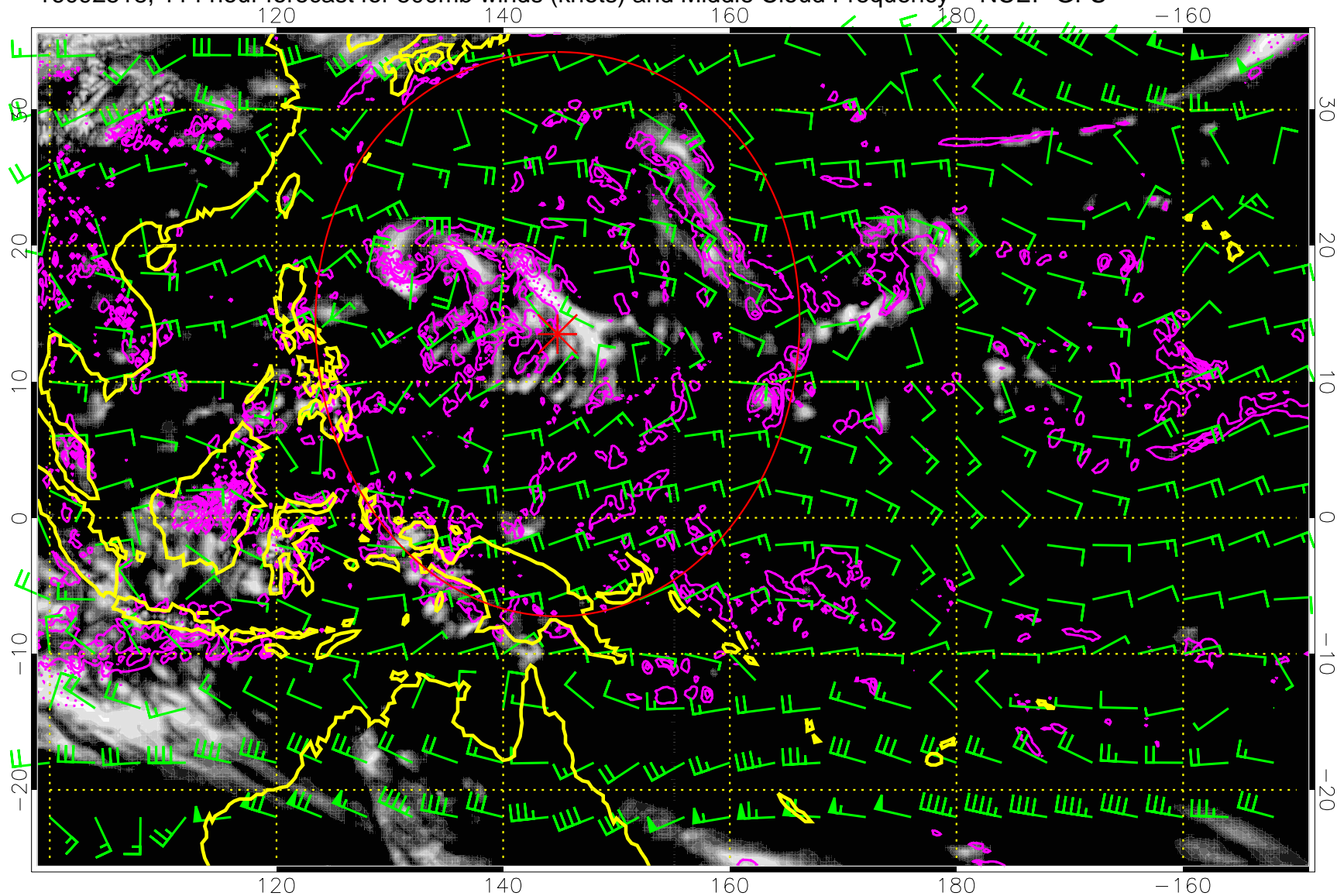
16092518, 114 hour forecast for 500mb winds (knots) and Middle Cloud Frequency -- NCEP GFS
