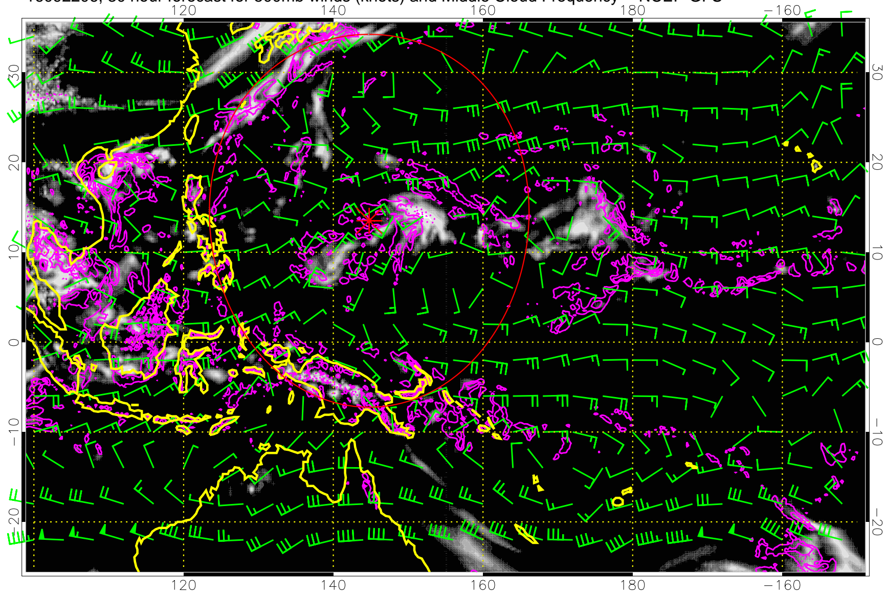
16092206, 30 hour forecast for 500mb winds (knots) and Middle Cloud Frequency -- NCEP GFS
