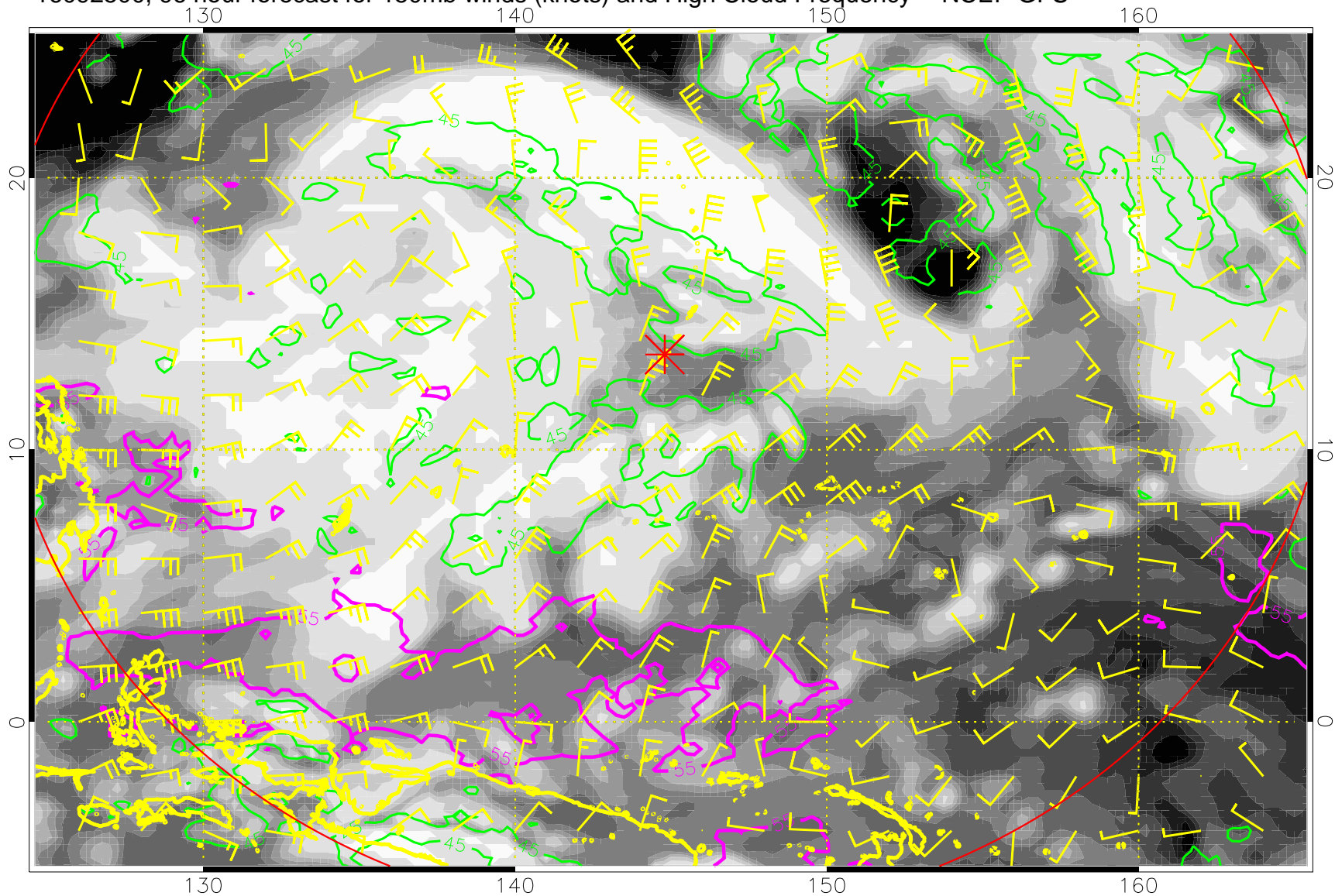
16092500, 96 hour forecast for 150mb winds (knots) and High Cloud Frequency -- NCEP GFS
