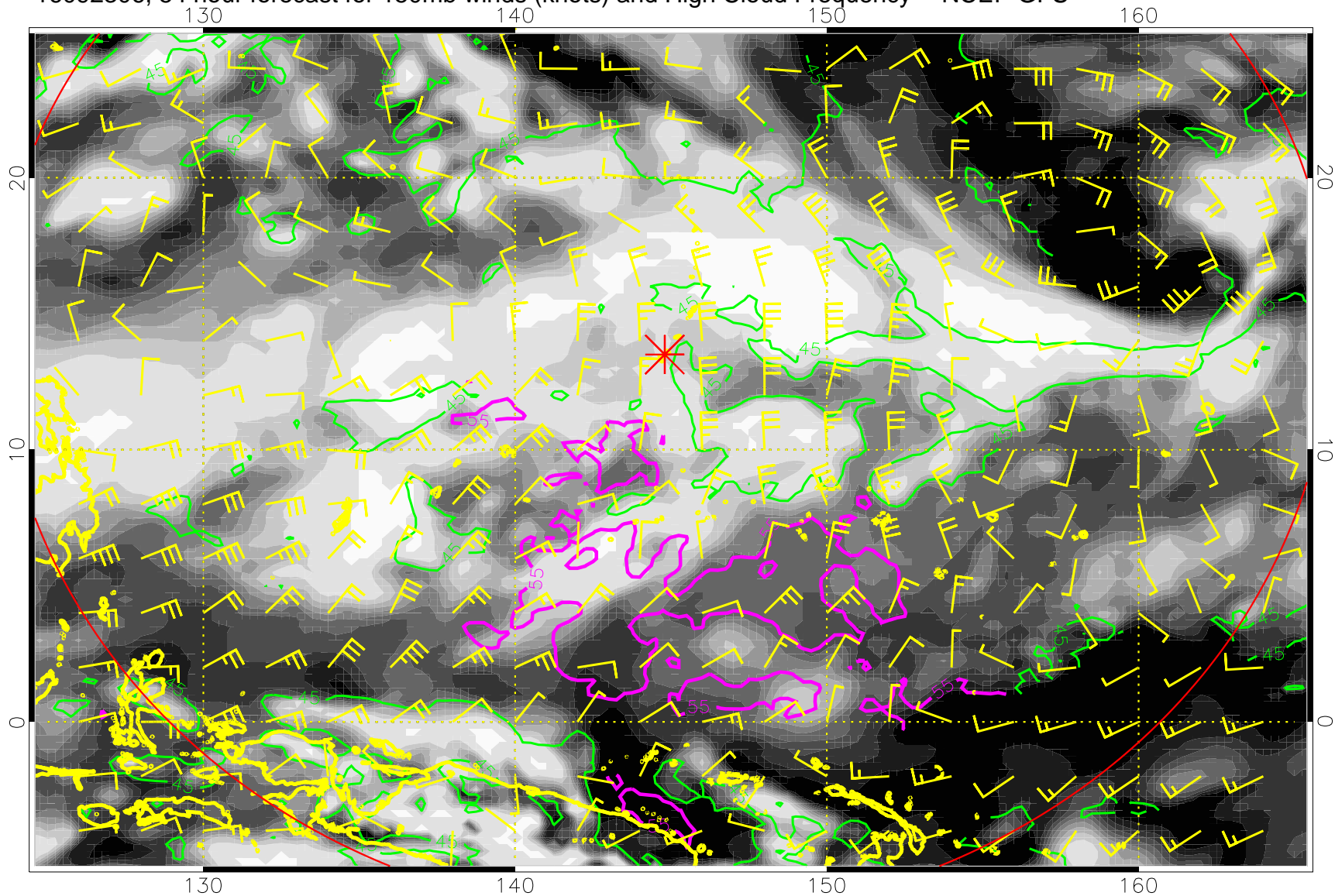
16092306, 54 hour forecast for 150mb winds (knots) and High Cloud Frequency -- NCEP GFS
