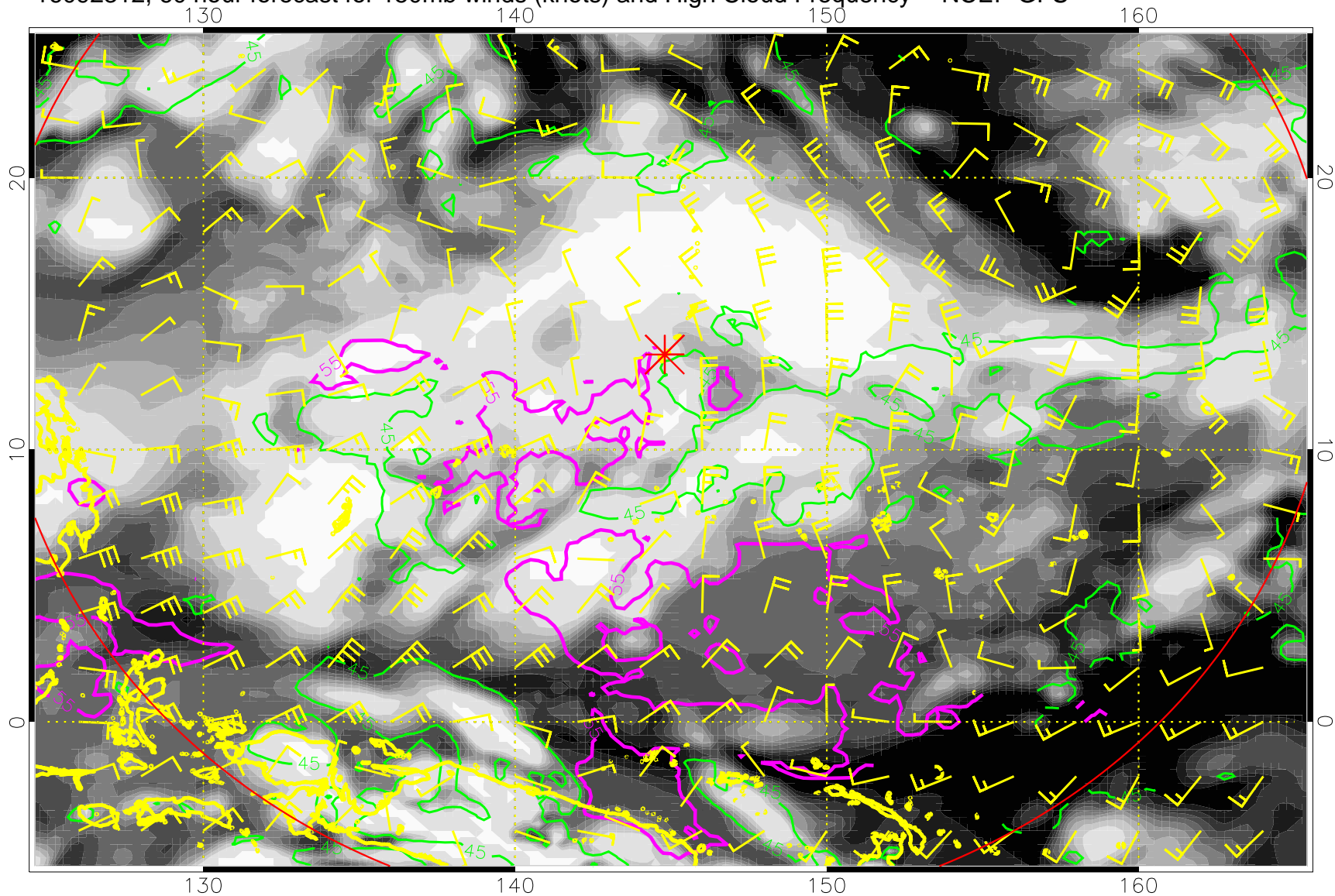
16092312, 60 hour forecast for 150mb winds (knots) and High Cloud Frequency -- NCEP GFS
