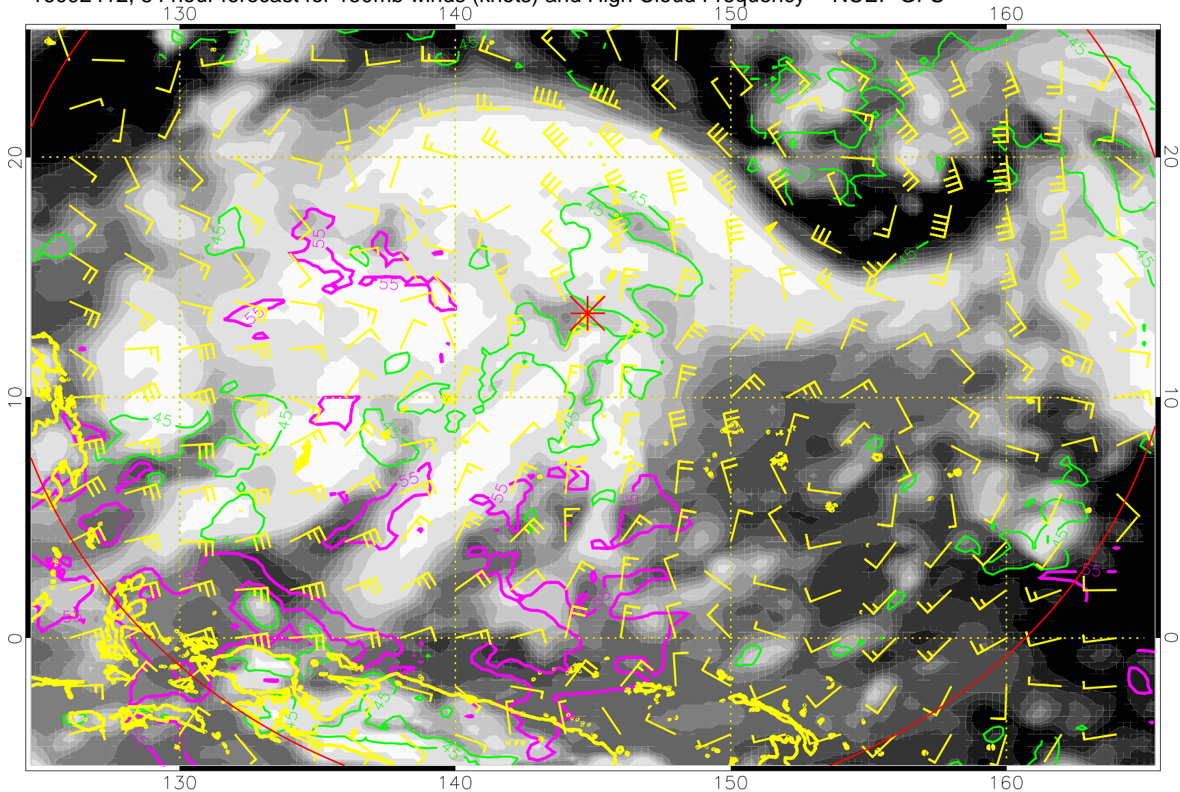
16092412, 84 hour forecast for 150mb winds (knots) and High Cloud Frequency -- NCEP GFS
