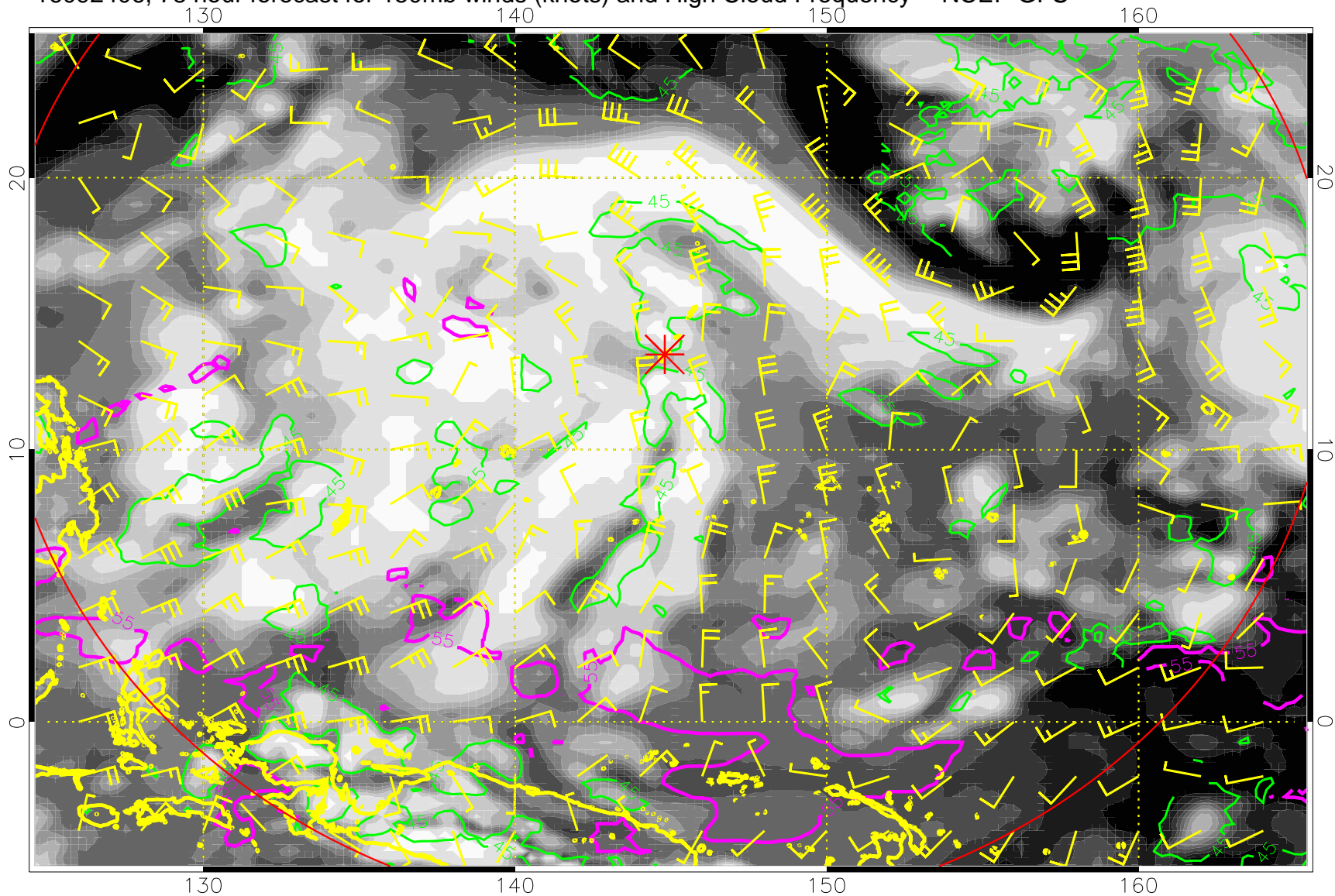
16092406, 78 hour forecast for 150mb winds (knots) and High Cloud Frequency -- NCEP GFS
