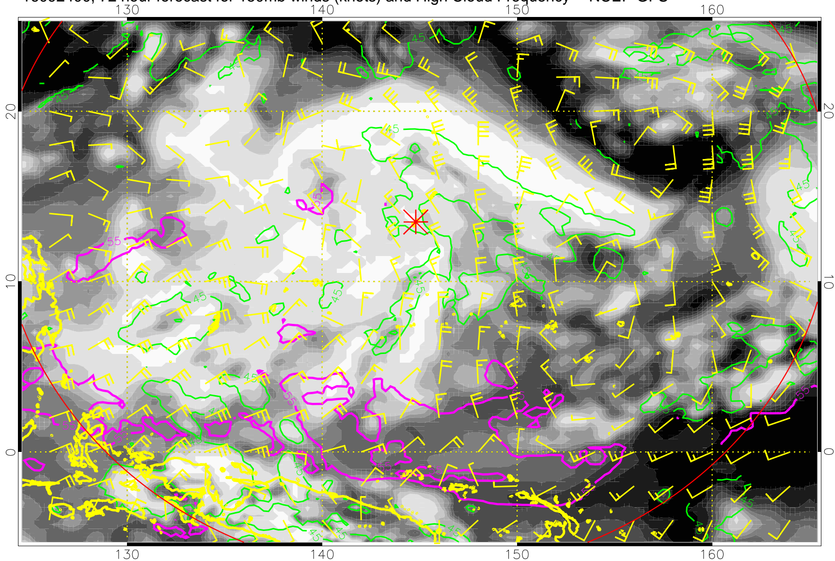
16092400, 72 hour forecast for 150mb winds (knots) and High Cloud Frequency -- NCEP GFS
