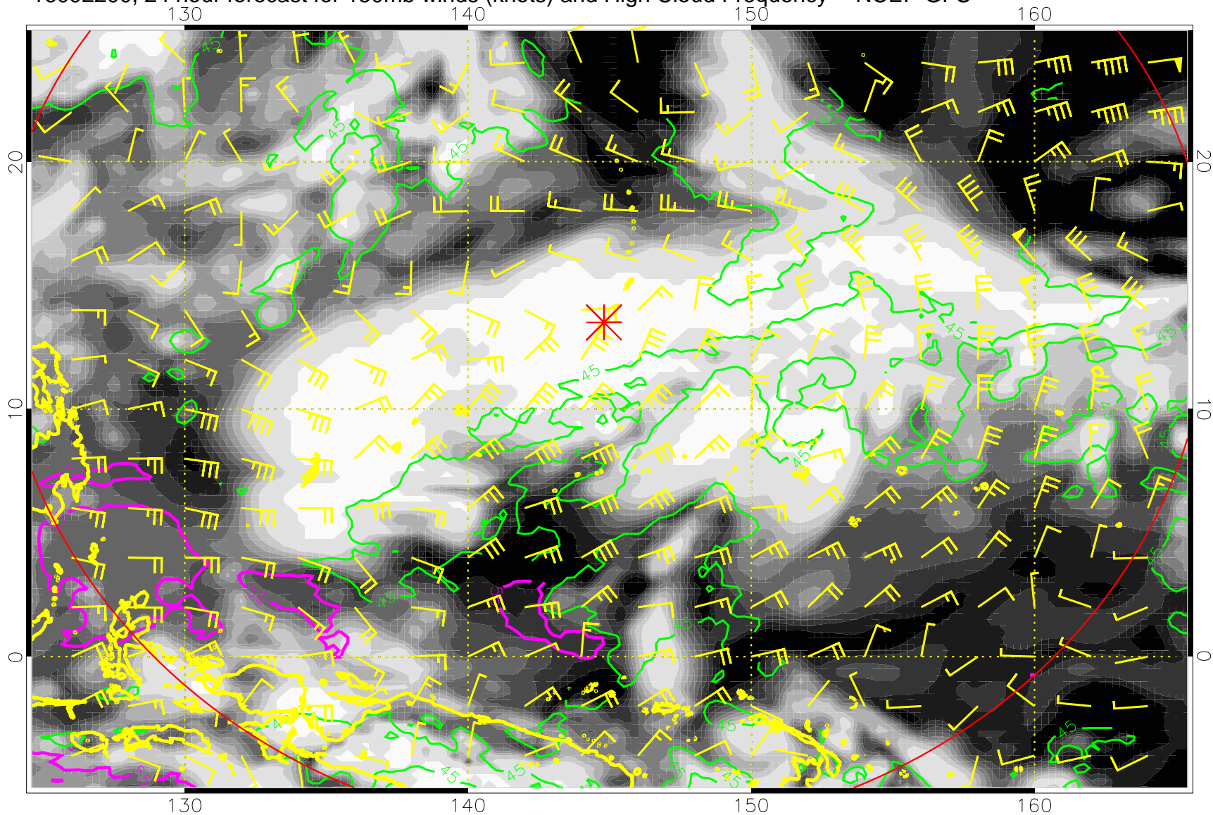
16092200, 24 hour forecast for 150mb winds (knots) and High Cloud Frequency -- NCEP GFS
