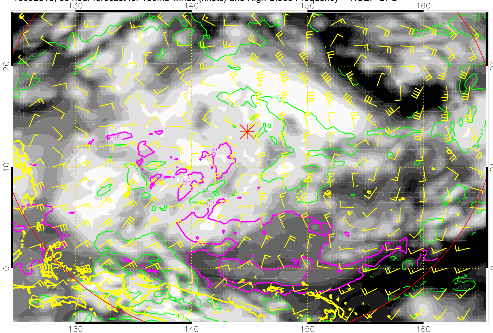
16092318, 66 hour forecast for 150mb winds (knots) and High Cloud Frequency -- NCEP GFS
