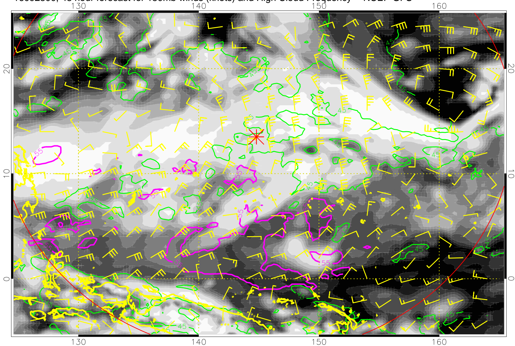
16092300, 48 hour forecast for 150mb winds (knots) and High Cloud Frequency -- NCEP GFS
