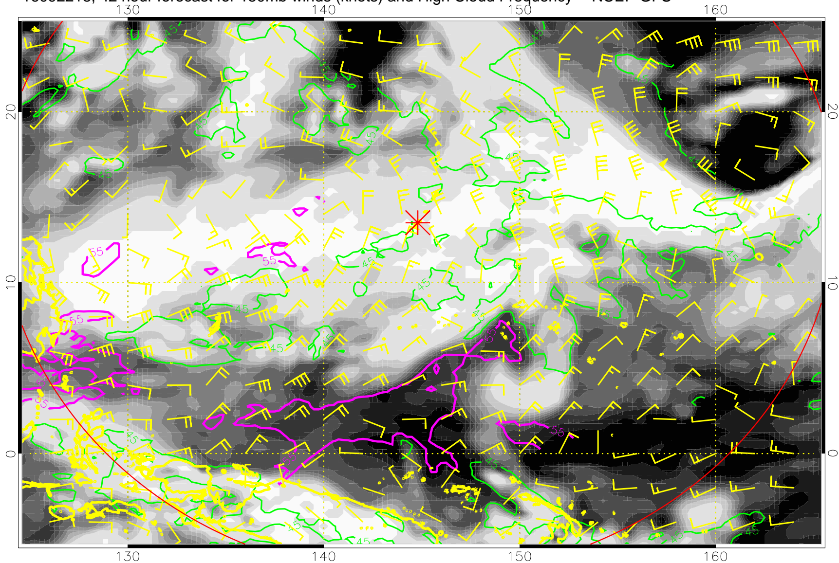
16092218, 42 hour forecast for 150mb winds (knots) and High Cloud Frequency -- NCEP GFS
