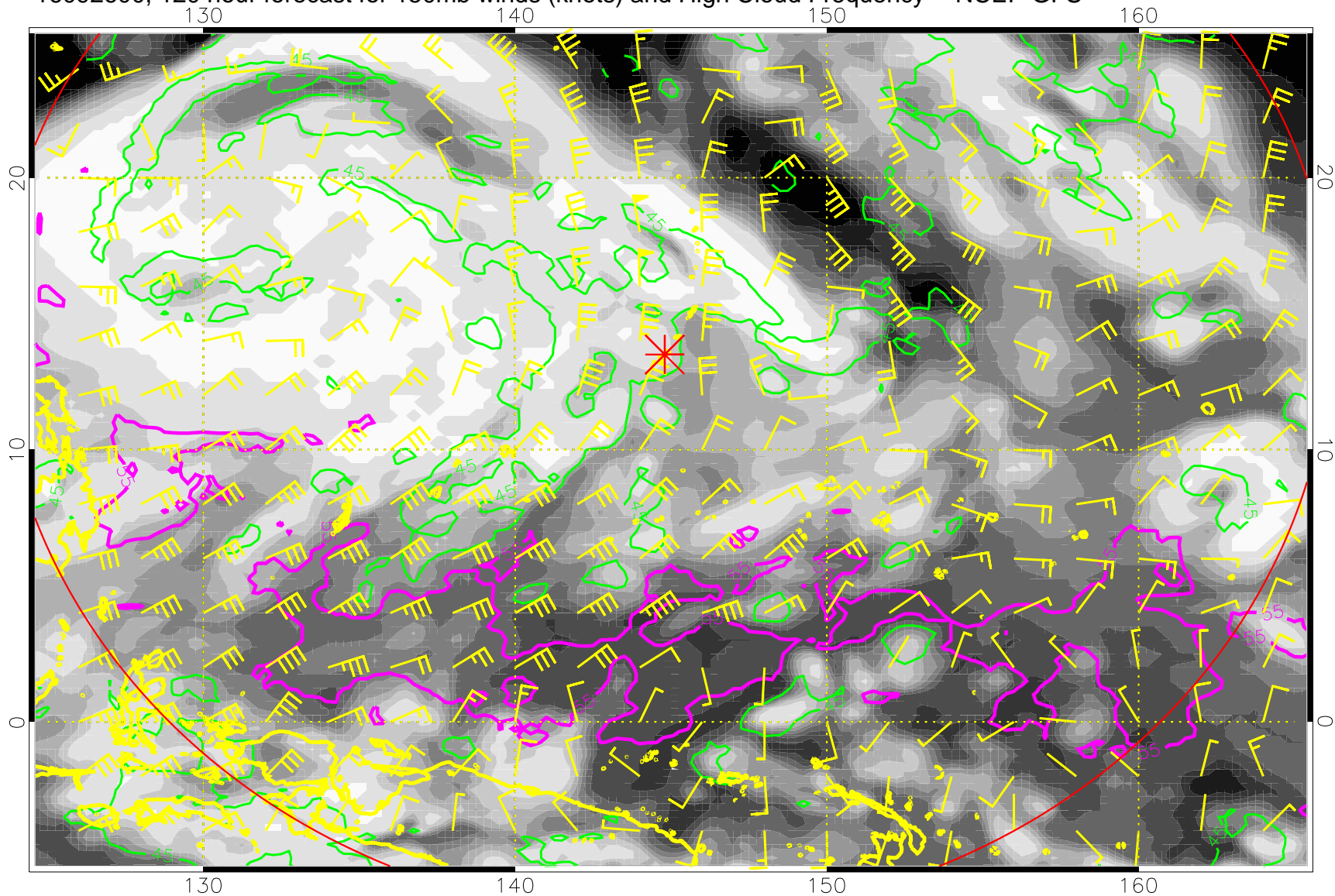
16092600, 120 hour forecast for 150mb winds (knots) and High Cloud Frequency -- NCEP GFS
