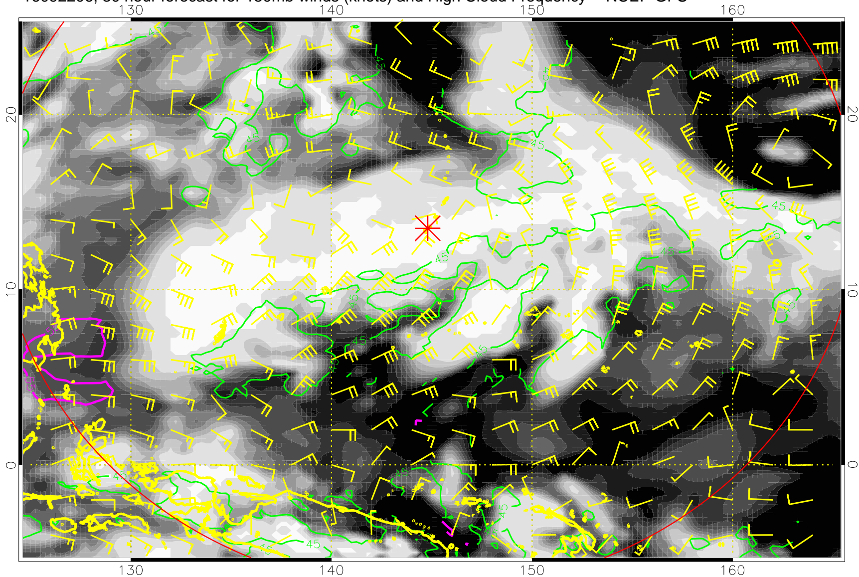
16092206, 30 hour forecast for 150mb winds (knots) and High Cloud Frequency -- NCEP GFS
