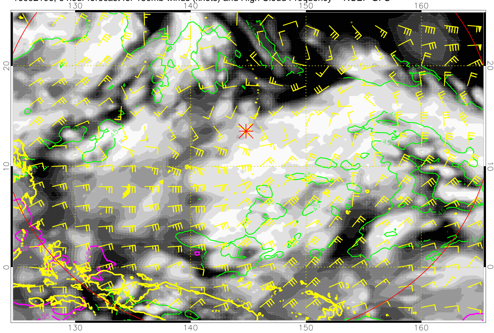
16092106, 6 hour forecast for 150mb winds (knots) and High Cloud Frequency -- NCEP GFS
