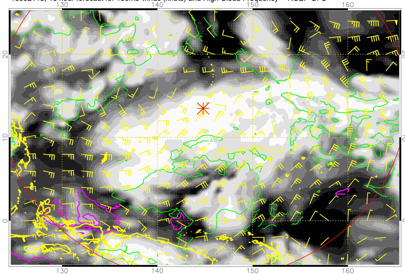
16092118, 18 hour forecast for 150mb winds (knots) and High Cloud Frequency -- NCEP GFS
