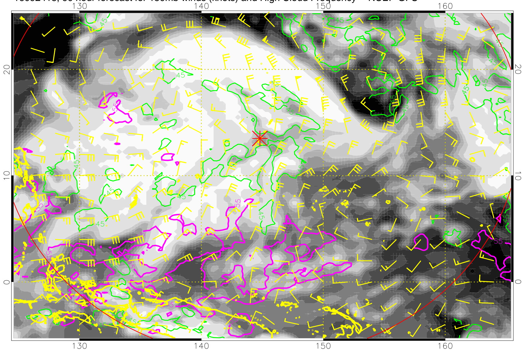
16092418, 90 hour forecast for 150mb winds (knots) and High Cloud Frequency -- NCEP GFS
