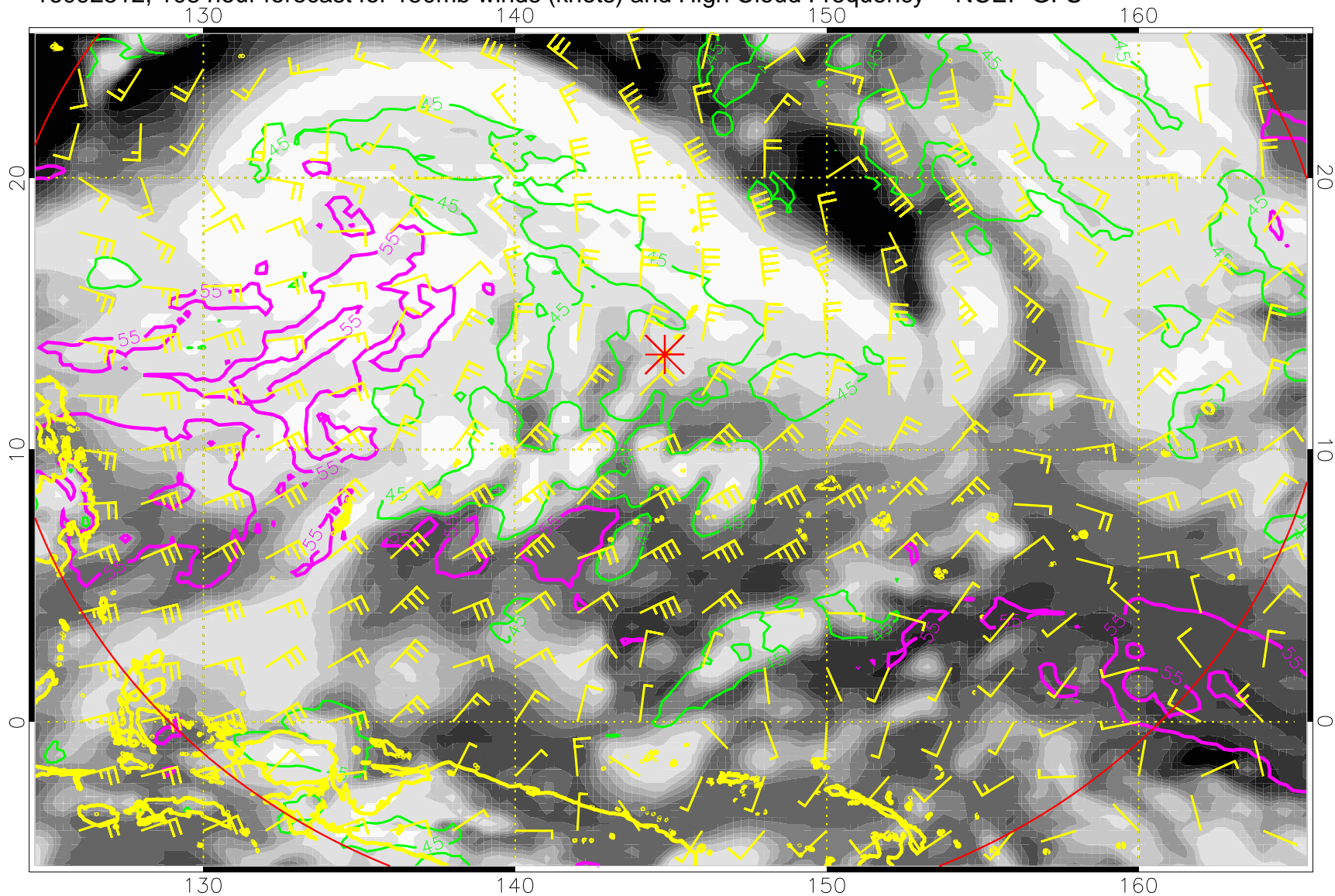
16092512, 108 hour forecast for 150mb winds (knots) and High Cloud Frequency -- NCEP GFS
