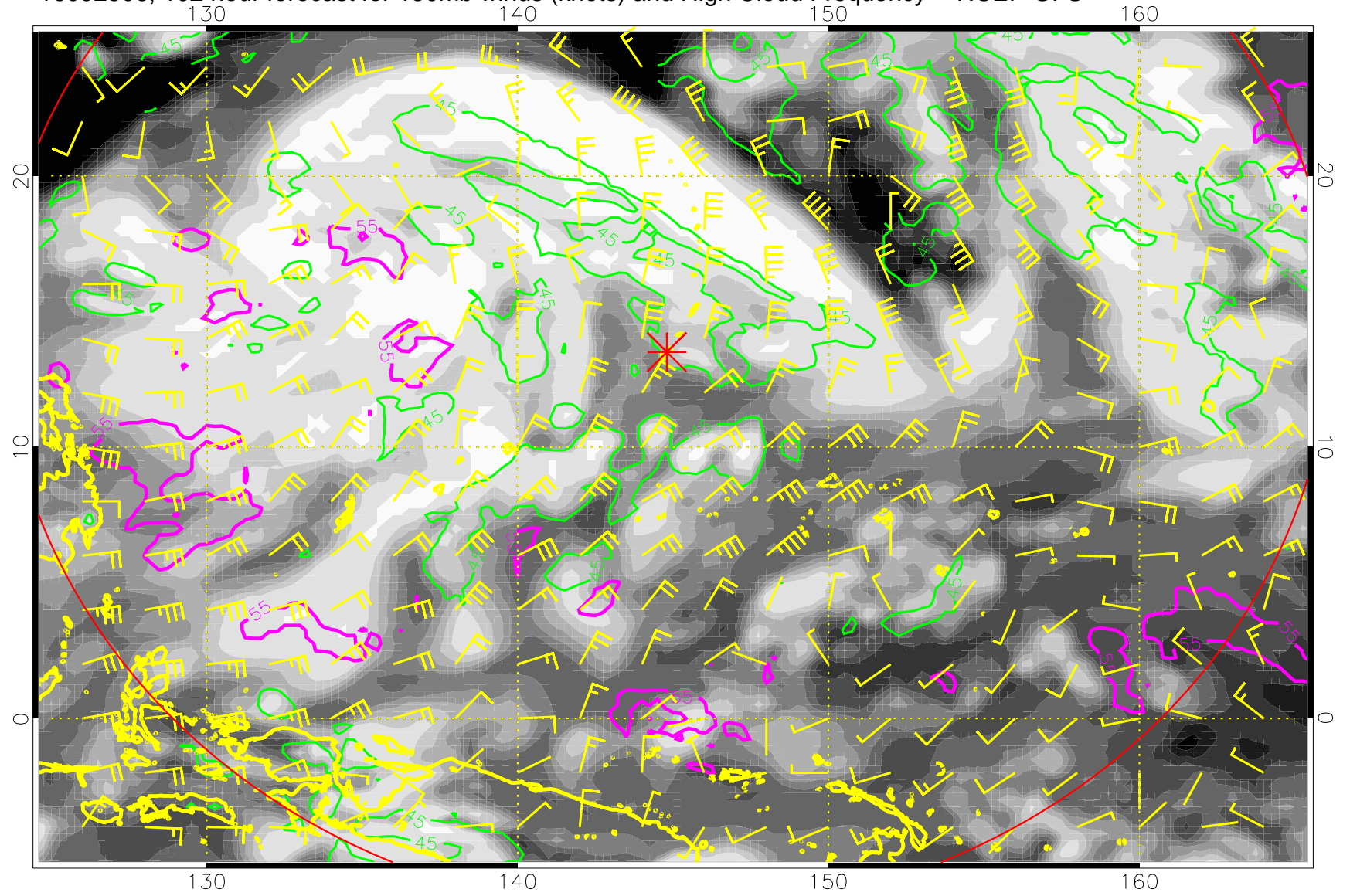
16092506, 102 hour forecast for 150mb winds (knots) and High Cloud Frequency -- NCEP GFS
