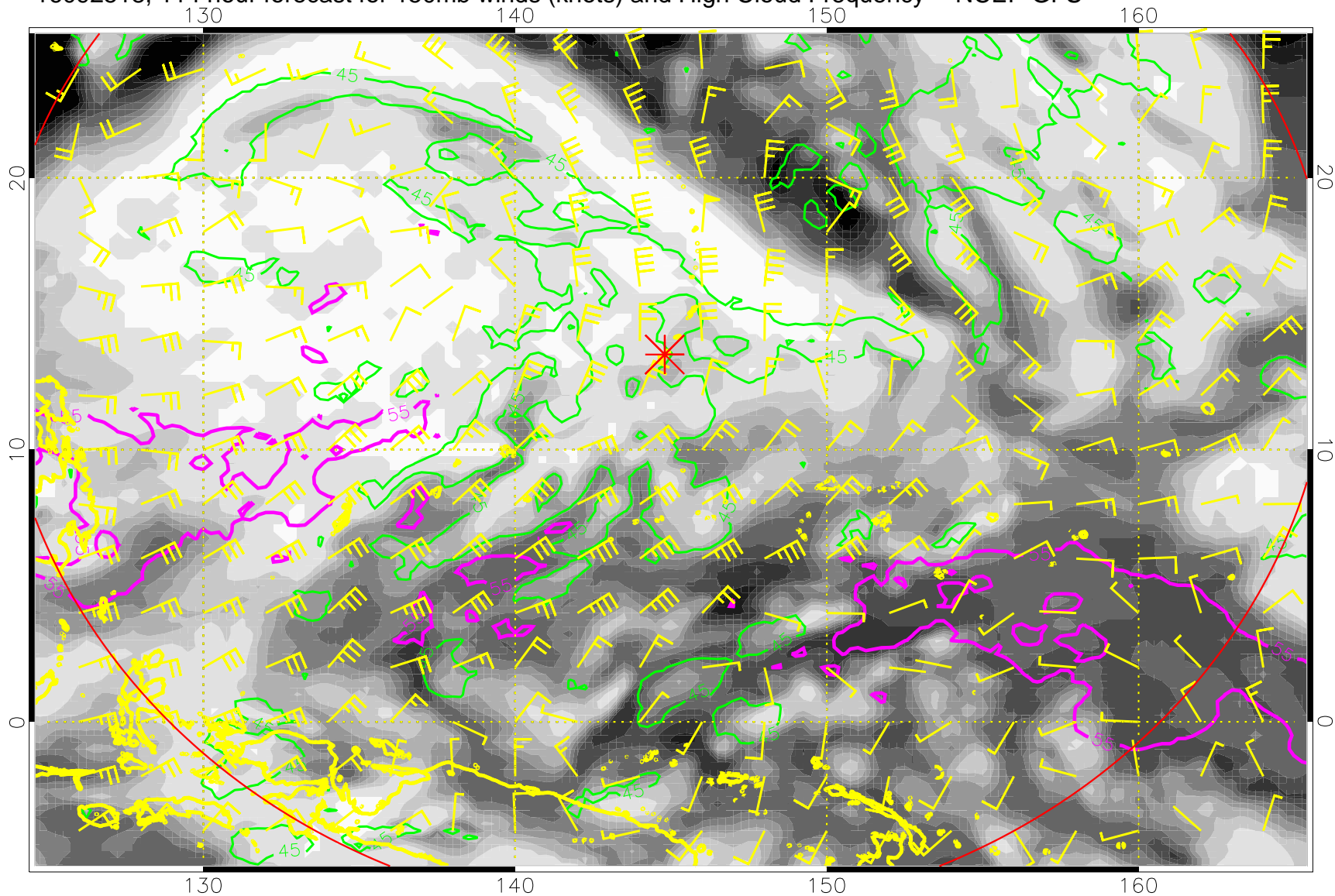
16092518, 114 hour forecast for 150mb winds (knots) and High Cloud Frequency -- NCEP GFS
