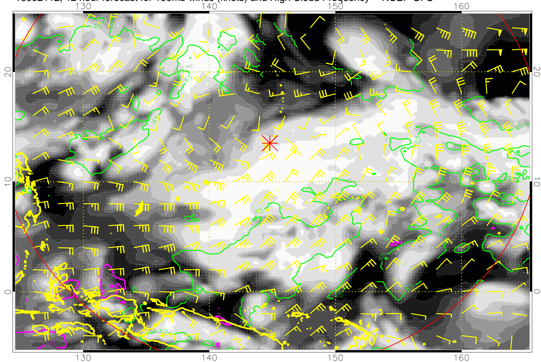
16092112, 12 hour forecast for 150mb winds (knots) and High Cloud Frequency -- NCEP GFS
