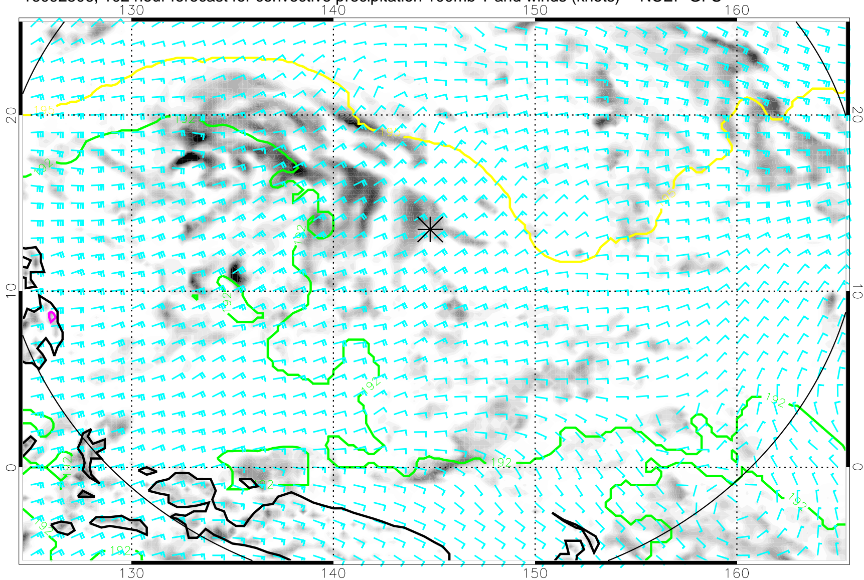
16092506, 102 hour forecast for convective precipitation 100mb T and winds (knots) -- NCEP GFS
