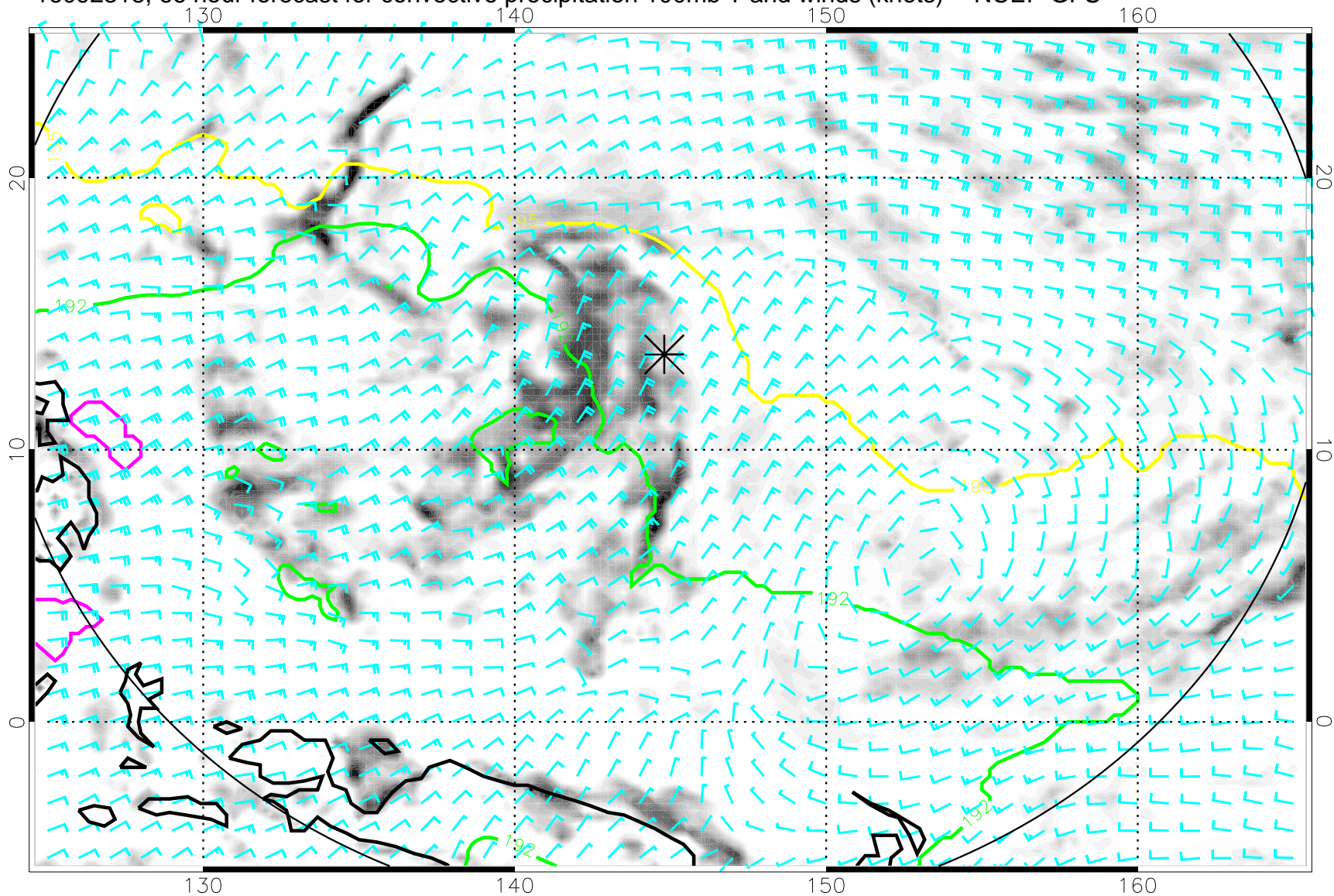
16092318, 66 hour forecast for convective precipitation 100mb T and winds (knots) -- NCEP GFS
