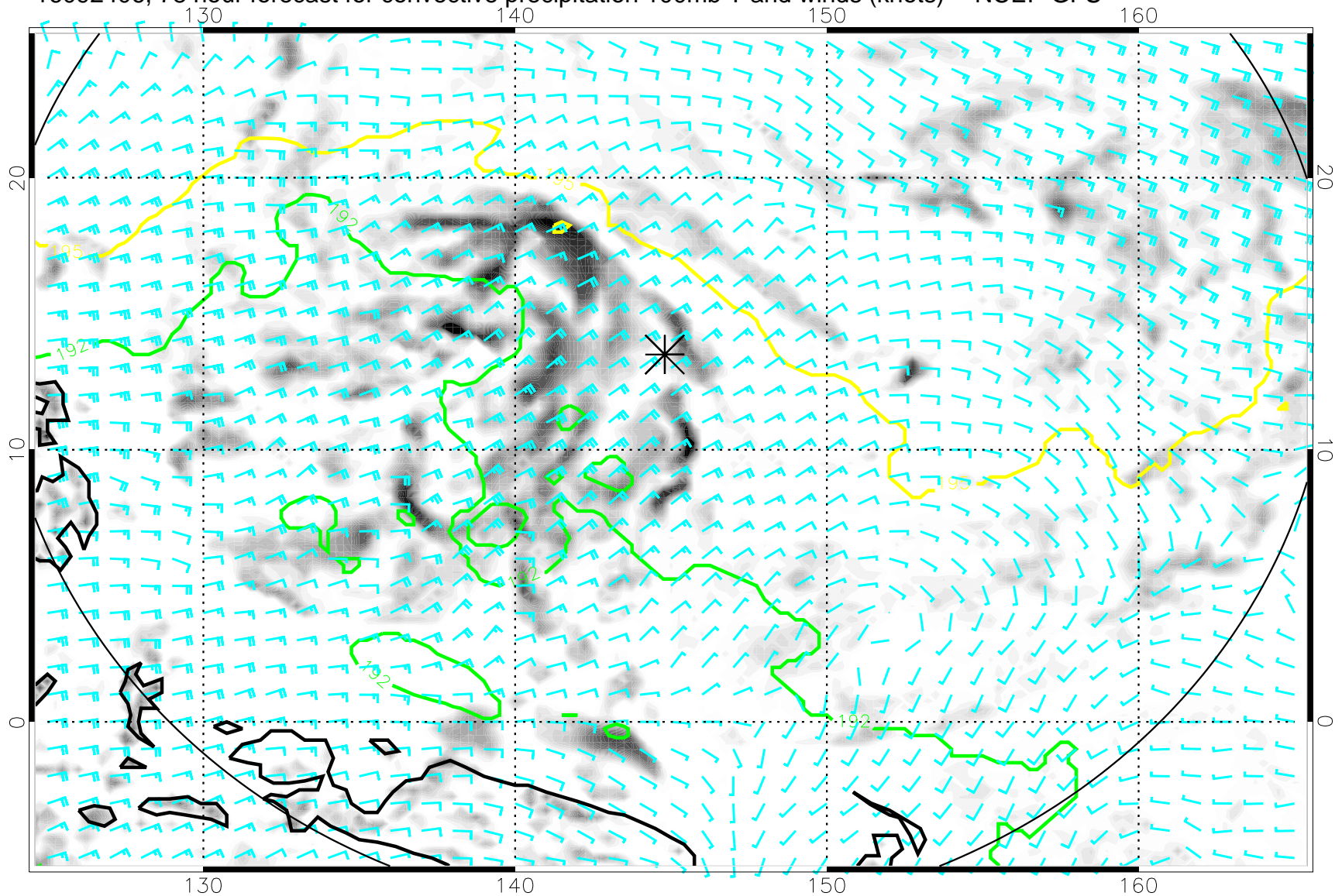
16092406, 78 hour forecast for convective precipitation 100mb T and winds (knots) -- NCEP GFS
