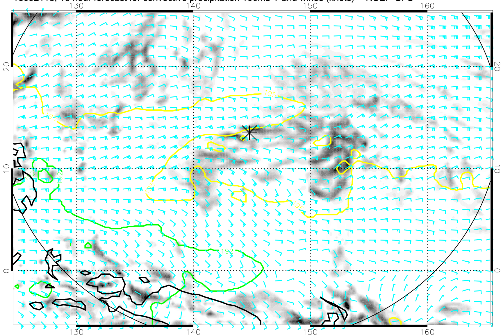
16092118, 18 hour forecast for convective precipitation 100mb T and winds (knots) -- NCEP GFS
