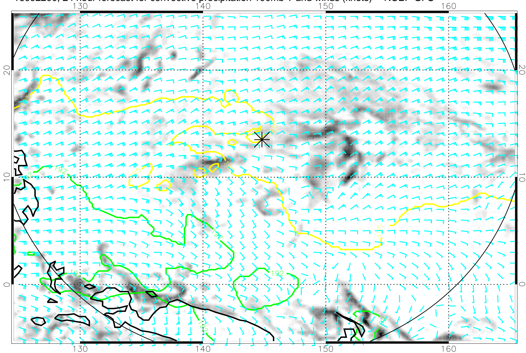
16092200, 24 hour forecast for convective precipitation 100mb T and winds (knots) -- NCEP GFS
