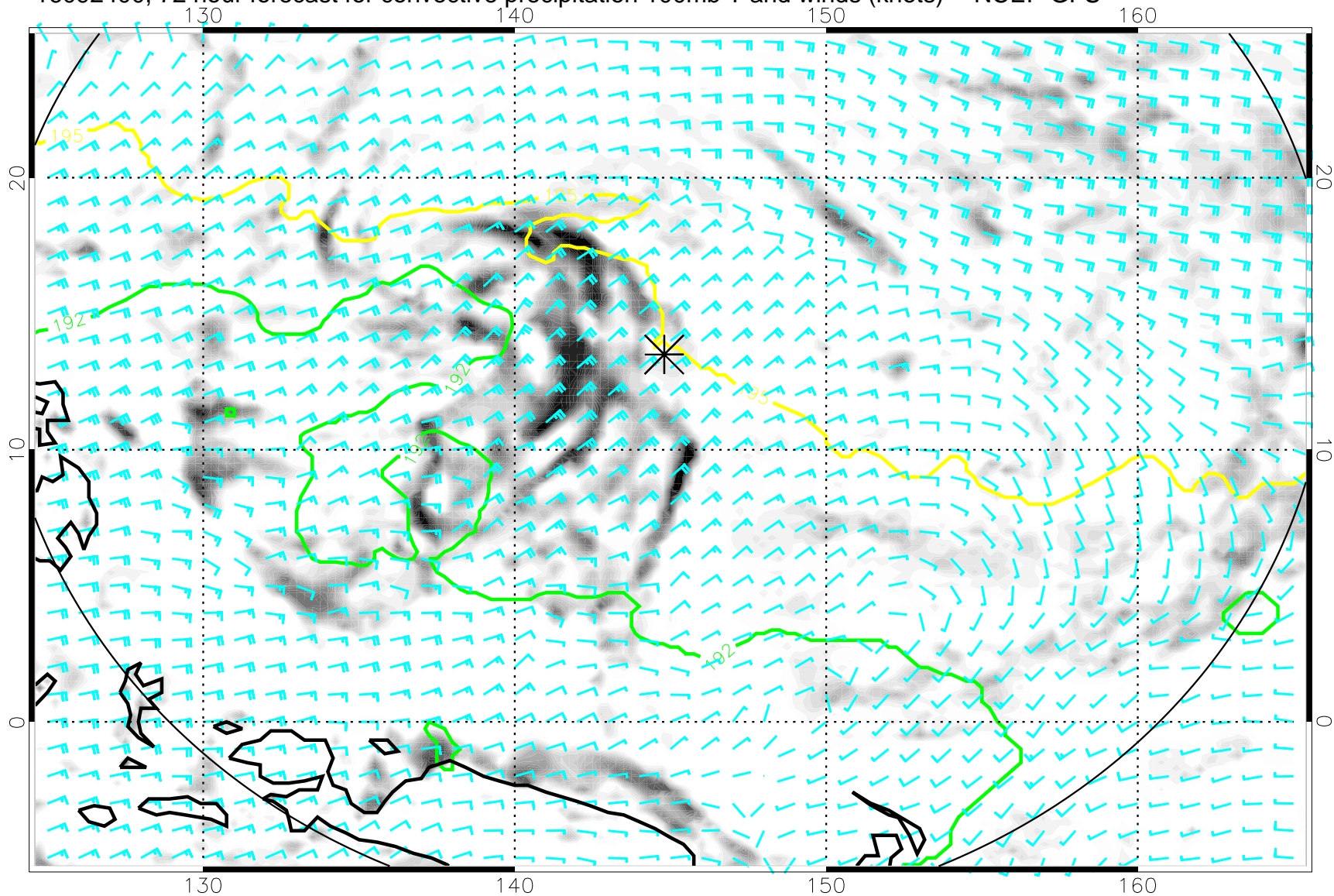
16092400, 72 hour forecast for convective precipitation 100mb T and winds (knots) -- NCEP GFS
