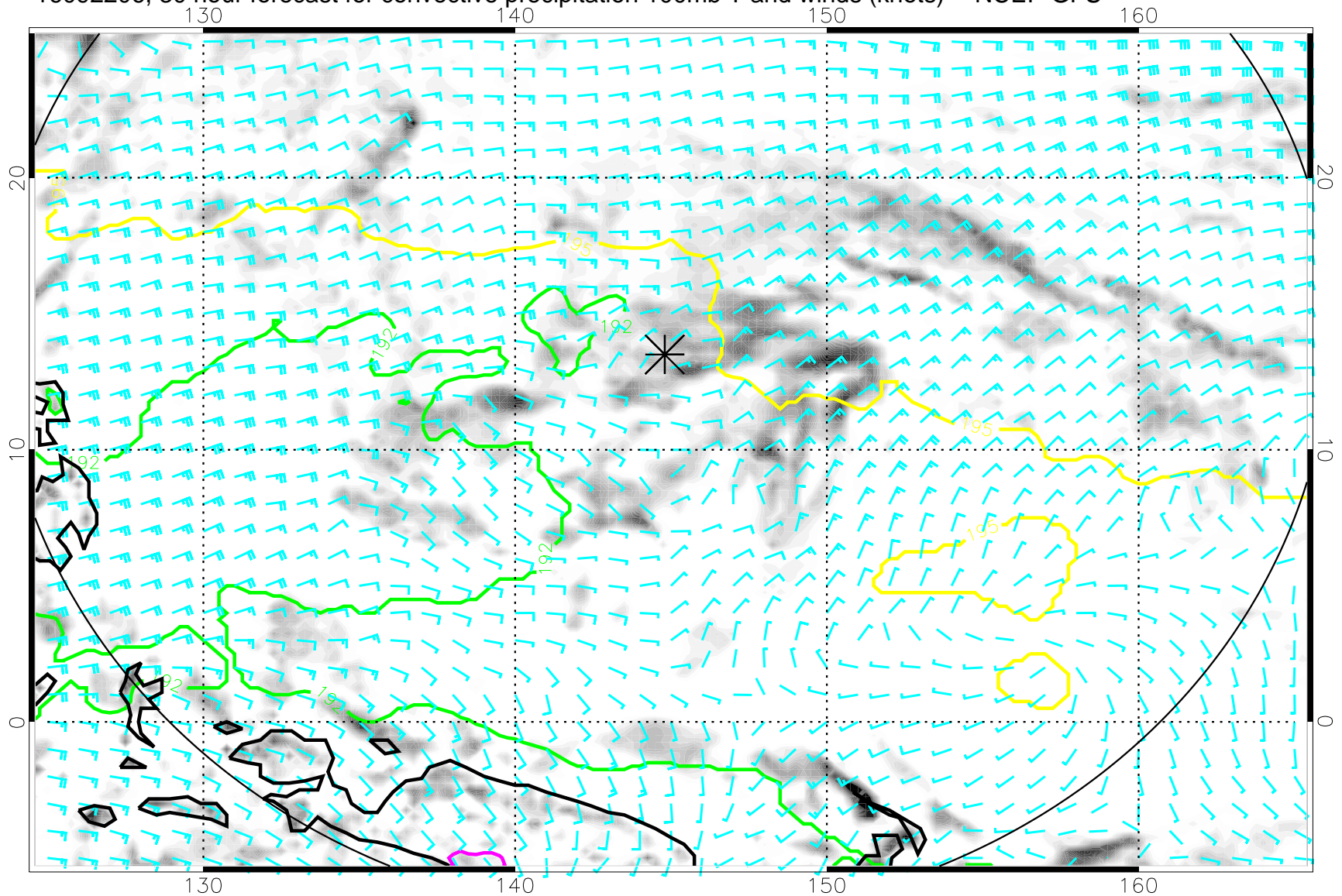
16092206, 30 hour forecast for convective precipitation 100mb T and winds (knots) -- NCEP GFS
