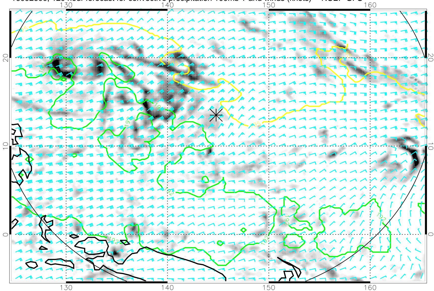
16092600, 120 hour forecast for convective precipitation 100mb T and winds (knots) -- NCEP GFS
