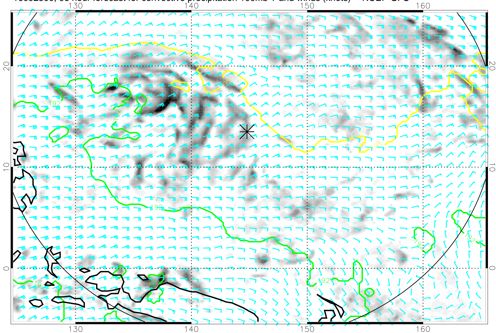
16092500, 96 hour forecast for convective precipitation 100mb T and winds (knots) -- NCEP GFS
