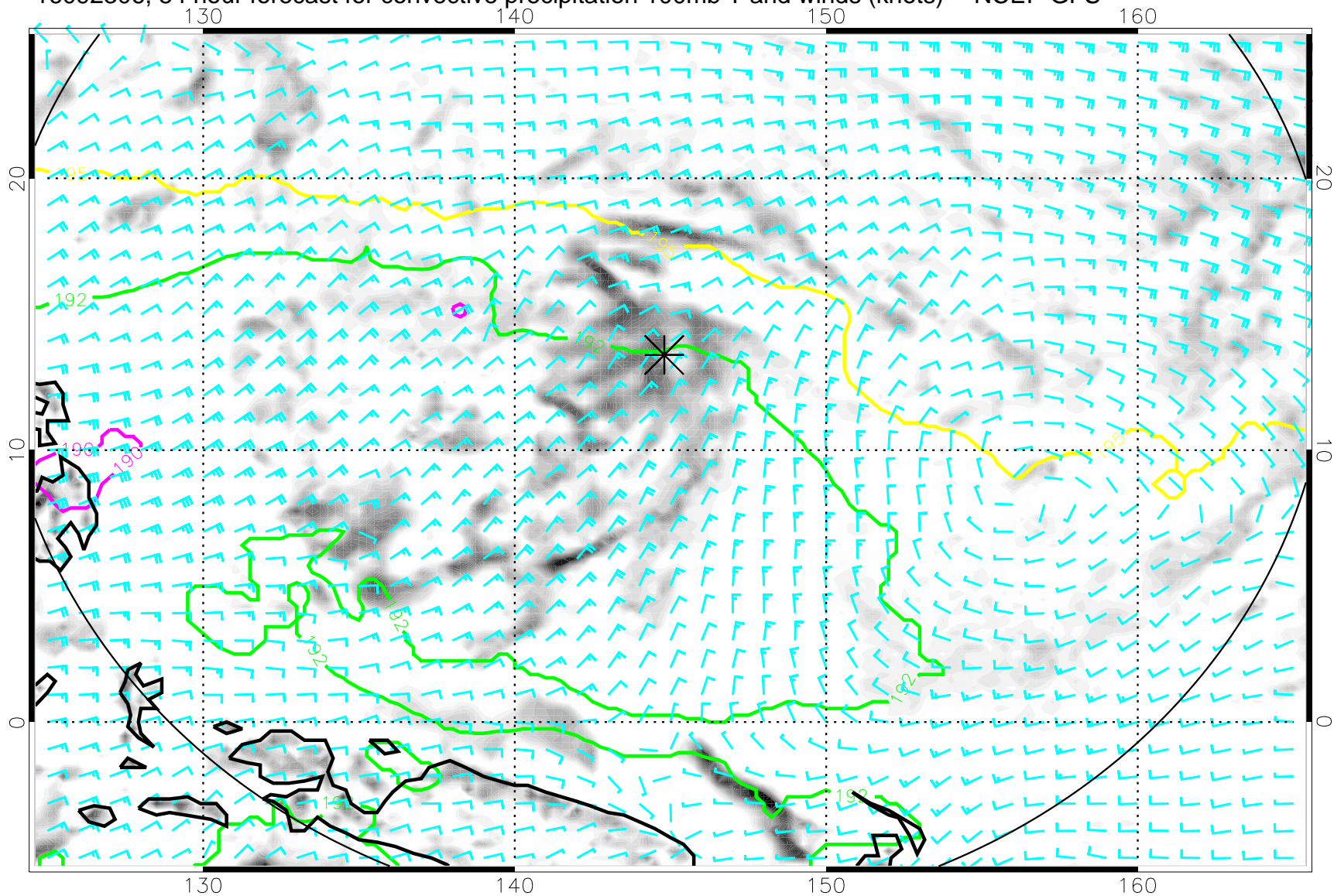
16092306, 54 hour forecast for convective precipitation 100mb T and winds (knots) -- NCEP GFS
