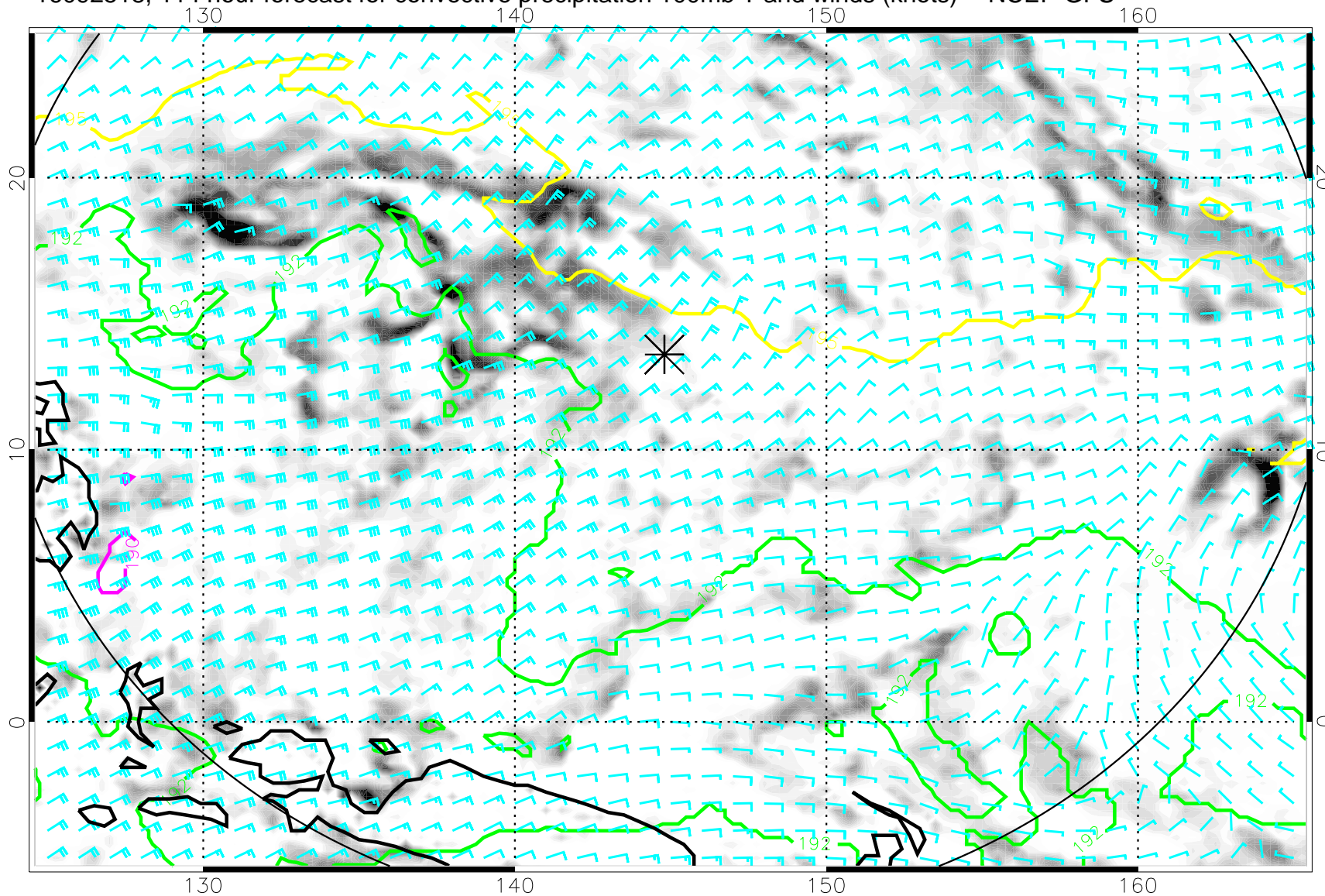
16092518, 114 hour forecast for convective precipitation 100mb T and winds (knots) -- NCEP GFS
