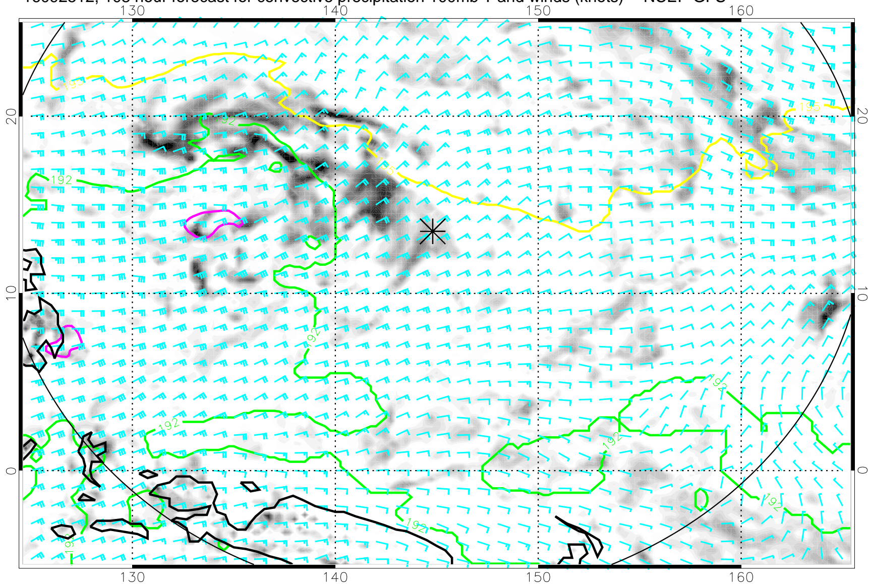
16092512, 108 hour forecast for convective precipitation 100mb T and winds (knots) -- NCEP GFS
