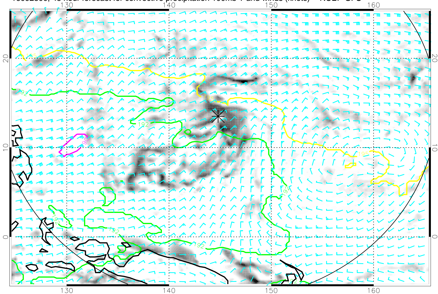
16092300, 48 hour forecast for convective precipitation 100mb T and winds (knots) -- NCEP GFS
