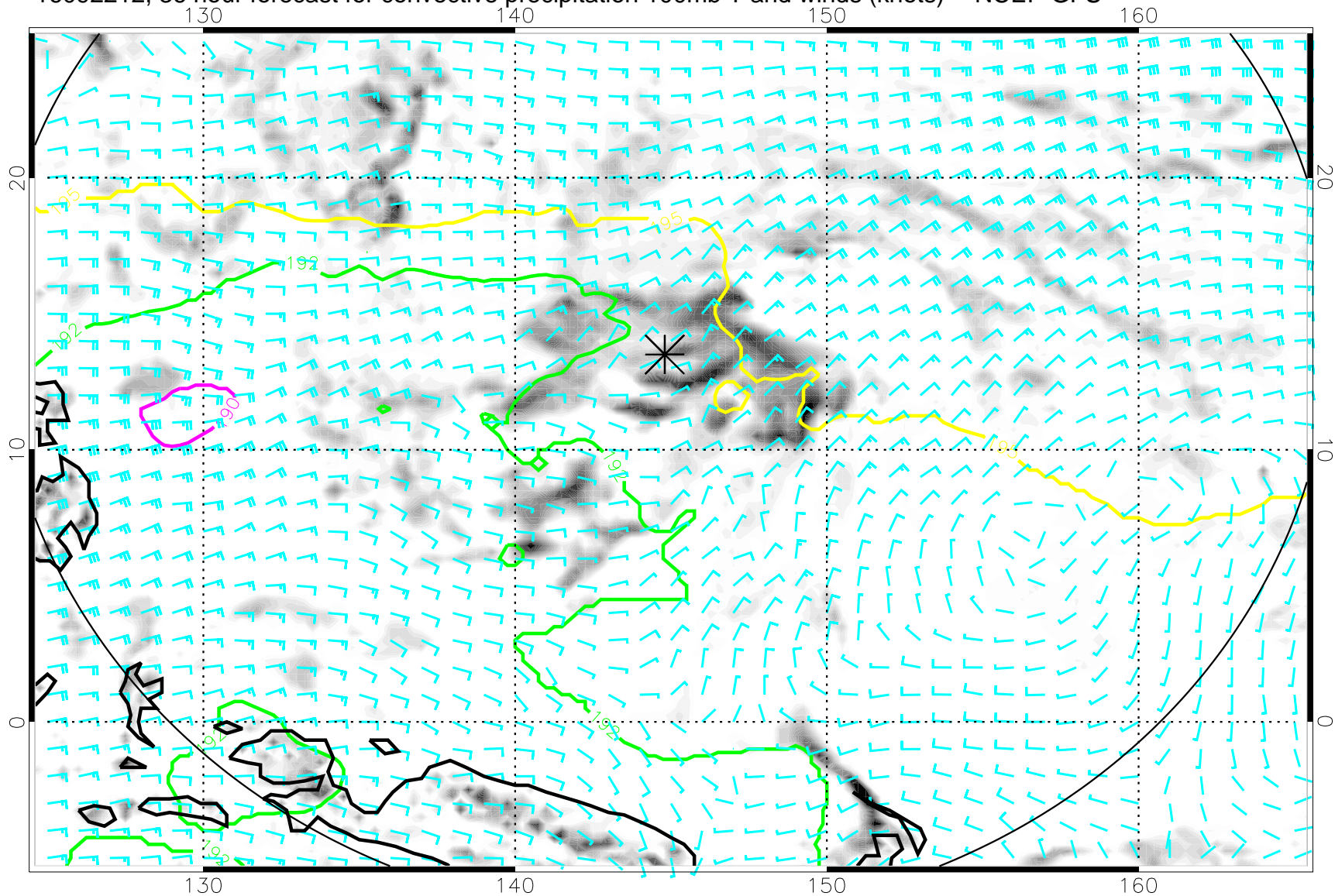
16092212, 36 hour forecast for convective precipitation 100mb T and winds (knots) -- NCEP GFS
