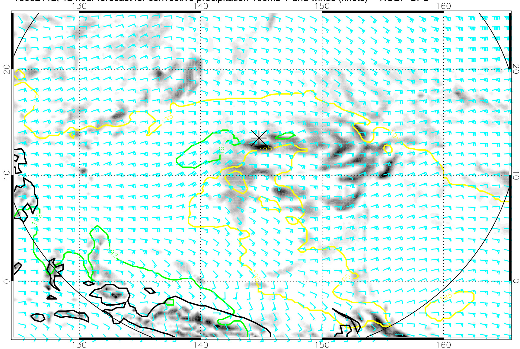
16092112, 12 hour forecast for convective precipitation 100mb T and winds (knots) -- NCEP GFS
