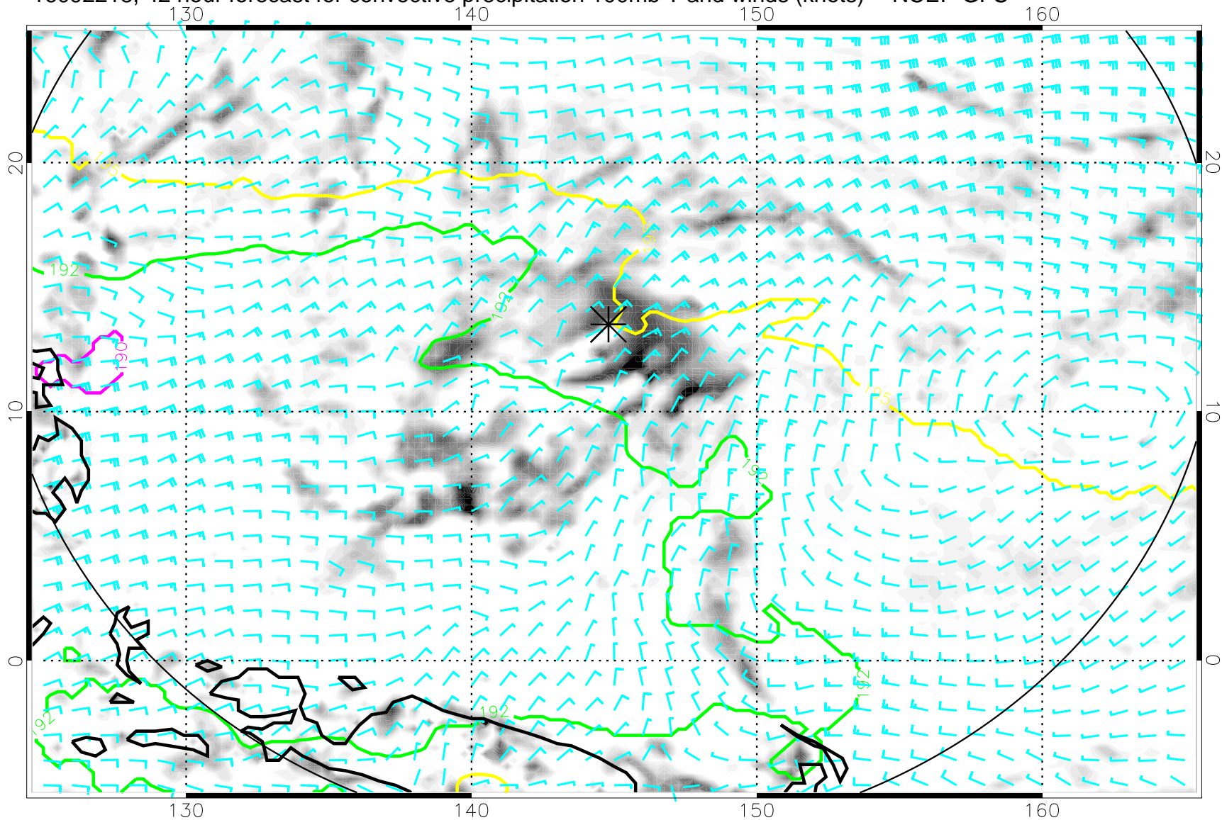
16092218, 42 hour forecast for convective precipitation 100mb T and winds (knots) -- NCEP GFS
