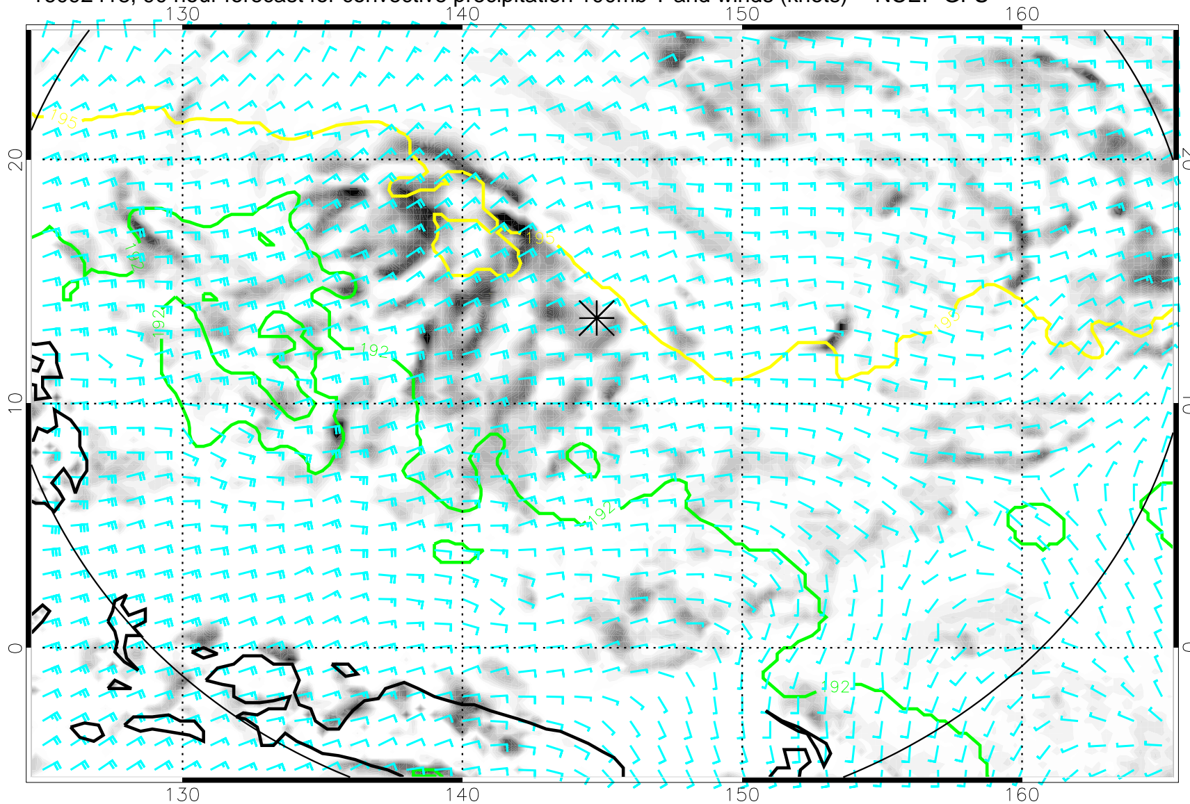
16092418, 90 hour forecast for convective precipitation 100mb T and winds (knots) -- NCEP GFS
