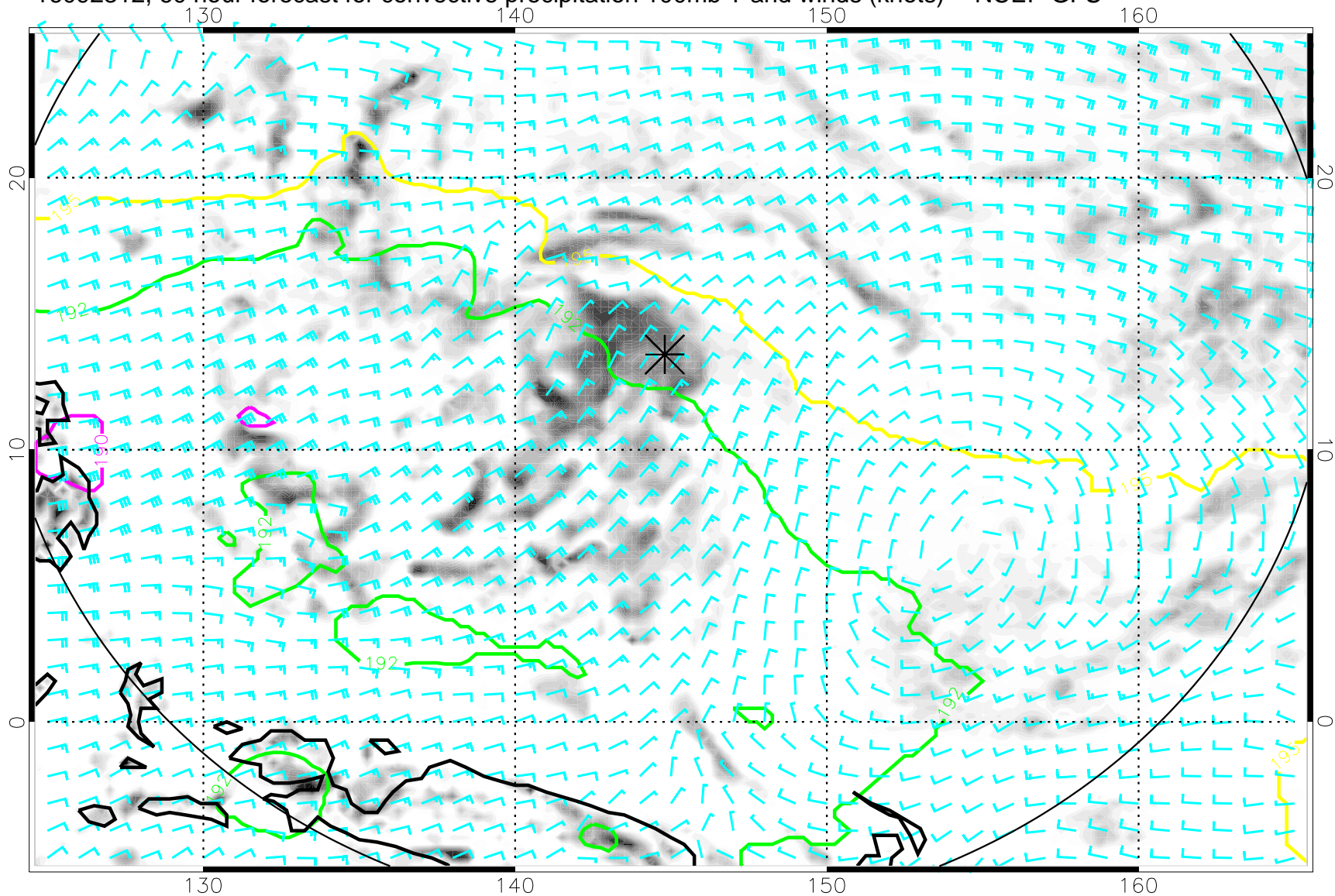
16092312, 60 hour forecast for convective precipitation 100mb T and winds (knots) -- NCEP GFS
