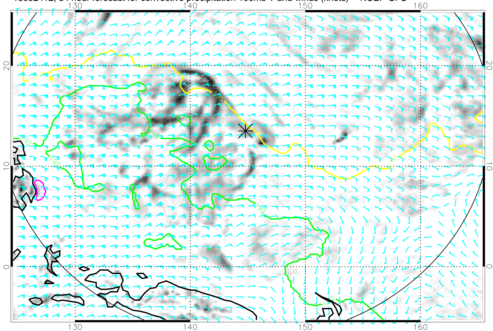
16092412, 84 hour forecast for convective precipitation 100mb T and winds (knots) -- NCEP GFS
