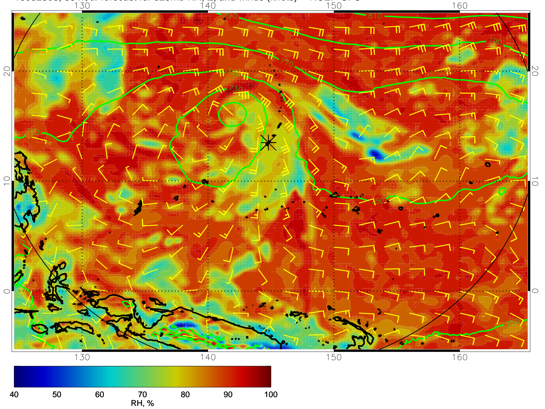
16092306, 66 hour forecast for 925mb RH, Z, and winds (knots) -- NCEP GFS
