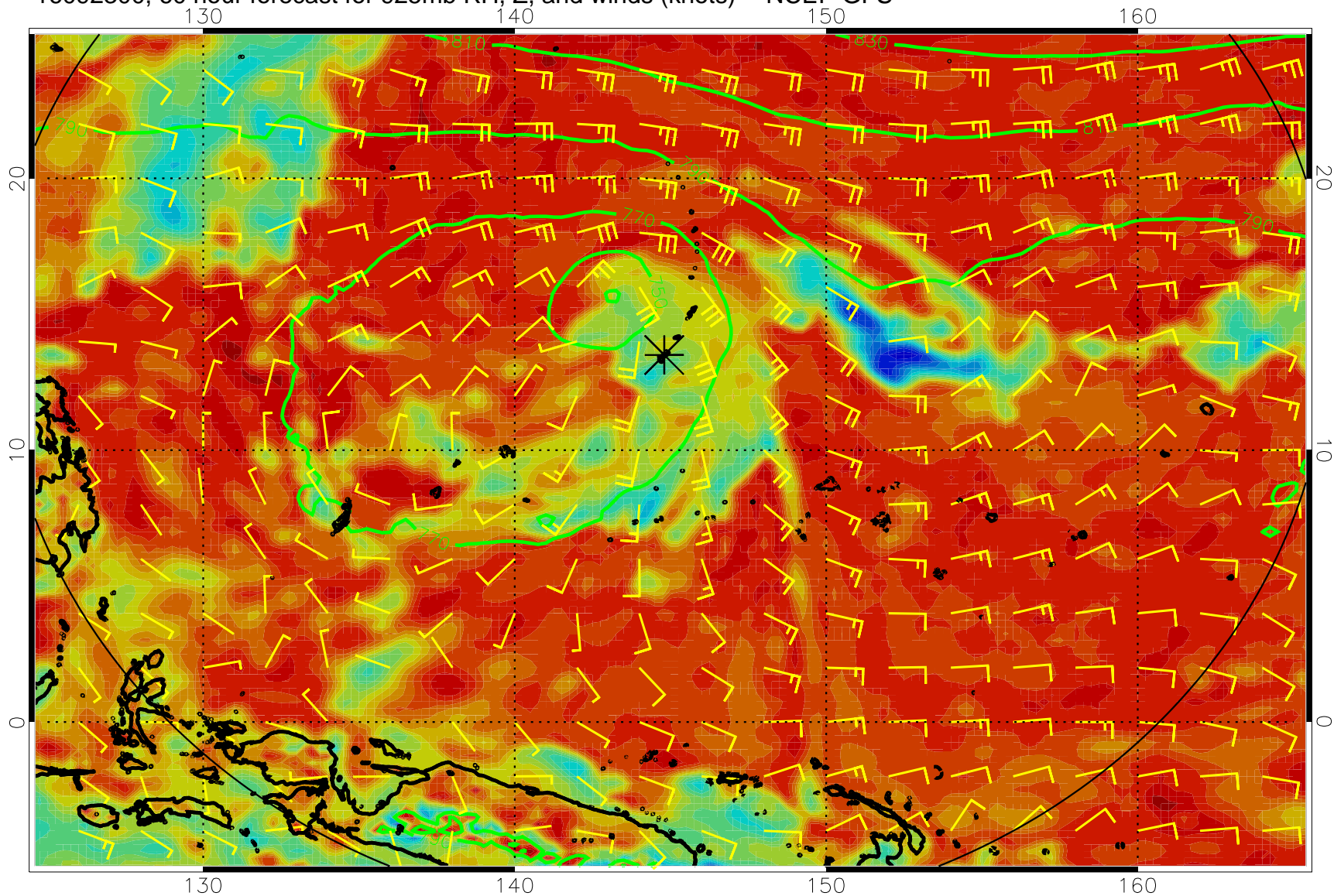
16092300, 60 hour forecast for 925mb RH, Z, and winds (knots) -- NCEP GFS
