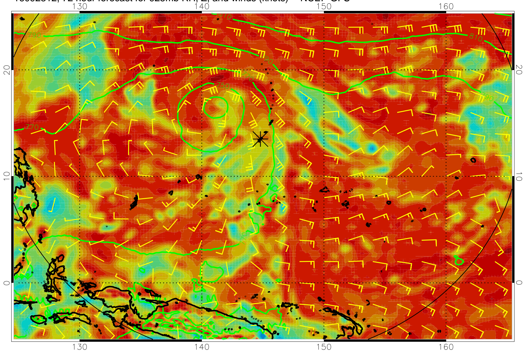
16092312, 72 hour forecast for 925mb RH, Z, and winds (knots) -- NCEP GFS
