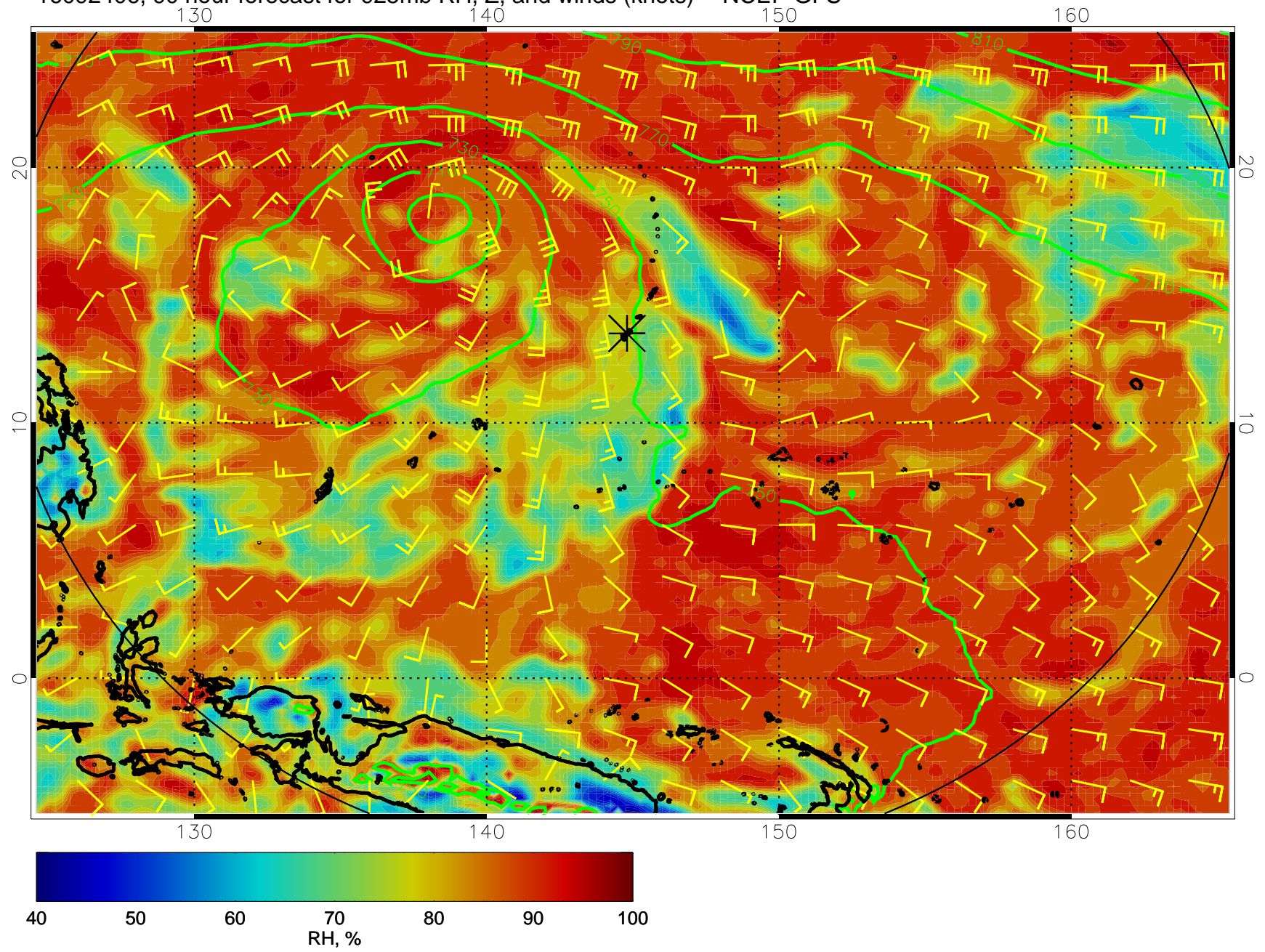
16092406, 90 hour forecast for 925mb RH, Z, and winds (knots) -- NCEP GFS
