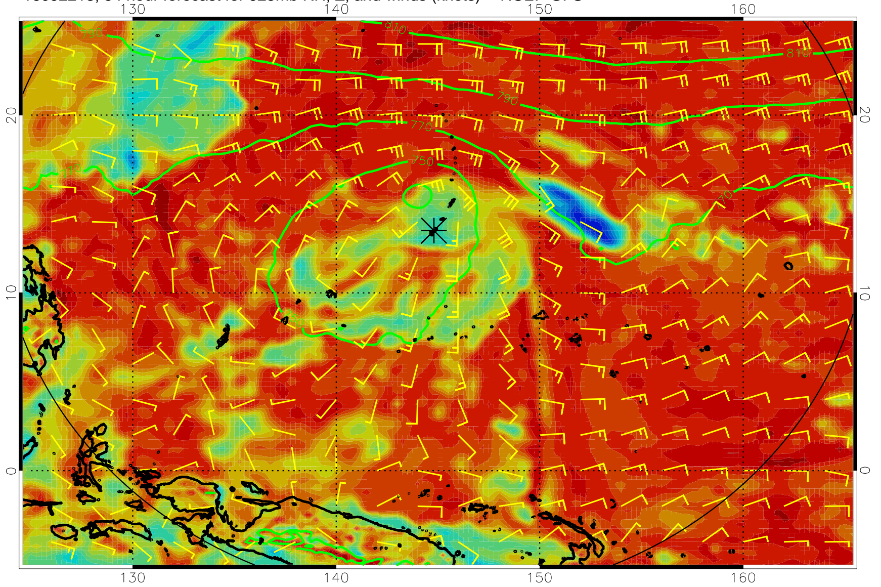
16092218, 54 hour forecast for 925mb RH, Z, and winds (knots) -- NCEP GFS
