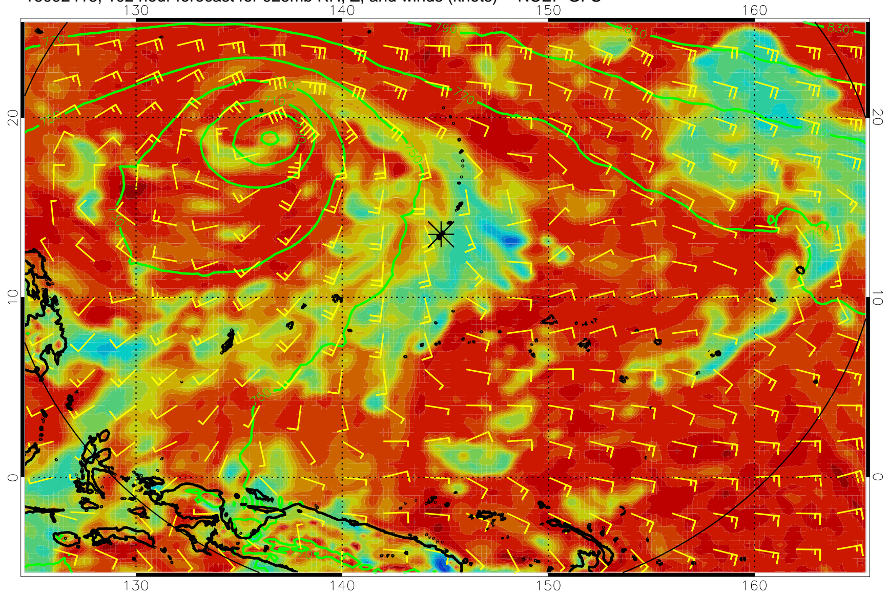
16092418, 102 hour forecast for 925mb RH, Z, and winds (knots) -- NCEP GFS
