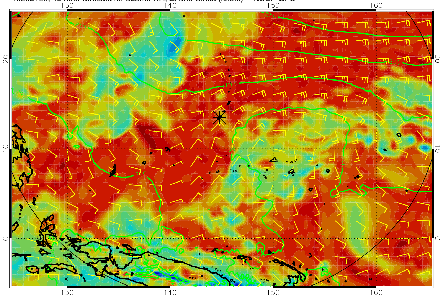
16092100, 12 hour forecast for 925mb RH, Z, and winds (knots) -- NCEP GFS
