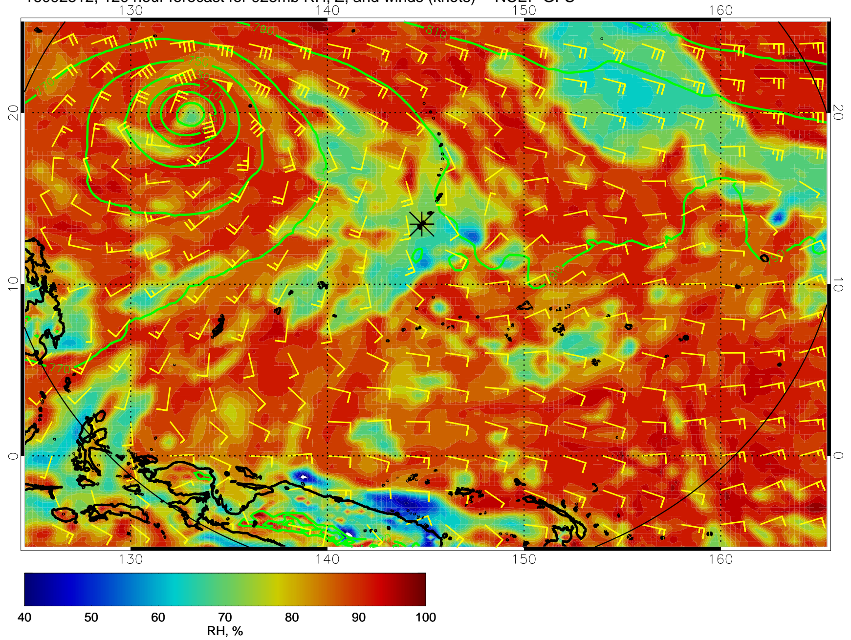
16092512, 120 hour forecast for 925mb RH, Z, and winds (knots) -- NCEP GFS
