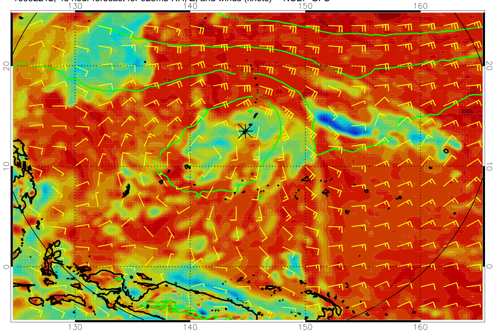
16092212, 48 hour forecast for 925mb RH, Z, and winds (knots) -- NCEP GFS
