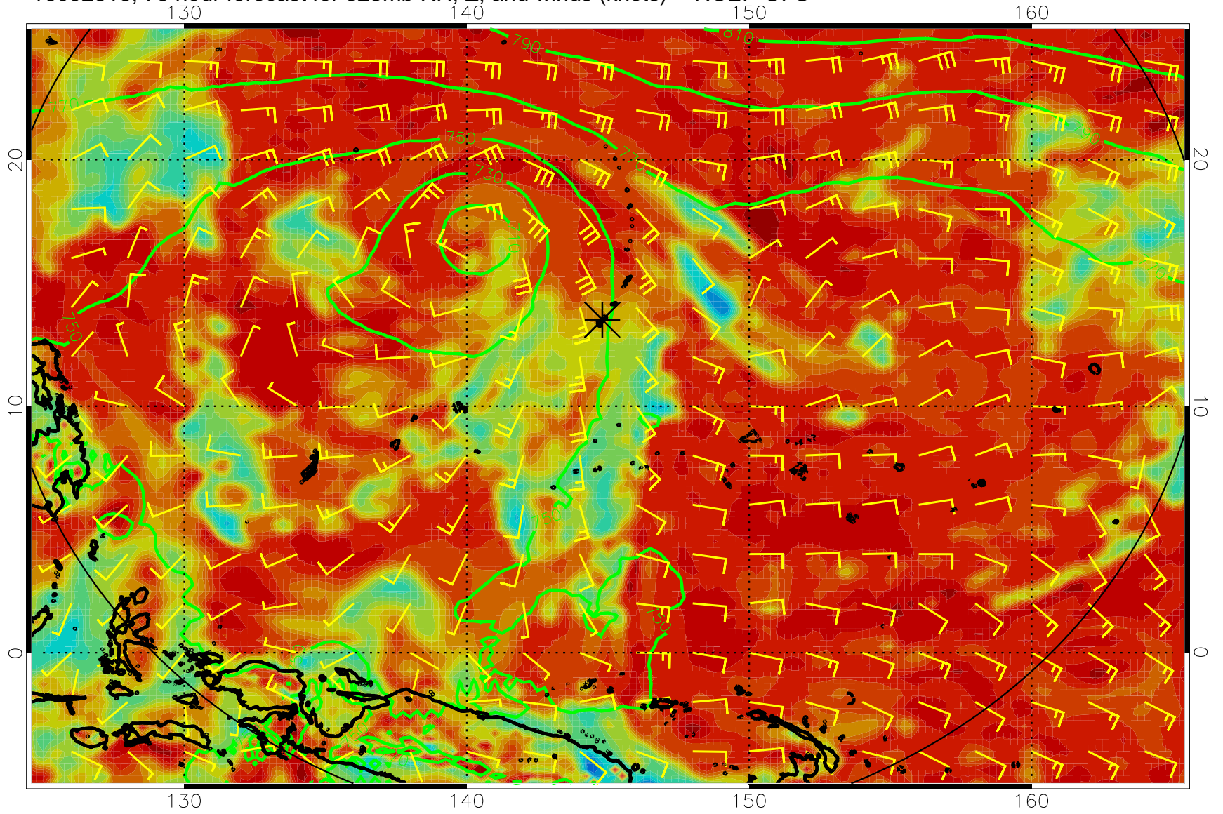
16092318, 78 hour forecast for 925mb RH, Z, and winds (knots) -- NCEP GFS
