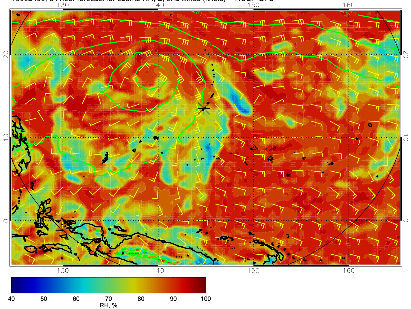
16092400, 84 hour forecast for 925mb RH, Z, and winds (knots) -- NCEP GFS
