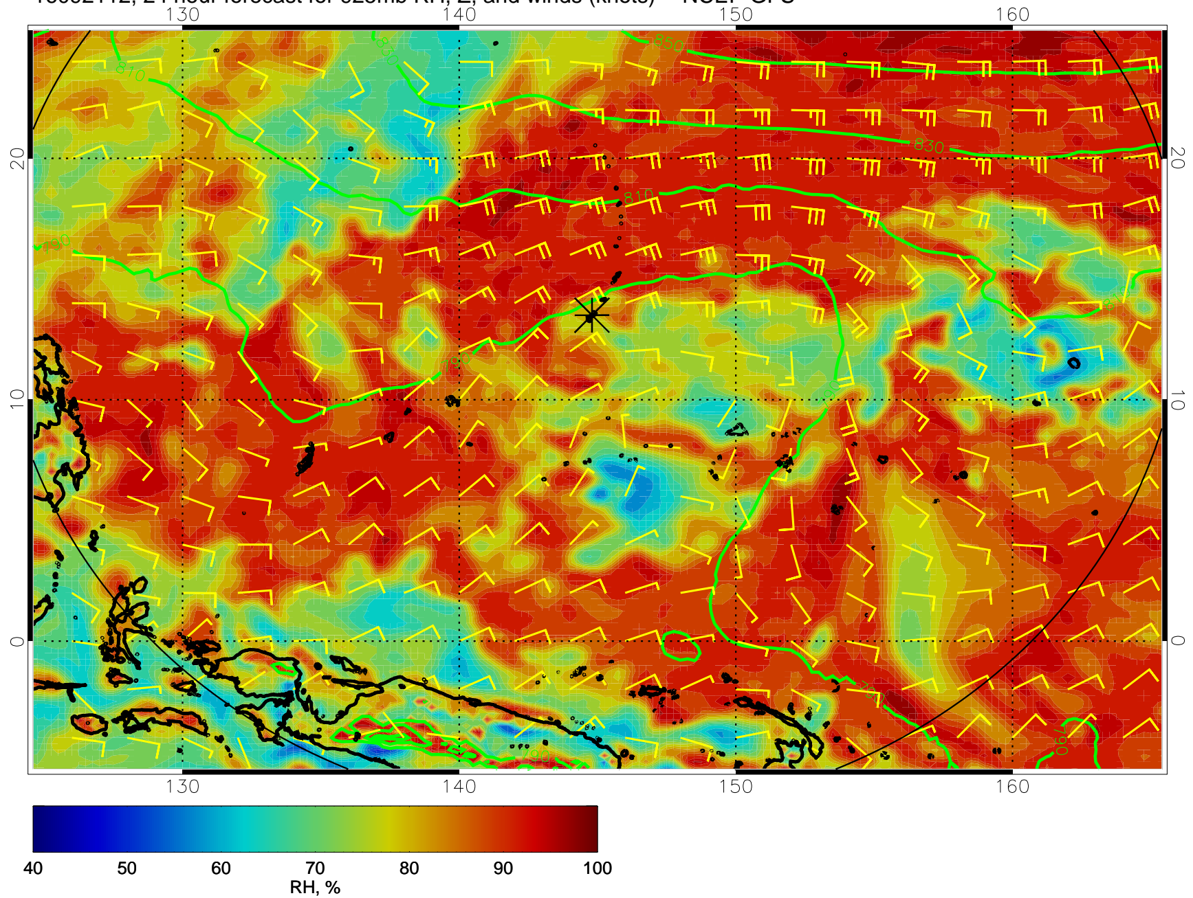
16092112, 24 hour forecast for 925mb RH, Z, and winds (knots) -- NCEP GFS
