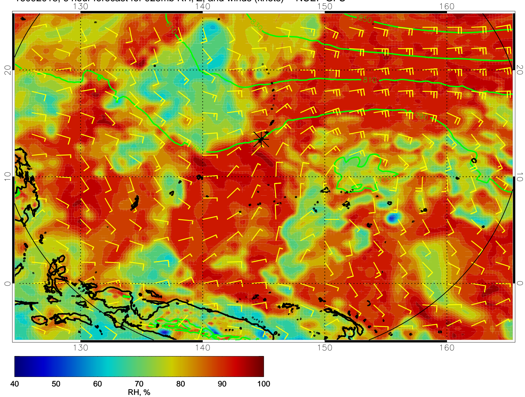
16092018, 6 hour forecast for 925mb RH, Z, and winds (knots) -- NCEP GFS
