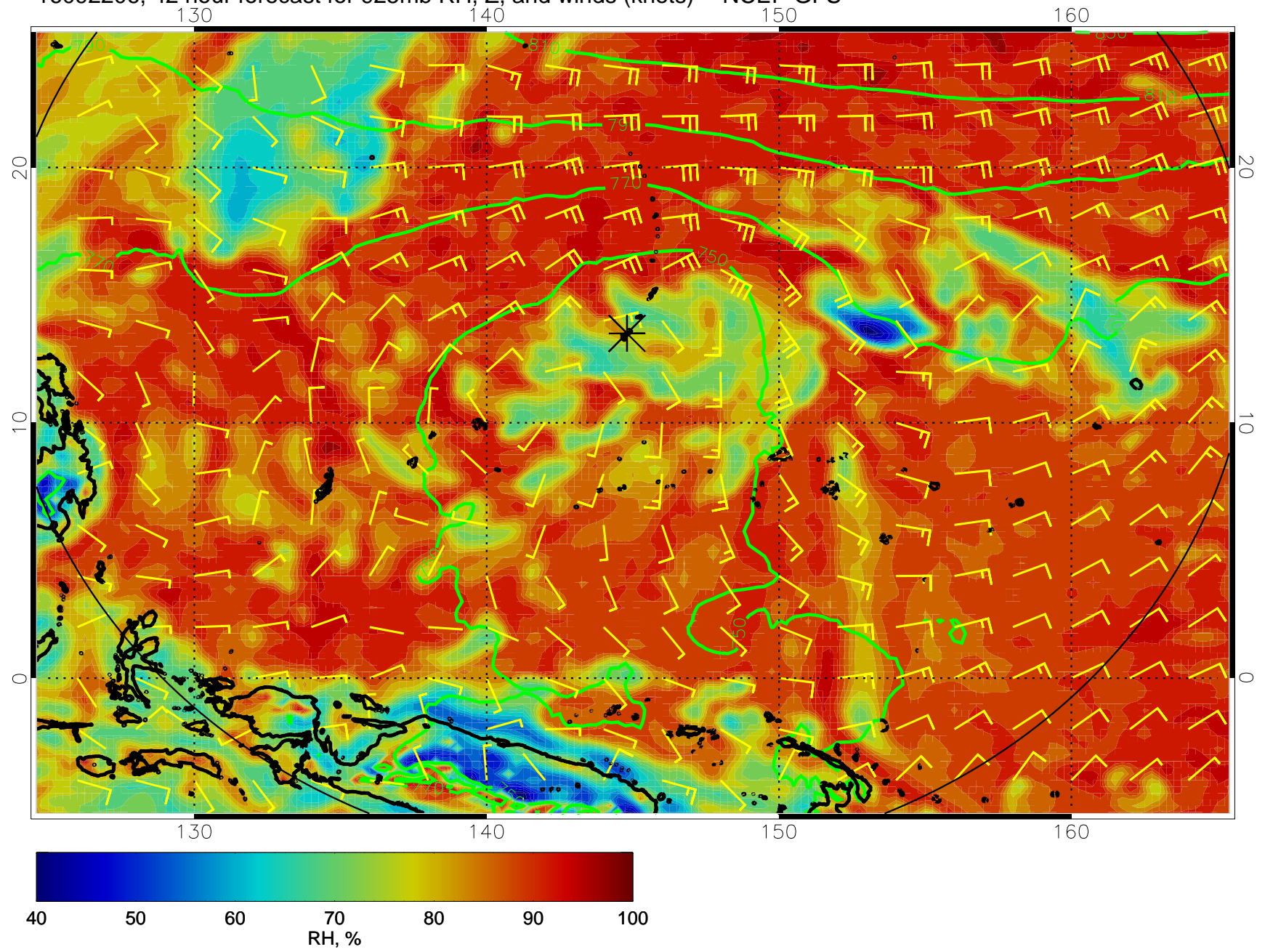
16092206, 42 hour forecast for 925mb RH, Z, and winds (knots) -- NCEP GFS
