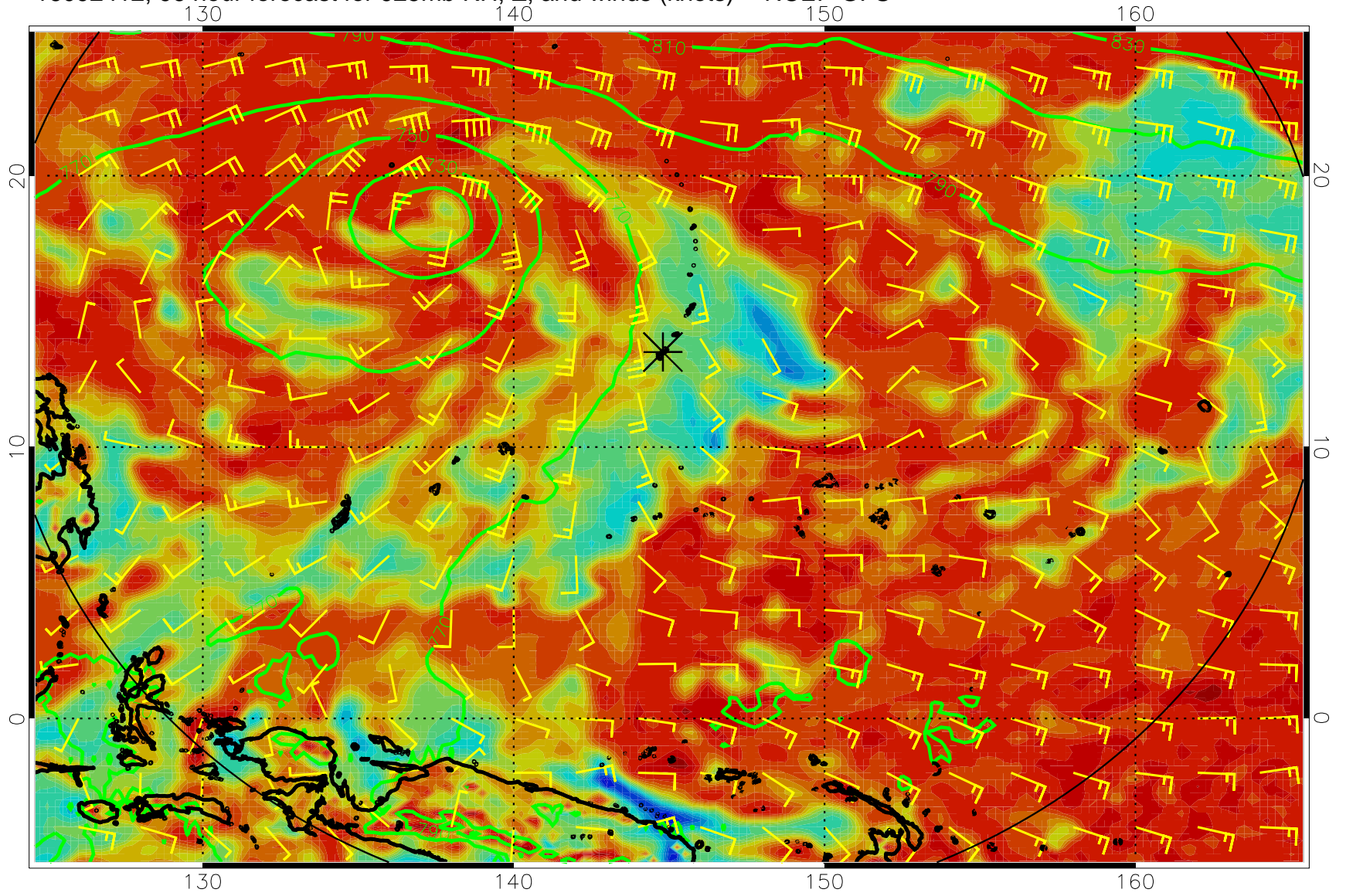
16092412, 96 hour forecast for 925mb RH, Z, and winds (knots) -- NCEP GFS
