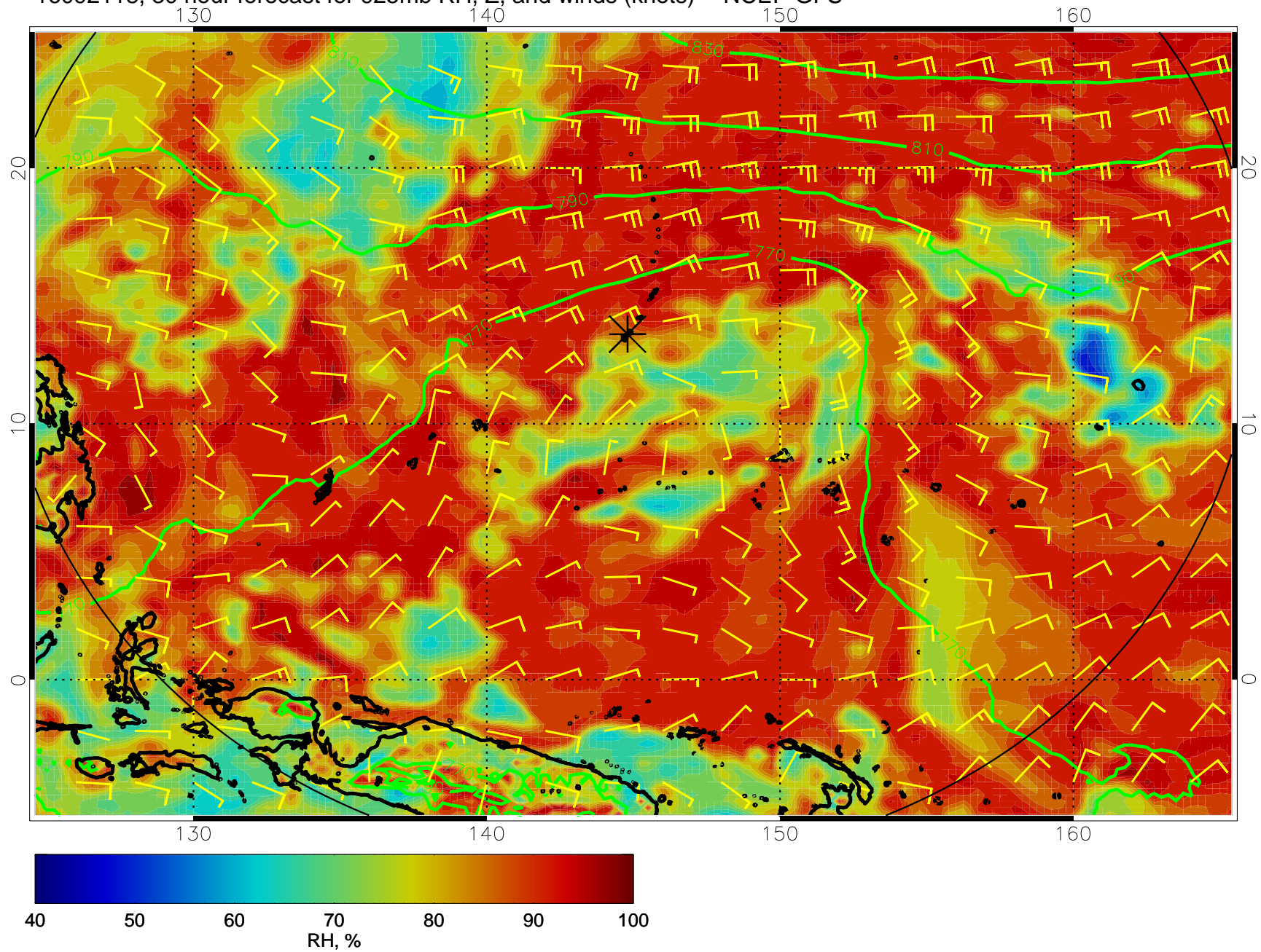
16092118, 30 hour forecast for 925mb RH, Z, and winds (knots) -- NCEP GFS
