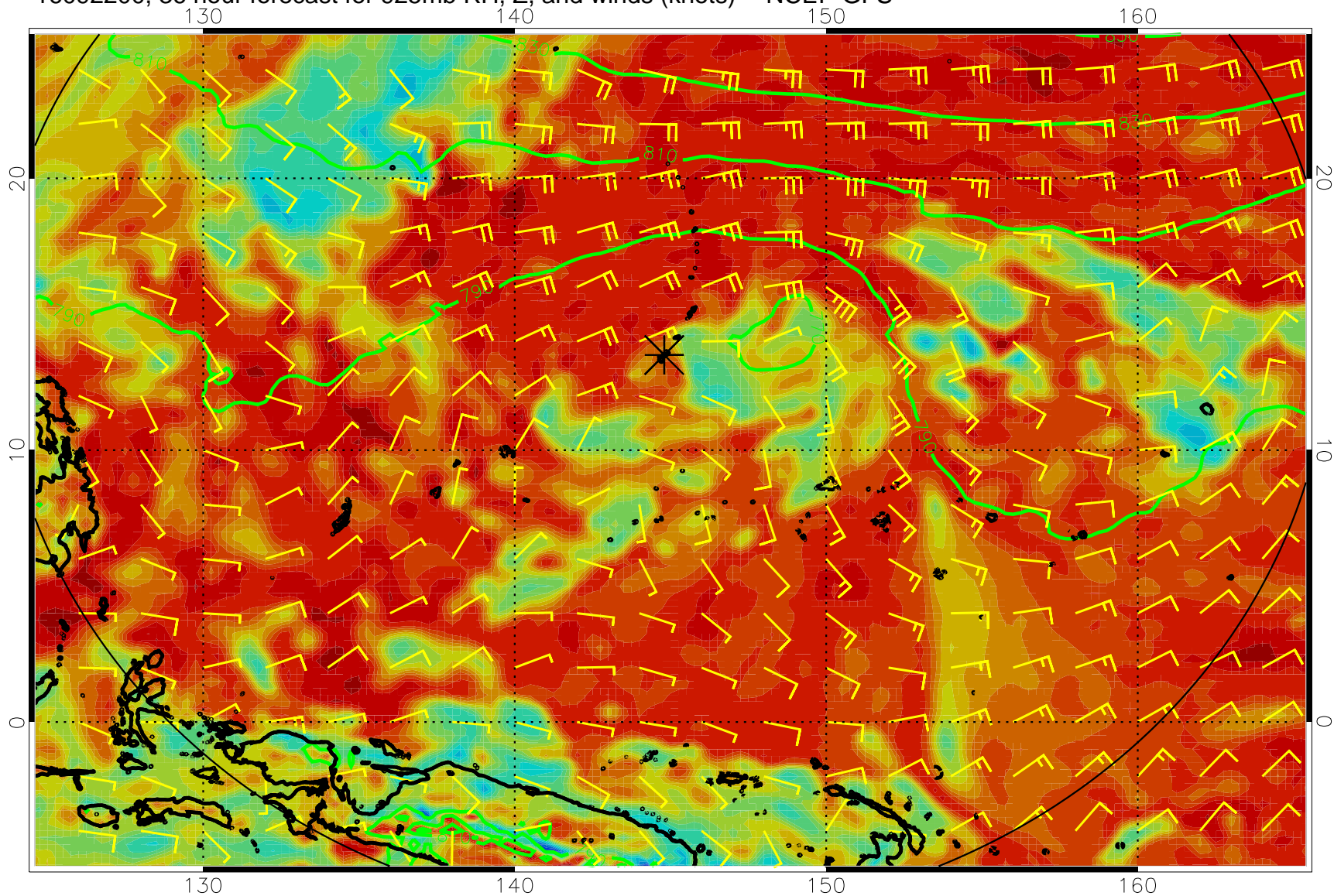
16092200, 36 hour forecast for 925mb RH, Z, and winds (knots) -- NCEP GFS
