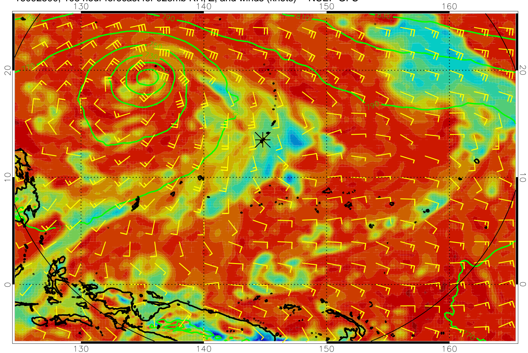
16092500, 108 hour forecast for 925mb RH, Z, and winds (knots) -- NCEP GFS
