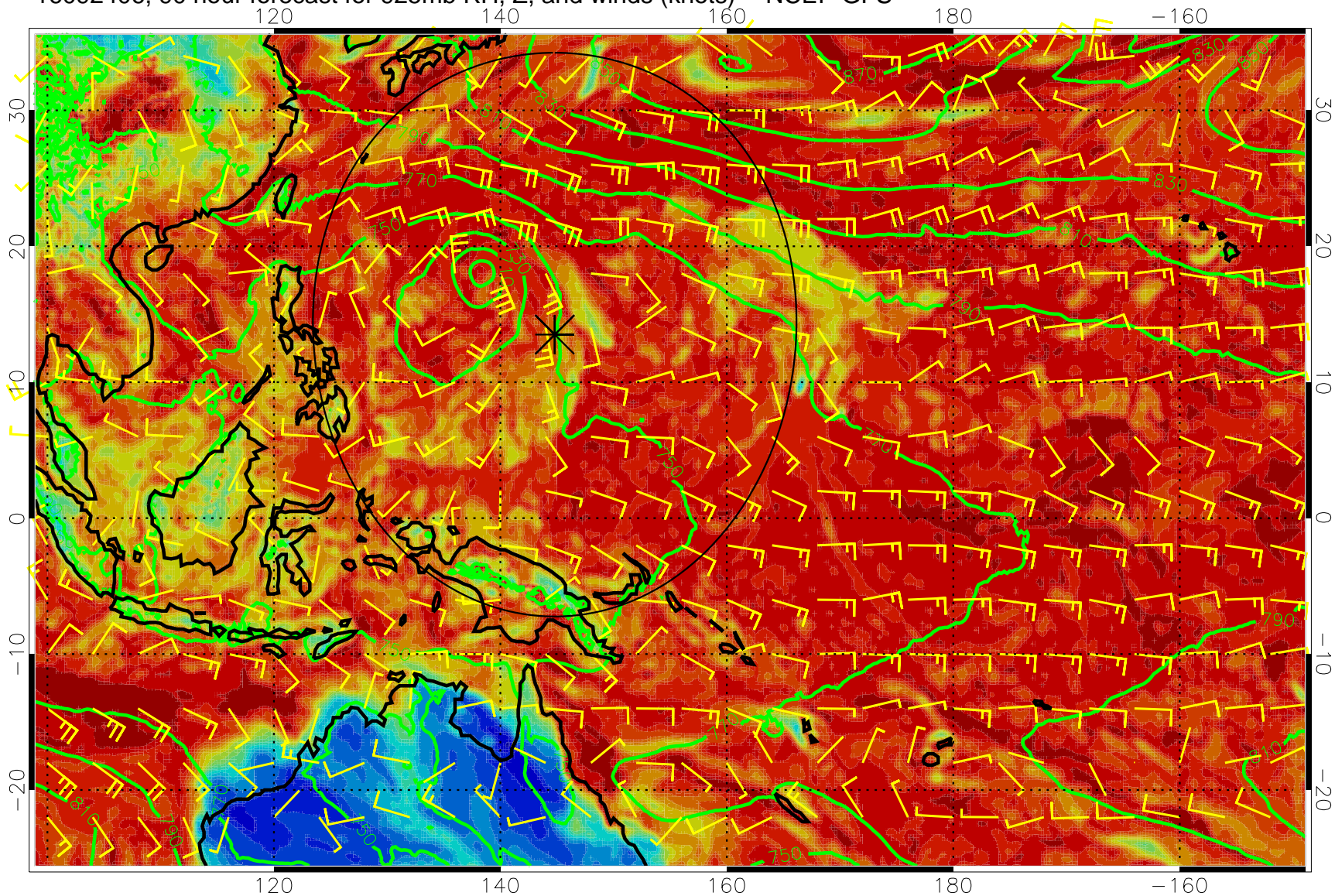
16092406, 90 hour forecast for 925mb RH, Z, and winds (knots) -- NCEP GFS
