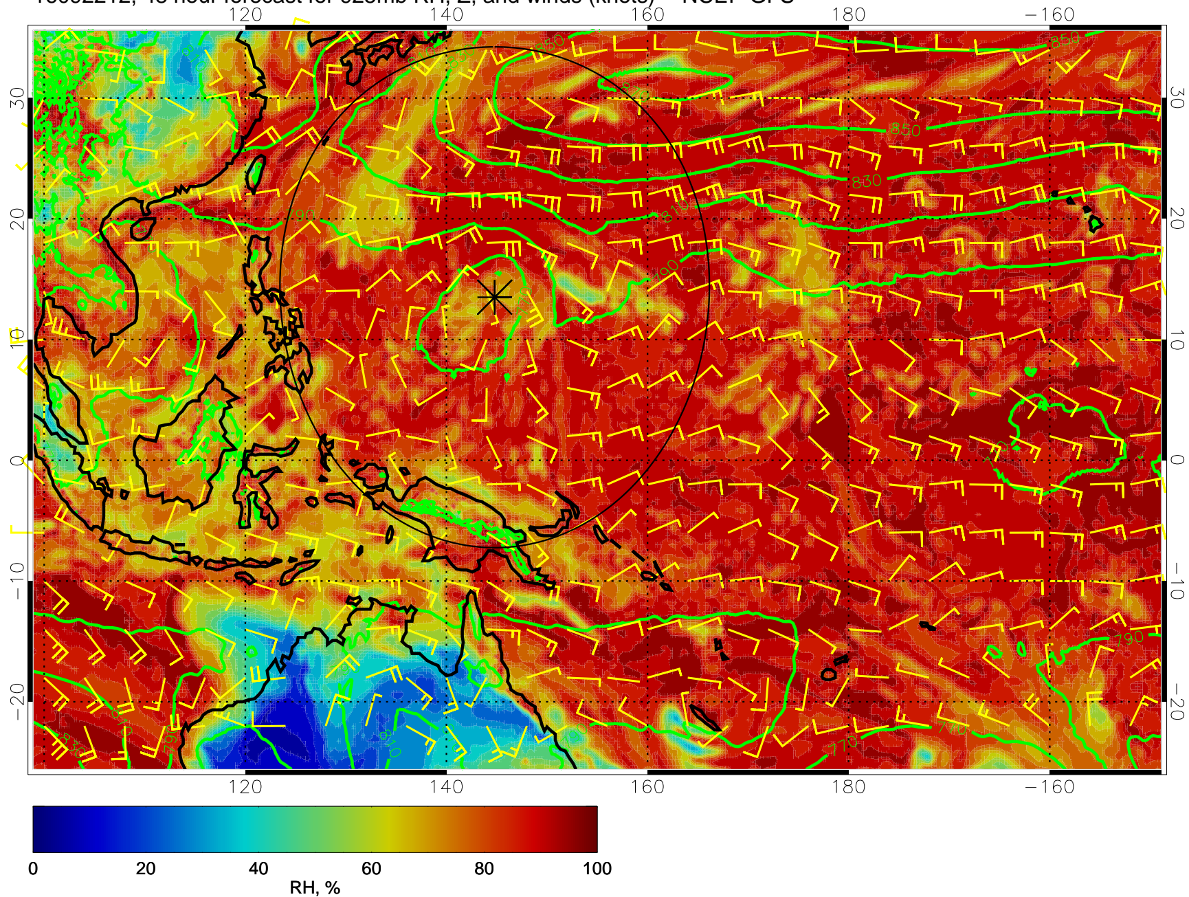
16092212, 48 hour forecast for 925mb RH, Z, and winds (knots) -- NCEP GFS
