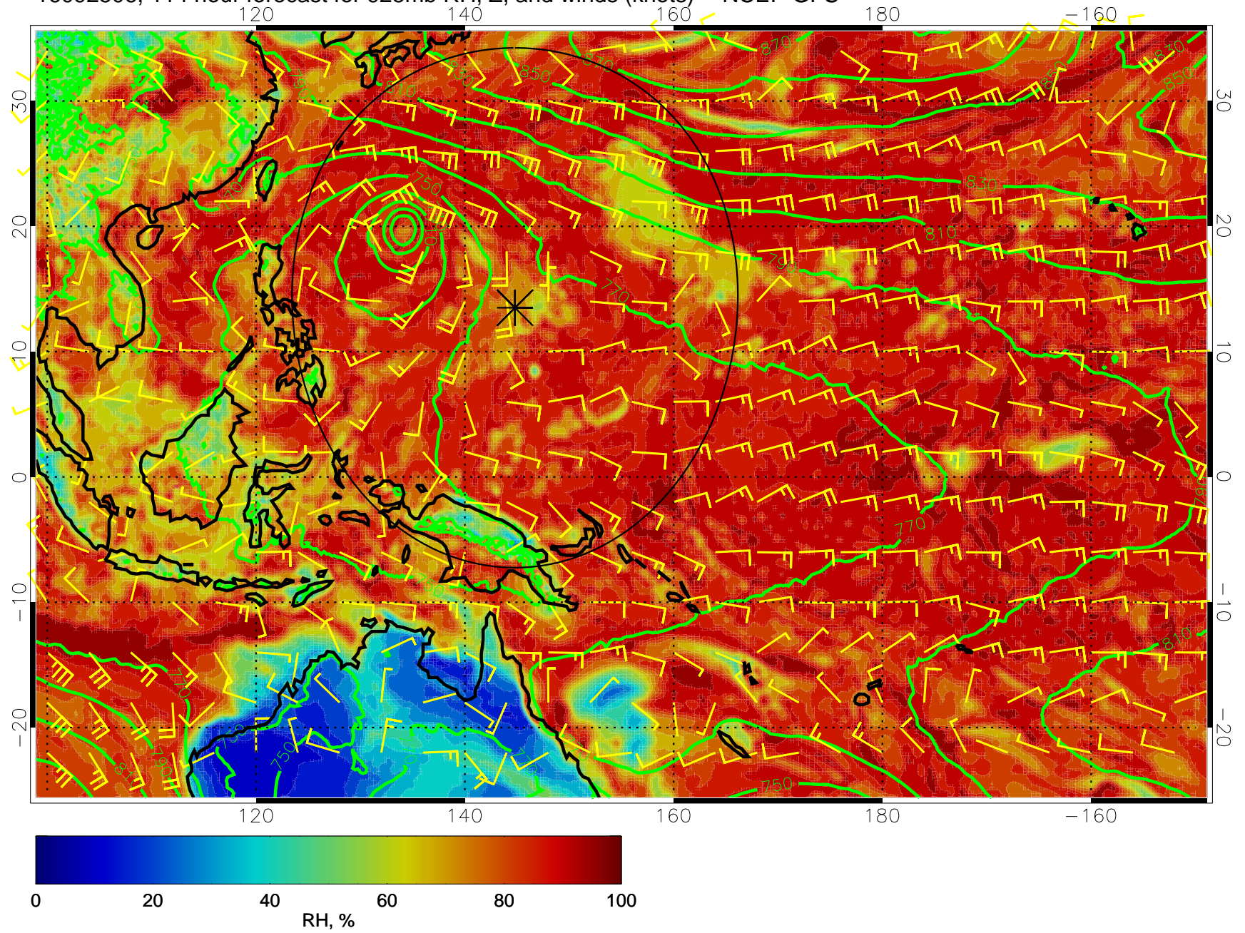
16092506, 114 hour forecast for 925mb RH, Z, and winds (knots) -- NCEP GFS
