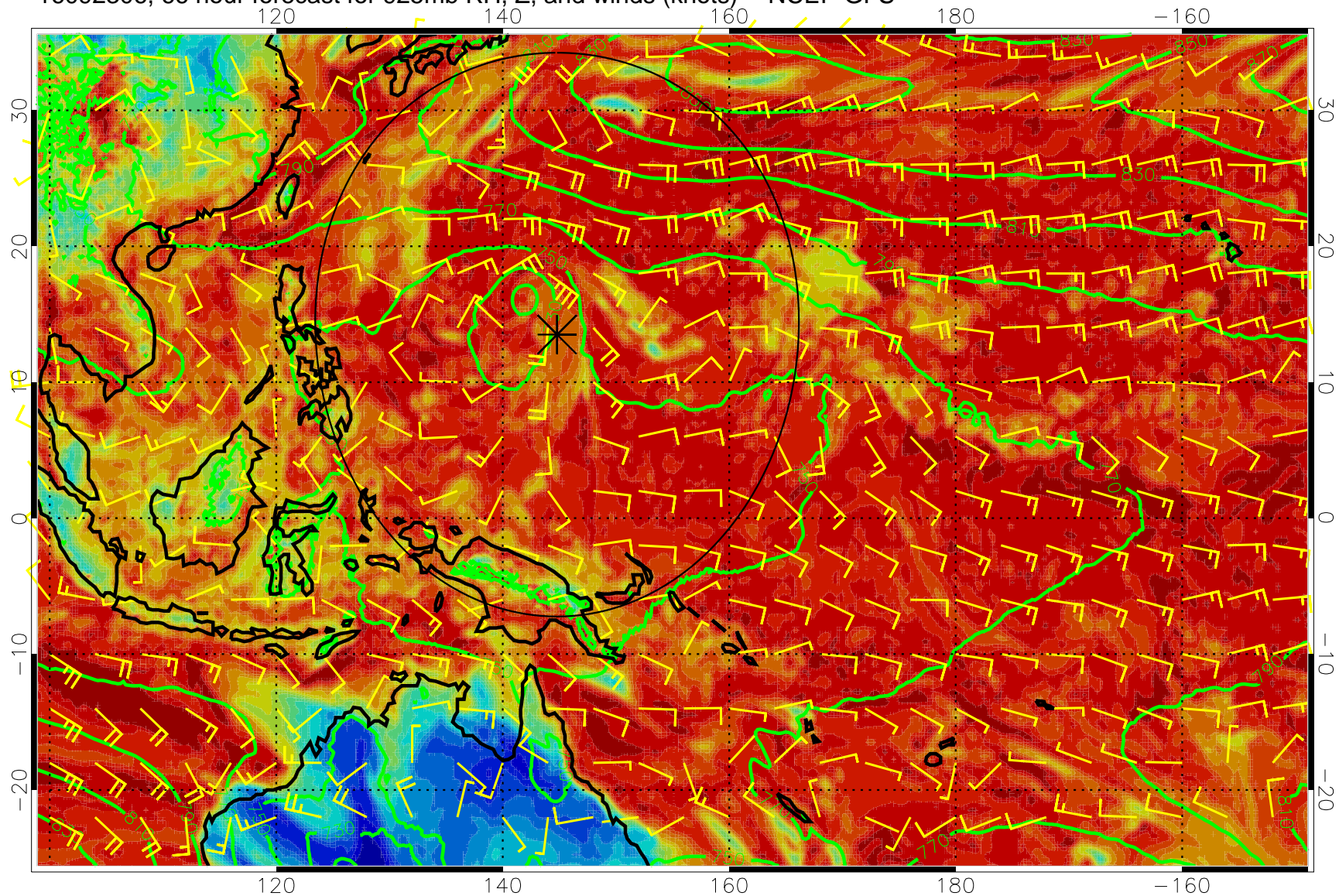
16092306, 66 hour forecast for 925mb RH, Z, and winds (knots) -- NCEP GFS
