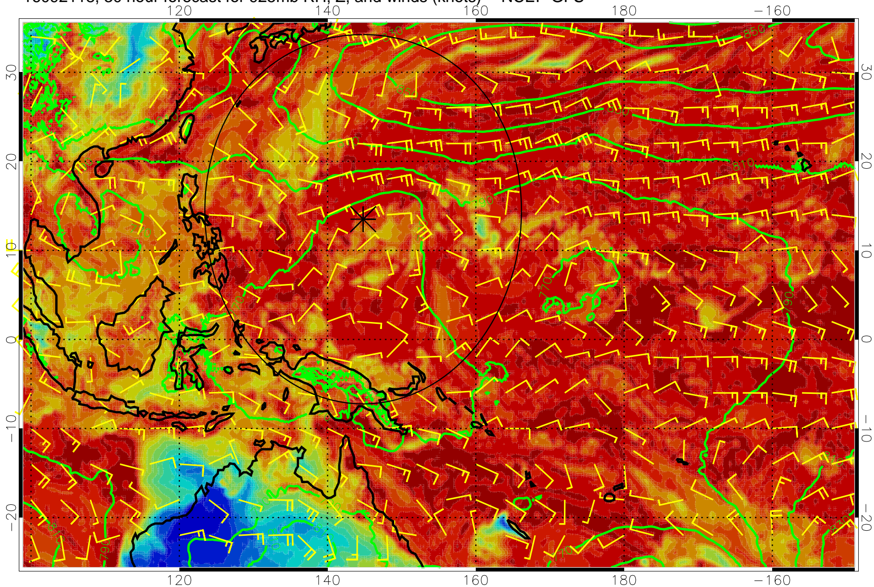
16092118, 30 hour forecast for 925mb RH, Z, and winds (knots) -- NCEP GFS
