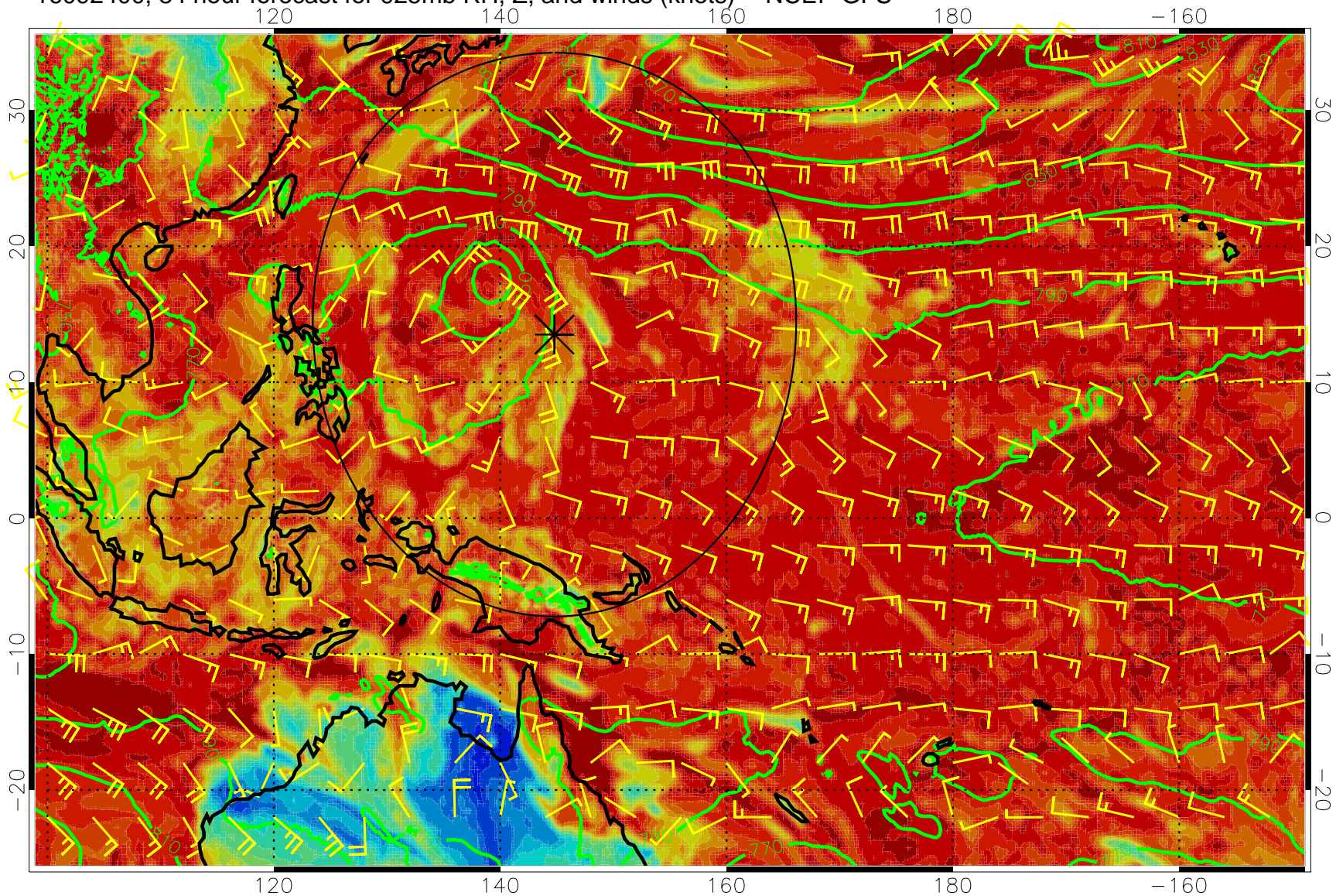
16092400, 84 hour forecast for 925mb RH, Z, and winds (knots) -- NCEP GFS
