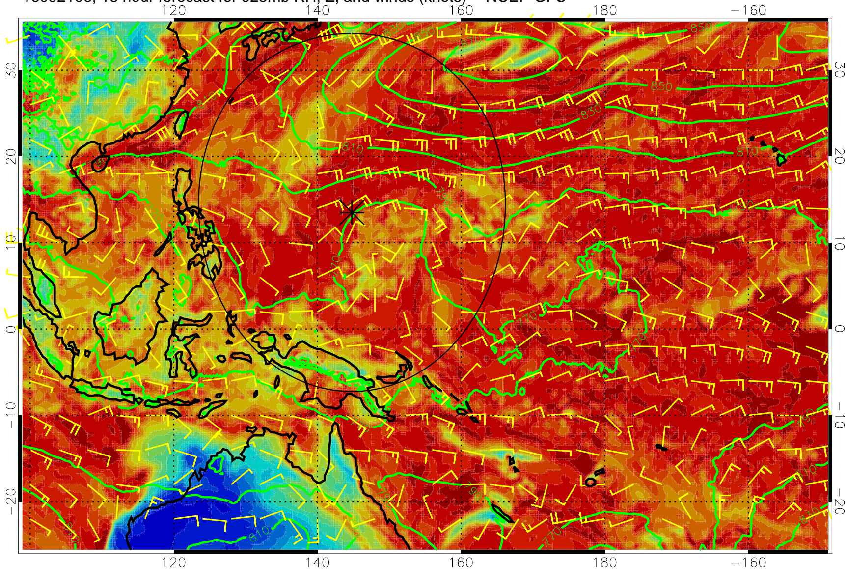
16092106, 18 hour forecast for 925mb RH, Z, and winds (knots) -- NCEP GFS
