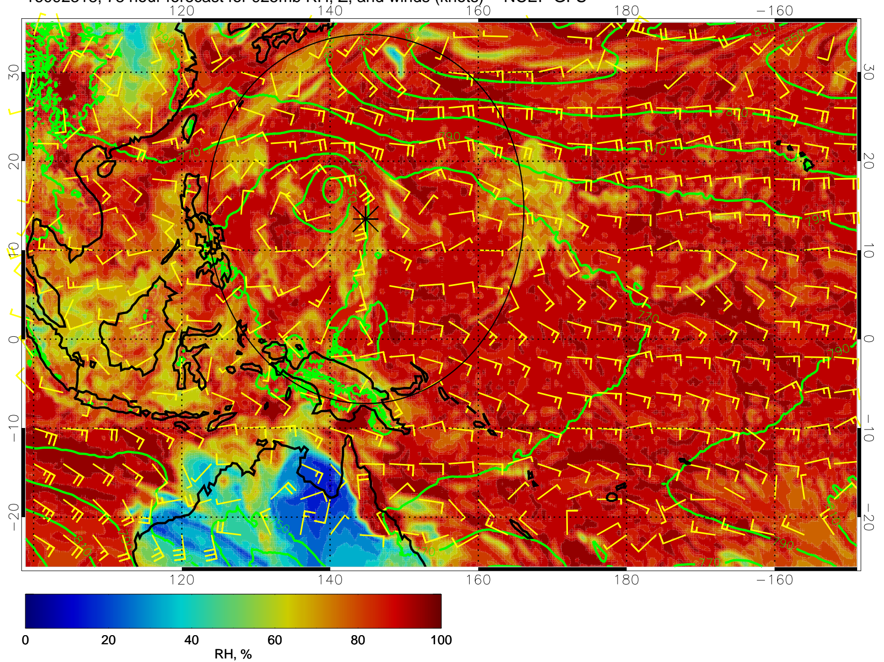
16092318, 78 hour forecast for 925mb RH, Z, and winds (knots) -- NCEP GFS
