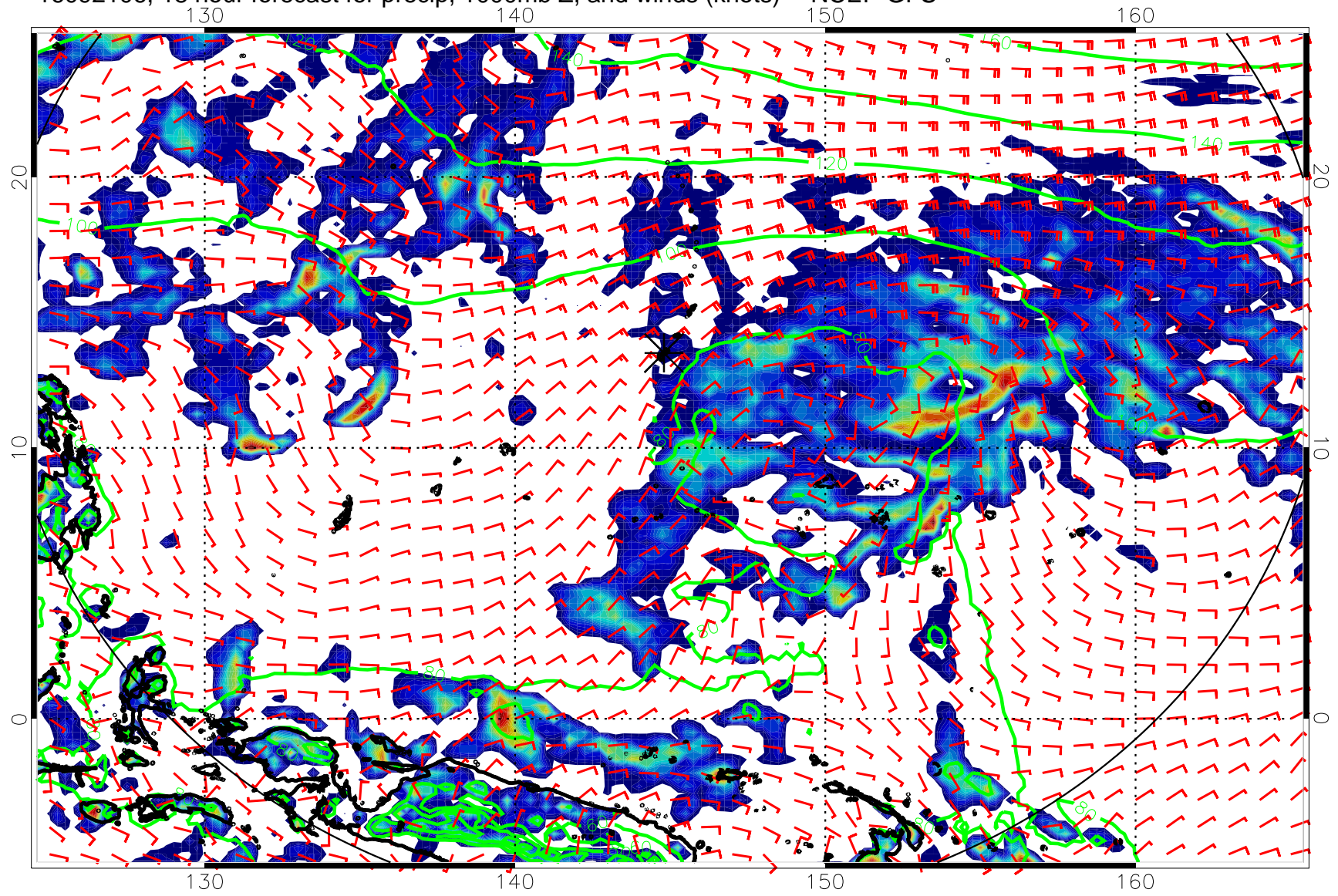
16092106, 18 hour forecast for precip, 1000mb Z, and winds (knots) -- NCEP GFS
