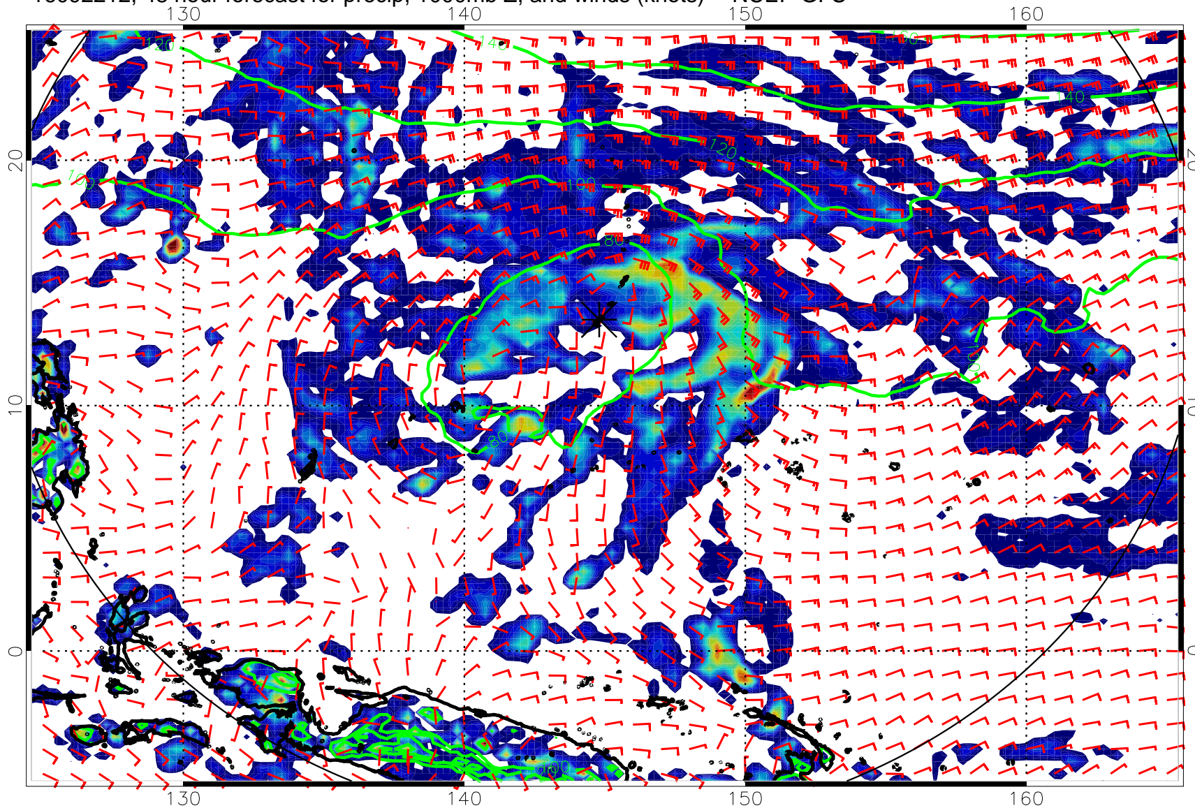
16092212, 48 hour forecast for precip, 1000mb Z, and winds (knots) -- NCEP GFS
