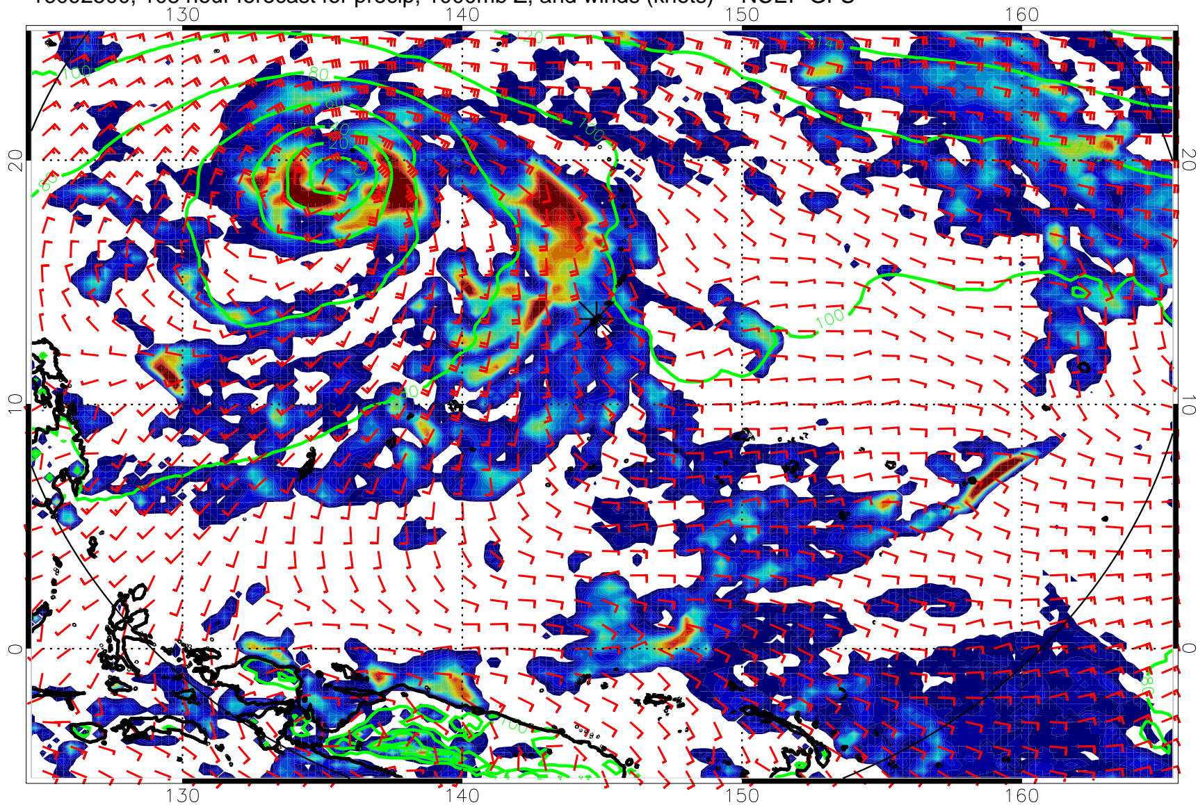
16092500, 108 hour forecast for precip, 1000mb Z, and winds (knots) -- NCEP GFS
