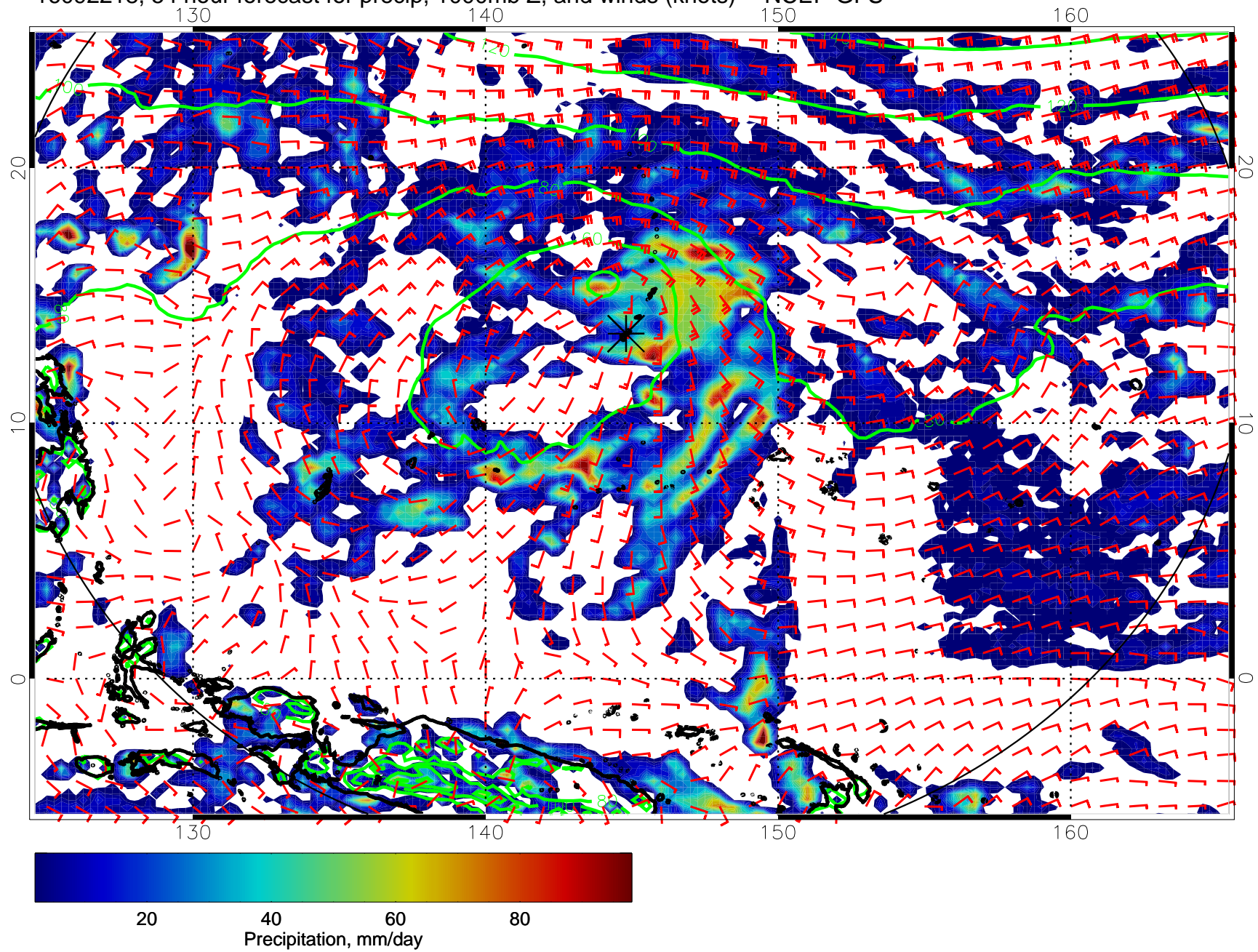
16092218, 54 hour forecast for precip, 1000mb Z, and winds (knots) -- NCEP GFS
