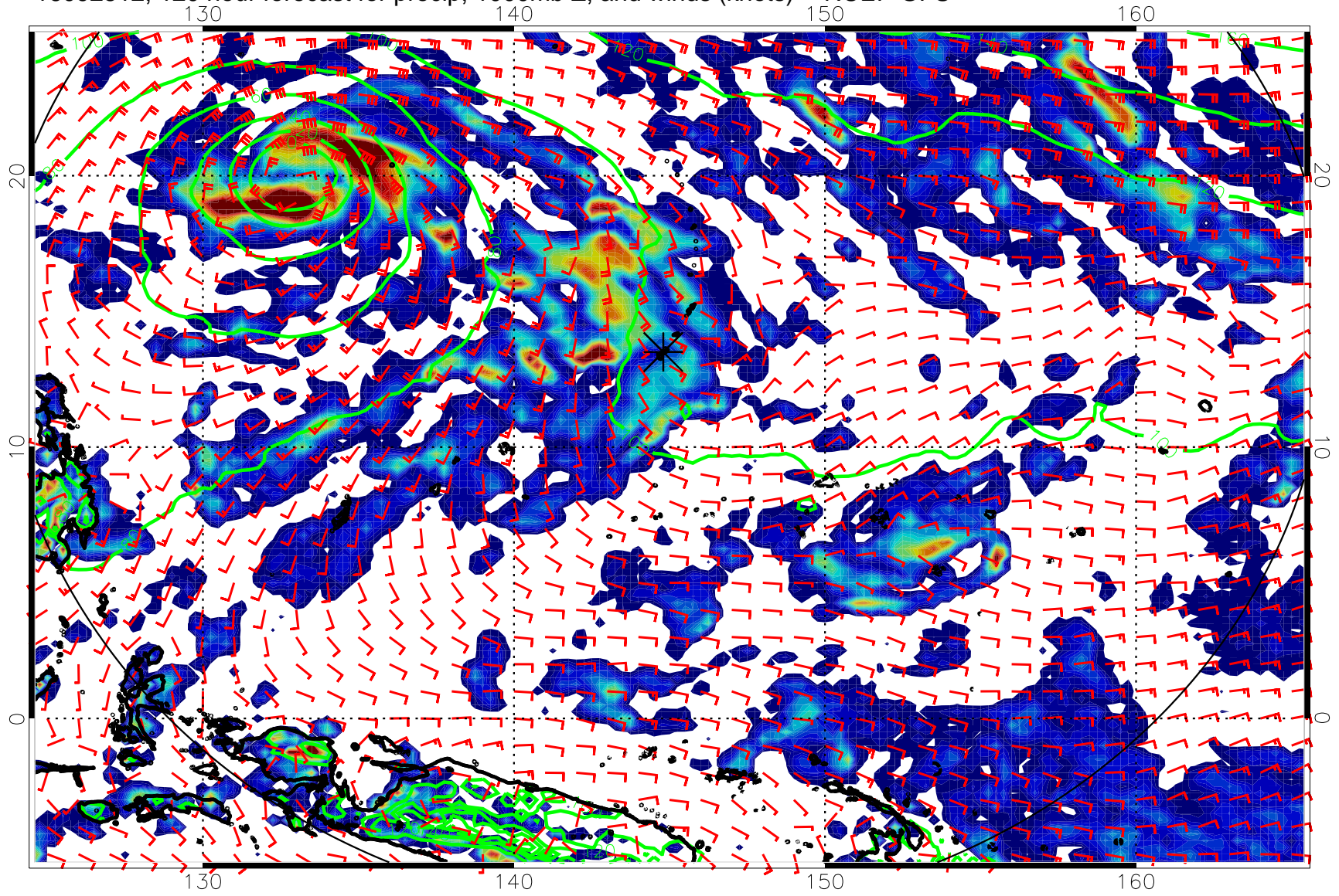
16092512, 120 hour forecast for precip, 1000mb Z, and winds (knots) -- NCEP GFS
