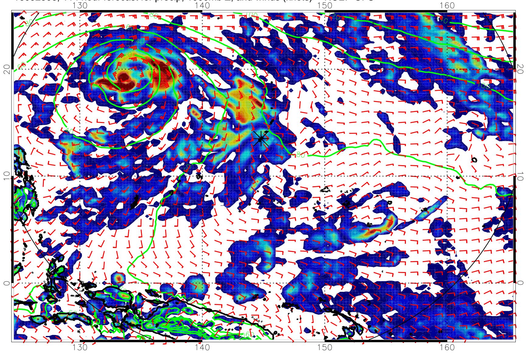
16092506, 114 hour forecast for precip, 1000mb Z, and winds (knots) -- NCEP GFS
