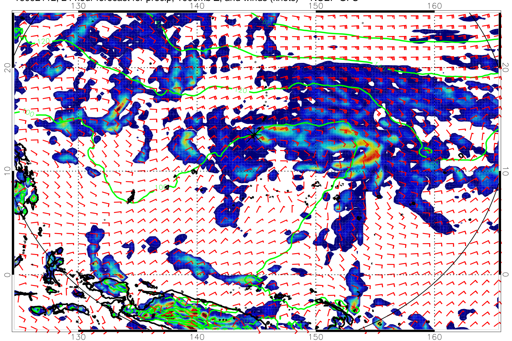
16092112, 24 hour forecast for precip, 1000mb Z, and winds (knots) -- NCEP GFS
