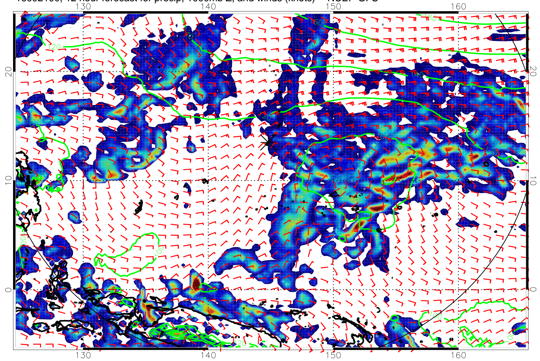
16092100, 12 hour forecast for precip, 1000mb Z, and winds (knots) -- NCEP GFS
