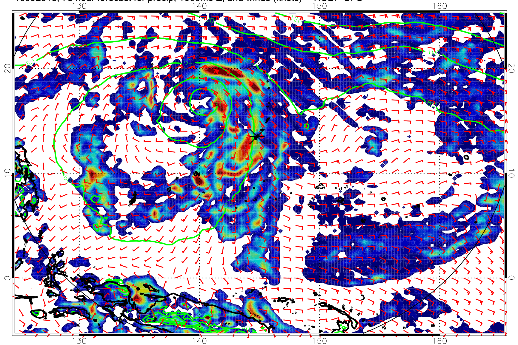
16092318, 78 hour forecast for precip, 1000mb Z, and winds (knots) -- NCEP GFS
