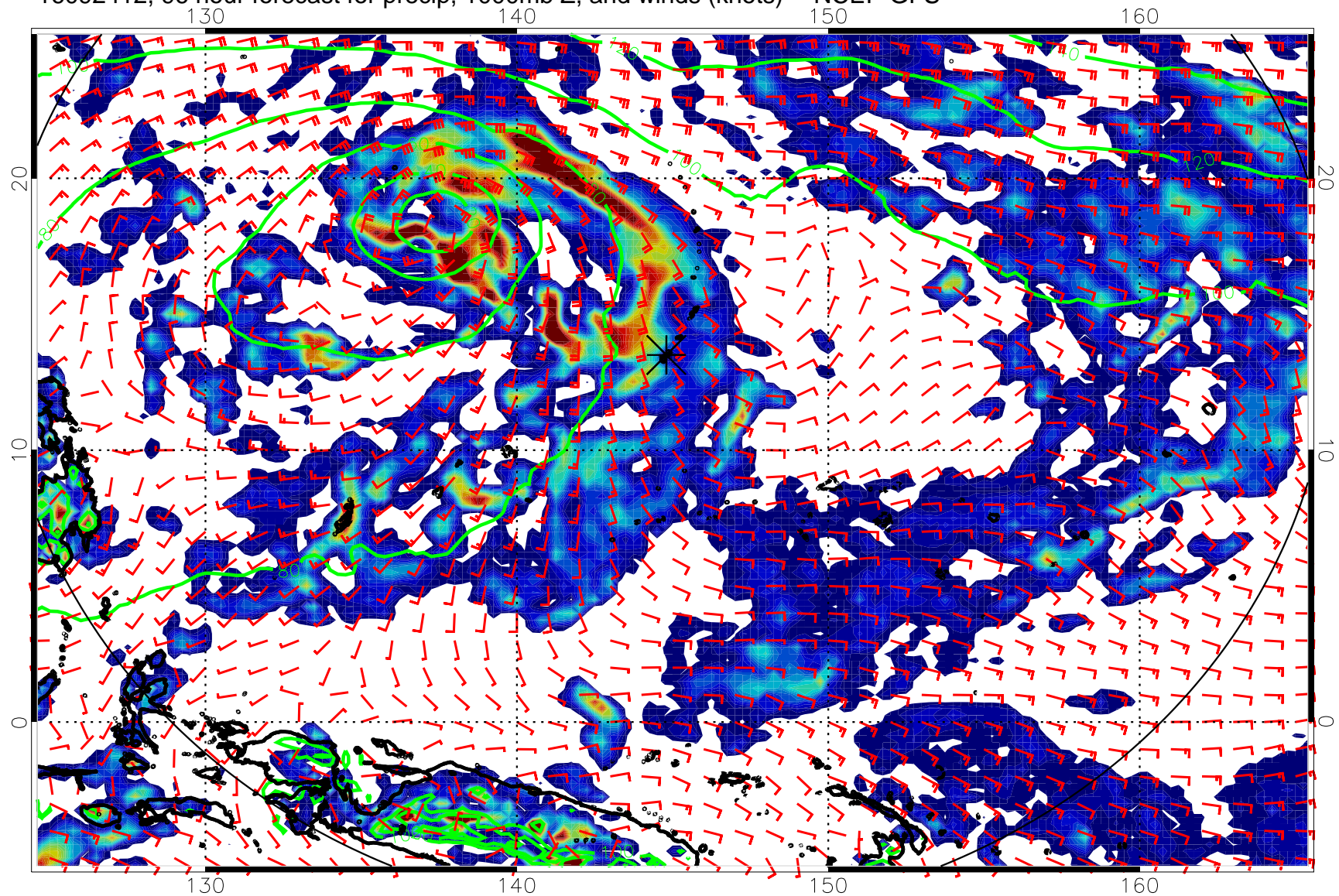
16092412, 96 hour forecast for precip, 1000mb Z, and winds (knots) -- NCEP GFS
