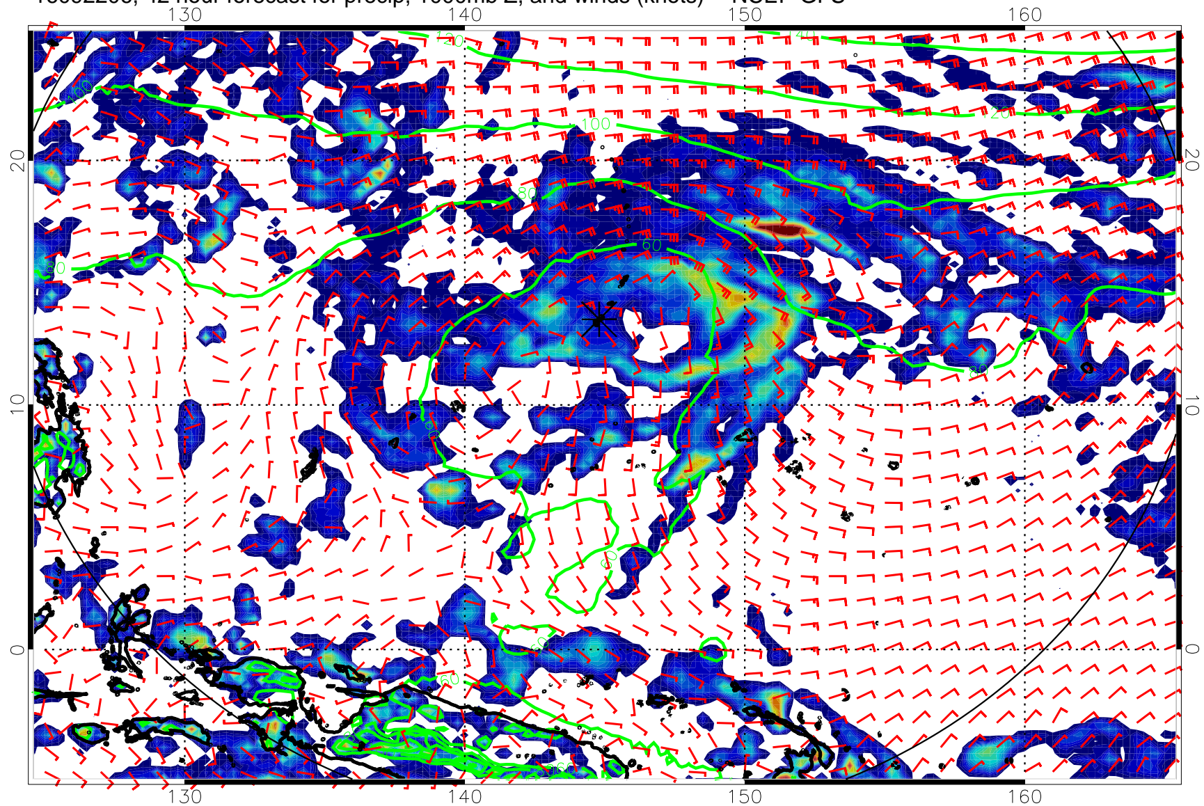
16092206, 42 hour forecast for precip, 1000mb Z, and winds (knots) -- NCEP GFS
