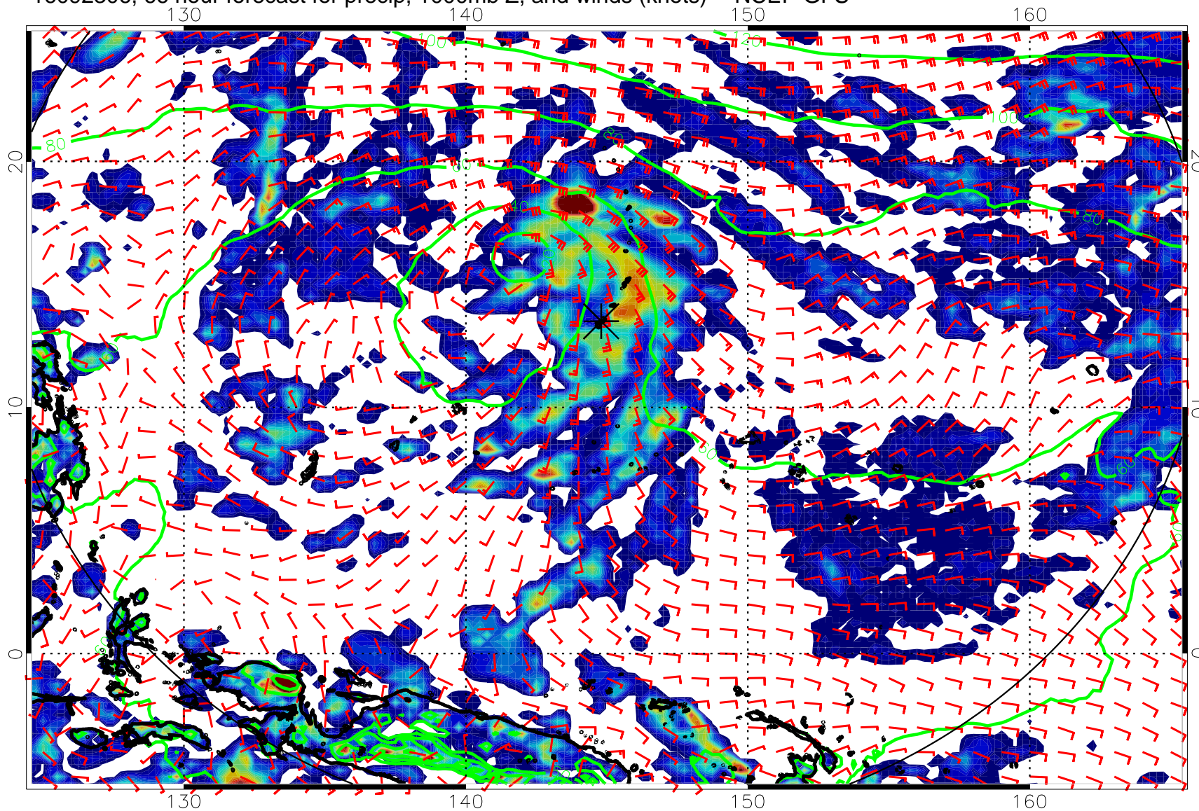
16092306, 66 hour forecast for precip, 1000mb Z, and winds (knots) -- NCEP GFS
