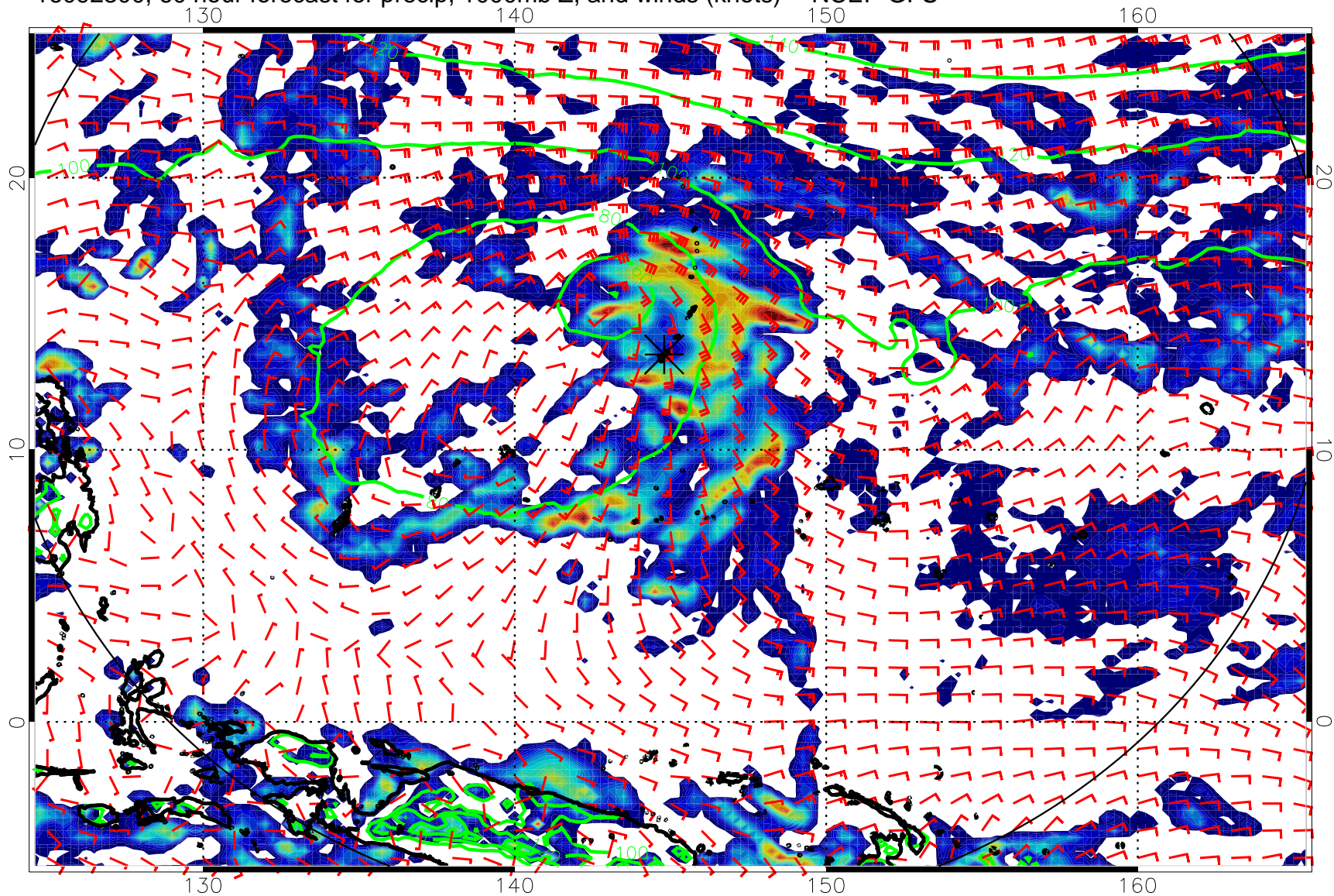
16092300, 60 hour forecast for precip, 1000mb Z, and winds (knots) -- NCEP GFS
