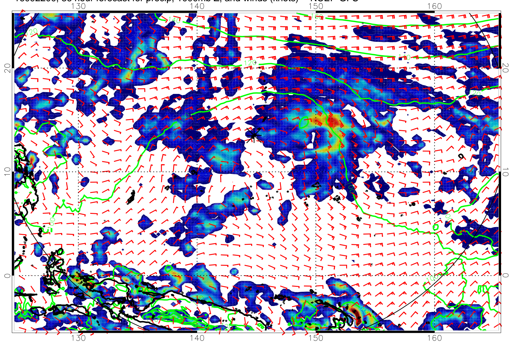
16092200, 36 hour forecast for precip, 1000mb Z, and winds (knots) -- NCEP GFS
