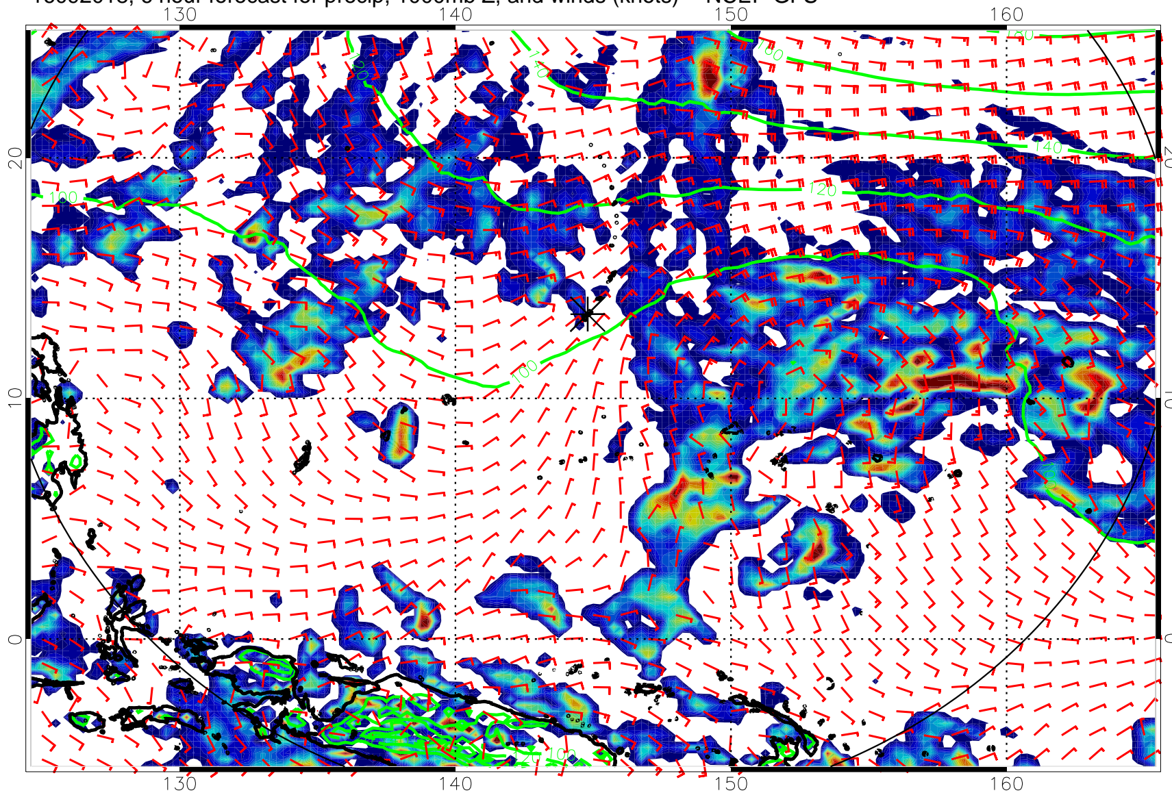
16092018, 6 hour forecast for precip, 1000mb Z, and winds (knots) -- NCEP GFS
