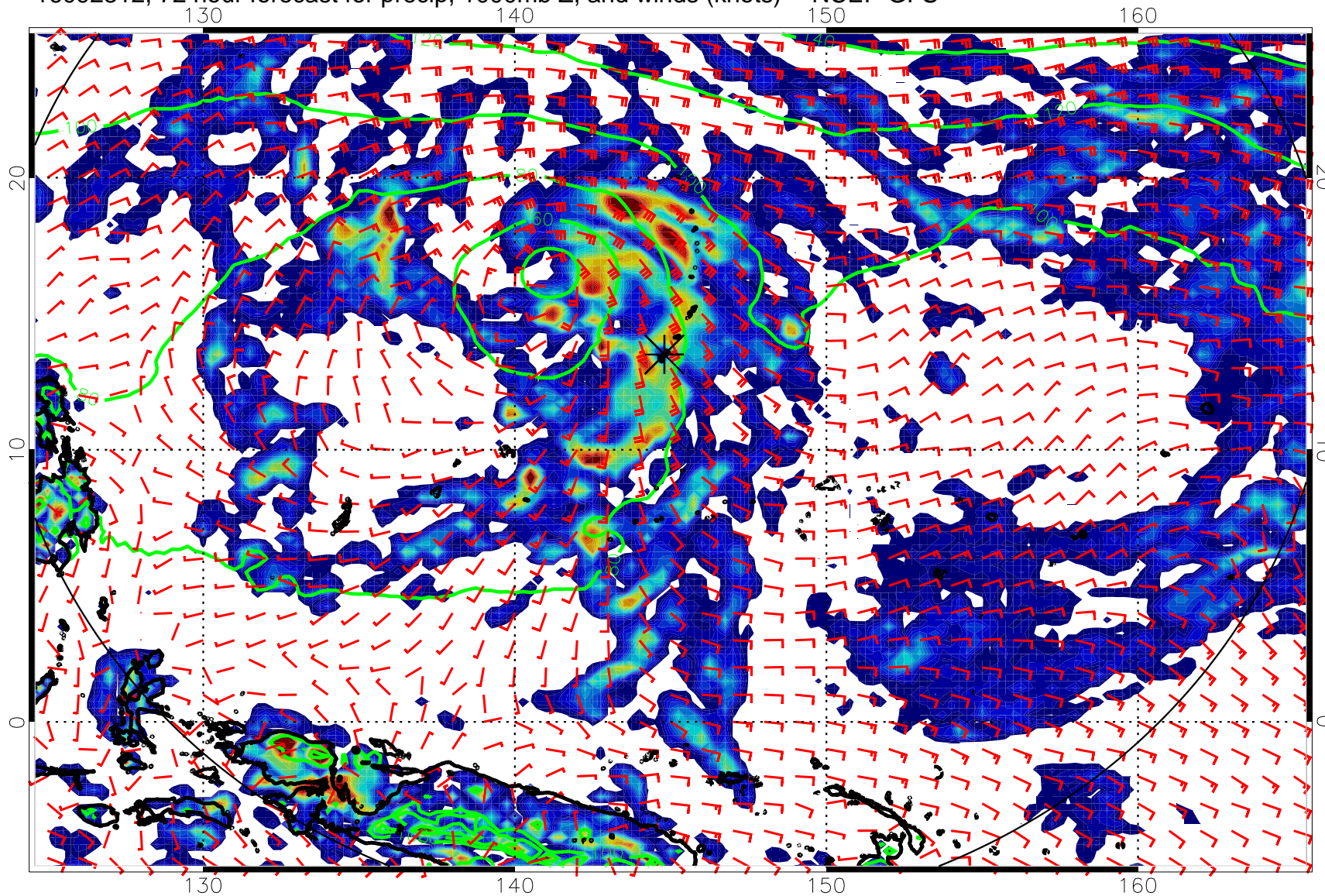
16092312, 72 hour forecast for precip, 1000mb Z, and winds (knots) -- NCEP GFS
