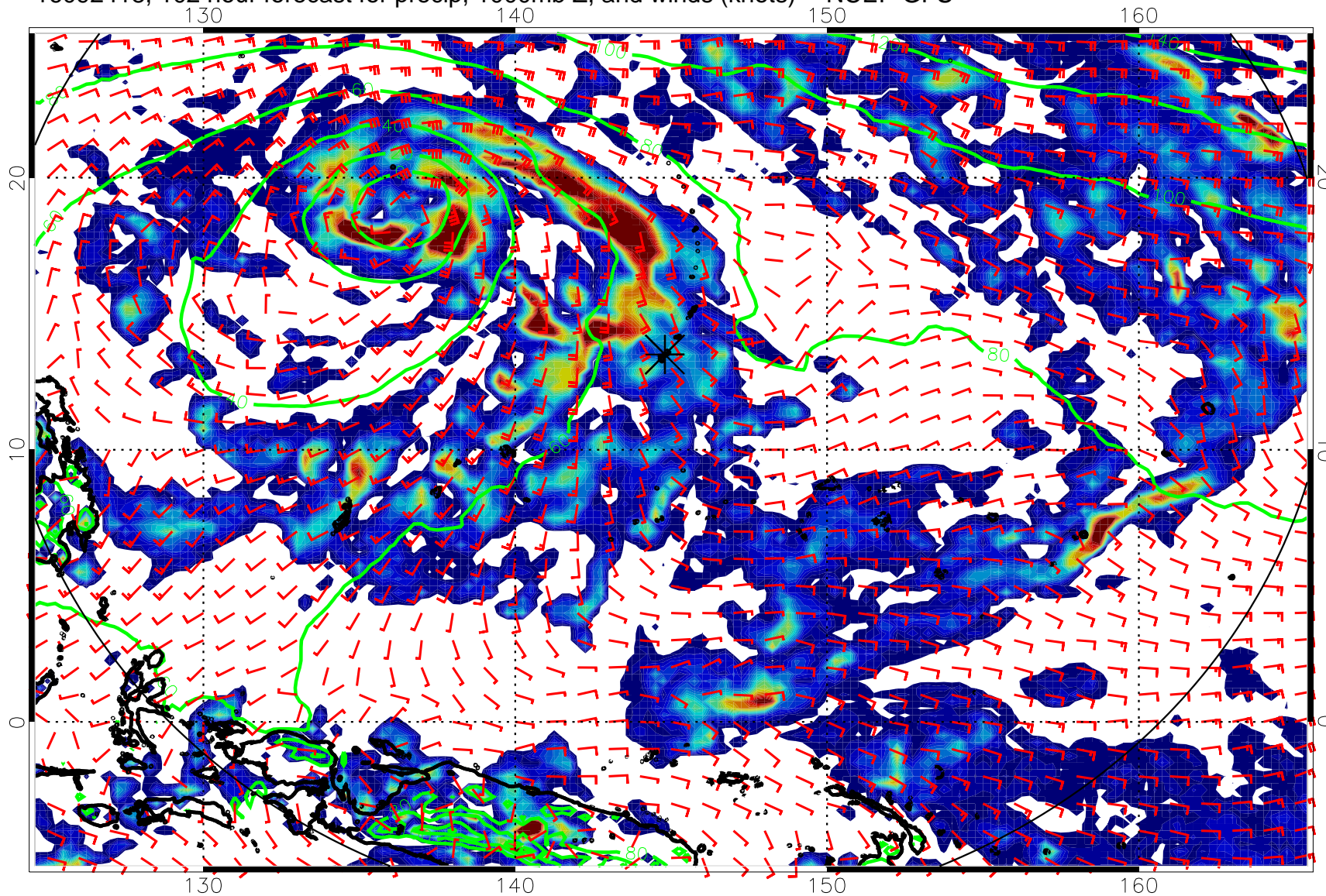
16092418, 102 hour forecast for precip, 1000mb Z, and winds (knots) -- NCEP GFS
