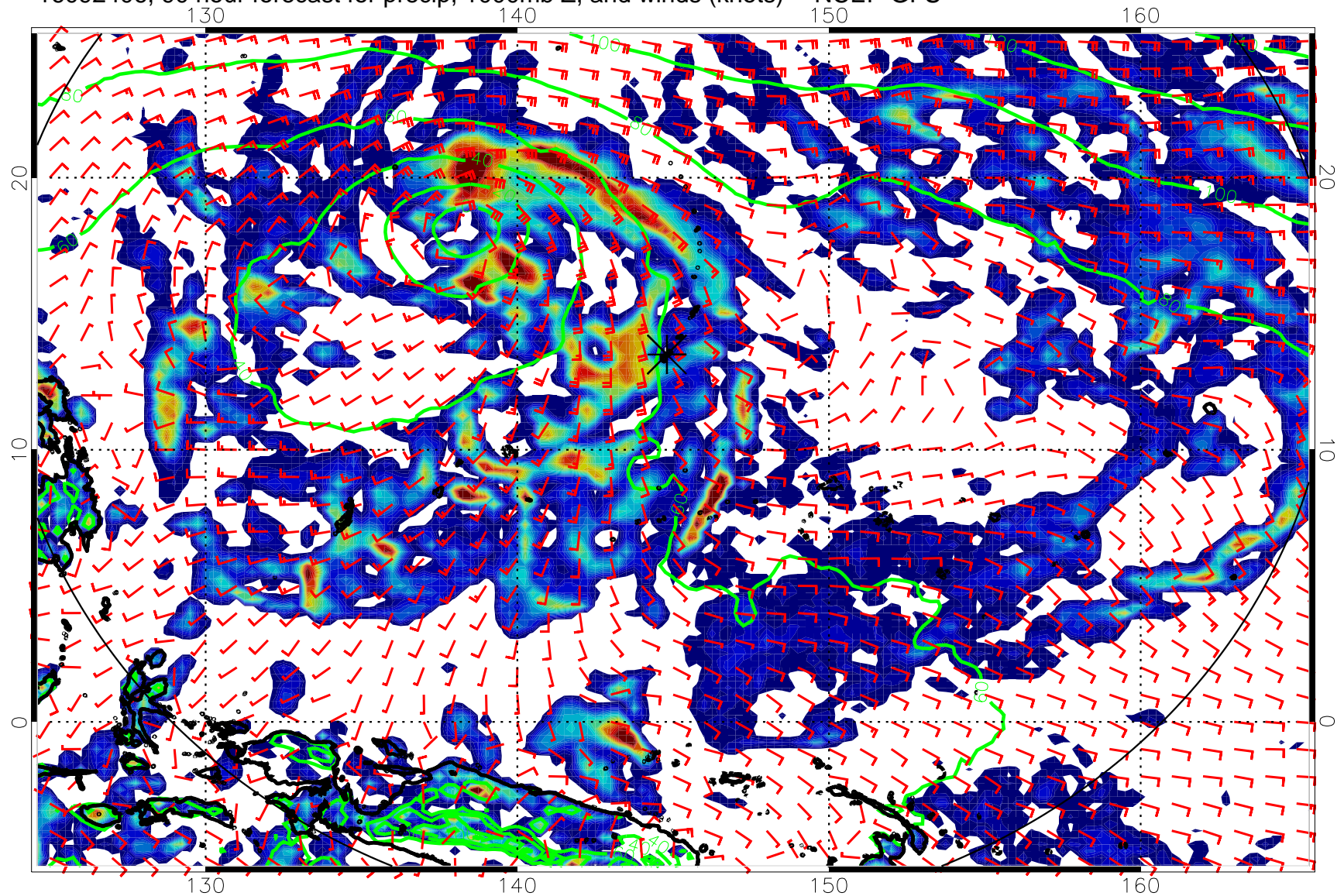
16092406, 90 hour forecast for precip, 1000mb Z, and winds (knots) -- NCEP GFS
