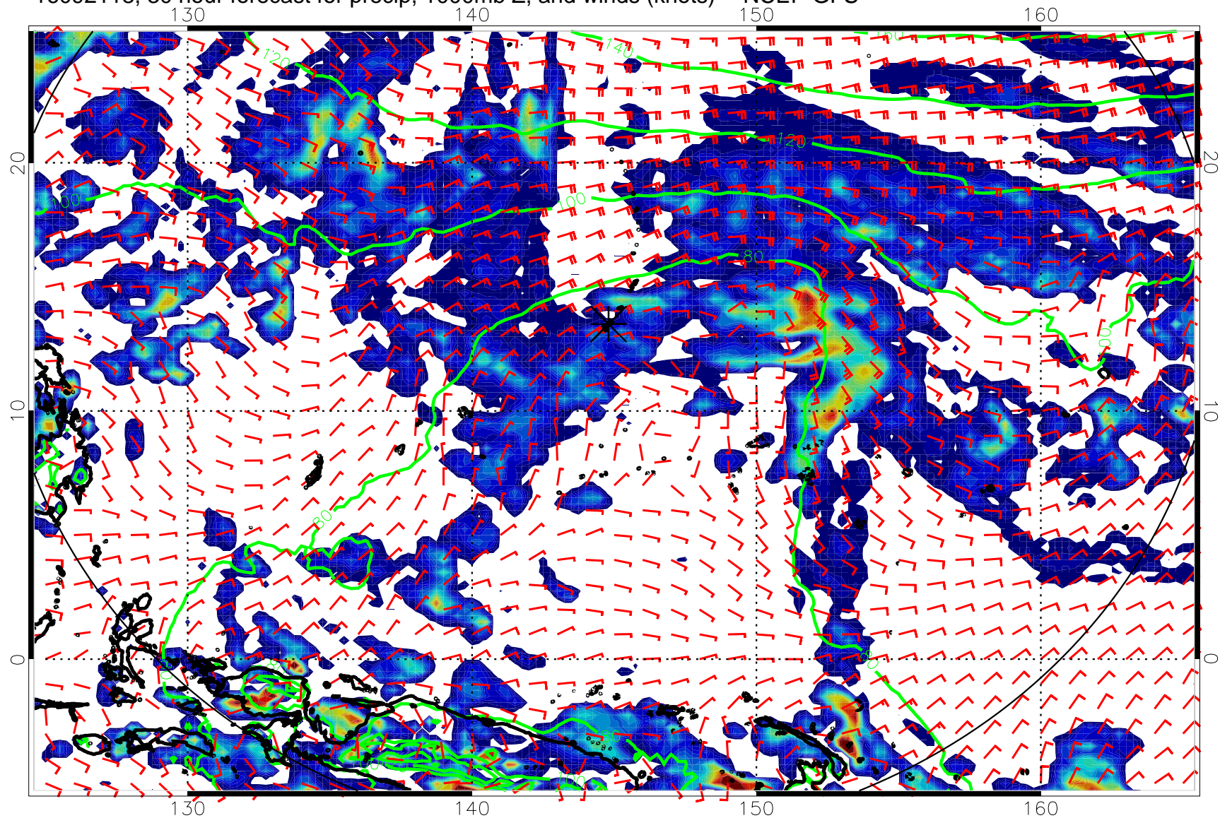
16092118, 30 hour forecast for precip, 1000mb Z, and winds (knots) -- NCEP GFS
