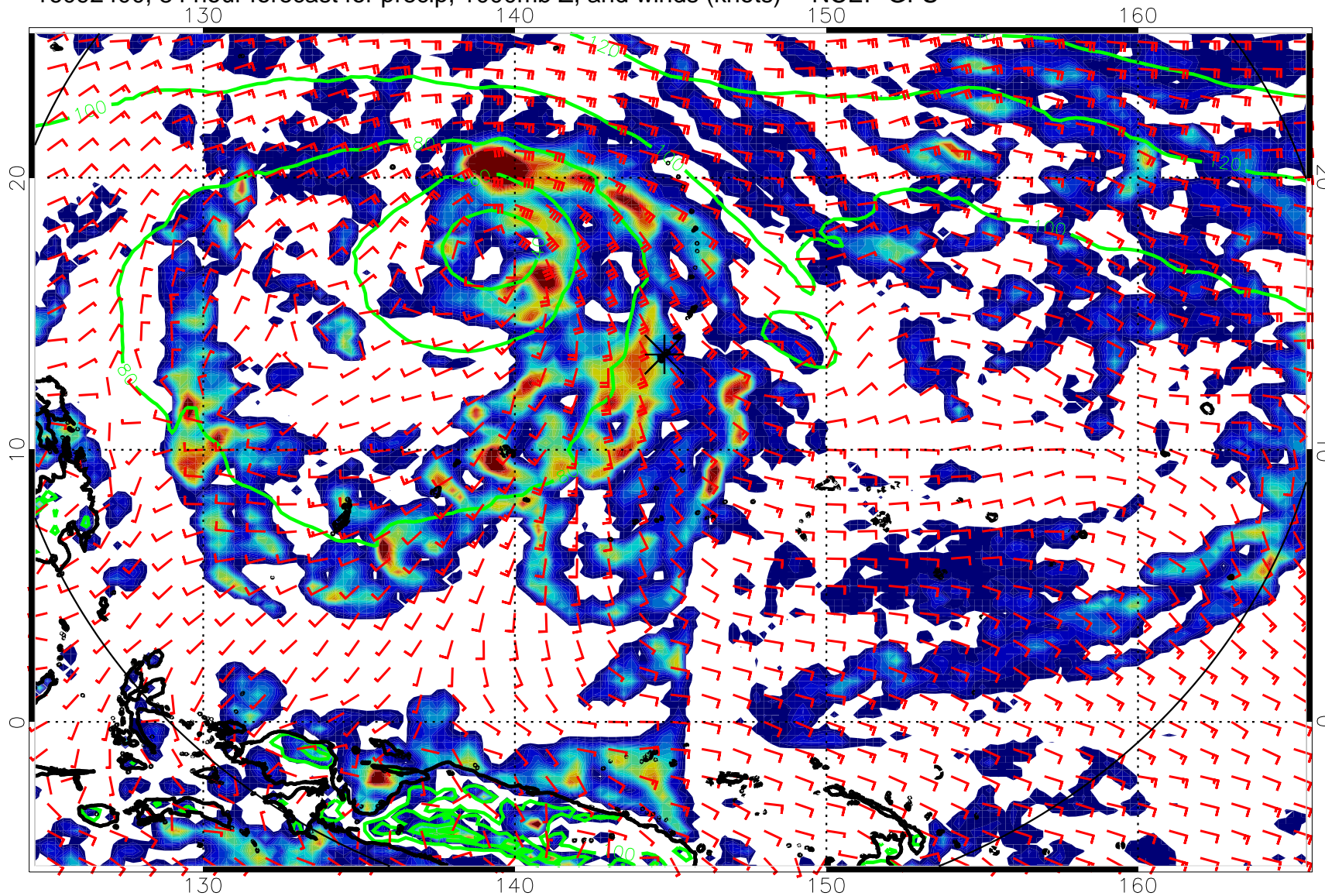
16092400, 84 hour forecast for precip, 1000mb Z, and winds (knots) -- NCEP GFS
