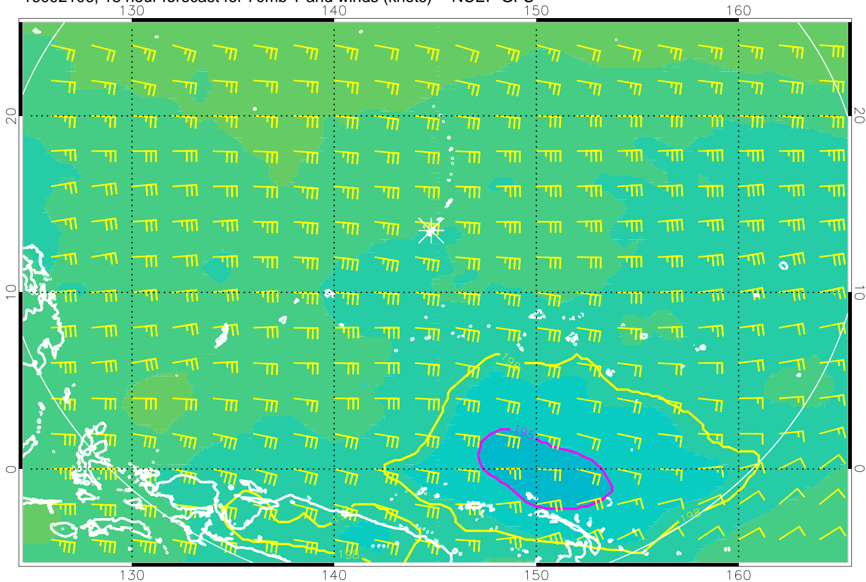
16092106, 18 hour forecast for 70mb T and winds (knots) -- NCEP GFS
