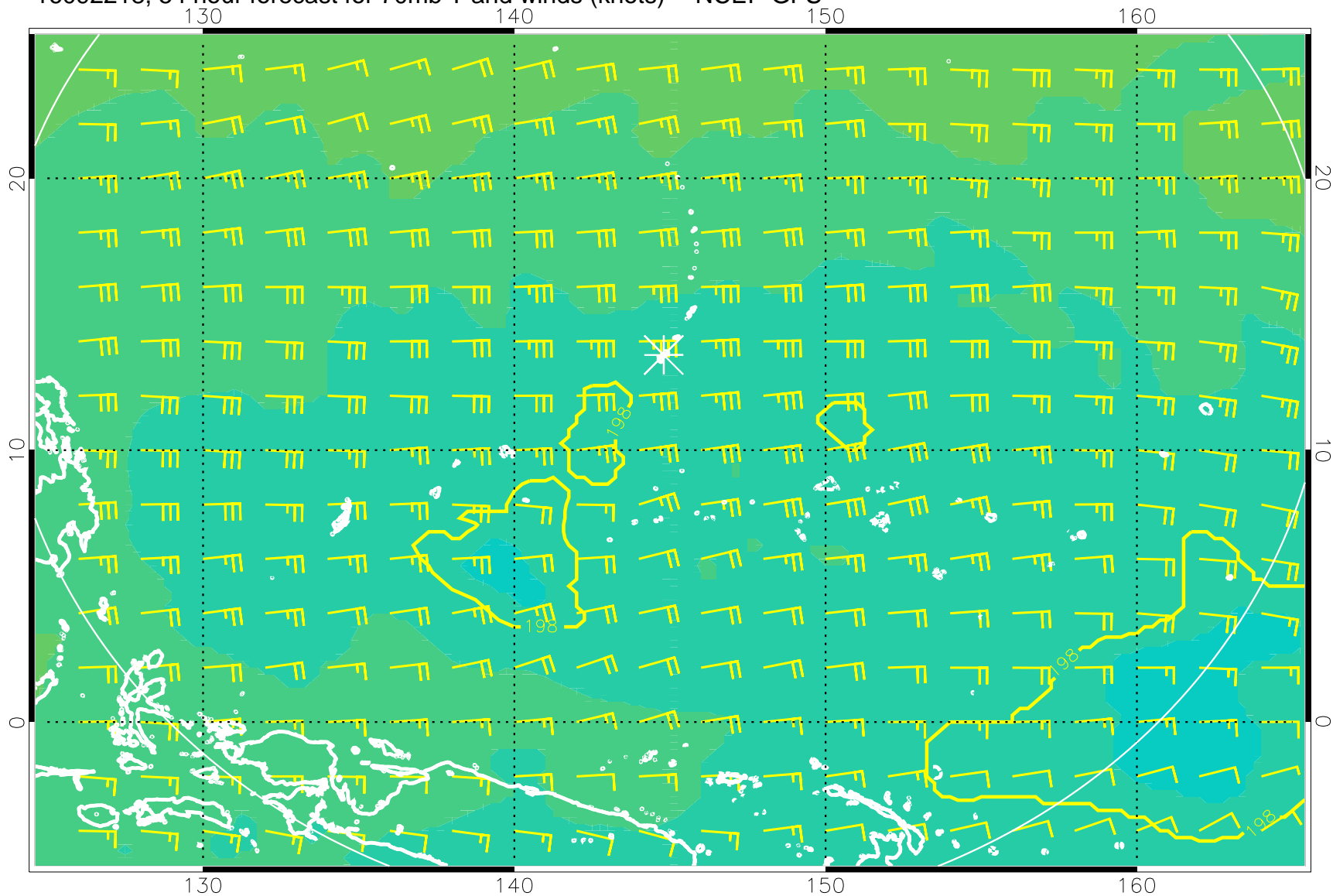
16092218, 54 hour forecast for 70mb T and winds (knots) -- NCEP GFS
