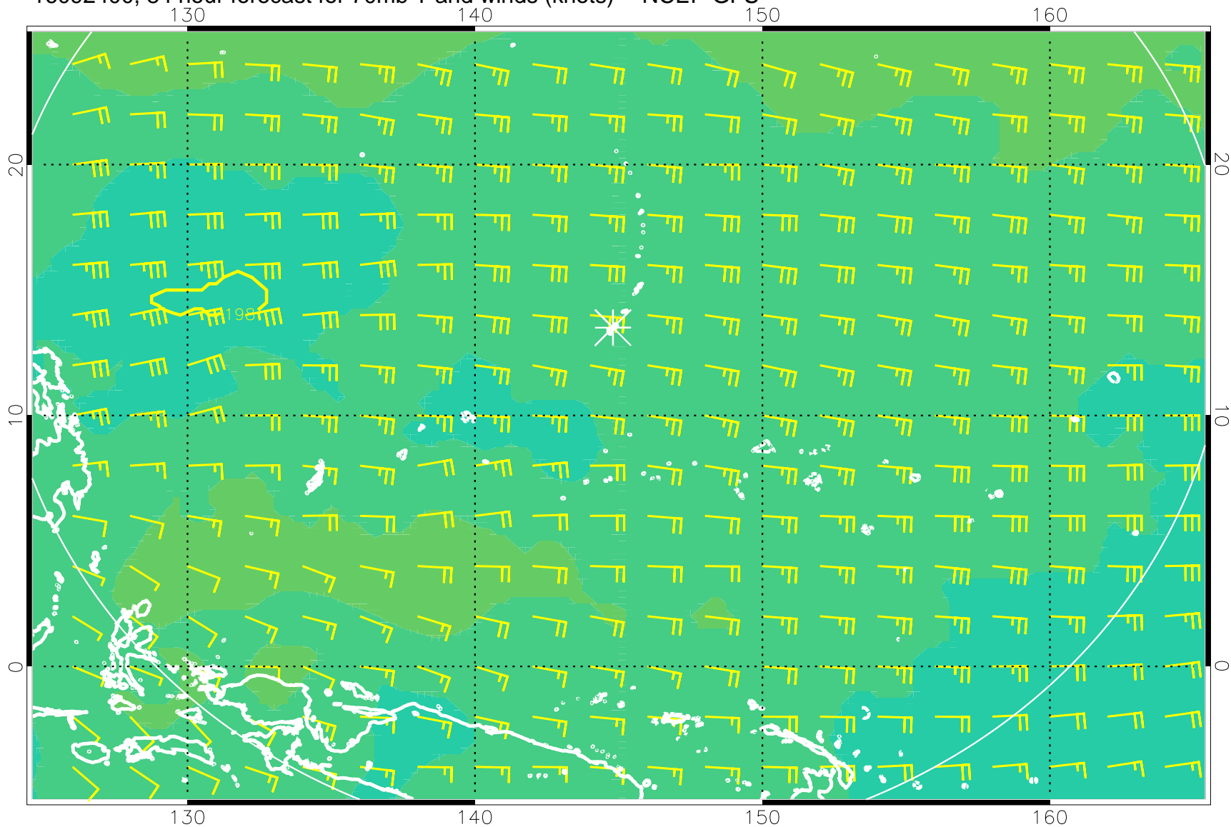
16092400, 84 hour forecast for 70mb T and winds (knots) -- NCEP GFS
