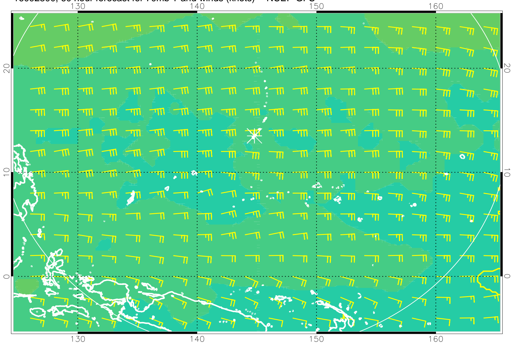
16092300, 60 hour forecast for 70mb T and winds (knots) -- NCEP GFS
