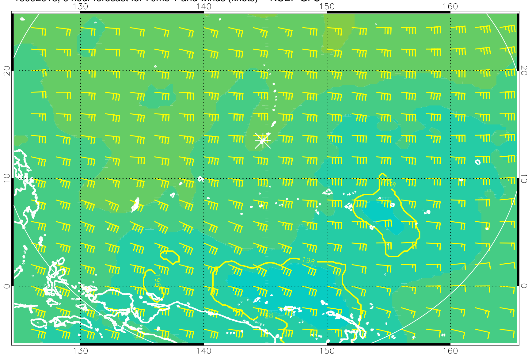
16092018, 6 hour forecast for 70mb T and winds (knots) -- NCEP GFS
