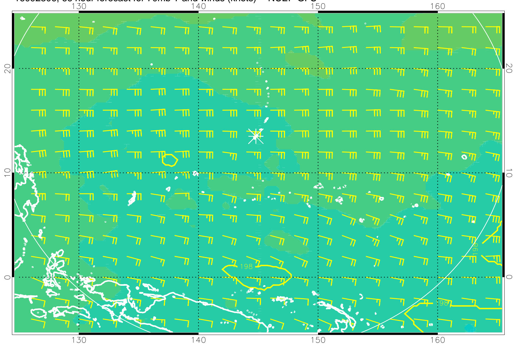
16092306, 66 hour forecast for 70mb T and winds (knots) -- NCEP GFS
