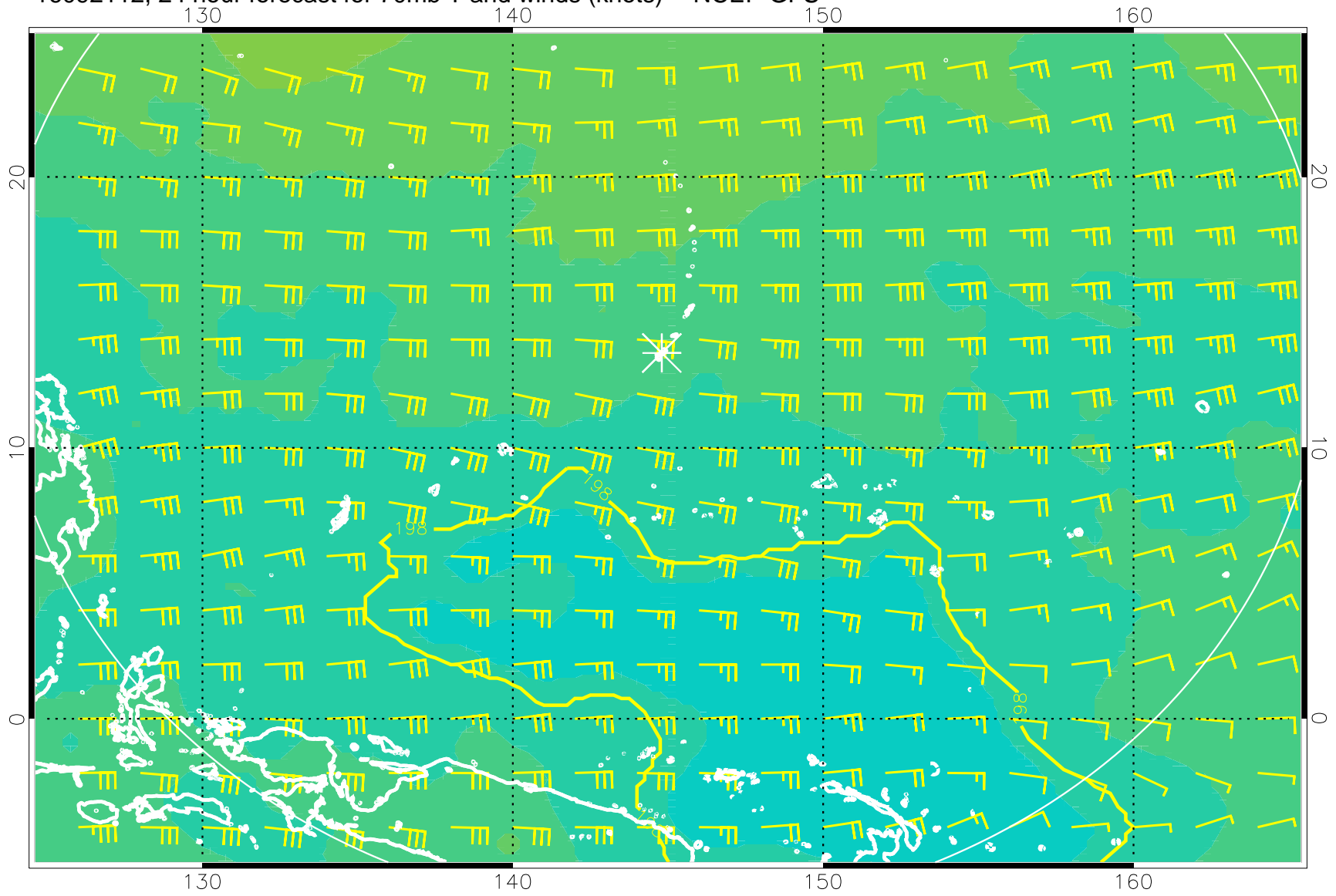
16092112, 24 hour forecast for 70mb T and winds (knots) -- NCEP GFS
