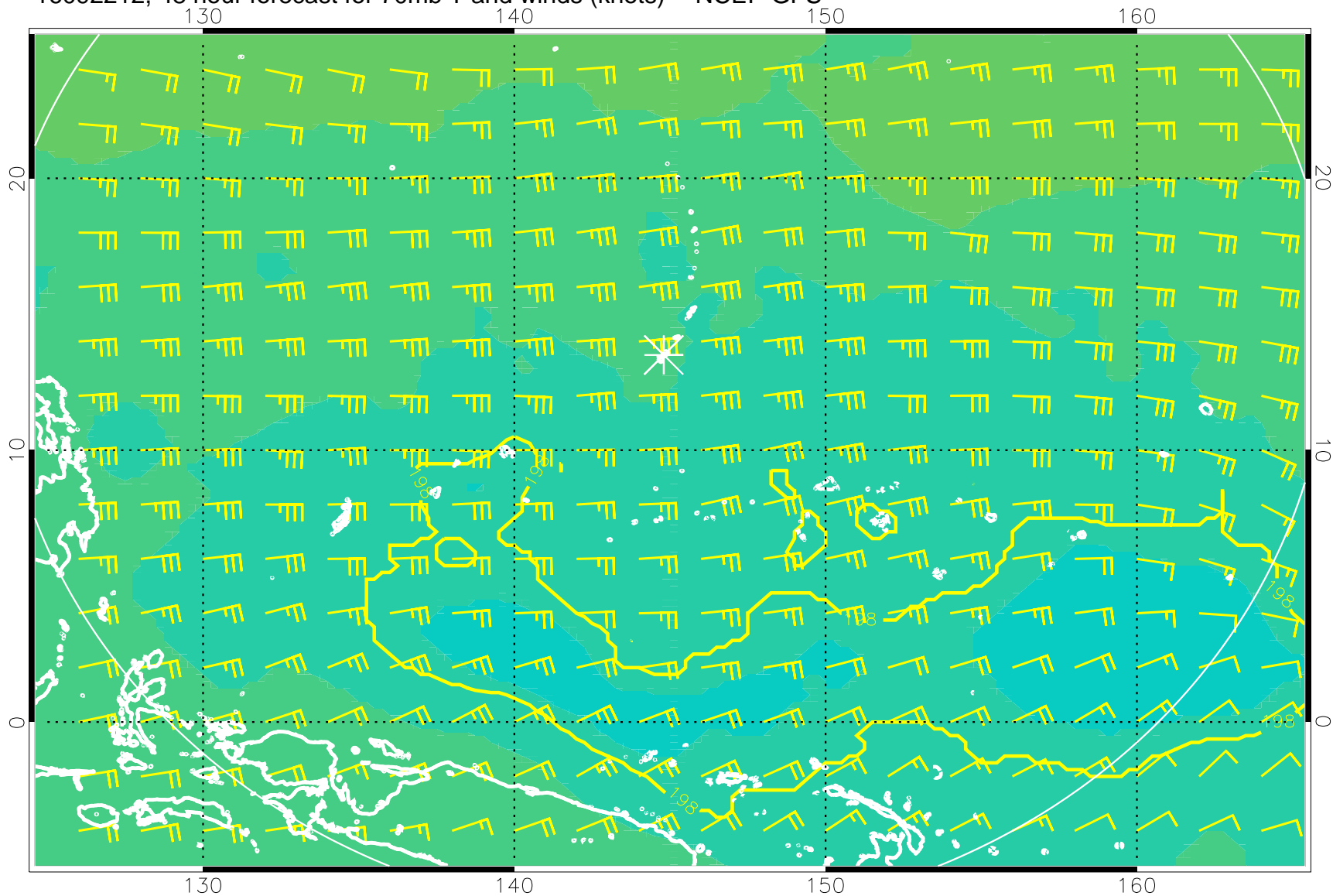
16092212, 48 hour forecast for 70mb T and winds (knots) -- NCEP GFS
