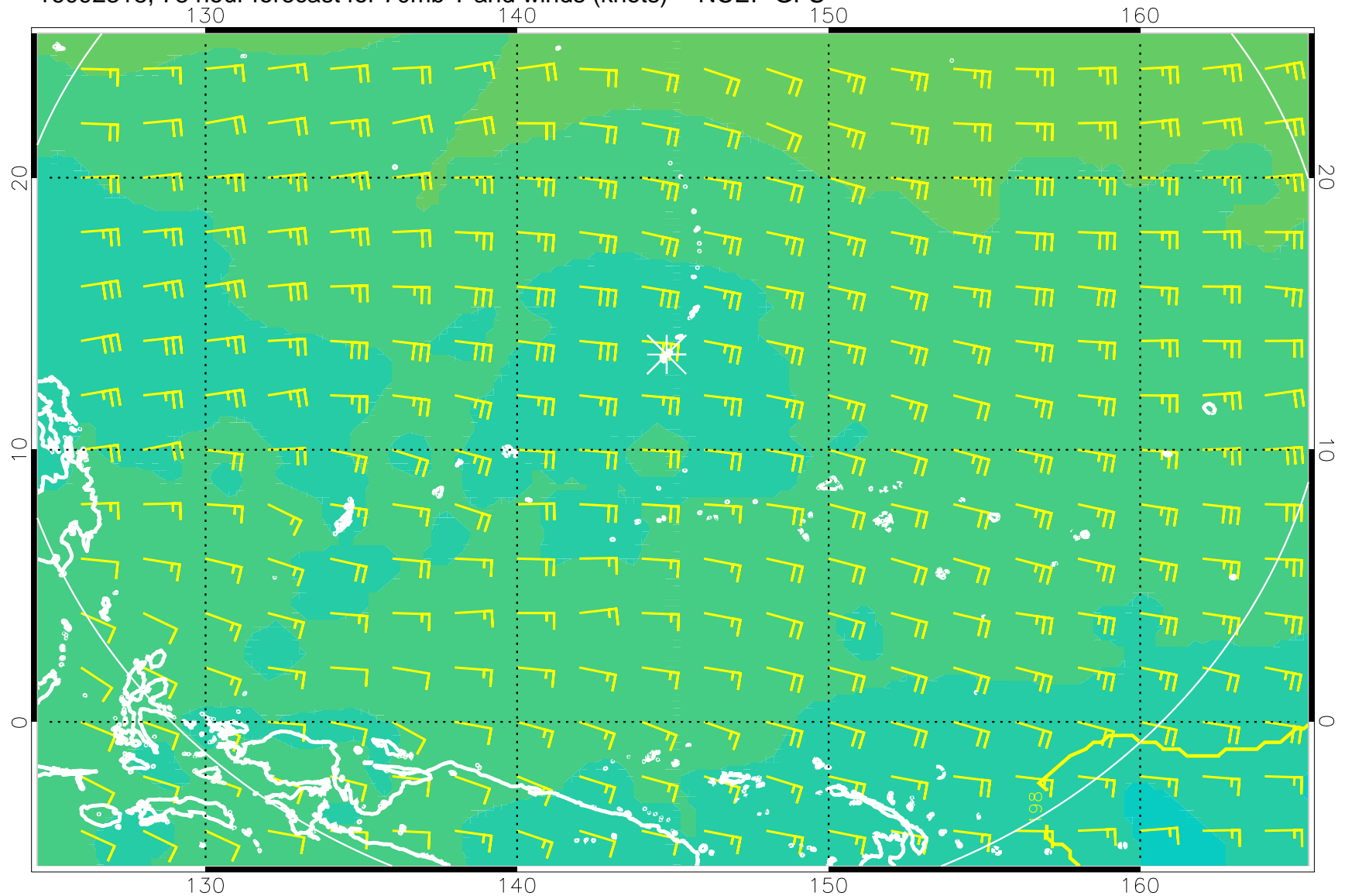
16092318, 78 hour forecast for 70mb T and winds (knots) -- NCEP GFS
