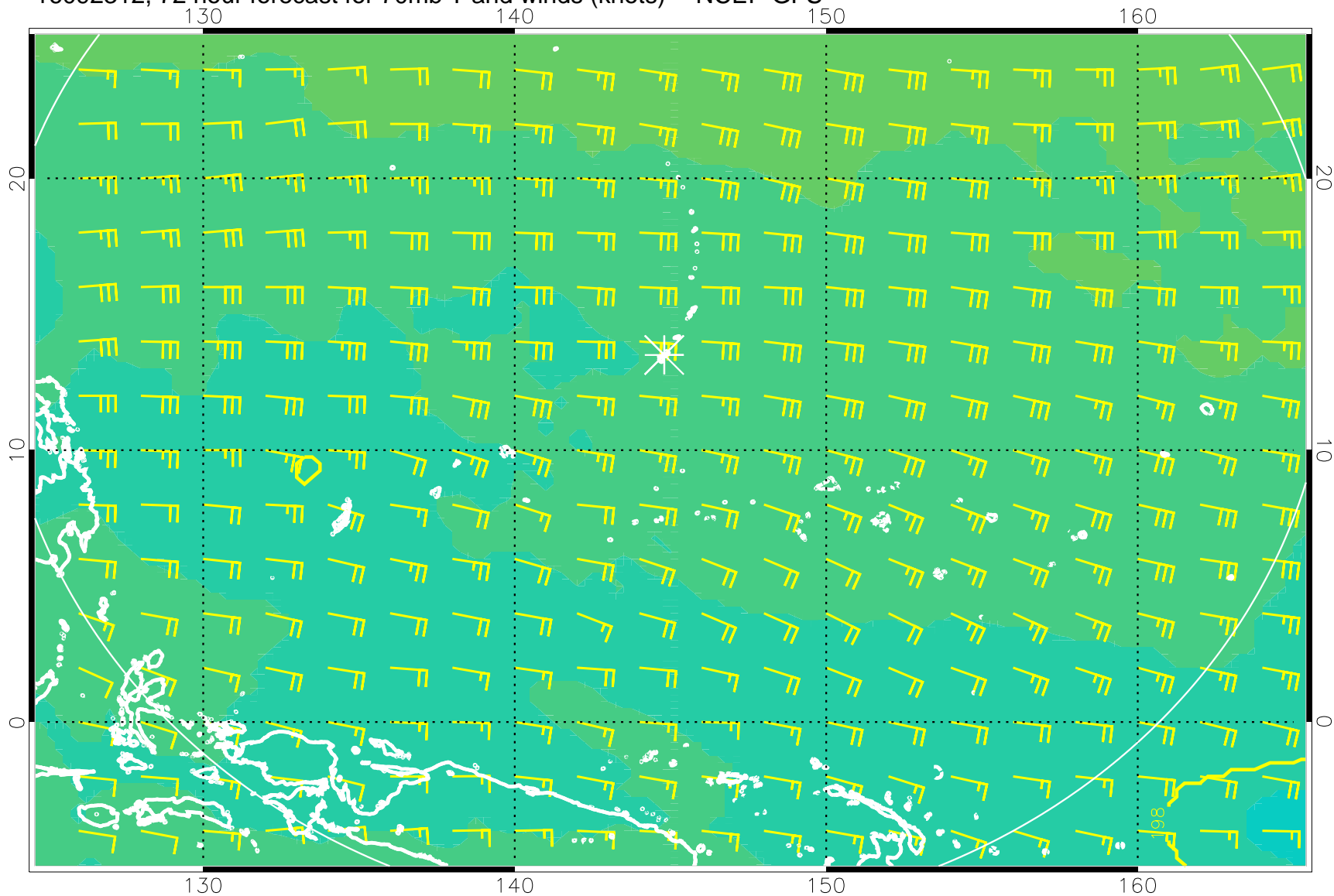
16092312, 72 hour forecast for 70mb T and winds (knots) -- NCEP GFS
