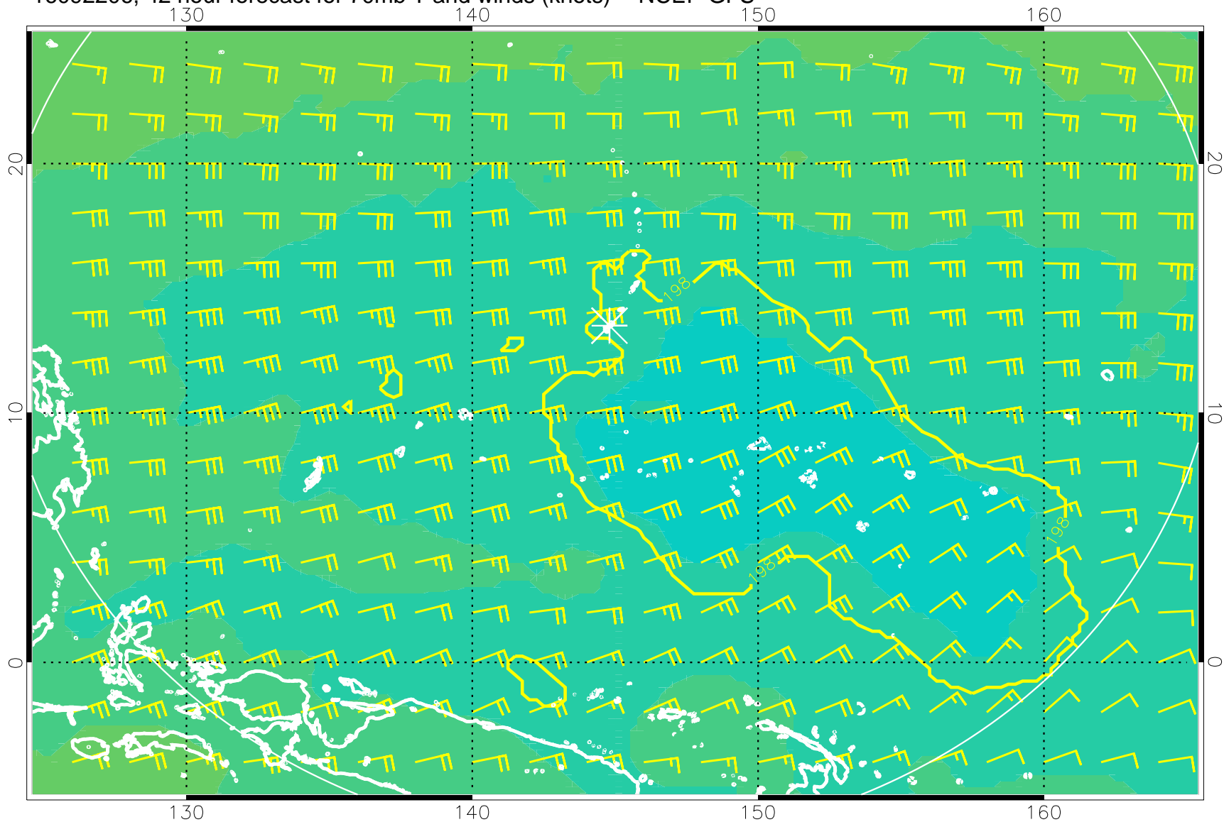
16092206, 42 hour forecast for 70mb T and winds (knots) -- NCEP GFS
