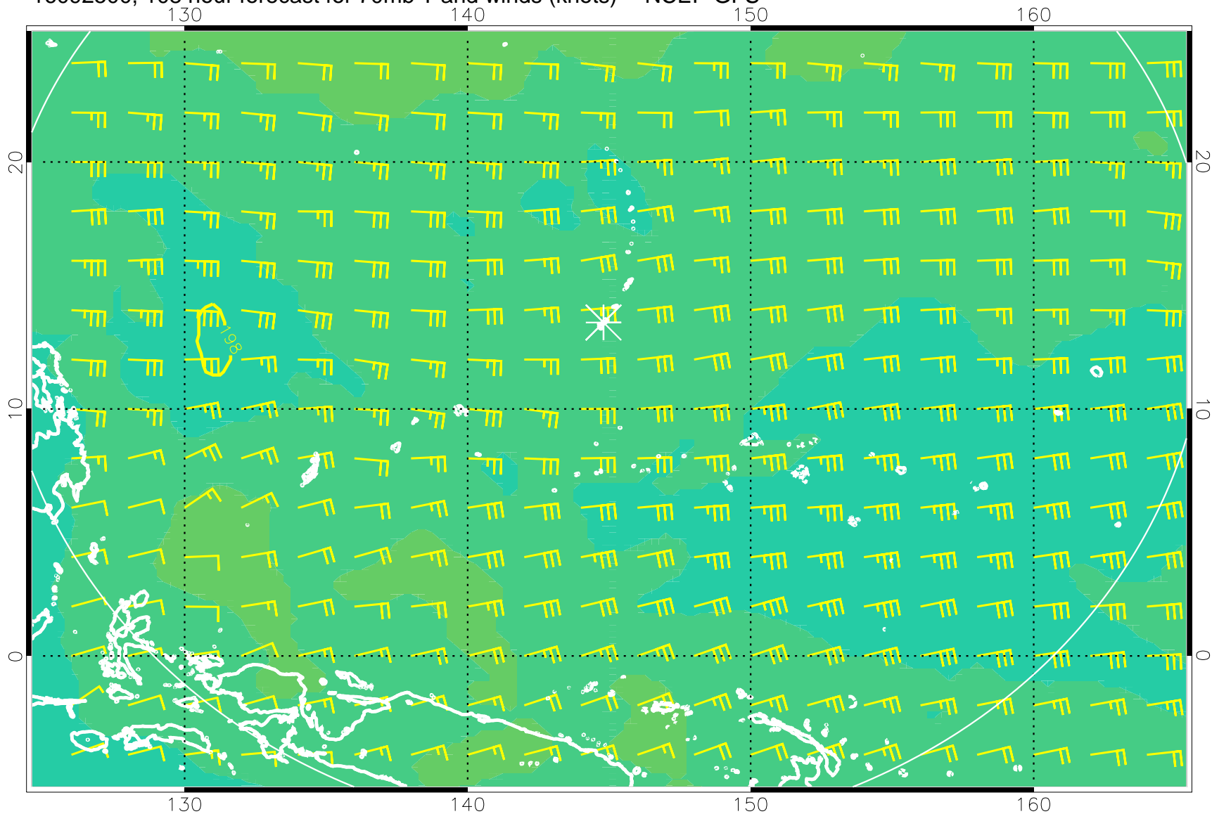
16092500, 108 hour forecast for 70mb T and winds (knots) -- NCEP GFS
