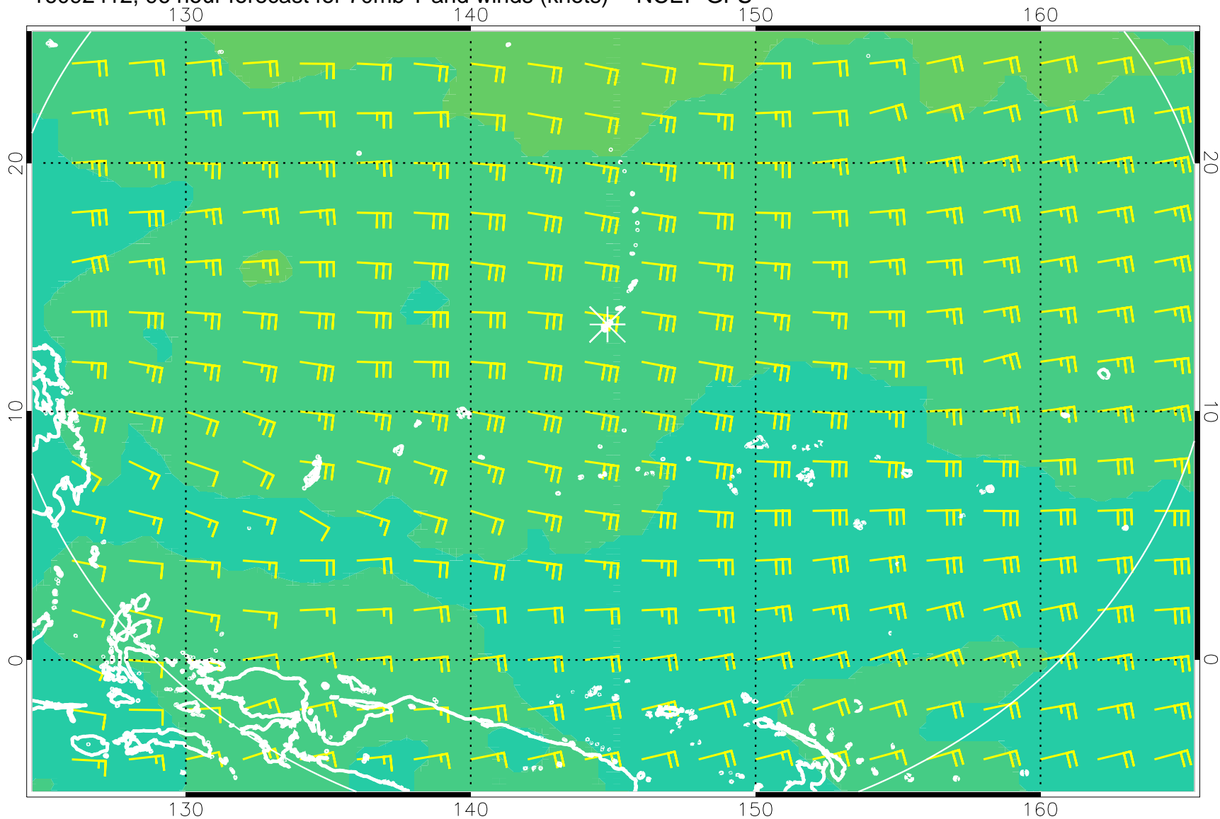
16092412, 96 hour forecast for 70mb T and winds (knots) -- NCEP GFS
