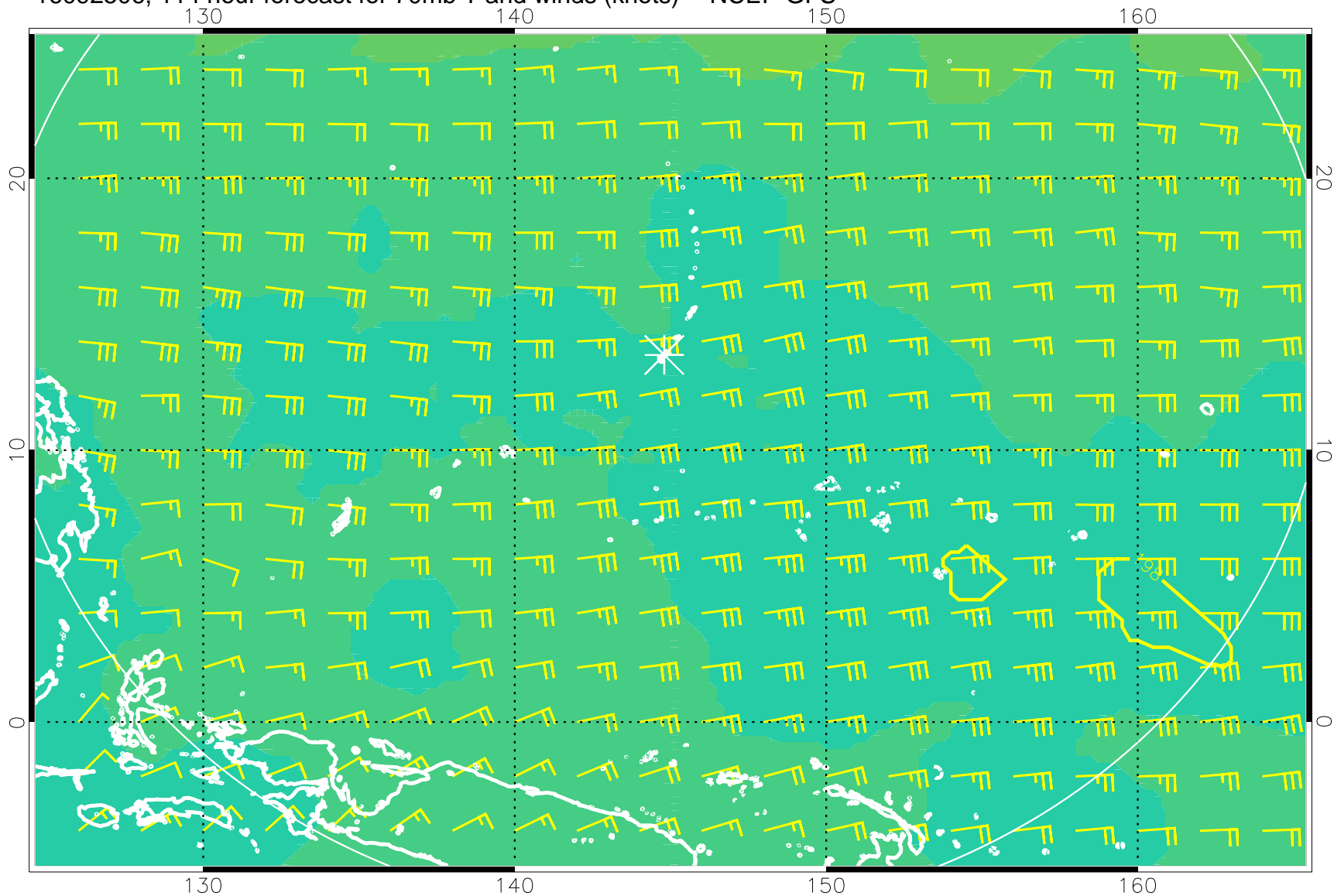
16092506, 114 hour forecast for 70mb T and winds (knots) -- NCEP GFS
