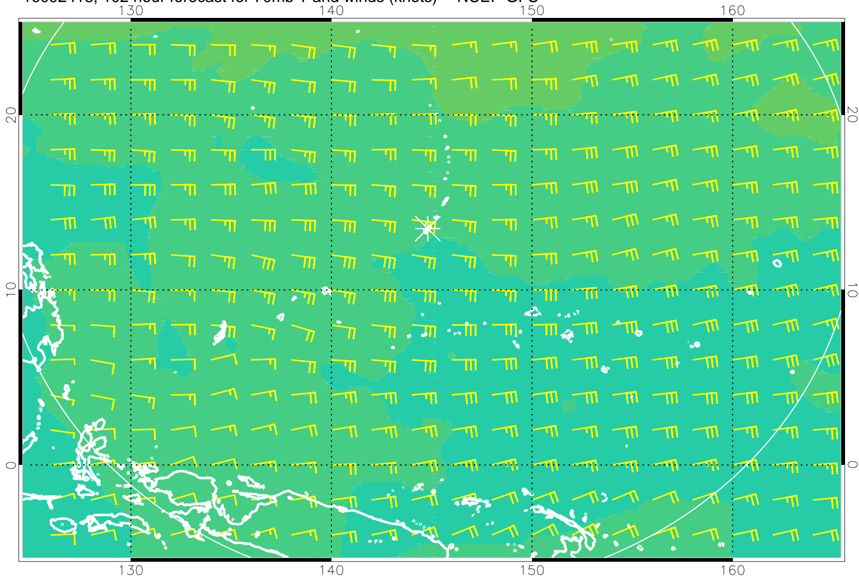
16092418, 102 hour forecast for 70mb T and winds (knots) -- NCEP GFS
