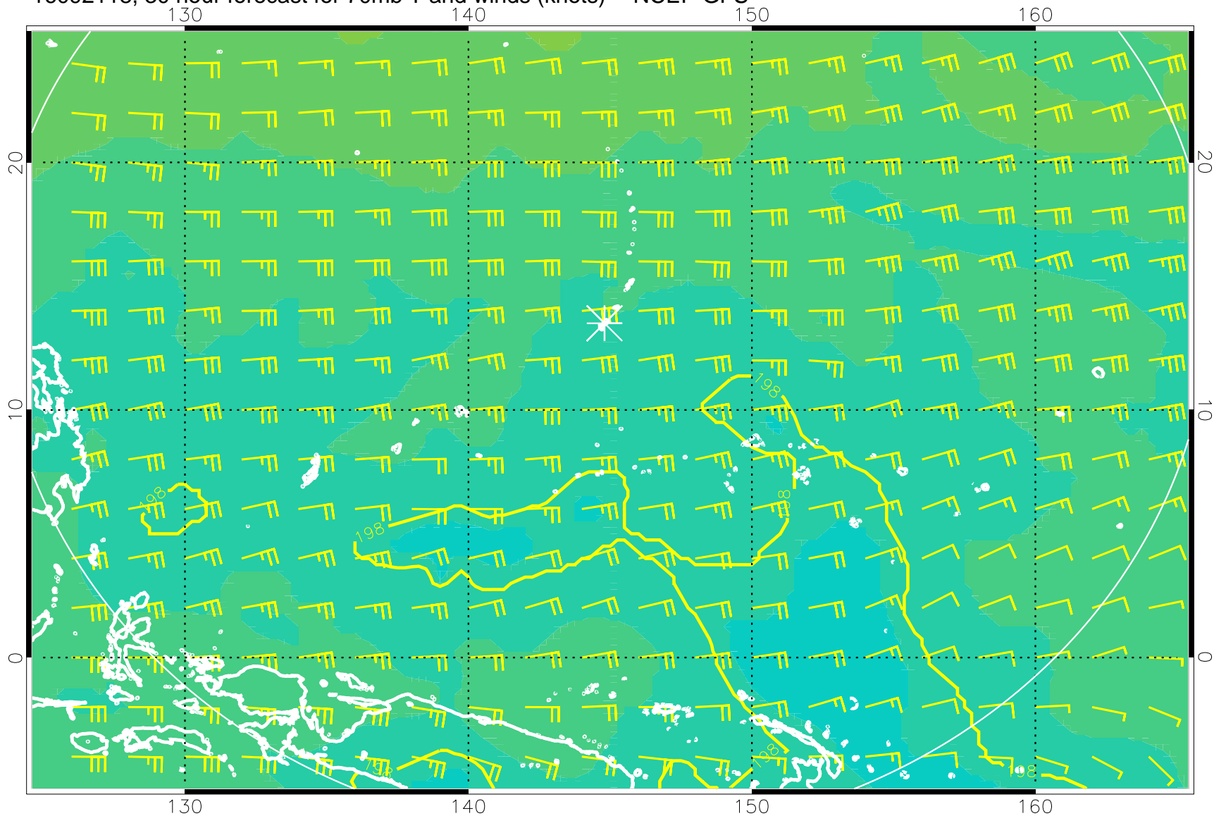
16092118, 30 hour forecast for 70mb T and winds (knots) -- NCEP GFS
