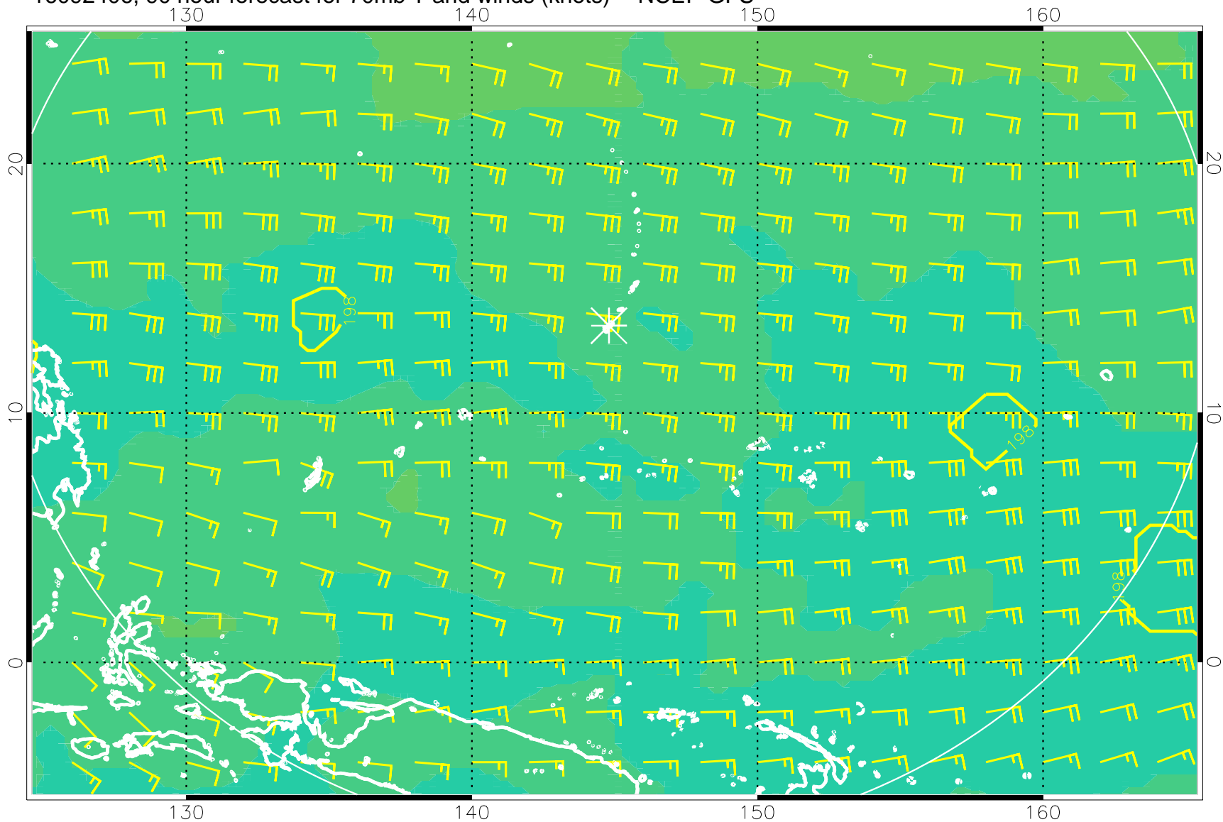
16092406, 90 hour forecast for 70mb T and winds (knots) -- NCEP GFS
