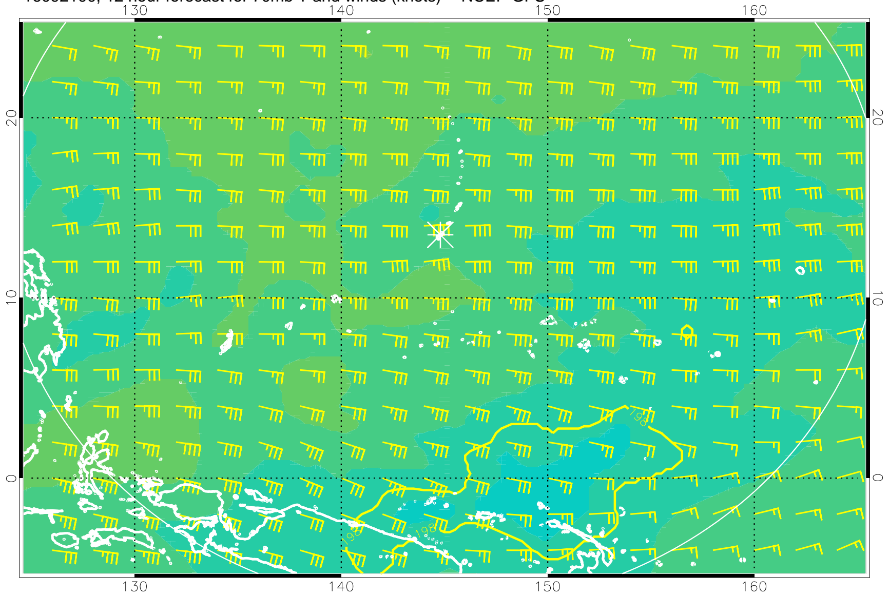
16092100, 12 hour forecast for 70mb T and winds (knots) -- NCEP GFS
