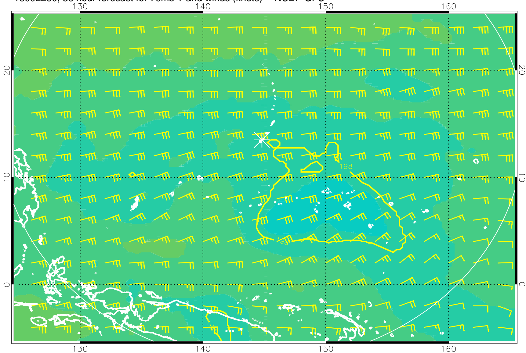
16092200, 36 hour forecast for 70mb T and winds (knots) -- NCEP GFS
