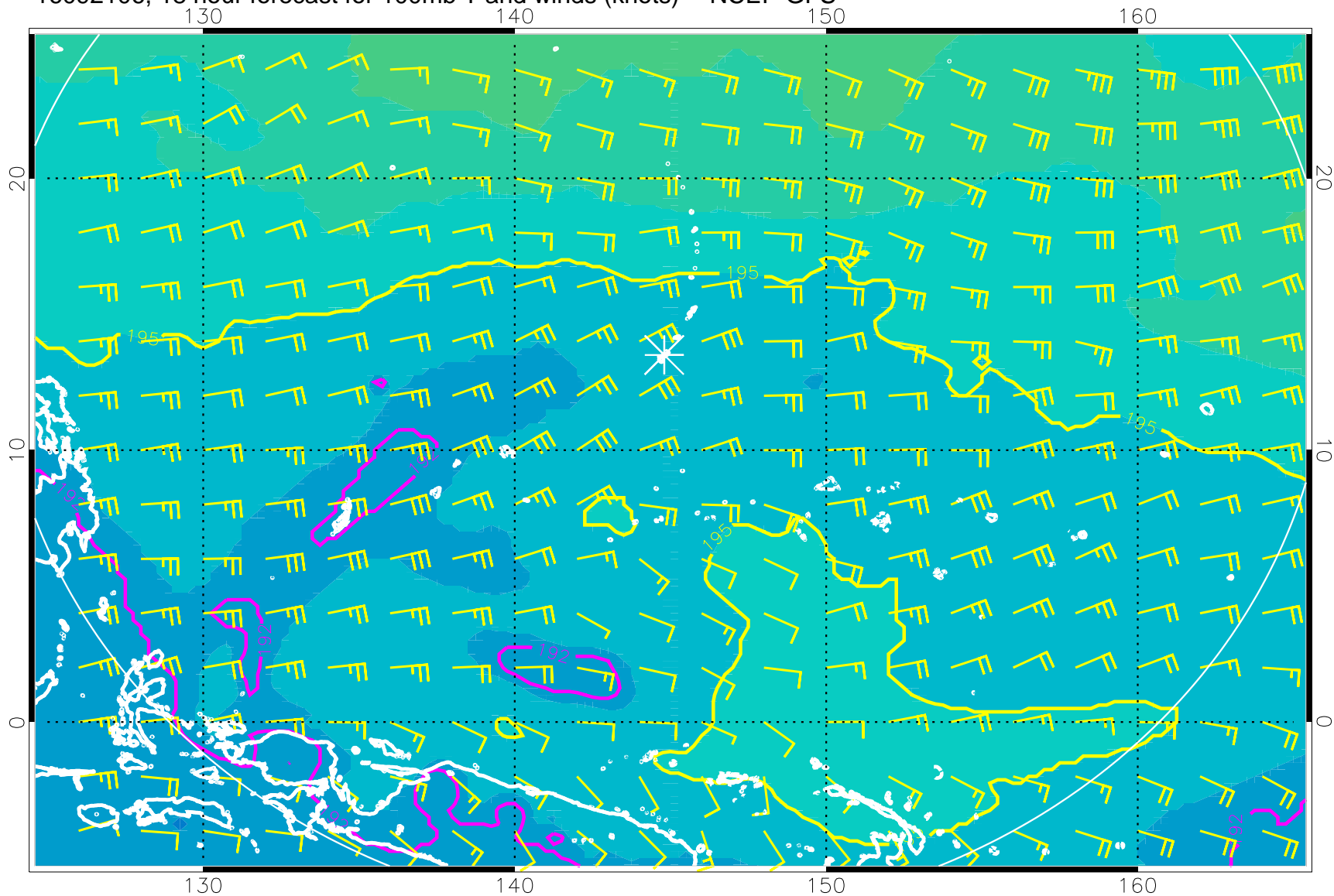
16092106, 18 hour forecast for 100mb T and winds (knots) -- NCEP GFS
