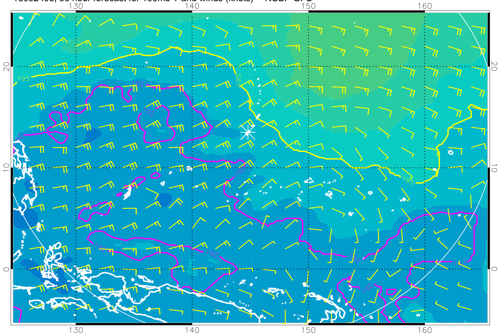
16092406, 90 hour forecast for 100mb T and winds (knots) -- NCEP GFS
