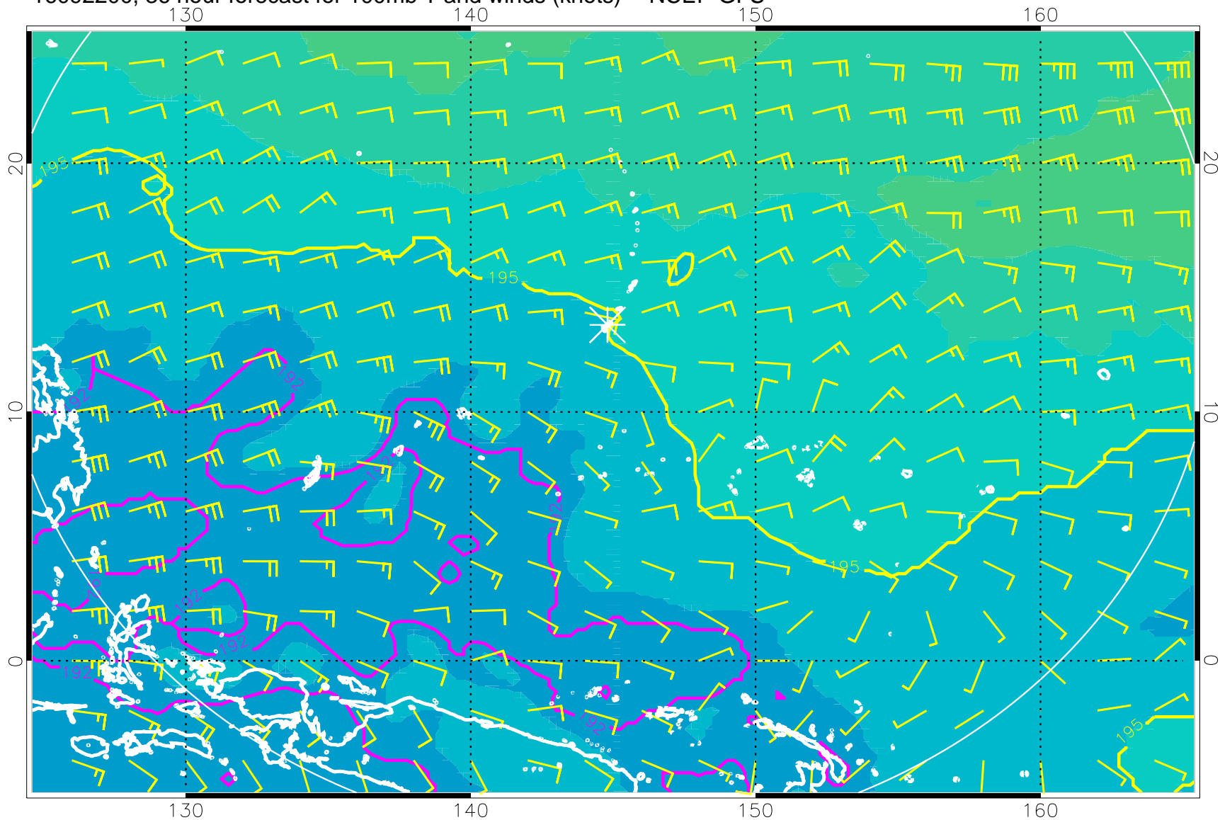
16092200, 36 hour forecast for 100mb T and winds (knots) -- NCEP GFS
