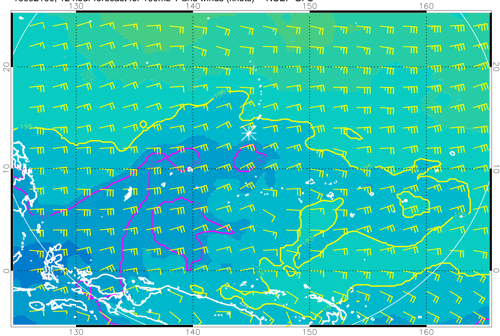
16092100, 12 hour forecast for 100mb T and winds (knots) -- NCEP GFS
