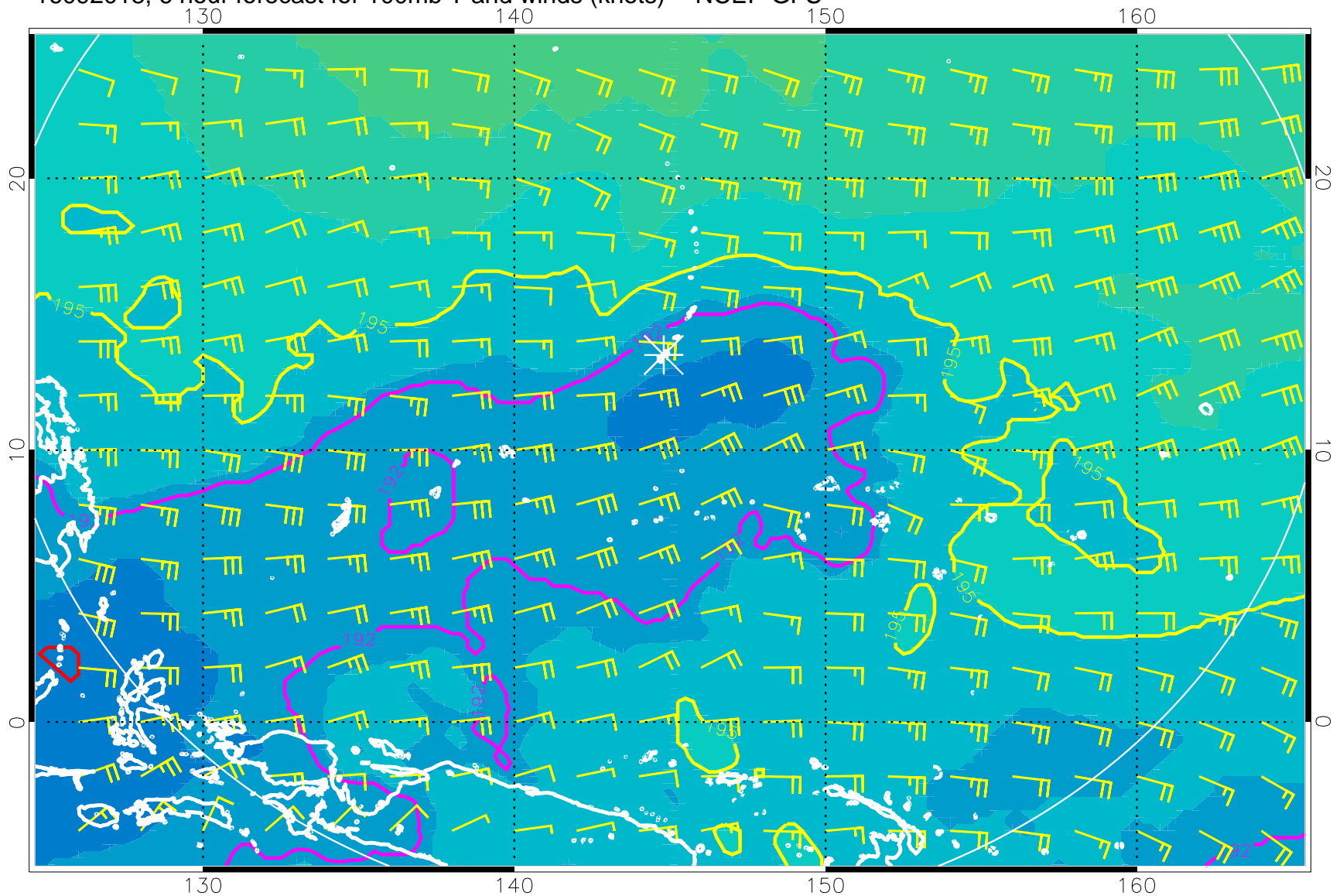
16092018, 6 hour forecast for 100mb T and winds (knots) -- NCEP GFS
