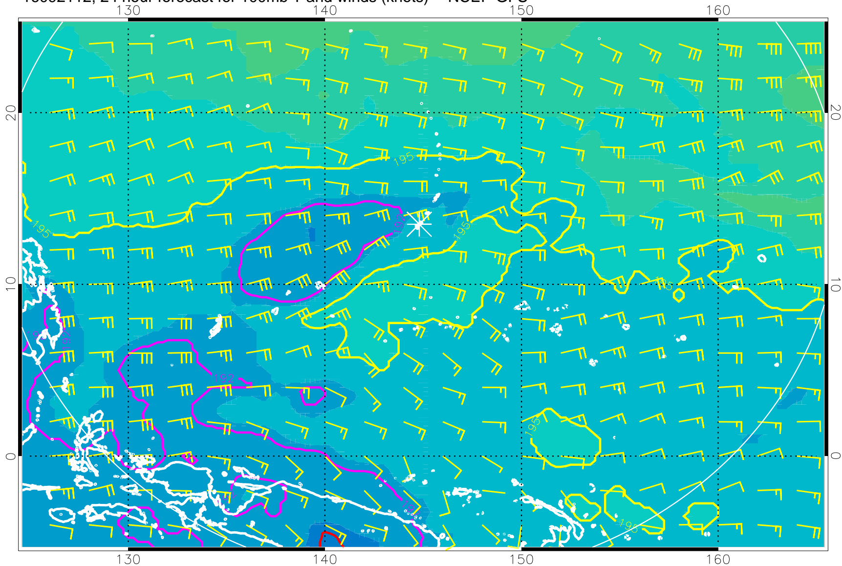
16092112, 24 hour forecast for 100mb T and winds (knots) -- NCEP GFS
