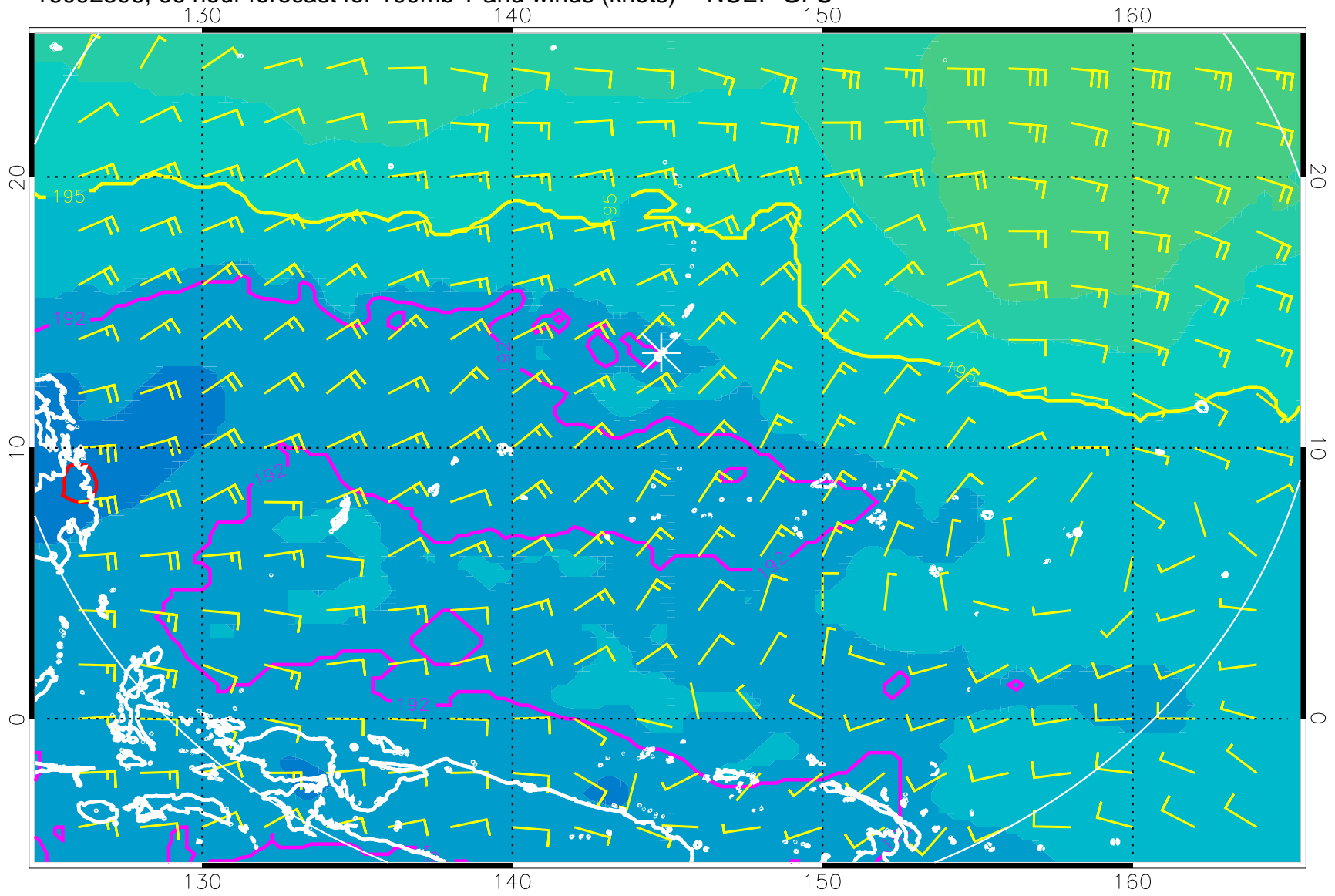
16092306, 66 hour forecast for 100mb T and winds (knots) -- NCEP GFS
