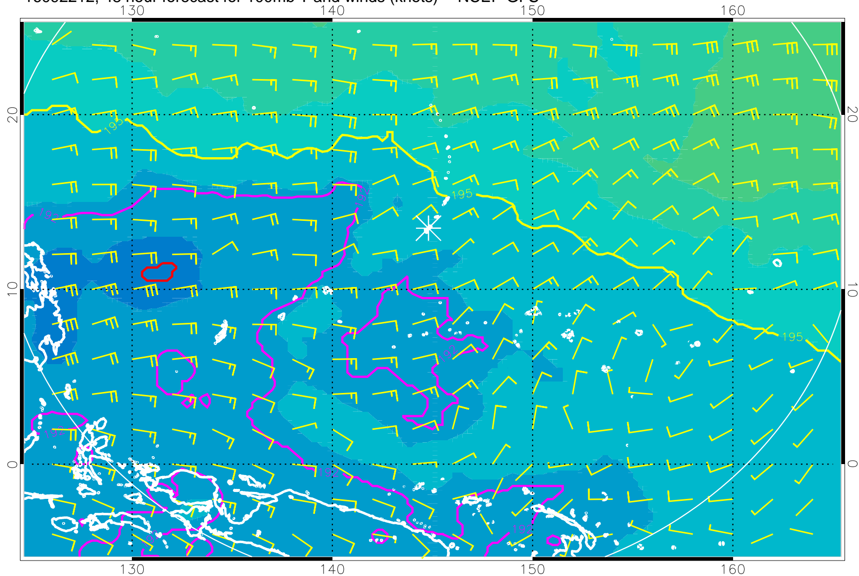
16092212, 48 hour forecast for 100mb T and winds (knots) -- NCEP GFS
