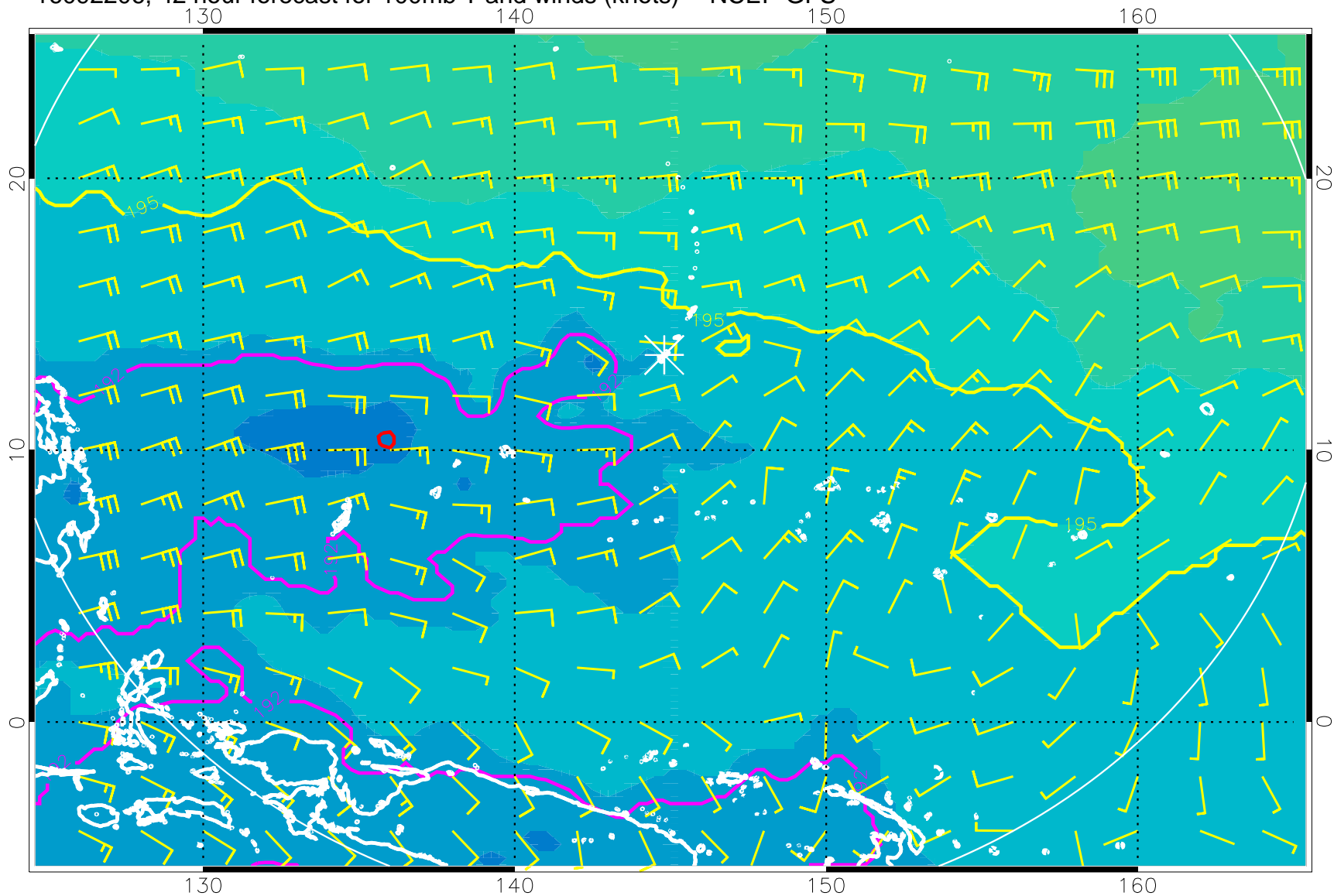
16092206, 42 hour forecast for 100mb T and winds (knots) -- NCEP GFS
