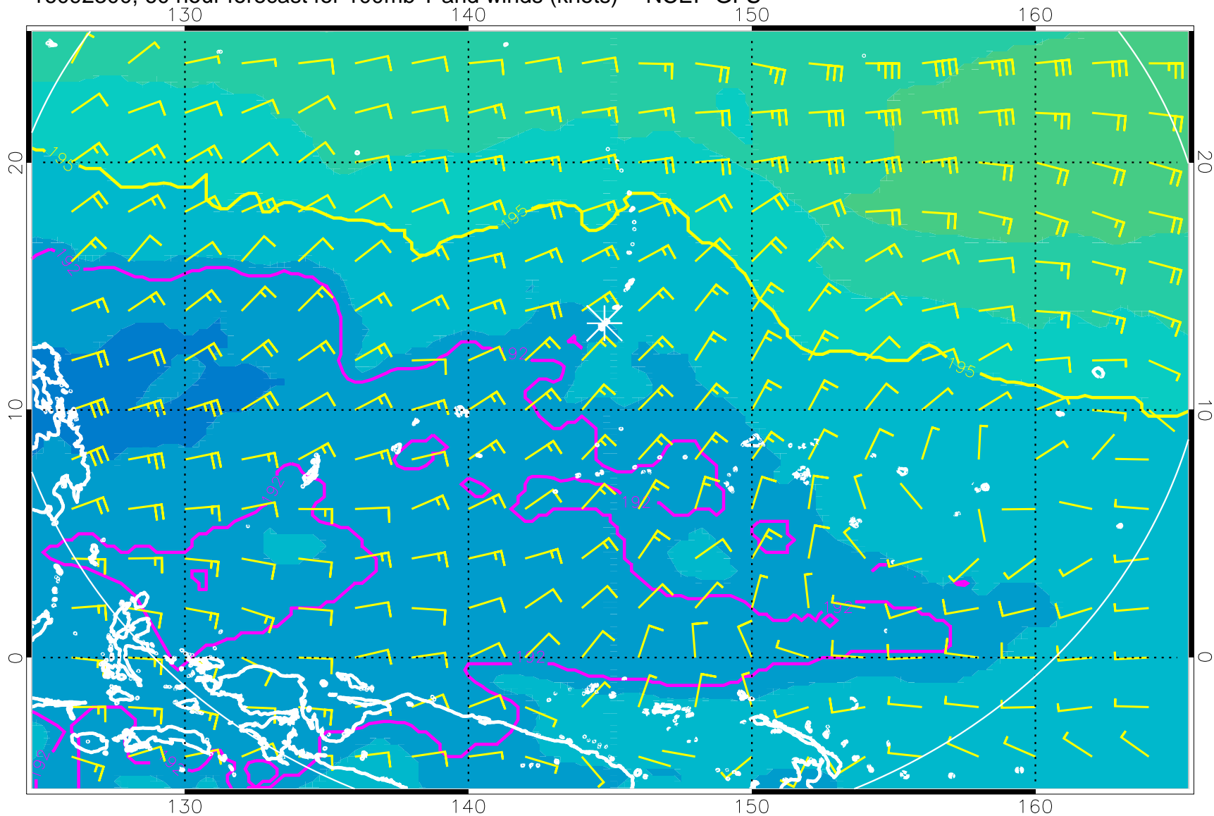
16092300, 60 hour forecast for 100mb T and winds (knots) -- NCEP GFS
