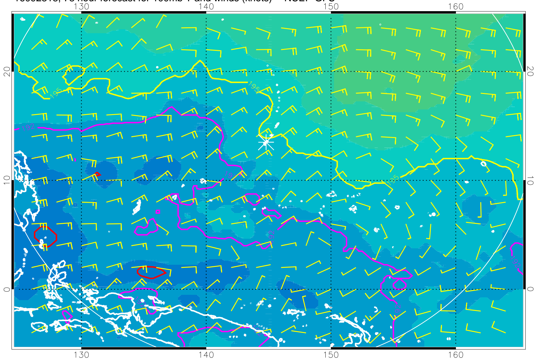
16092318, 78 hour forecast for 100mb T and winds (knots) -- NCEP GFS
