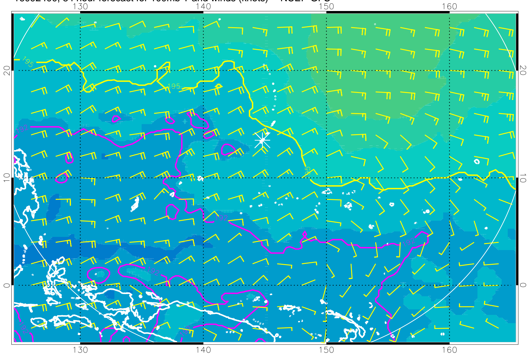
16092400, 84 hour forecast for 100mb T and winds (knots) -- NCEP GFS
