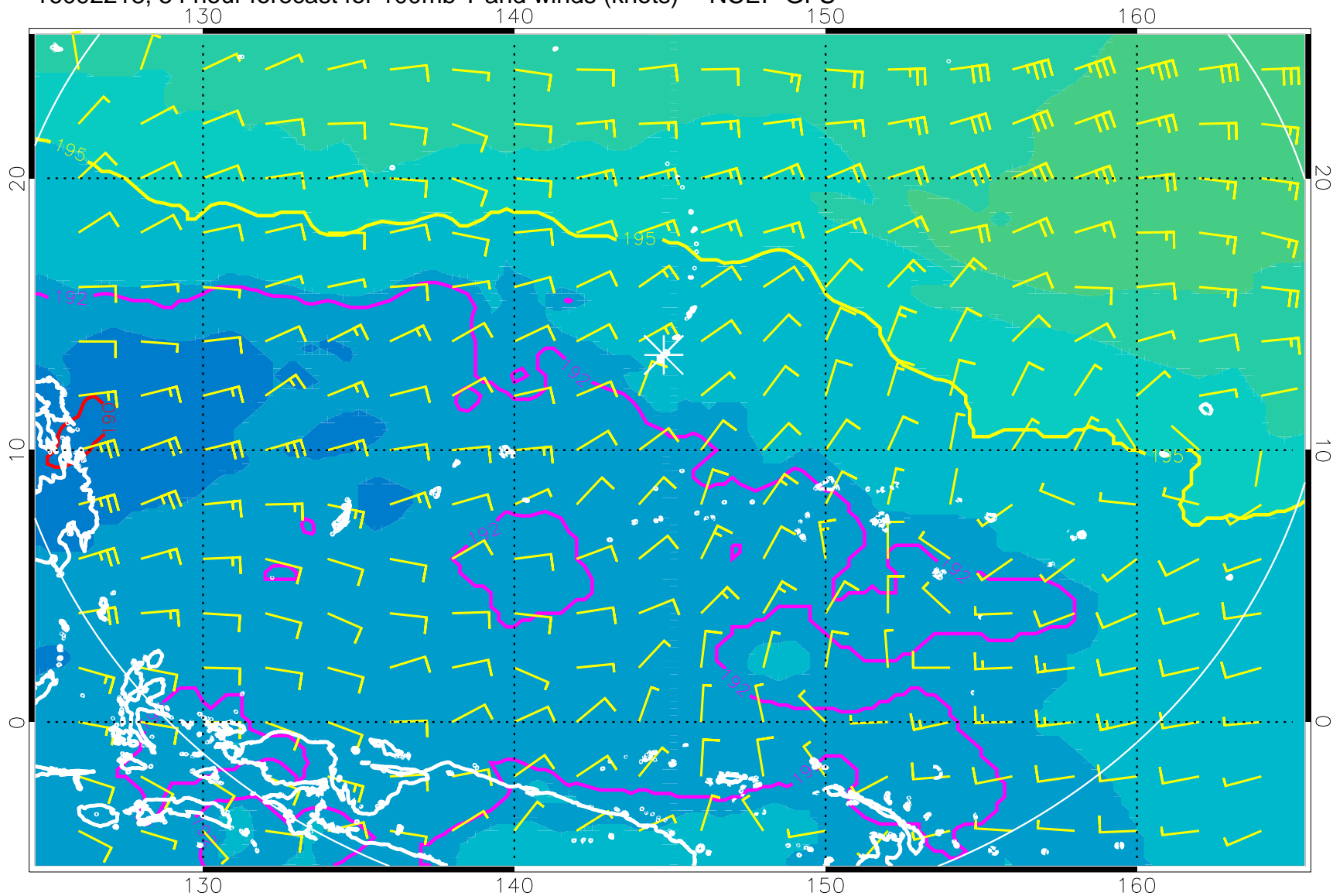
16092218, 54 hour forecast for 100mb T and winds (knots) -- NCEP GFS
