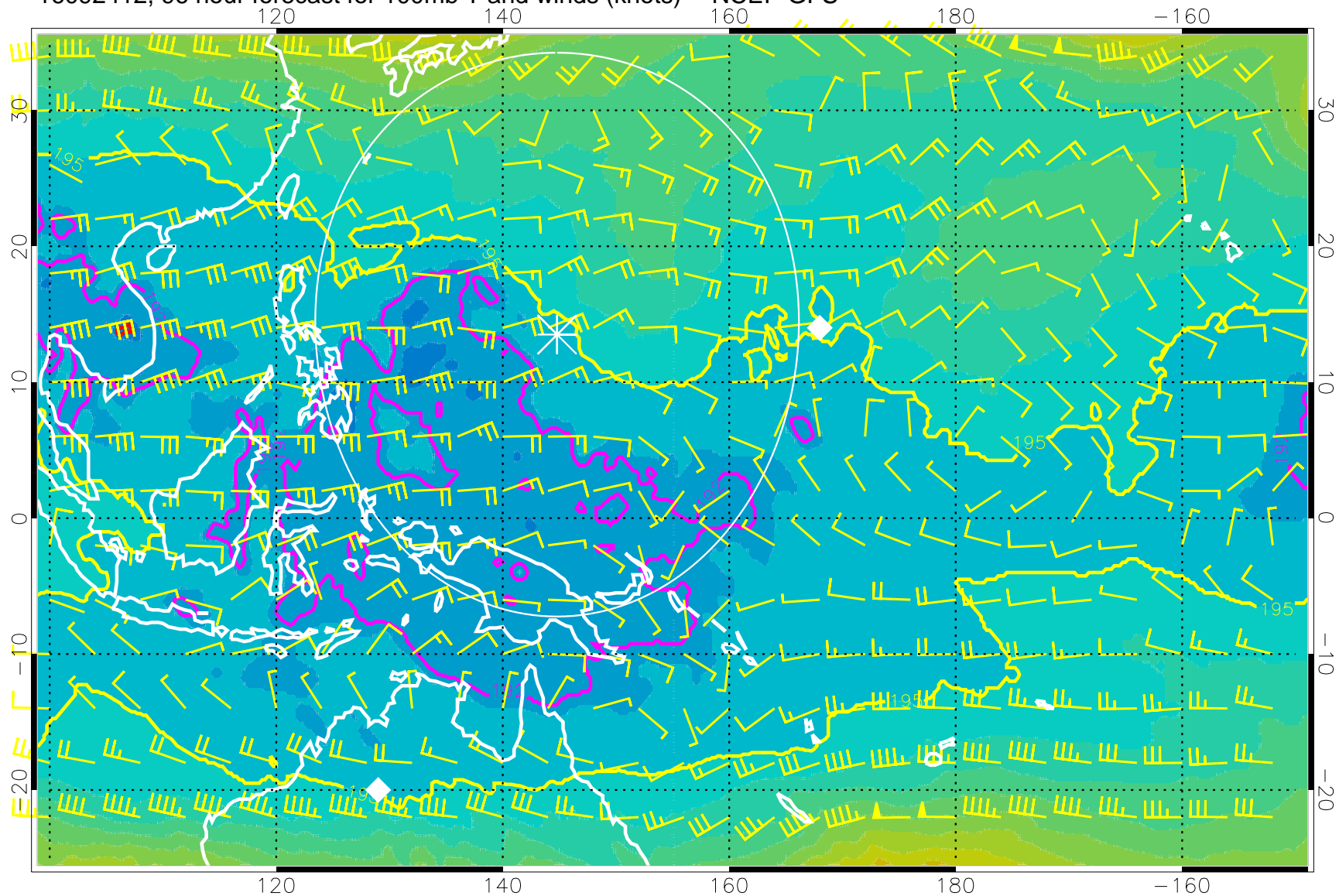
16092412, 96 hour forecast for 100mb T and winds (knots) -- NCEP GFS
