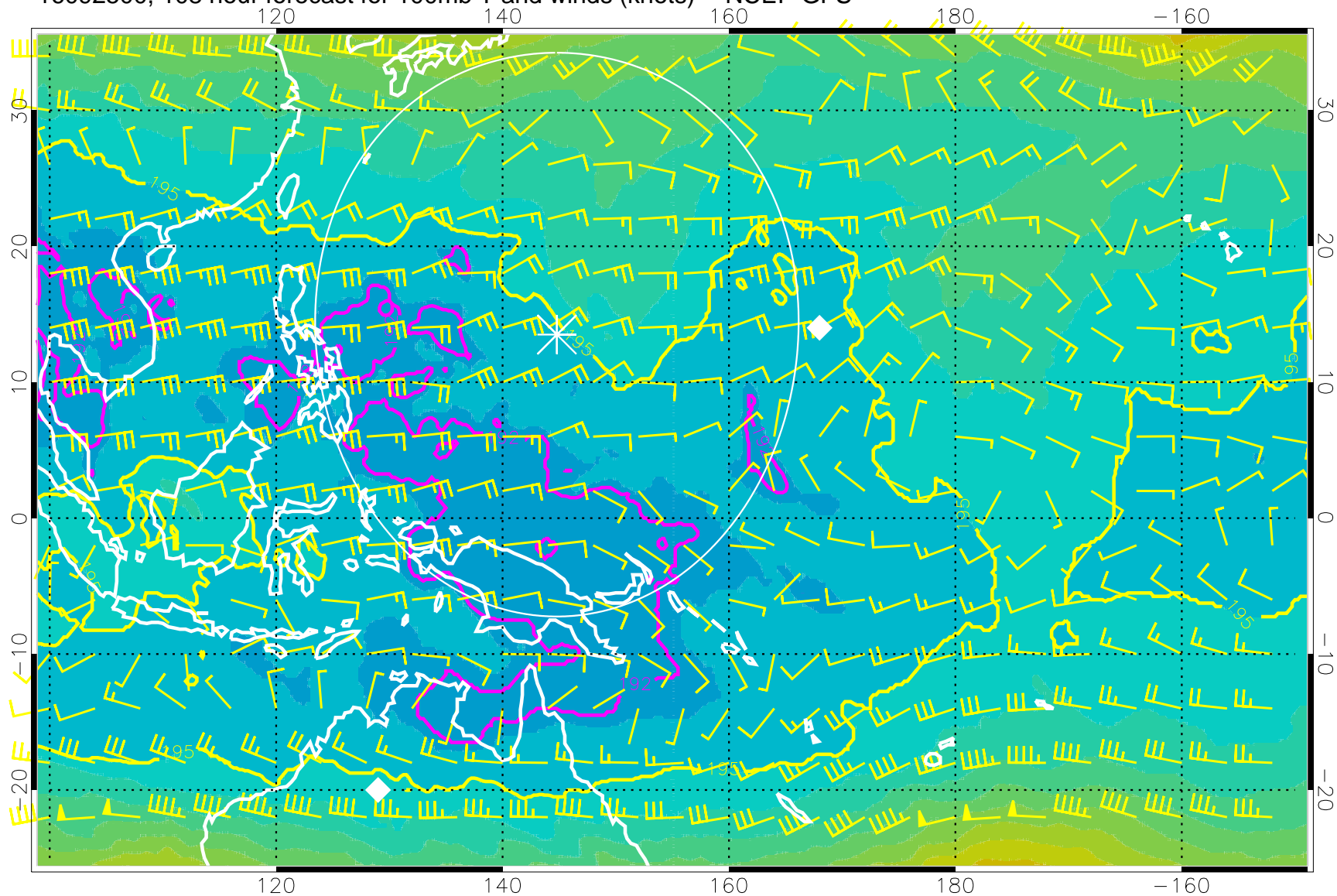
16092500, 108 hour forecast for 100mb T and winds (knots) -- NCEP GFS
