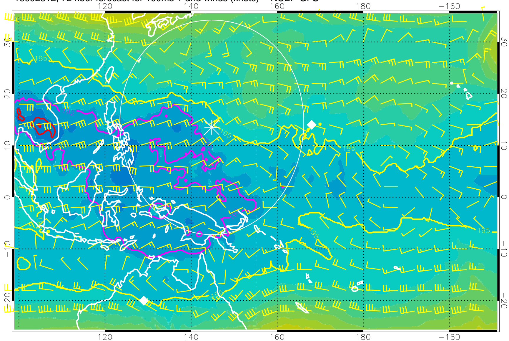
16092312, 72 hour forecast for 100mb T and winds (knots) -- NCEP GFS
