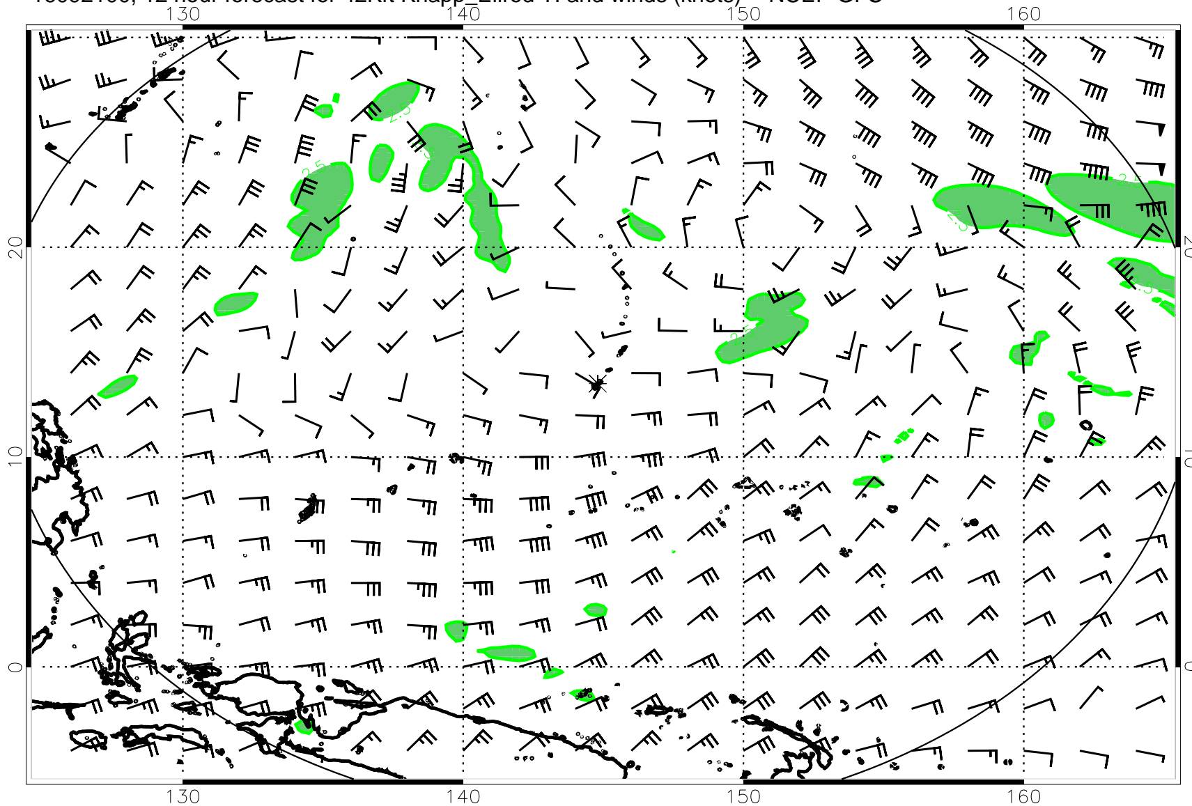
16092100, 12 hour forecast for 42Kft Knapp_Ellrod TI and winds (knots) -- NCEP GFS
