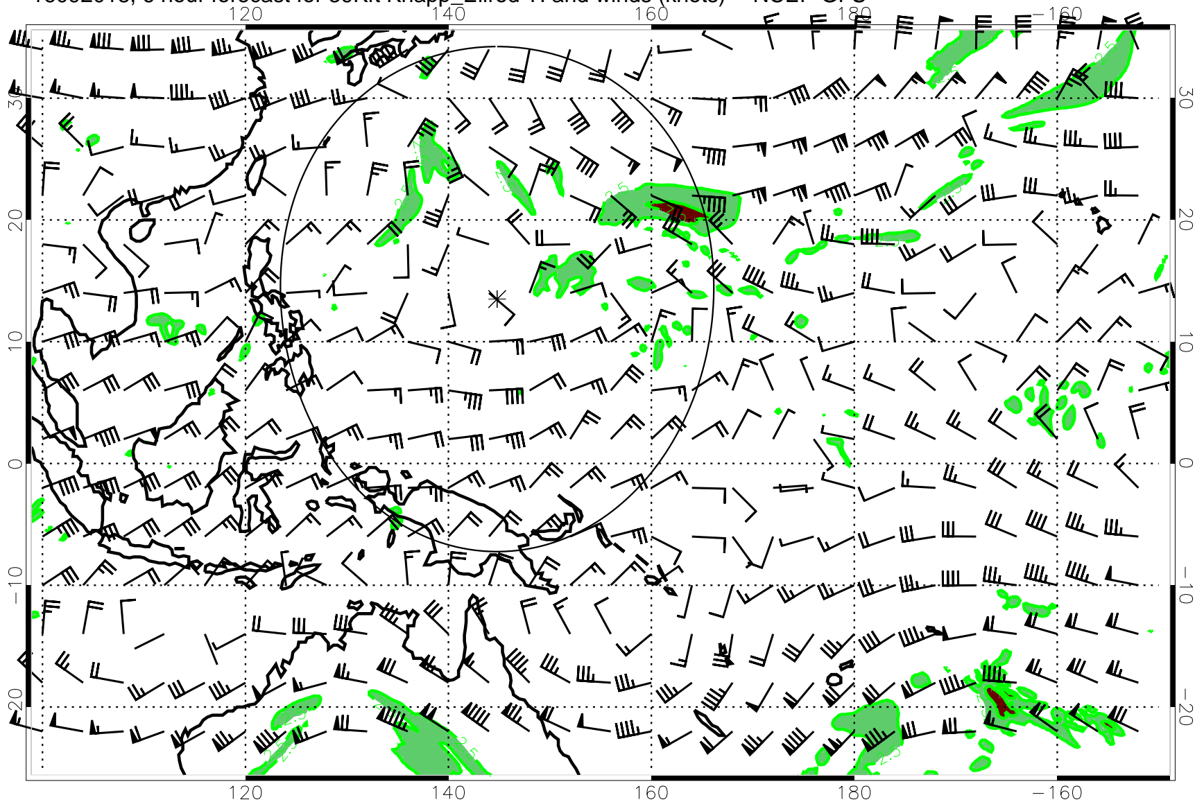
16092018, 6 hour forecast for 39Kft Knapp_Ellrod TI and winds (knots) -- NCEP GFS
