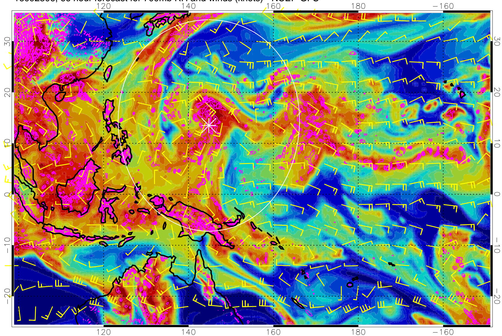
16092306, 66 hour forecast for 700mb RH and winds (knots) - NCEP GFS
