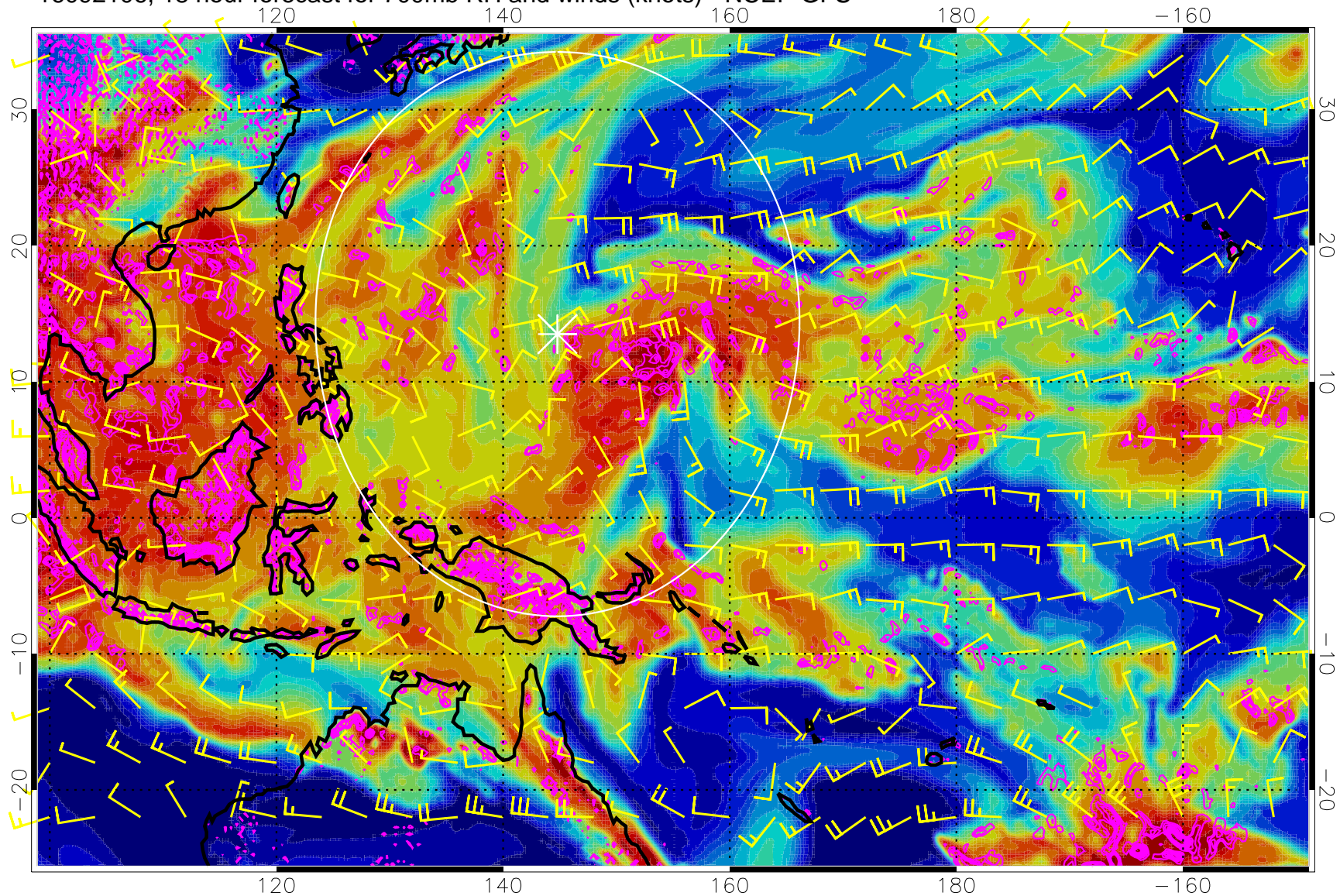
16092106, 18 hour forecast for 700mb RH and winds (knots) - NCEP GFS
