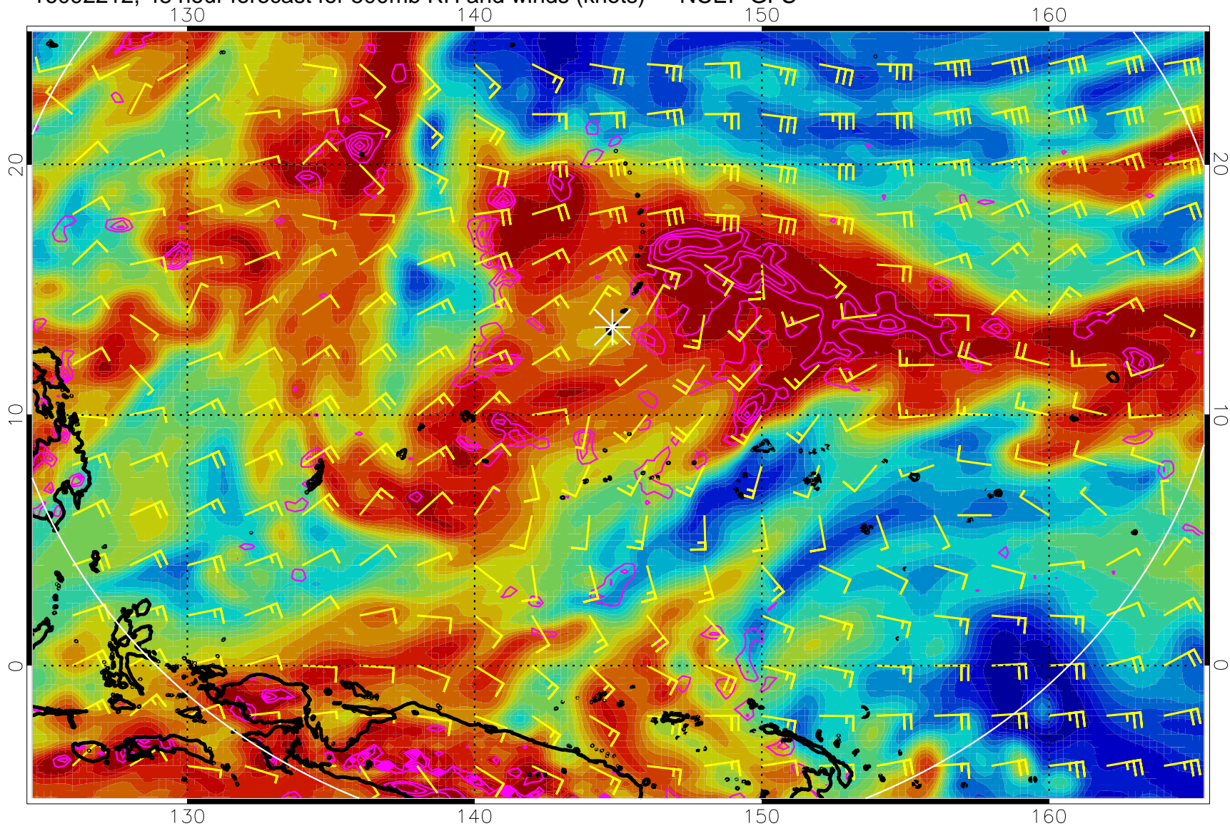
16092212, 48 hour forecast for 500mb RH and winds (knots) -- NCEP GFS
